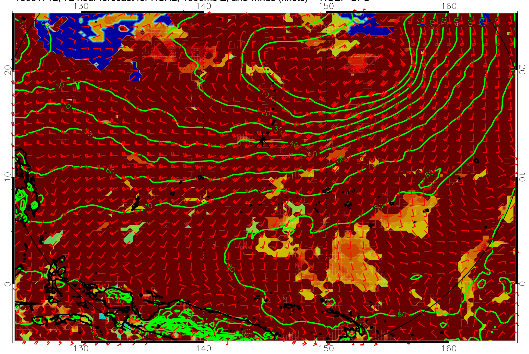
16081712, 72 hour forecast for HCAL, 1000mb Z, and winds (knots) -- NCEP GFS
