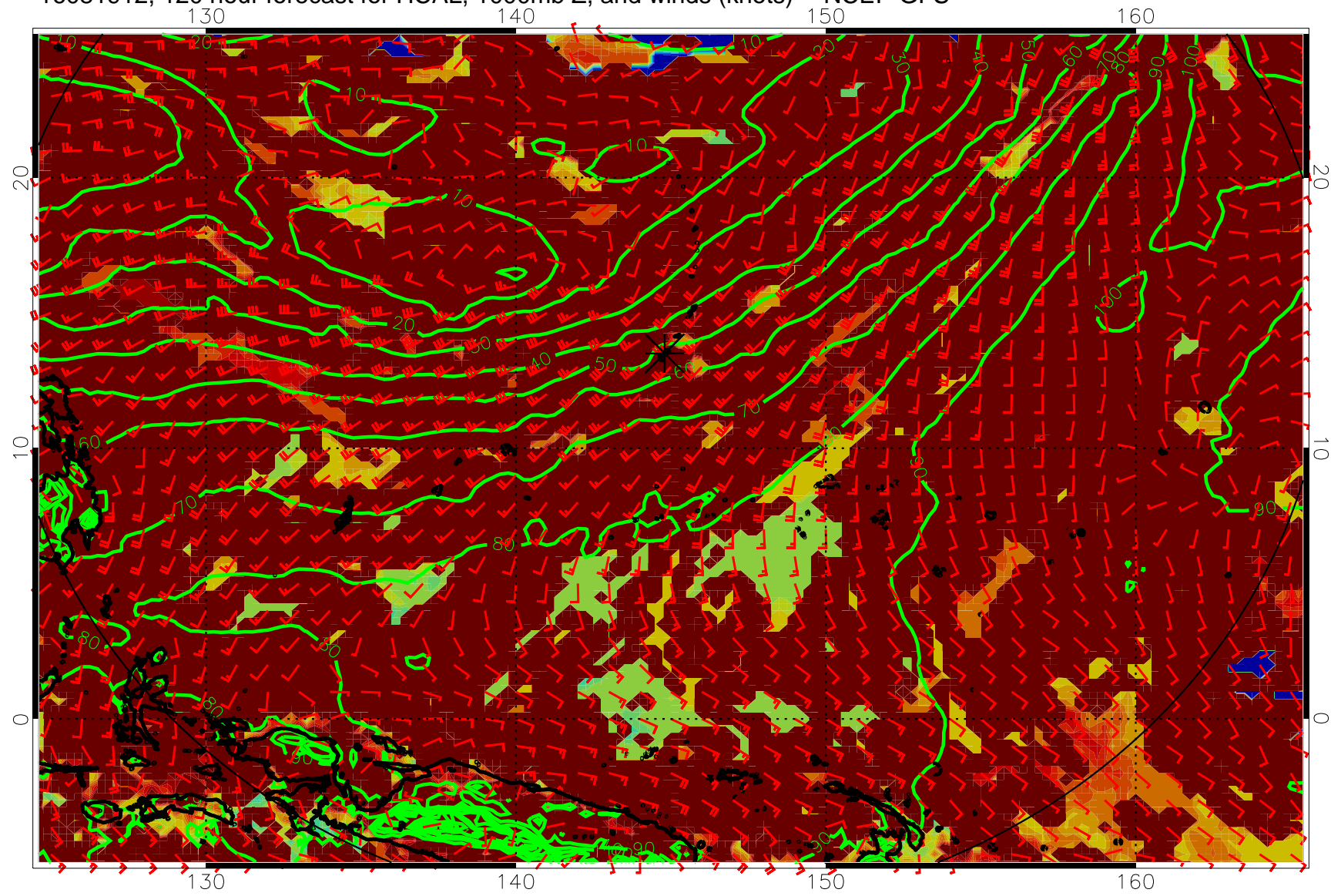
16081912, 120 hour forecast for HCAL, 1000mb Z, and winds (knots) -- NCEP GFS
