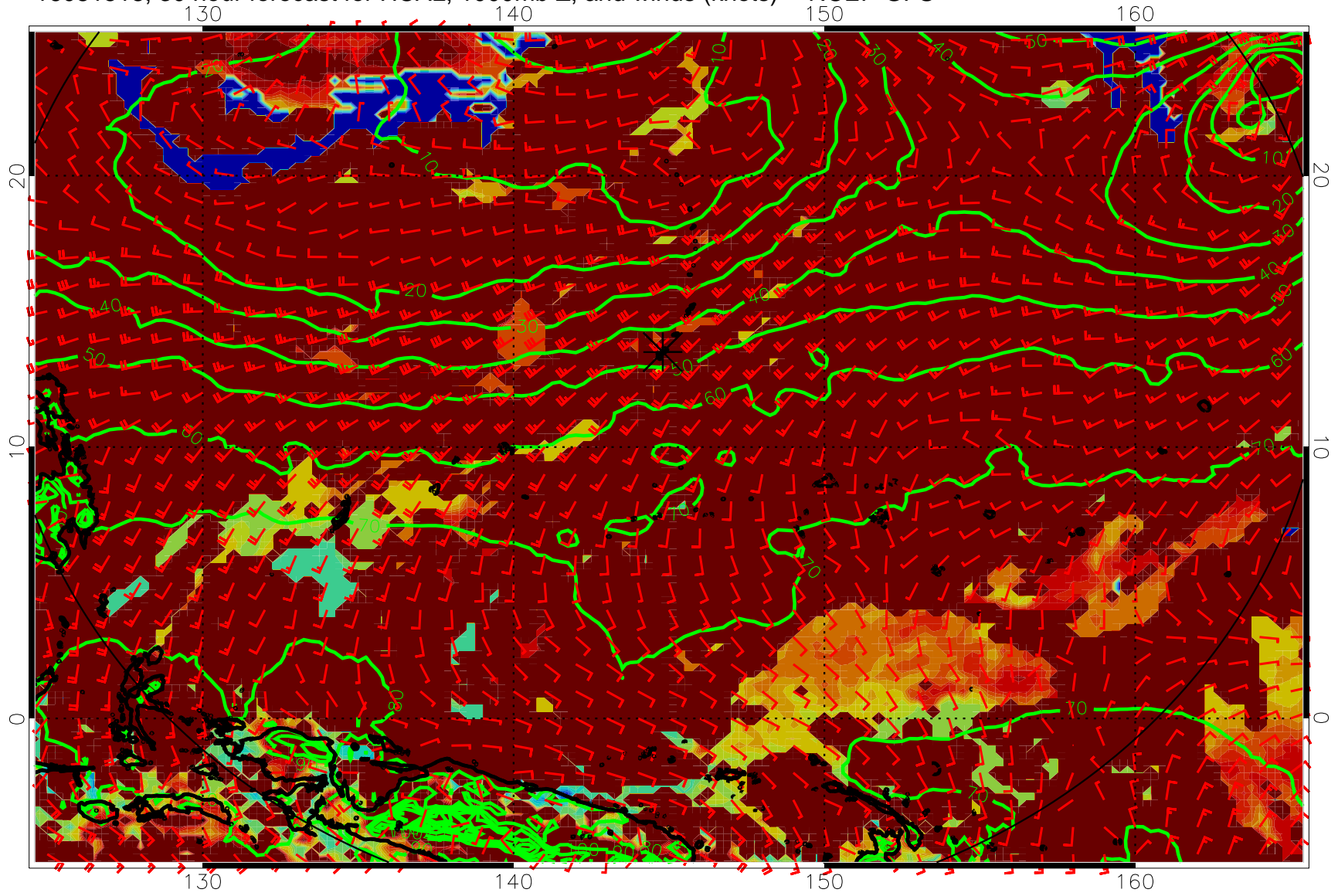
16081518, 30 hour forecast for HCAL, 1000mb Z, and winds (knots) -- NCEP GFS
