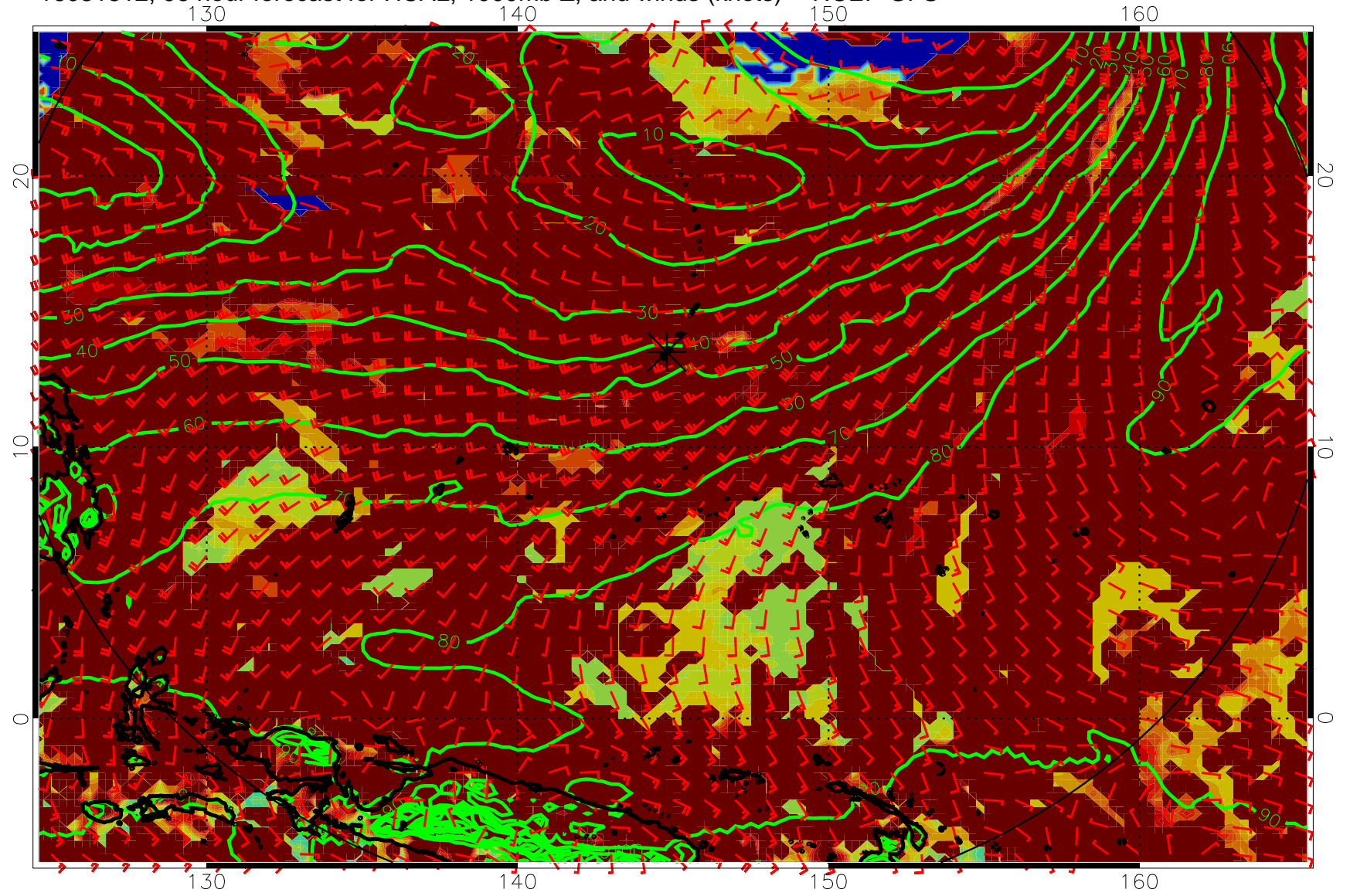
16081812, 96 hour forecast for HCAL, 1000mb Z, and winds (knots) -- NCEP GFS
