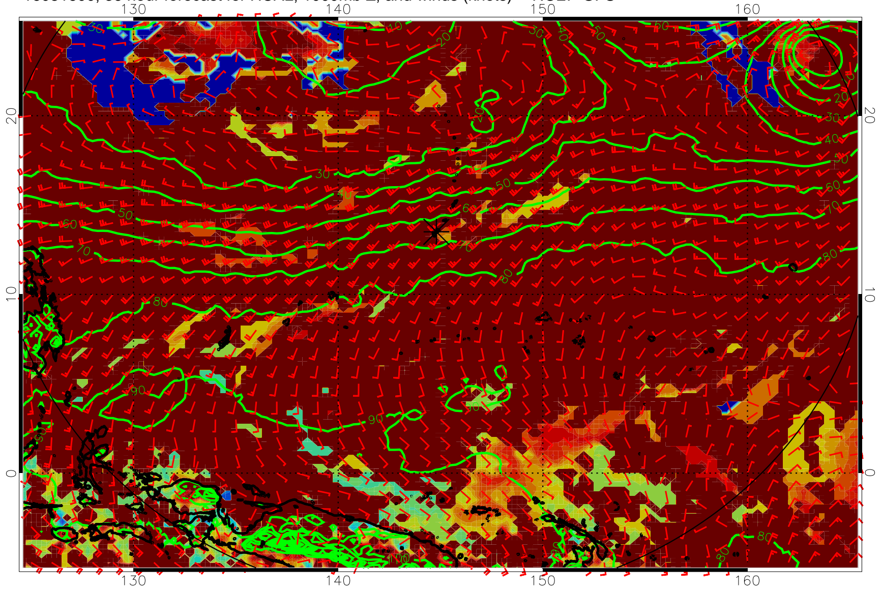
16081600, 36 hour forecast for HCAL, 1000mb Z, and winds (knots) -- NCEP GFS
