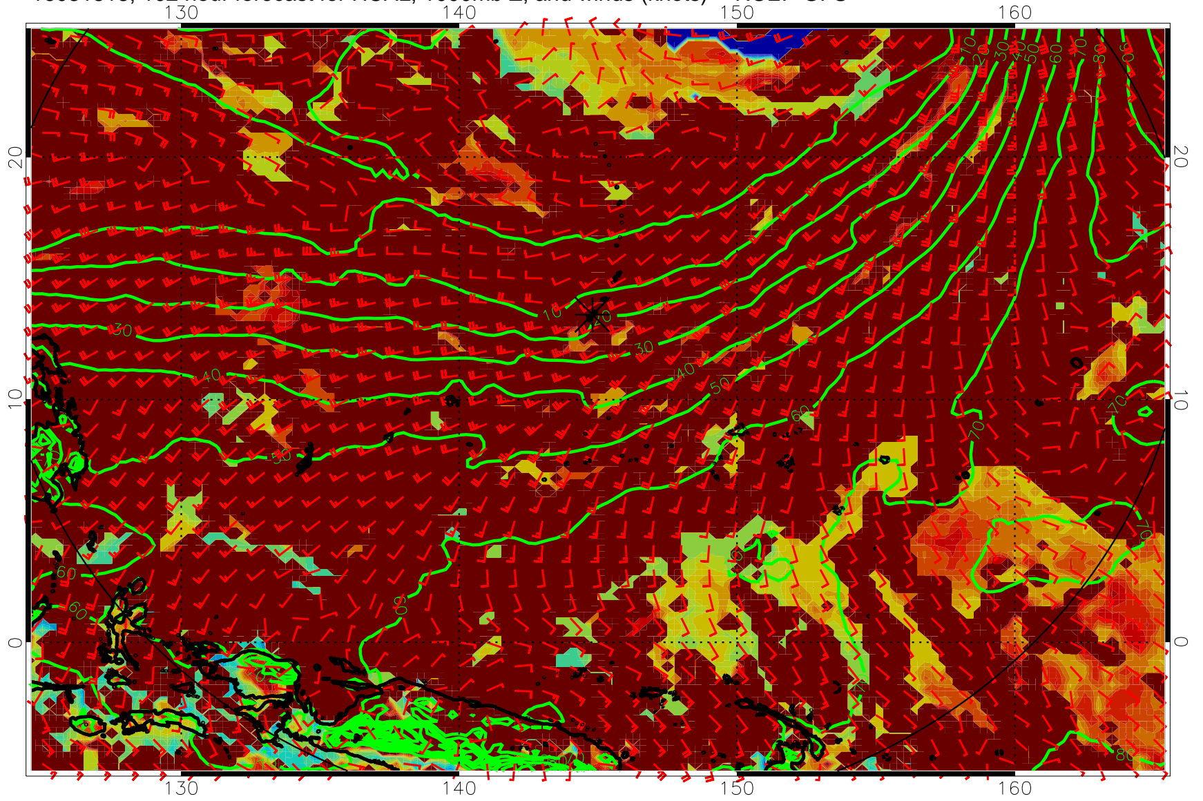
16081818, 102 hour forecast for HCAL, 1000mb Z, and winds (knots) -- NCEP GFS
