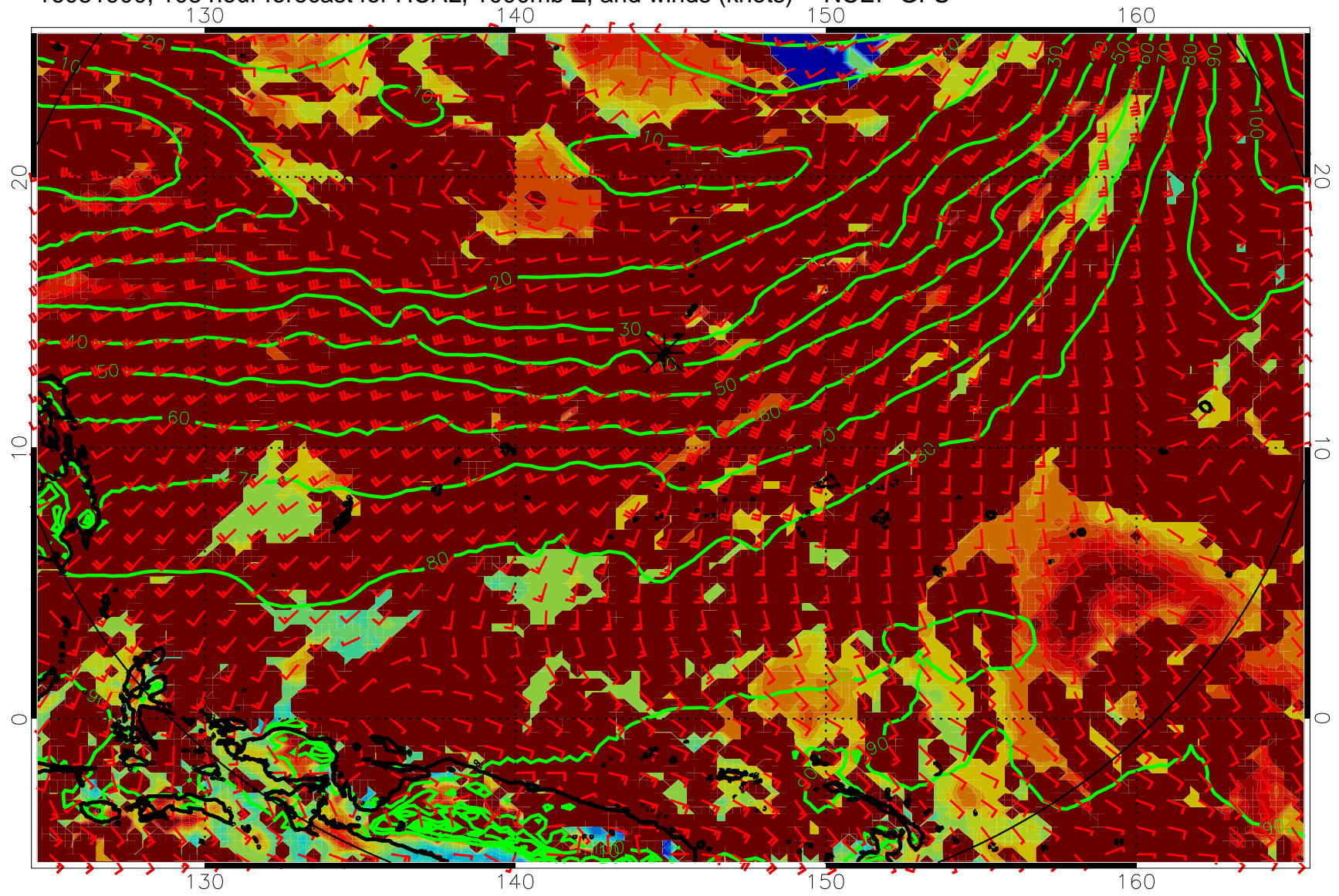
16081900, 108 hour forecast for HCAL, 1000mb Z, and winds (knots) -- NCEP GFS
