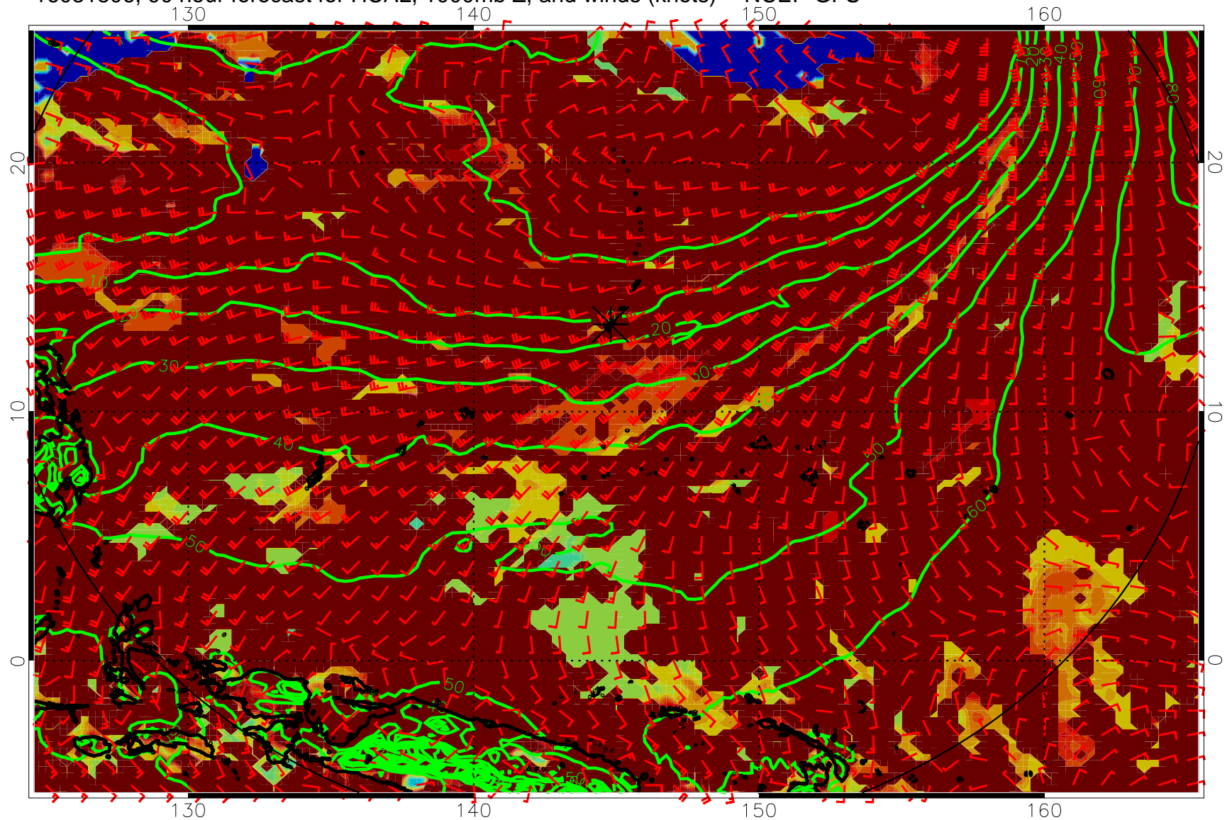
16081806, 90 hour forecast for HCAL, 1000mb Z, and winds (knots) -- NCEP GFS
