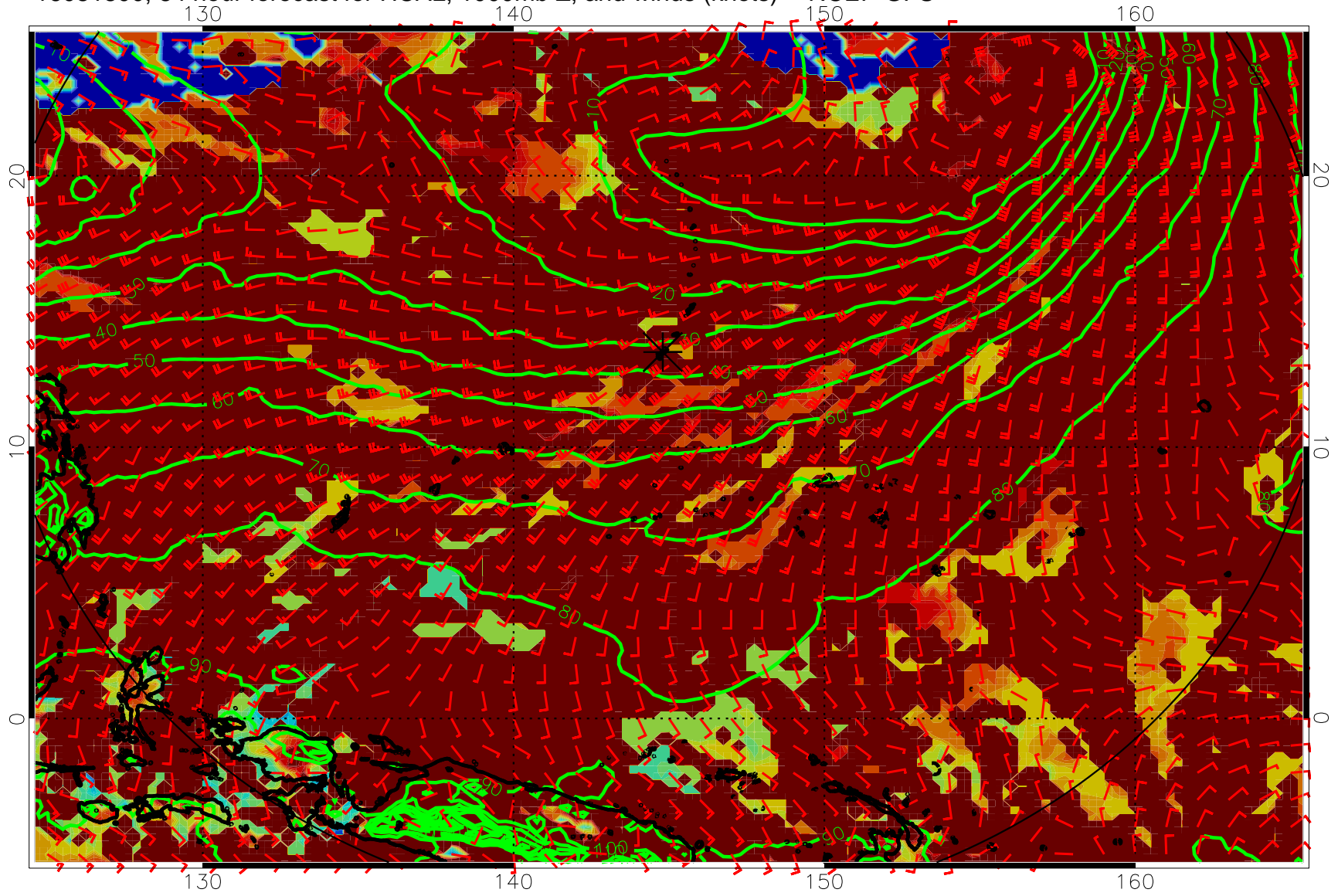
16081800, 84 hour forecast for HCAL, 1000mb Z, and winds (knots) -- NCEP GFS
