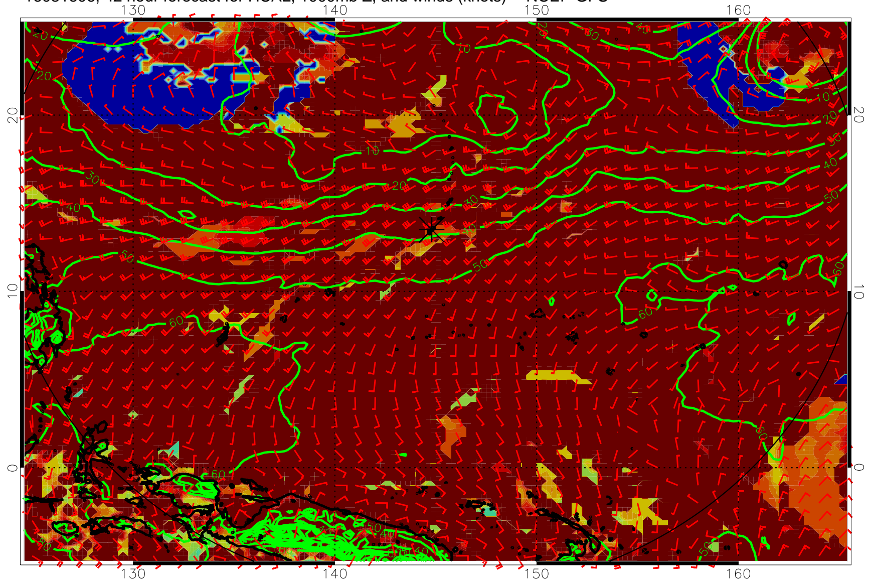
16081606, 42 hour forecast for HCAL, 1000mb Z, and winds (knots) -- NCEP GFS
