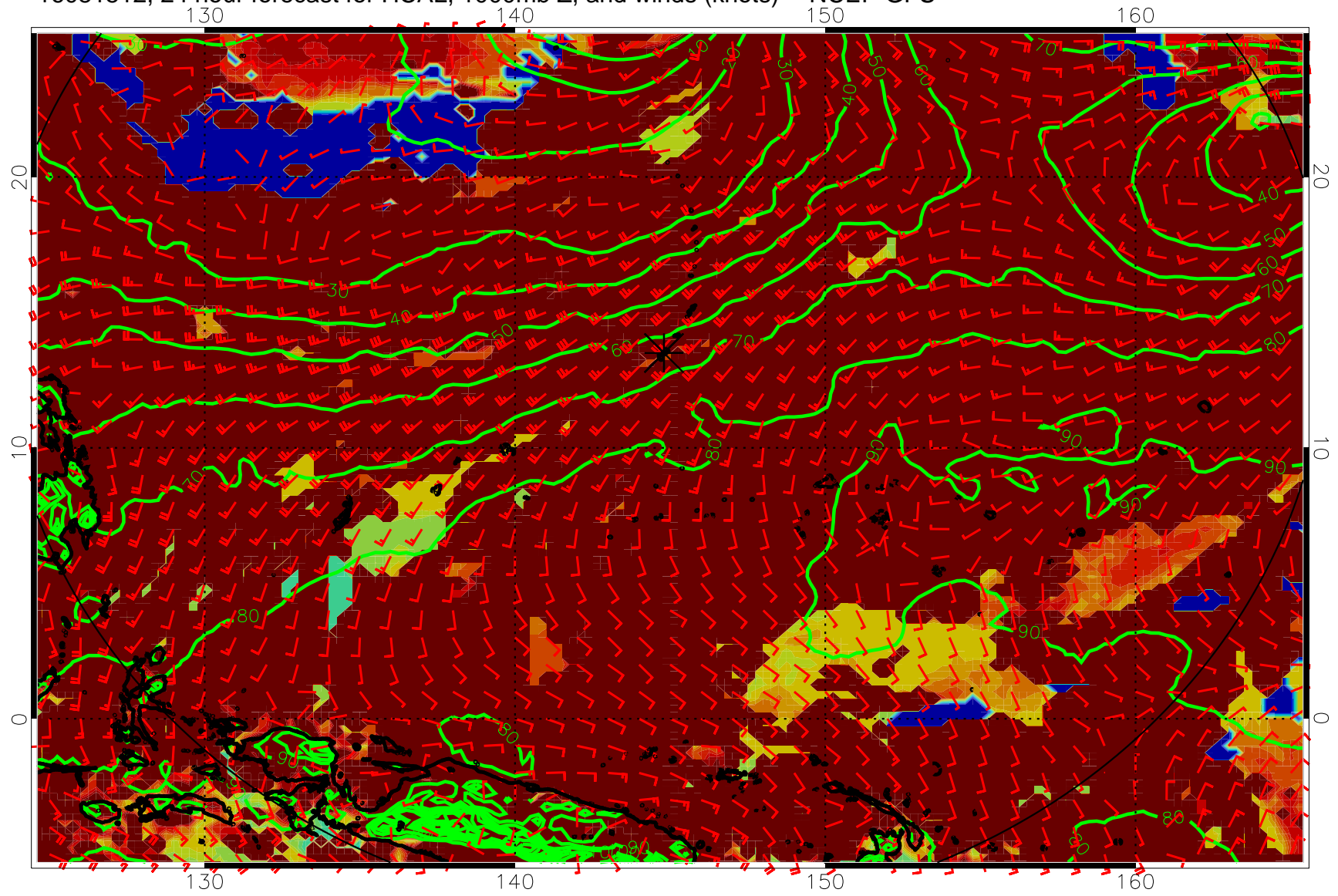
16081512, 24 hour forecast for HCAL, 1000mb Z, and winds (knots) -- NCEP GFS
