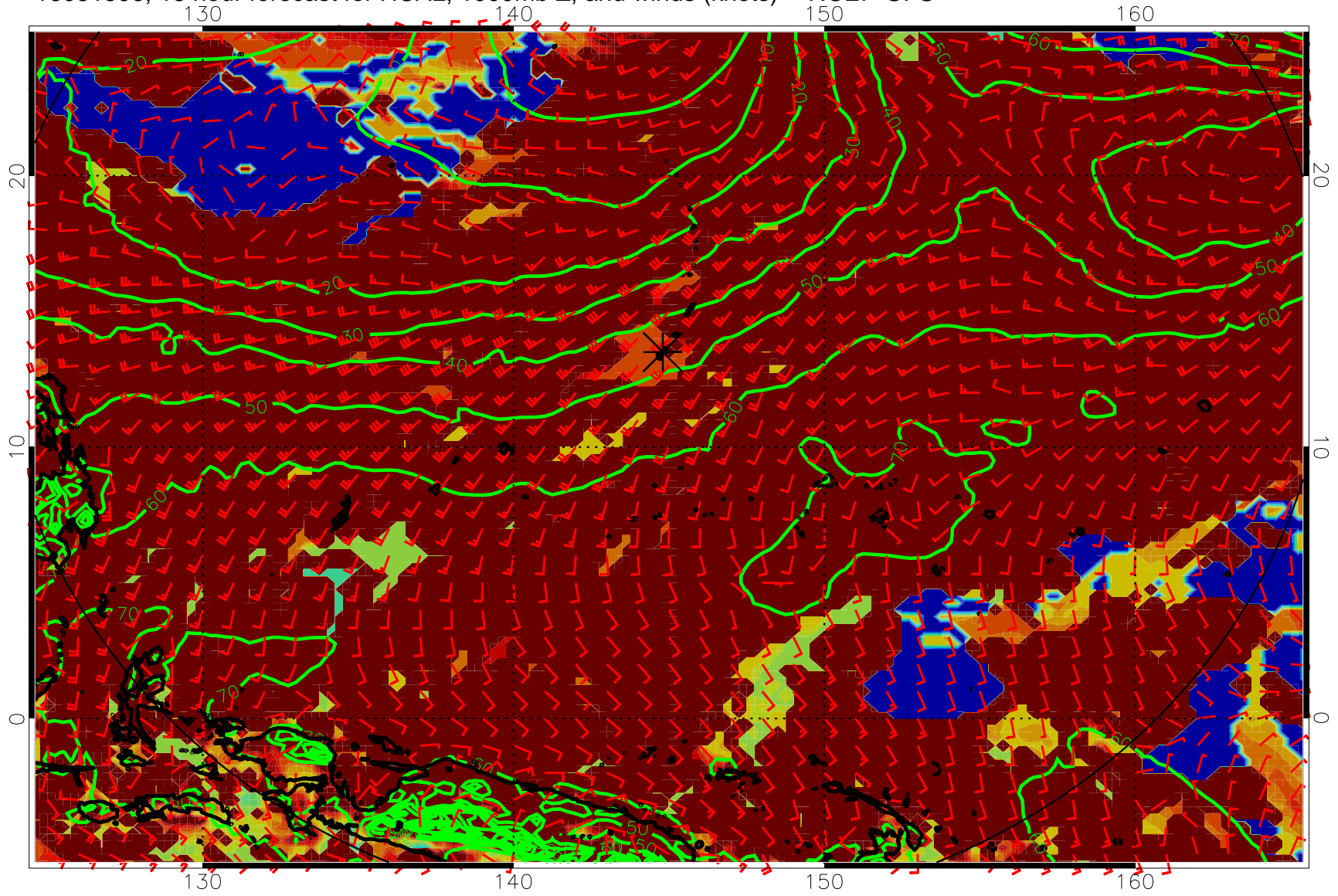
16081506, 18 hour forecast for HCAL, 1000mb Z, and winds (knots) -- NCEP GFS
