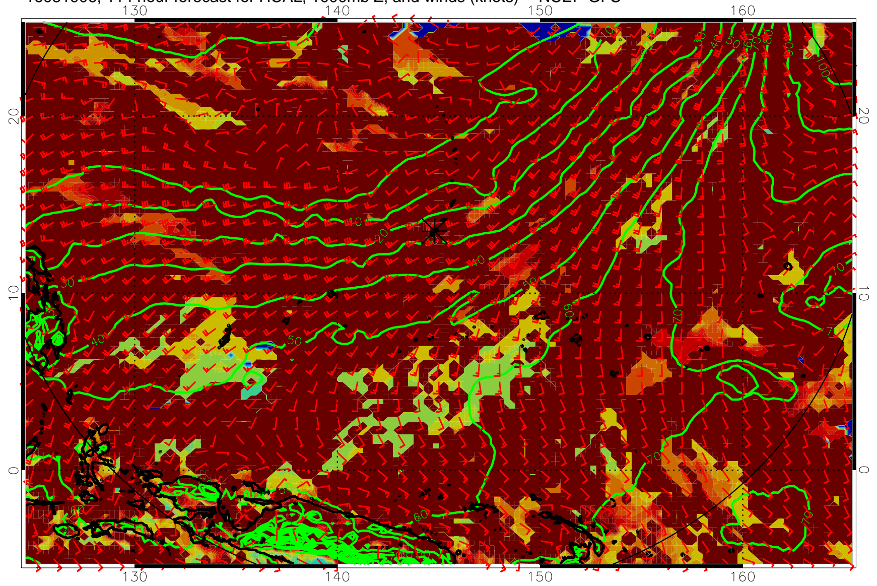
16081906, 114 hour forecast for HCAL, 1000mb Z, and winds (knots) -- NCEP GFS
