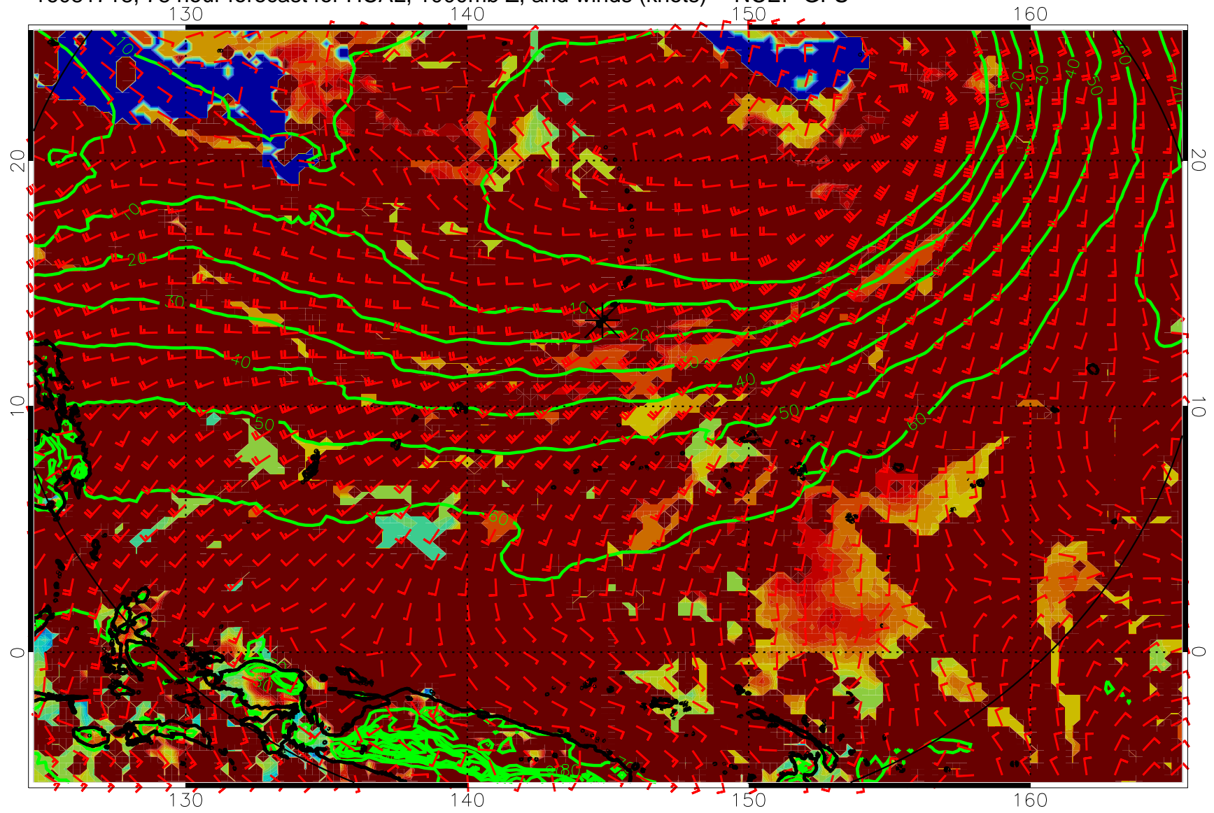
16081718, 78 hour forecast for HCAL, 1000mb Z, and winds (knots) -- NCEP GFS
