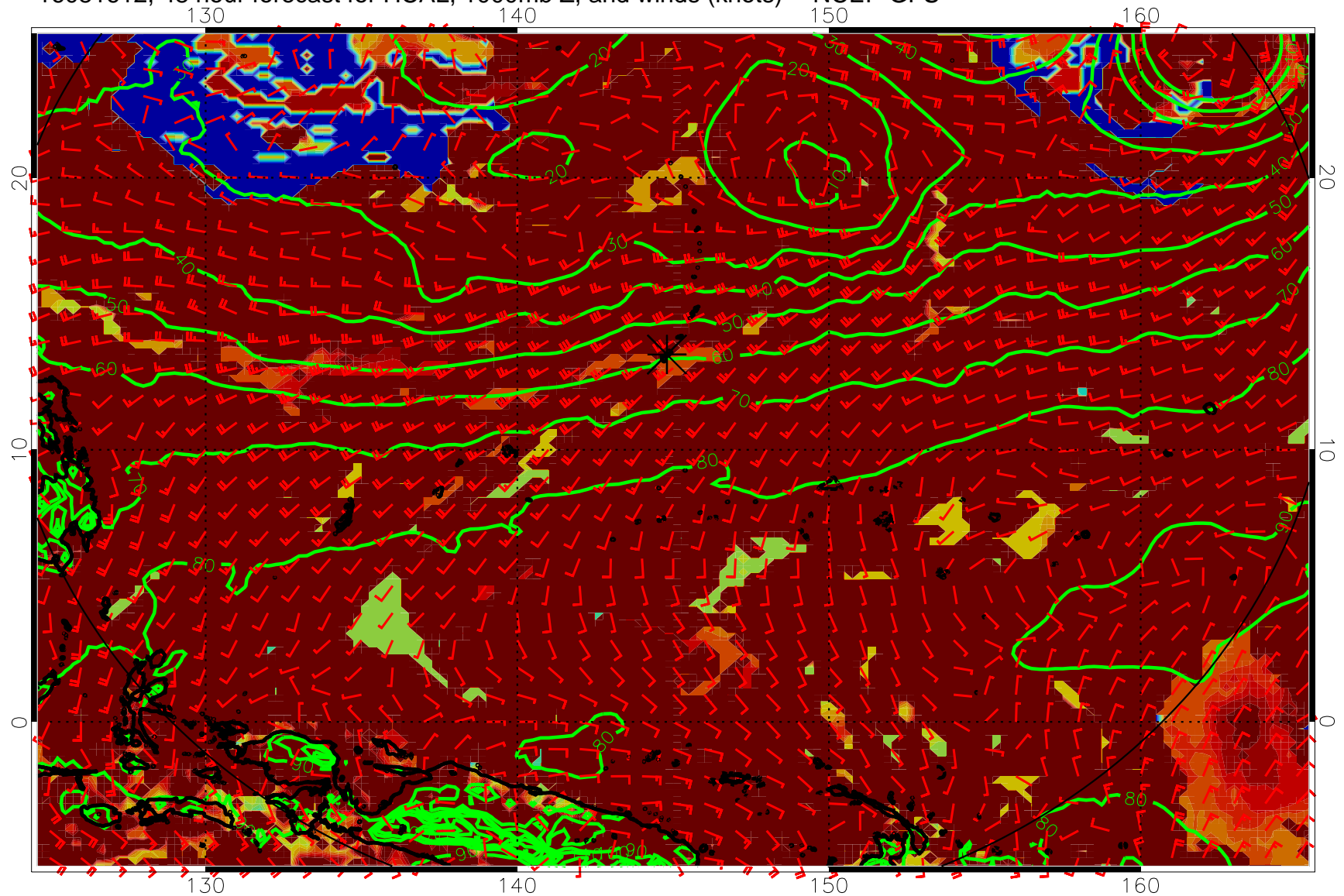
16081612, 48 hour forecast for HCAL, 1000mb Z, and winds (knots) -- NCEP GFS
