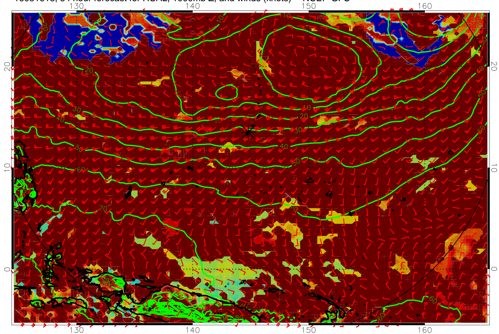
16081618, 54 hour forecast for HCAL, 1000mb Z, and winds (knots) -- NCEP GFS
