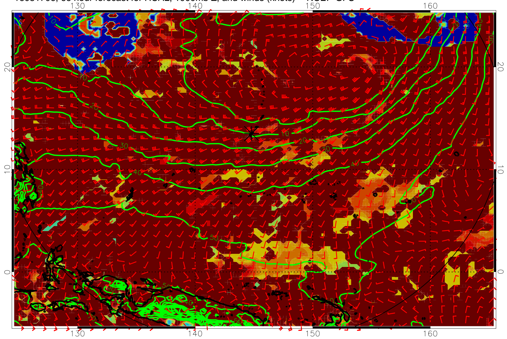
16081706, 66 hour forecast for HCAL, 1000mb Z, and winds (knots) -- NCEP GFS
