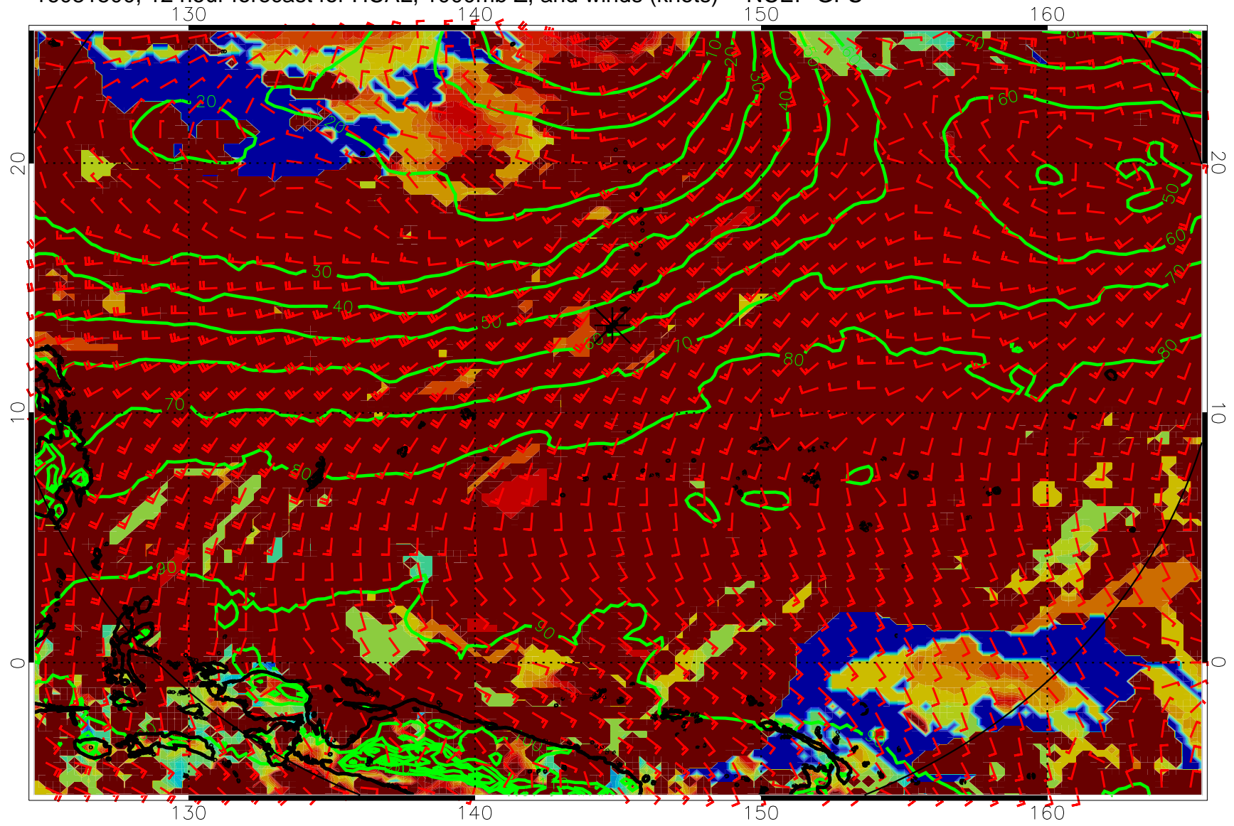
16081500, 12 hour forecast for HCAL, 1000mb Z, and winds (knots) -- NCEP GFS
