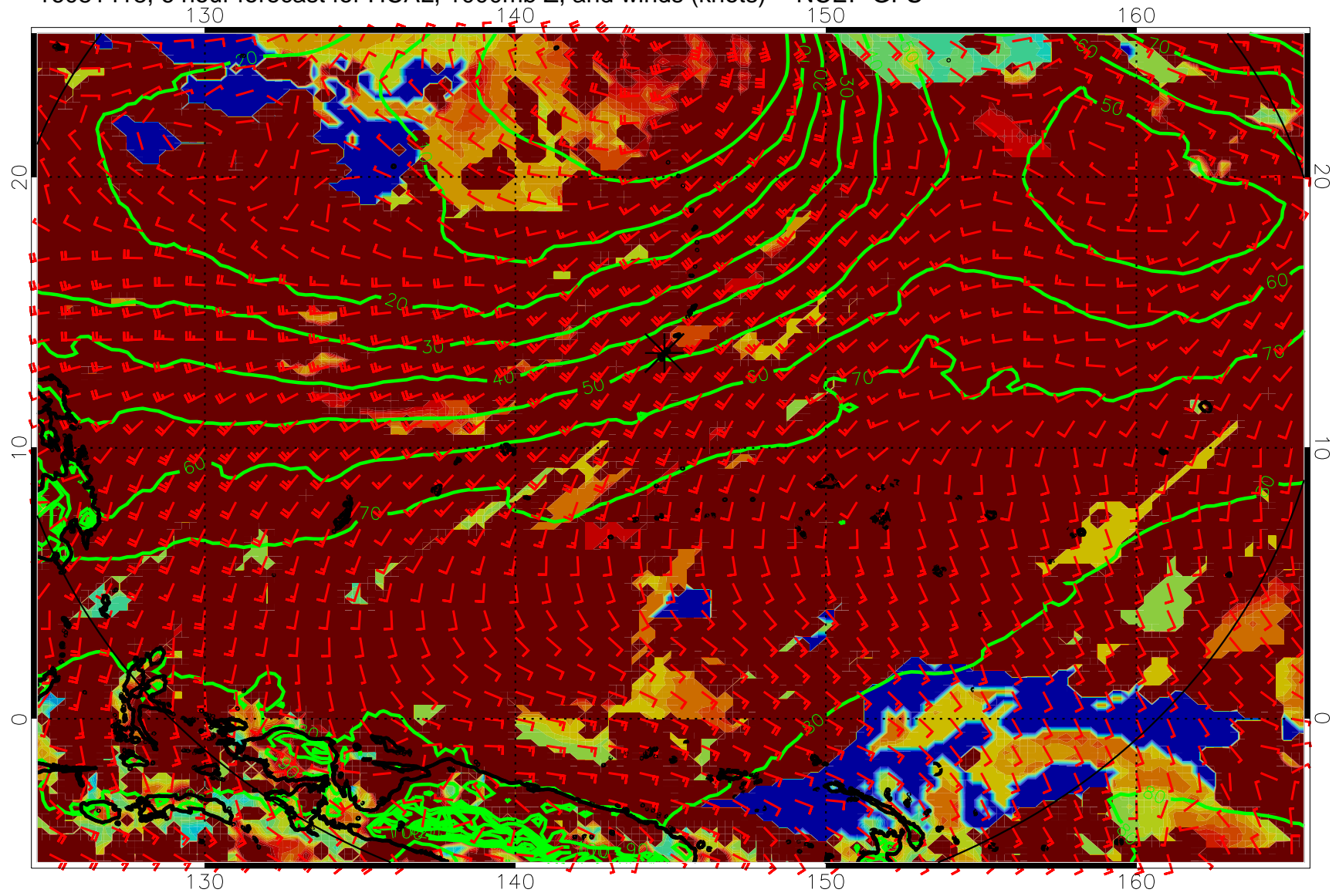
16081418, 6 hour forecast for HCAL, 1000mb Z, and winds (knots) -- NCEP GFS
