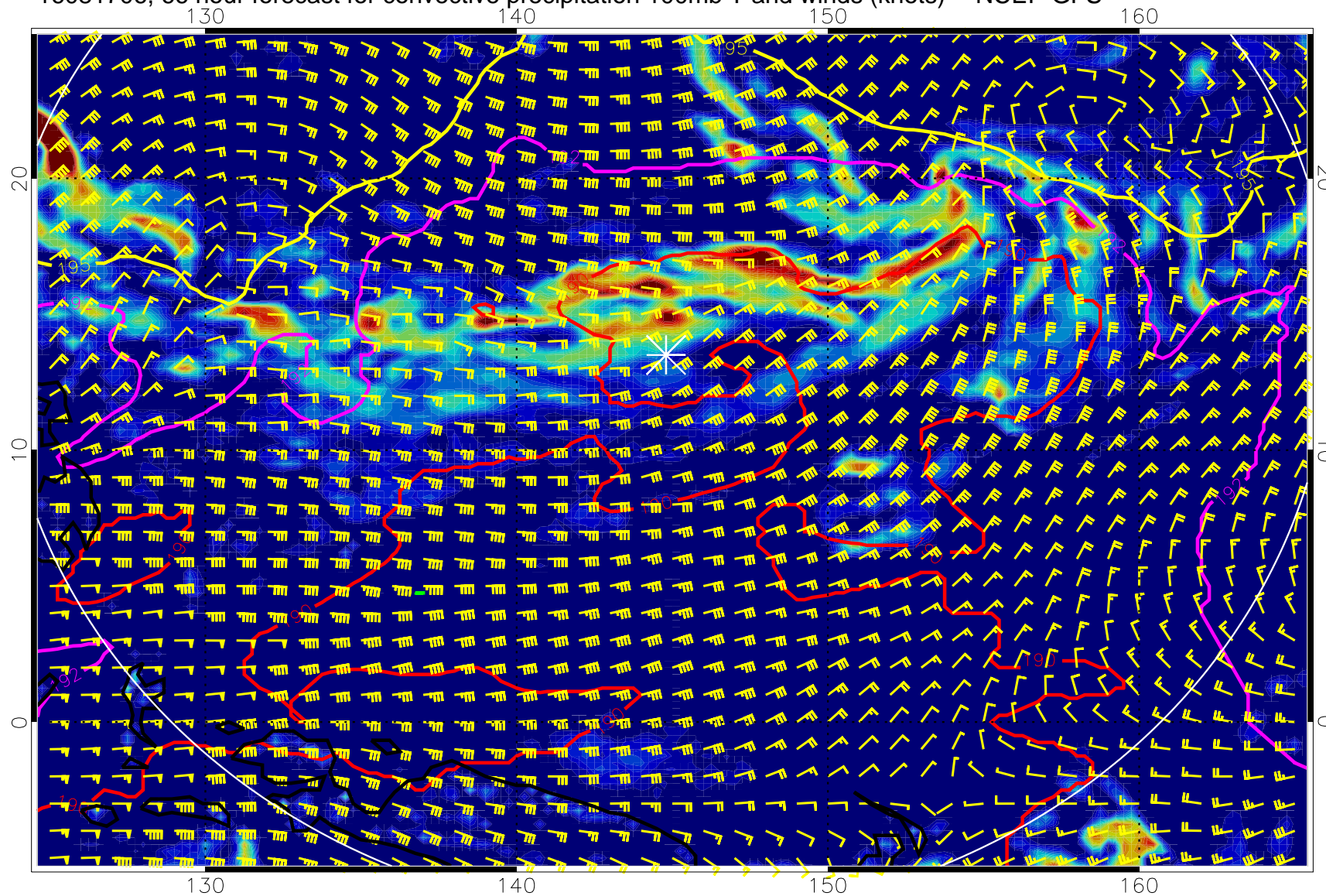
16081706, 66 hour forecast for convective precipitation 100mb T and winds (knots) -- NCEP GFS
