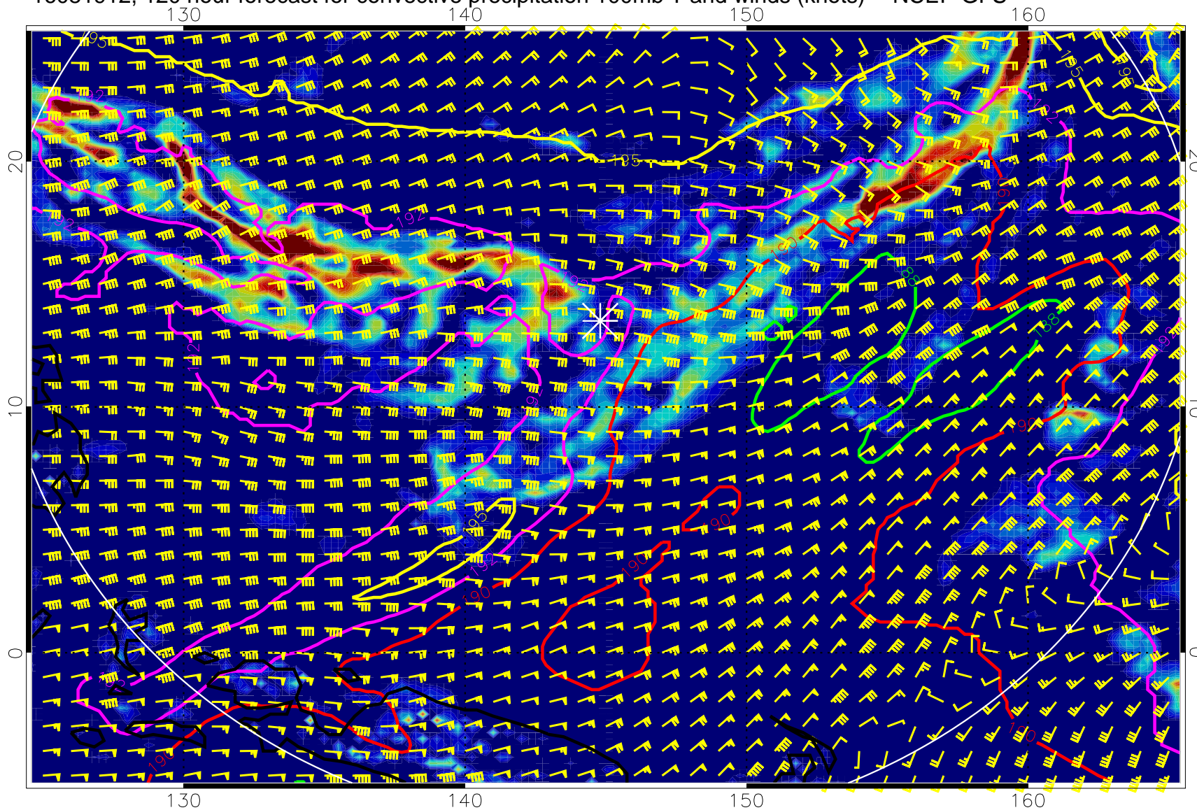
16081912, 120 hour forecast for convective precipitation 100mb T and winds (knots) -- NCEP GFS
