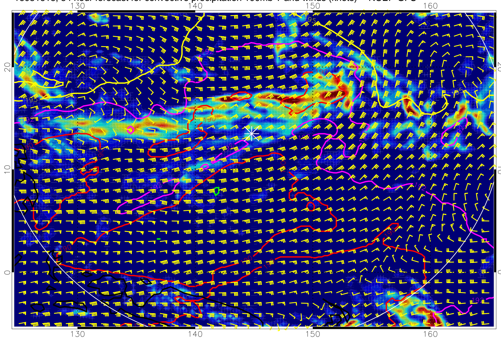
16081618, 54 hour forecast for convective precipitation 100mb T and winds (knots) -- NCEP GFS
