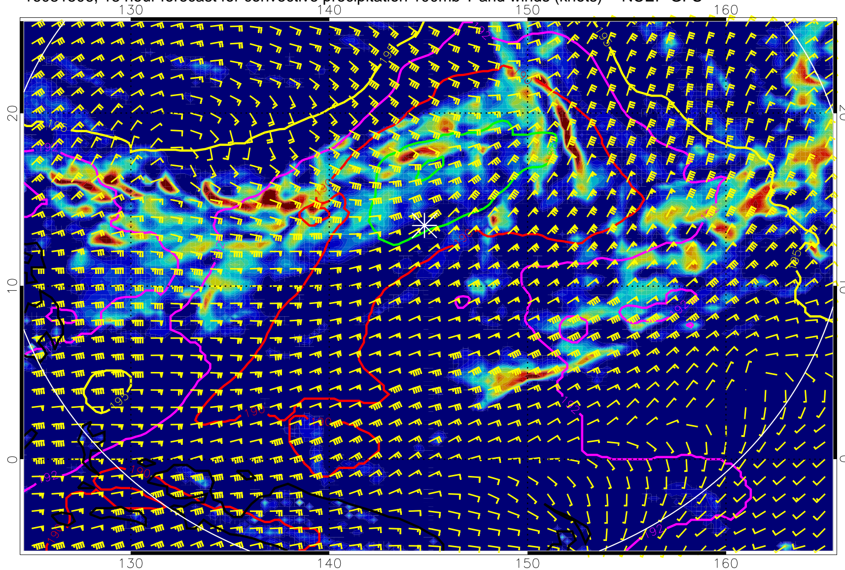
16081506, 18 hour forecast for convective precipitation 100mb T and winds (knots) -- NCEP GFS
