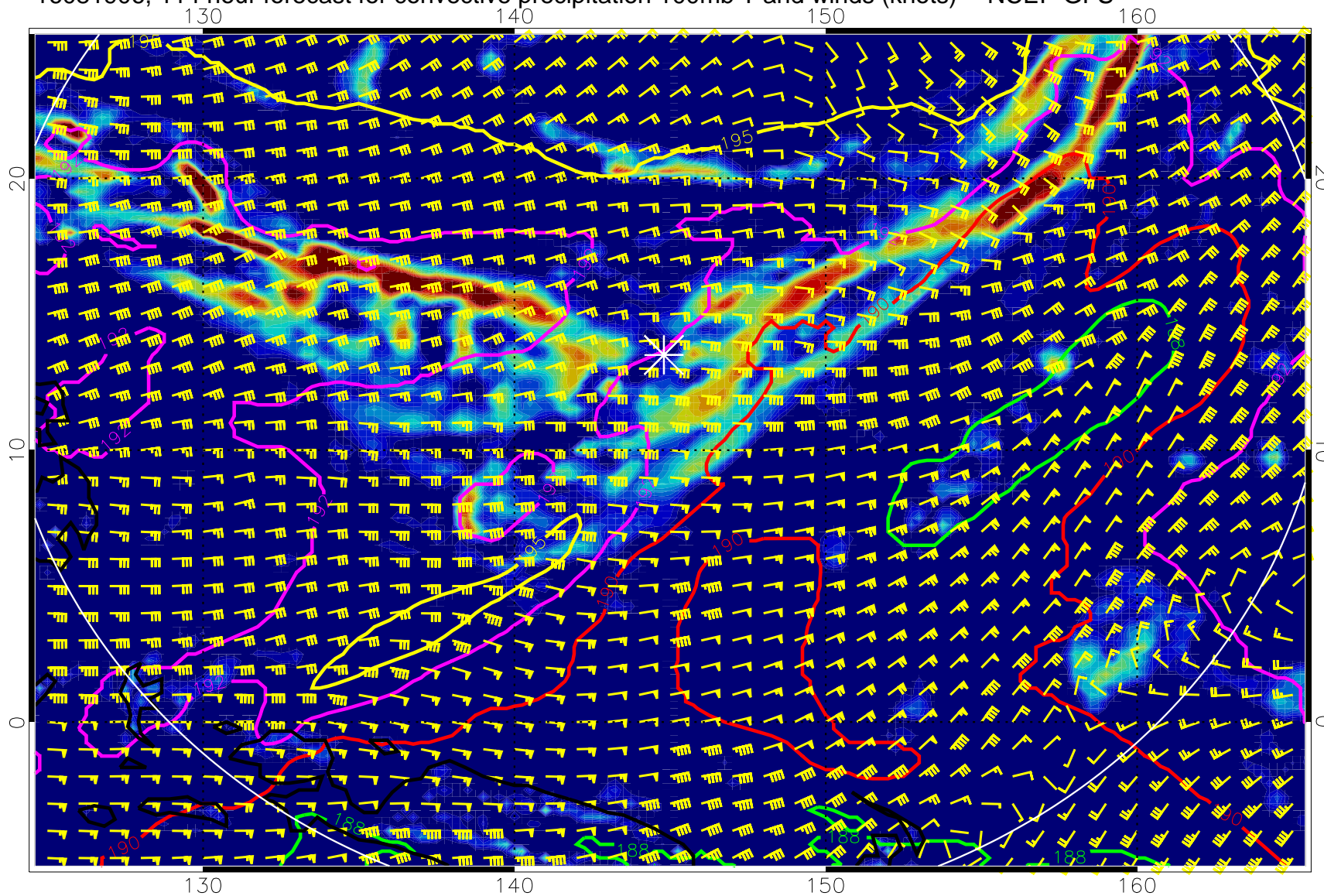
16081906, 114 hour forecast for convective precipitation 100mb T and winds (knots) -- NCEP GFS
