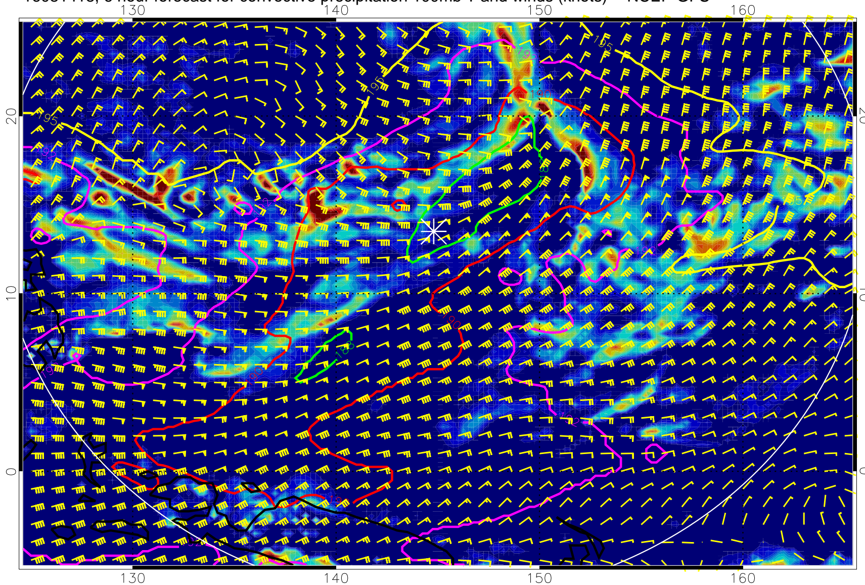
16081418, 6 hour forecast for convective precipitation 100mb T and winds (knots) -- NCEP GFS
