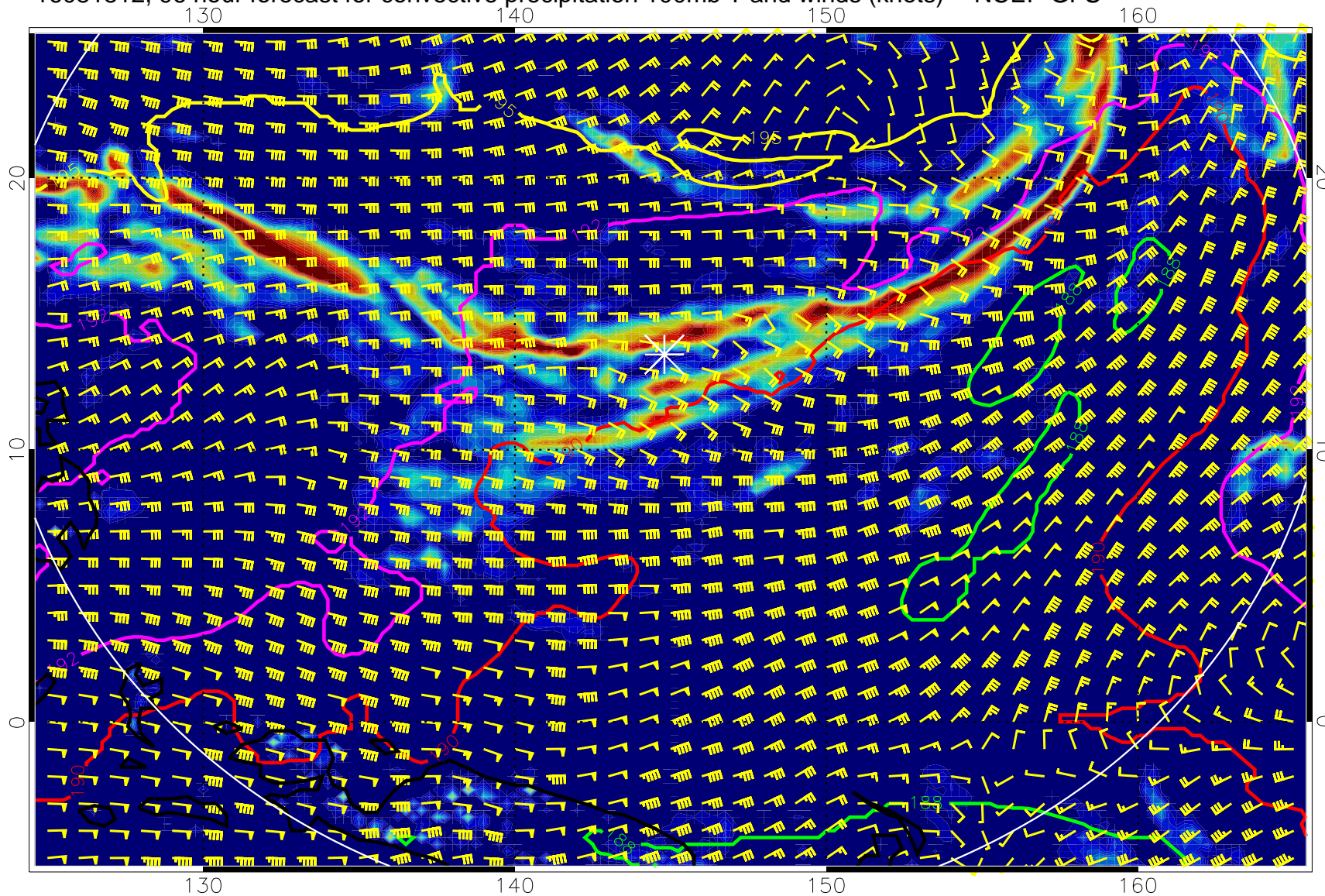
16081812, 96 hour forecast for convective precipitation 100mb T and winds (knots) -- NCEP GFS
