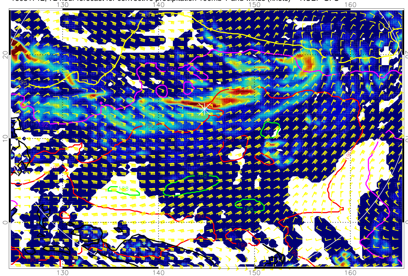
16081712, 72 hour forecast for convective precipitation 100mb T and winds (knots) -- NCEP GFS
