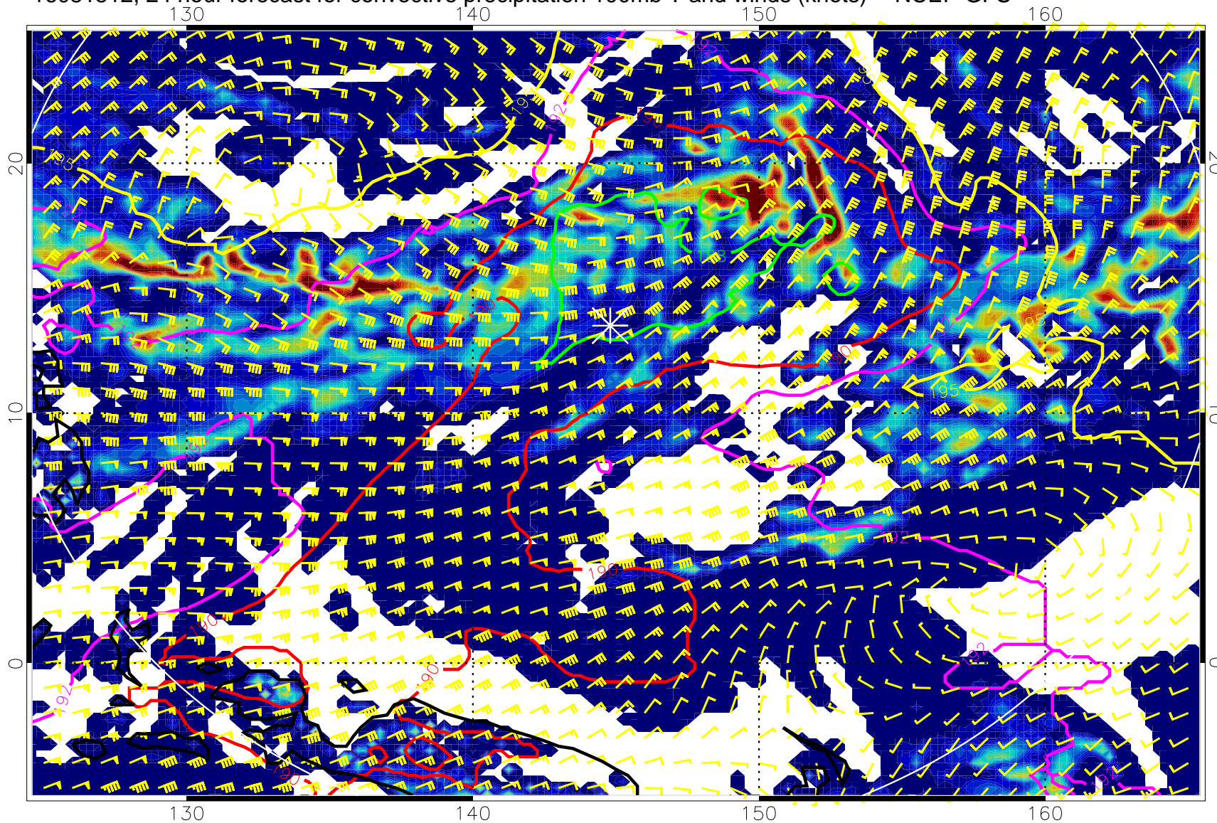
16081512, 24 hour forecast for convective precipitation 100mb T and winds (knots) -- NCEP GFS
