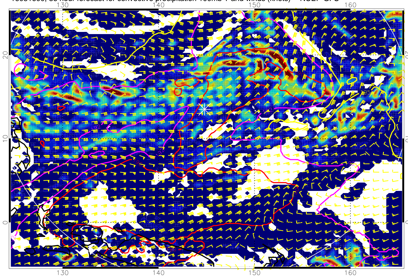
16081600, 36 hour forecast for convective precipitation 100mb T and winds (knots) -- NCEP GFS
