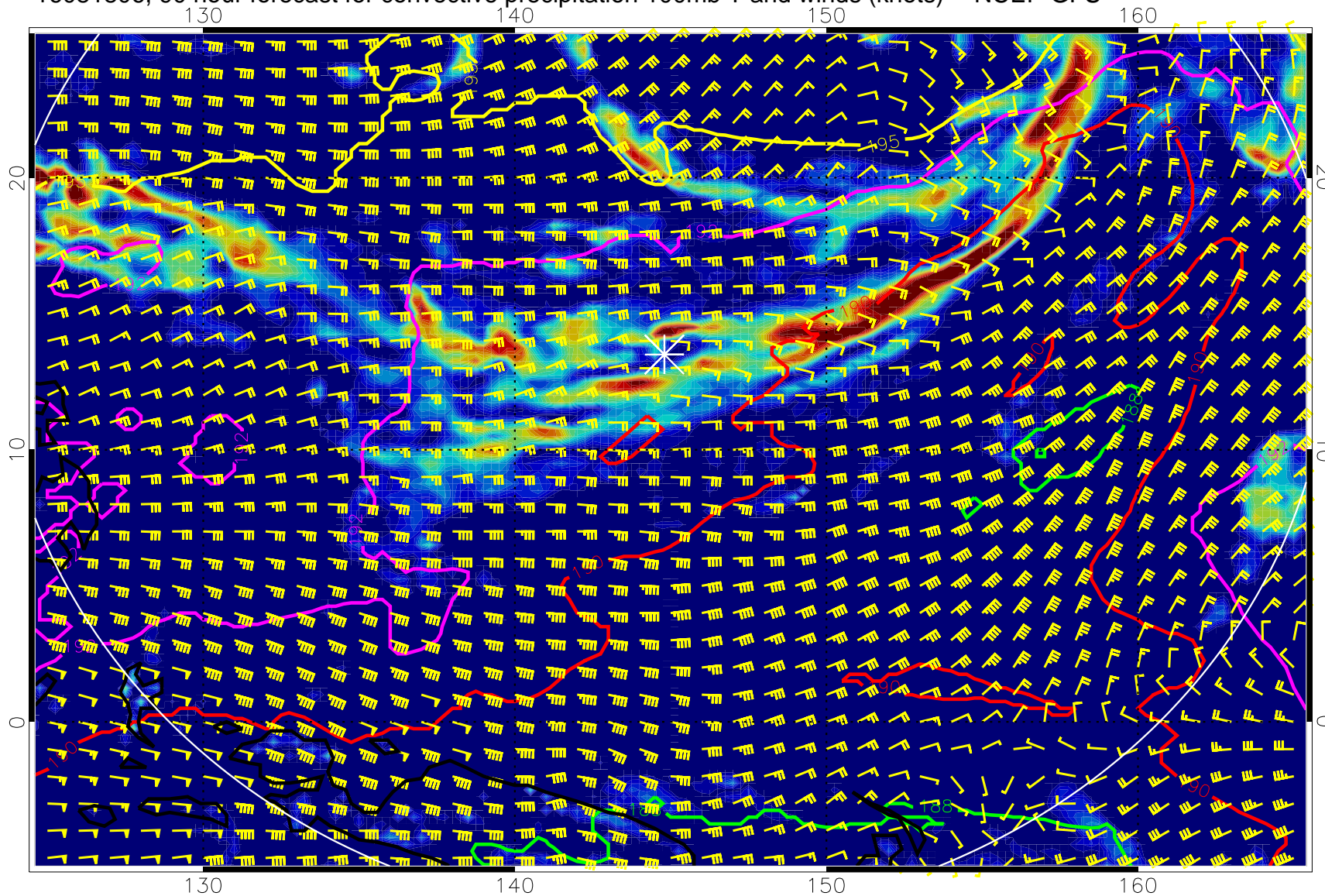
16081806, 90 hour forecast for convective precipitation 100mb T and winds (knots) -- NCEP GFS
