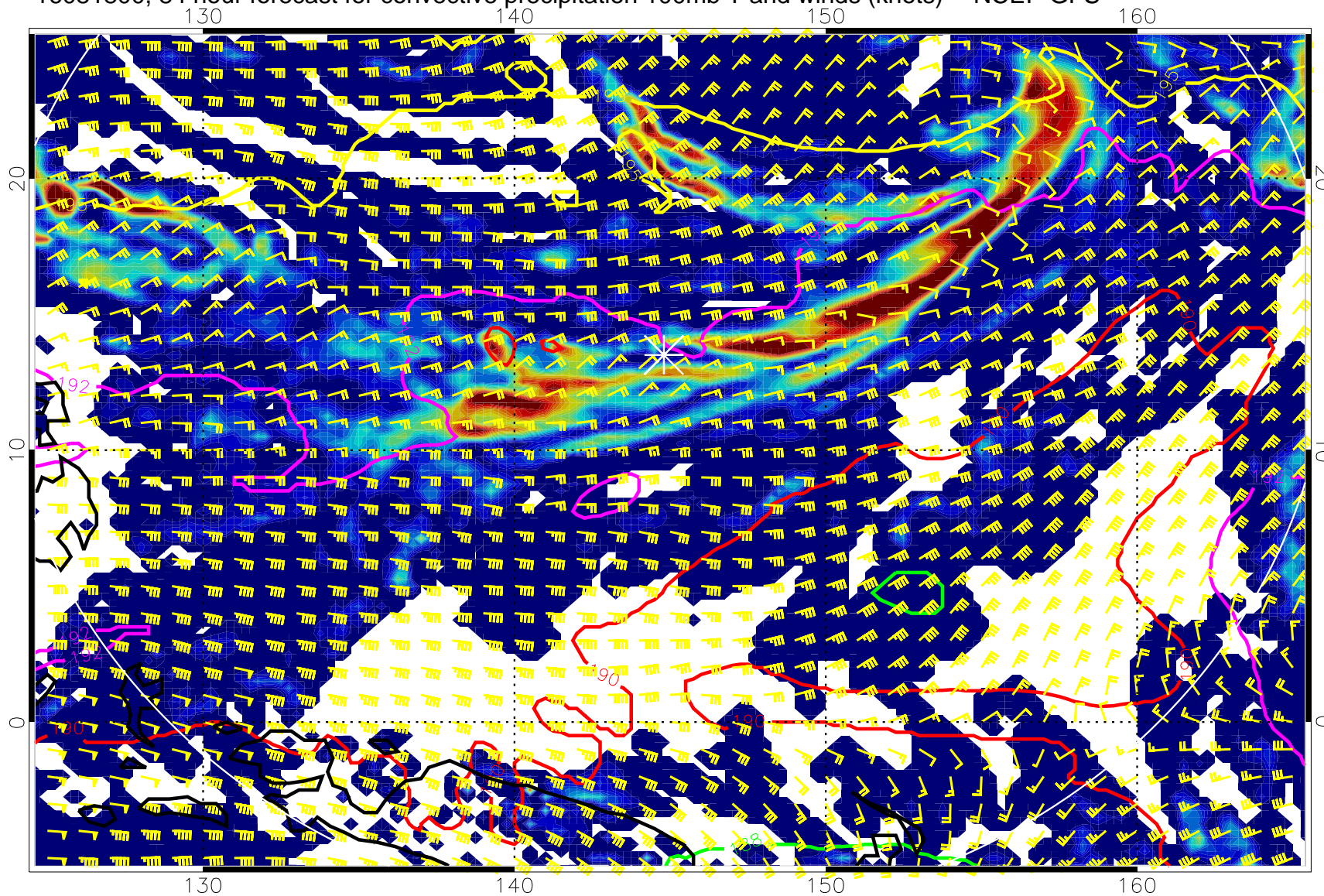
16081800, 84 hour forecast for convective precipitation 100mb T and winds (knots) -- NCEP GFS
