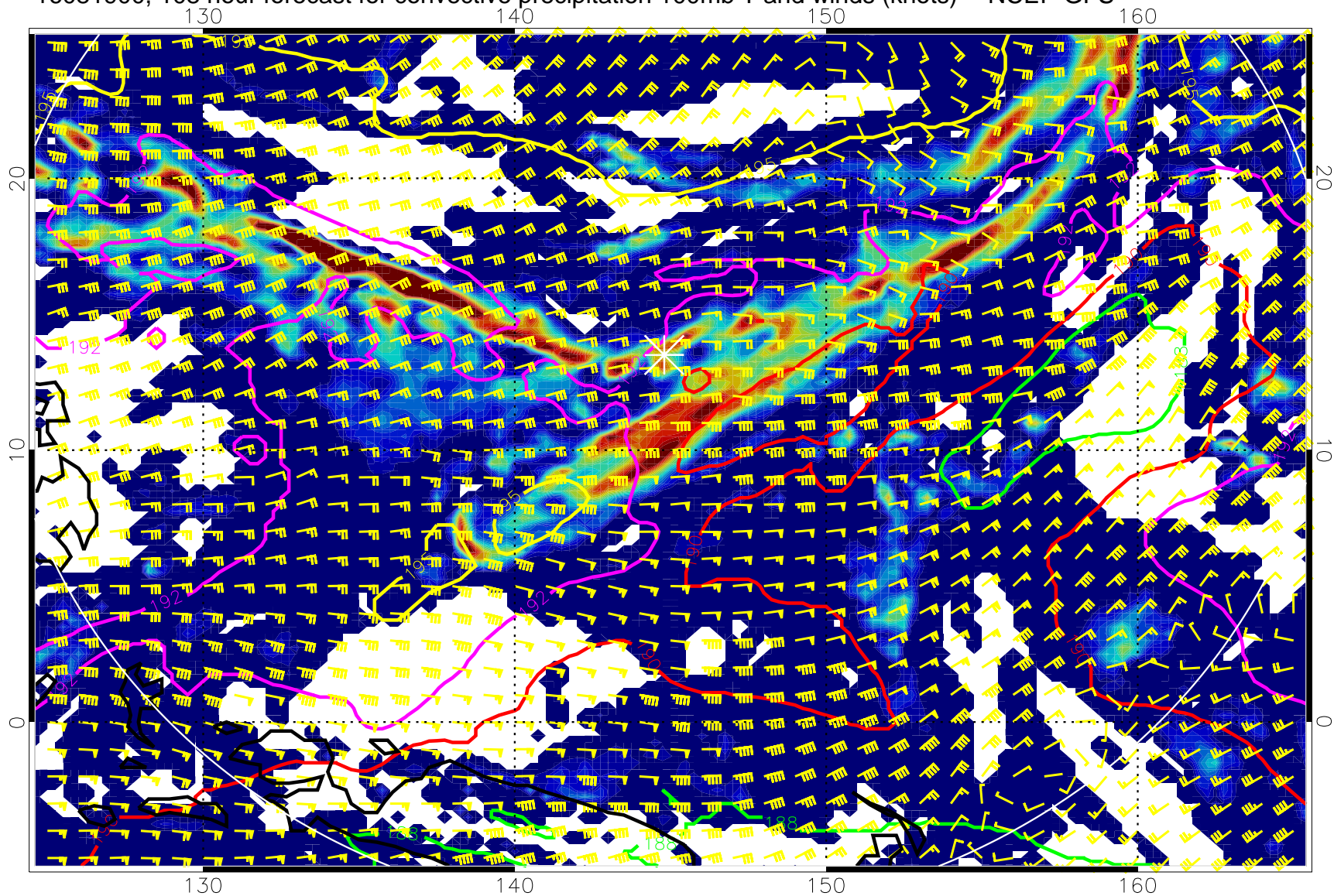
16081900, 108 hour forecast for convective precipitation 100mb T and winds (knots) -- NCEP GFS
