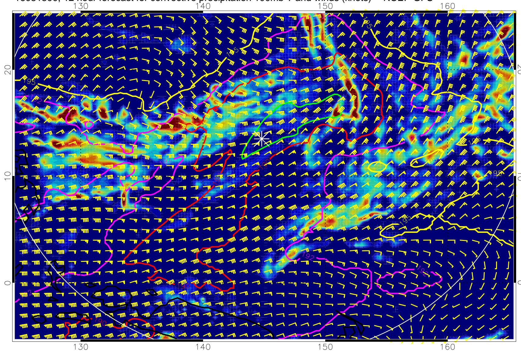
16081500, 12 hour forecast for convective precipitation 100mb T and winds (knots) -- NCEP GFS
