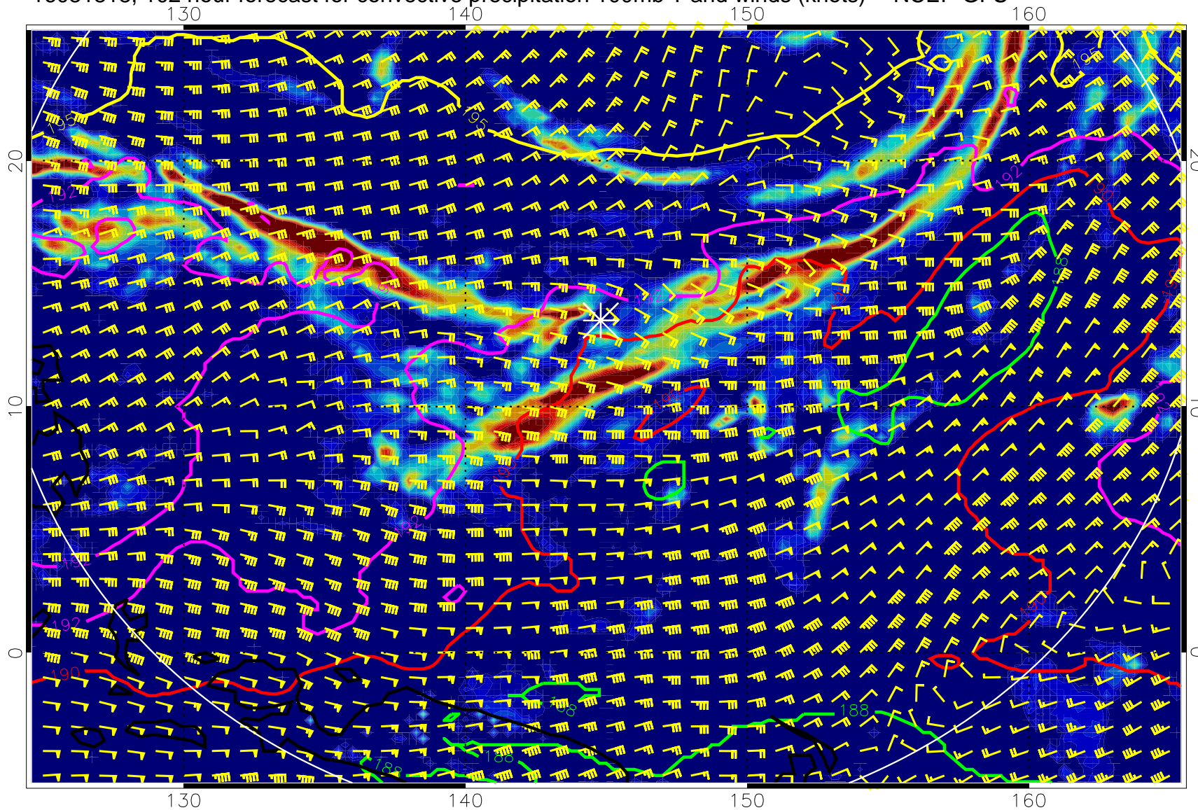
16081818, 102 hour forecast for convective precipitation 100mb T and winds (knots) -- NCEP GFS
