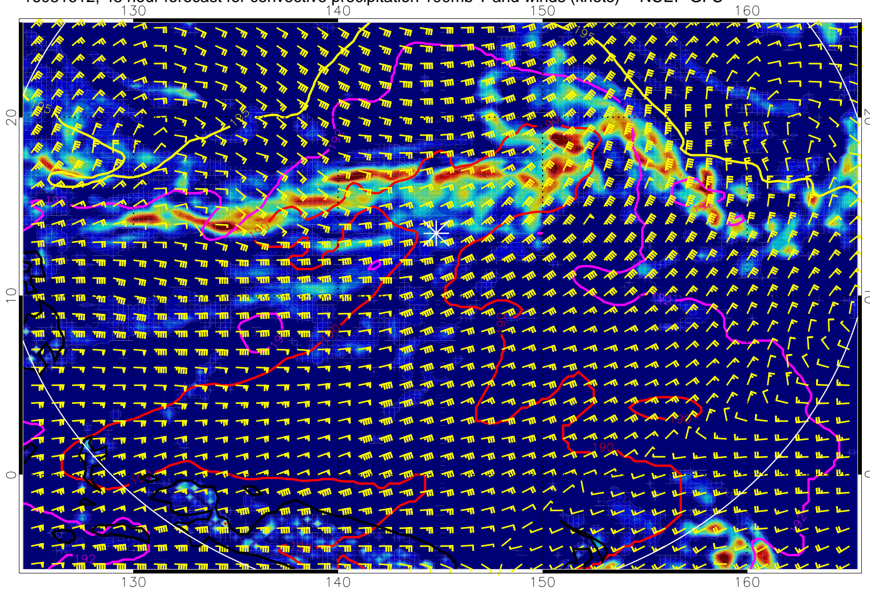
16081612, 48 hour forecast for convective precipitation 100mb T and winds (knots) -- NCEP GFS
