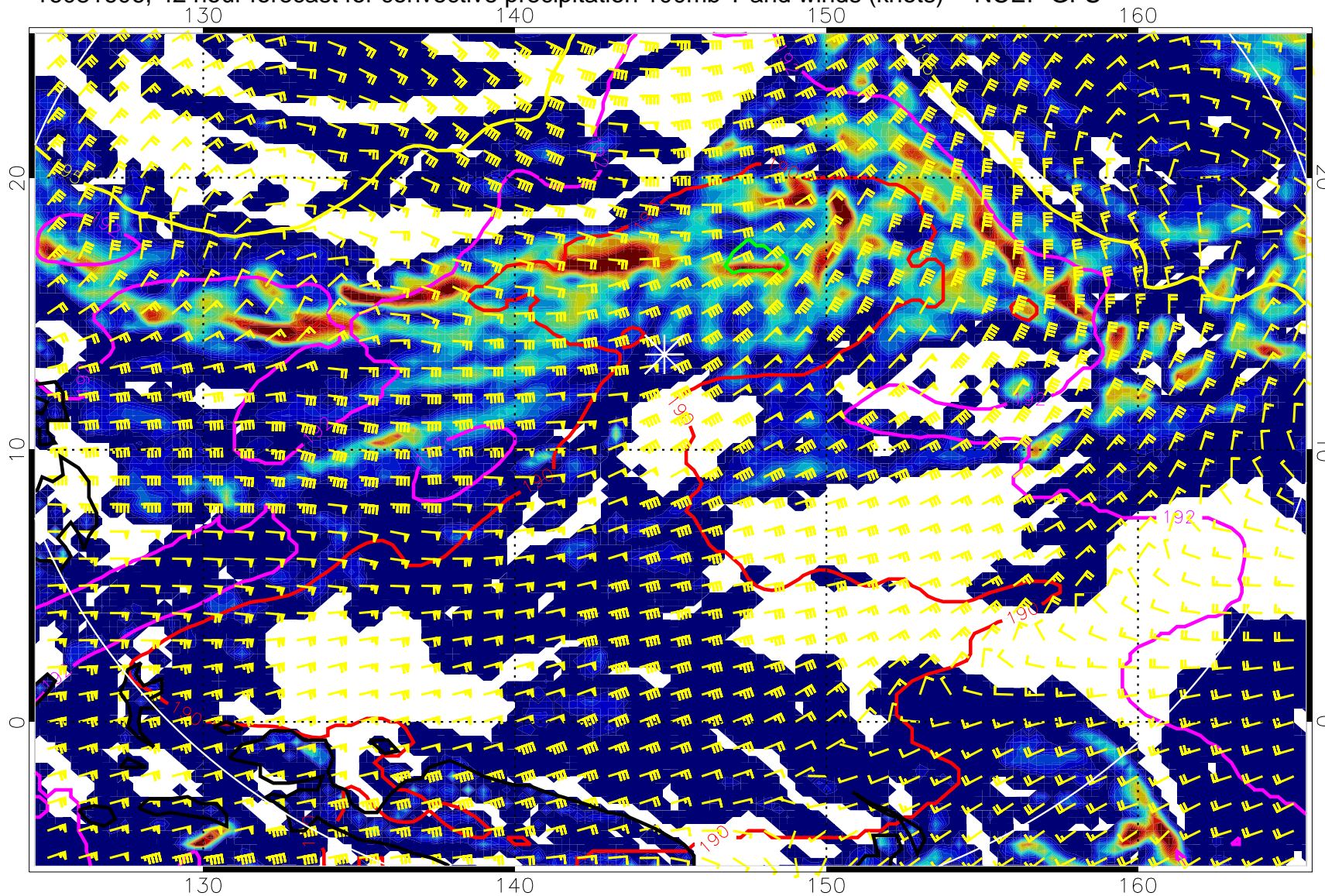
16081606, 42 hour forecast for convective precipitation 100mb T and winds (knots) -- NCEP GFS
