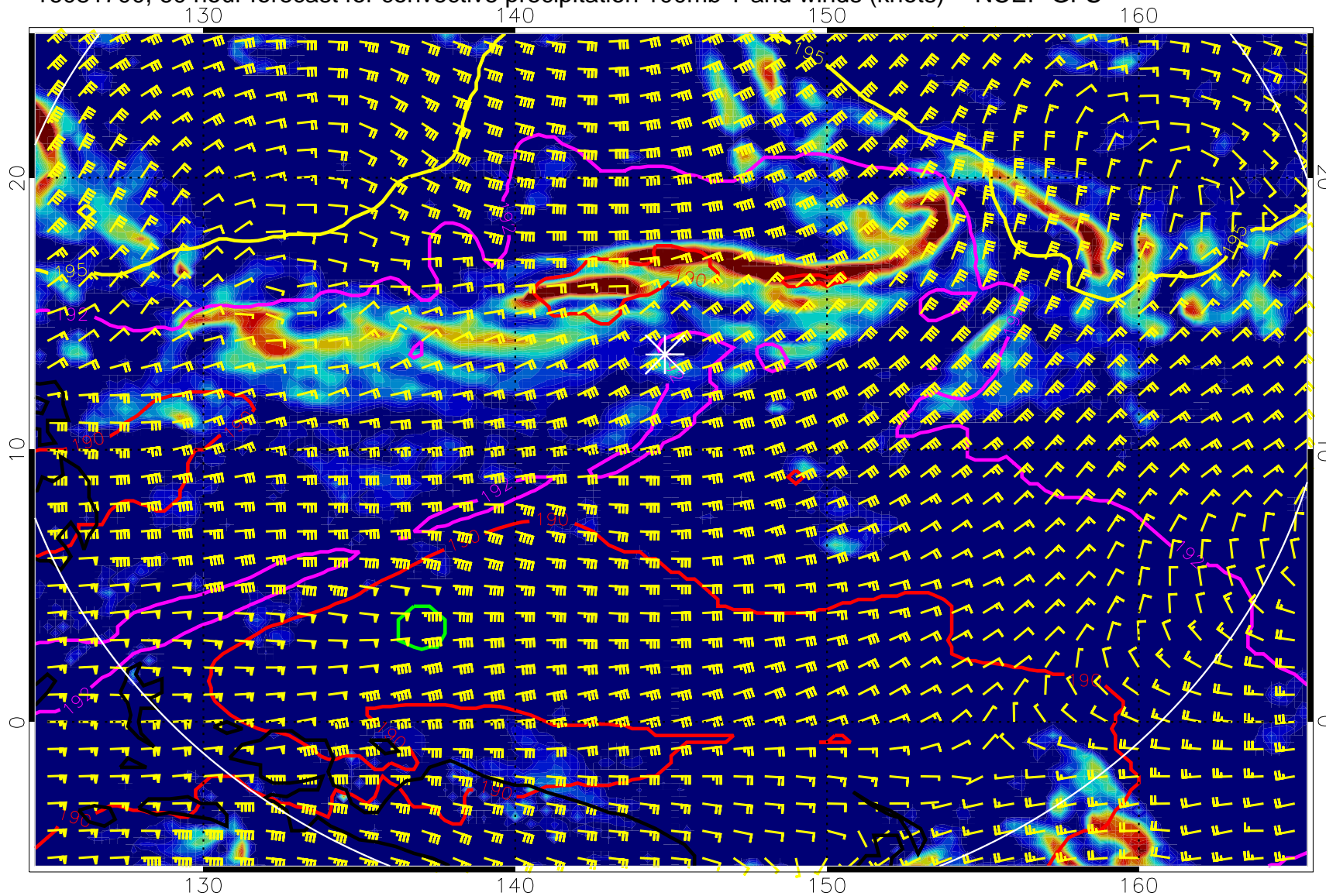
16081700, 60 hour forecast for convective precipitation 100mb T and winds (knots) -- NCEP GFS
