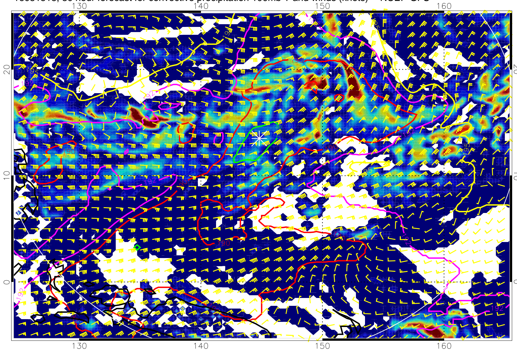
16081518, 30 hour forecast for convective precipitation 100mb T and winds (knots) -- NCEP GFS
