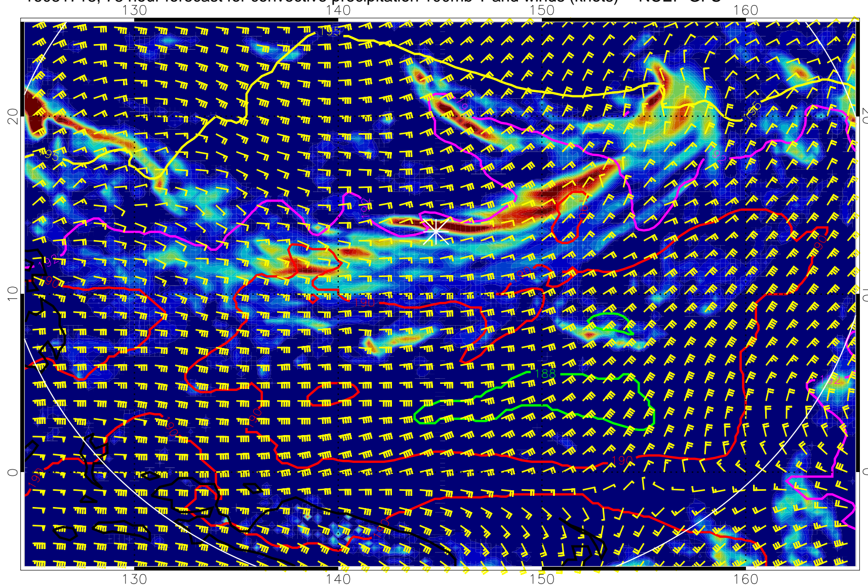
16081718, 78 hour forecast for convective precipitation 100mb T and winds (knots) -- NCEP GFS
