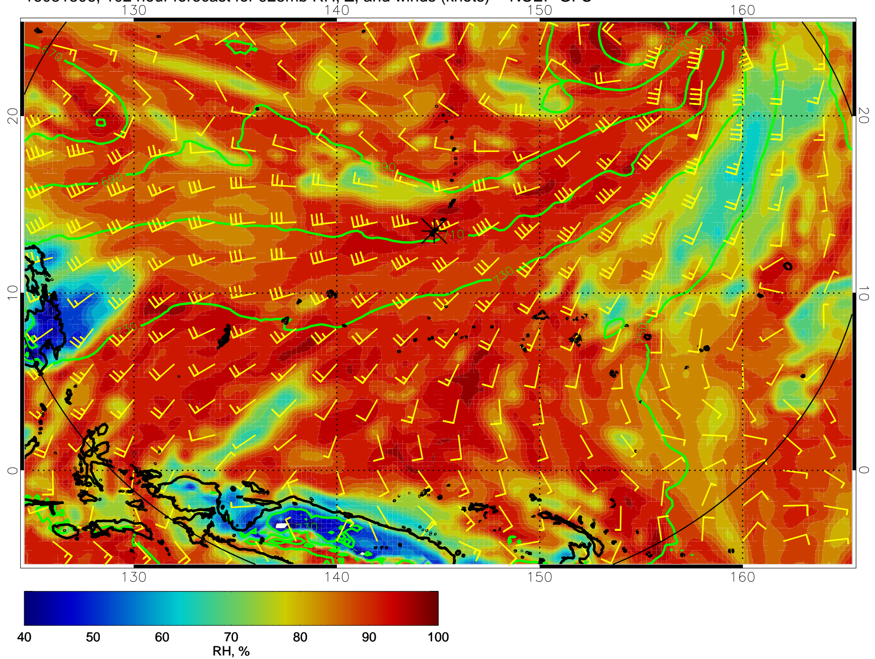
16081806, 102 hour forecast for 925mb RH, Z, and winds (knots) -- NCEP GFS
