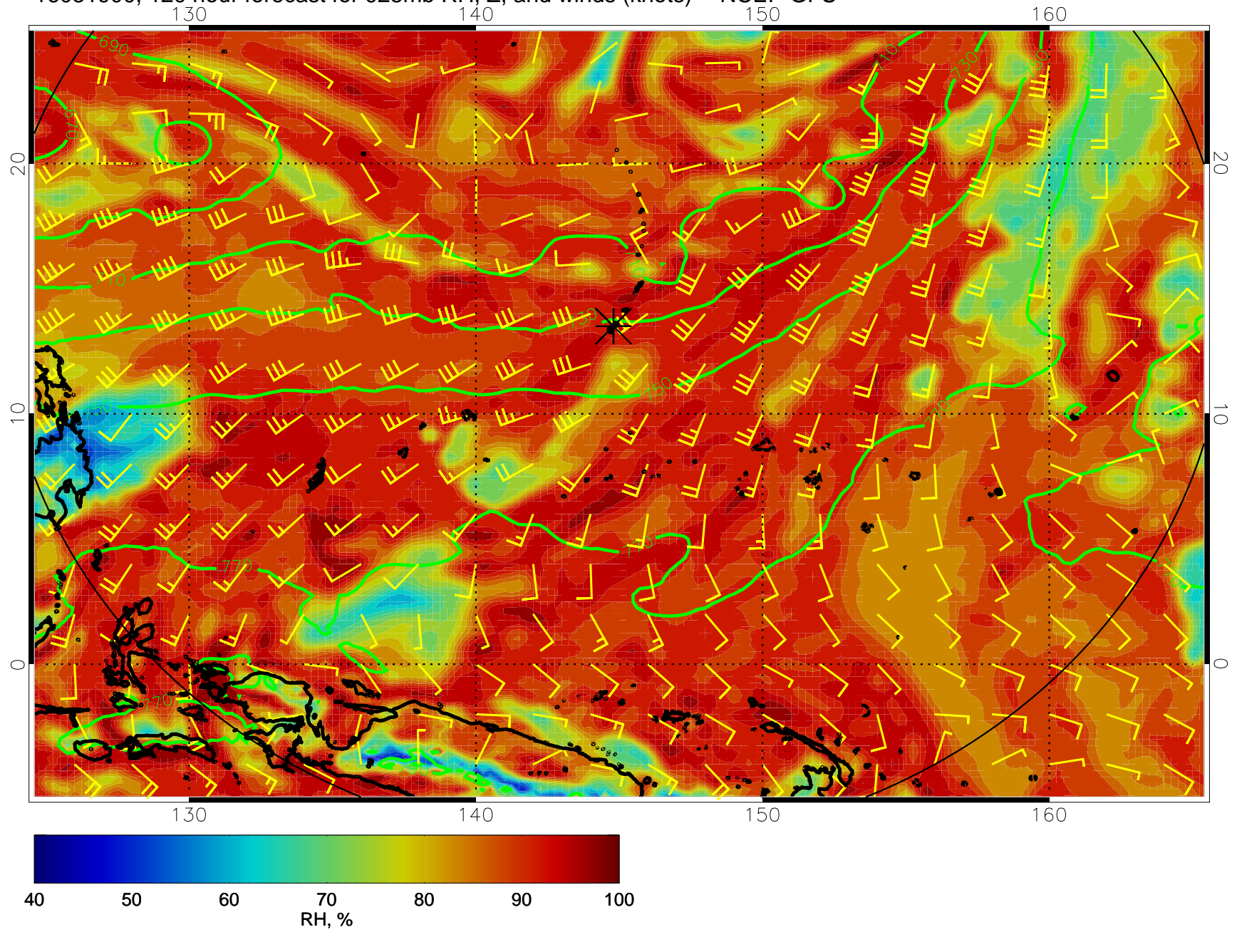
16081900, 120 hour forecast for 925mb RH, Z, and winds (knots) -- NCEP GFS
