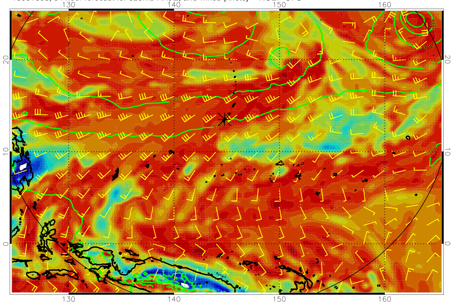
16081606, 54 hour forecast for 925mb RH, Z, and winds (knots) -- NCEP GFS
