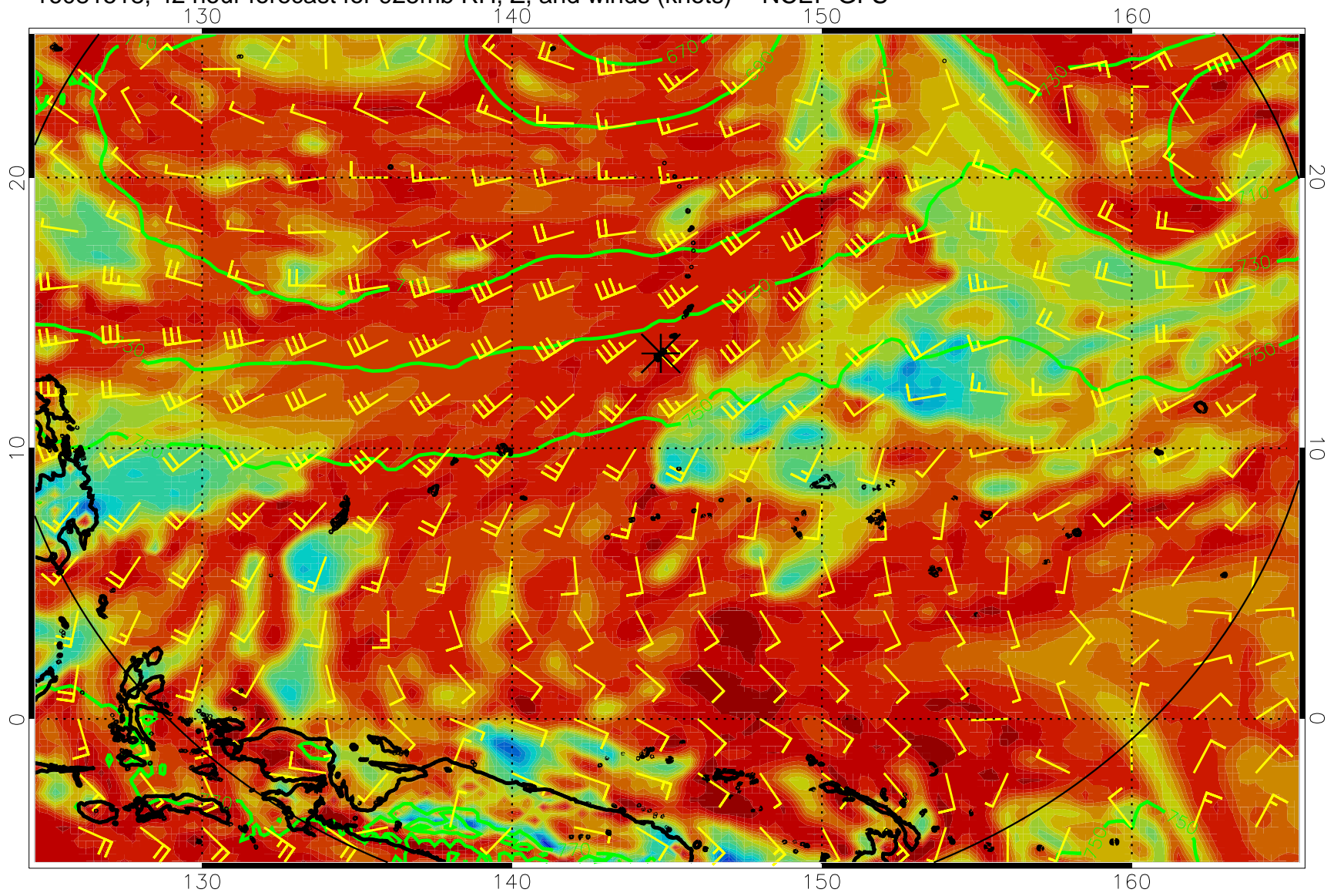
16081518, 42 hour forecast for 925mb RH, Z, and winds (knots) -- NCEP GFS
