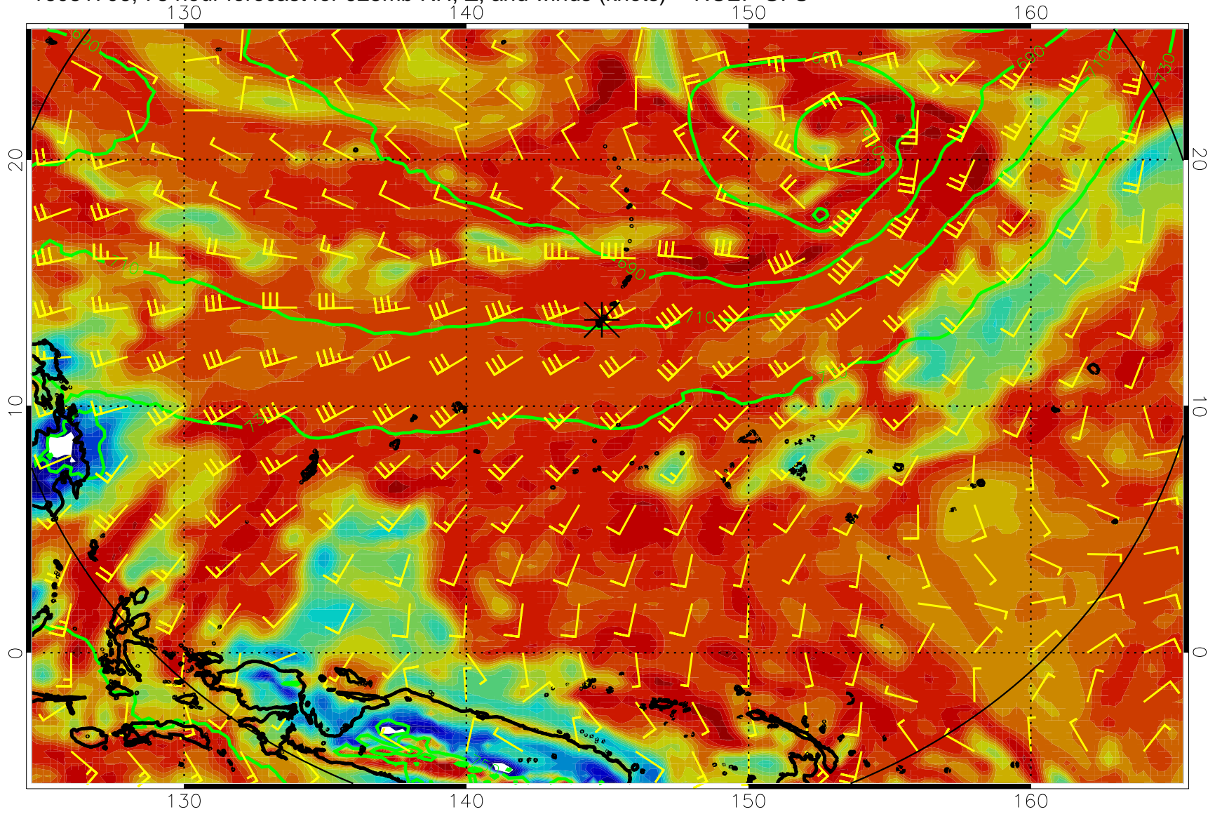
16081706, 78 hour forecast for 925mb RH, Z, and winds (knots) -- NCEP GFS
