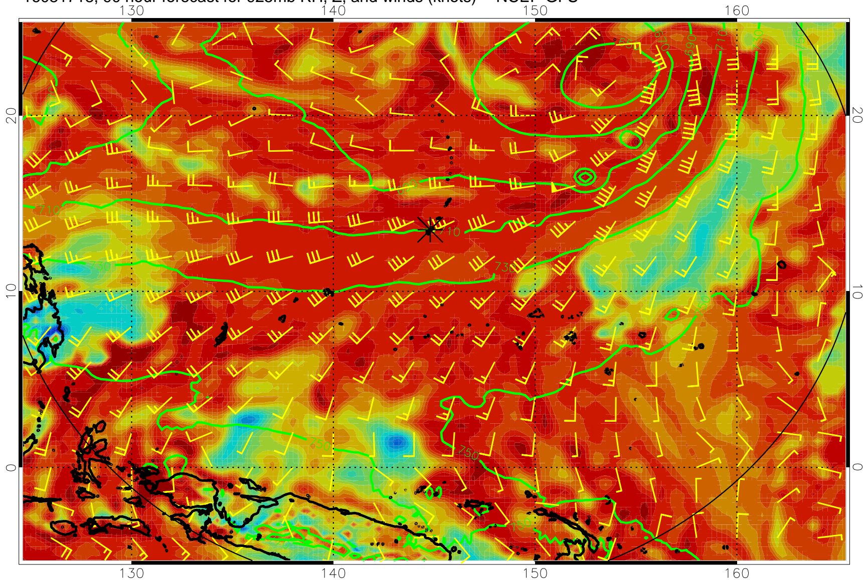
16081718, 90 hour forecast for 925mb RH, Z, and winds (knots) -- NCEP GFS
