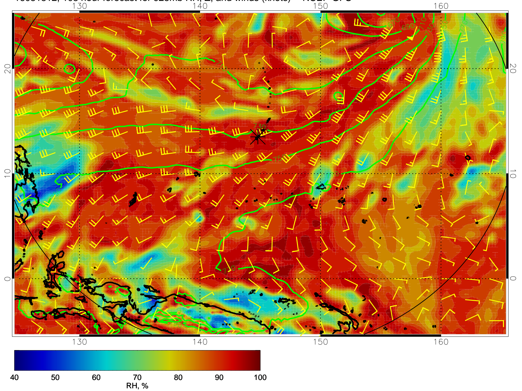
16081812, 108 hour forecast for 925mb RH, Z, and winds (knots) -- NCEP GFS
