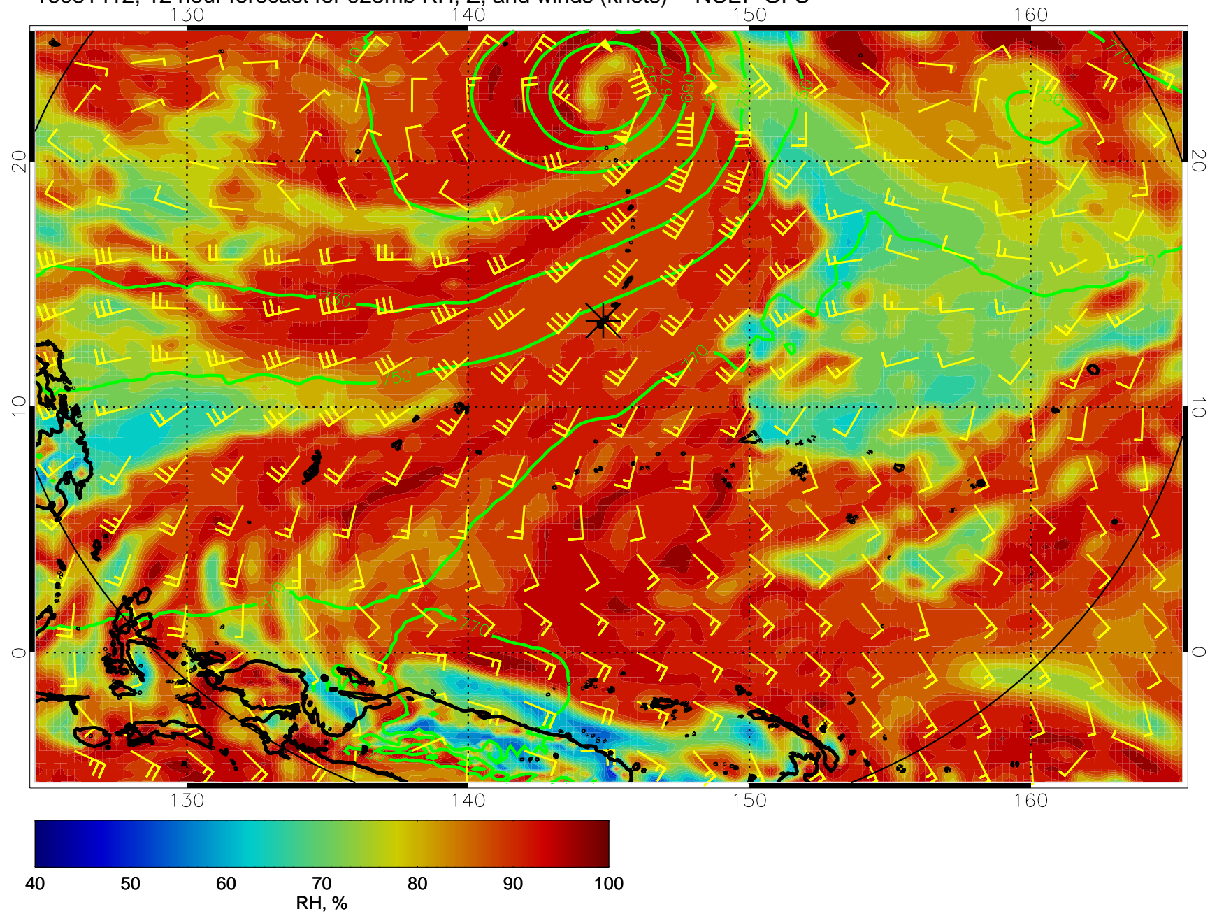
16081412, 12 hour forecast for 925mb RH, Z, and winds (knots) -- NCEP GFS
