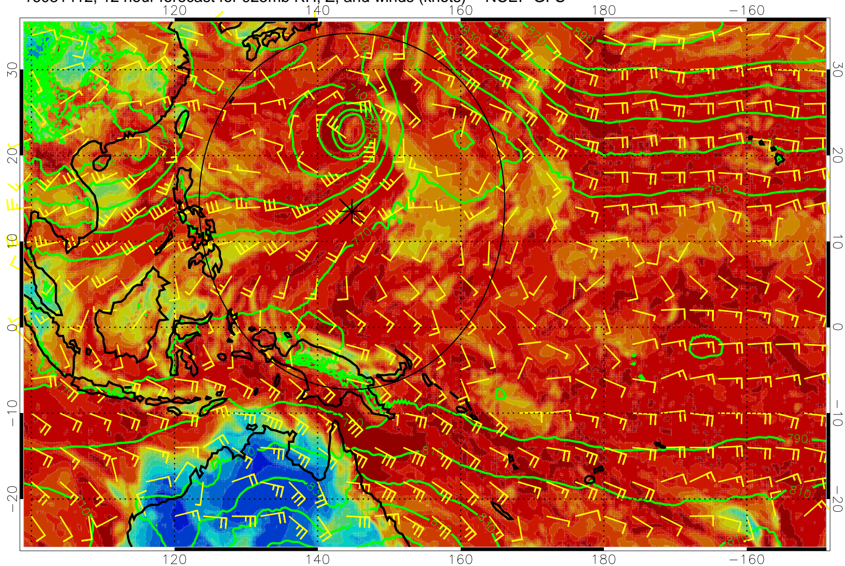
16081412, 12 hour forecast for 925mb RH, Z, and winds (knots) -- NCEP GFS
