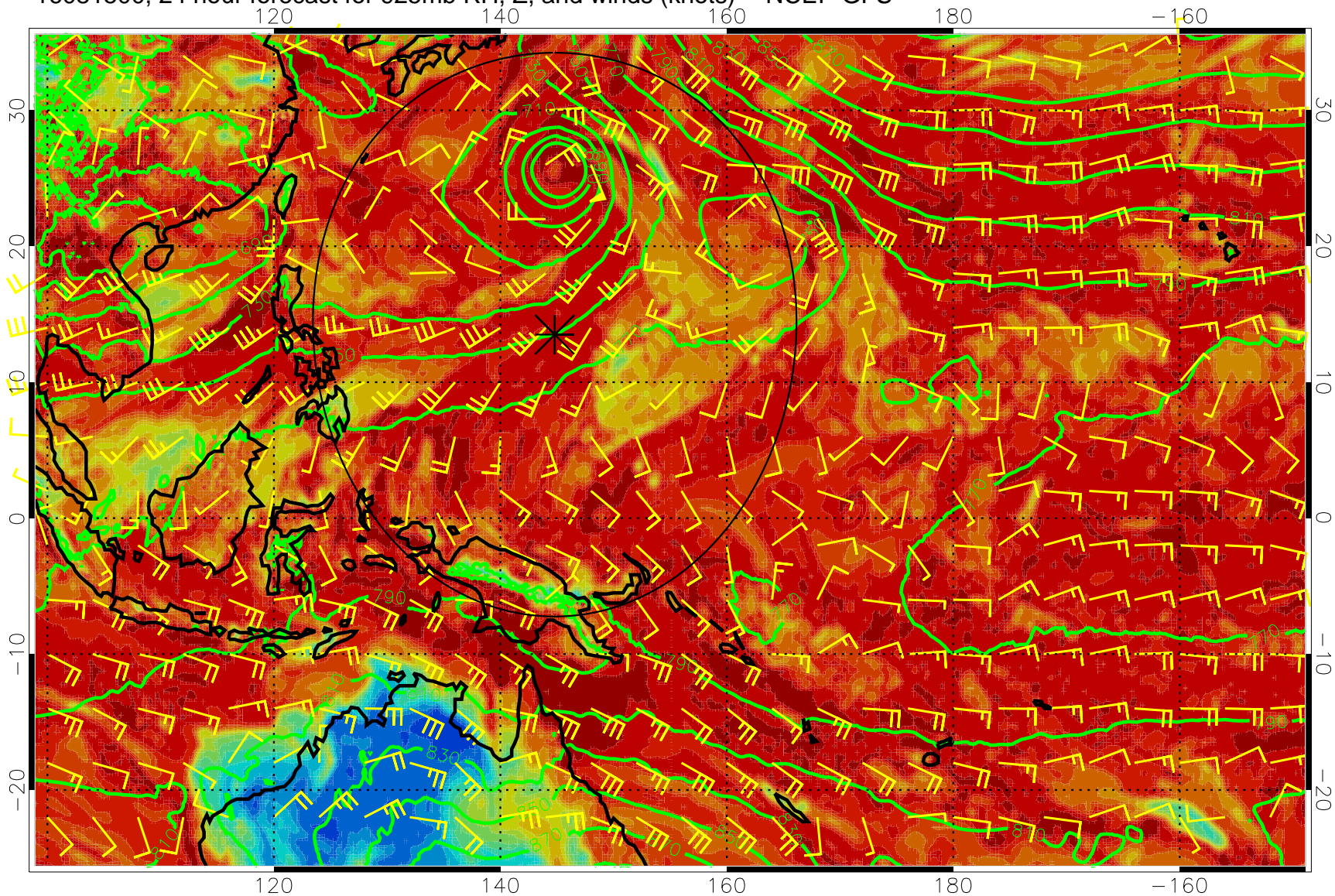
16081500, 24 hour forecast for 925mb RH, Z, and winds (knots) -- NCEP GFS
