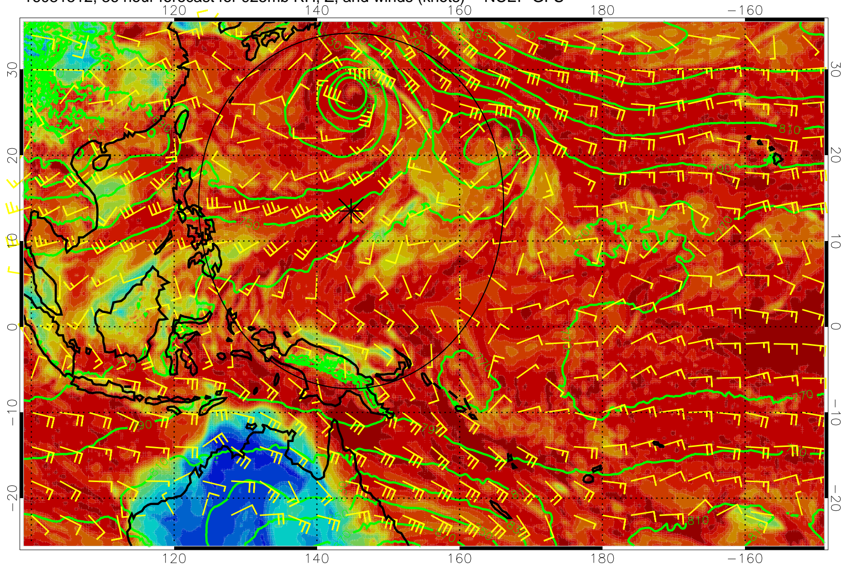
16081512, 36 hour forecast for 925mb RH, Z, and winds (knots) -- NCEP GFS
