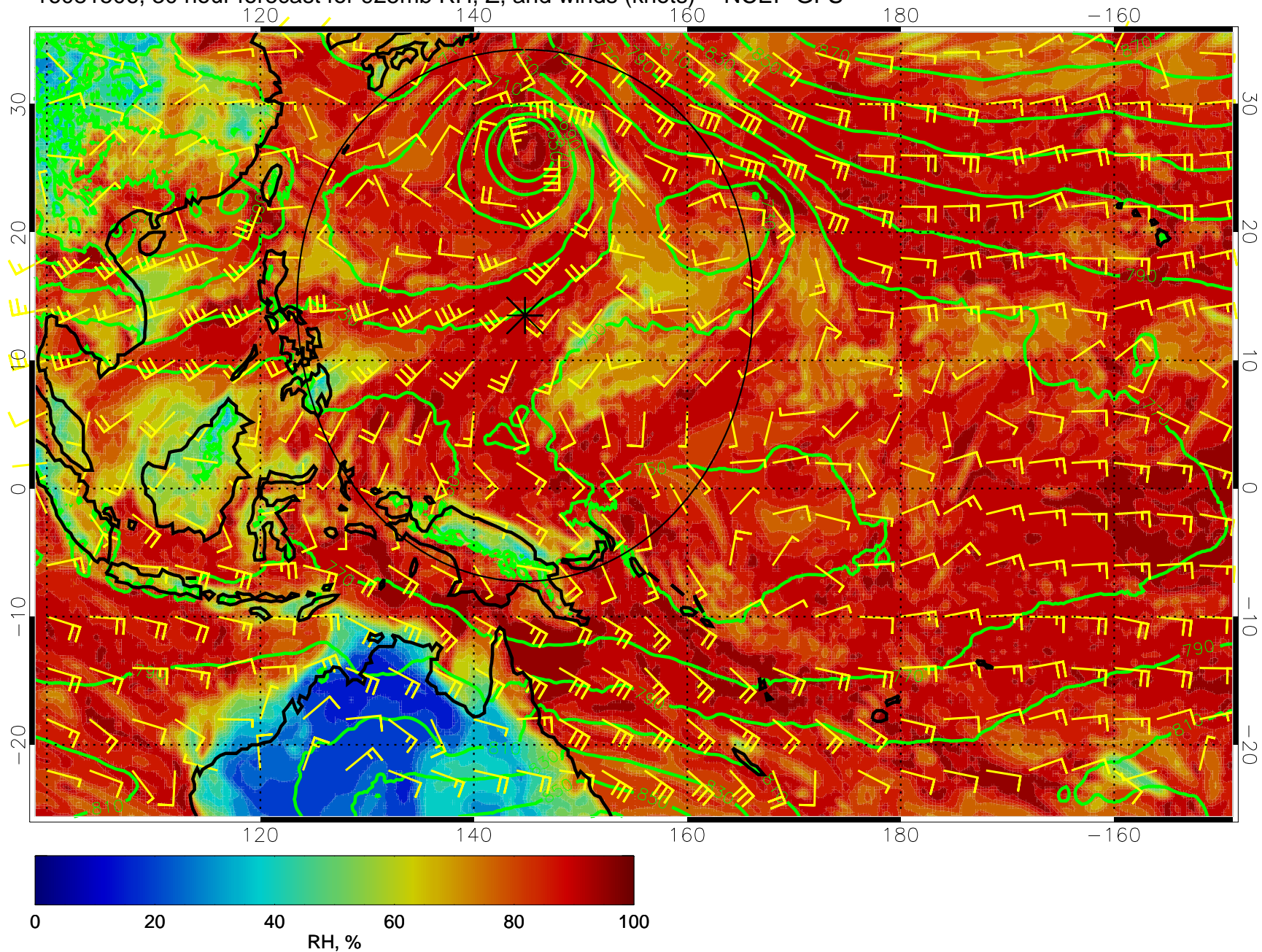
16081506, 30 hour forecast for 925mb RH, Z, and winds (knots) -- NCEP GFS
