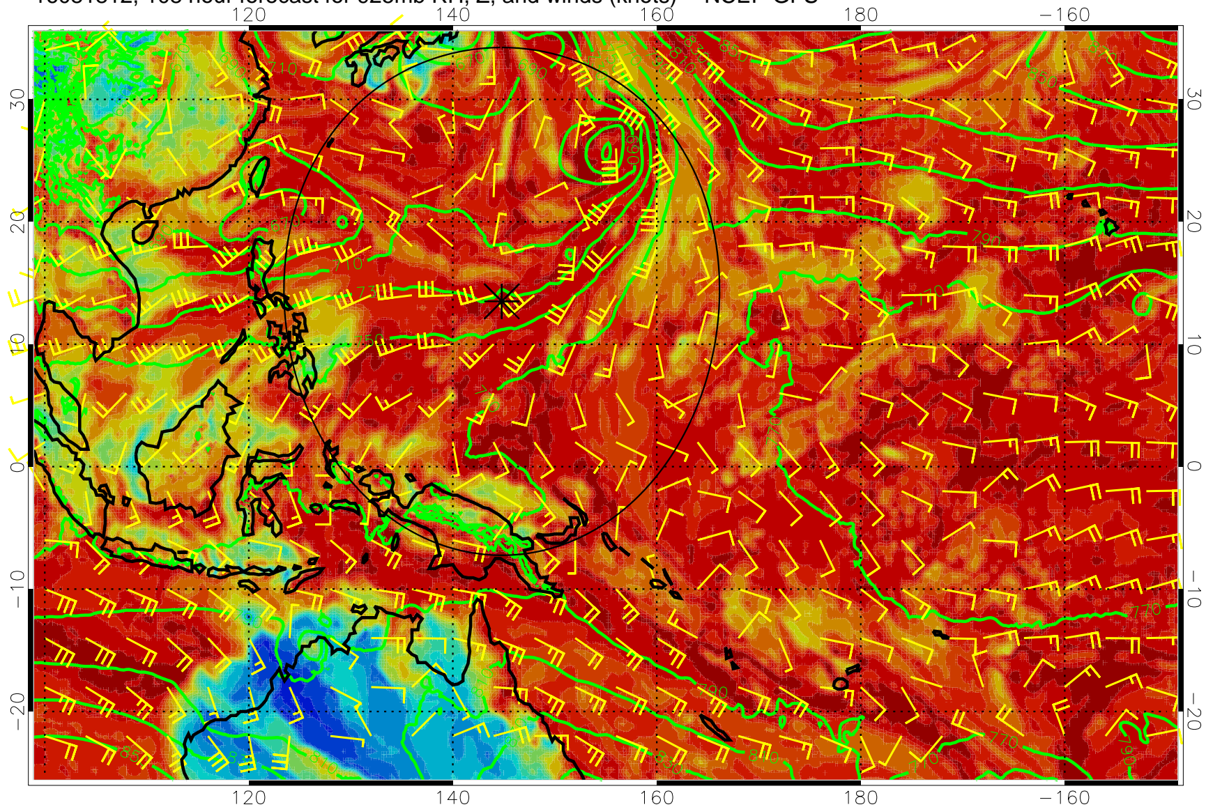
16081812, 108 hour forecast for 925mb RH, Z, and winds (knots) -- NCEP GFS
