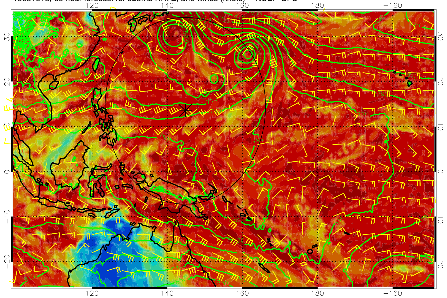
16081618, 66 hour forecast for 925mb RH, Z, and winds (knots) -- NCEP GFS
