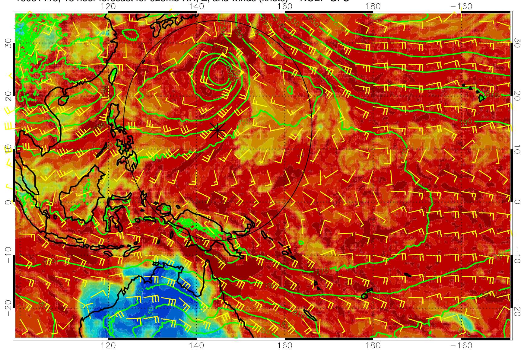
16081418, 18 hour forecast for 925mb RH, Z, and winds (knots) -- NCEP GFS
