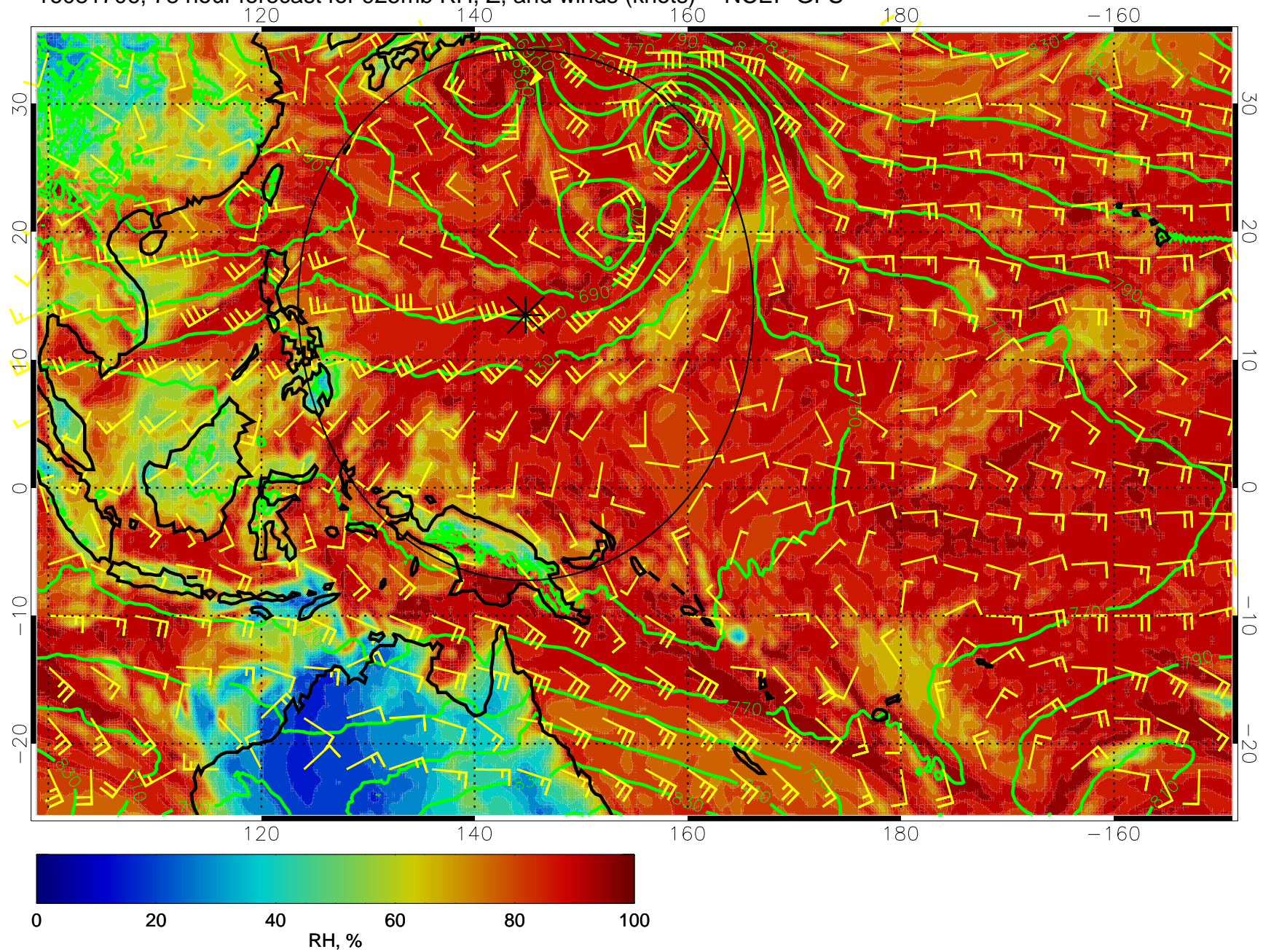
16081706, 78 hour forecast for 925mb RH, Z, and winds (knots) -- NCEP GFS
