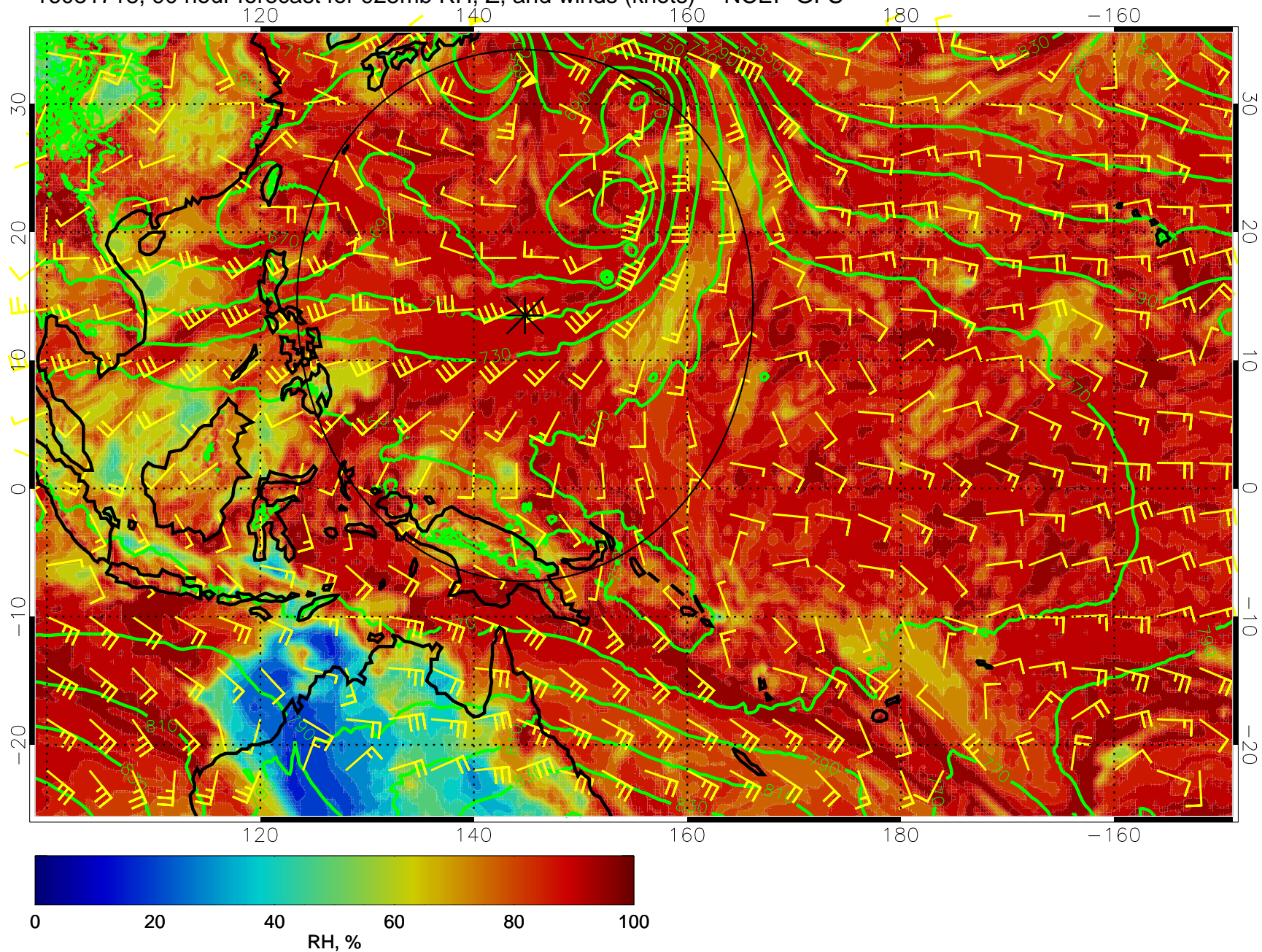
16081718, 90 hour forecast for 925mb RH, Z, and winds (knots) -- NCEP GFS
