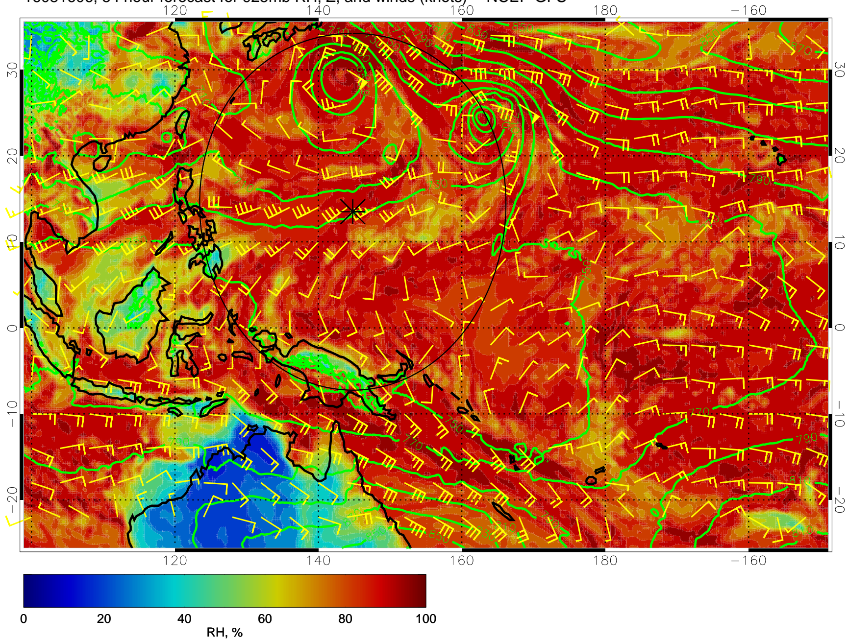
16081606, 54 hour forecast for 925mb RH, Z, and winds (knots) -- NCEP GFS
