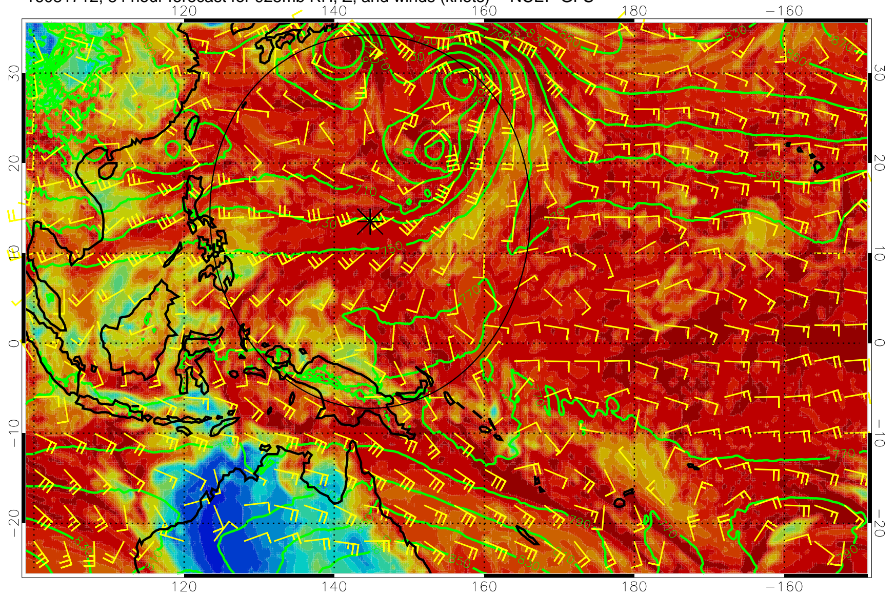
16081712, 84 hour forecast for 925mb RH, Z, and winds (knots) -- NCEP GFS
