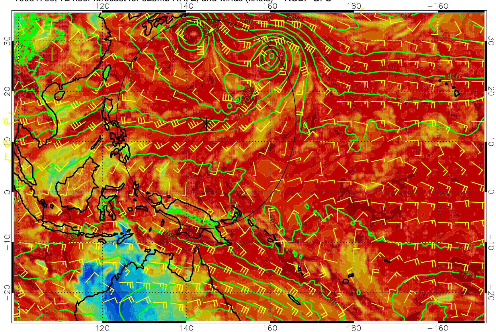
16081700, 72 hour forecast for 925mb RH, Z, and winds (knots) -- NCEP GFS
