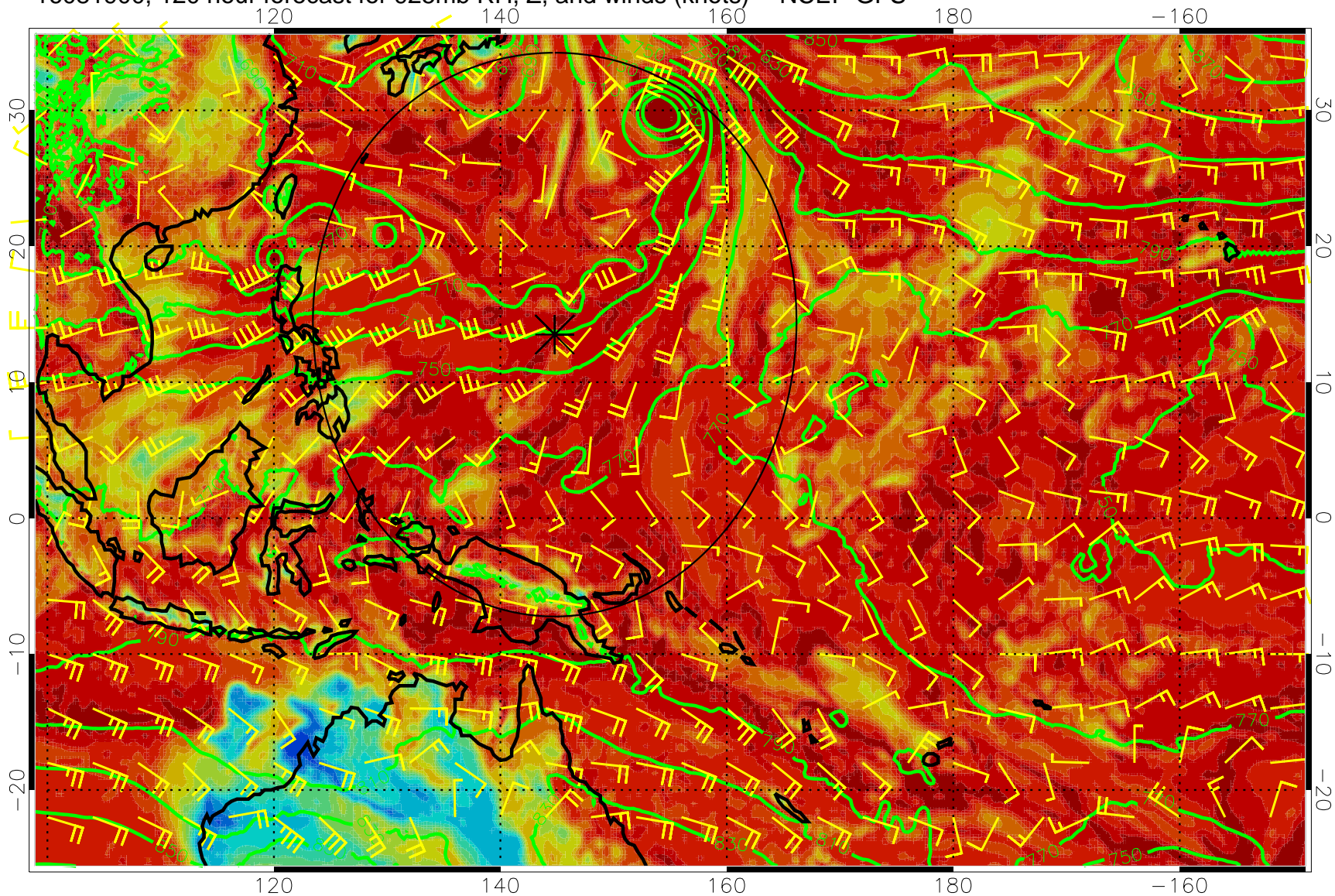
16081900, 120 hour forecast for 925mb RH, Z, and winds (knots) -- NCEP GFS
