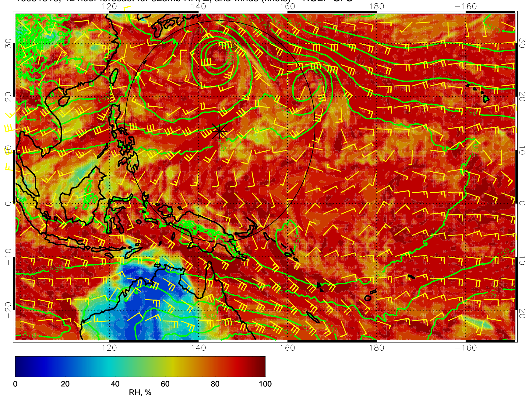
16081518, 42 hour forecast for 925mb RH, Z, and winds (knots) -- NCEP GFS
