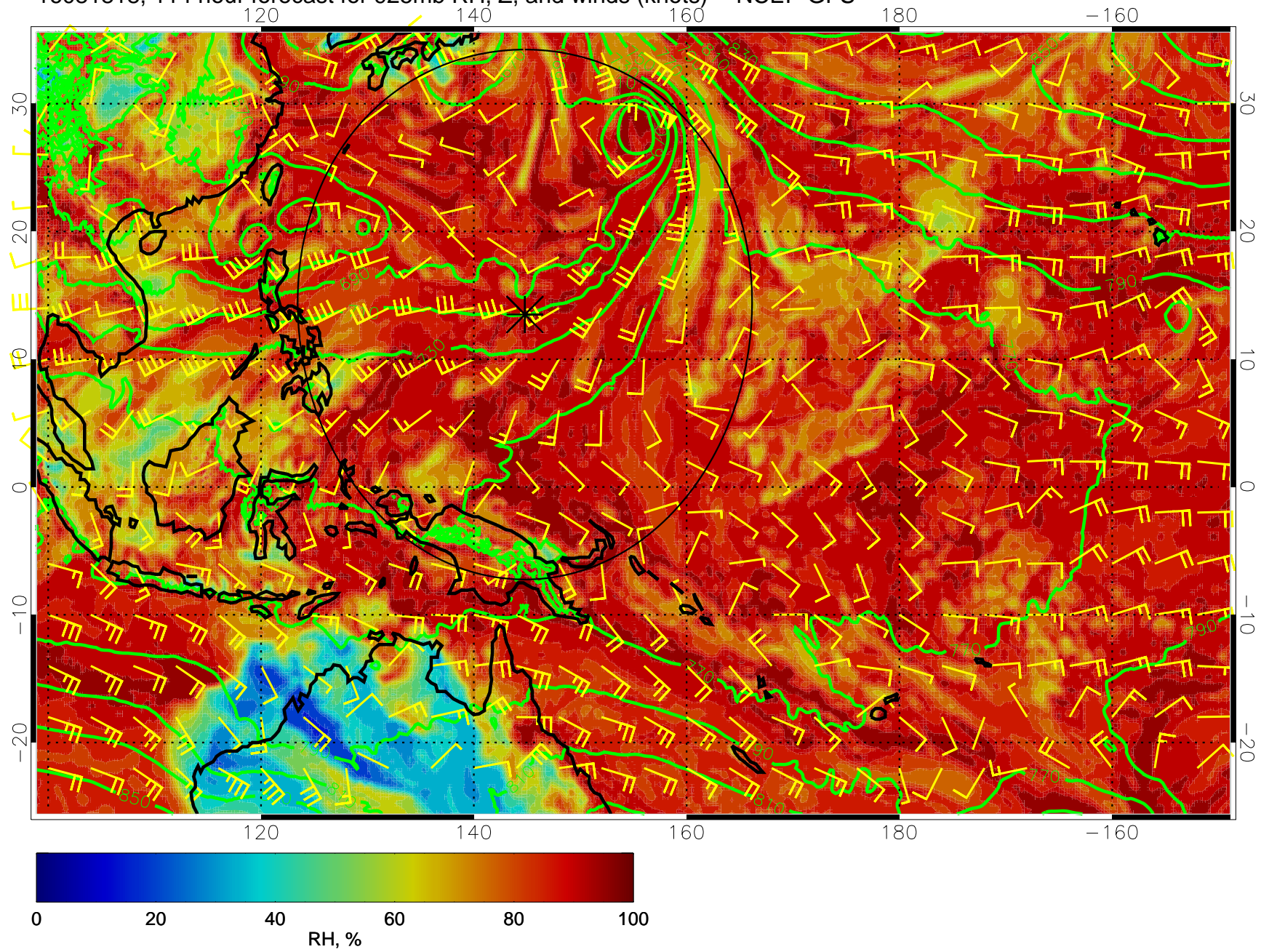
16081818, 114 hour forecast for 925mb RH, Z, and winds (knots) -- NCEP GFS
