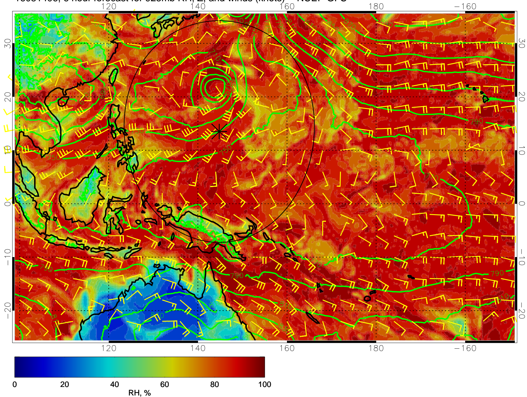
16081406, 6 hour forecast for 925mb RH, Z, and winds (knots) -- NCEP GFS
