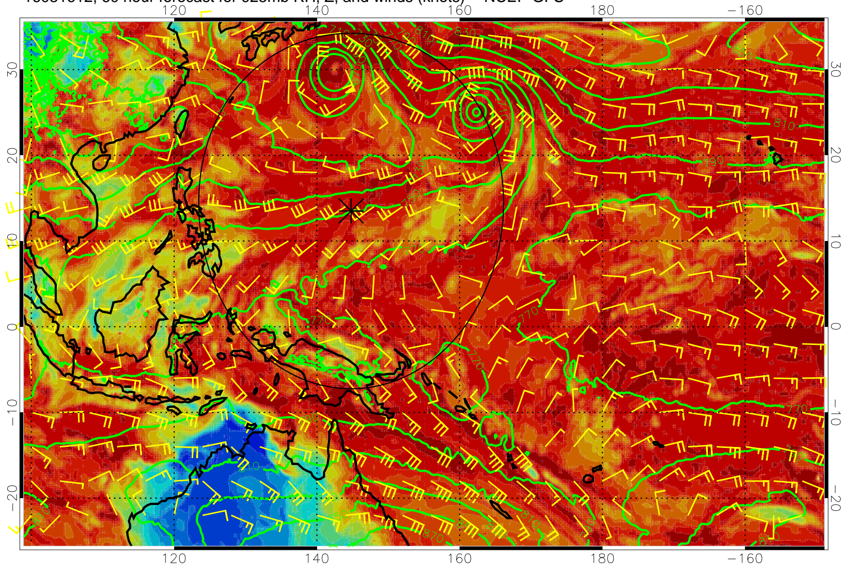
16081612, 60 hour forecast for 925mb RH, Z, and winds (knots) -- NCEP GFS
