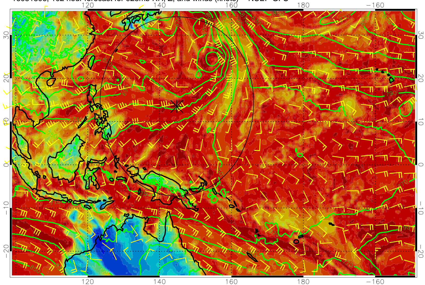
16081806, 102 hour forecast for 925mb RH, Z, and winds (knots) -- NCEP GFS
