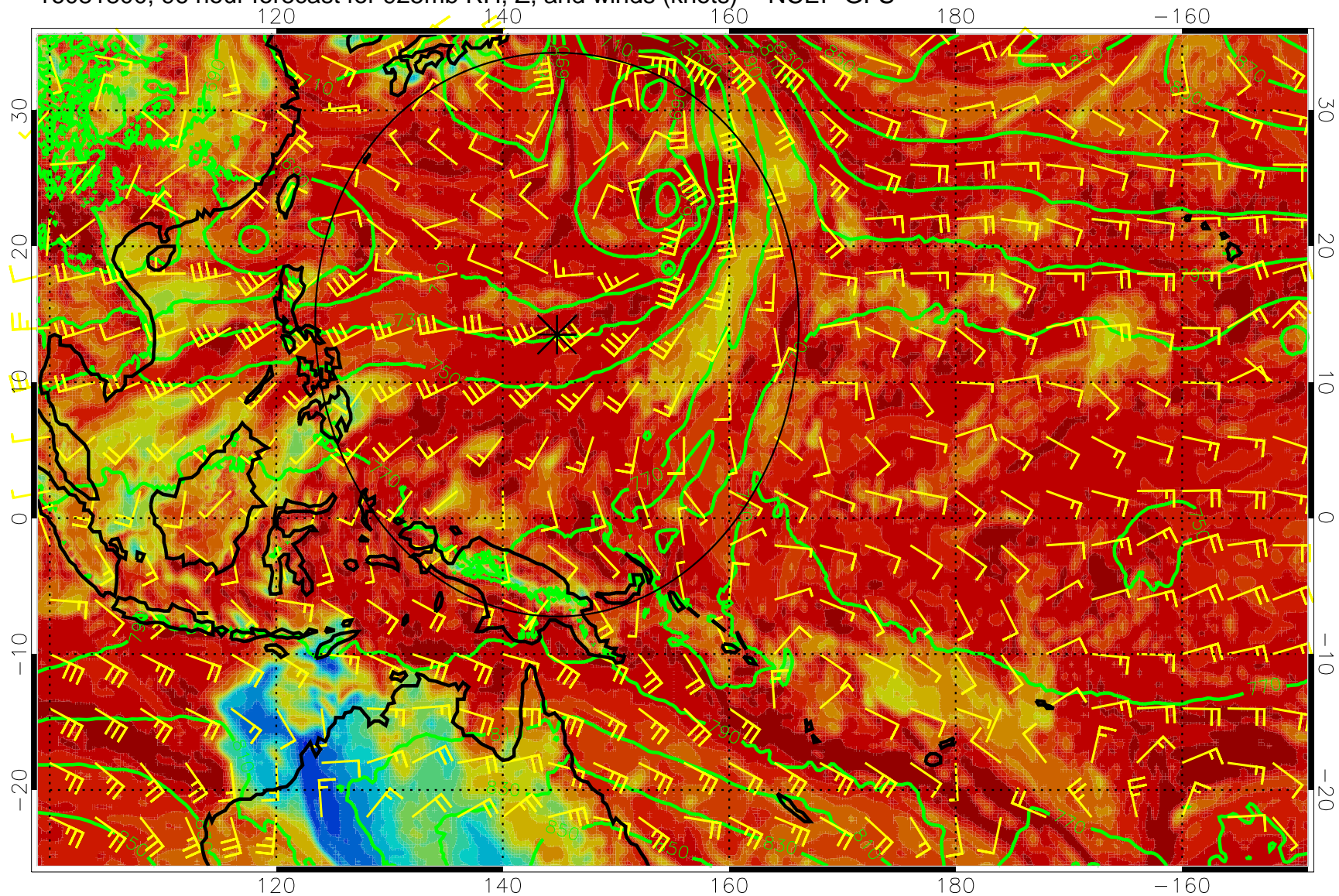
16081800, 96 hour forecast for 925mb RH, Z, and winds (knots) -- NCEP GFS
