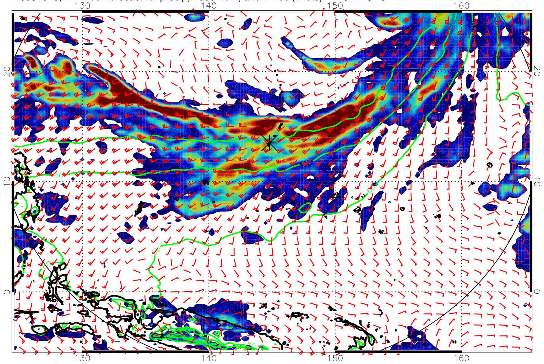
16081818, 114 hour forecast for precip, 1000mb Z, and winds (knots) -- NCEP GFS
