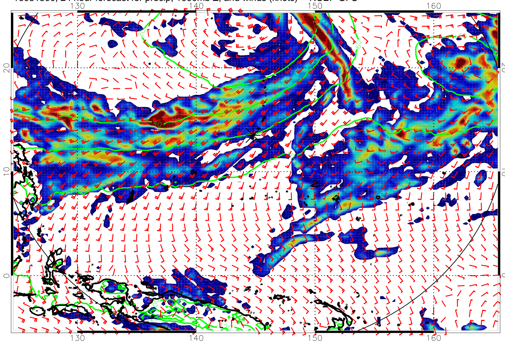
16081500, 24 hour forecast for precip, 1000mb Z, and winds (knots) -- NCEP GFS
