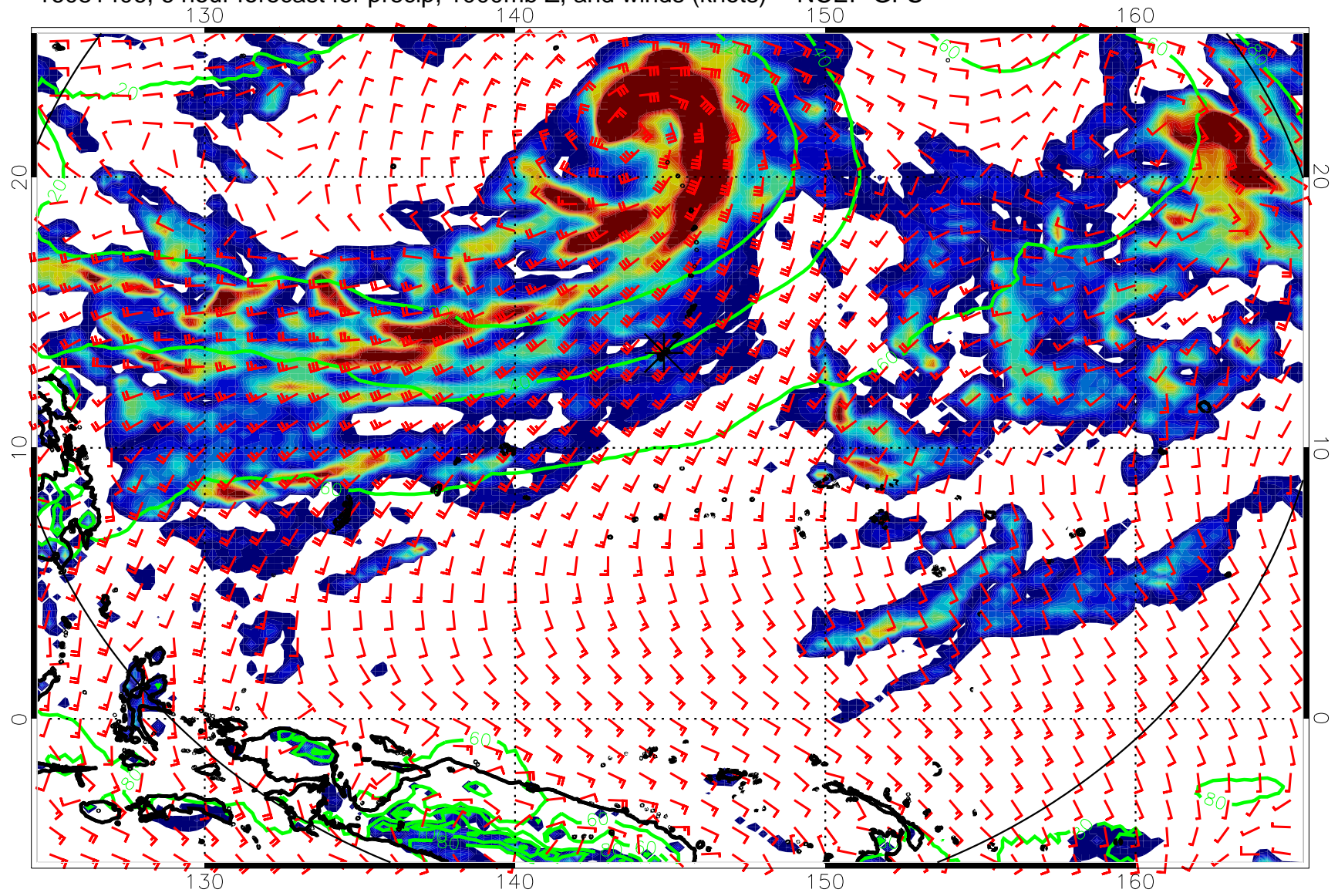
16081406, 6 hour forecast for precip, 1000mb Z, and winds (knots) -- NCEP GFS
