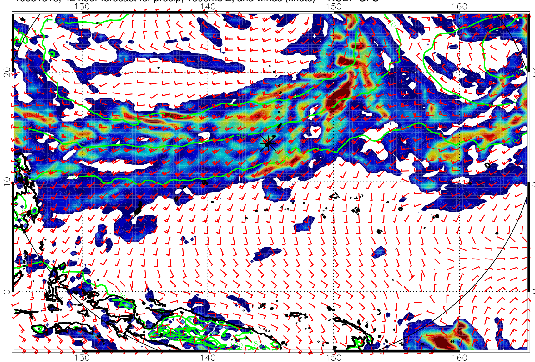
16081518, 42 hour forecast for precip, 1000mb Z, and winds (knots) -- NCEP GFS
