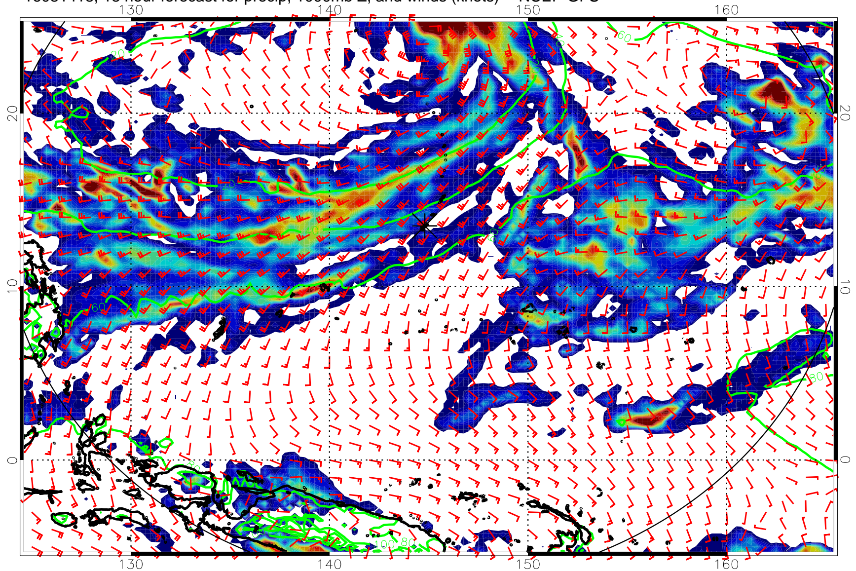
16081418, 18 hour forecast for precip, 1000mb Z, and winds (knots) -- NCEP GFS
