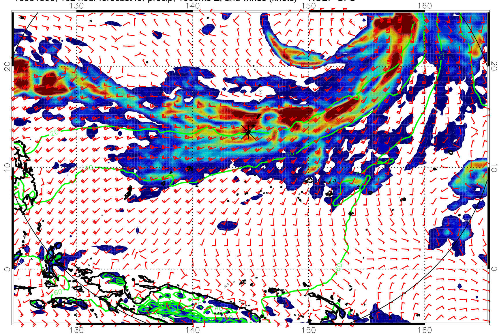
16081806, 102 hour forecast for precip, 1000mb Z, and winds (knots) -- NCEP GFS
