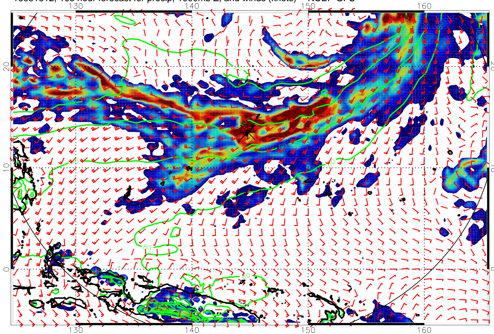
16081812, 108 hour forecast for precip, 1000mb Z, and winds (knots) -- NCEP GFS
