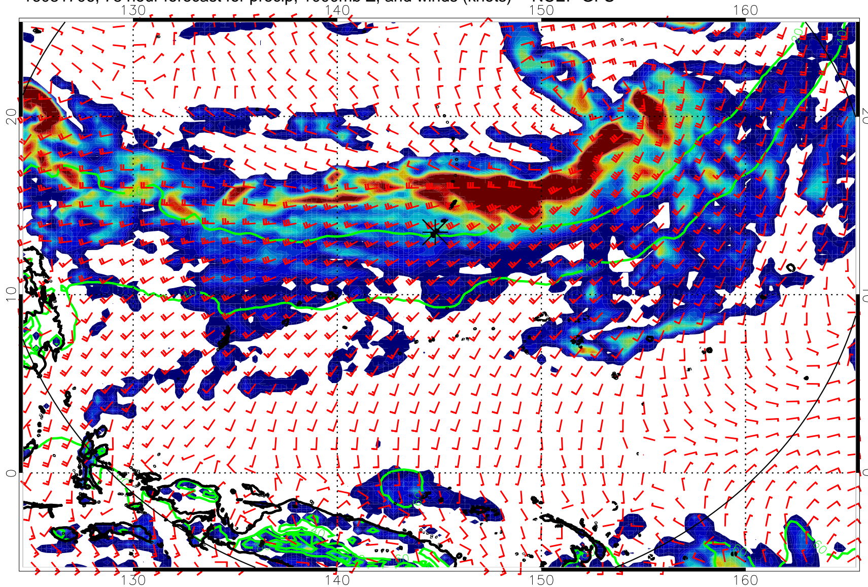
16081706, 78 hour forecast for precip, 1000mb Z, and winds (knots) -- NCEP GFS
