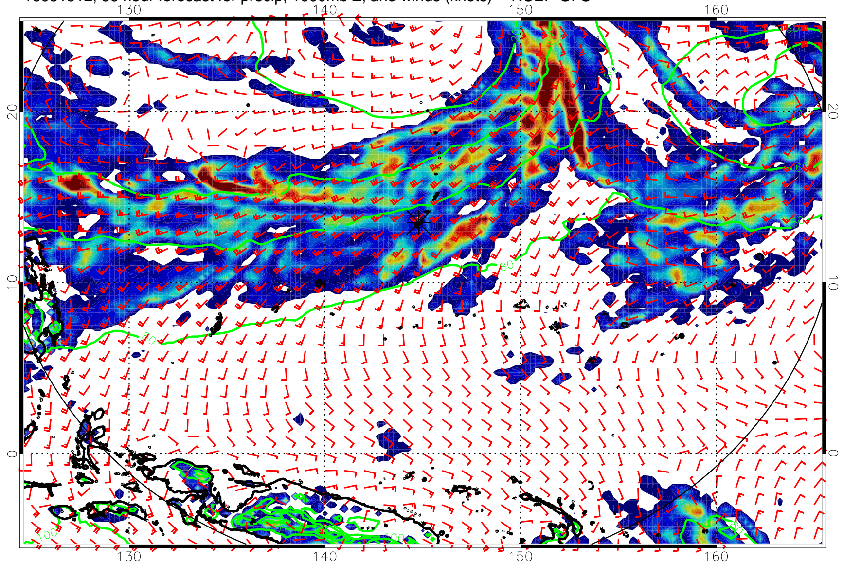
16081512, 36 hour forecast for precip, 1000mb Z, and winds (knots) -- NCEP GFS
