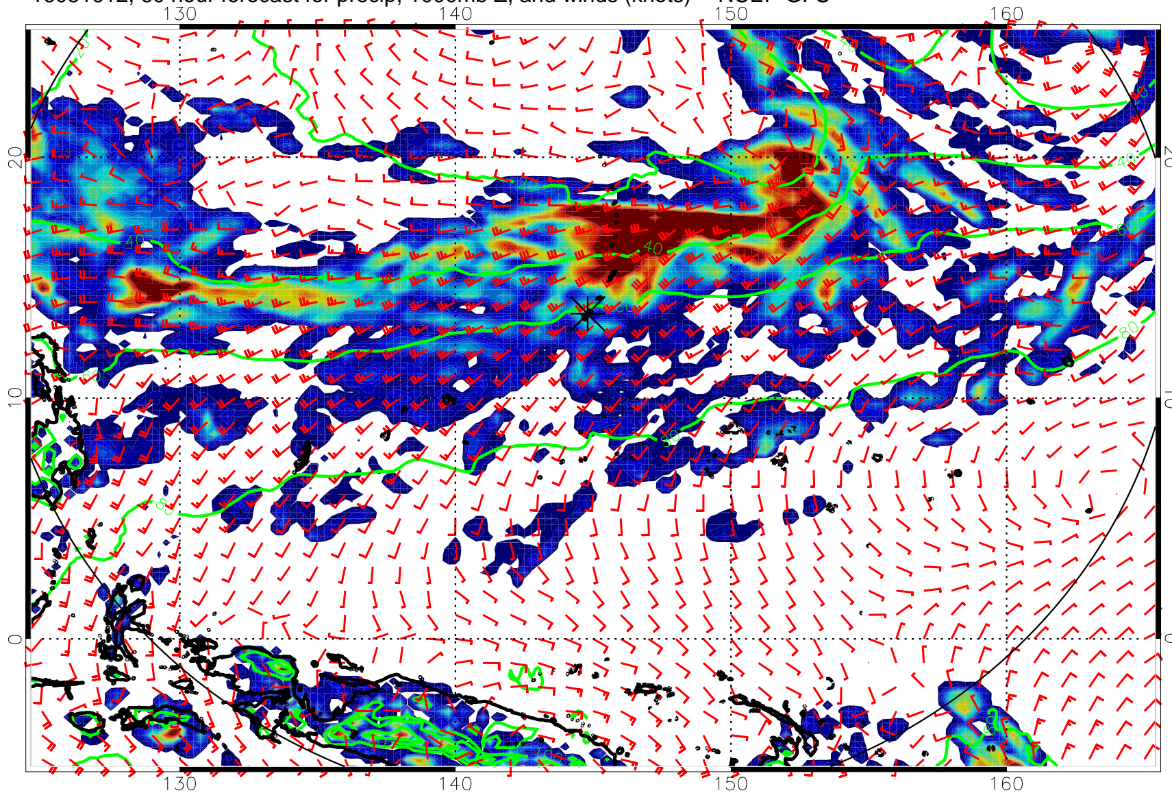
16081612, 60 hour forecast for precip, 1000mb Z, and winds (knots) -- NCEP GFS
