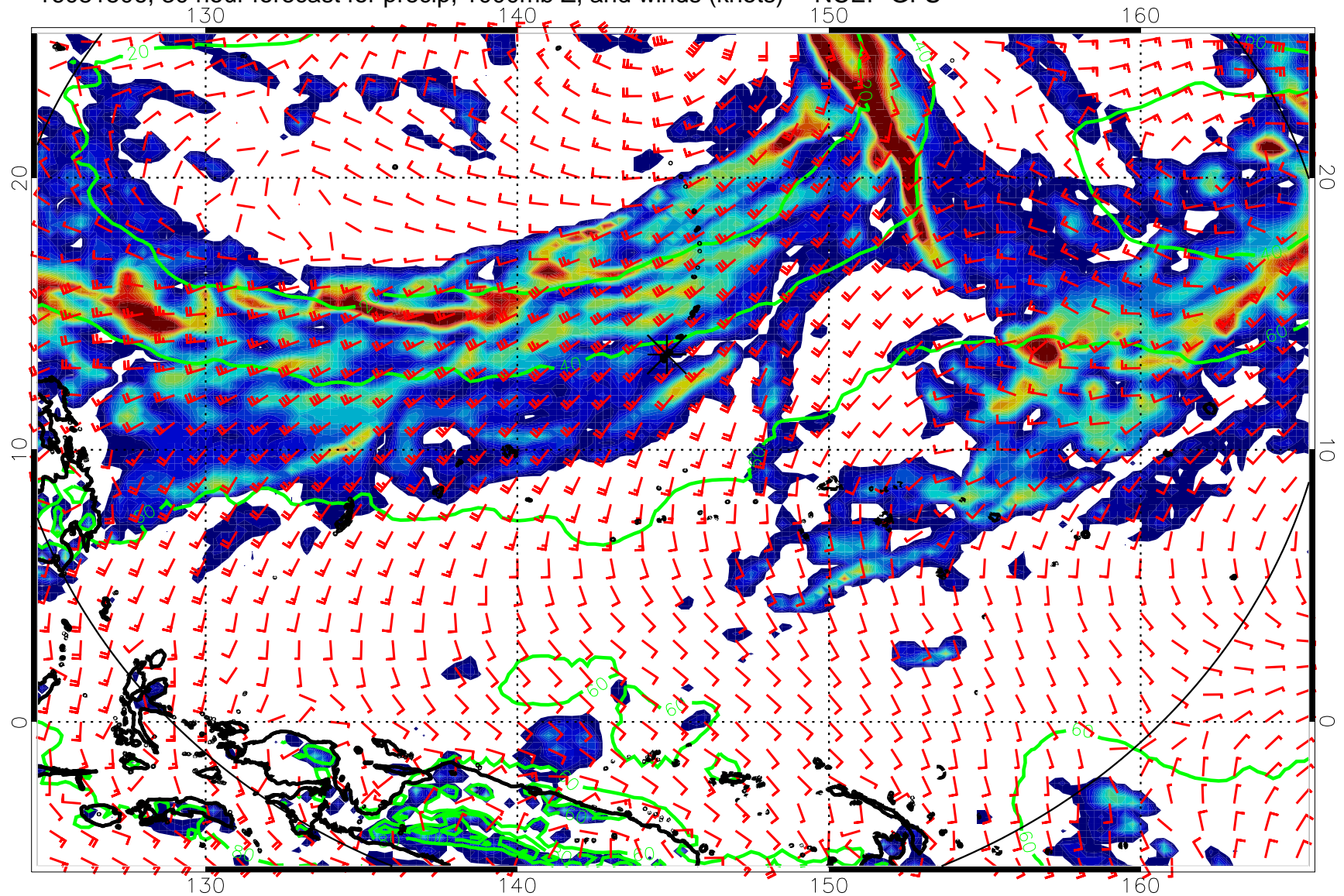
16081506, 30 hour forecast for precip, 1000mb Z, and winds (knots) -- NCEP GFS
