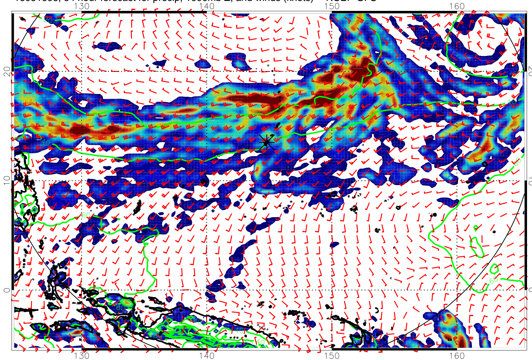
16081606, 54 hour forecast for precip, 1000mb Z, and winds (knots) -- NCEP GFS
