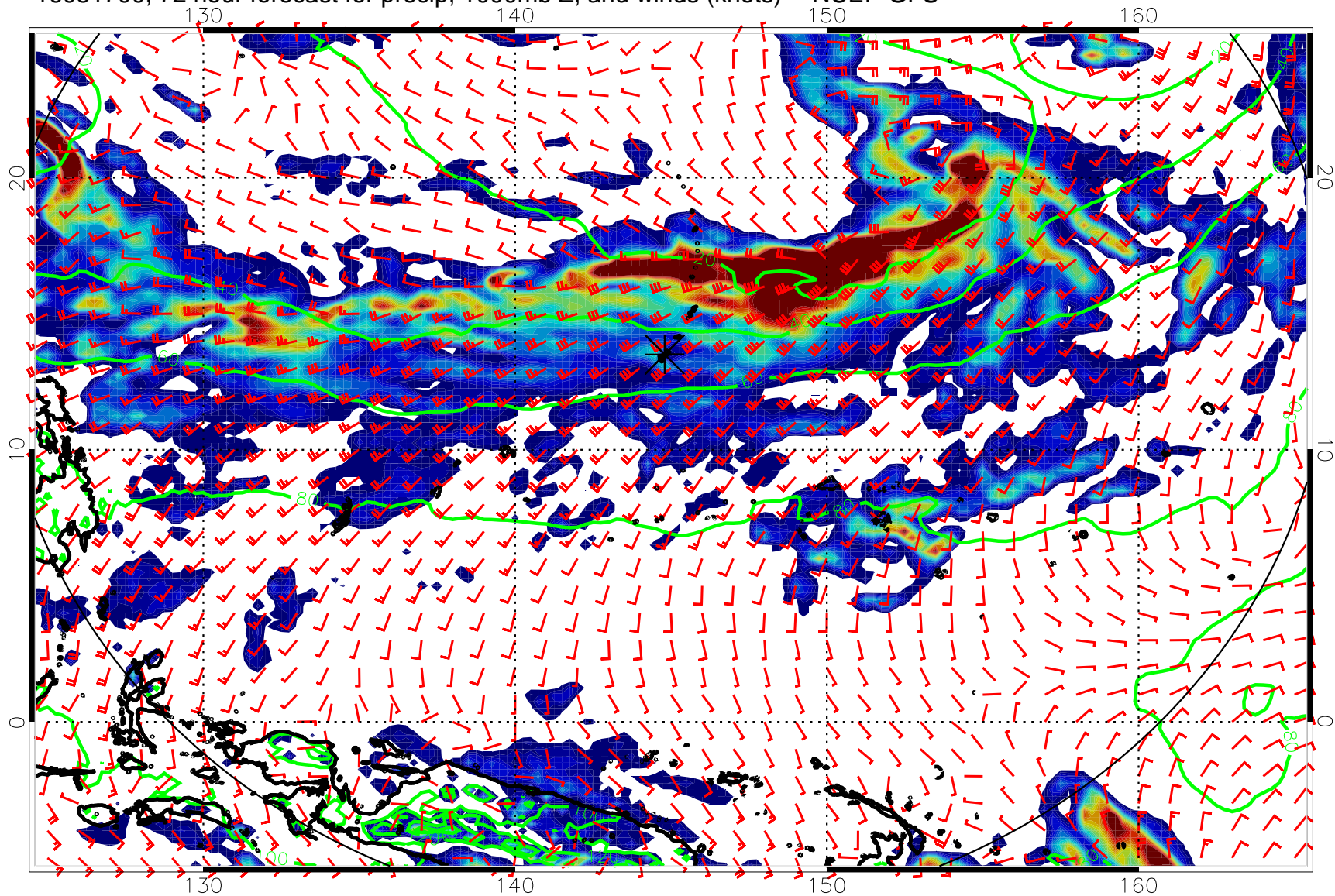
16081700, 72 hour forecast for precip, 1000mb Z, and winds (knots) -- NCEP GFS
