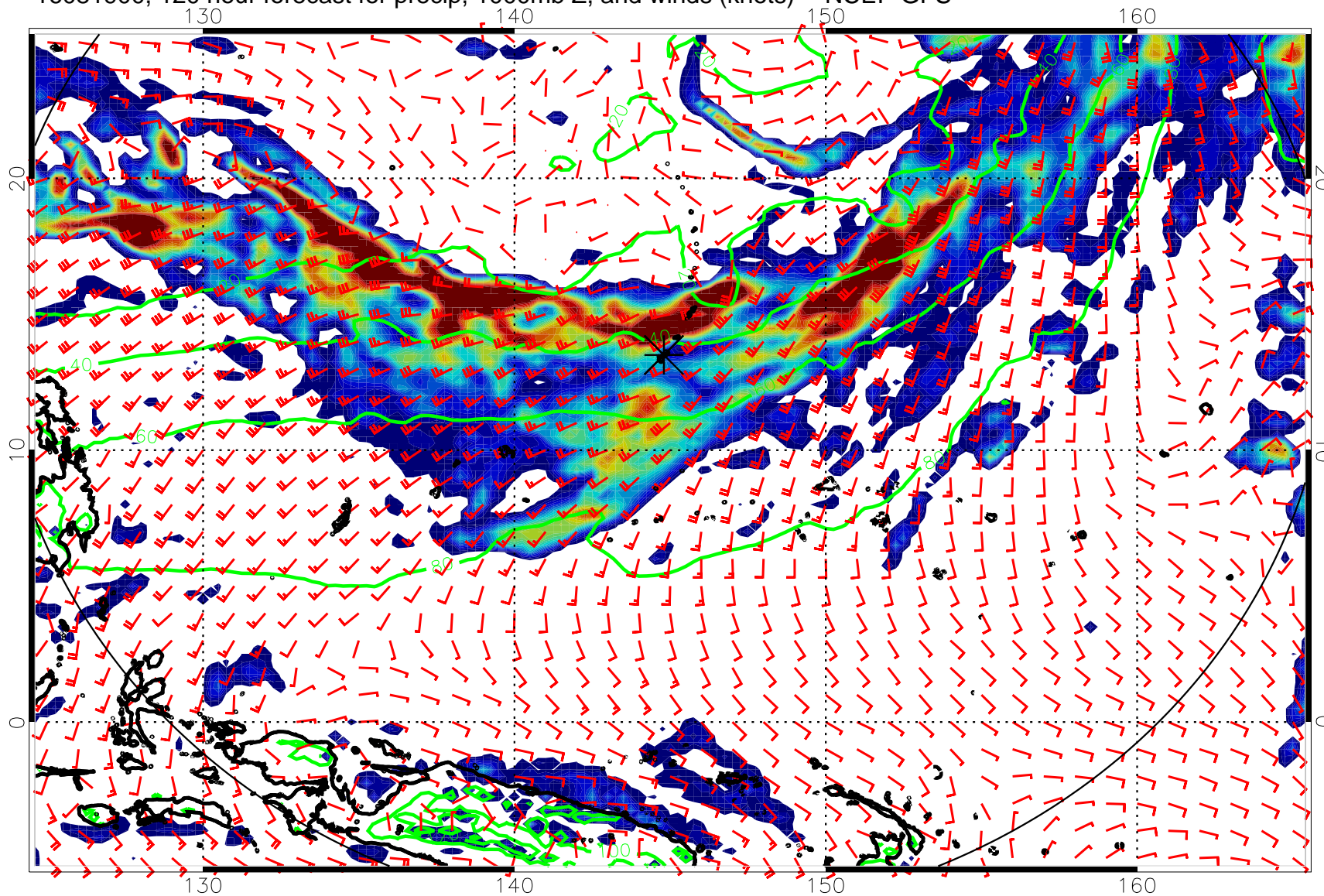
16081900, 120 hour forecast for precip, 1000mb Z, and winds (knots) -- NCEP GFS
