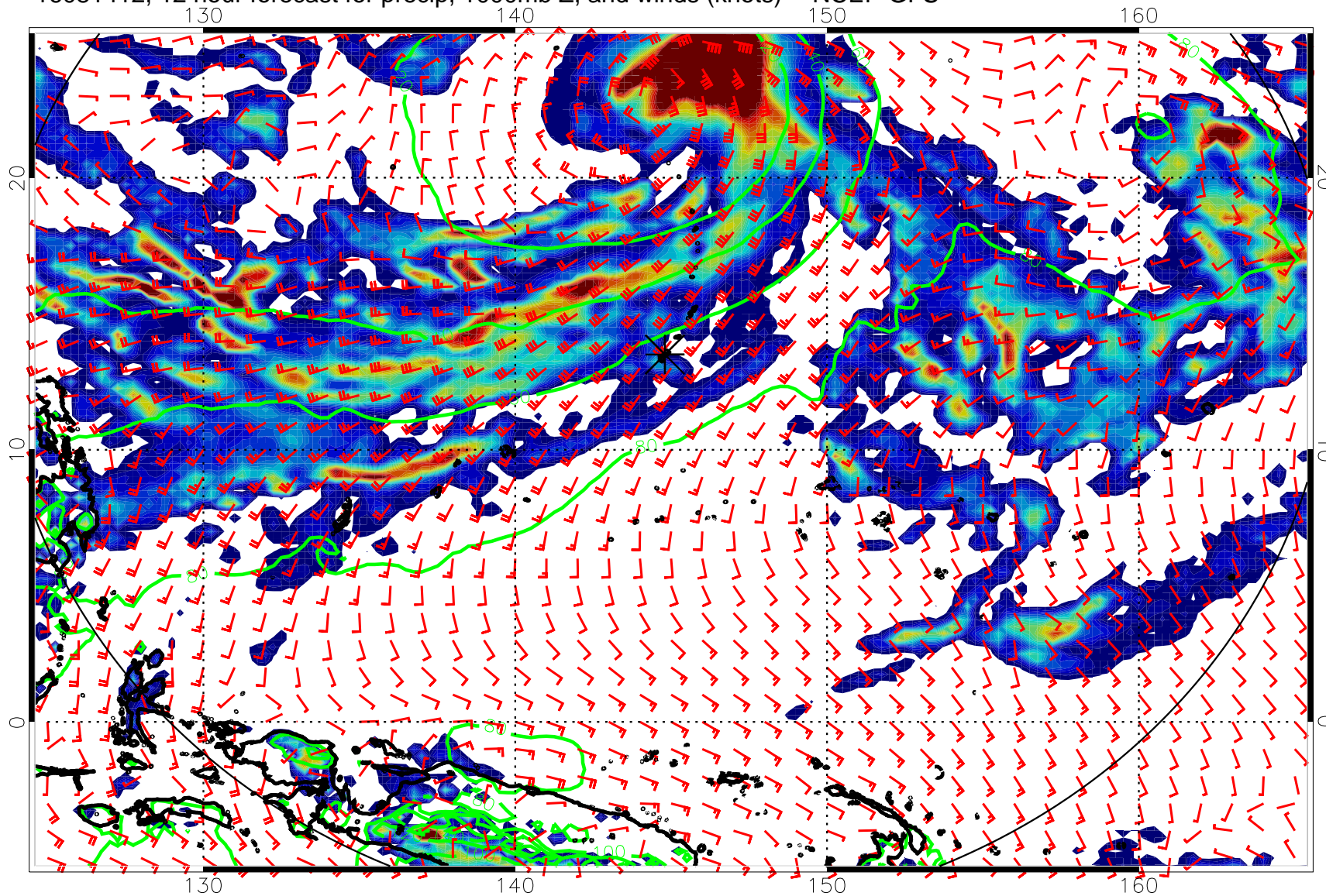
16081412, 12 hour forecast for precip, 1000mb Z, and winds (knots) -- NCEP GFS
