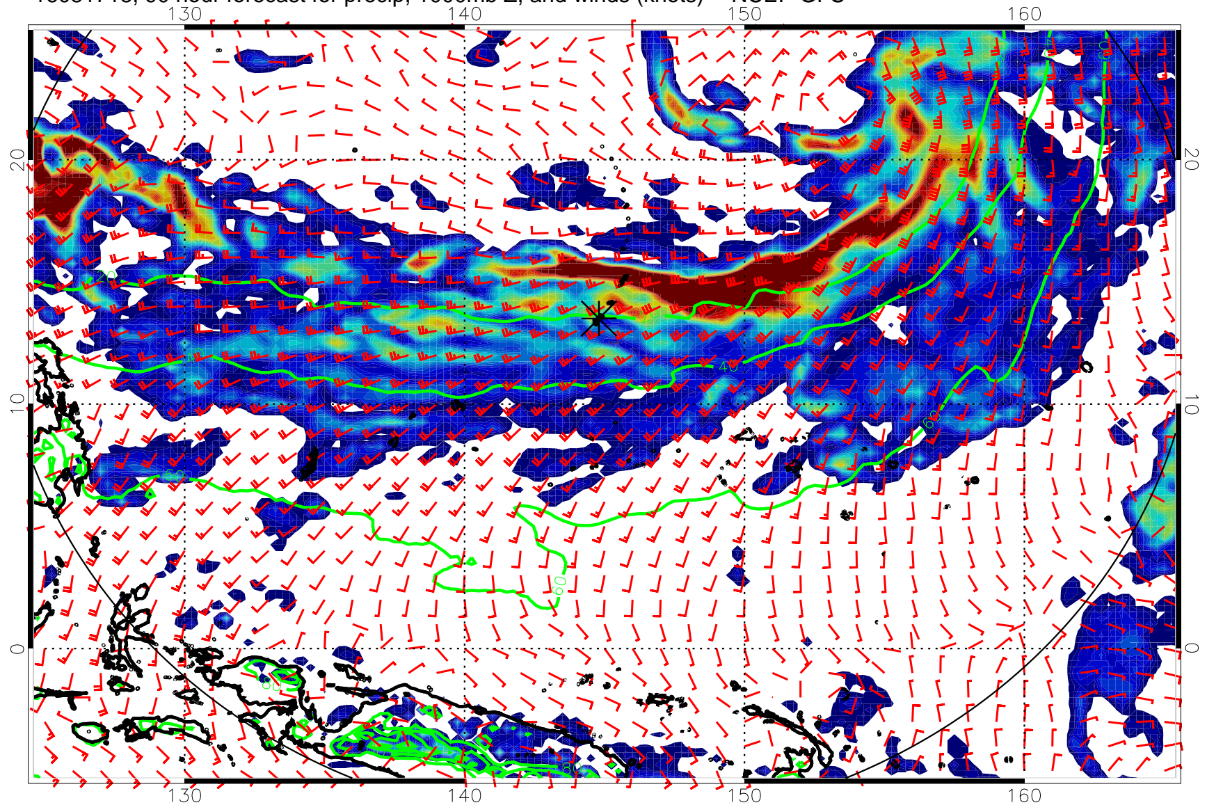
16081718, 90 hour forecast for precip, 1000mb Z, and winds (knots) -- NCEP GFS
