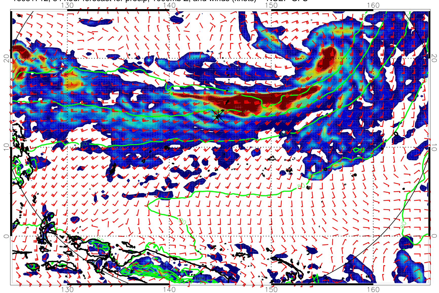
16081712, 84 hour forecast for precip, 1000mb Z, and winds (knots) -- NCEP GFS
