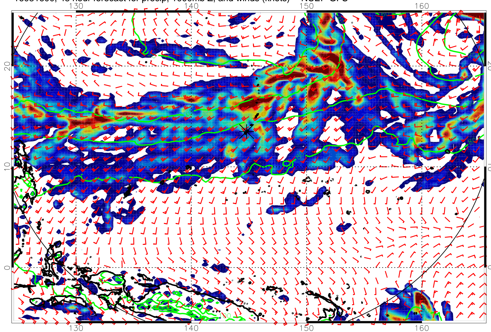
16081600, 48 hour forecast for precip, 1000mb Z, and winds (knots) -- NCEP GFS
