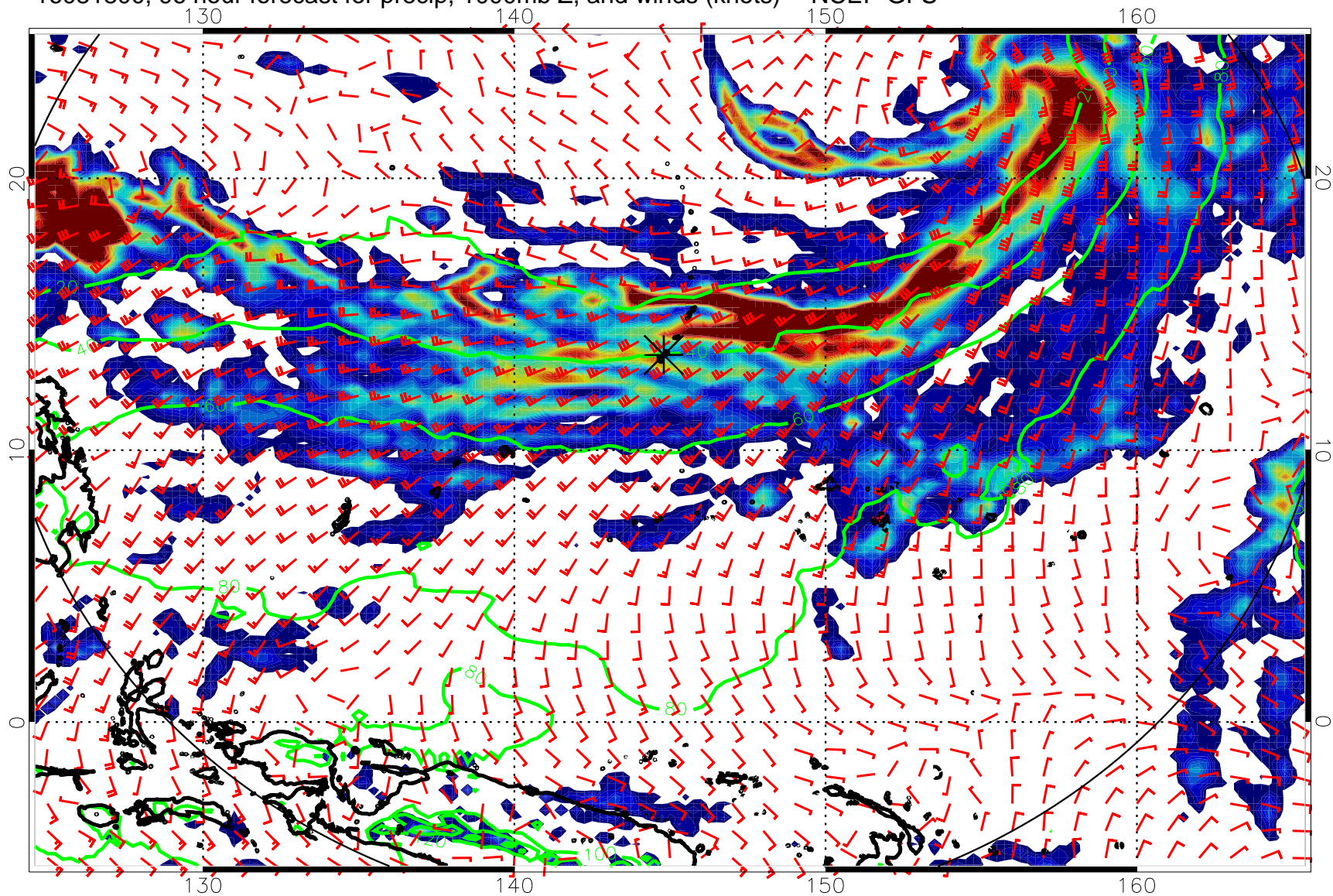
16081800, 96 hour forecast for precip, 1000mb Z, and winds (knots) -- NCEP GFS
