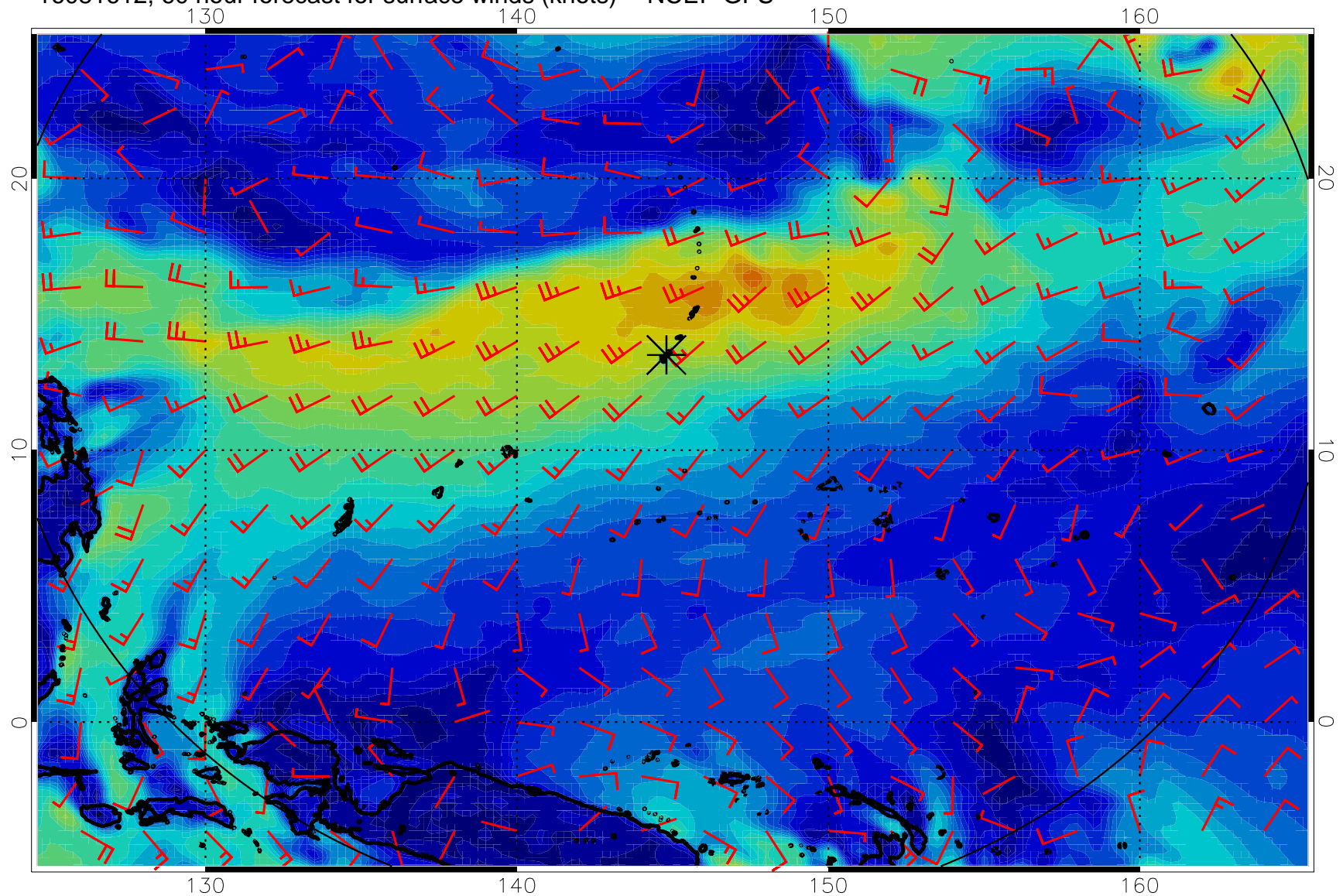
16081612, 60 hour forecast for surface winds (knots) -- NCEP GFS
