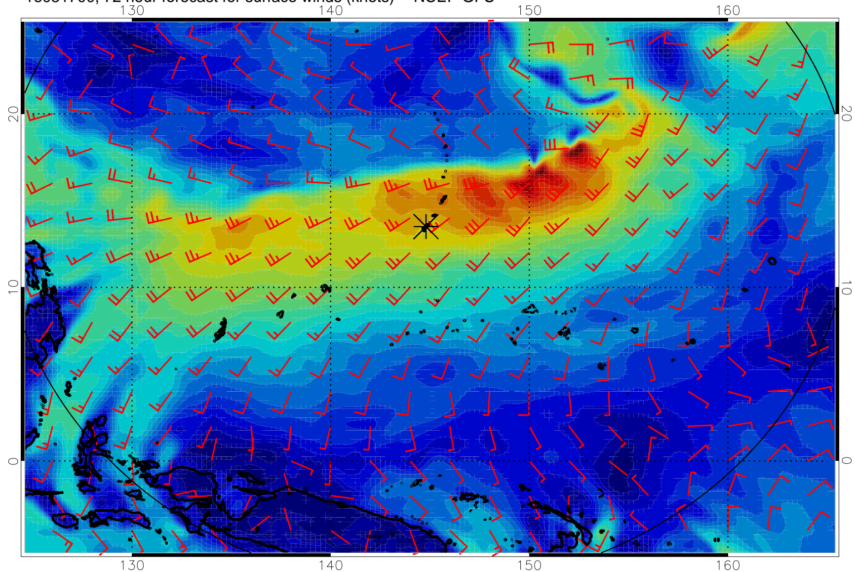
16081700, 72 hour forecast for surface winds (knots) -- NCEP GFS
