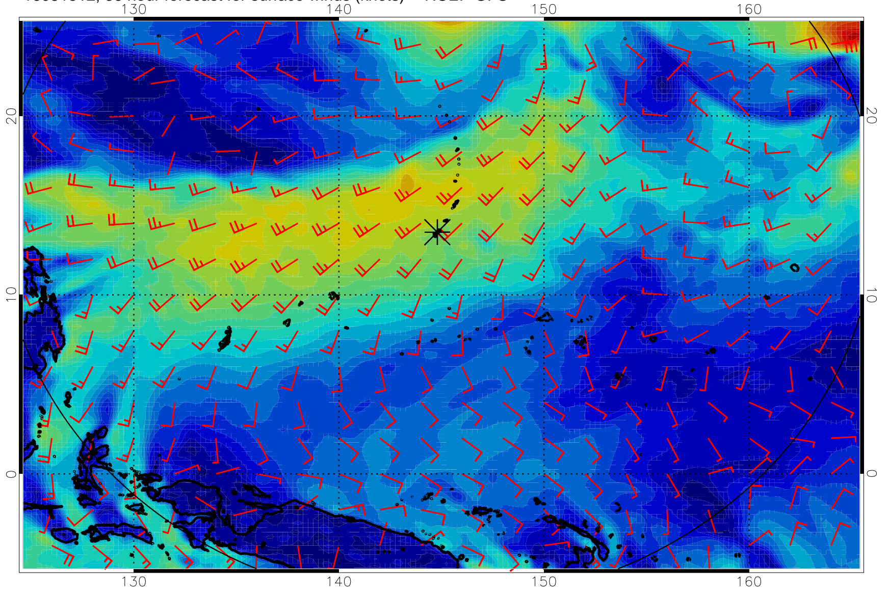
16081512, 36 hour forecast for surface winds (knots) -- NCEP GFS
