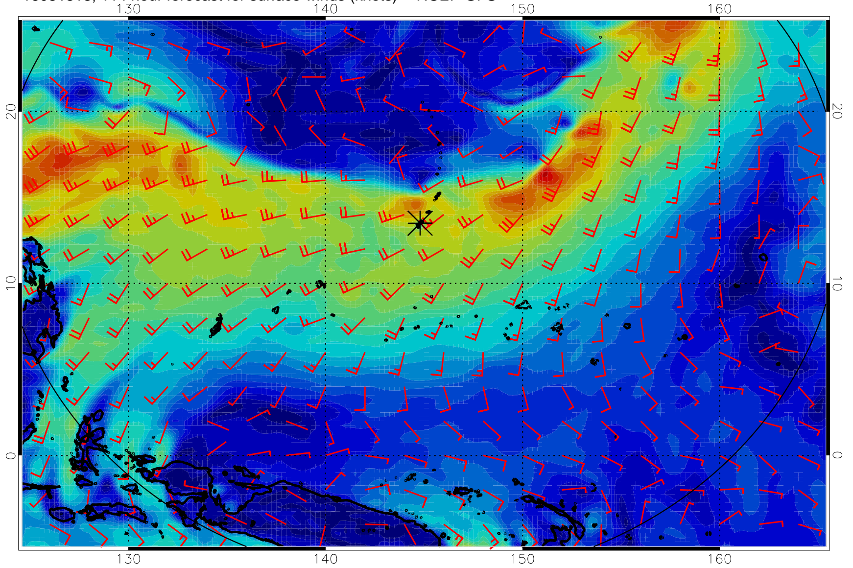
16081818, 114 hour forecast for surface winds (knots) -- NCEP GFS
