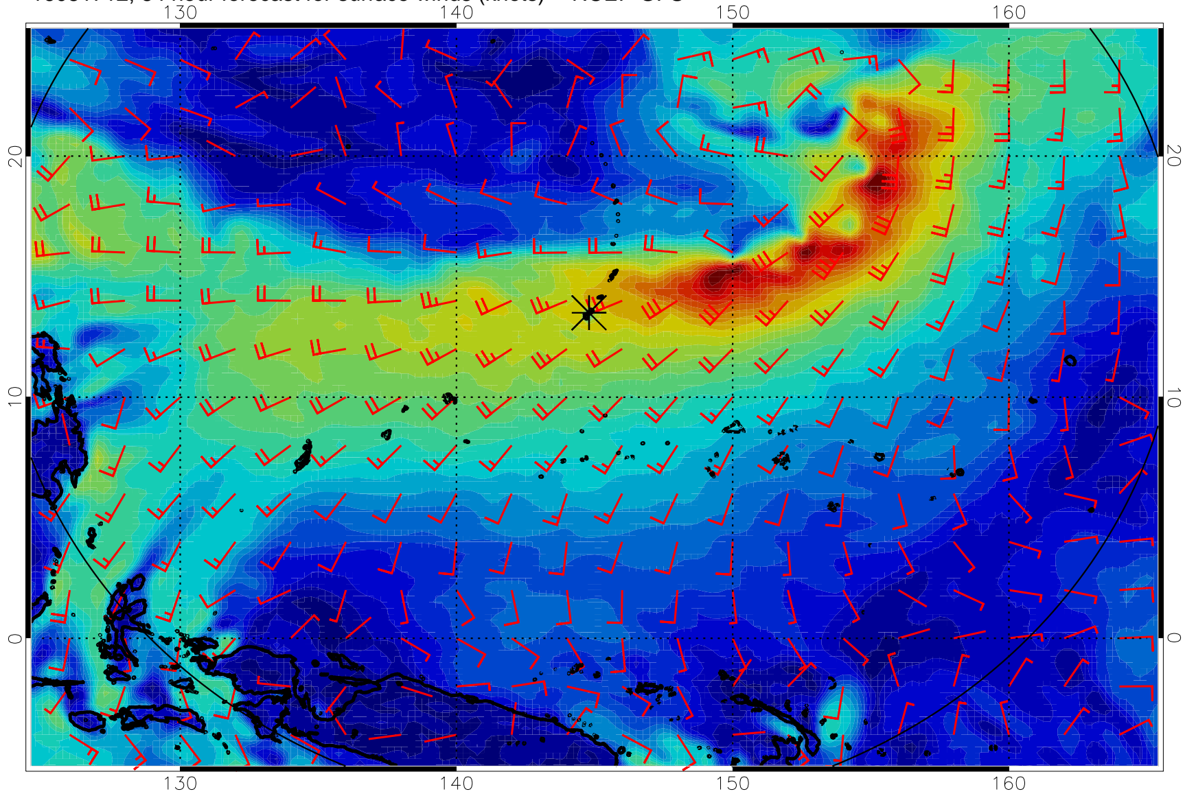
16081712, 84 hour forecast for surface winds (knots) -- NCEP GFS
