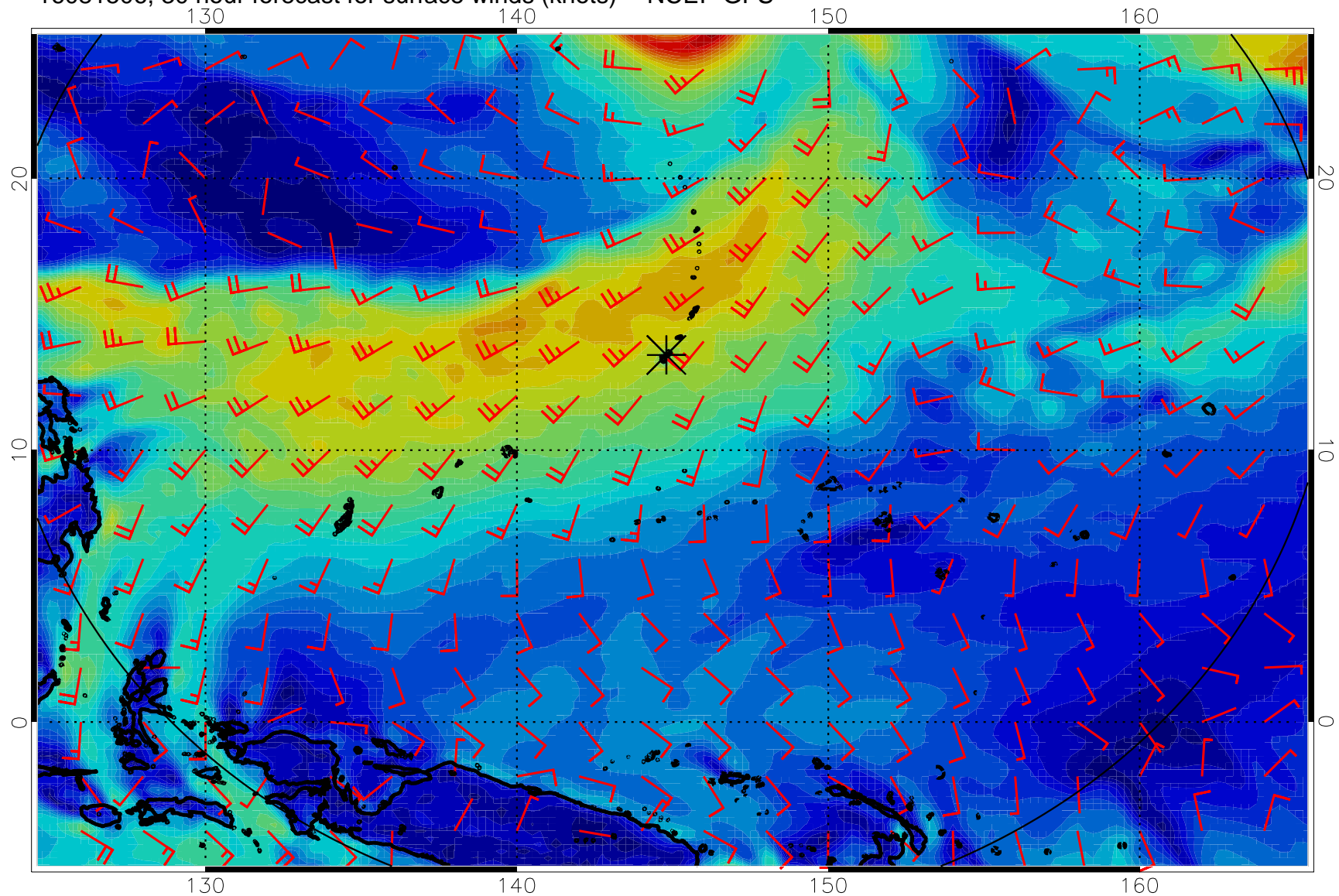
16081506, 30 hour forecast for surface winds (knots) -- NCEP GFS
