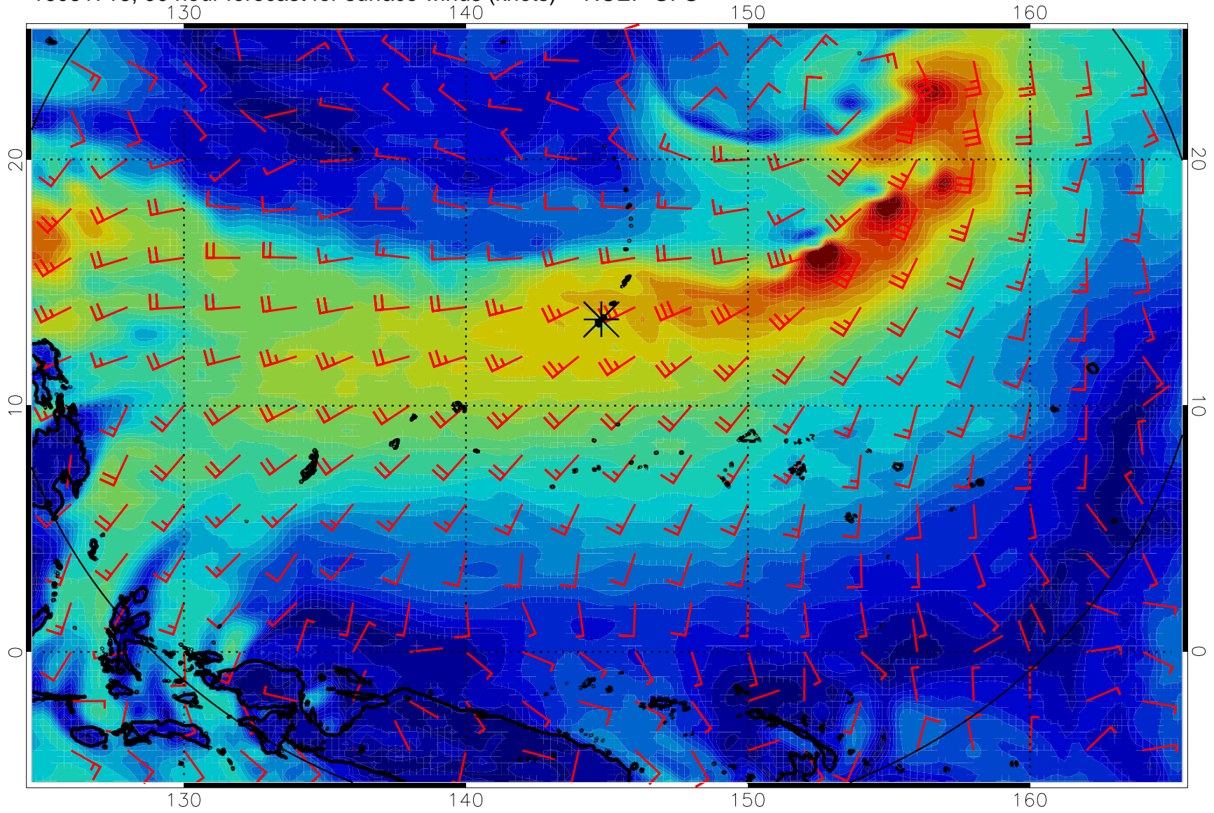
16081718, 90 hour forecast for surface winds (knots) -- NCEP GFS
