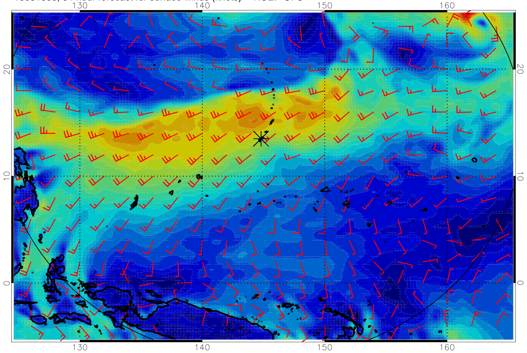
16081606, 54 hour forecast for surface winds (knots) -- NCEP GFS
