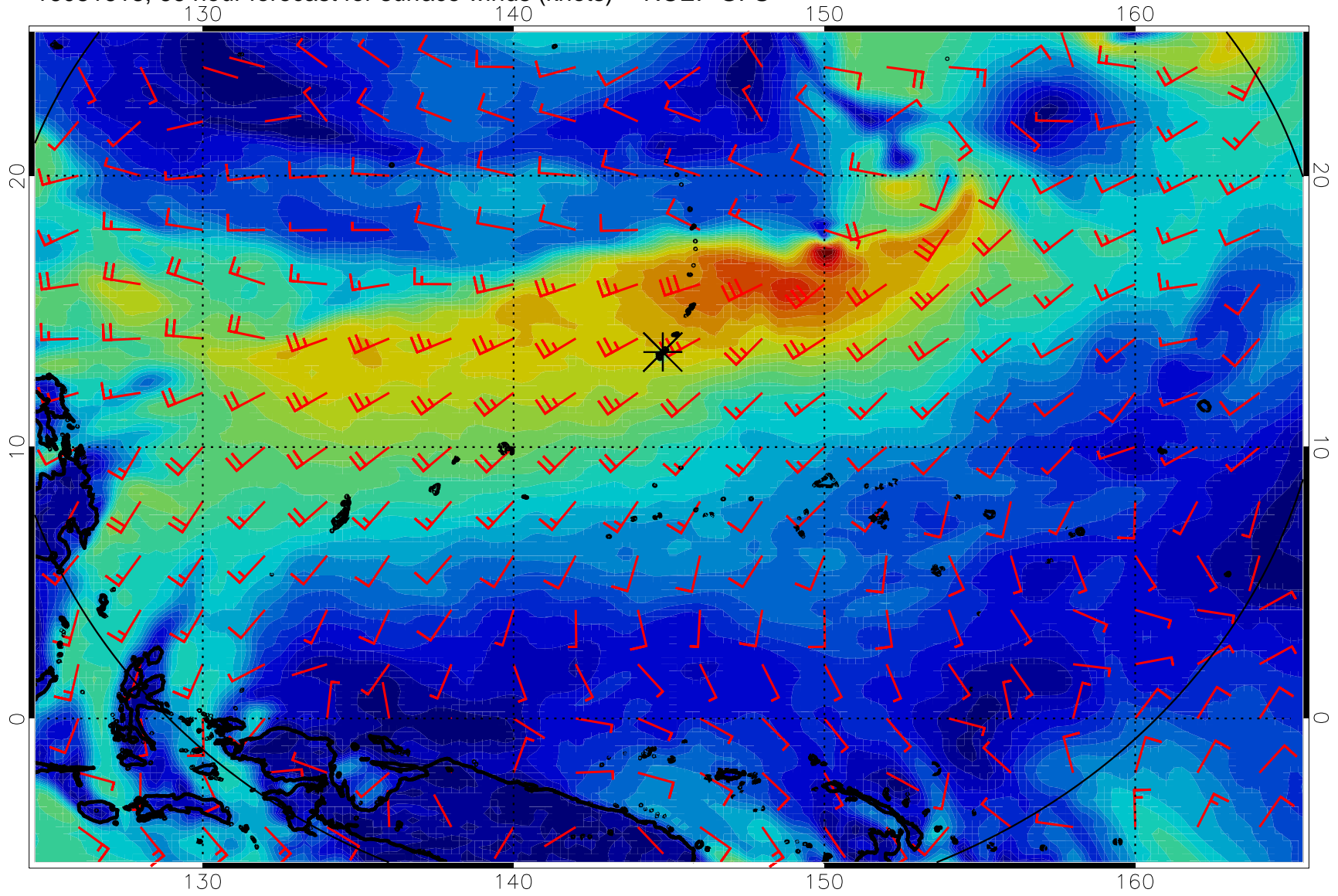
16081618, 66 hour forecast for surface winds (knots) -- NCEP GFS
