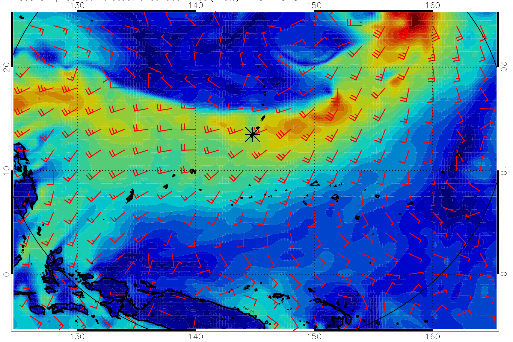
16081812, 108 hour forecast for surface winds (knots) -- NCEP GFS
