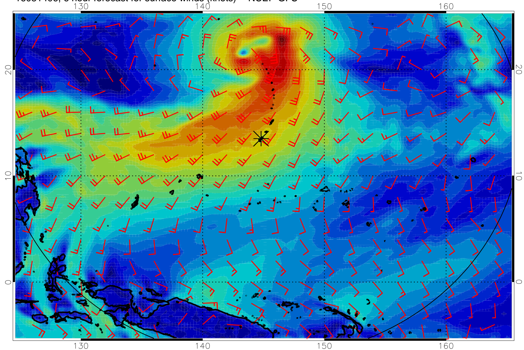
16081406, 6 hour forecast for surface winds (knots) -- NCEP GFS
