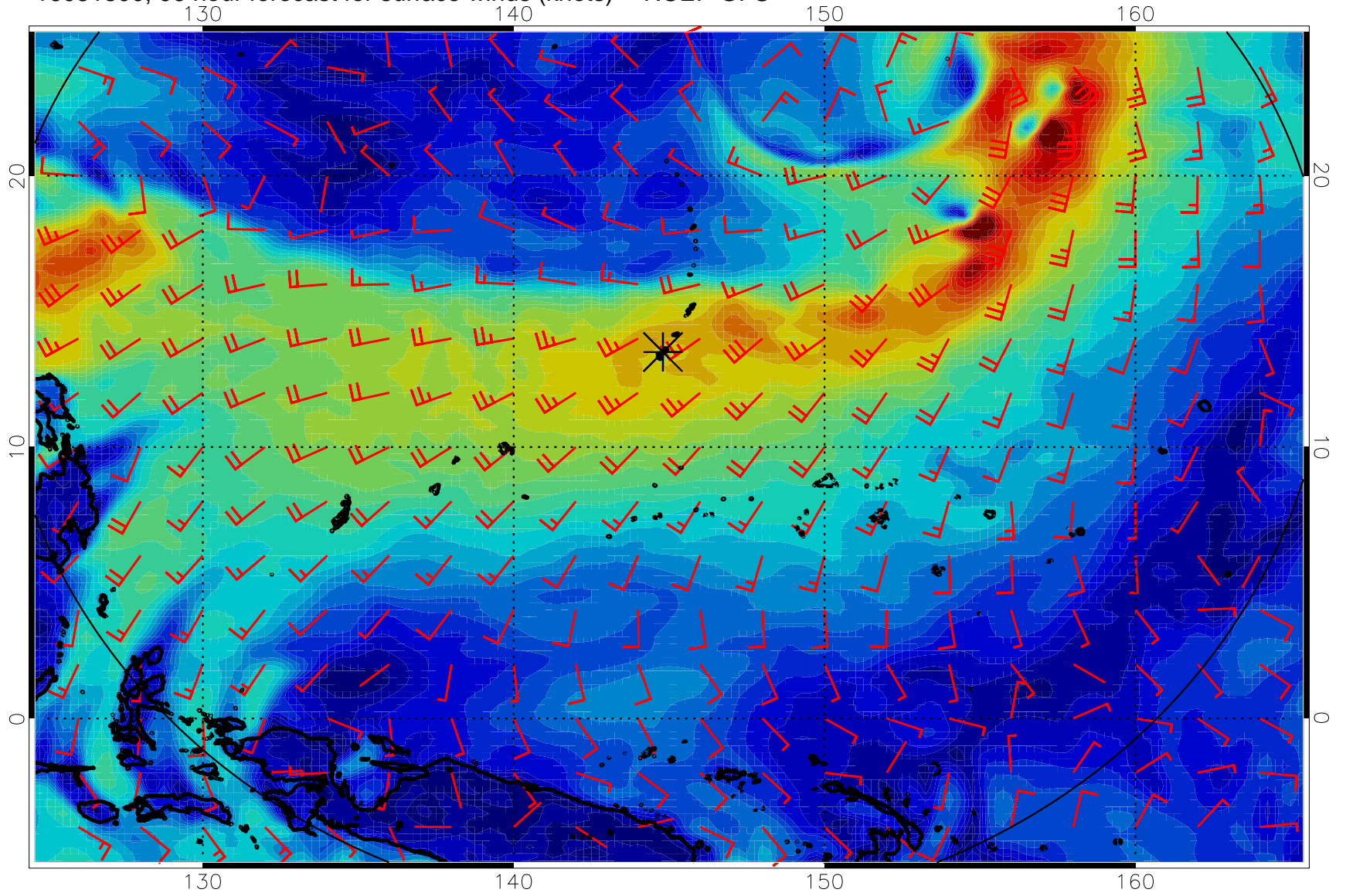
16081800, 96 hour forecast for surface winds (knots) -- NCEP GFS
