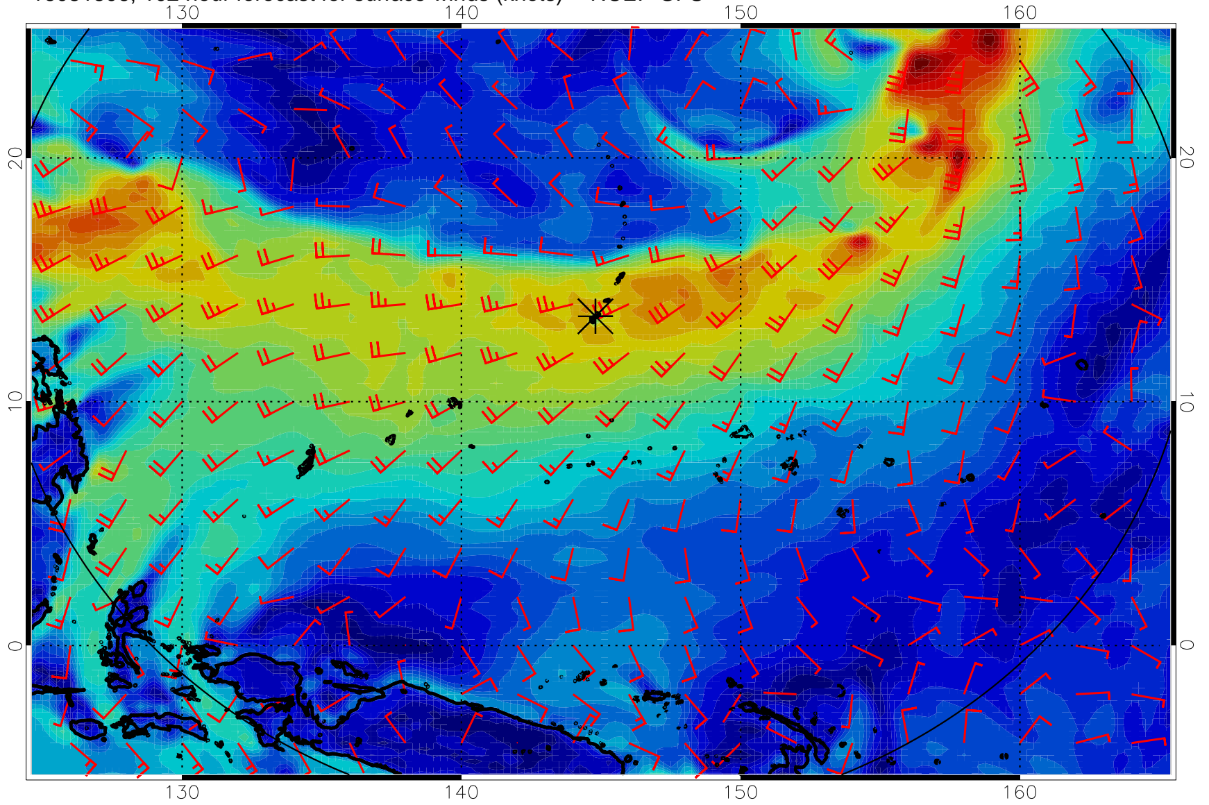
16081806, 102 hour forecast for surface winds (knots) -- NCEP GFS
