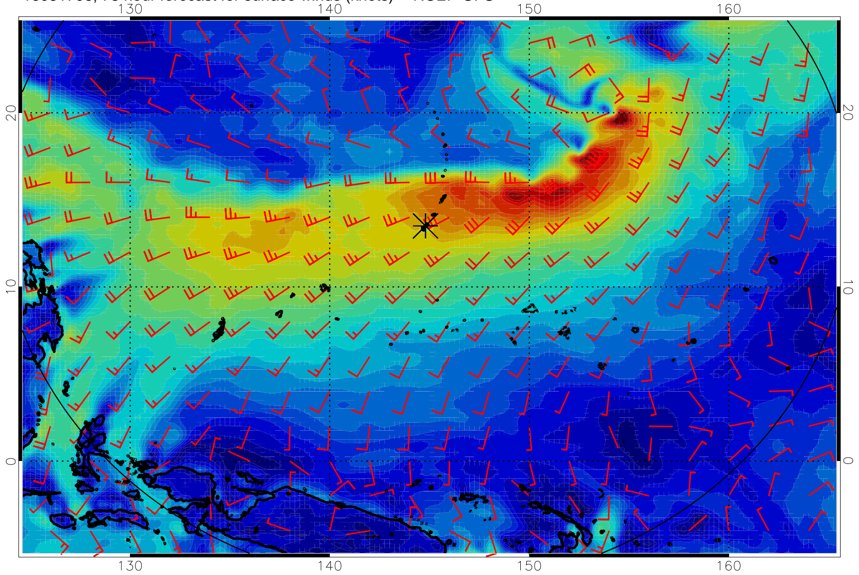
16081706, 78 hour forecast for surface winds (knots) -- NCEP GFS
