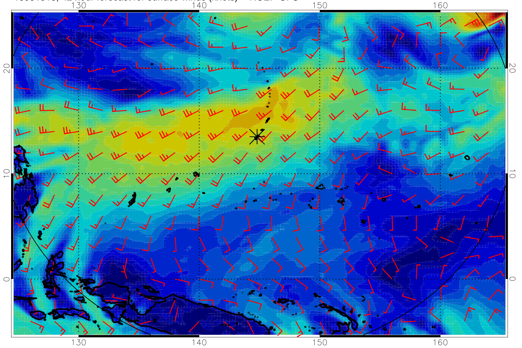
16081518, 42 hour forecast for surface winds (knots) -- NCEP GFS
