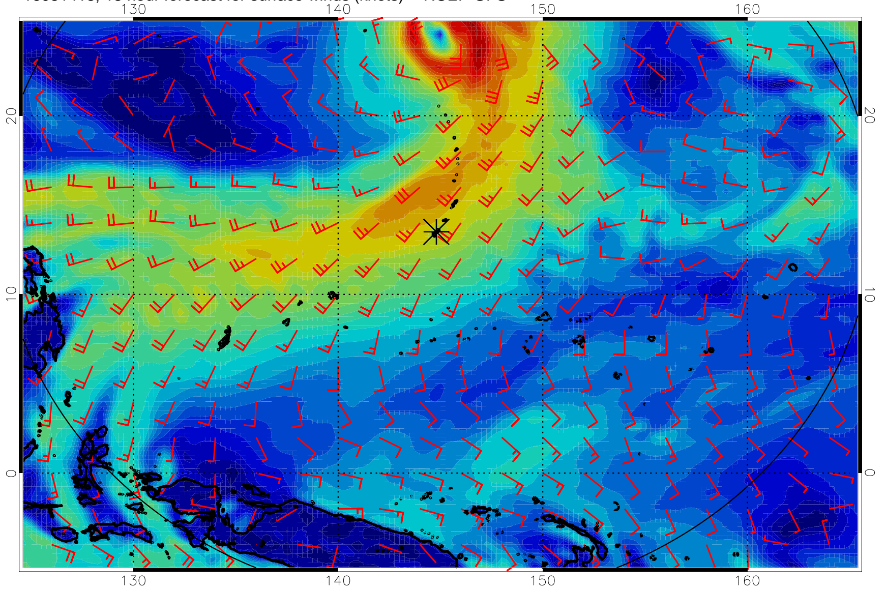
16081418, 18 hour forecast for surface winds (knots) -- NCEP GFS
