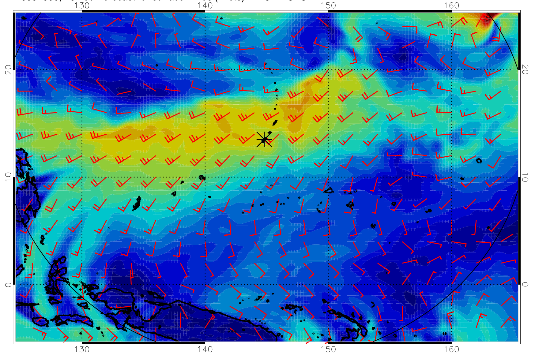
16081600, 48 hour forecast for surface winds (knots) -- NCEP GFS
