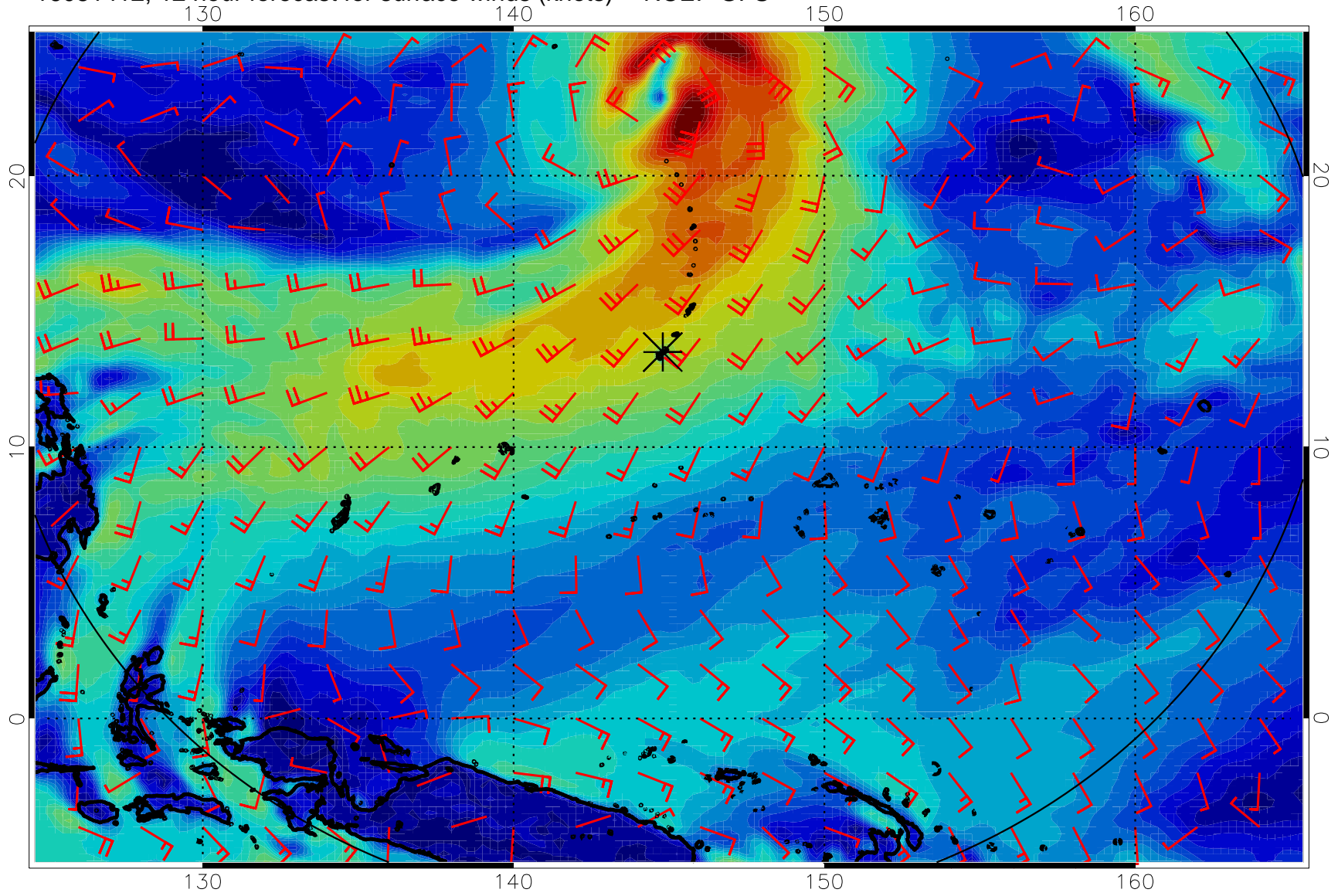
16081412, 12 hour forecast for surface winds (knots) -- NCEP GFS
