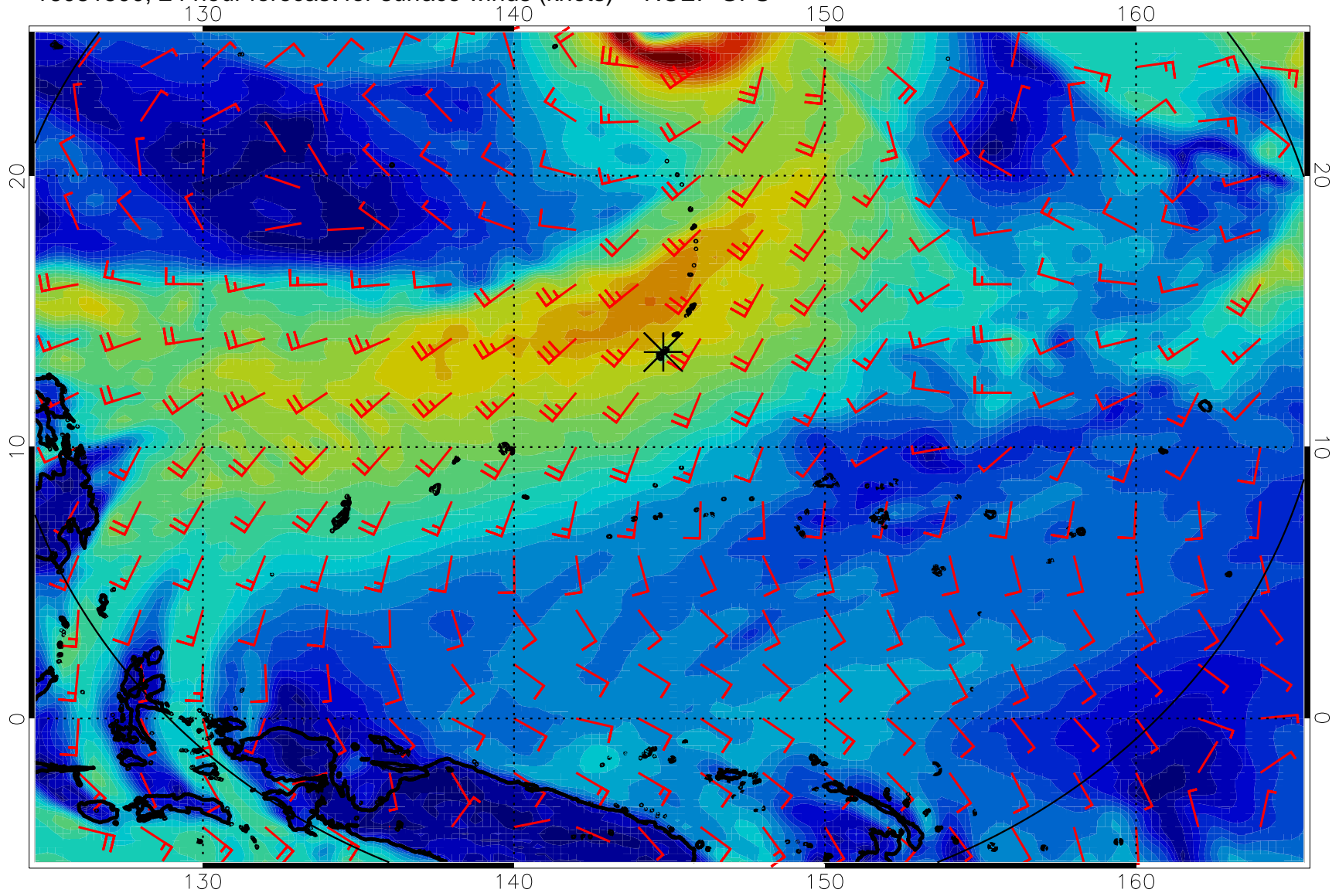
16081500, 24 hour forecast for surface winds (knots) -- NCEP GFS
