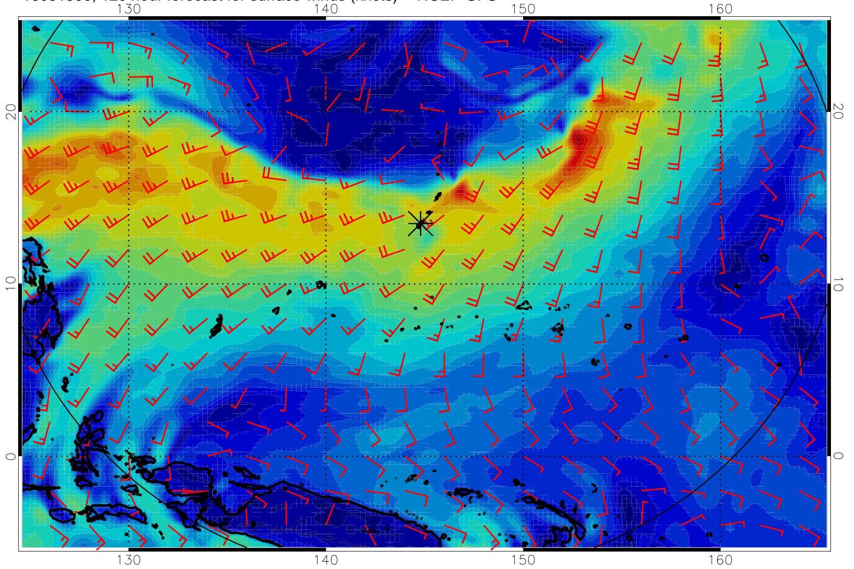
16081900, 120 hour forecast for surface winds (knots) -- NCEP GFS
