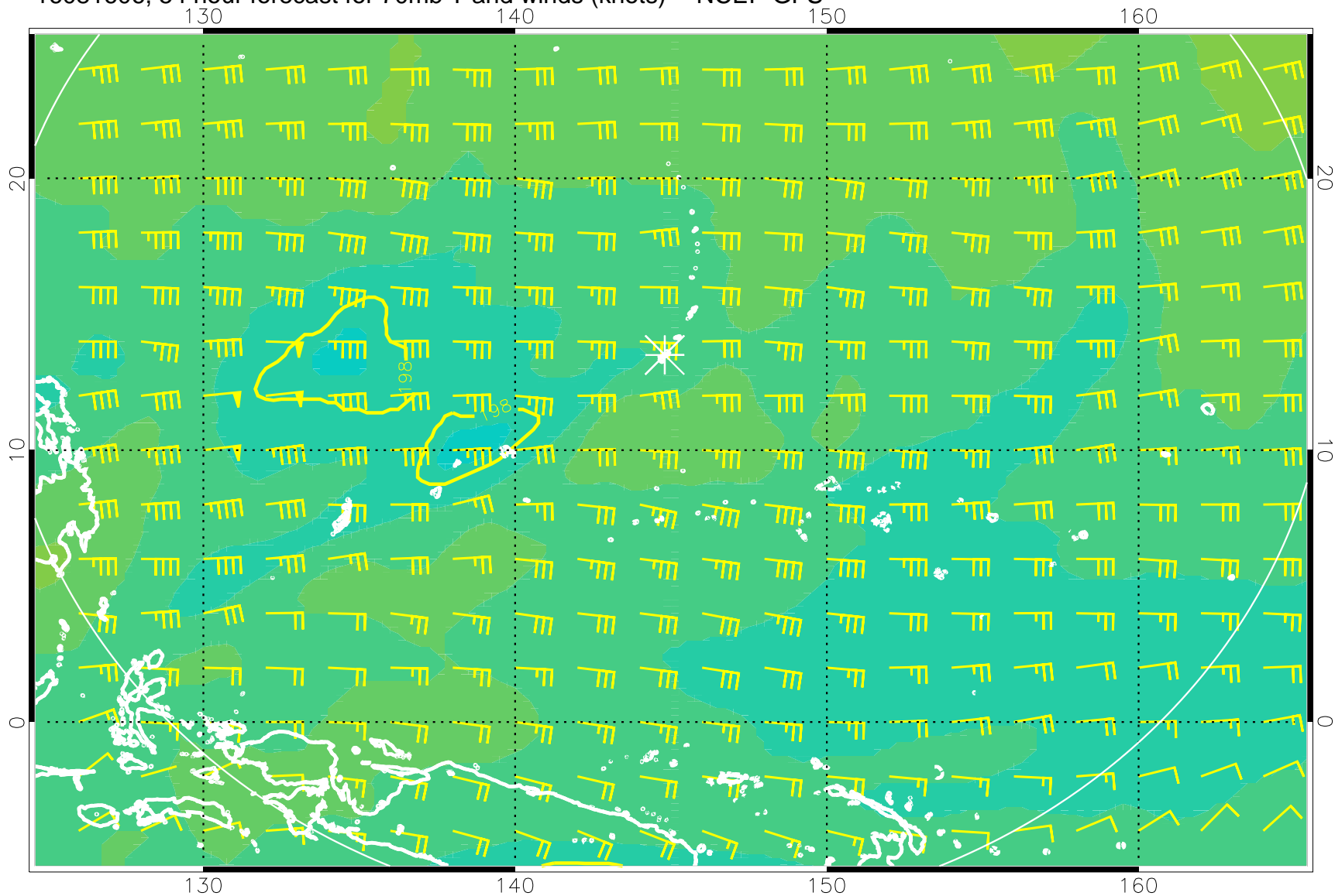
16081606, 54 hour forecast for 70mb T and winds (knots) -- NCEP GFS
