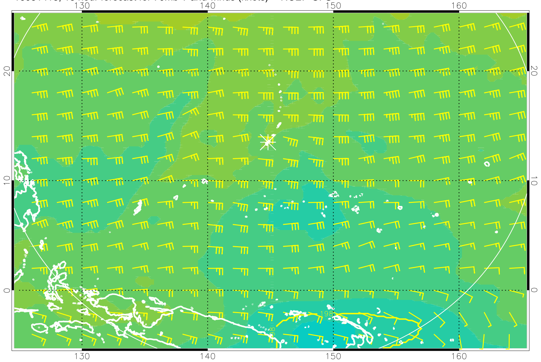
16081418, 18 hour forecast for 70mb T and winds (knots) -- NCEP GFS
