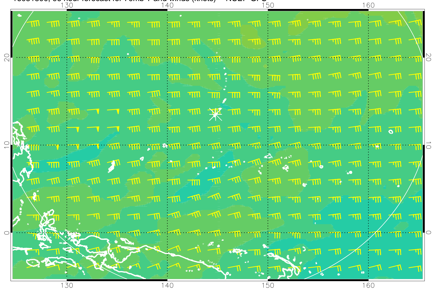
16081800, 96 hour forecast for 70mb T and winds (knots) -- NCEP GFS
