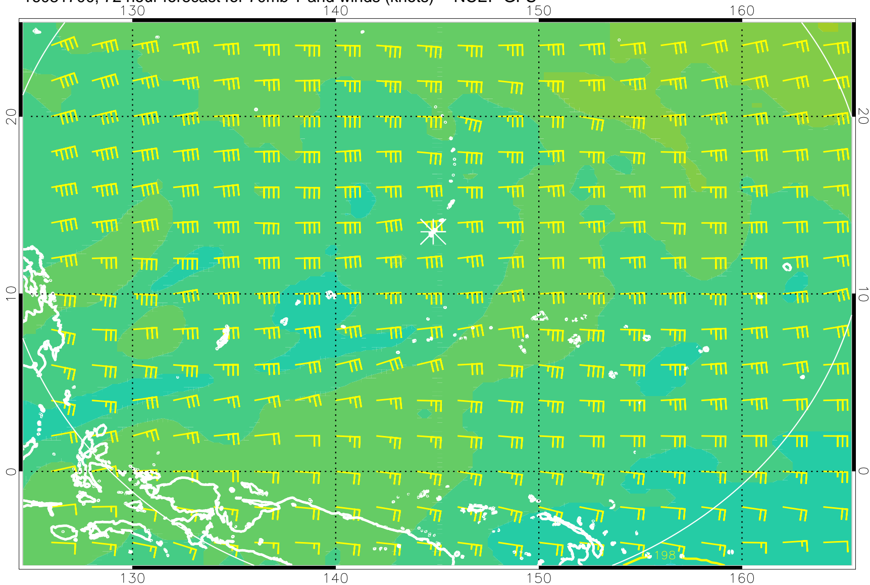
16081700, 72 hour forecast for 70mb T and winds (knots) -- NCEP GFS
