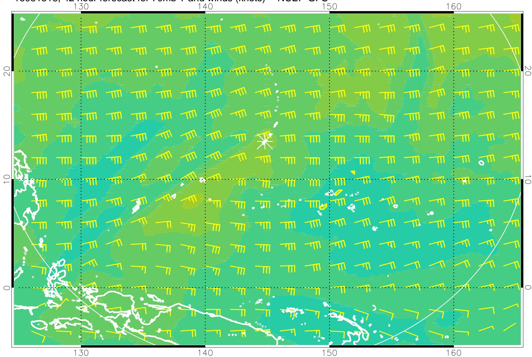
16081518, 42 hour forecast for 70mb T and winds (knots) -- NCEP GFS
