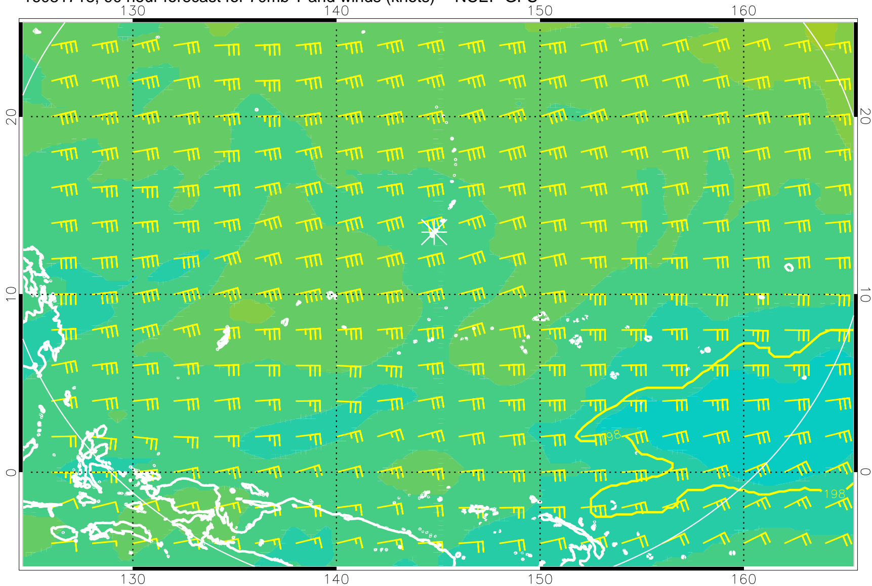
16081718, 90 hour forecast for 70mb T and winds (knots) -- NCEP GFS
