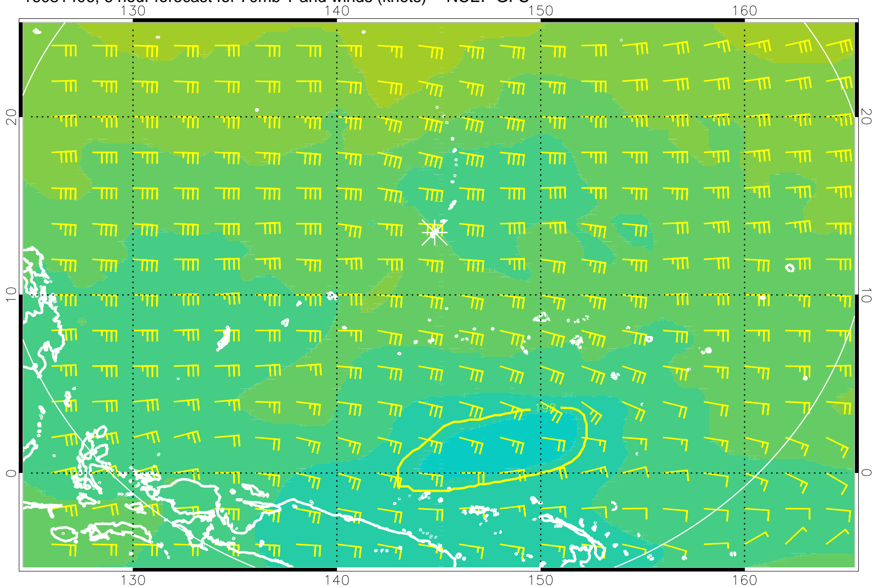
16081406, 6 hour forecast for 70mb T and winds (knots) -- NCEP GFS
