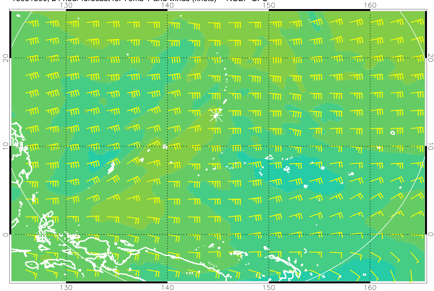
16081500, 24 hour forecast for 70mb T and winds (knots) -- NCEP GFS
