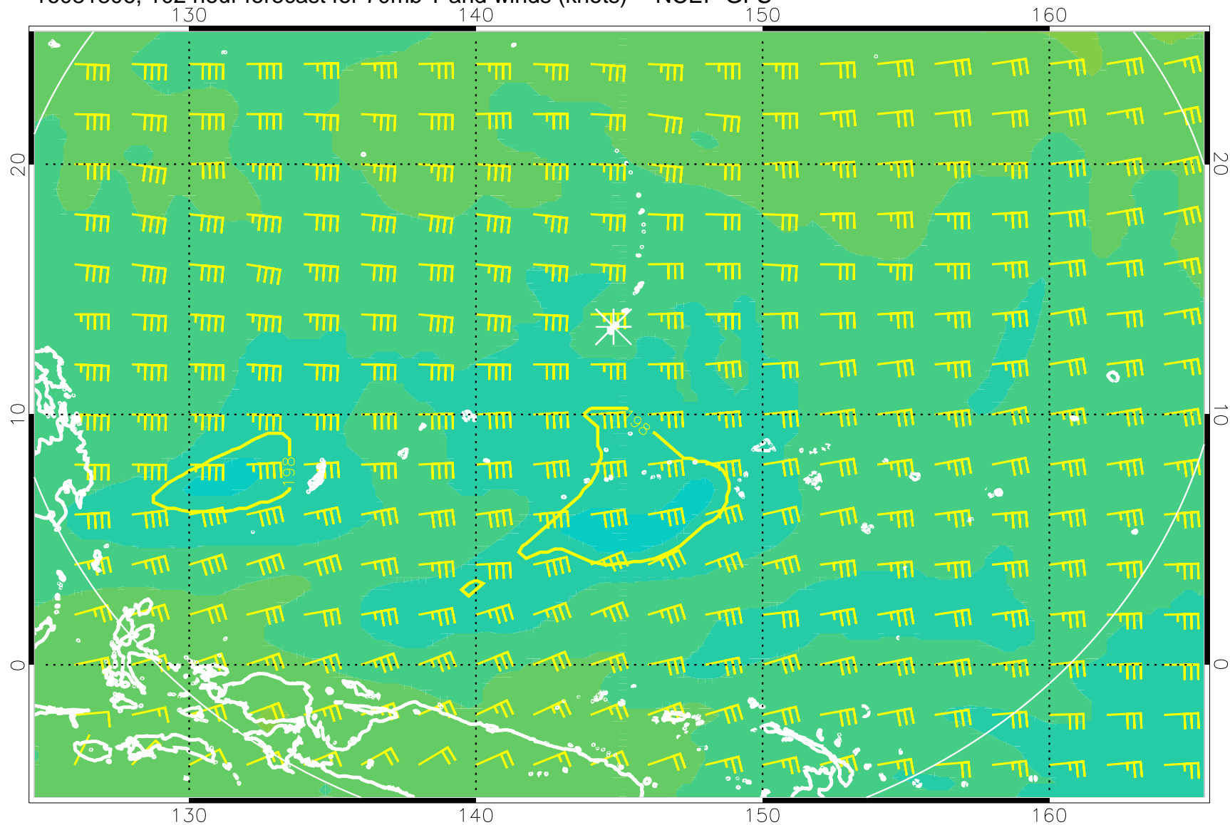
16081806, 102 hour forecast for 70mb T and winds (knots) -- NCEP GFS
