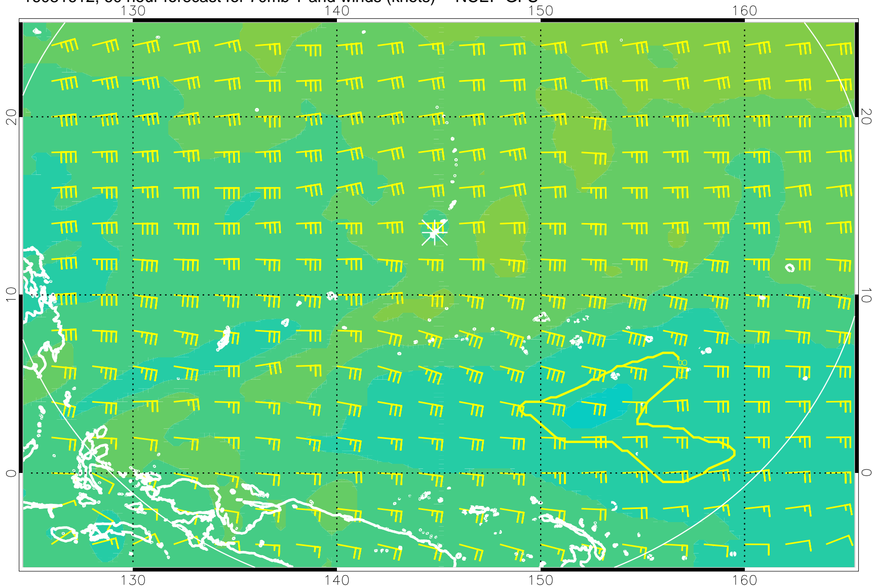
16081612, 60 hour forecast for 70mb T and winds (knots) -- NCEP GFS
