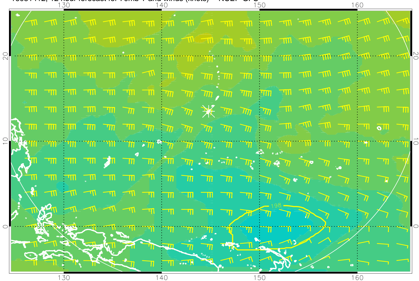
16081412, 12 hour forecast for 70mb T and winds (knots) -- NCEP GFS
