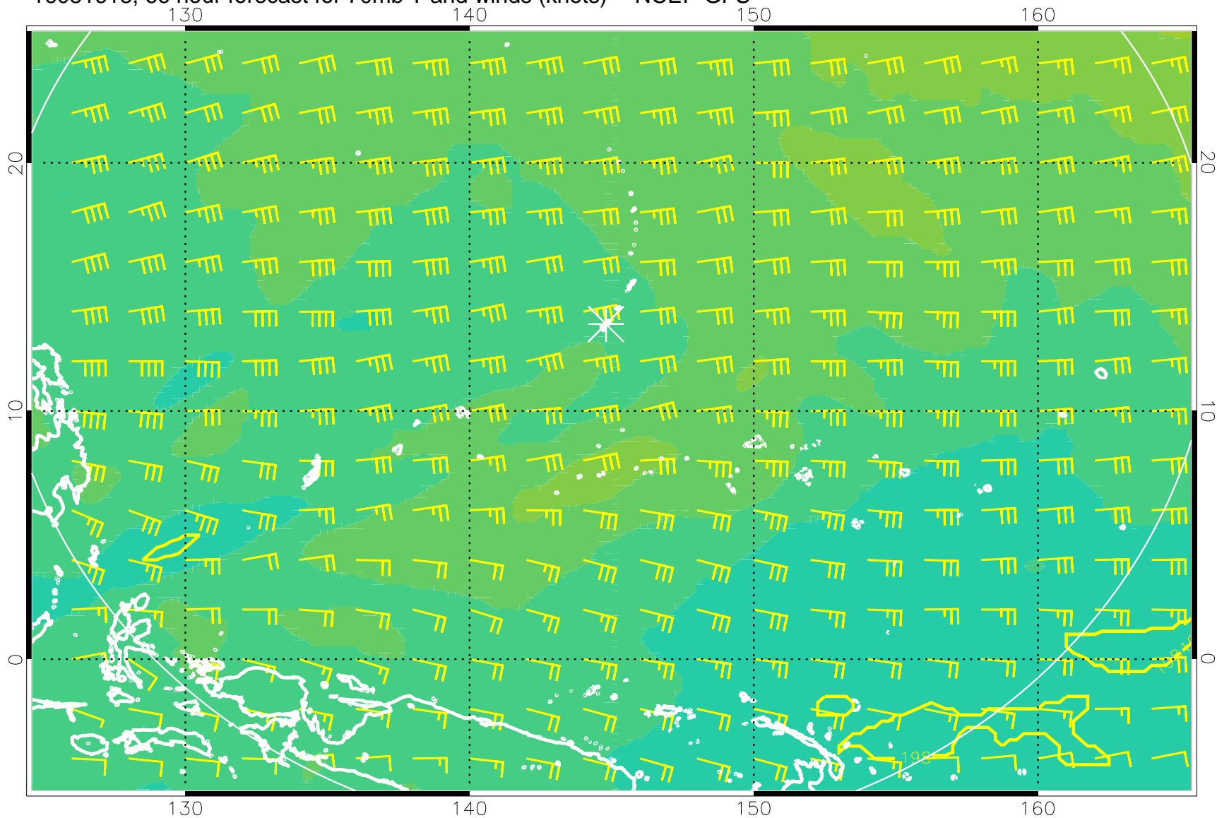
16081618, 66 hour forecast for 70mb T and winds (knots) -- NCEP GFS
