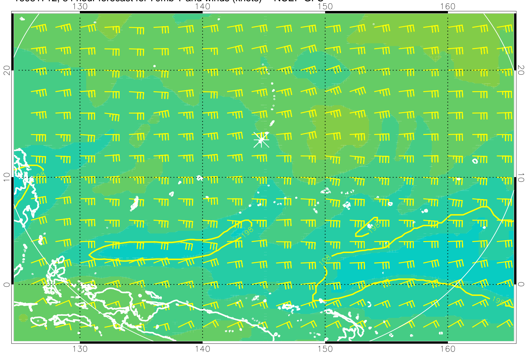
16081712, 84 hour forecast for 70mb T and winds (knots) -- NCEP GFS
