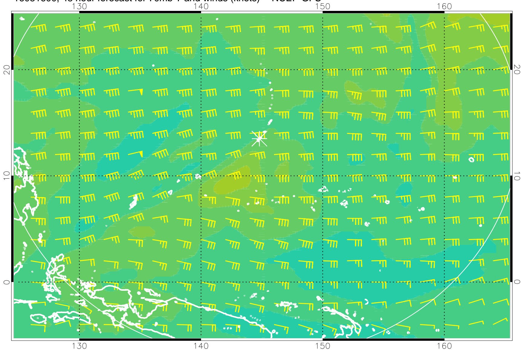
16081600, 48 hour forecast for 70mb T and winds (knots) -- NCEP GFS
