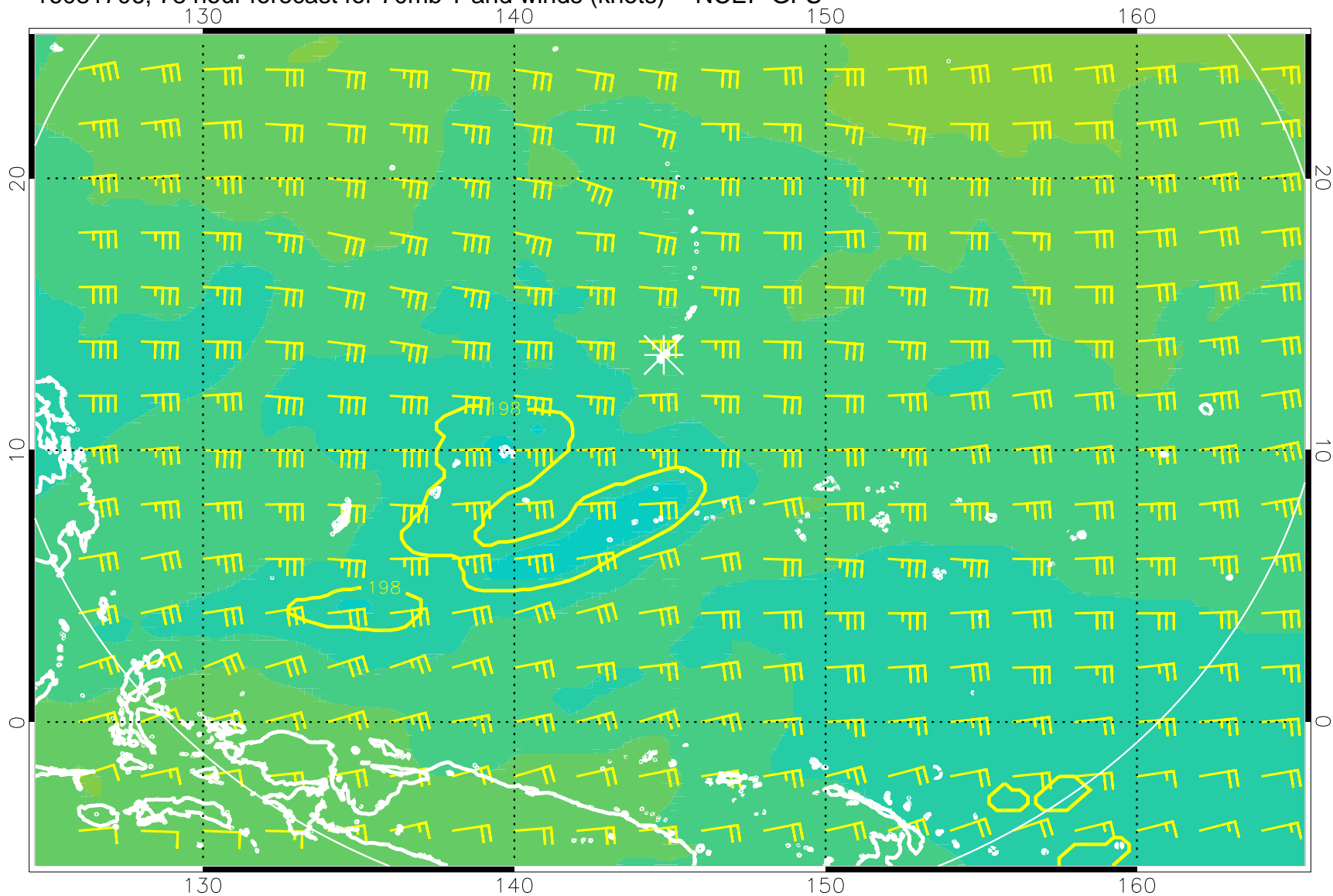
16081706, 78 hour forecast for 70mb T and winds (knots) -- NCEP GFS
