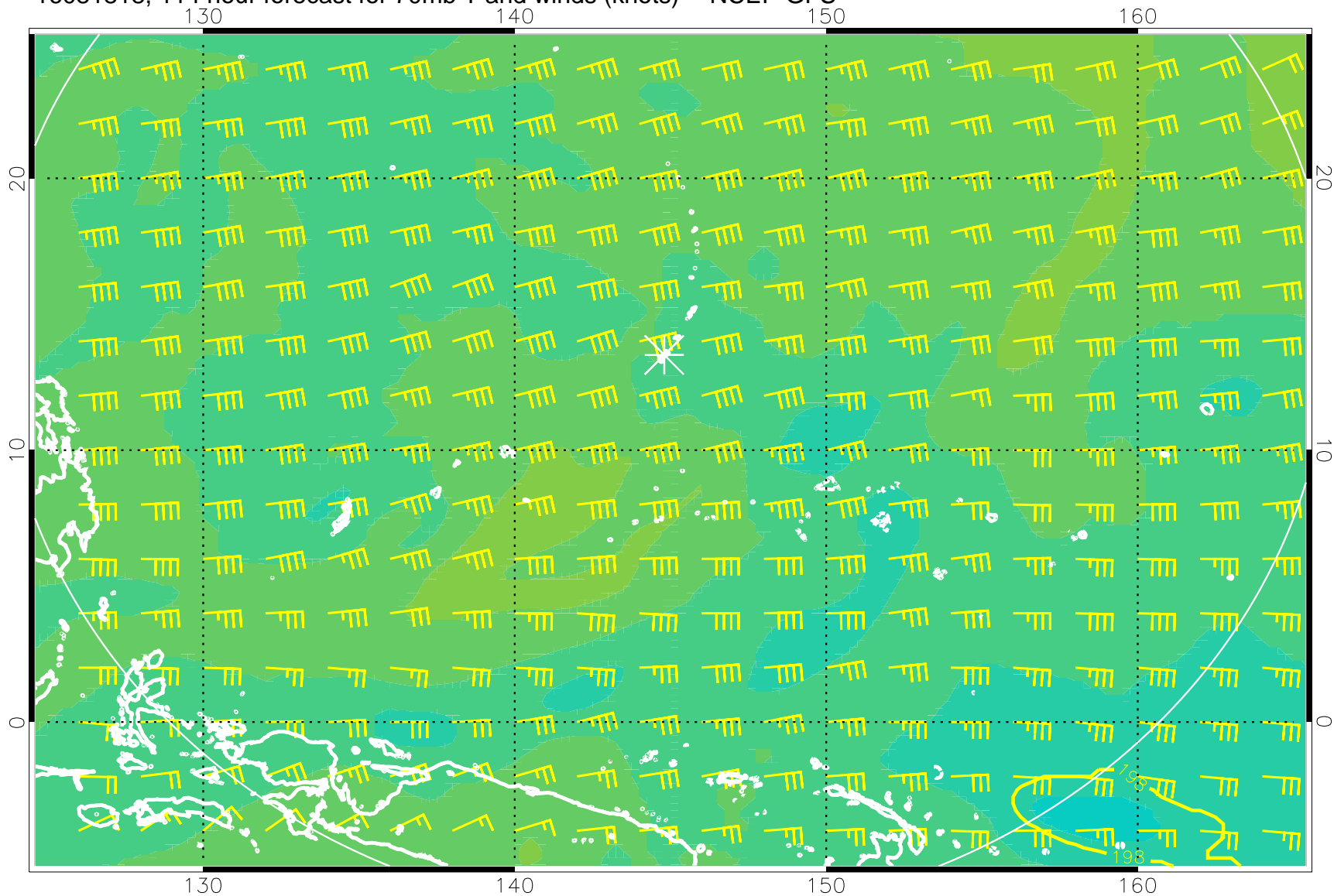
16081818, 114 hour forecast for 70mb T and winds (knots) -- NCEP GFS
