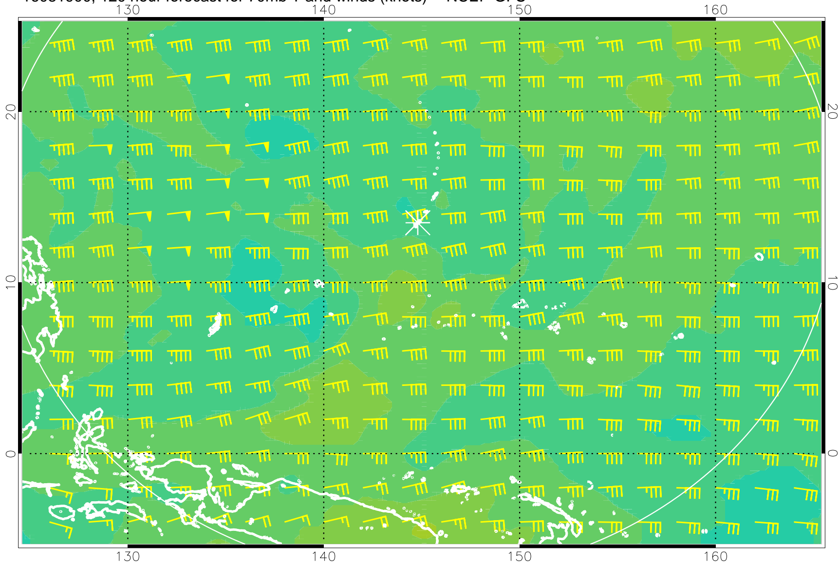
16081900, 120 hour forecast for 70mb T and winds (knots) -- NCEP GFS
