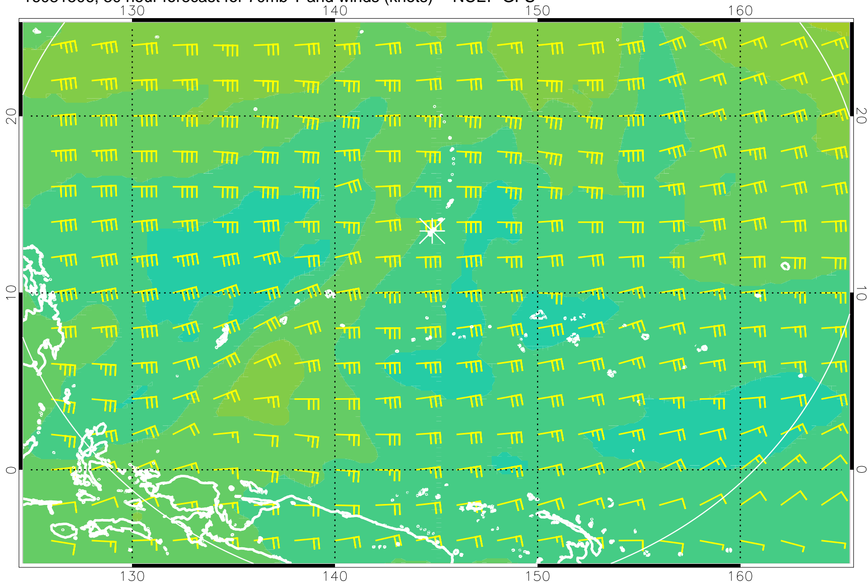
16081506, 30 hour forecast for 70mb T and winds (knots) -- NCEP GFS
