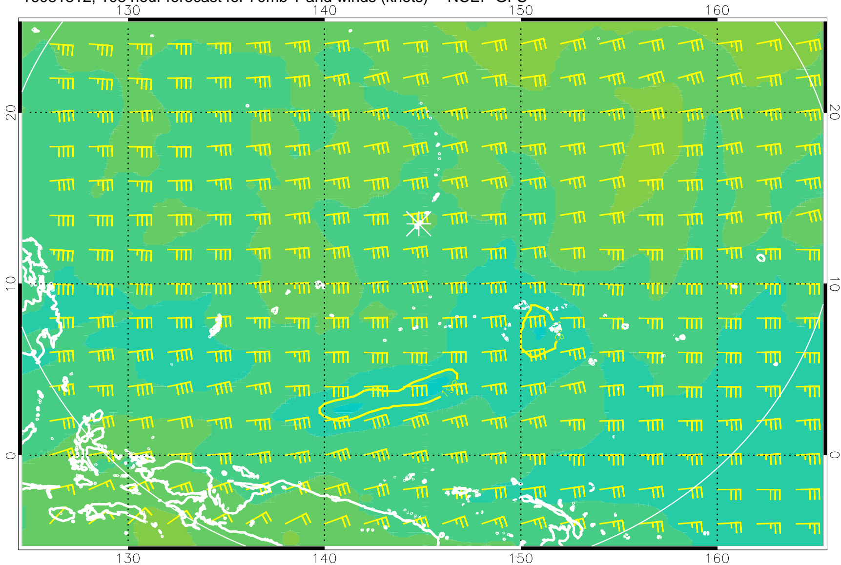
16081812, 108 hour forecast for 70mb T and winds (knots) -- NCEP GFS
