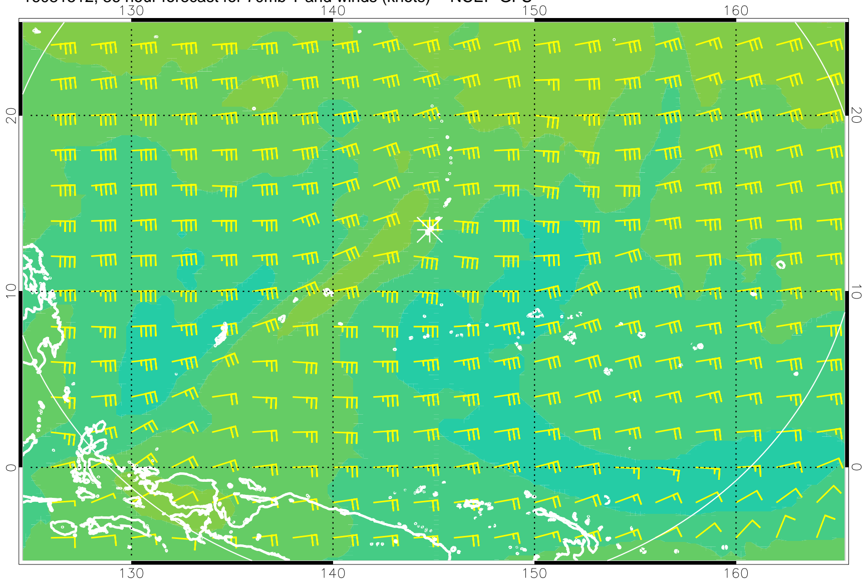
16081512, 36 hour forecast for 70mb T and winds (knots) -- NCEP GFS
