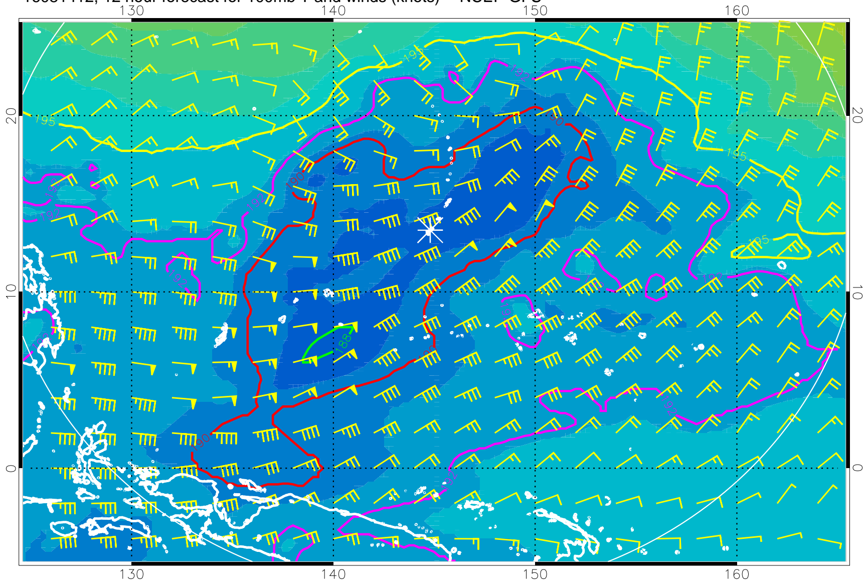
16081412, 12 hour forecast for 100mb T and winds (knots) -- NCEP GFS
