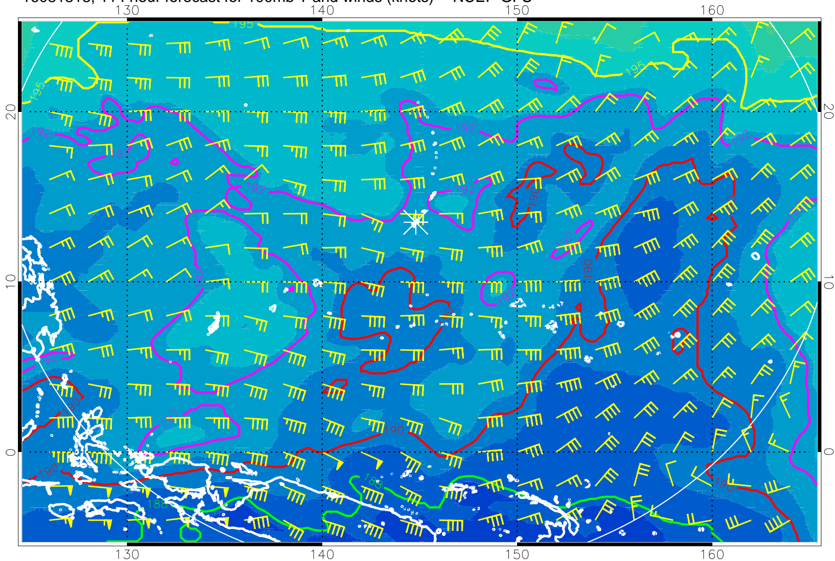
16081818, 114 hour forecast for 100mb T and winds (knots) -- NCEP GFS
