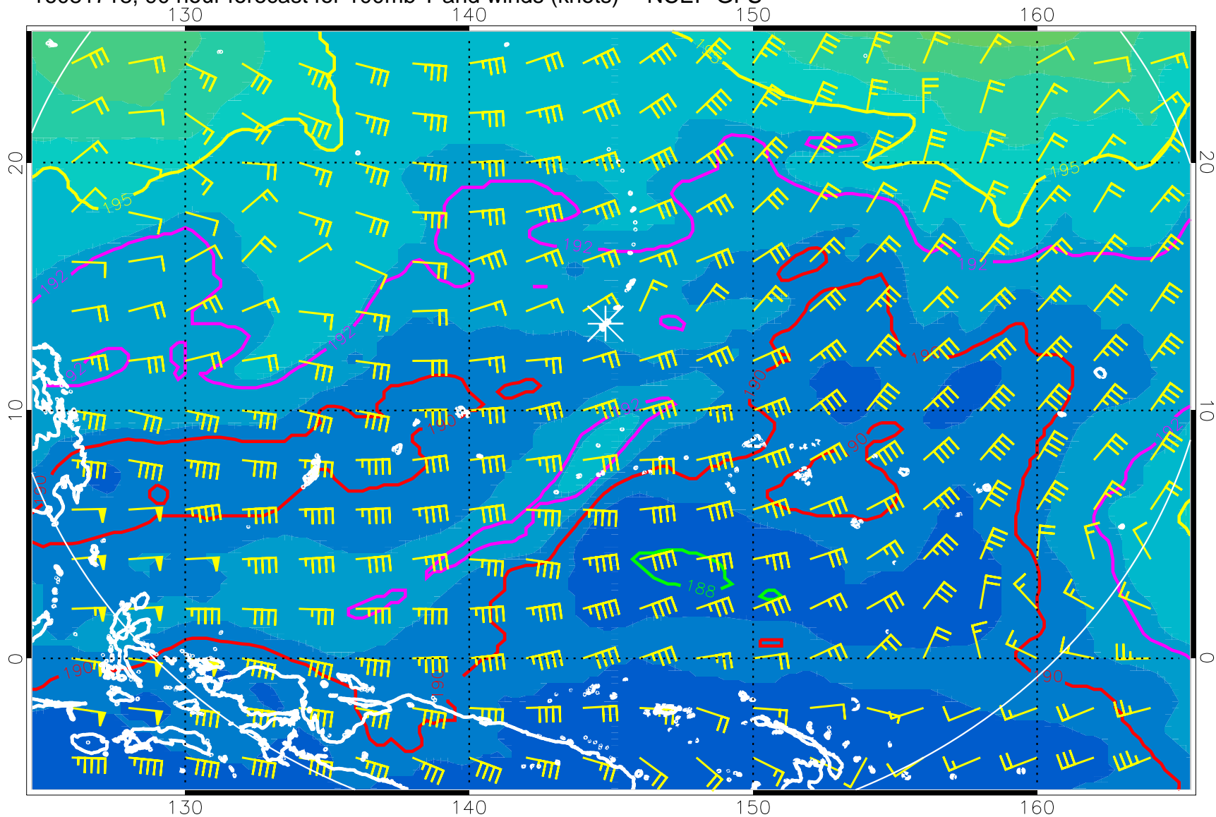
16081718, 90 hour forecast for 100mb T and winds (knots) -- NCEP GFS
