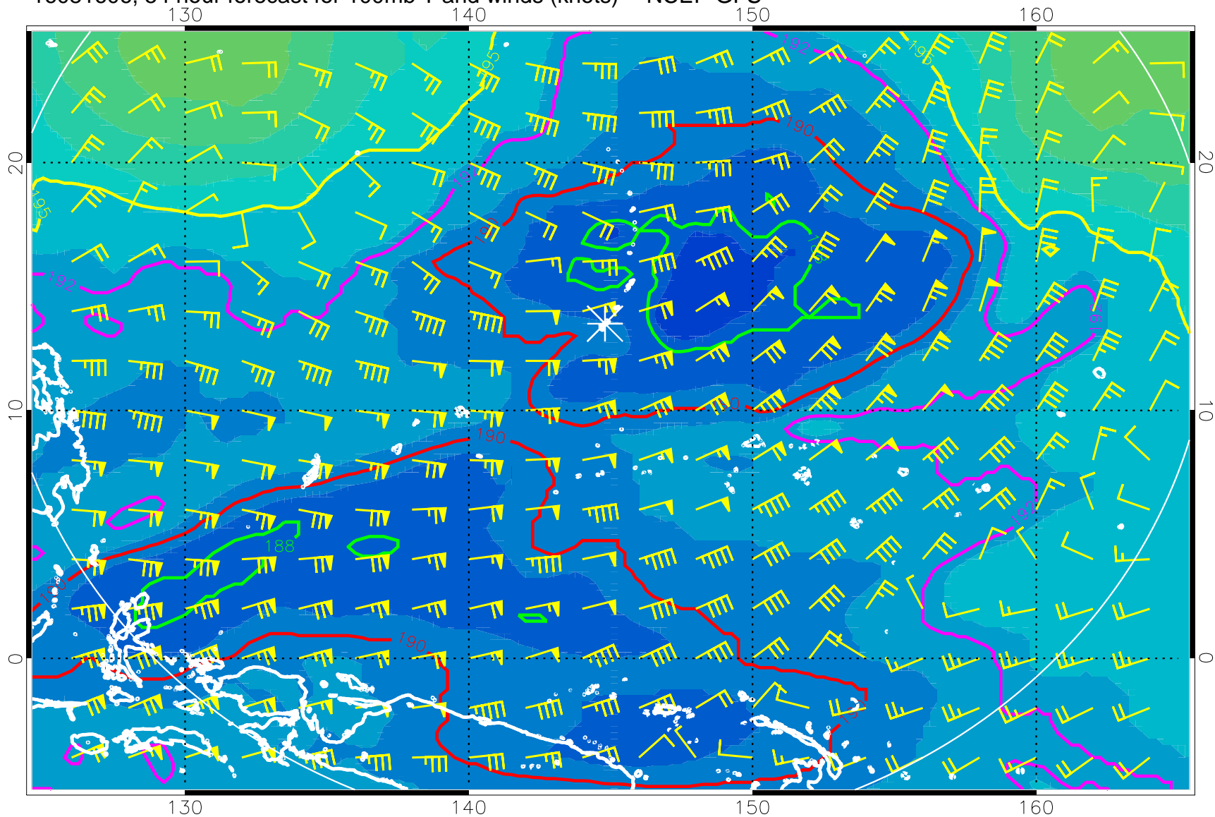
16081606, 54 hour forecast for 100mb T and winds (knots) -- NCEP GFS
