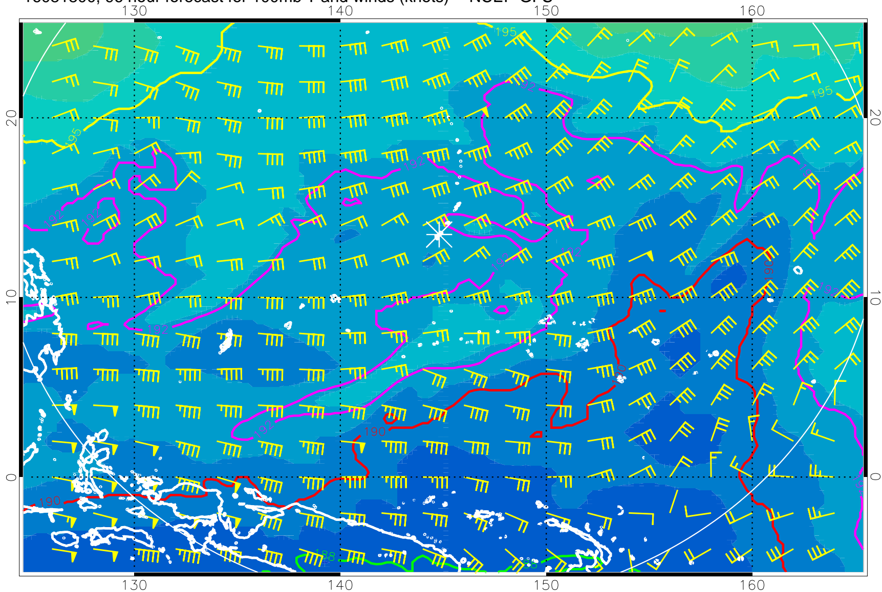
16081800, 96 hour forecast for 100mb T and winds (knots) -- NCEP GFS
