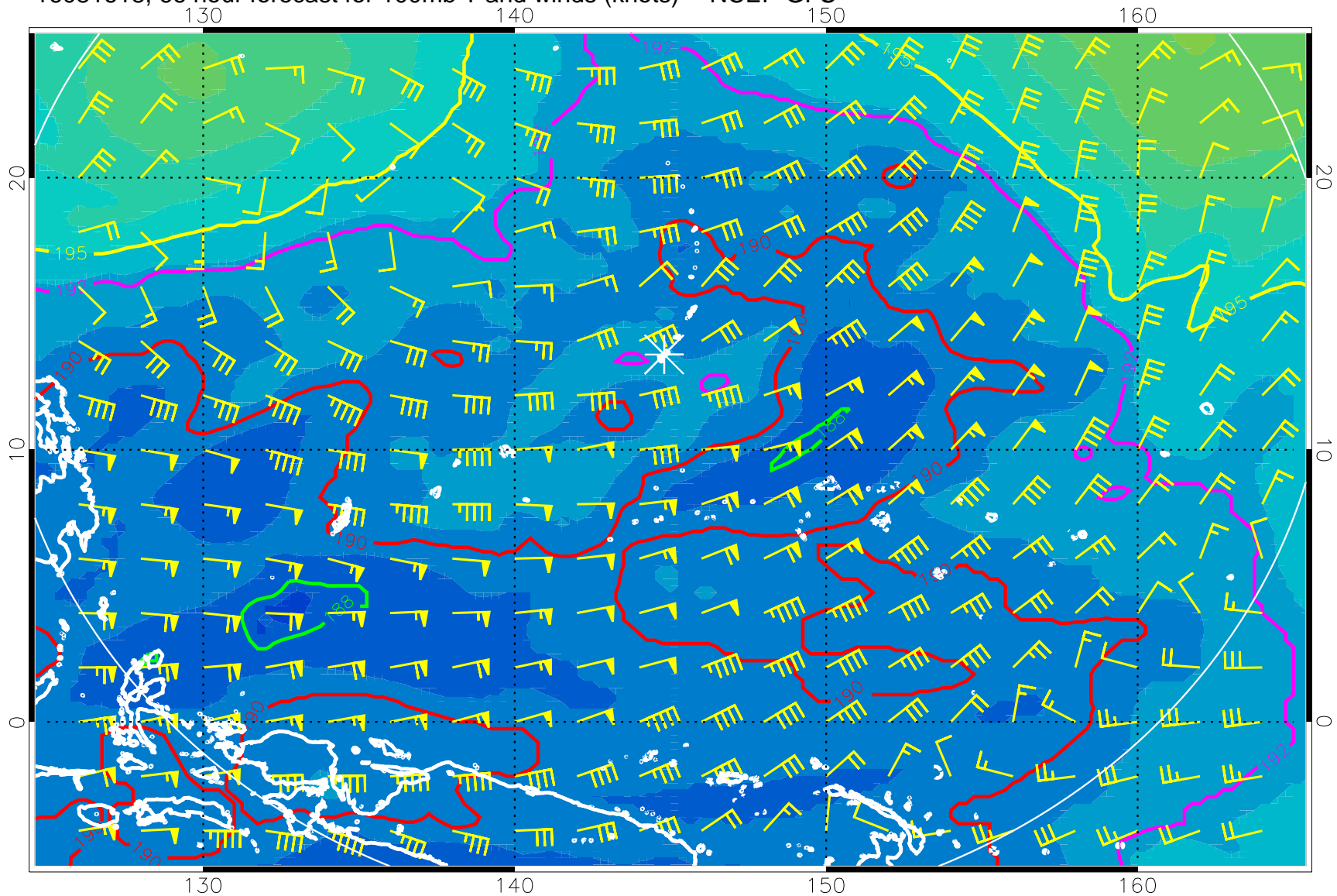
16081618, 66 hour forecast for 100mb T and winds (knots) -- NCEP GFS
