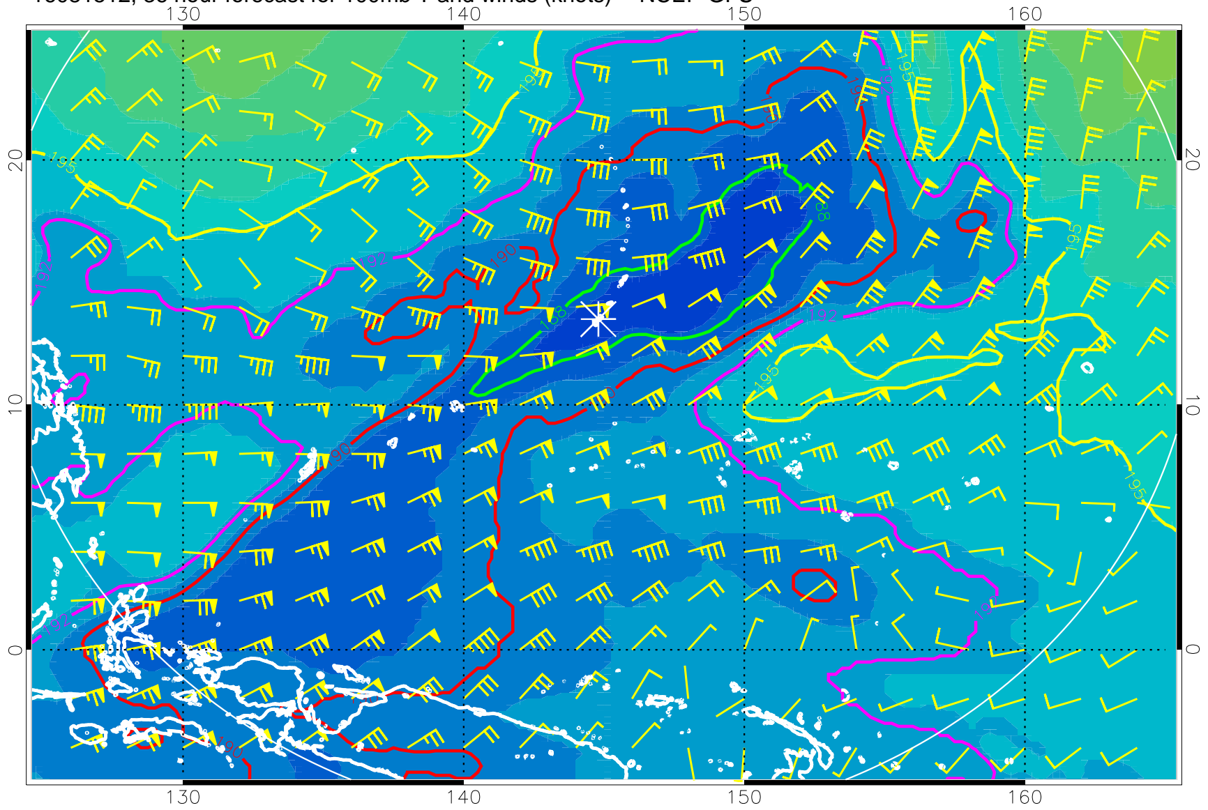
16081512, 36 hour forecast for 100mb T and winds (knots) -- NCEP GFS
