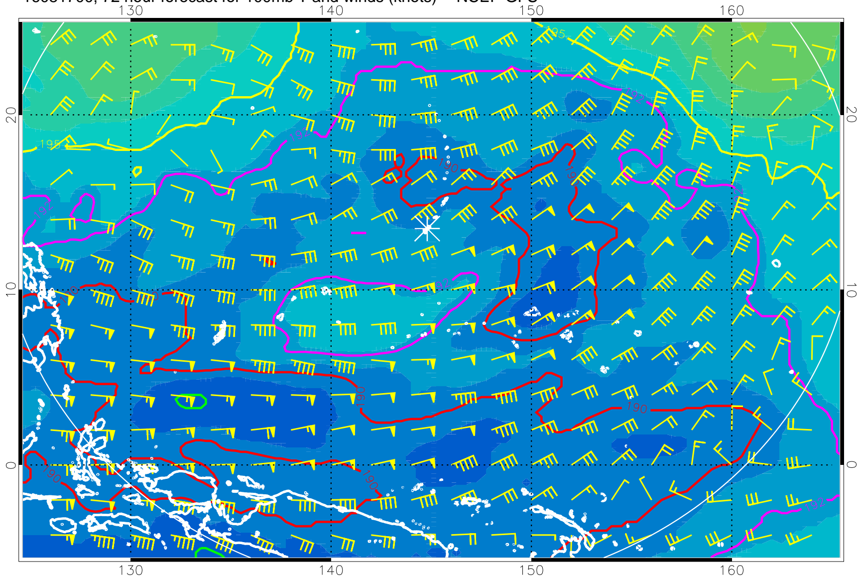
16081700, 72 hour forecast for 100mb T and winds (knots) -- NCEP GFS
