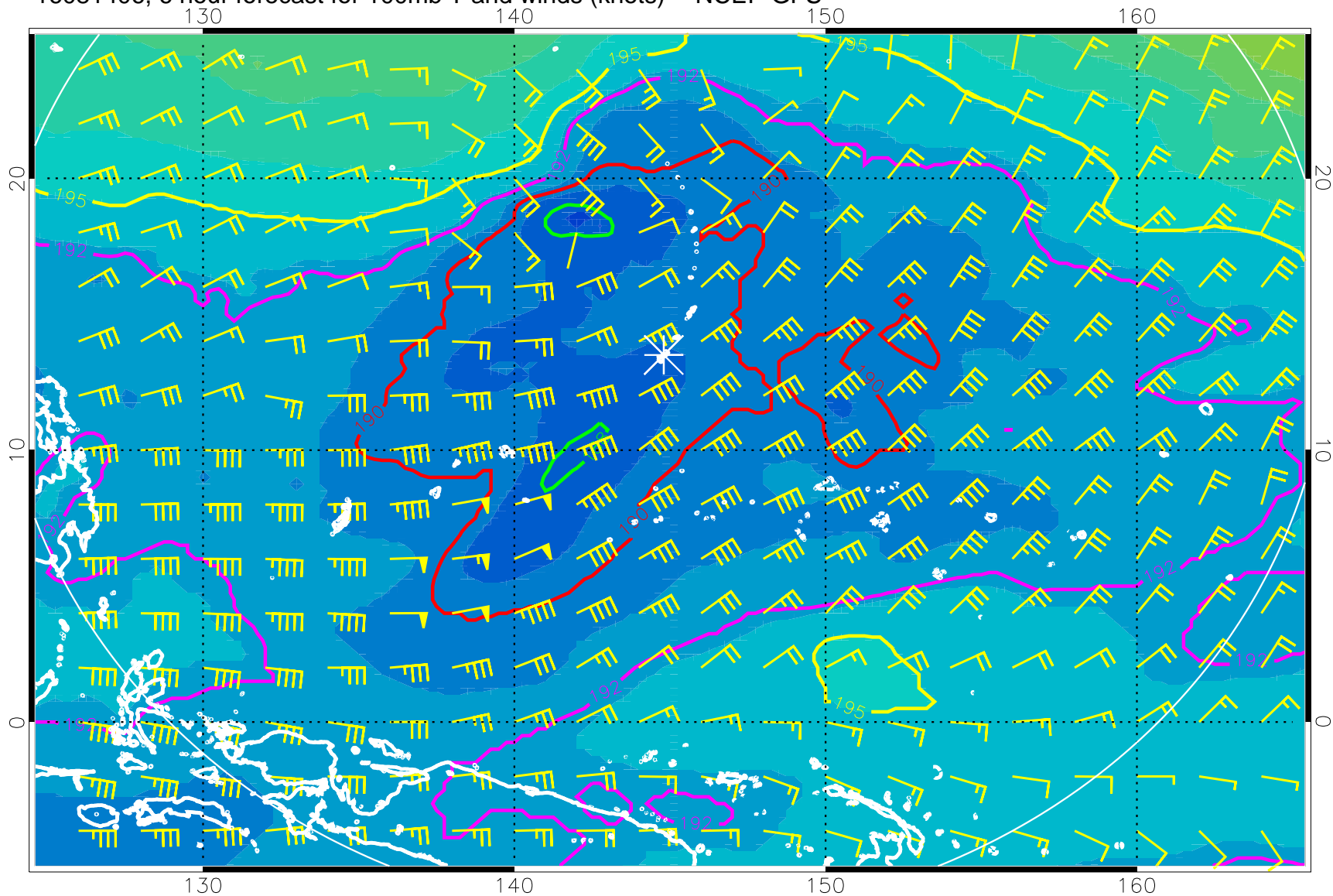
16081406, 6 hour forecast for 100mb T and winds (knots) -- NCEP GFS
