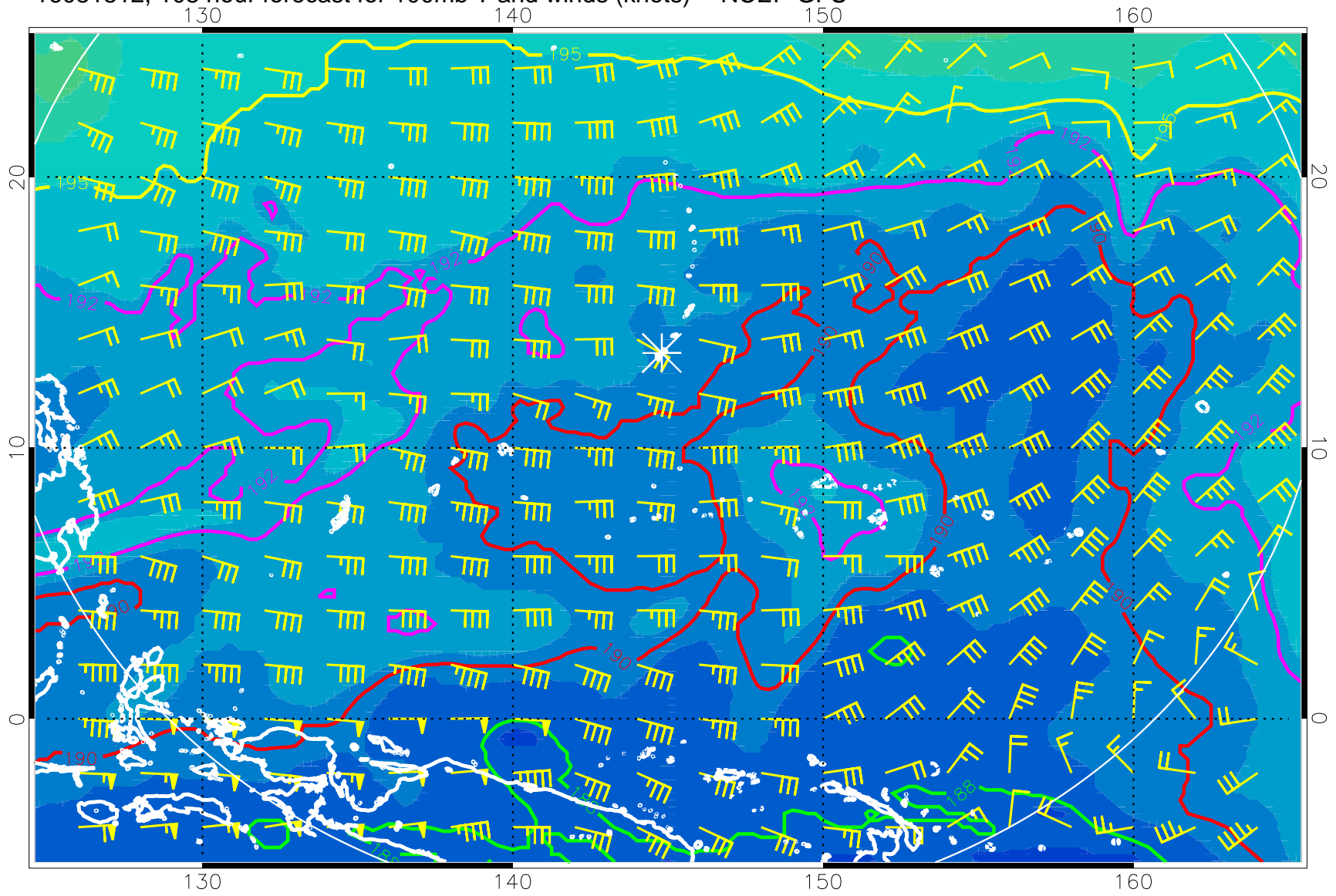
16081812, 108 hour forecast for 100mb T and winds (knots) -- NCEP GFS
