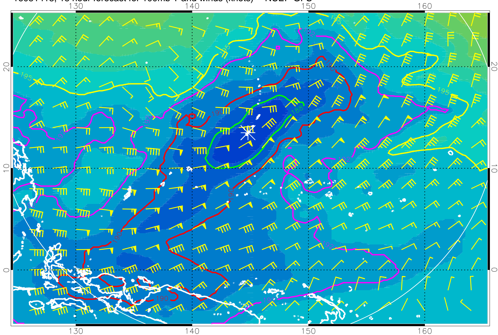
16081418, 18 hour forecast for 100mb T and winds (knots) -- NCEP GFS
