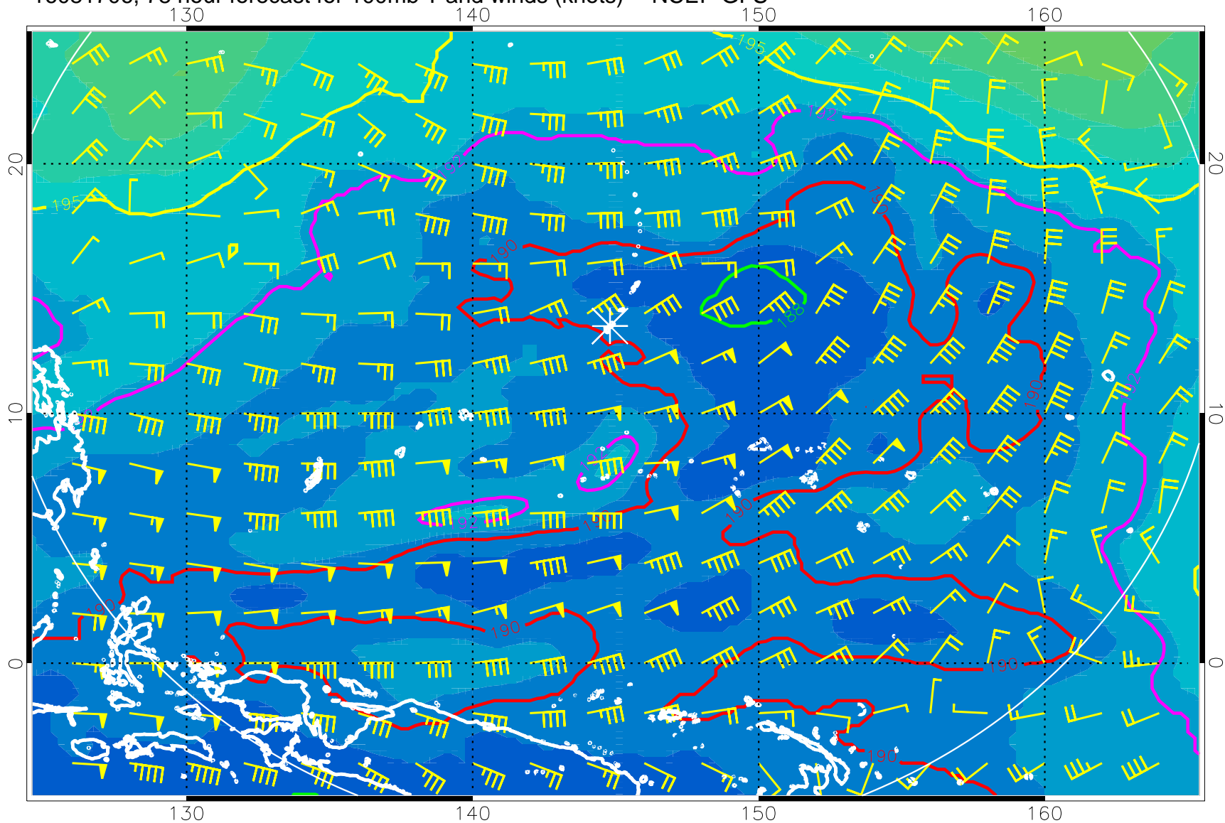
16081706, 78 hour forecast for 100mb T and winds (knots) -- NCEP GFS
