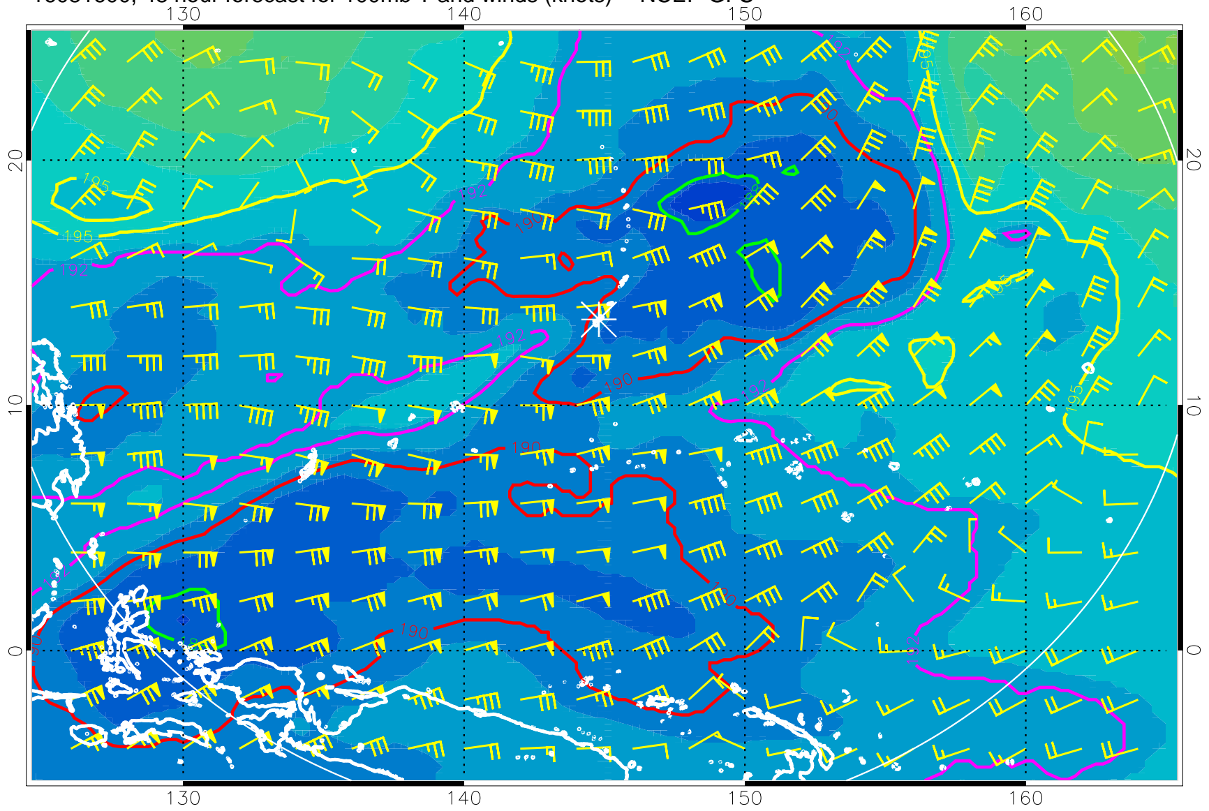
16081600, 48 hour forecast for 100mb T and winds (knots) -- NCEP GFS
