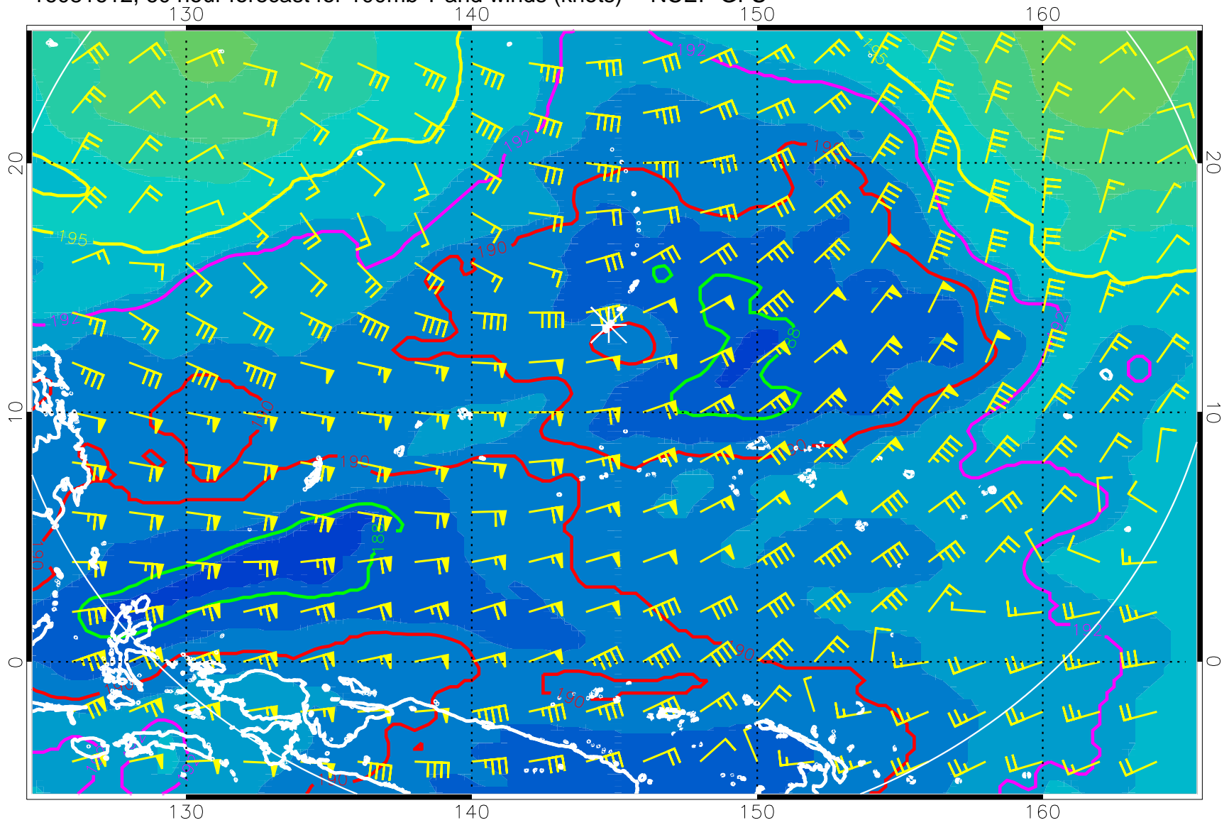
16081612, 60 hour forecast for 100mb T and winds (knots) -- NCEP GFS
