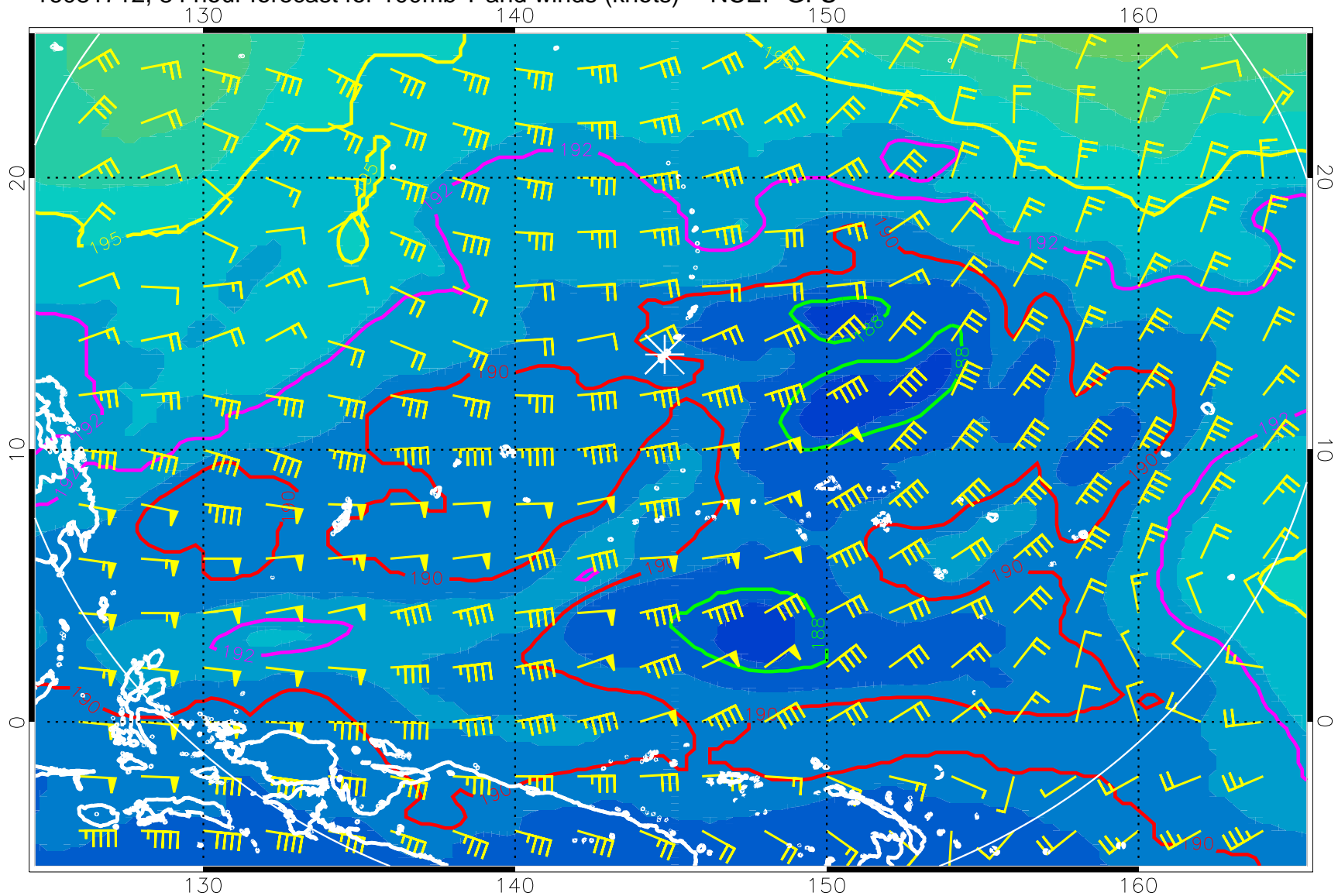
16081712, 84 hour forecast for 100mb T and winds (knots) -- NCEP GFS
