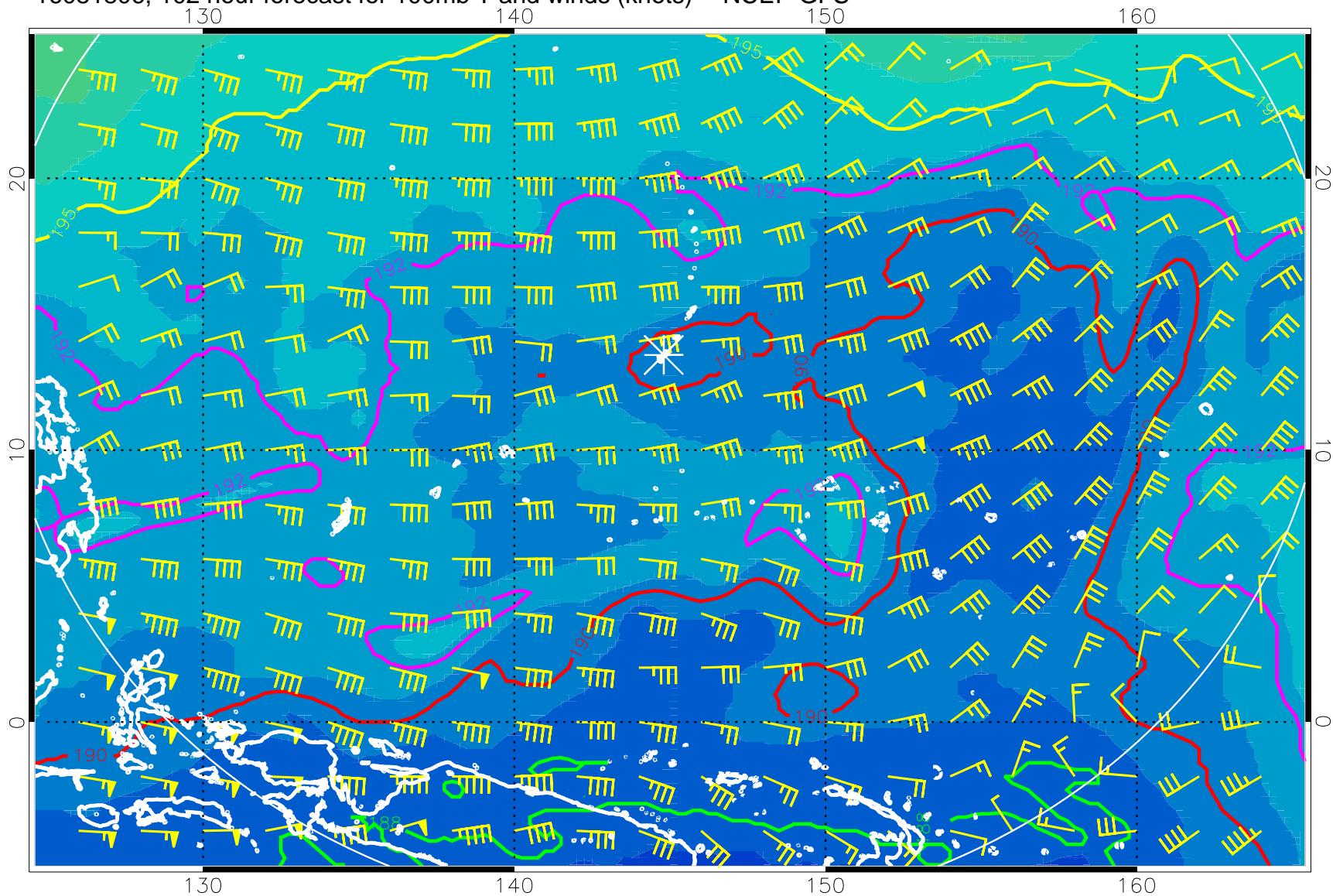
16081806, 102 hour forecast for 100mb T and winds (knots) -- NCEP GFS
