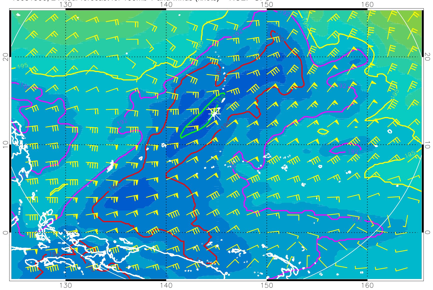
16081500, 24 hour forecast for 100mb T and winds (knots) -- NCEP GFS
