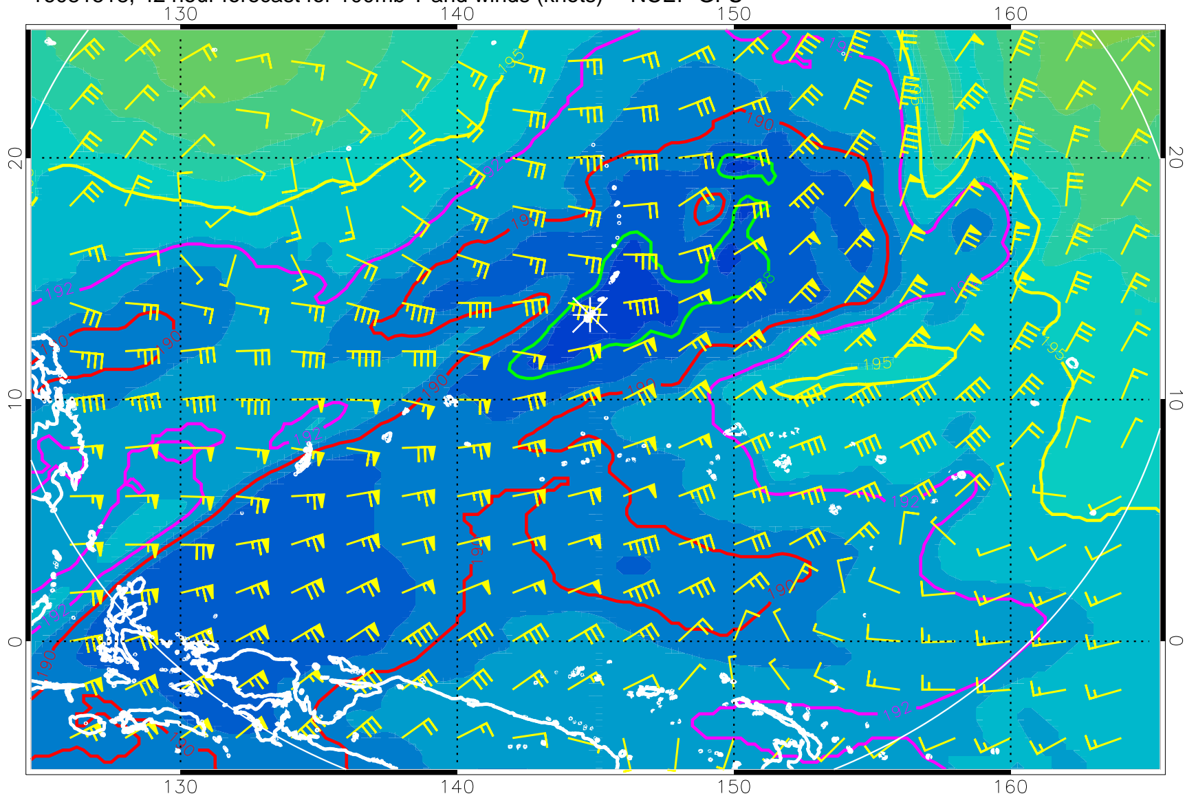
16081518, 42 hour forecast for 100mb T and winds (knots) -- NCEP GFS
