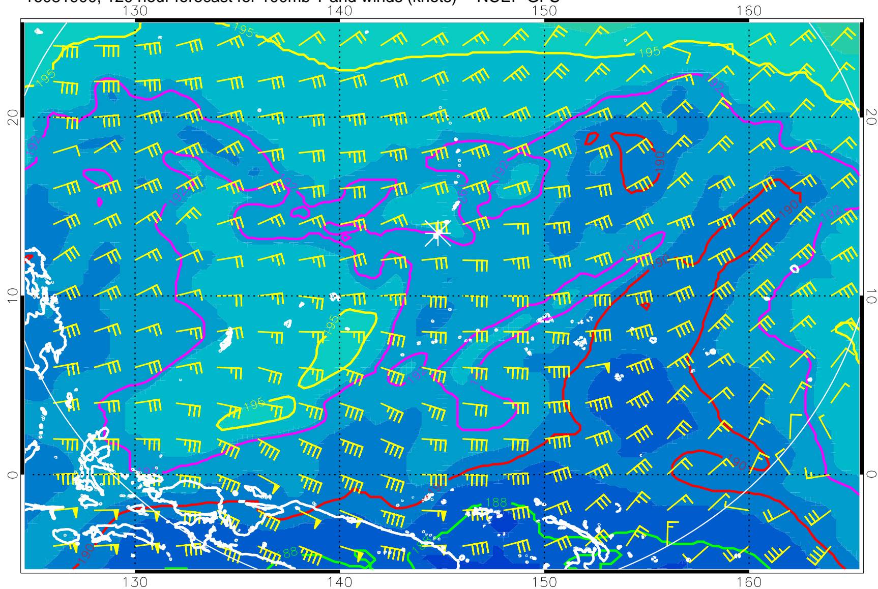
16081900, 120 hour forecast for 100mb T and winds (knots) -- NCEP GFS
