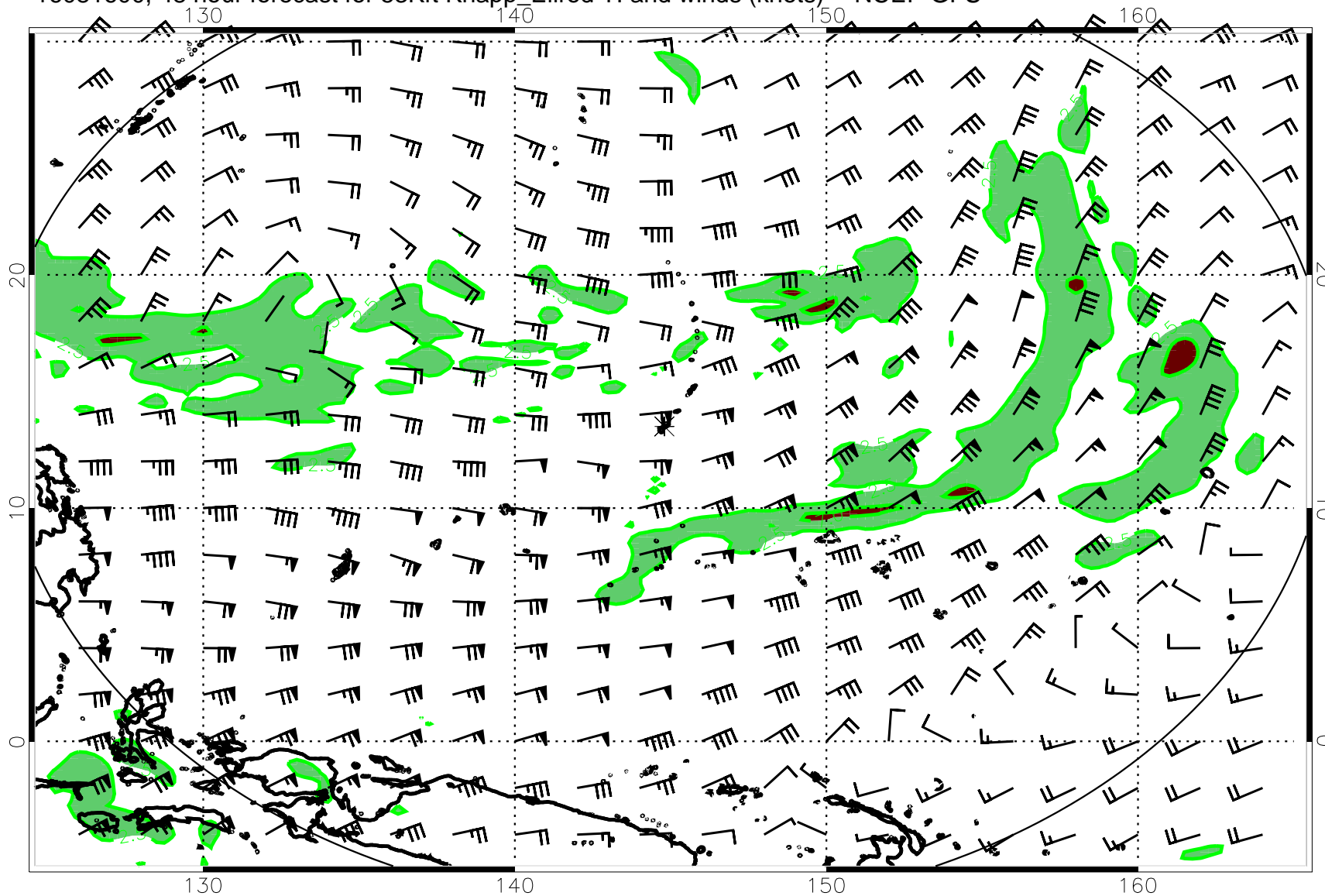
16081600, 48 hour forecast for 53Kft Knapp_Ellrod TI and winds (knots) -- NCEP GFS
