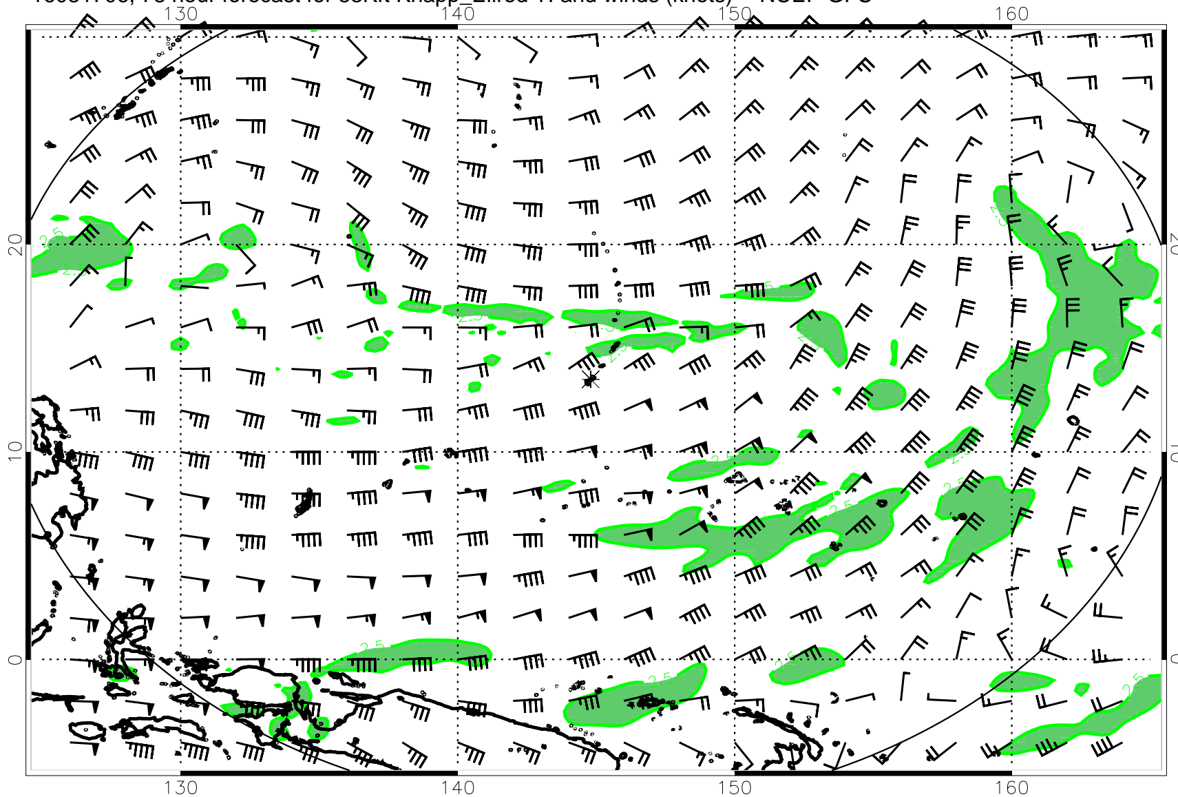
16081706, 78 hour forecast for 53Kft Knapp_Ellrod TI and winds (knots) -- NCEP GFS
