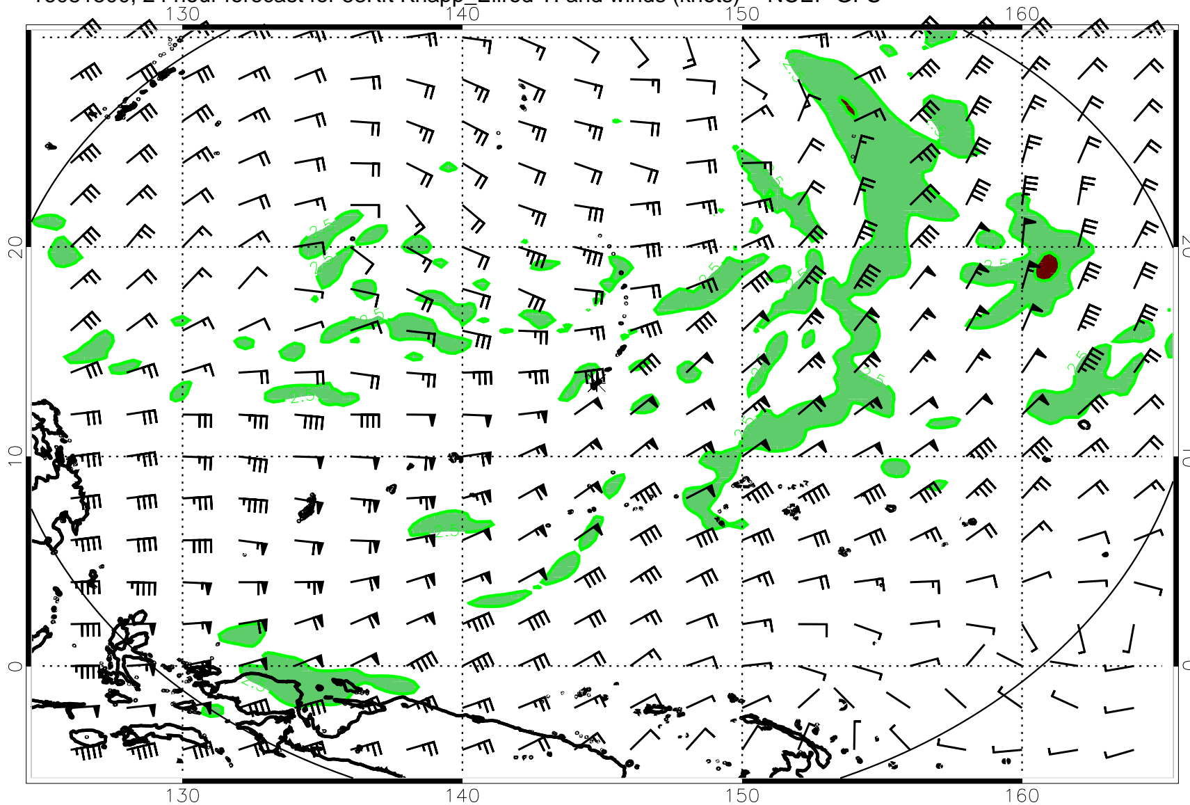
16081500, 24 hour forecast for 53Kft Knapp_Ellrod TI and winds (knots) -- NCEP GFS
