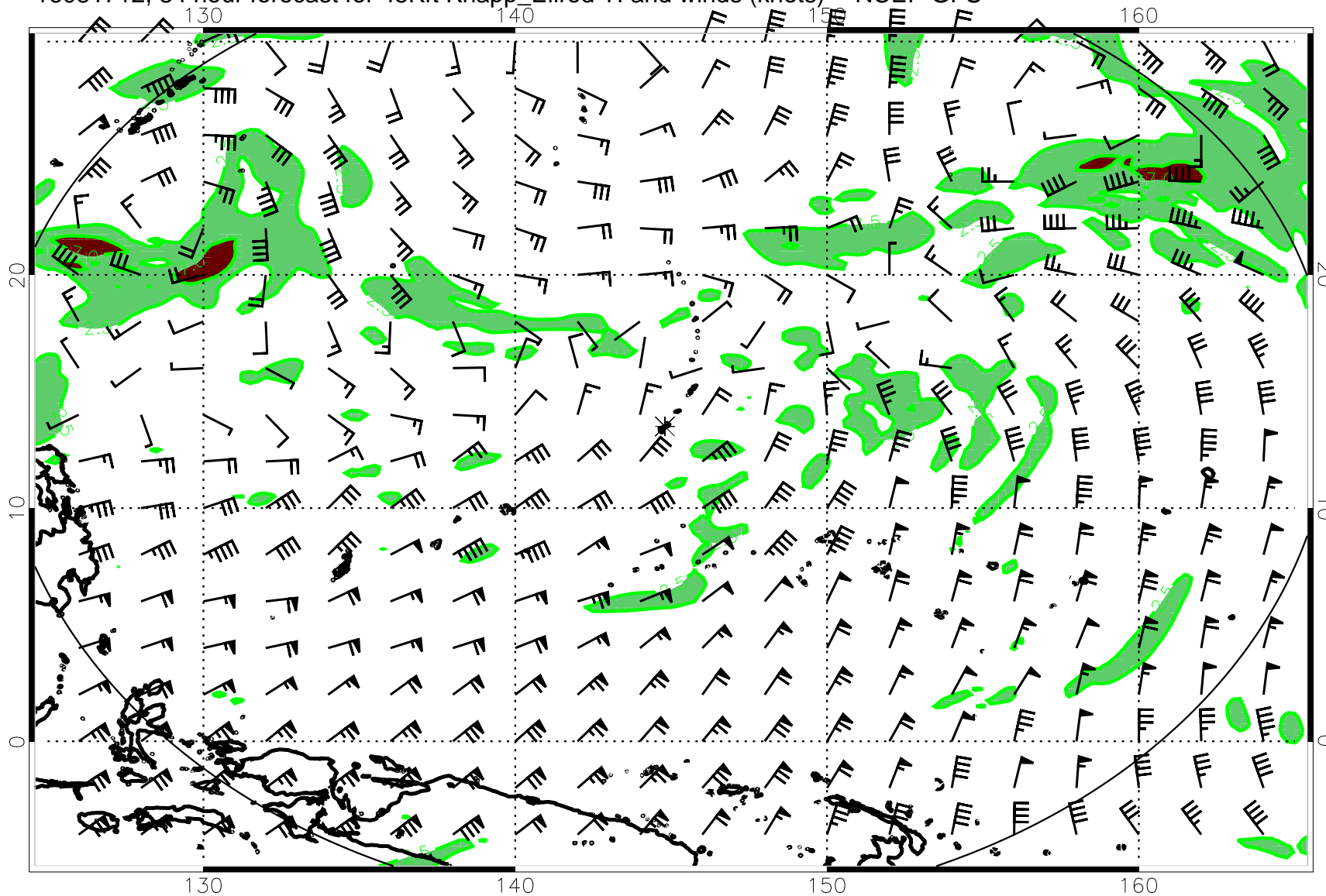
16081712, 84 hour forecast for 45Kft Knapp_Ellrod TI and winds (knots) -- NCEP GFS
