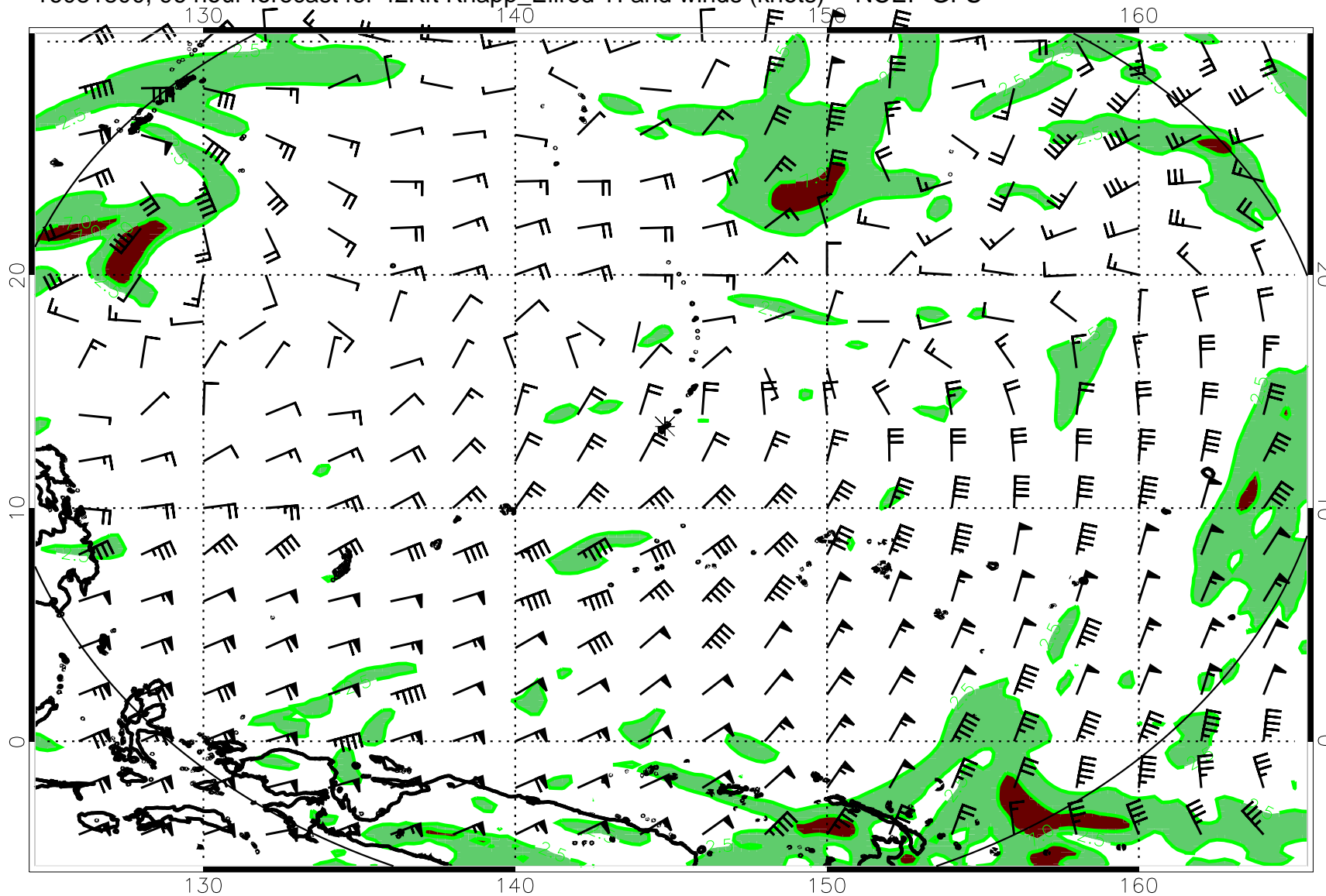
16081800, 96 hour forecast for 42Kft Knapp_Ellrod TI and winds (knots) -- NCEP GFS
