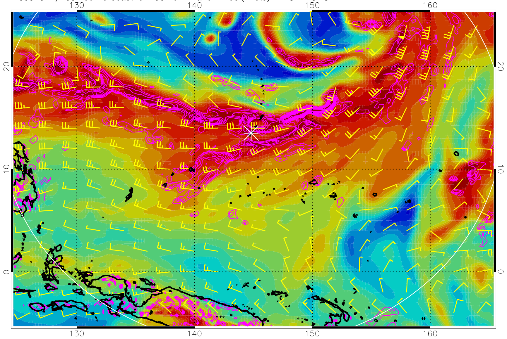
16081812, 108 hour forecast for 700mb RH and winds (knots) -- NCEP GFS
