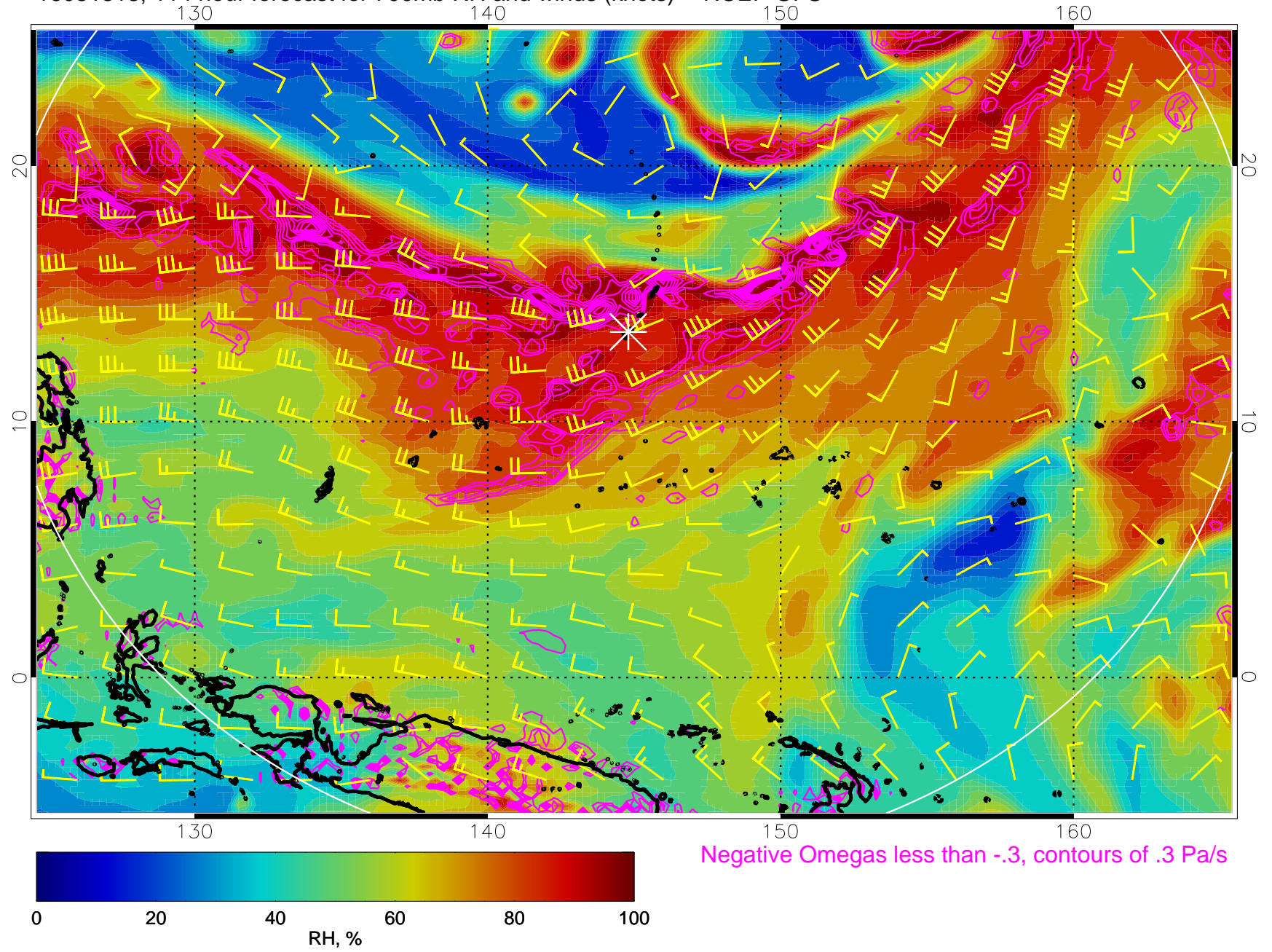
16081818, 114 hour forecast for 700mb RH and winds (knots) -- NCEP GFS
