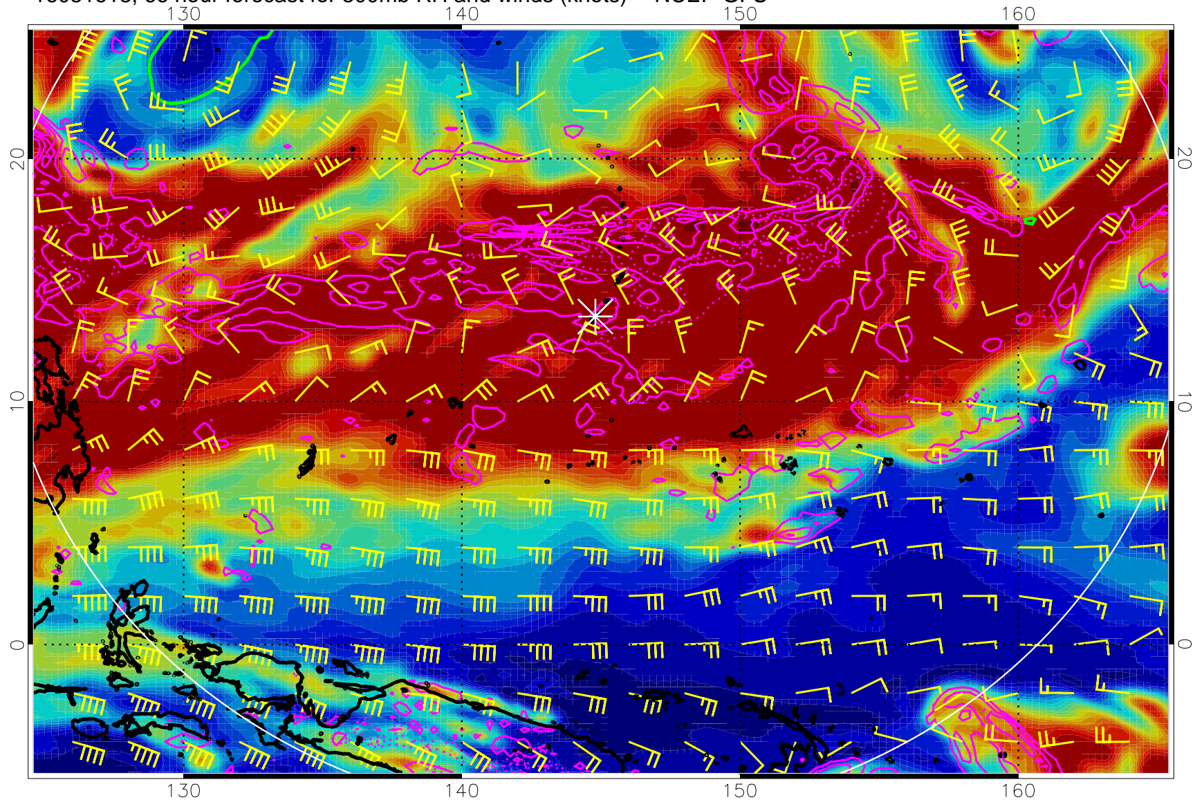
16081618, 66 hour forecast for 300mb RH and winds (knots) -- NCEP GFS
