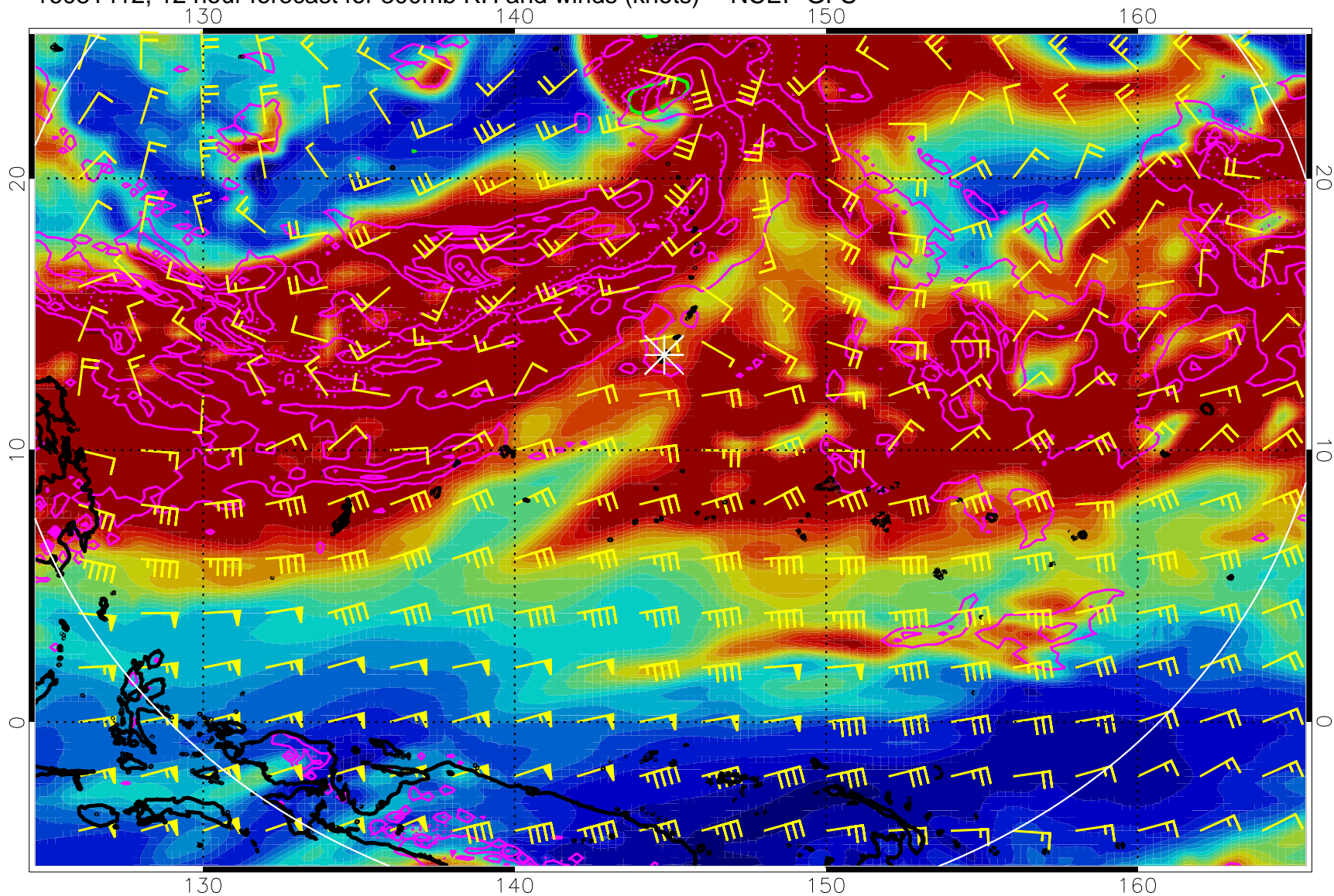
16081412, 12 hour forecast for 300mb RH and winds (knots) -- NCEP GFS
