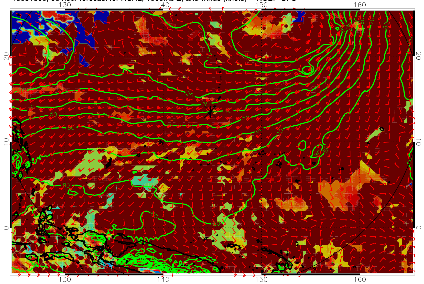
16081800, 96 hour forecast for HCAL, 1000mb Z, and winds (knots) -- NCEP GFS
