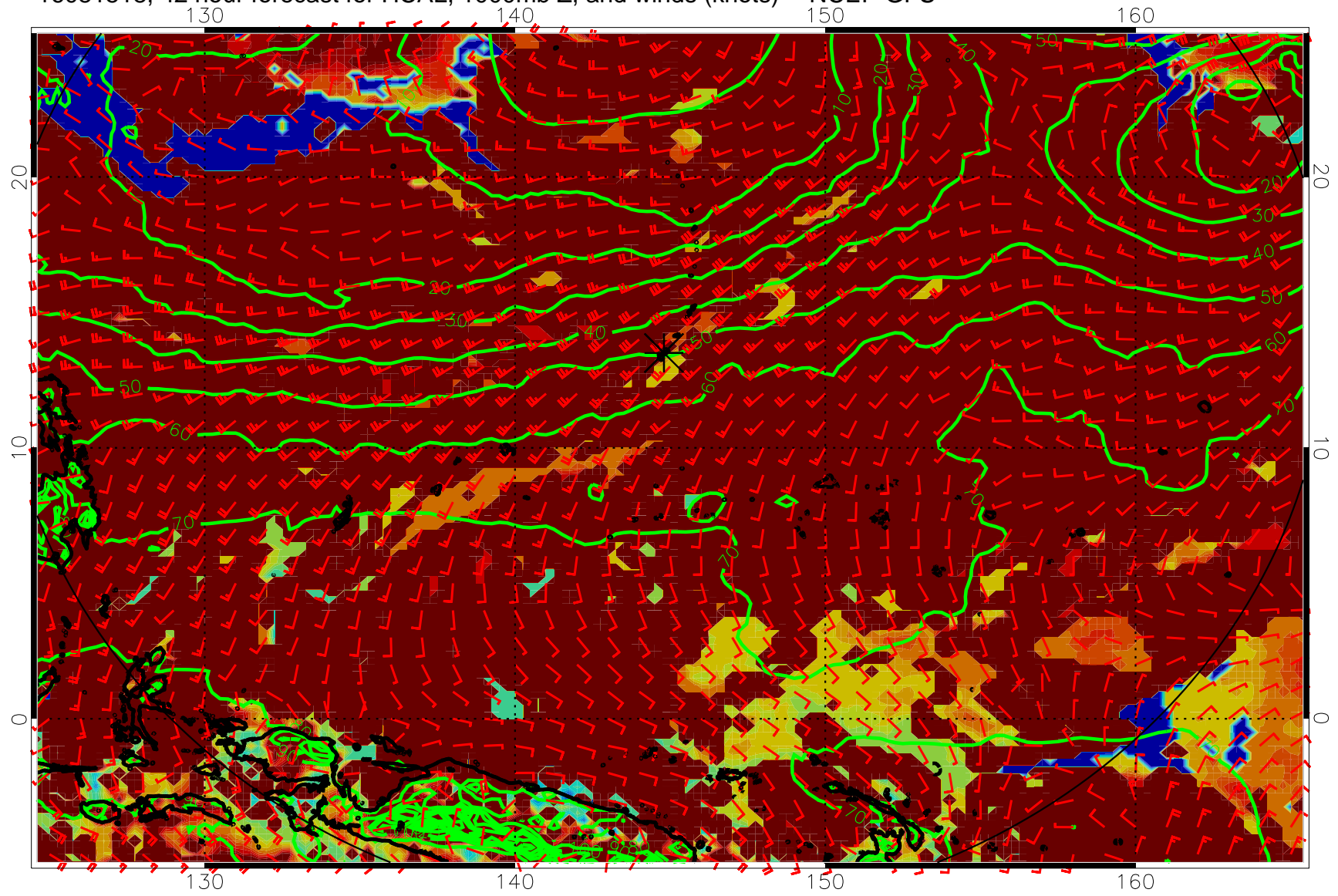
16081518, 42 hour forecast for HCAL, 1000mb Z, and winds (knots) -- NCEP GFS
