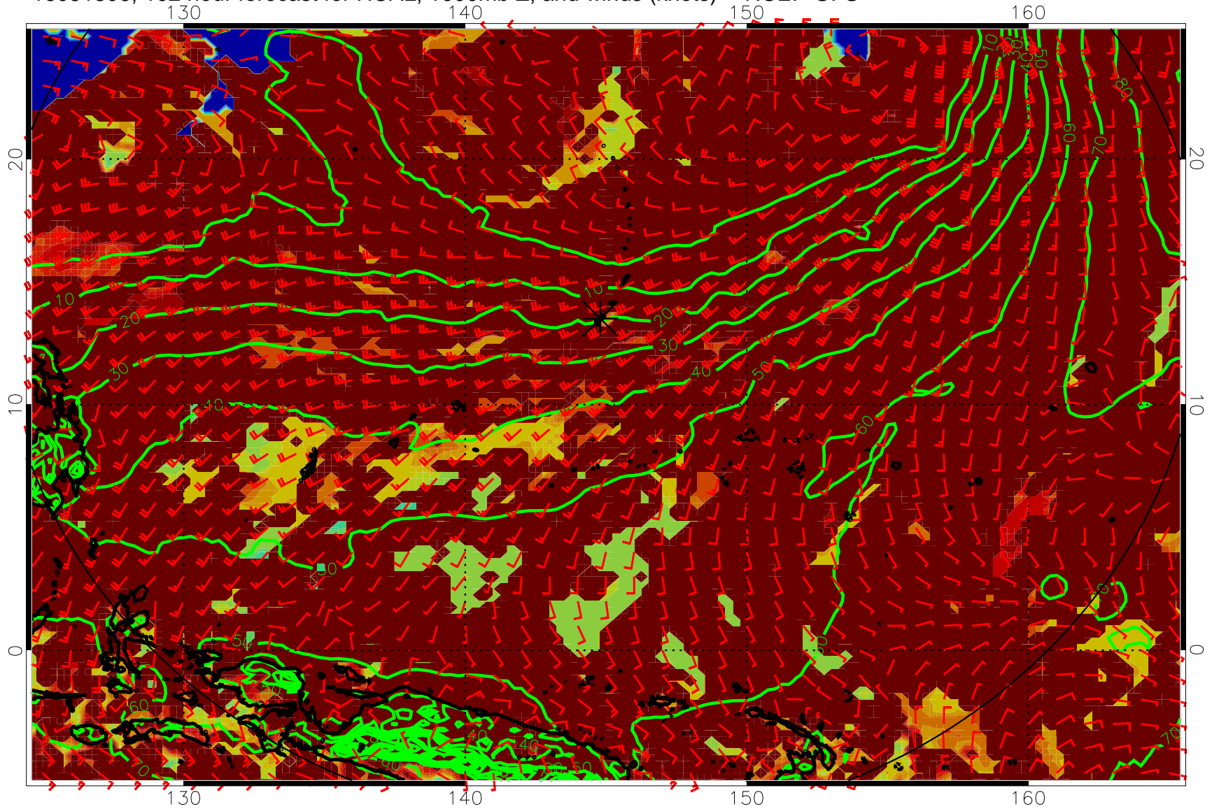
16081806, 102 hour forecast for HCAL, 1000mb Z, and winds (knots) -- NCEP GFS
