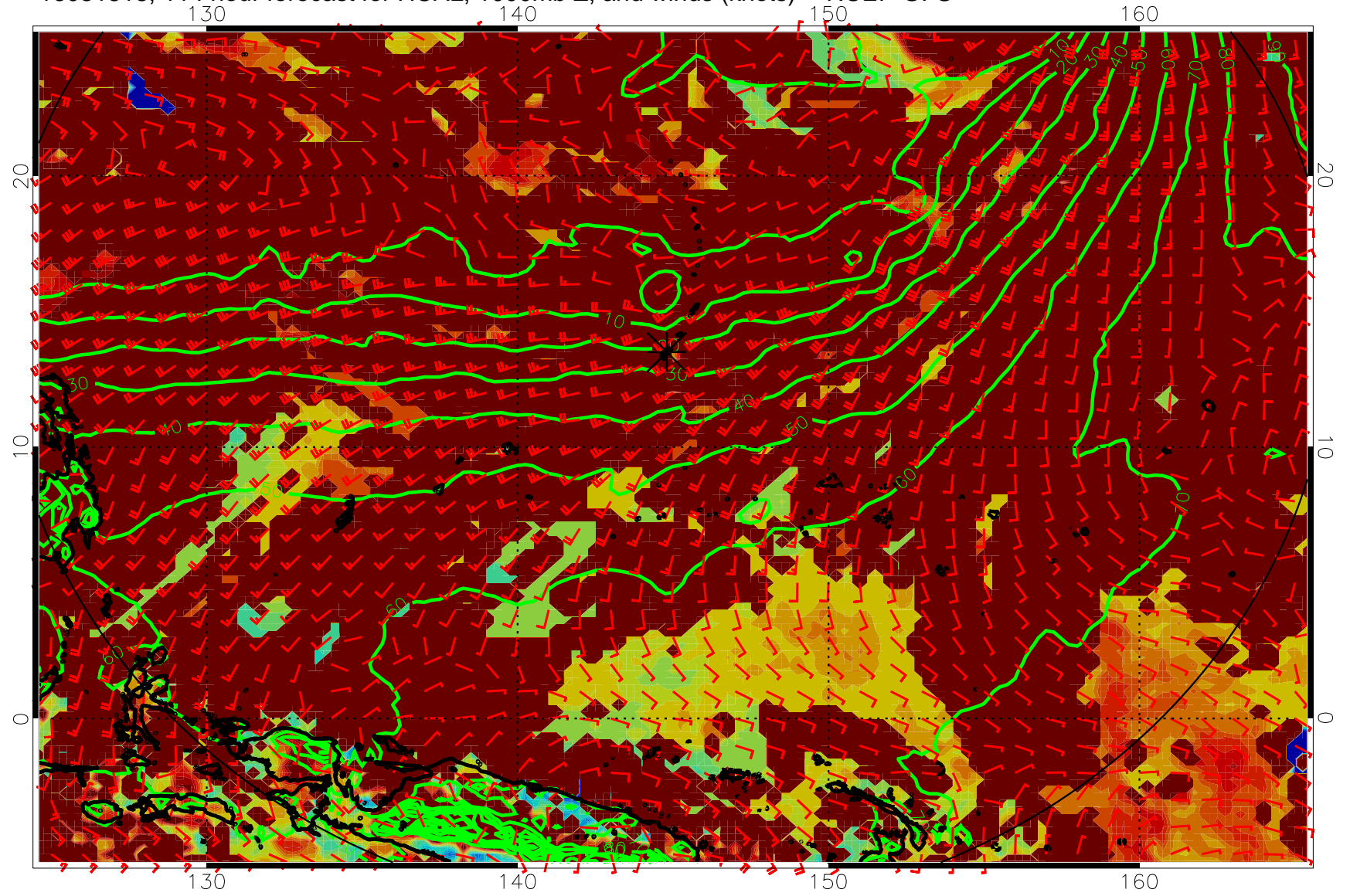
16081818, 114 hour forecast for HCAL, 1000mb Z, and winds (knots) -- NCEP GFS
