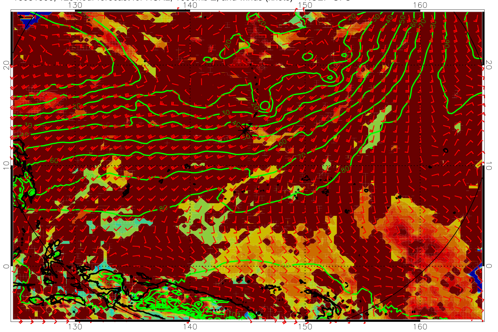
16081900, 120 hour forecast for HCAL, 1000mb Z, and winds (knots) -- NCEP GFS
