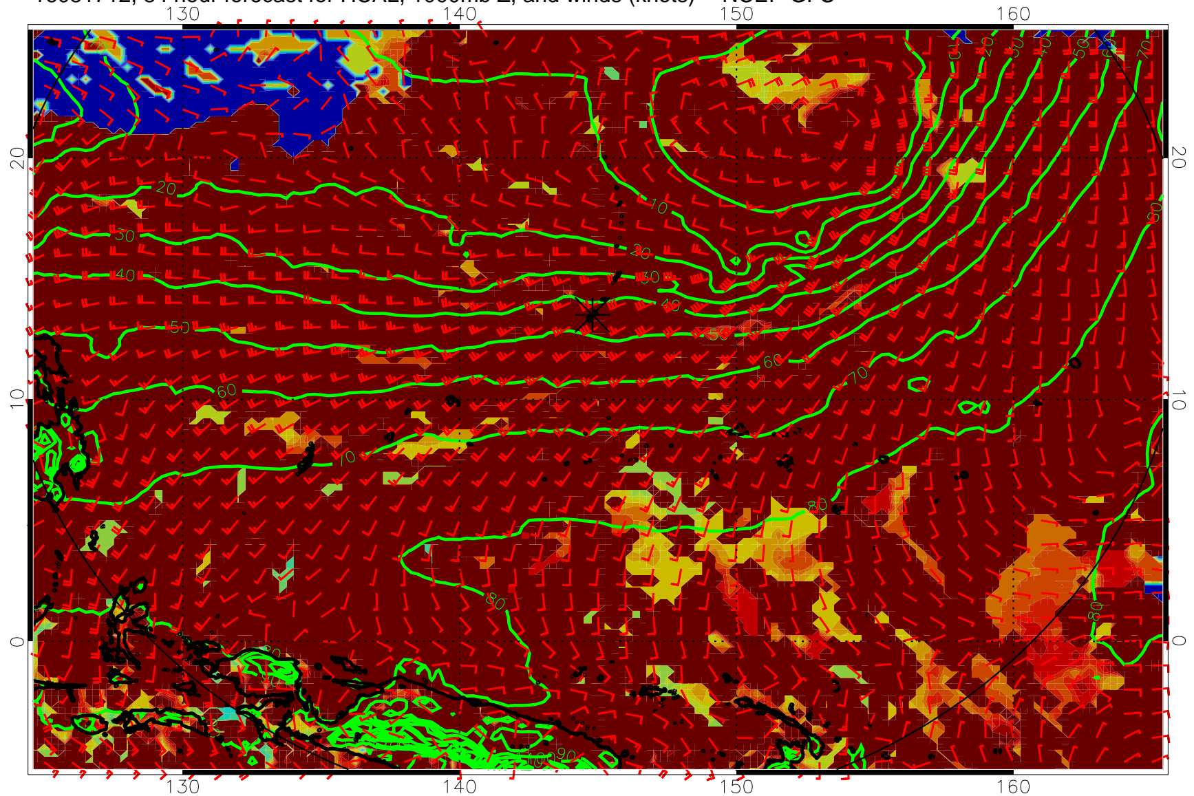
16081712, 84 hour forecast for HCAL, 1000mb Z, and winds (knots) -- NCEP GFS
