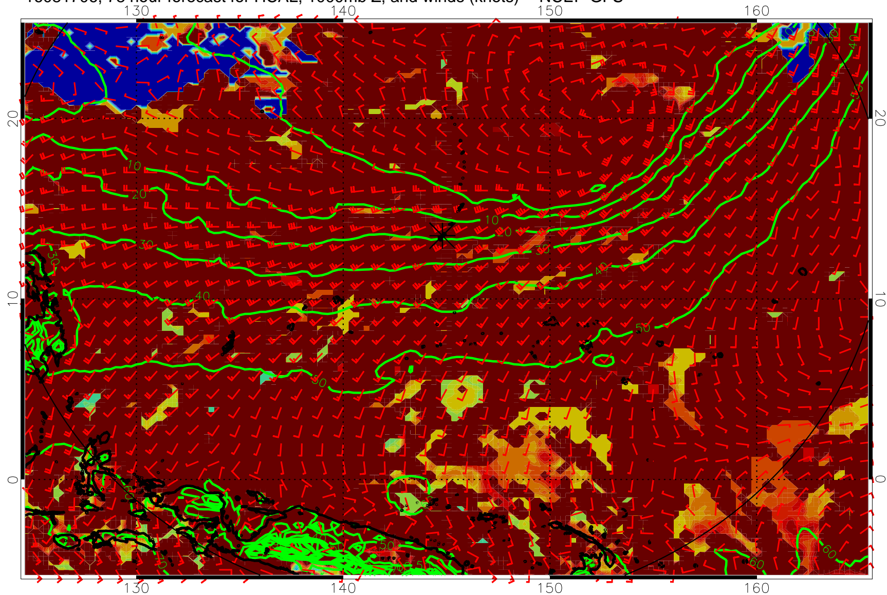
16081706, 78 hour forecast for HCAL, 1000mb Z, and winds (knots) -- NCEP GFS
