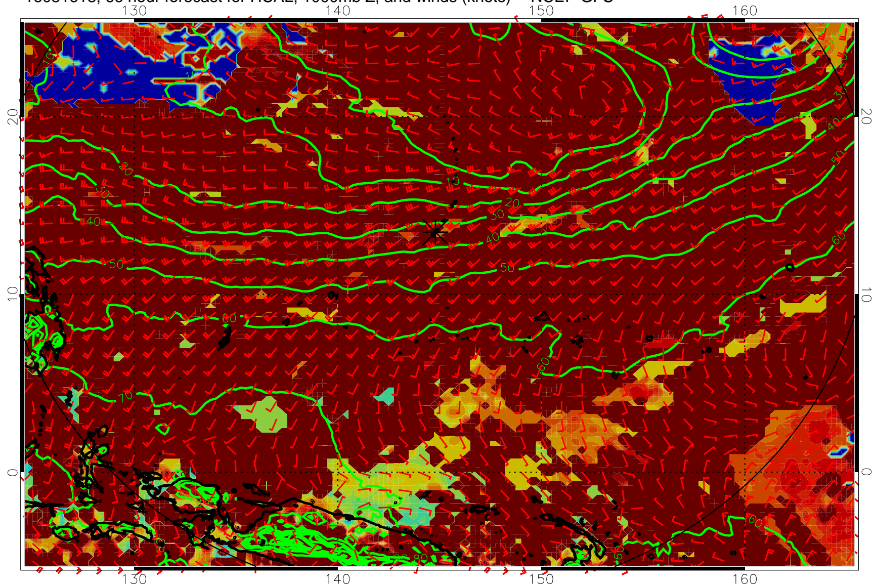
16081618, 66 hour forecast for HCAL, 1000mb Z, and winds (knots) -- NCEP GFS
