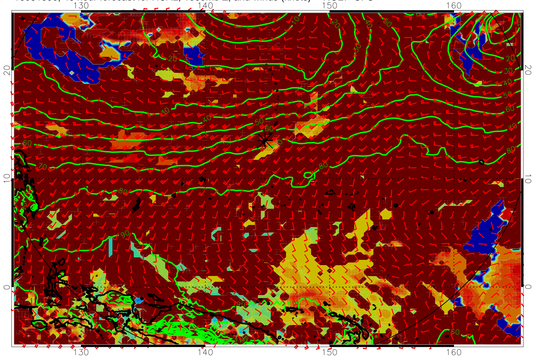
16081600, 48 hour forecast for HCAL, 1000mb Z, and winds (knots) -- NCEP GFS
