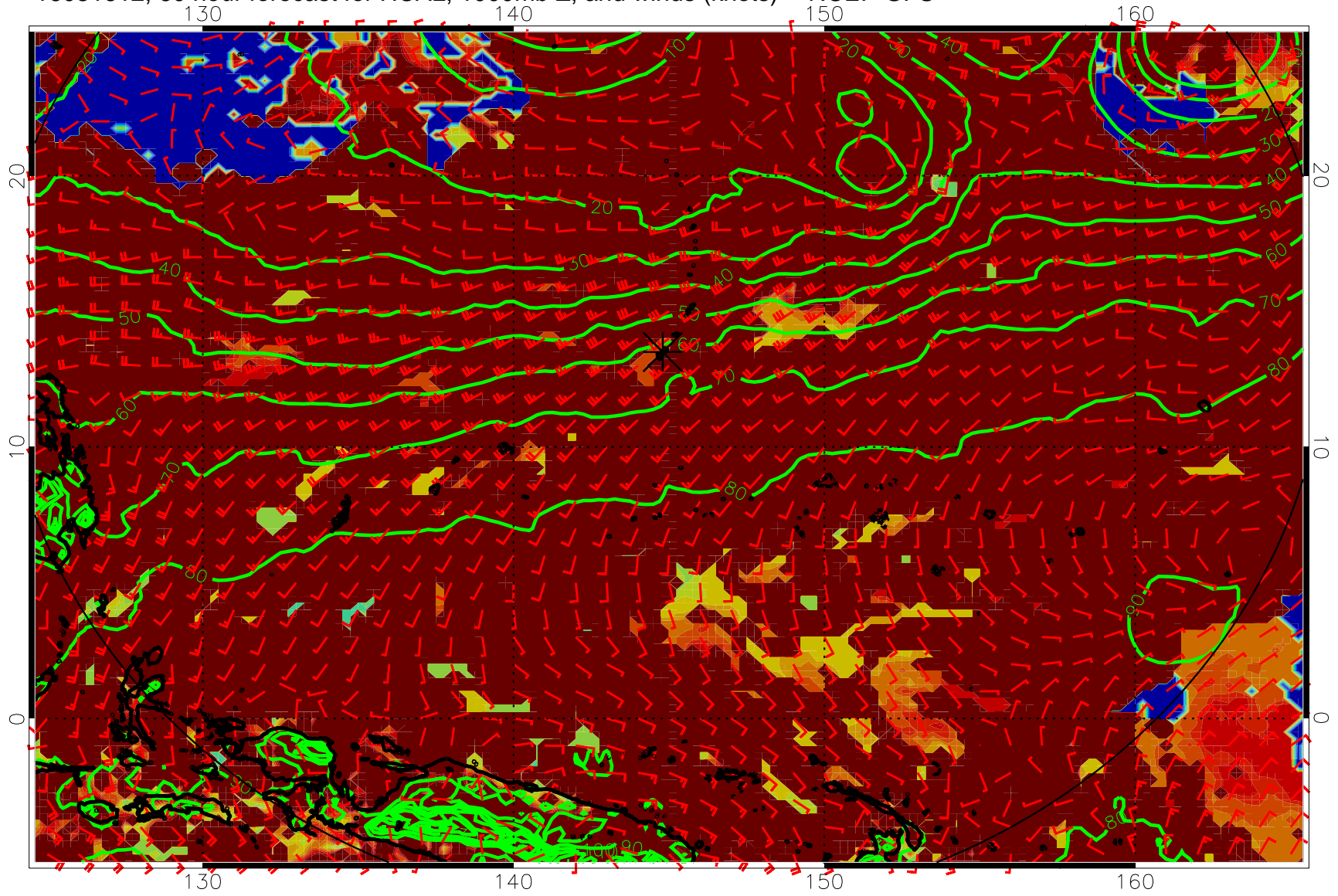
16081612, 60 hour forecast for HCAL, 1000mb Z, and winds (knots) -- NCEP GFS
