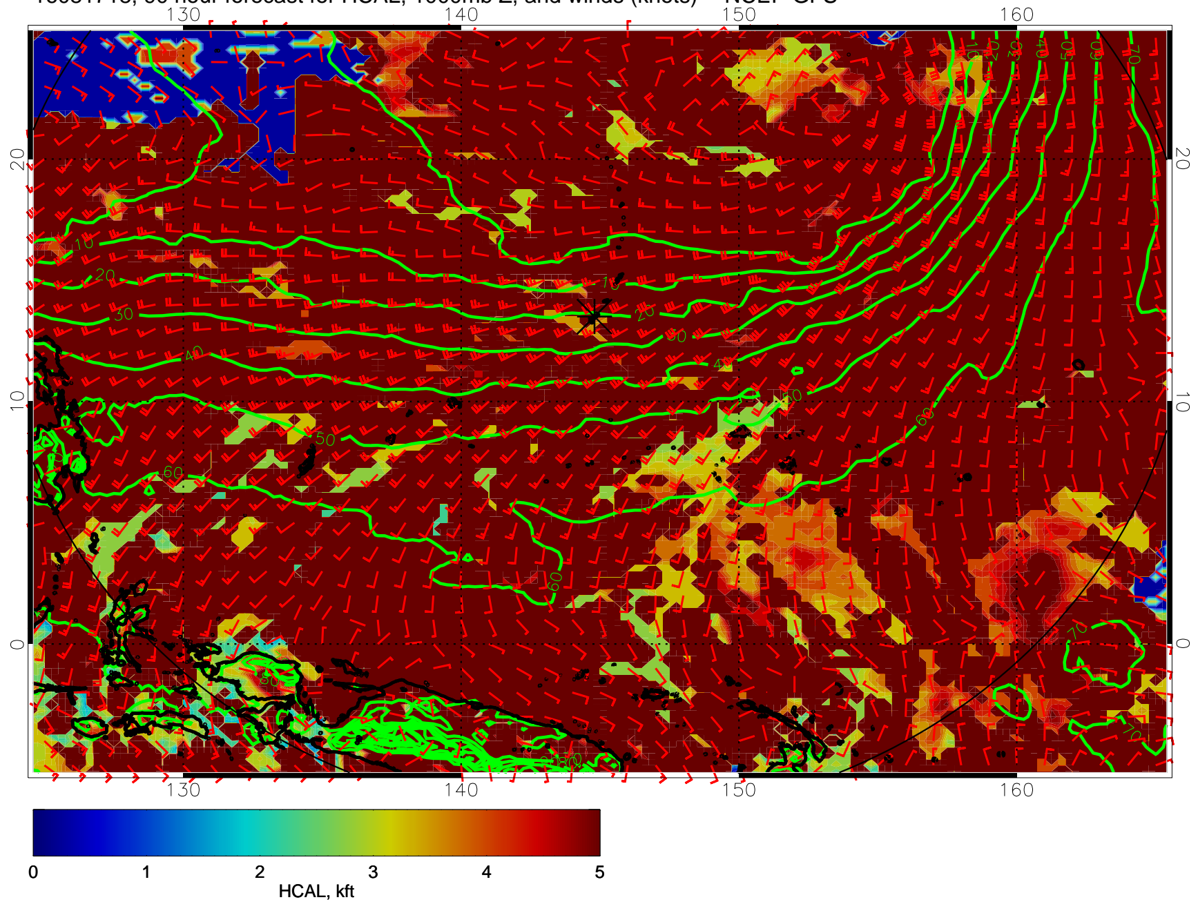
16081718, 90 hour forecast for HCAL, 1000mb Z, and winds (knots) -- NCEP GFS
