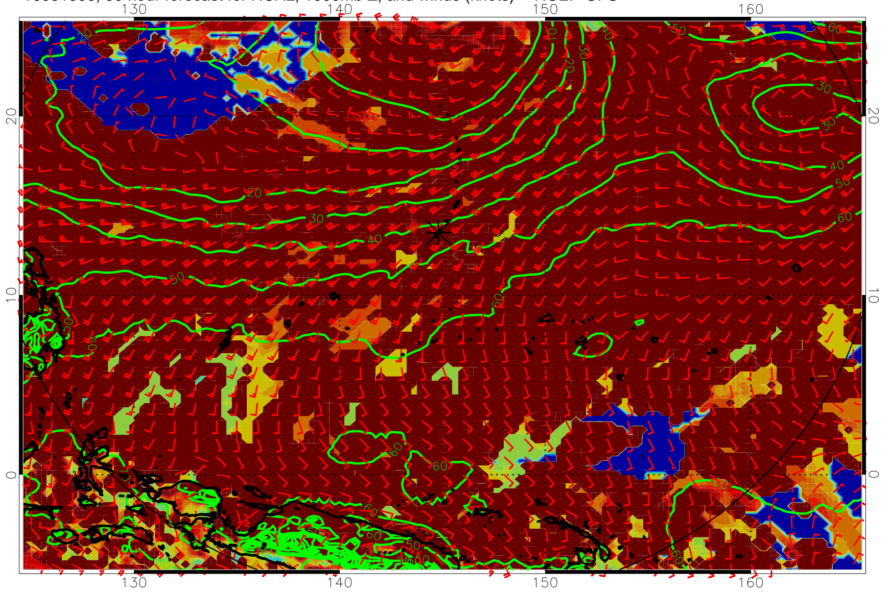
16081506, 30 hour forecast for HCAL, 1000mb Z, and winds (knots) -- NCEP GFS
