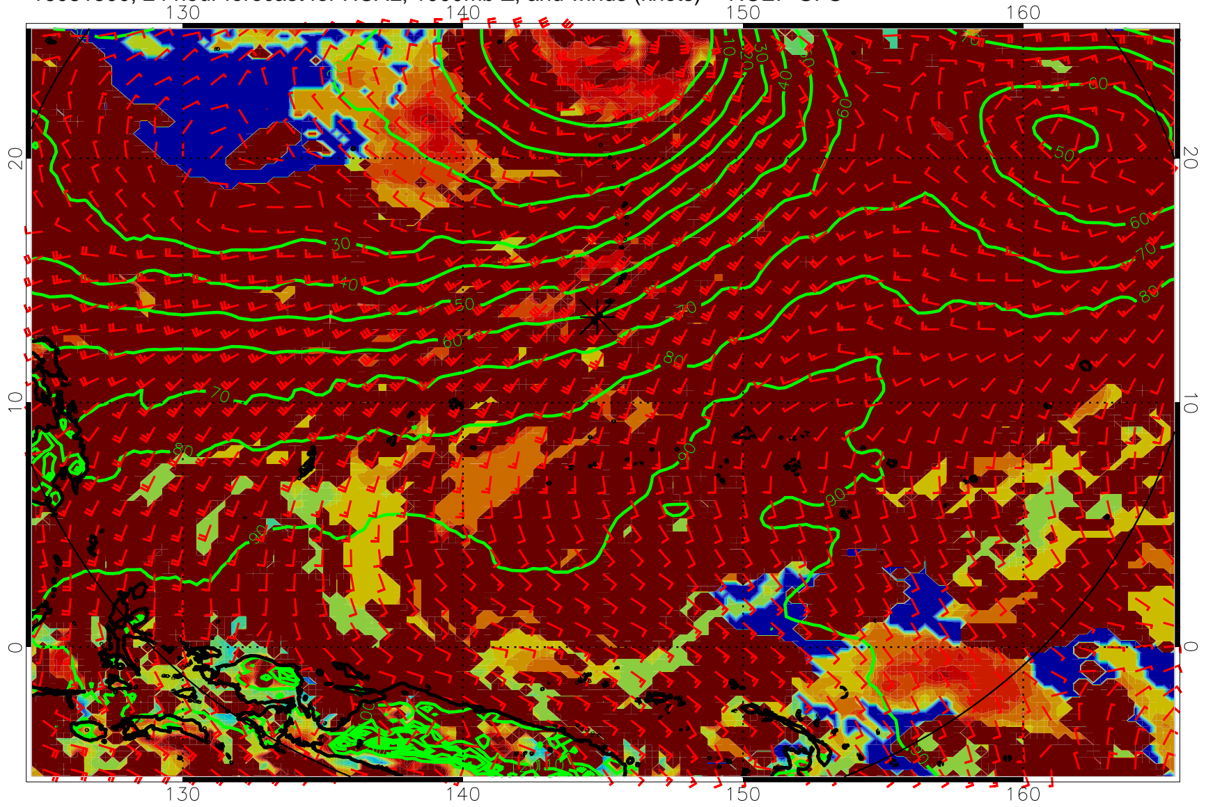
16081500, 24 hour forecast for HCAL, 1000mb Z, and winds (knots) -- NCEP GFS
