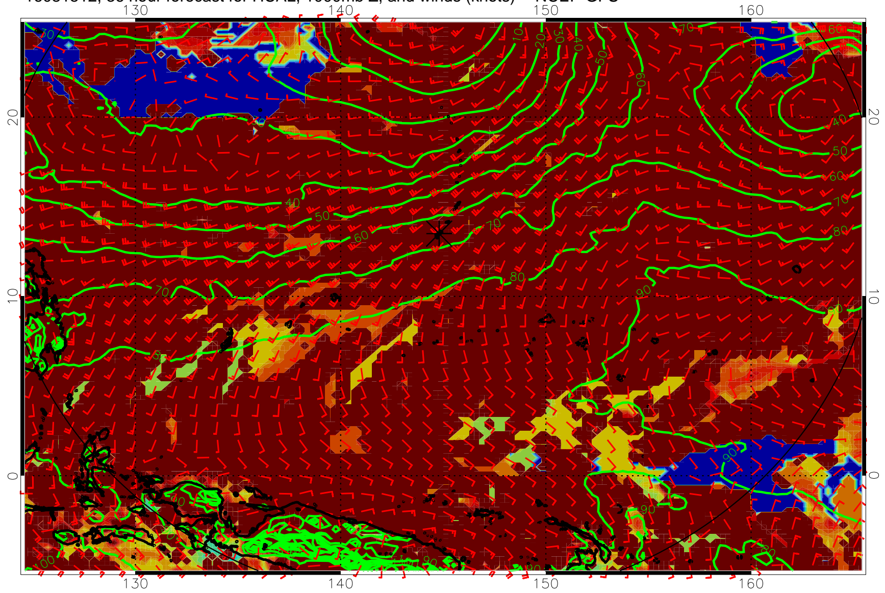
16081512, 36 hour forecast for HCAL, 1000mb Z, and winds (knots) -- NCEP GFS
