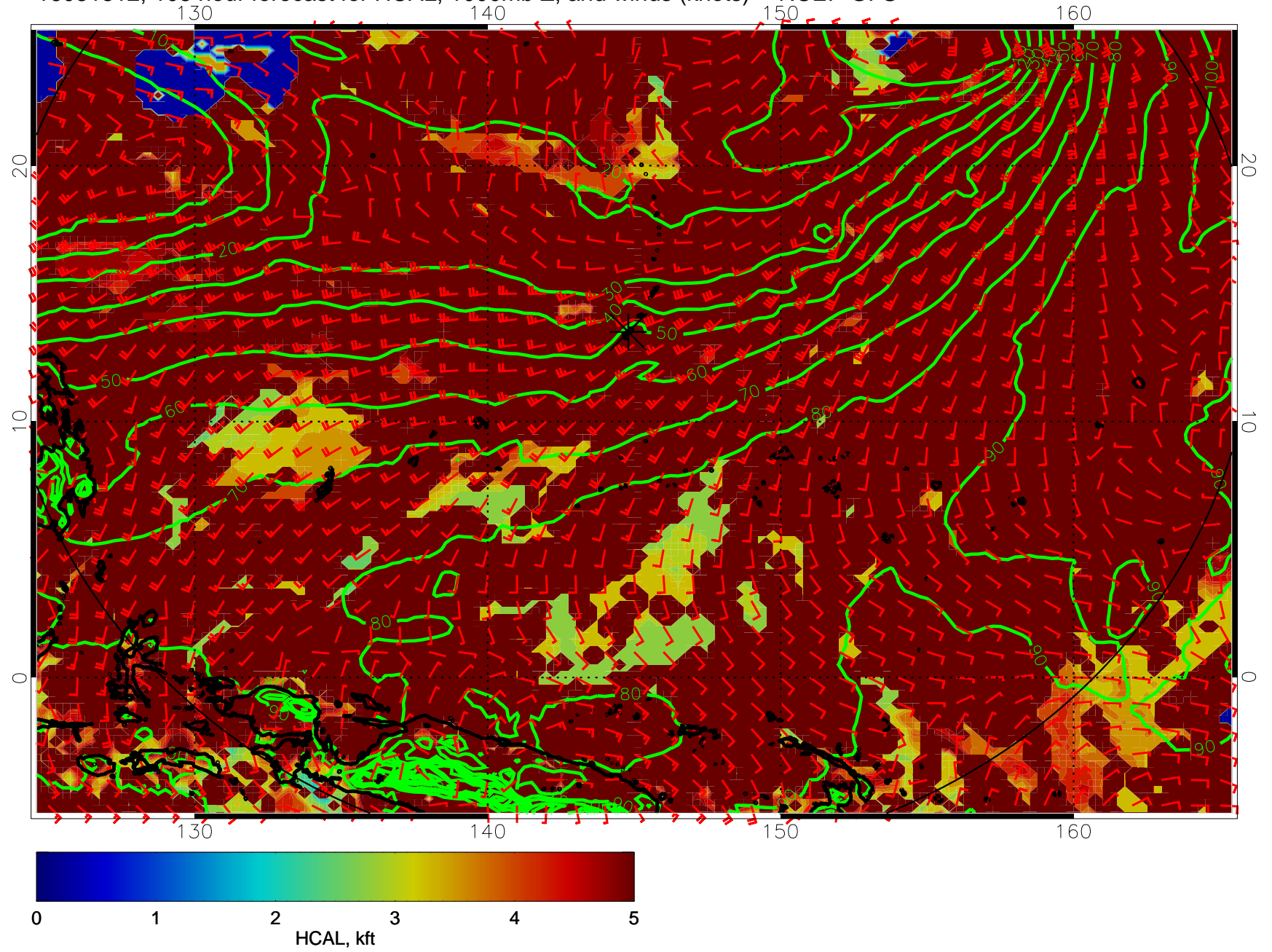
16081812, 108 hour forecast for HCAL, 1000mb Z, and winds (knots) -- NCEP GFS
