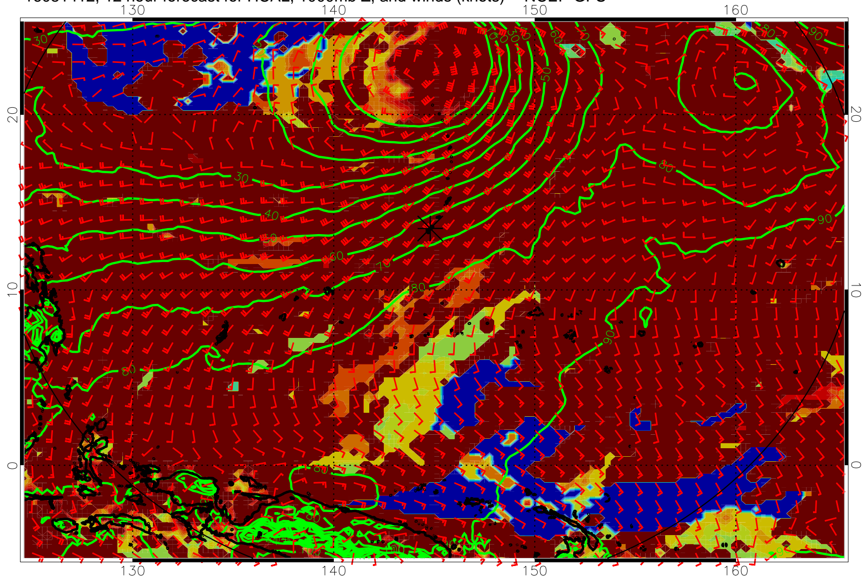
16081412, 12 hour forecast for HCAL, 1000mb Z, and winds (knots) -- NCEP GFS
