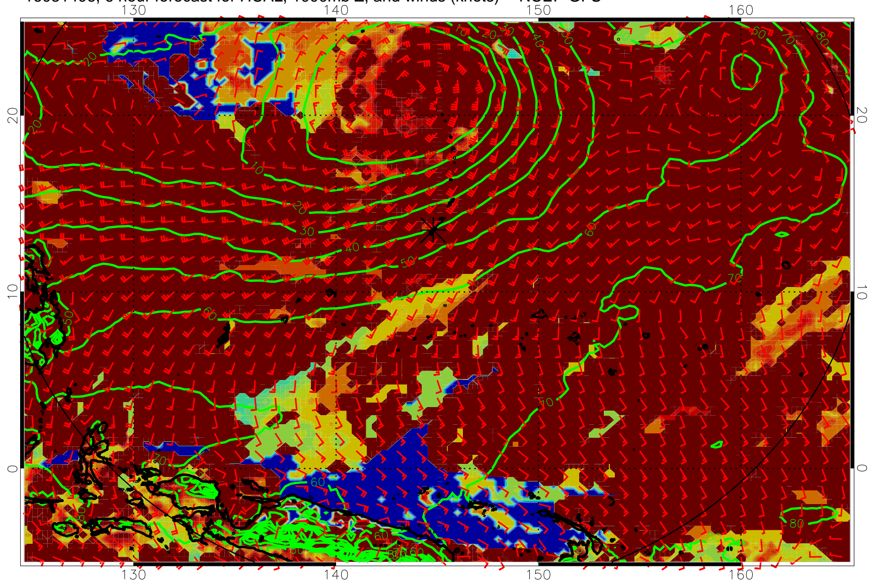
16081406, 6 hour forecast for HCAL, 1000mb Z, and winds (knots) -- NCEP GFS
