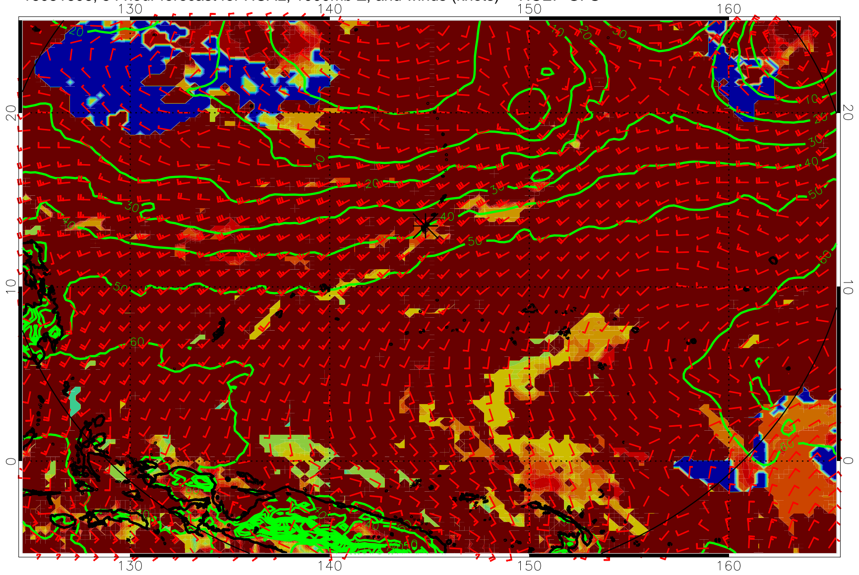
16081606, 54 hour forecast for HCAL, 1000mb Z, and winds (knots) -- NCEP GFS
