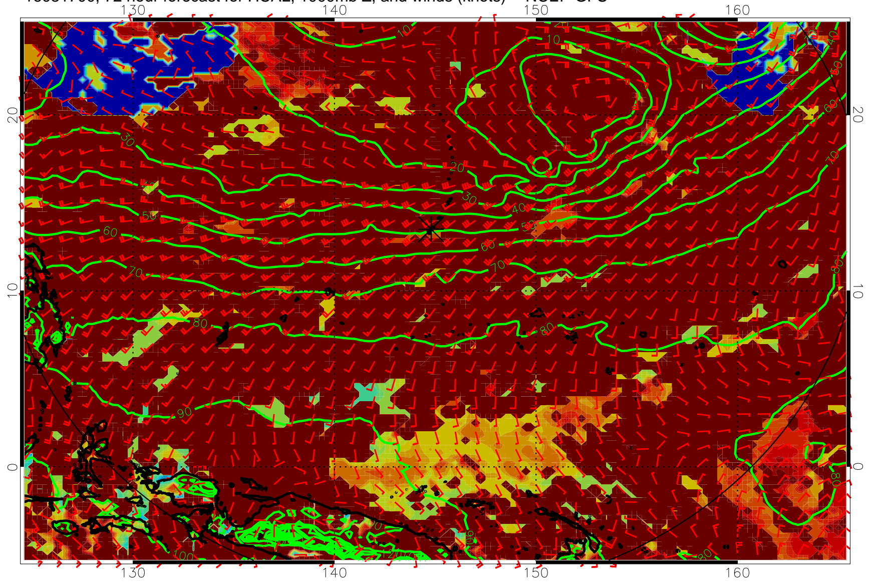
16081700, 72 hour forecast for HCAL, 1000mb Z, and winds (knots) -- NCEP GFS
