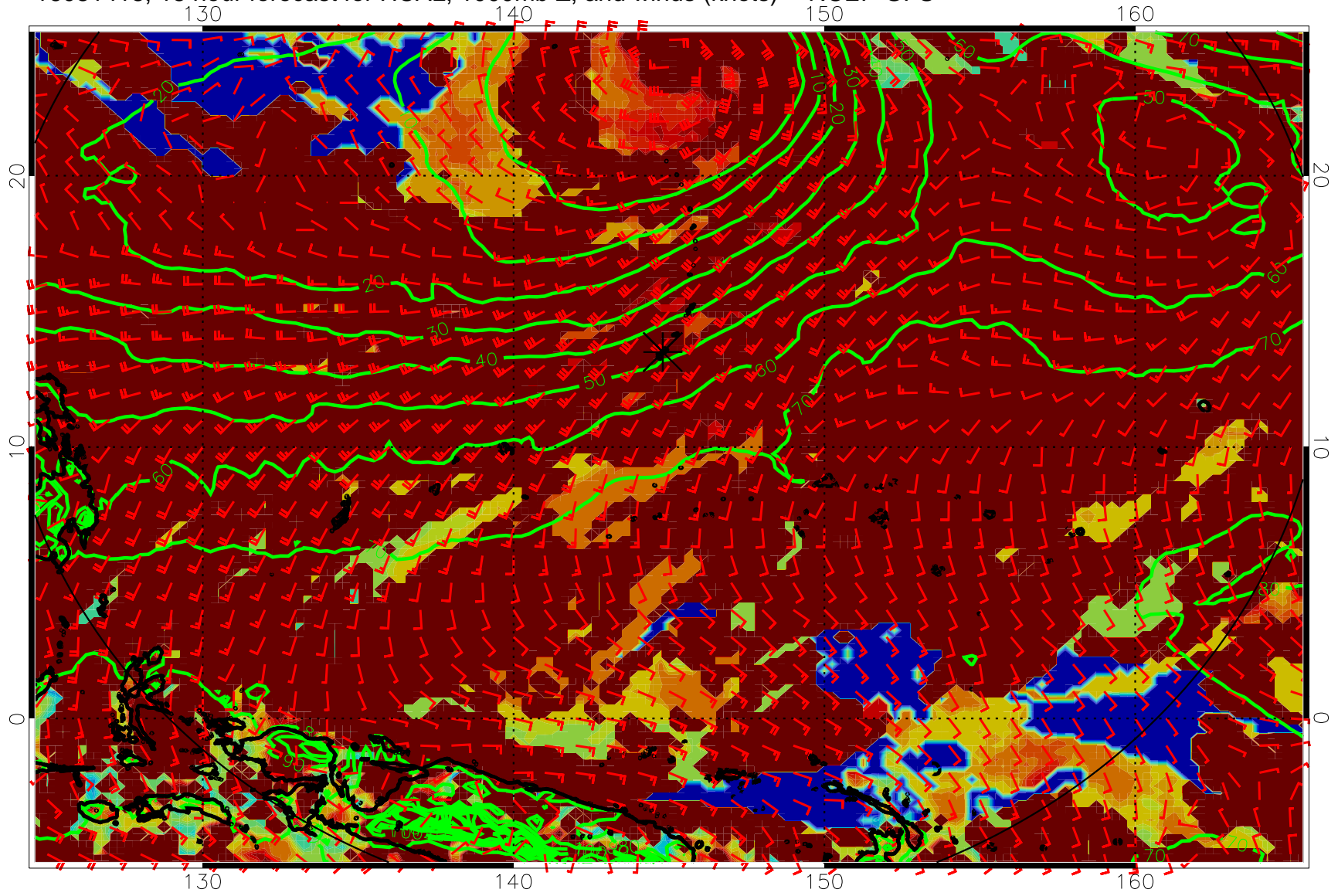
16081418, 18 hour forecast for HCAL, 1000mb Z, and winds (knots) -- NCEP GFS
