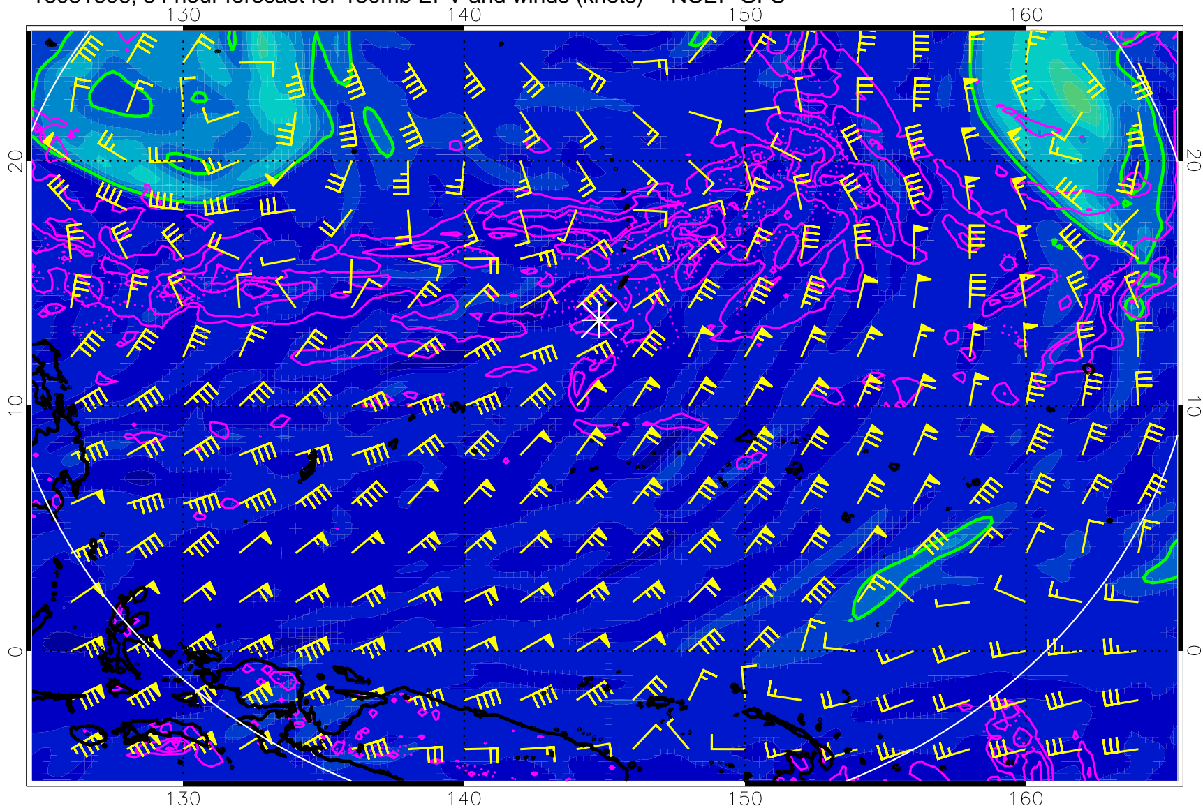
16081606, 54 hour forecast for 150mb EPV and winds (knots) -- NCEP GFS
