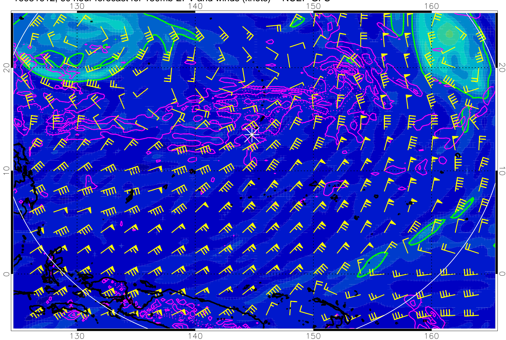
16081612, 60 hour forecast for 150mb EPV and winds (knots) -- NCEP GFS
