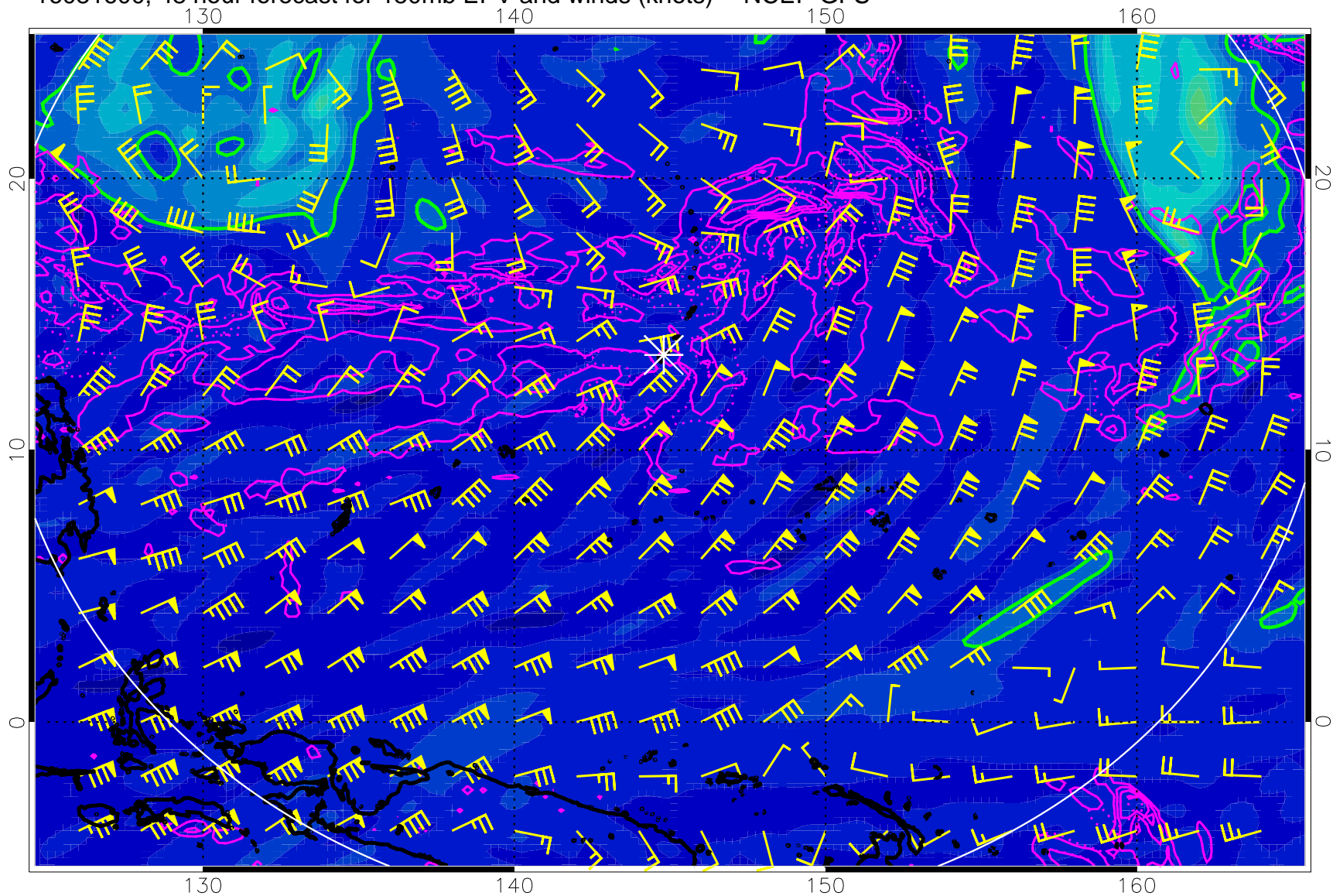
16081600, 48 hour forecast for 150mb EPV and winds (knots) -- NCEP GFS
