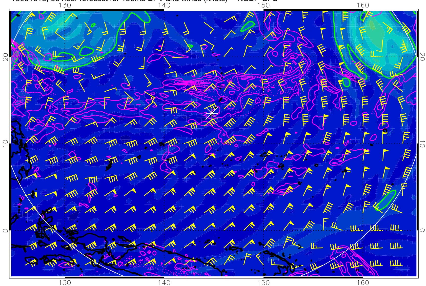
16081618, 66 hour forecast for 150mb EPV and winds (knots) -- NCEP GFS
