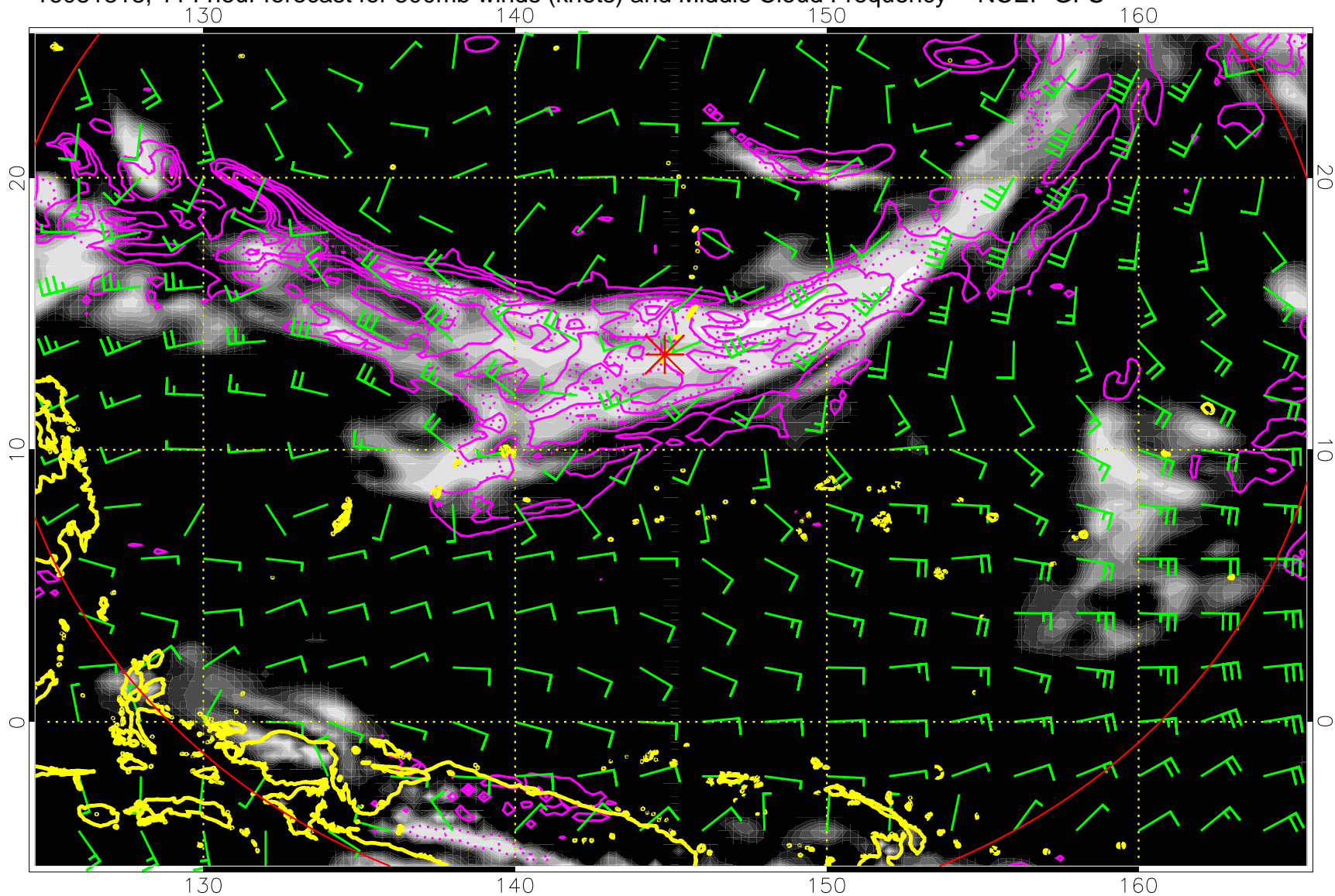
16081818, 114 hour forecast for 500mb winds (knots) and Middle Cloud Frequency -- NCEP GFS
