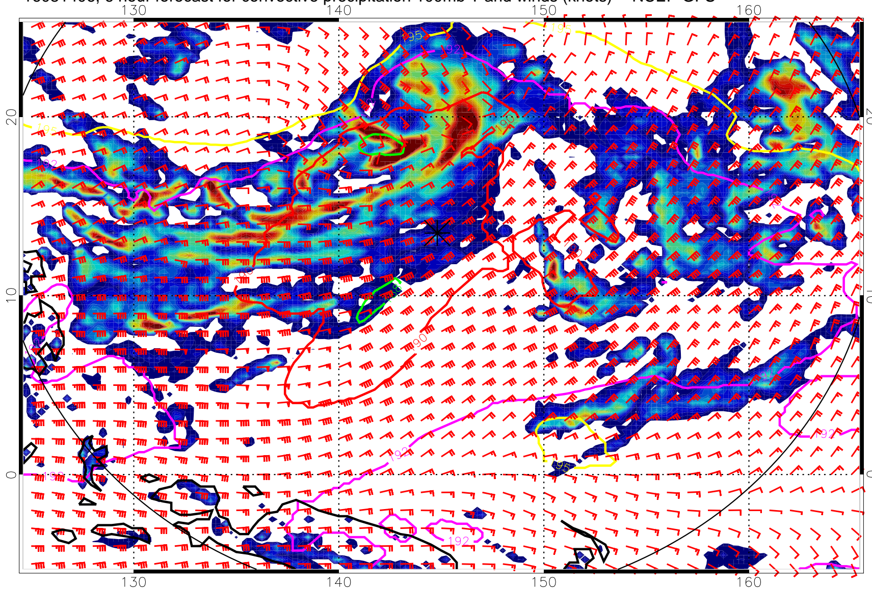
16081406, 6 hour forecast for convective precipitation 100mb T and winds (knots) -- NCEP GFS
