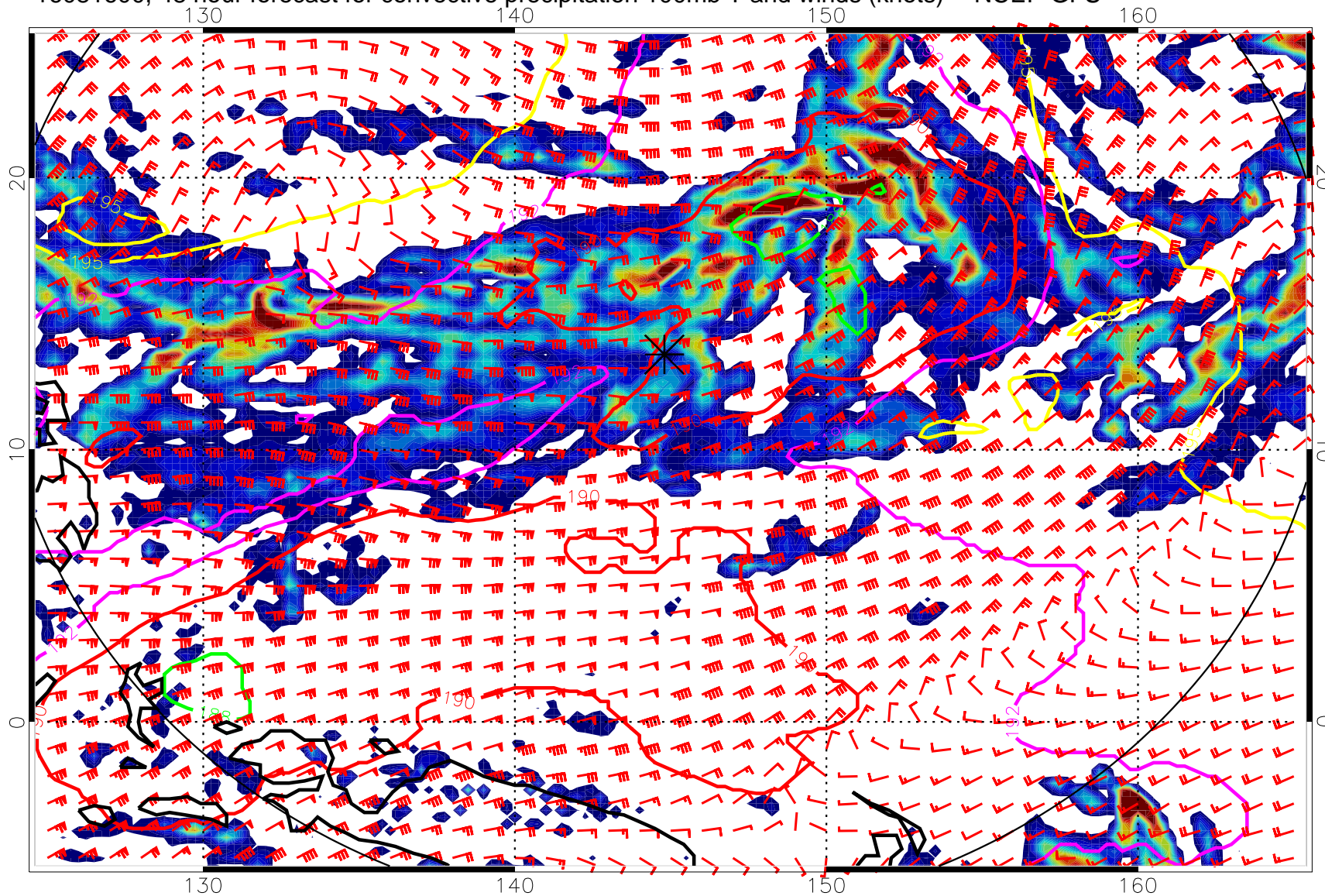
16081600, 48 hour forecast for convective precipitation 100mb T and winds (knots) -- NCEP GFS
