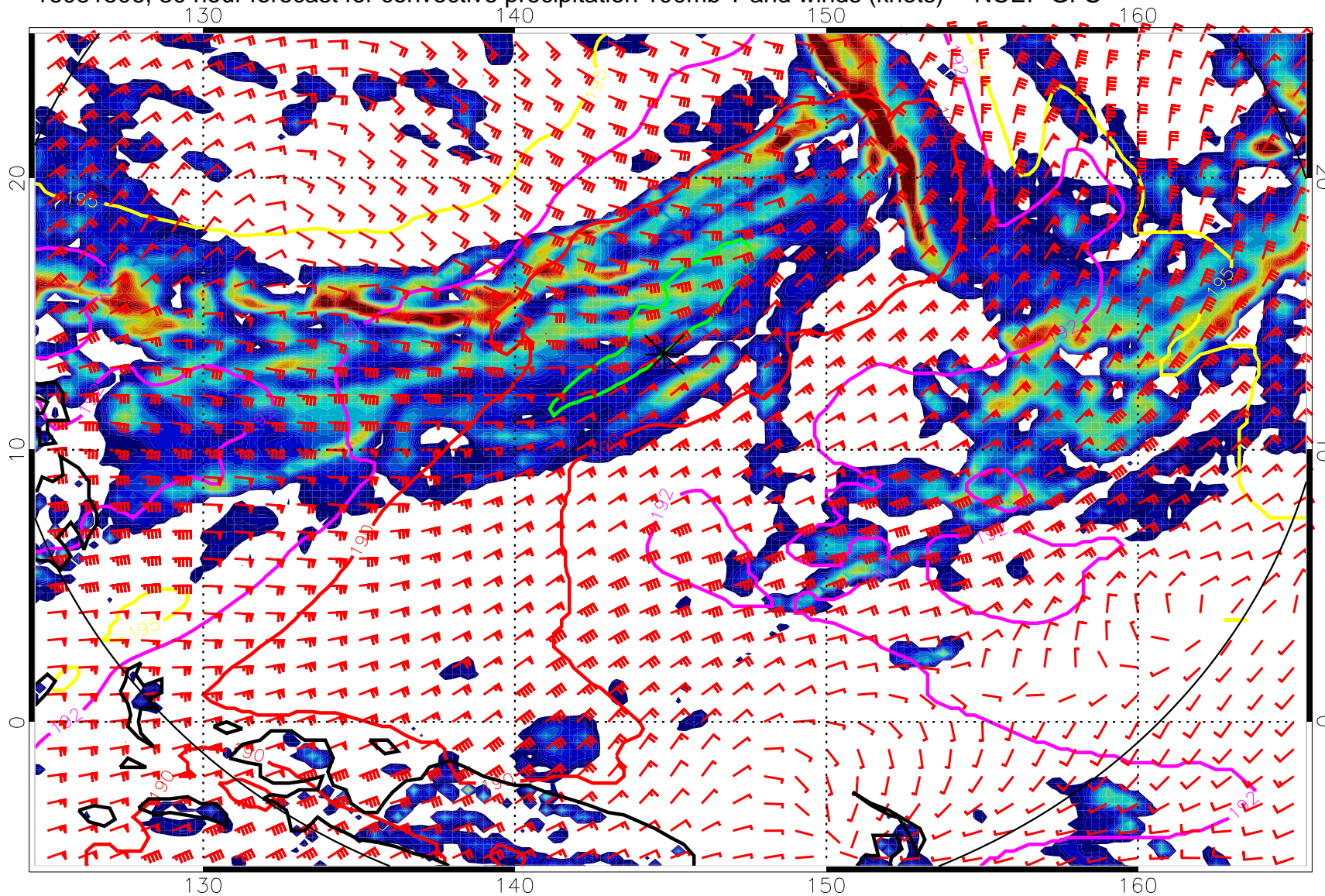
16081506, 30 hour forecast for convective precipitation 100mb T and winds (knots) -- NCEP GFS
