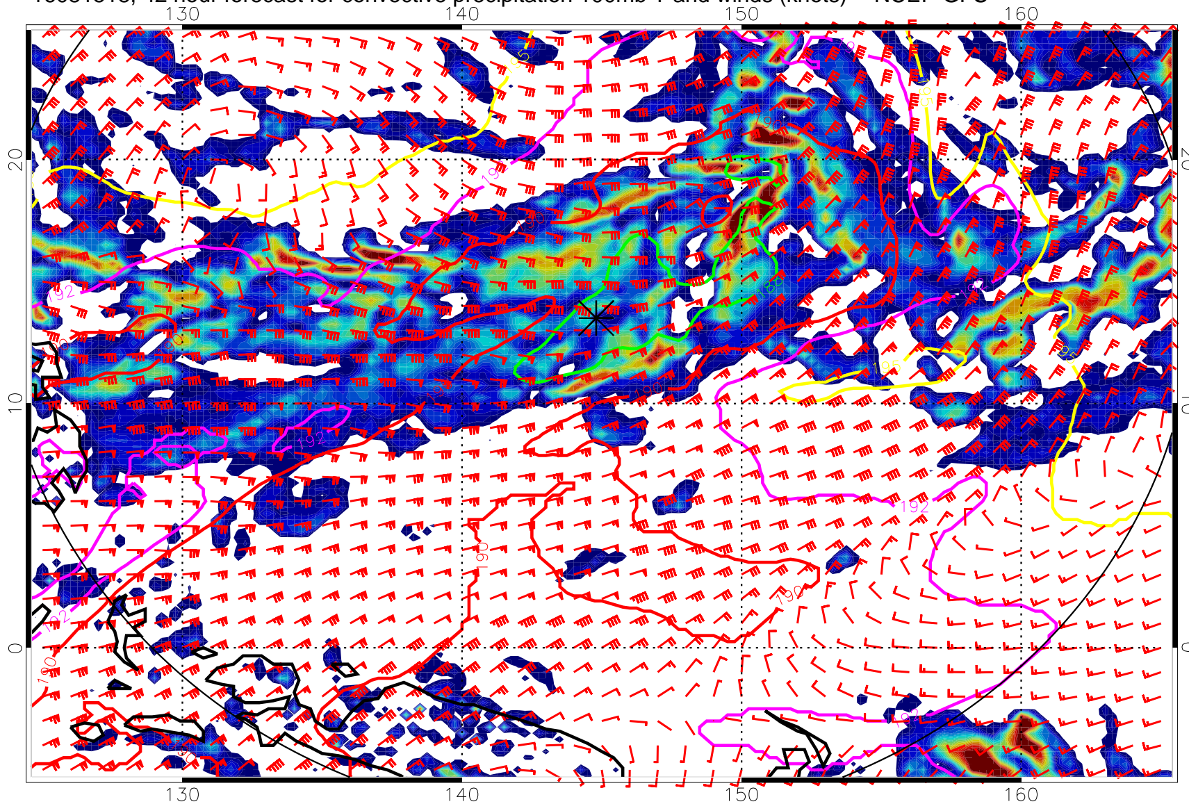
16081518, 42 hour forecast for convective precipitation 100mb T and winds (knots) -- NCEP GFS
