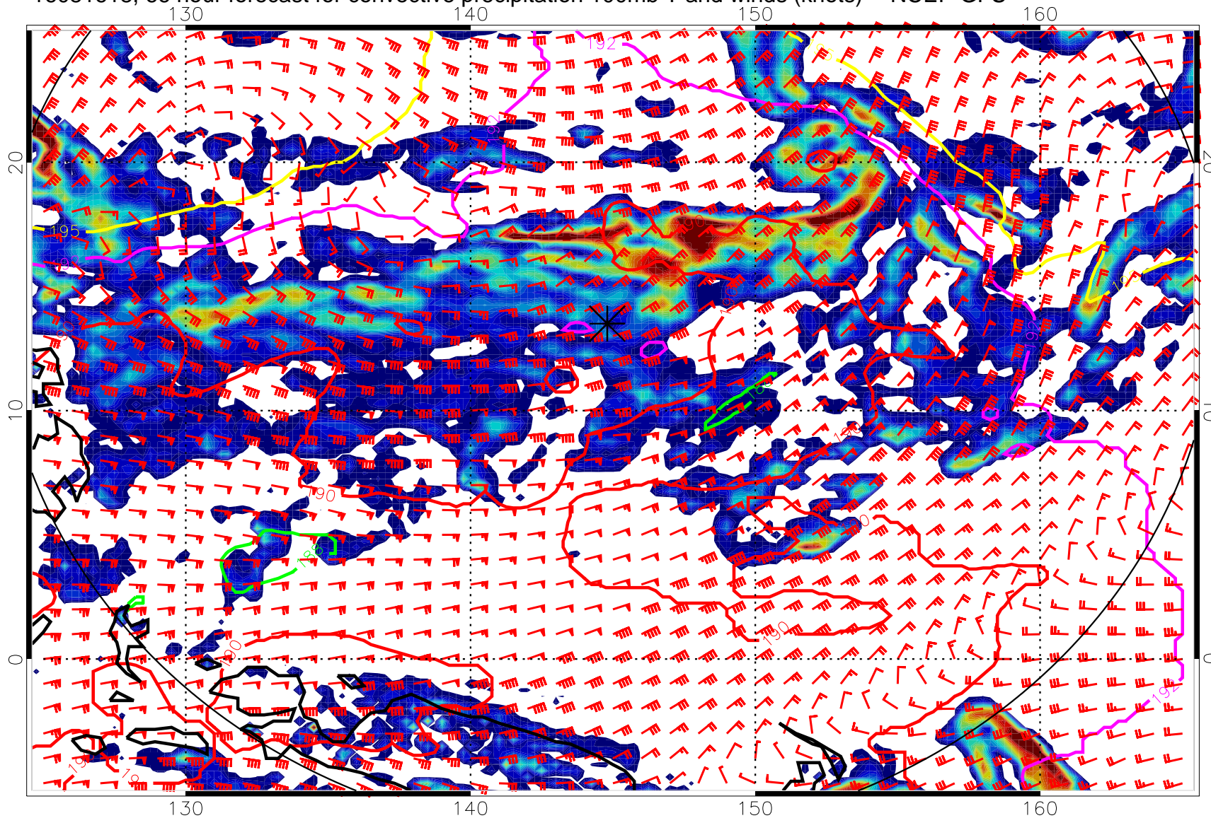
16081618, 66 hour forecast for convective precipitation 100mb T and winds (knots) -- NCEP GFS
