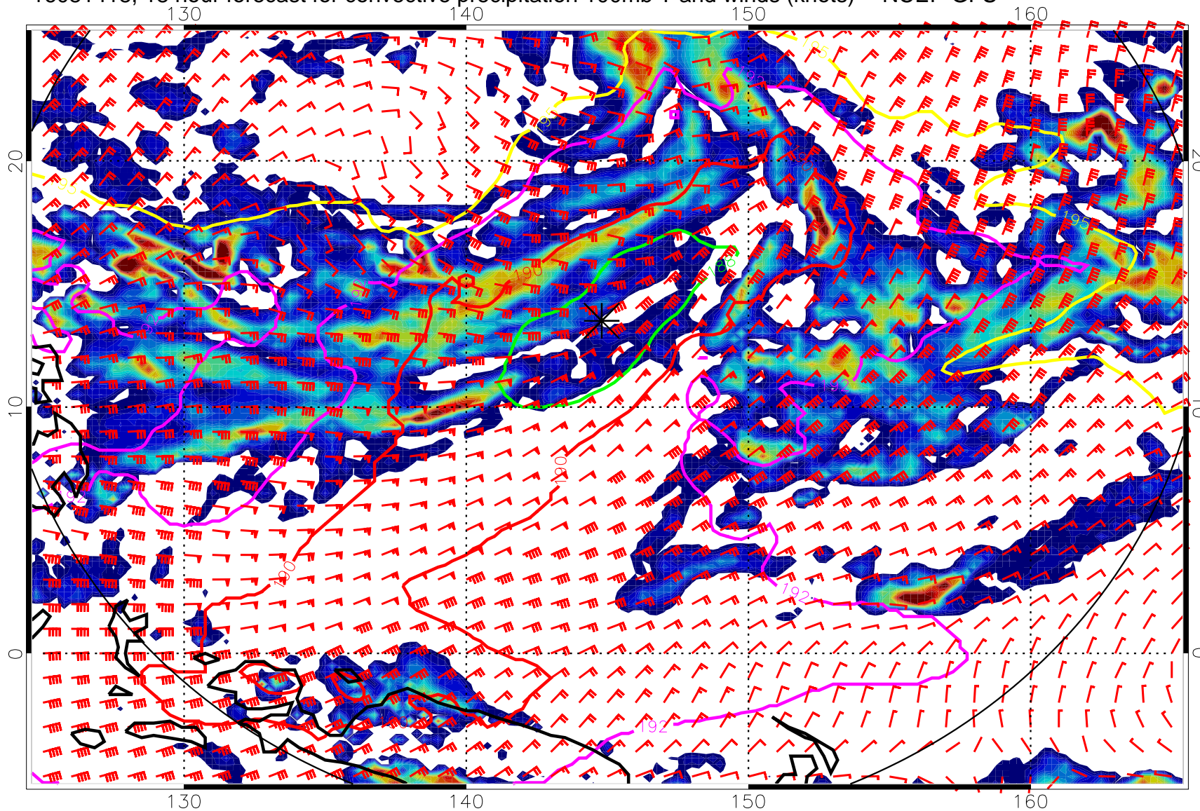
16081418, 18 hour forecast for convective precipitation 100mb T and winds (knots) -- NCEP GFS
