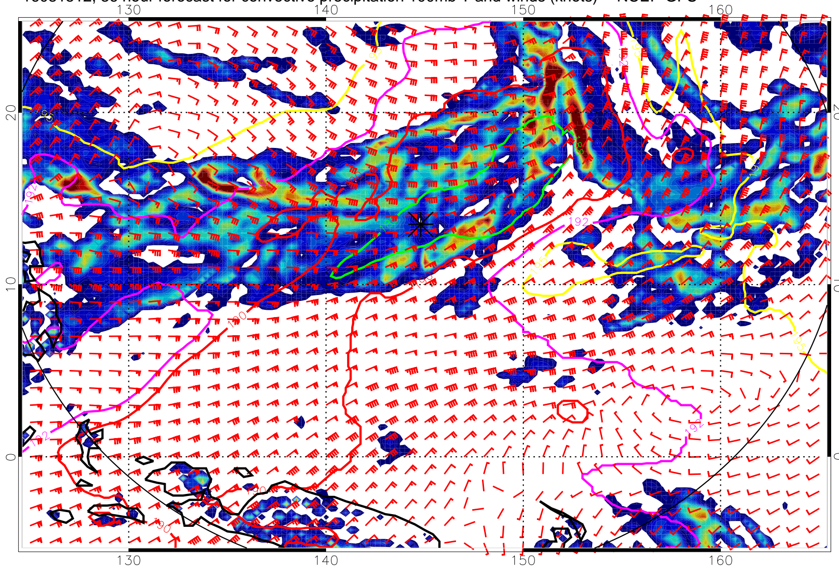
16081512, 36 hour forecast for convective precipitation 100mb T and winds (knots) -- NCEP GFS
