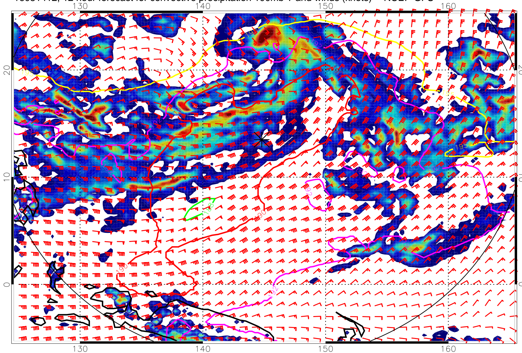
16081412, 12 hour forecast for convective precipitation 100mb T and winds (knots) -- NCEP GFS
