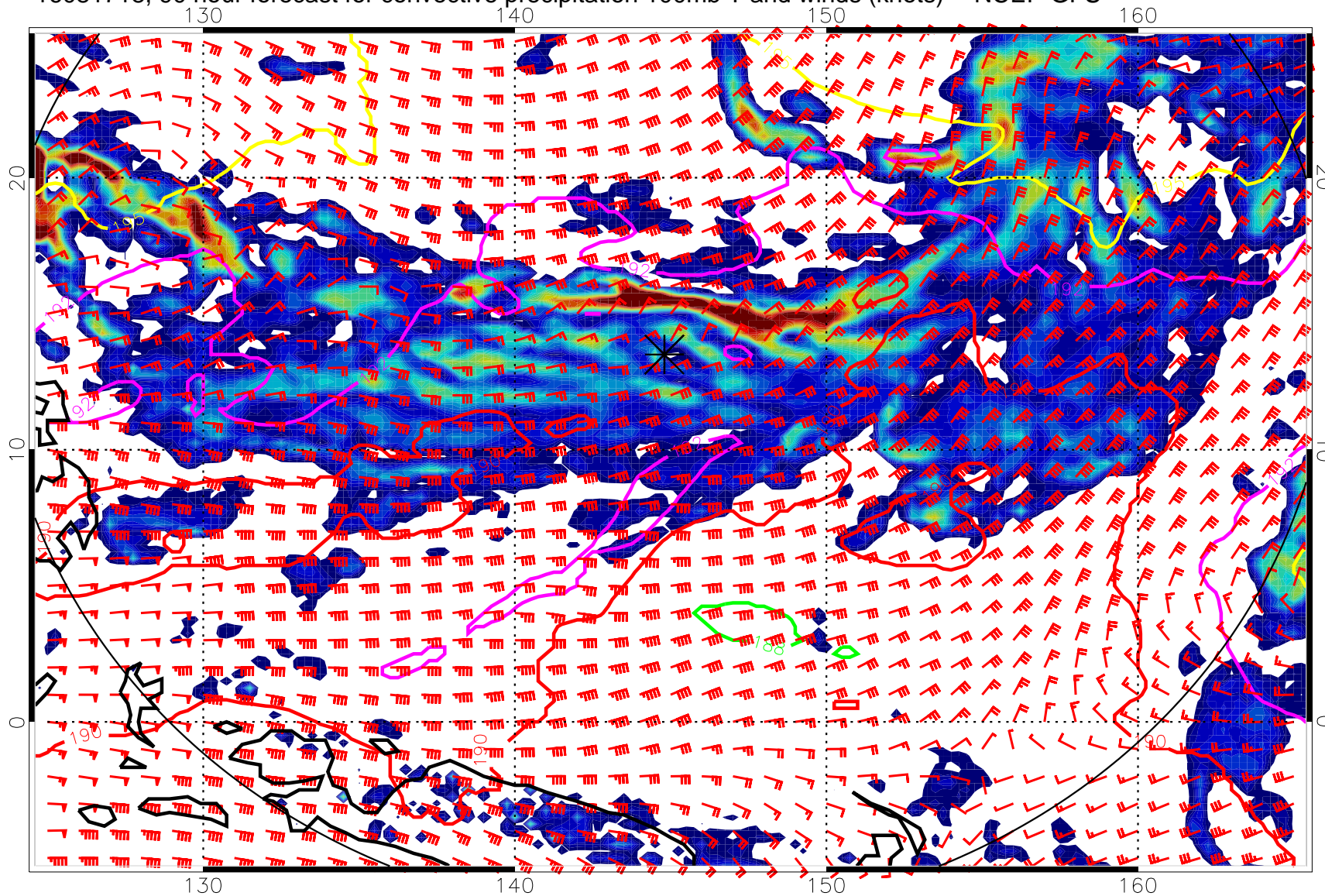
16081718, 90 hour forecast for convective precipitation 100mb T and winds (knots) -- NCEP GFS
