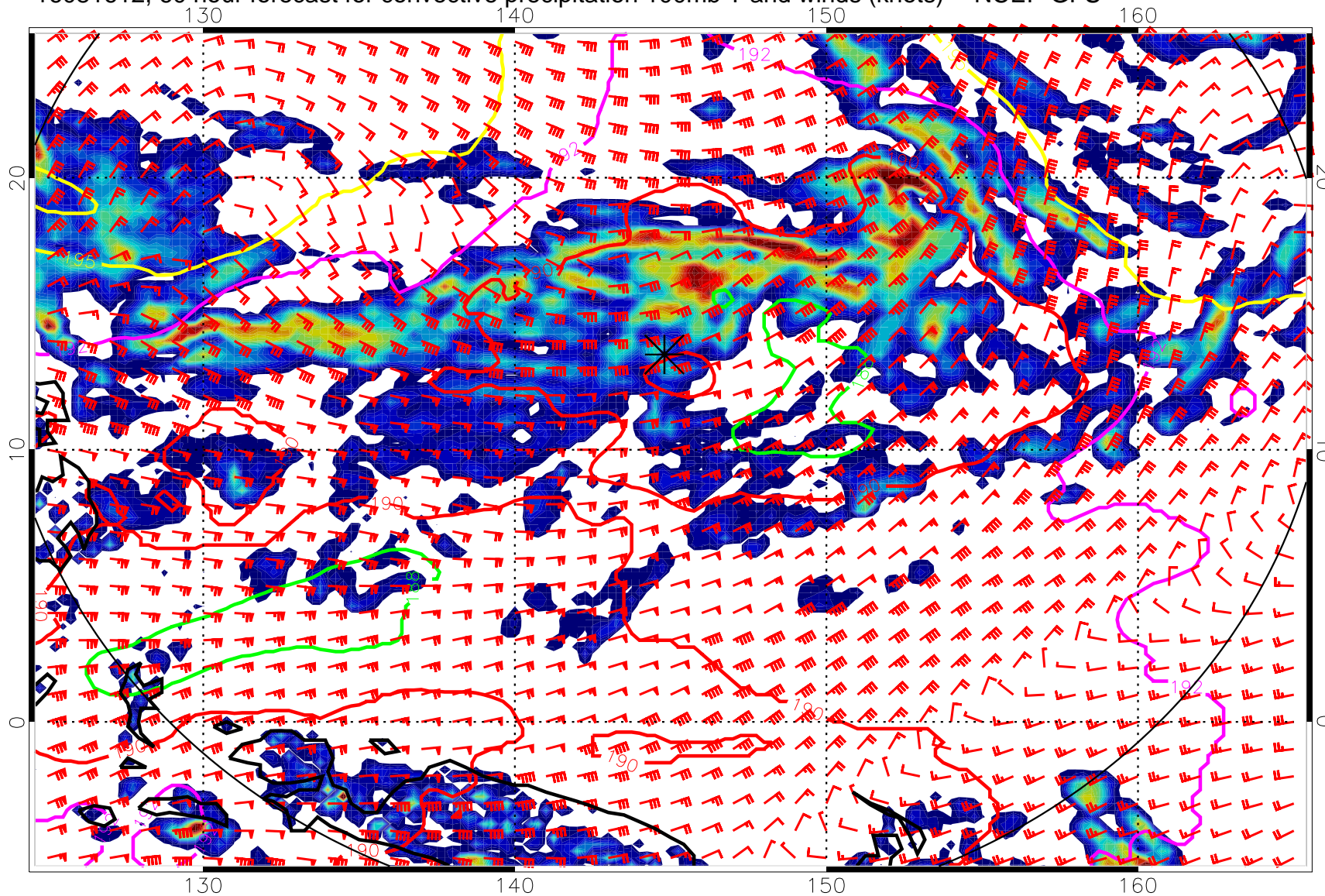
16081612, 60 hour forecast for convective precipitation 100mb T and winds (knots) -- NCEP GFS
