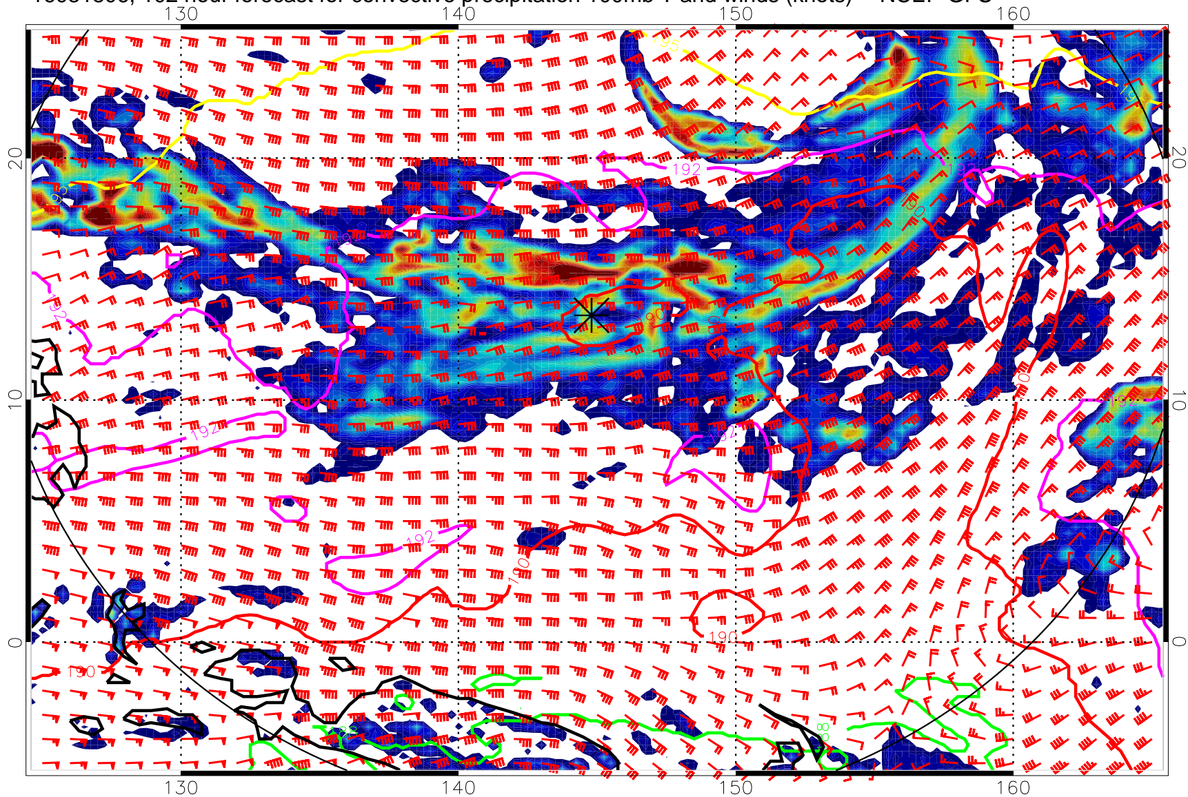
16081806, 102 hour forecast for convective precipitation 100mb T and winds (knots) -- NCEP GFS
