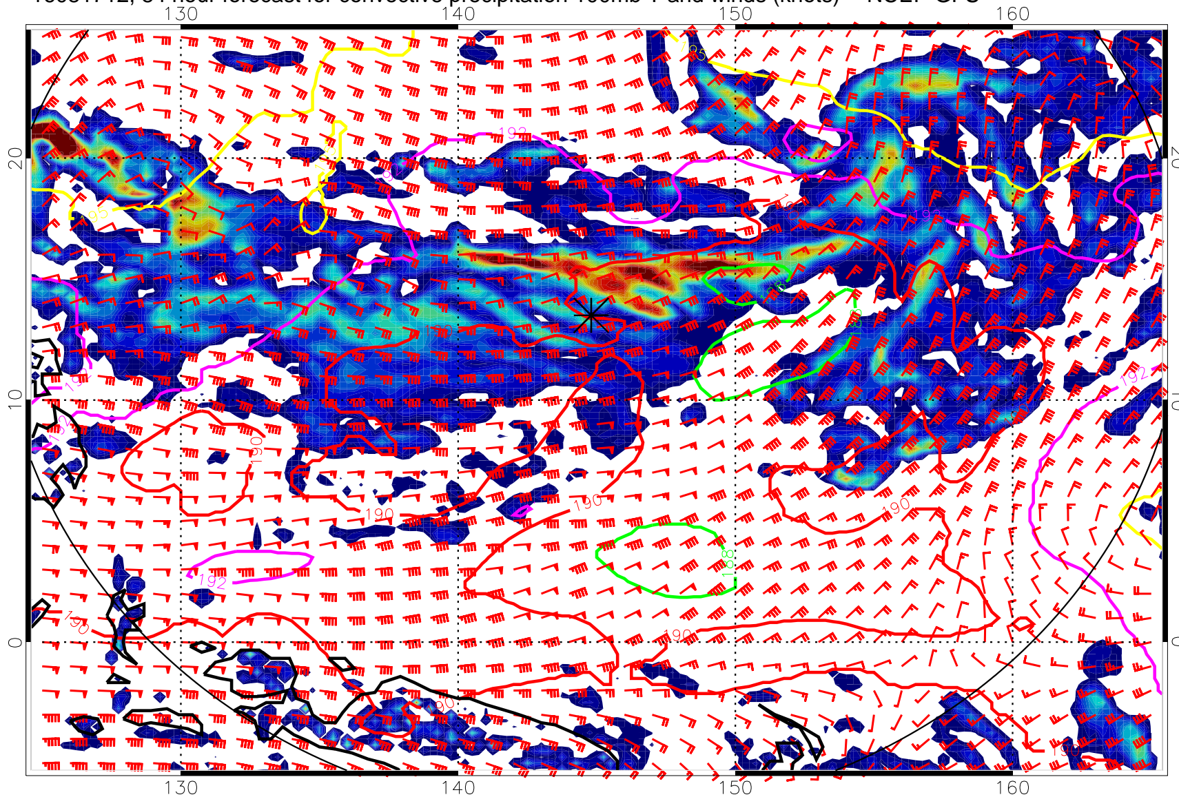
16081712, 84 hour forecast for convective precipitation 100mb T and winds (knots) -- NCEP GFS
