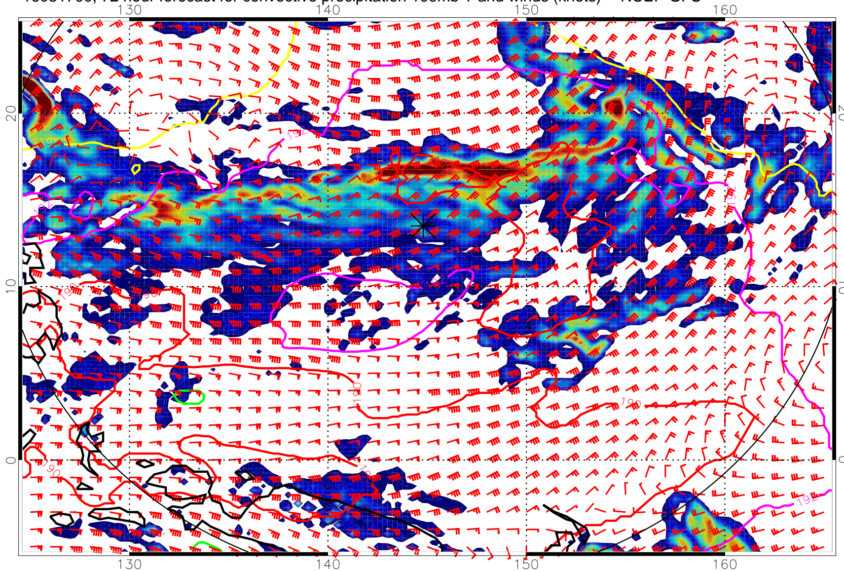
16081700, 72 hour forecast for convective precipitation 100mb T and winds (knots) -- NCEP GFS
