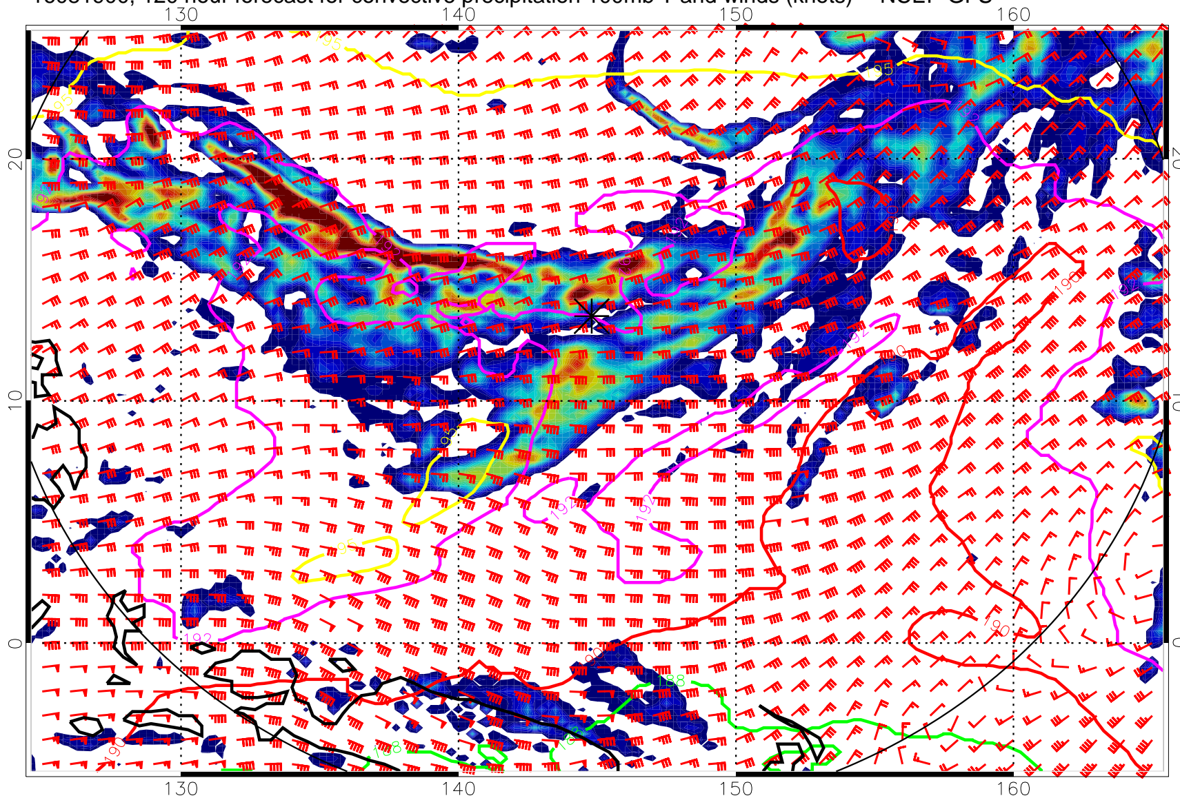
16081900, 120 hour forecast for convective precipitation 100mb T and winds (knots) -- NCEP GFS
