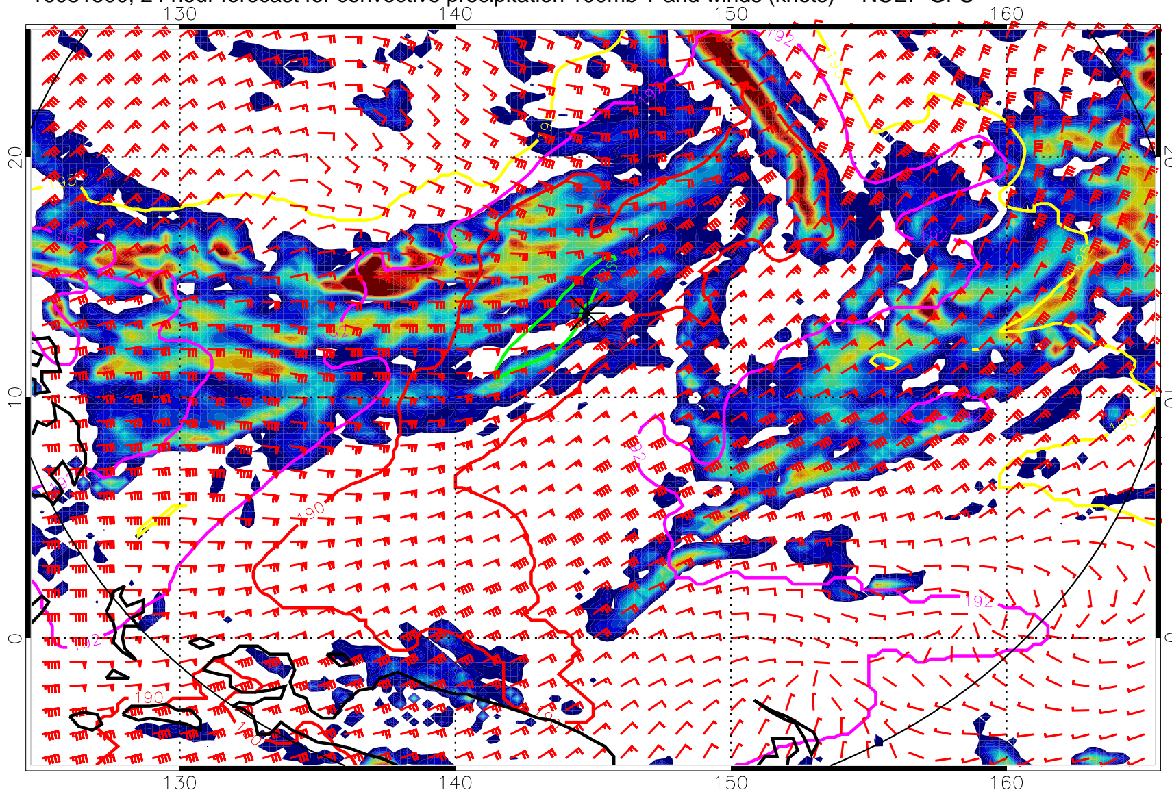
16081500, 24 hour forecast for convective precipitation 100mb T and winds (knots) -- NCEP GFS
