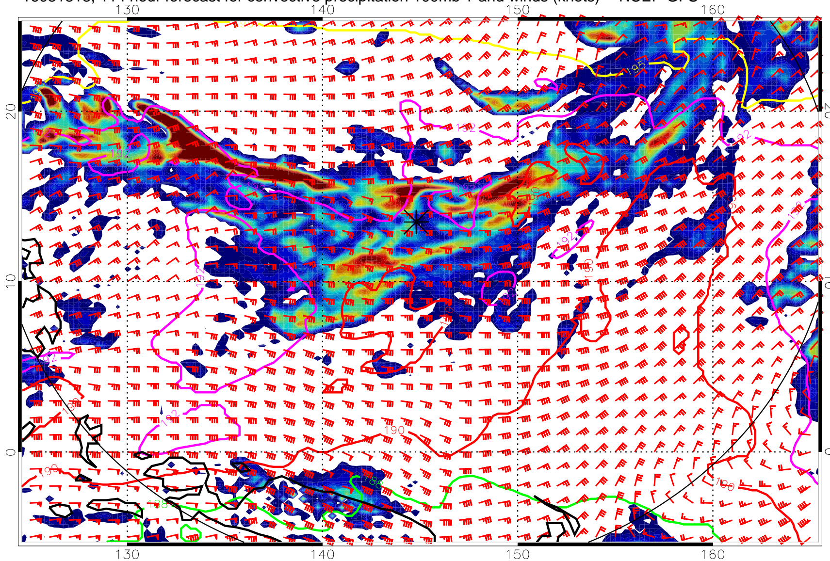
16081818, 114 hour forecast for convective precipitation 100mb T and winds (knots) -- NCEP GFS
