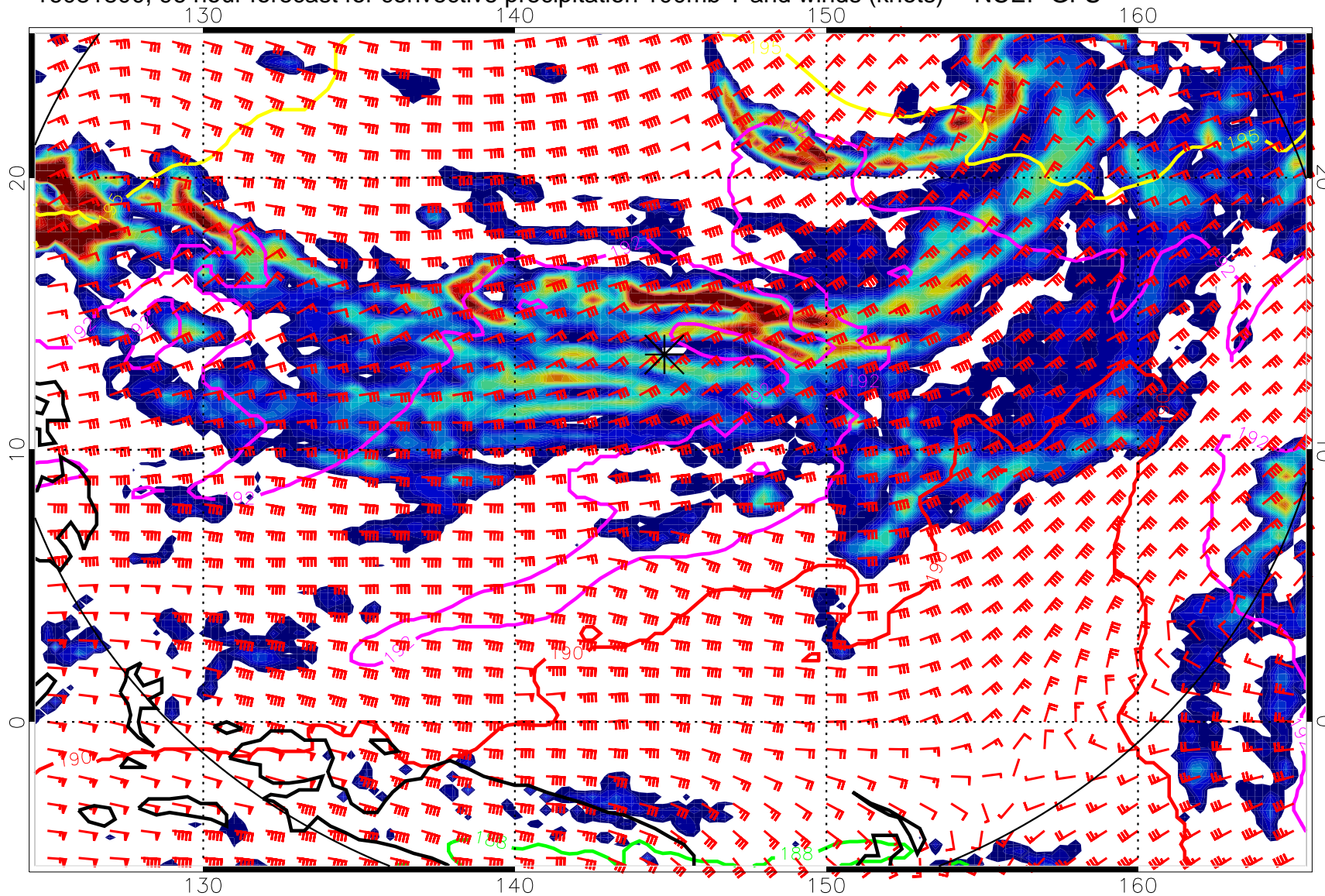
16081800, 96 hour forecast for convective precipitation 100mb T and winds (knots) -- NCEP GFS
