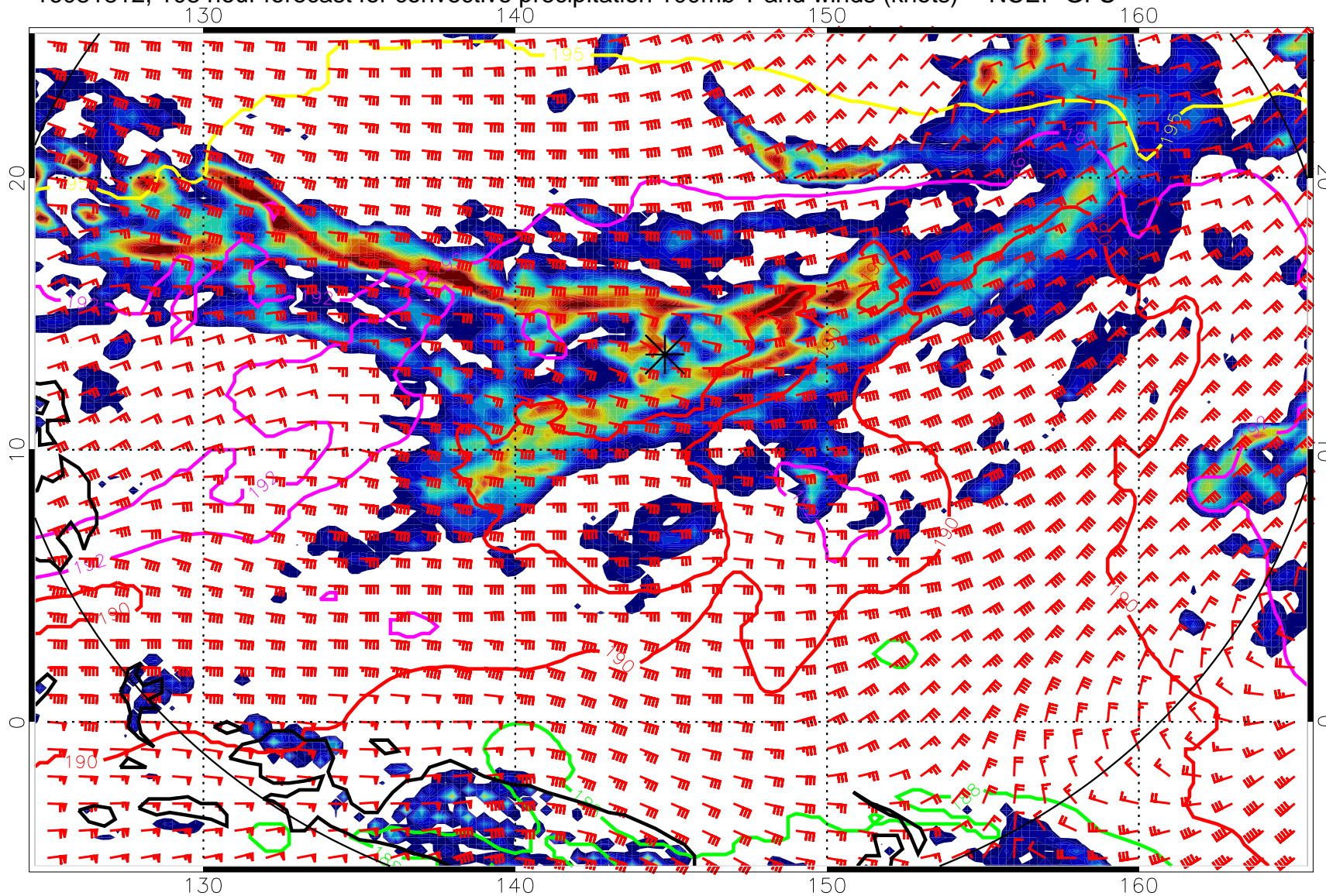
16081812, 108 hour forecast for convective precipitation 100mb T and winds (knots) -- NCEP GFS
