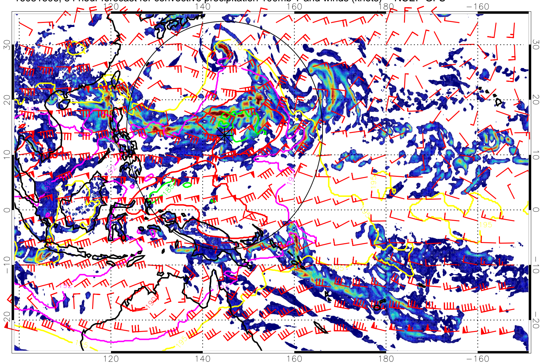
16081606, 54 hour forecast for convective precipitation 100mb T and winds (knots) -- NCEP GFS
