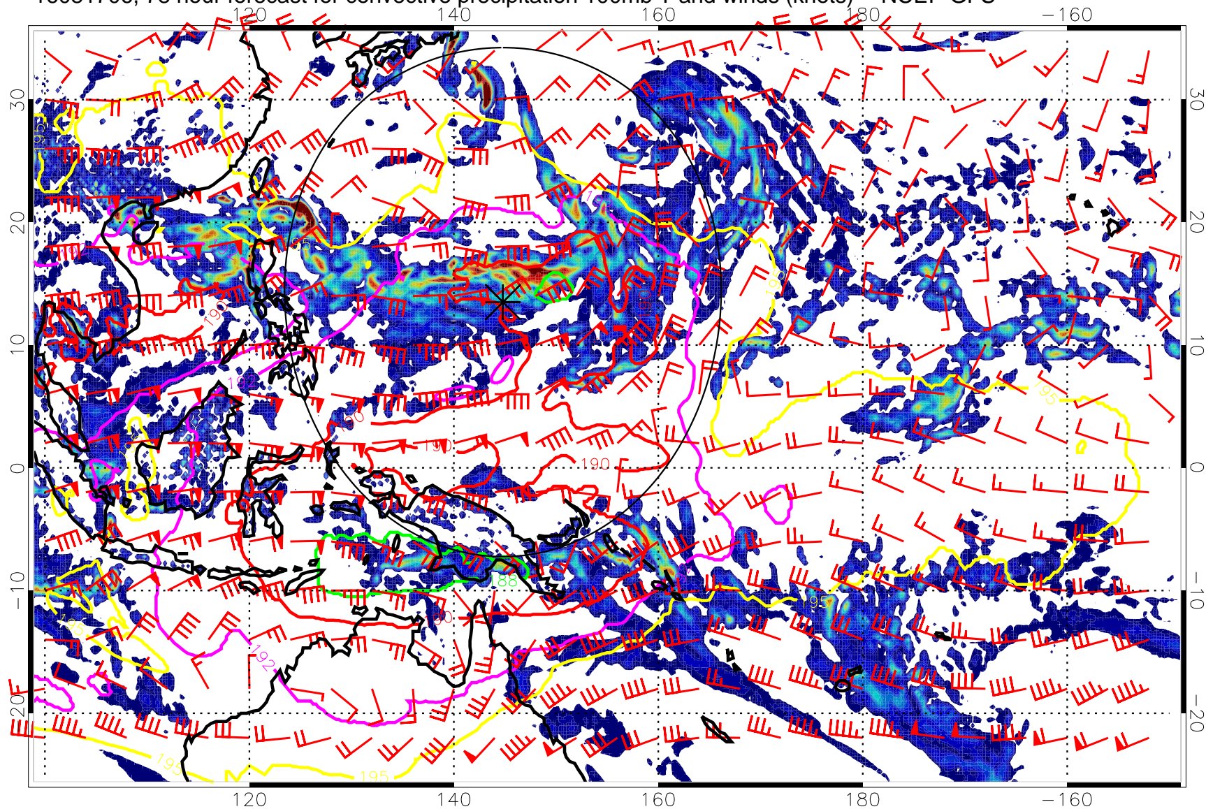
16081706, 78 hour forecast for convective precipitation 100mb T and winds (knots) -- NCEP GFS
