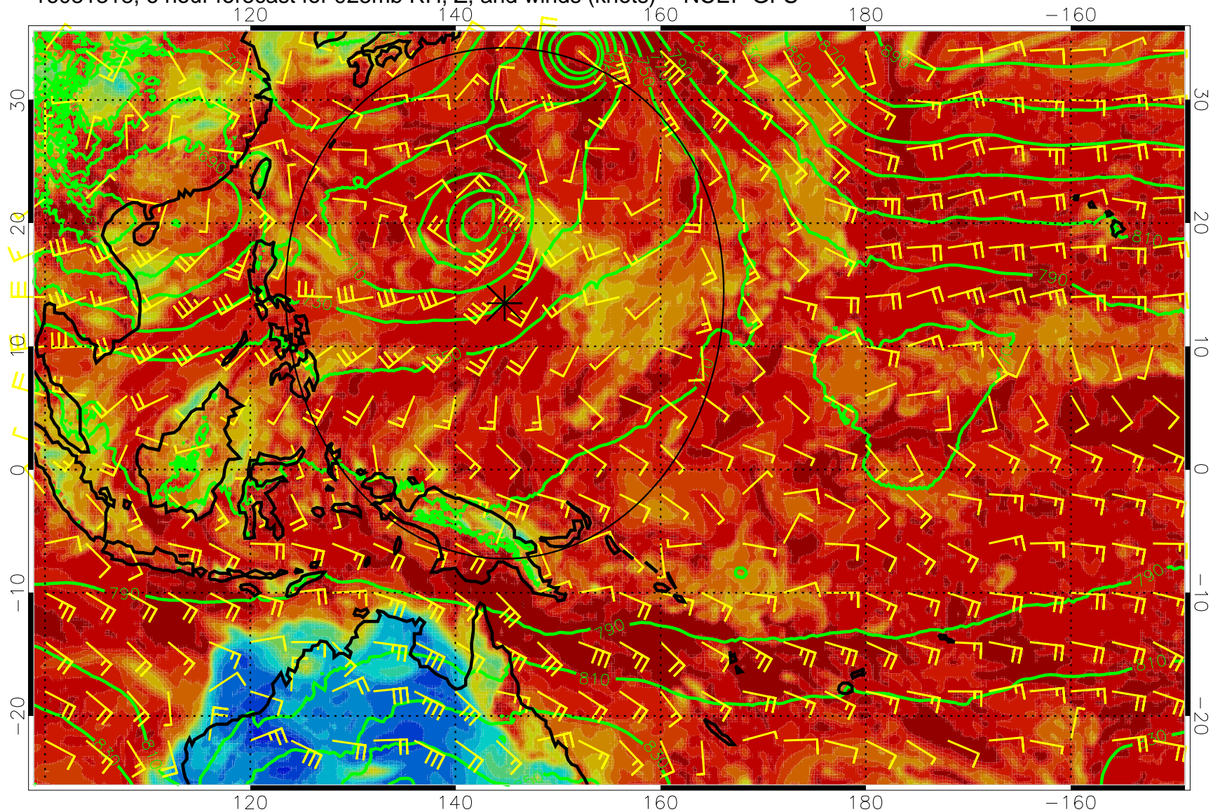
16081318, 6 hour forecast for 925mb RH, Z, and winds (knots) -- NCEP GFS
