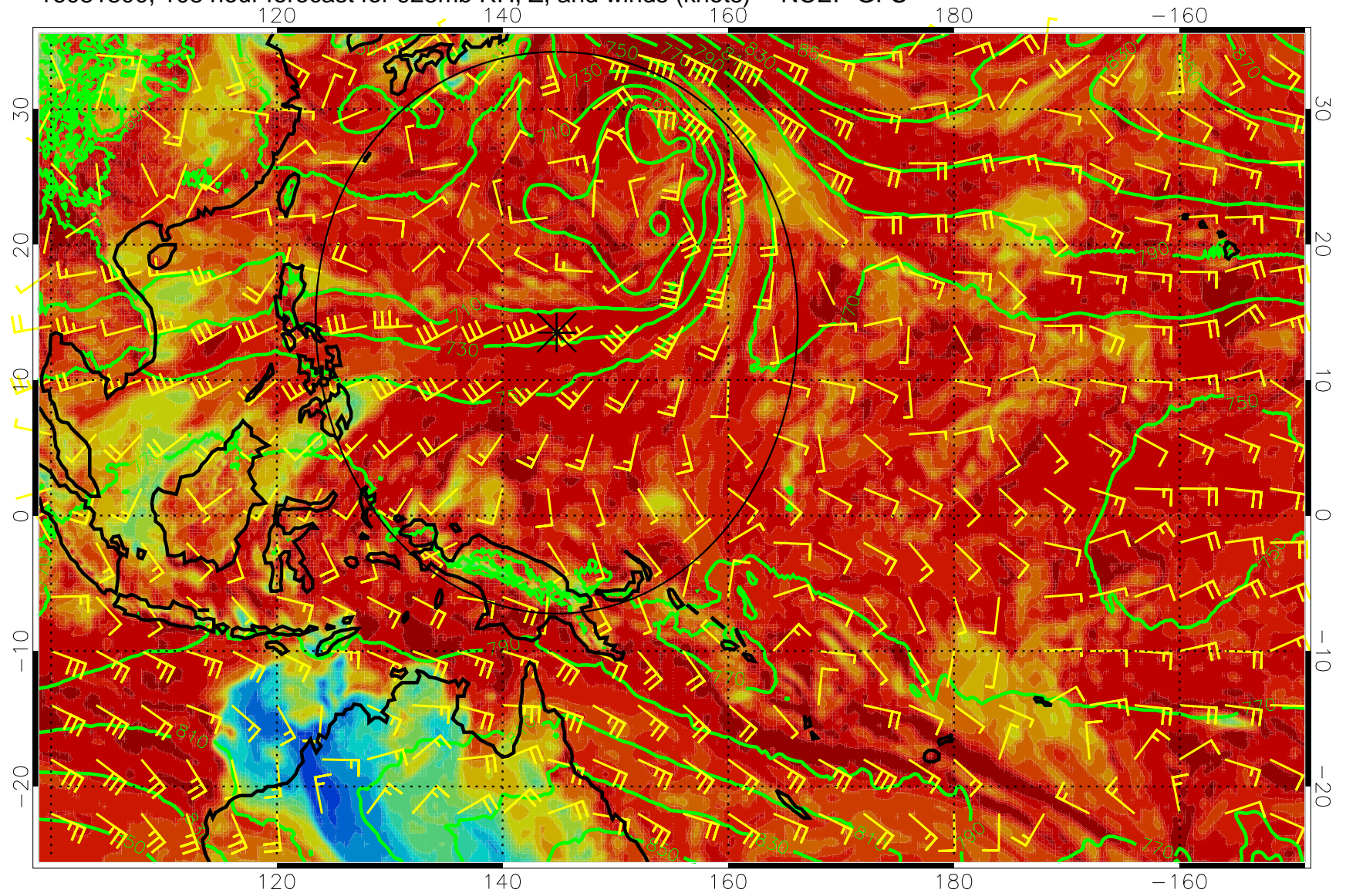
16081800, 108 hour forecast for 925mb RH, Z, and winds (knots) -- NCEP GFS
