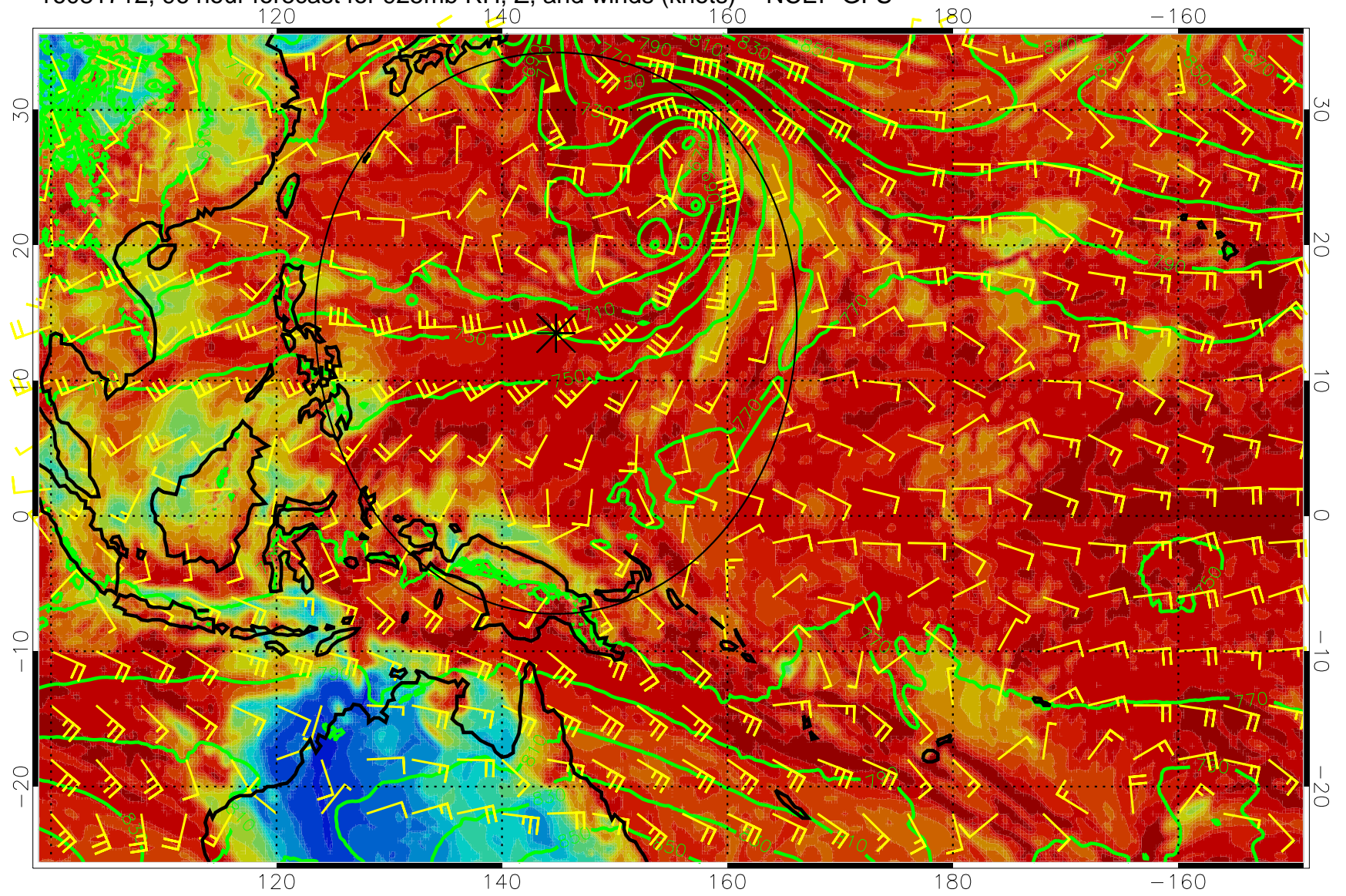
16081712, 96 hour forecast for 925mb RH, Z, and winds (knots) -- NCEP GFS
