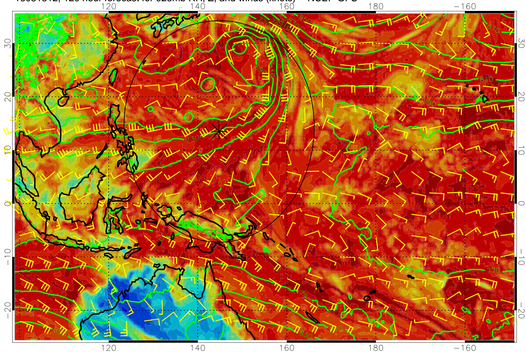
16081812, 120 hour forecast for 925mb RH, Z, and winds (knots) -- NCEP GFS
