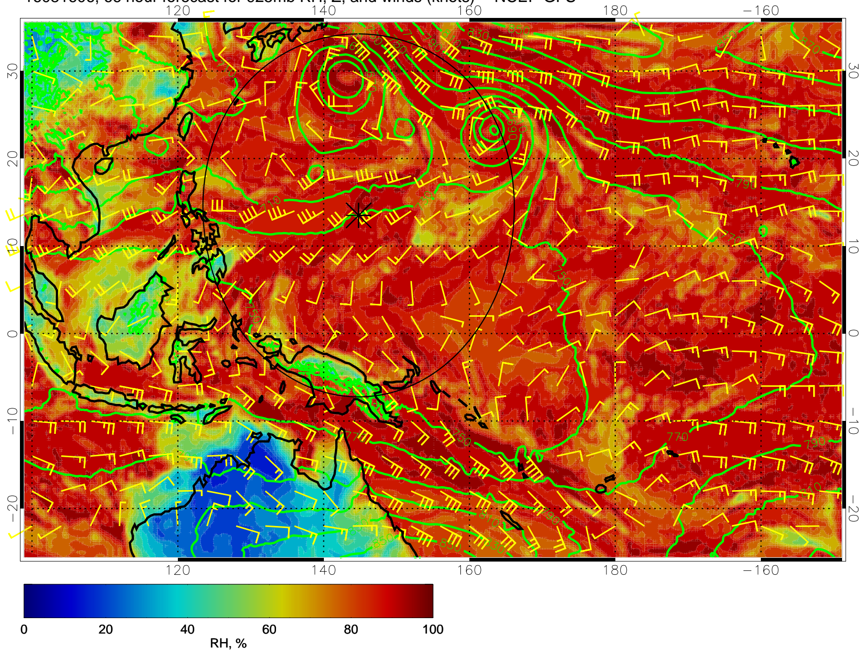
16081606, 66 hour forecast for 925mb RH, Z, and winds (knots) -- NCEP GFS
