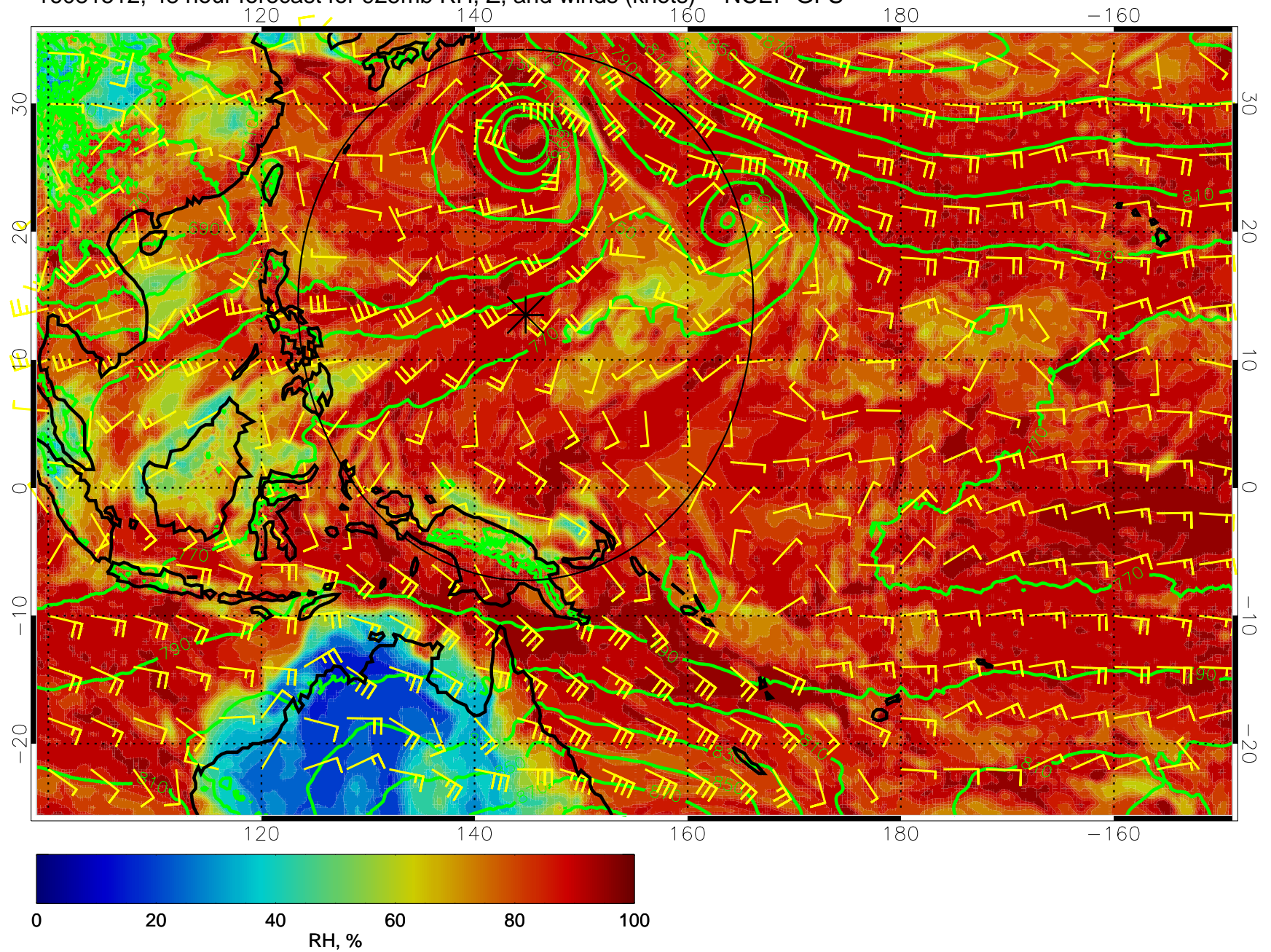
16081512, 48 hour forecast for 925mb RH, Z, and winds (knots) -- NCEP GFS
