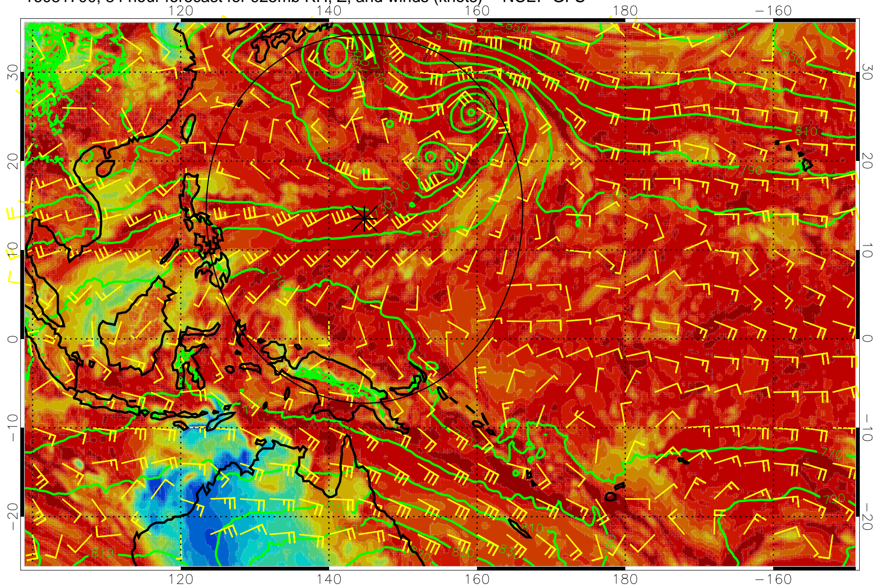
16081700, 84 hour forecast for 925mb RH, Z, and winds (knots) -- NCEP GFS
