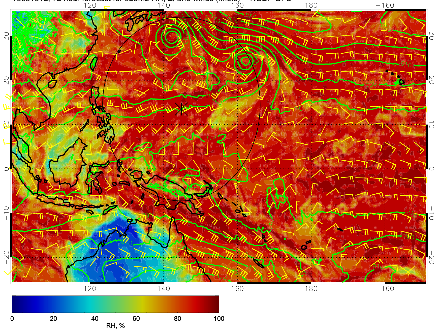
16081612, 72 hour forecast for 925mb RH, Z, and winds (knots) -- NCEP GFS
