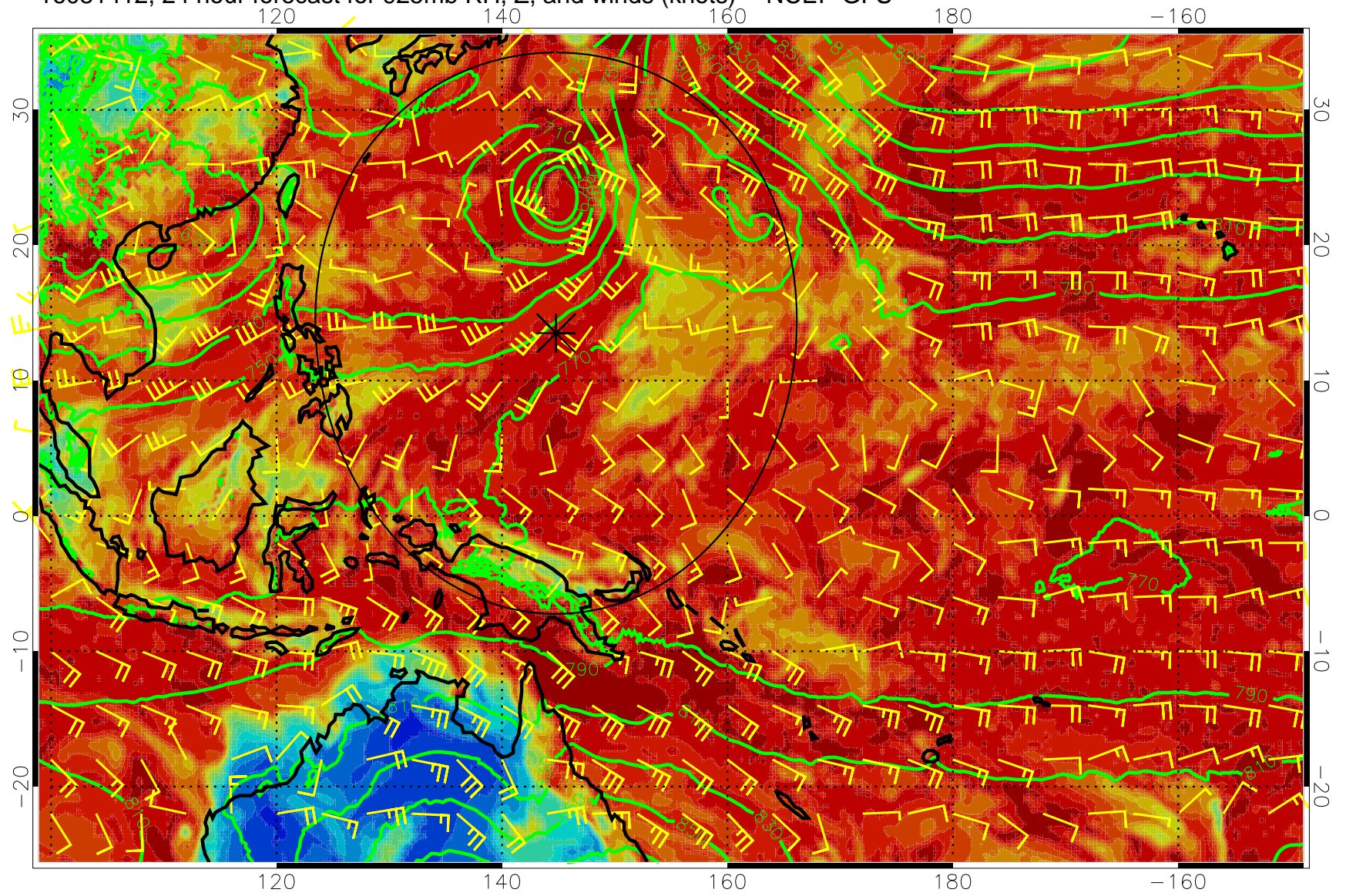
16081412, 24 hour forecast for 925mb RH, Z, and winds (knots) -- NCEP GFS
