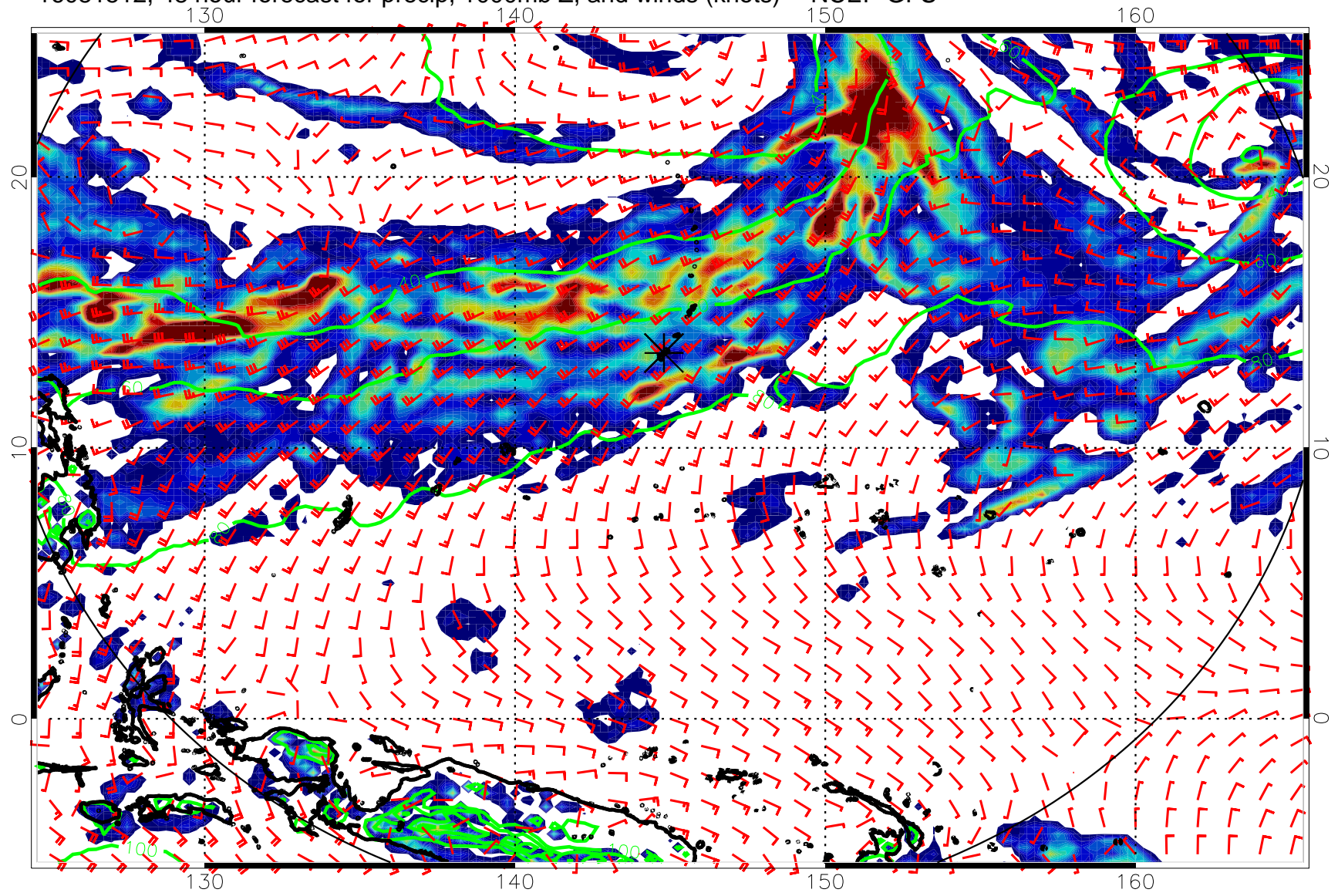
16081512, 48 hour forecast for precip, 1000mb Z, and winds (knots) -- NCEP GFS
