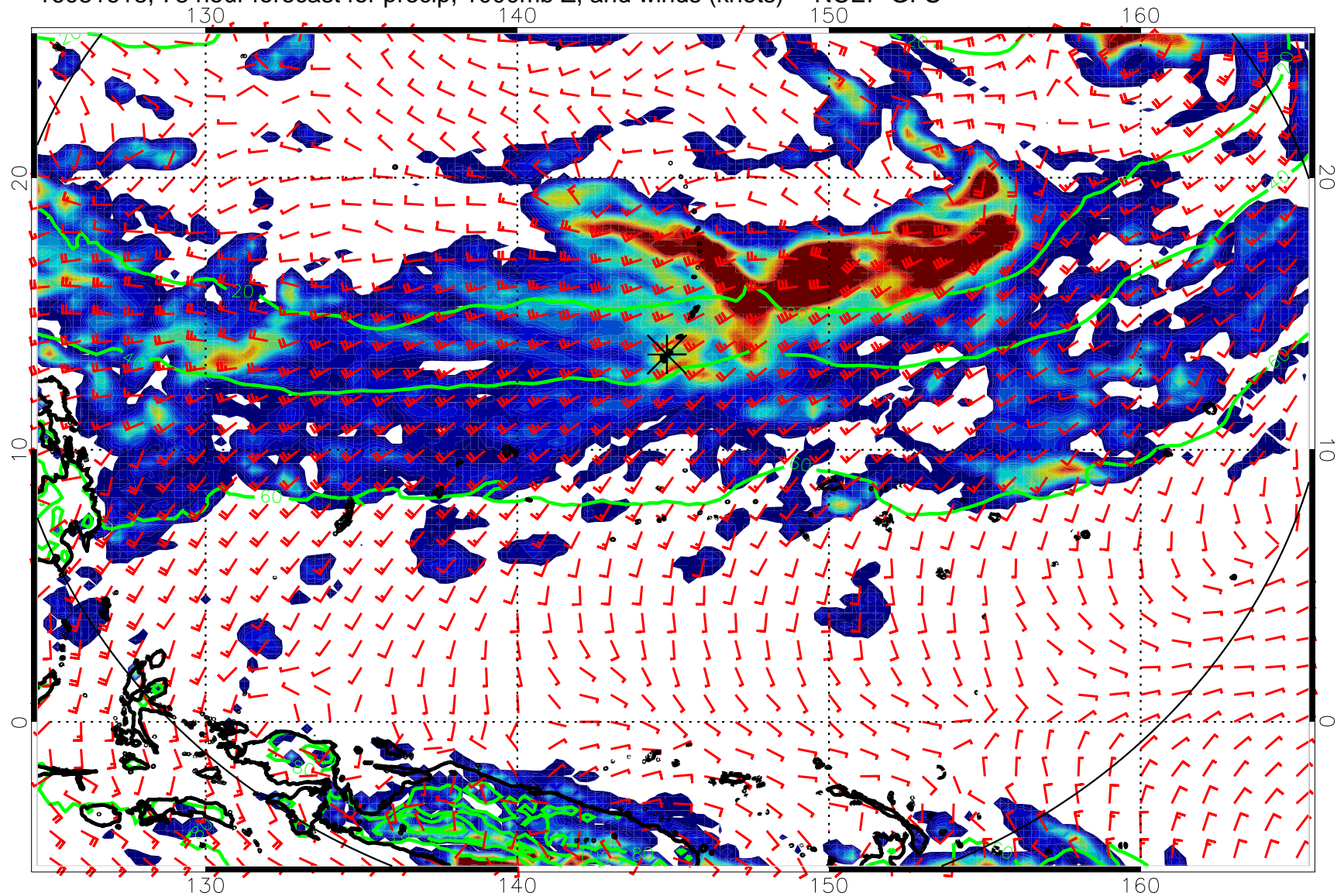
16081618, 78 hour forecast for precip, 1000mb Z, and winds (knots) -- NCEP GFS
