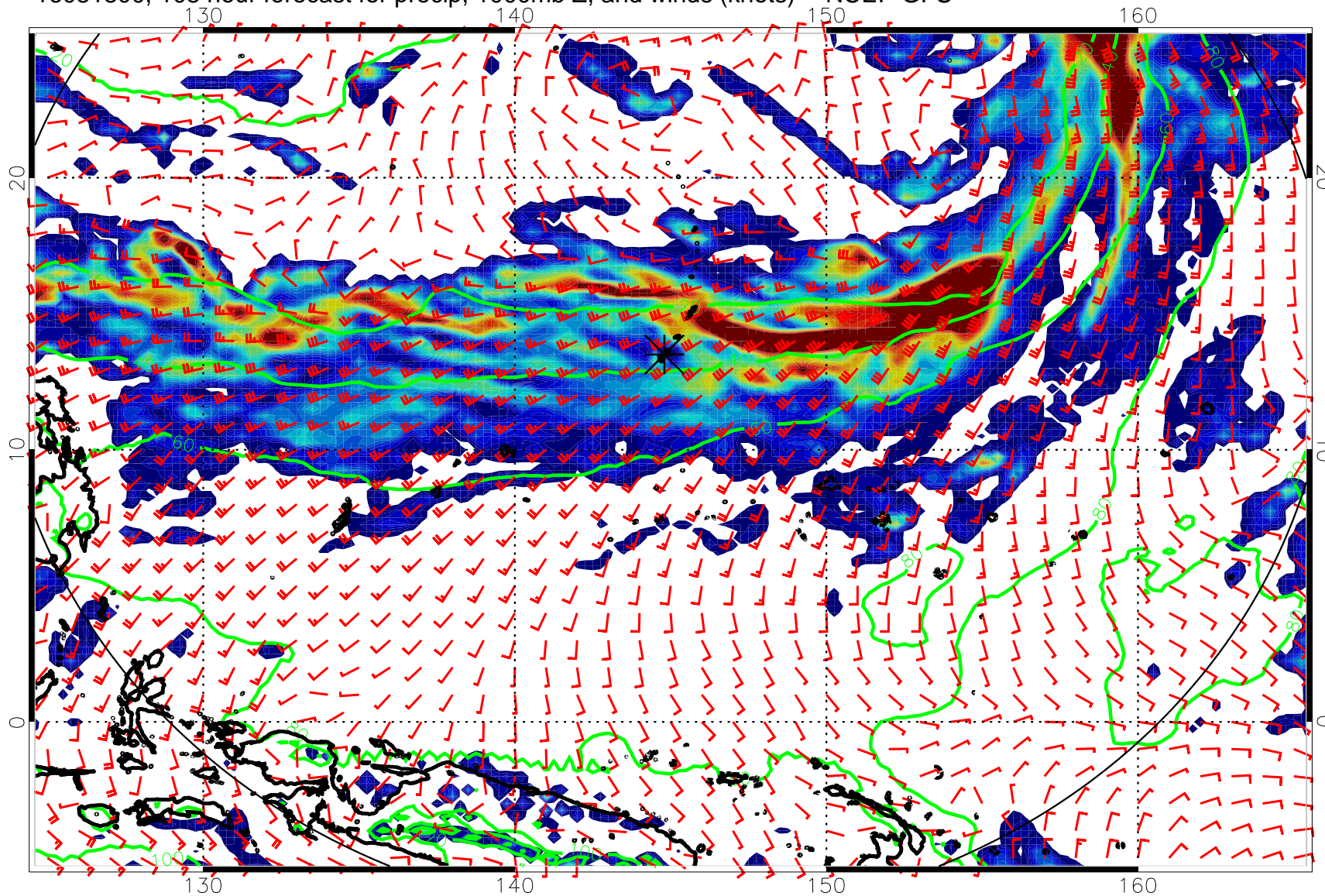
16081800, 108 hour forecast for precip, 1000mb Z, and winds (knots) -- NCEP GFS
