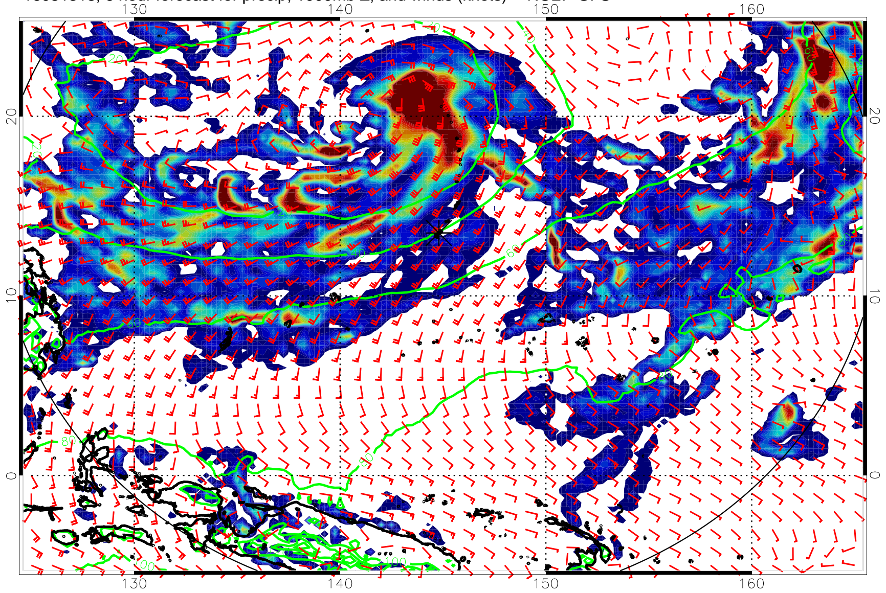
16081318, 6 hour forecast for precip, 1000mb Z, and winds (knots) -- NCEP GFS
