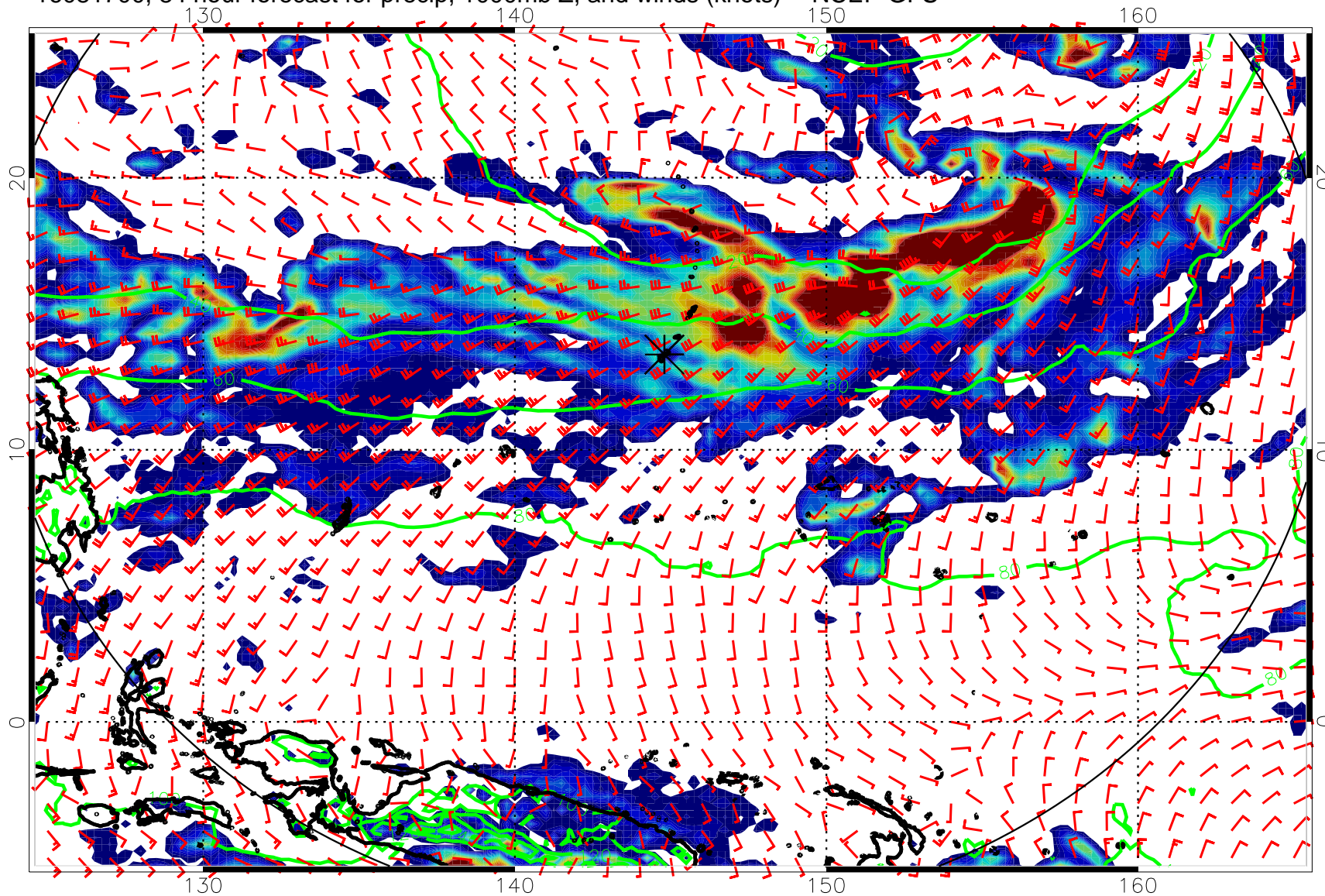
16081700, 84 hour forecast for precip, 1000mb Z, and winds (knots) -- NCEP GFS
