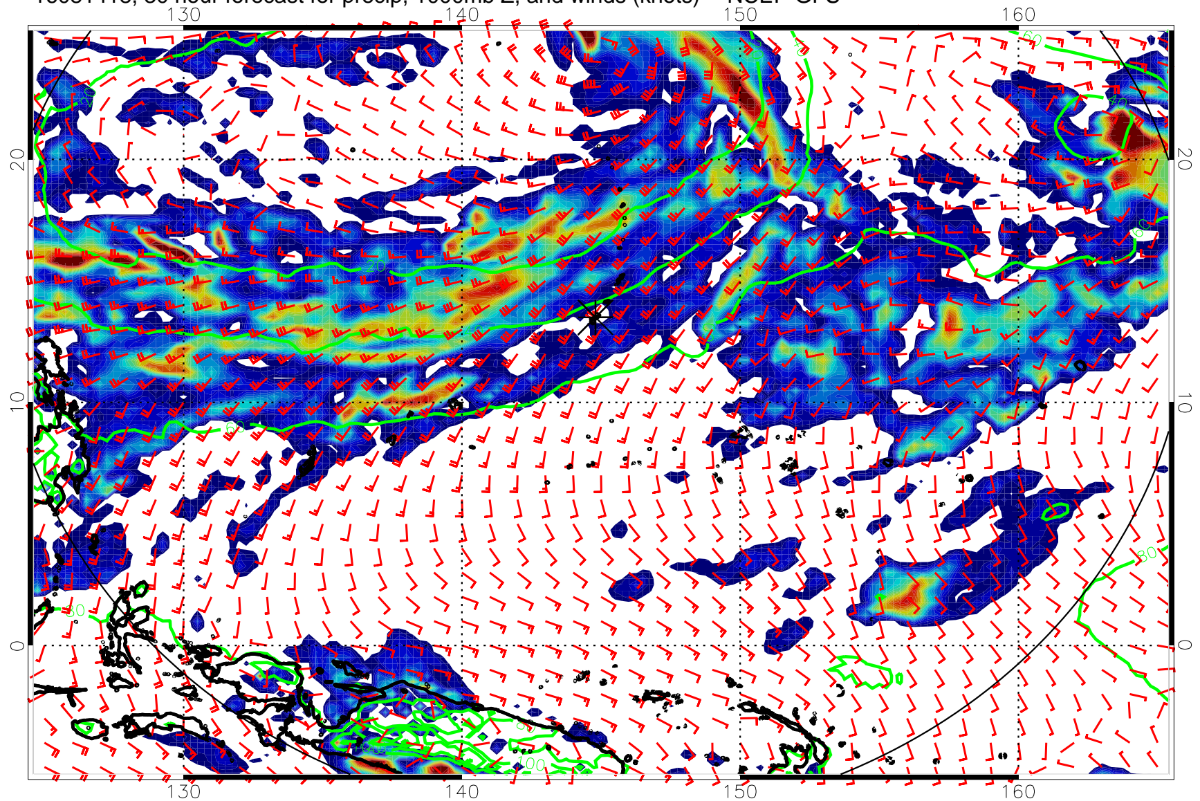
16081418, 30 hour forecast for precip, 1000mb Z, and winds (knots) -- NCEP GFS
