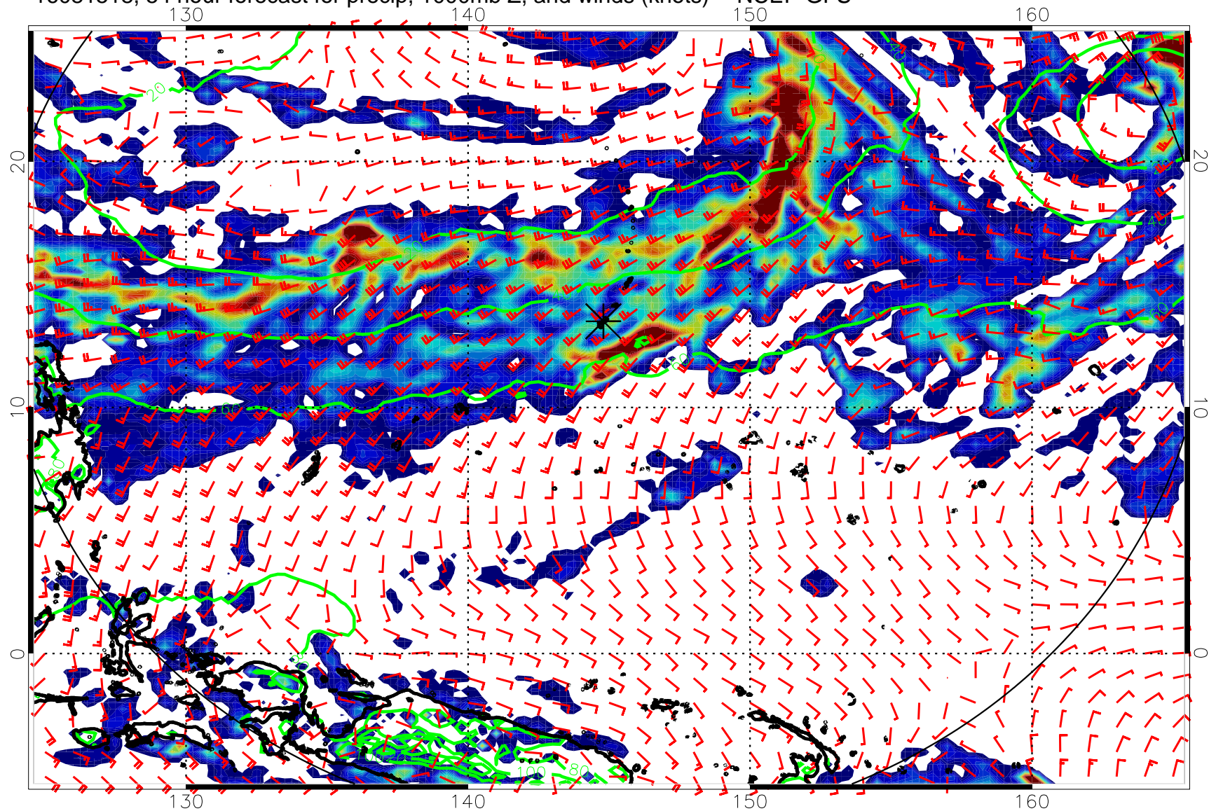
16081518, 54 hour forecast for precip, 1000mb Z, and winds (knots) -- NCEP GFS
