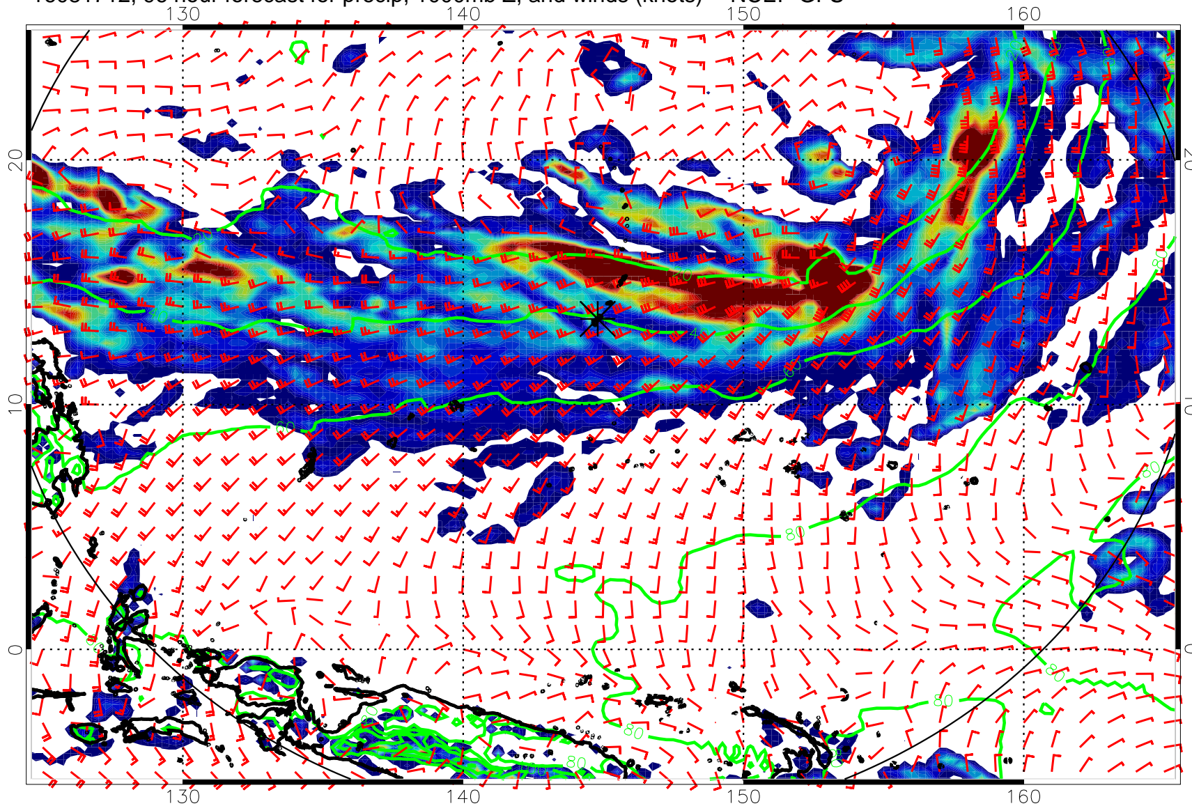
16081712, 96 hour forecast for precip, 1000mb Z, and winds (knots) -- NCEP GFS
