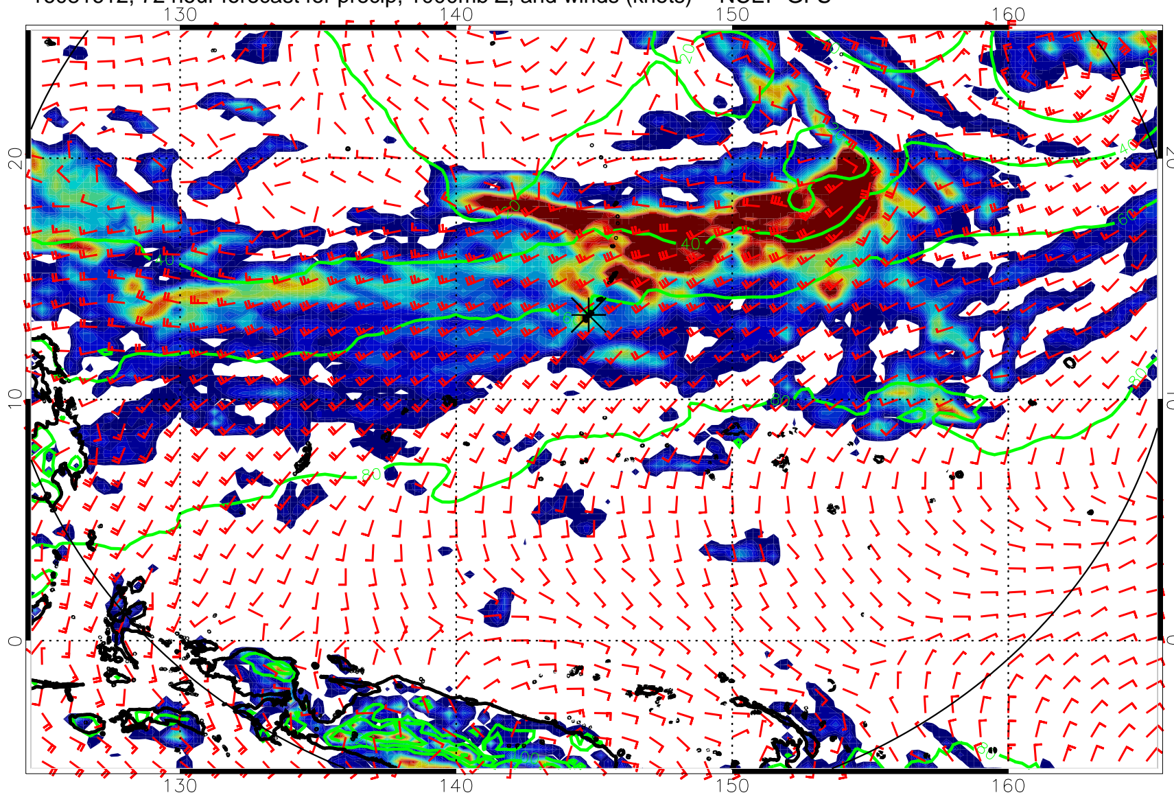
16081612, 72 hour forecast for precip, 1000mb Z, and winds (knots) -- NCEP GFS
