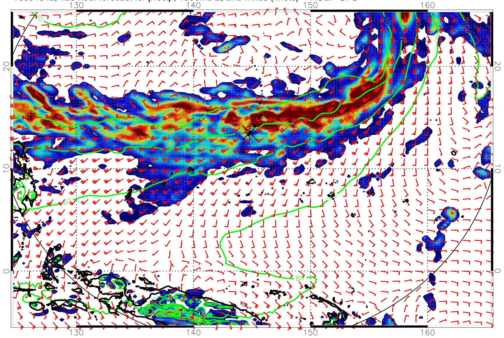
16081812, 120 hour forecast for precip, 1000mb Z, and winds (knots) -- NCEP GFS
