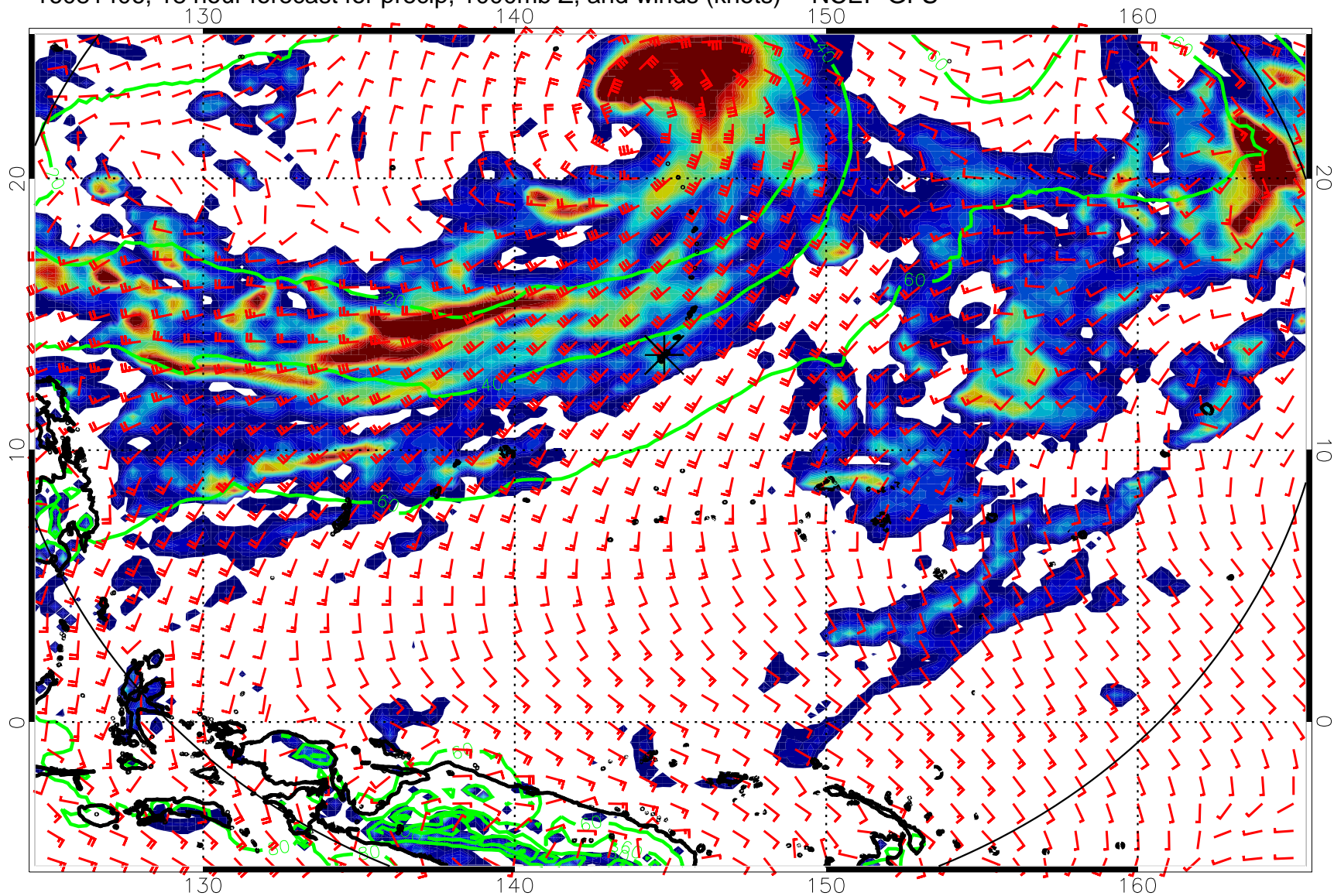
16081406, 18 hour forecast for precip, 1000mb Z, and winds (knots) -- NCEP GFS
