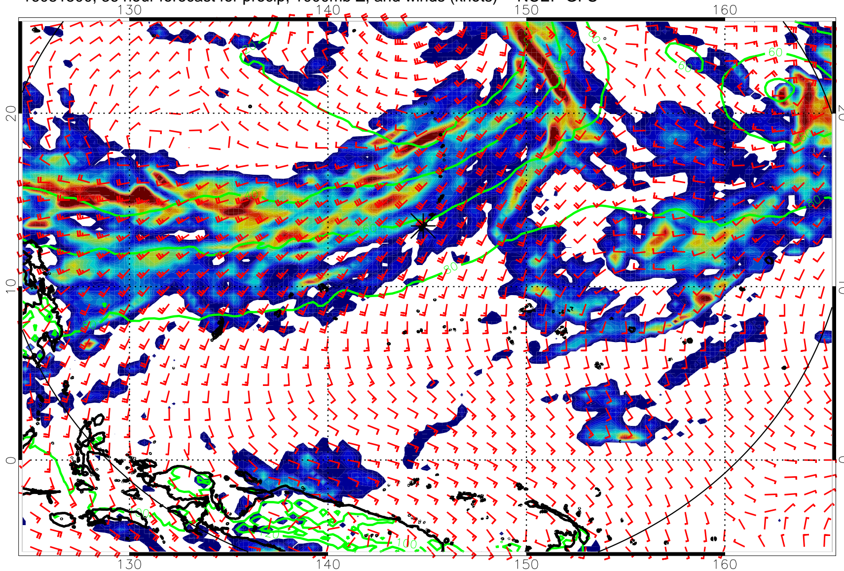
16081500, 36 hour forecast for precip, 1000mb Z, and winds (knots) -- NCEP GFS
