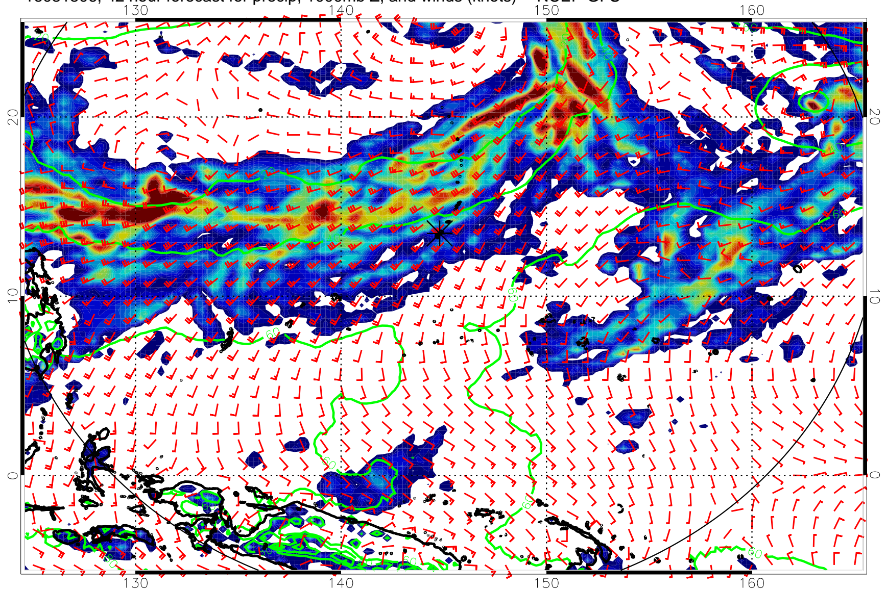
16081506, 42 hour forecast for precip, 1000mb Z, and winds (knots) -- NCEP GFS
