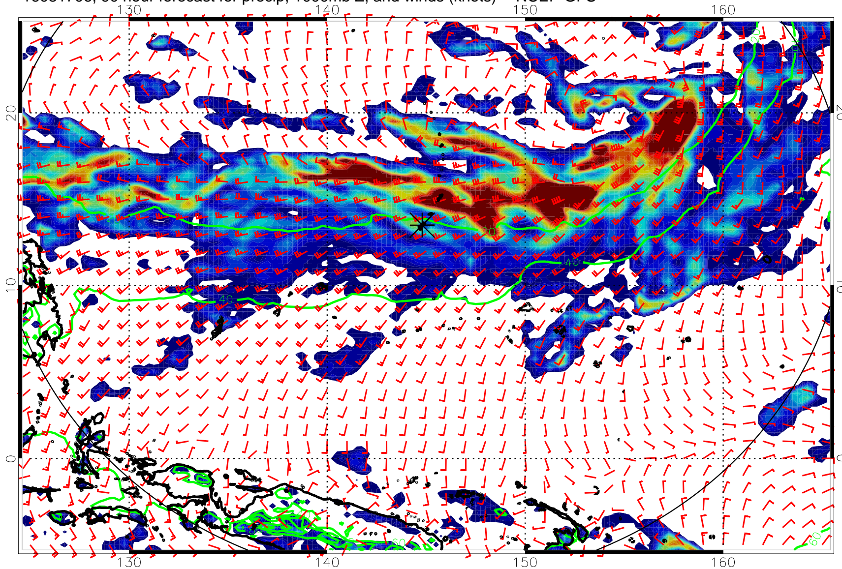
16081706, 90 hour forecast for precip, 1000mb Z, and winds (knots) -- NCEP GFS
