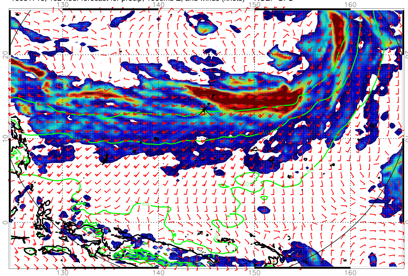
16081718, 102 hour forecast for precip, 1000mb Z, and winds (knots) -- NCEP GFS
