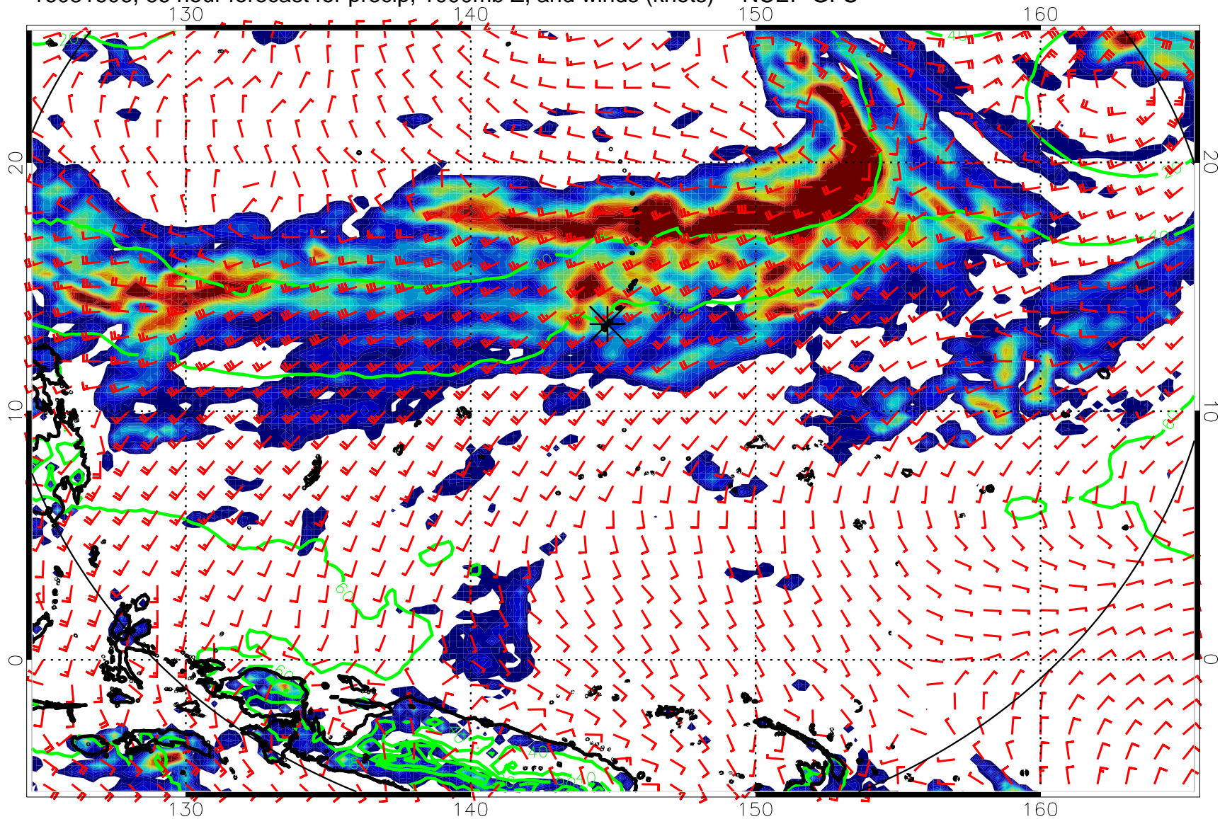
16081606, 66 hour forecast for precip, 1000mb Z, and winds (knots) -- NCEP GFS
