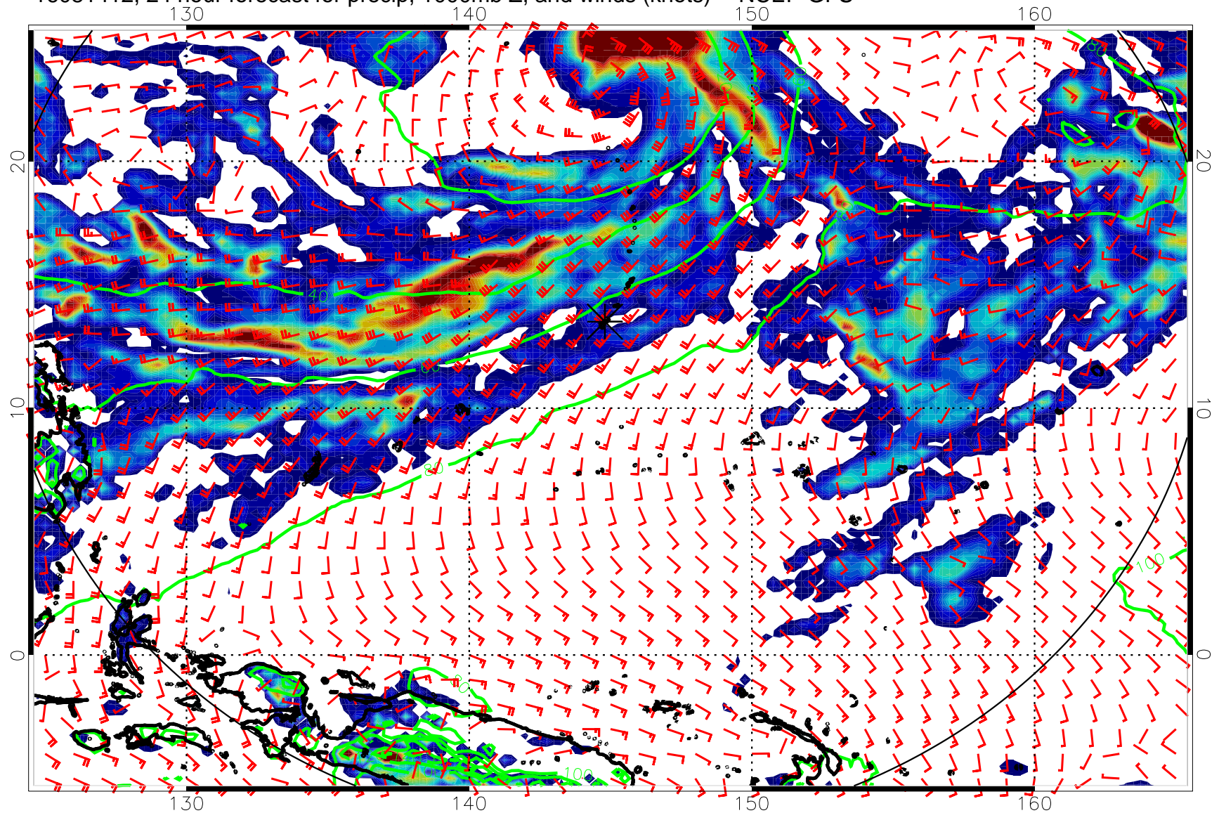
16081412, 24 hour forecast for precip, 1000mb Z, and winds (knots) -- NCEP GFS
