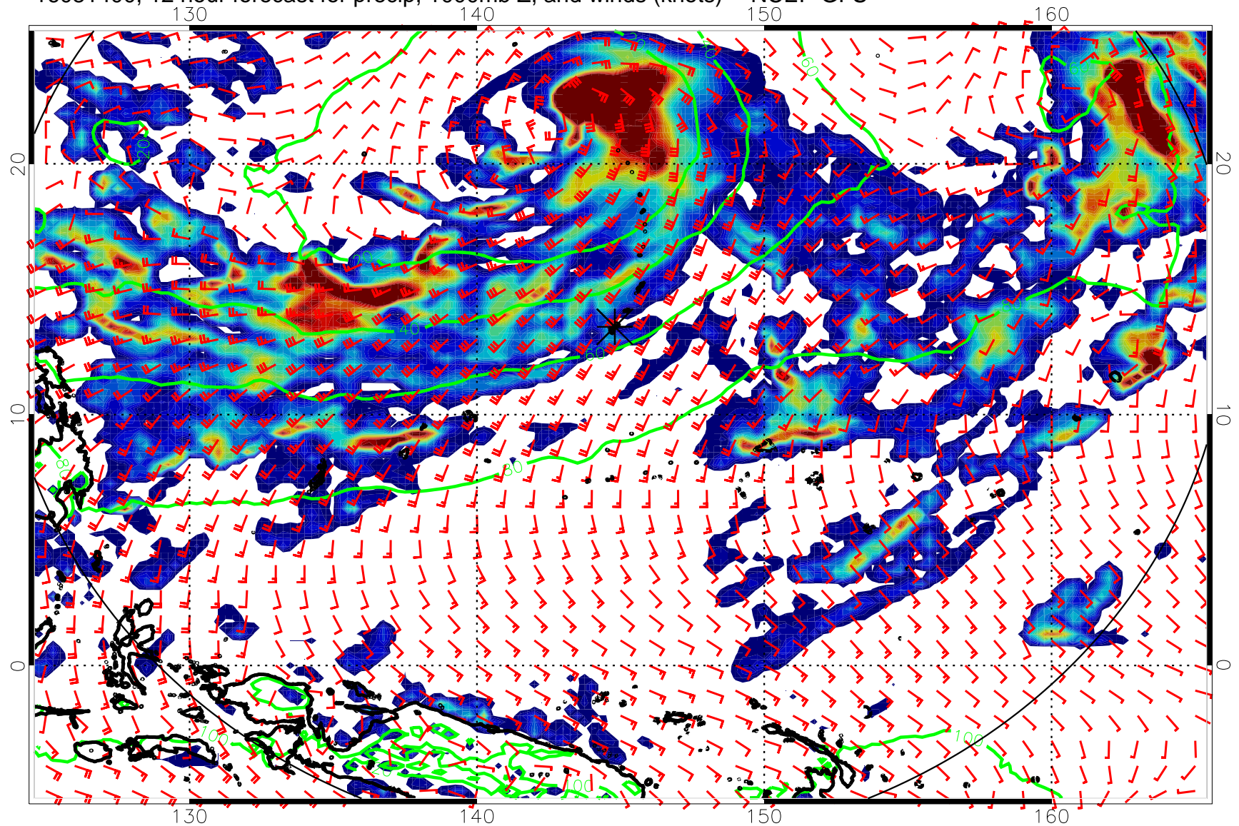
16081400, 12 hour forecast for precip, 1000mb Z, and winds (knots) -- NCEP GFS
