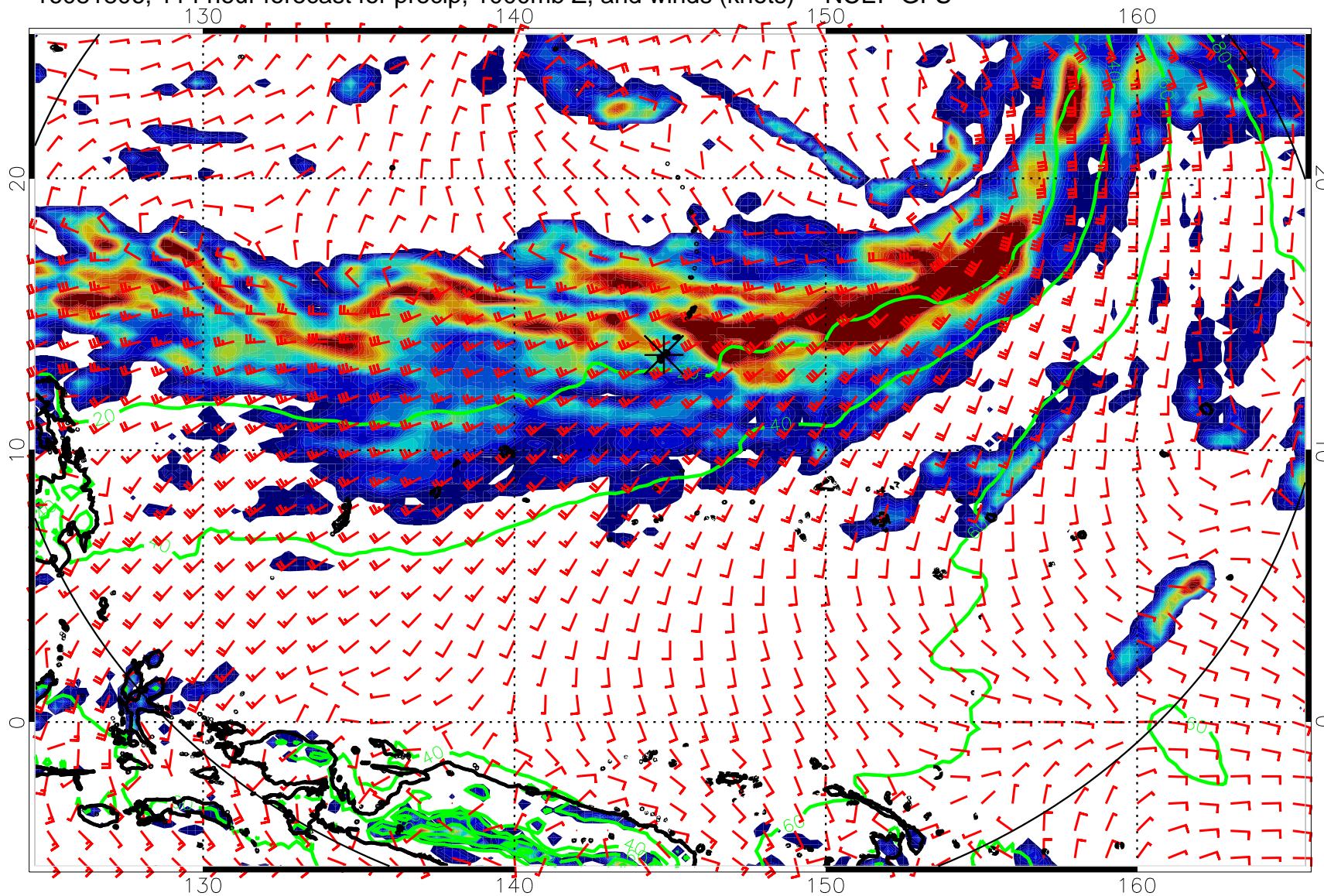
16081806, 114 hour forecast for precip, 1000mb Z, and winds (knots) -- NCEP GFS
