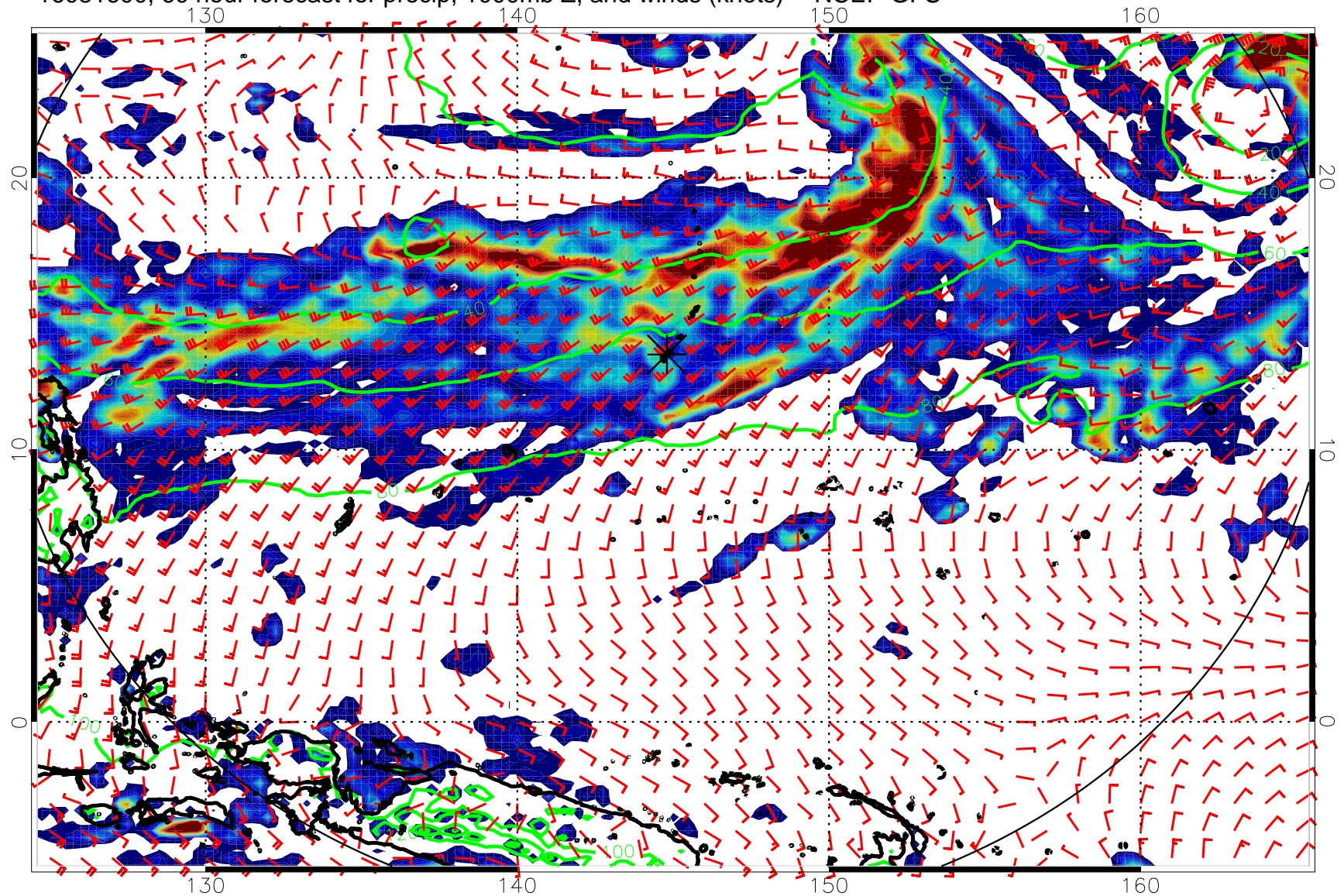
16081600, 60 hour forecast for precip, 1000mb Z, and winds (knots) -- NCEP GFS
