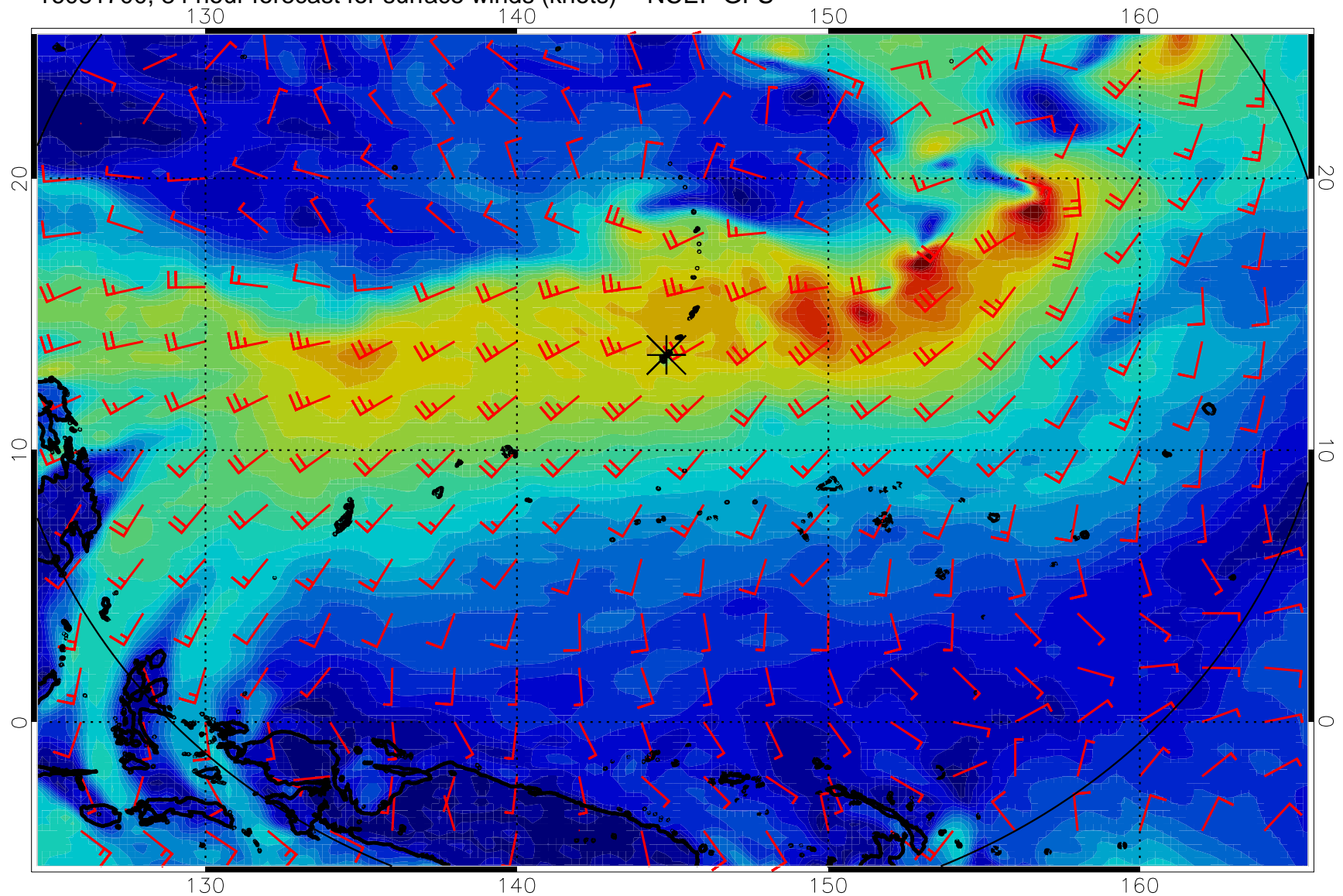
16081700, 84 hour forecast for surface winds (knots) -- NCEP GFS
