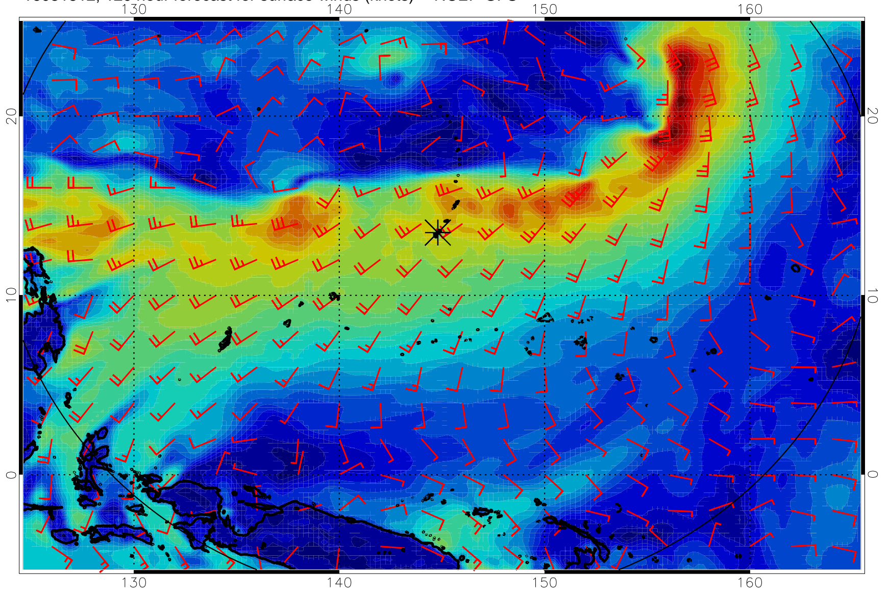
16081812, 120 hour forecast for surface winds (knots) -- NCEP GFS
