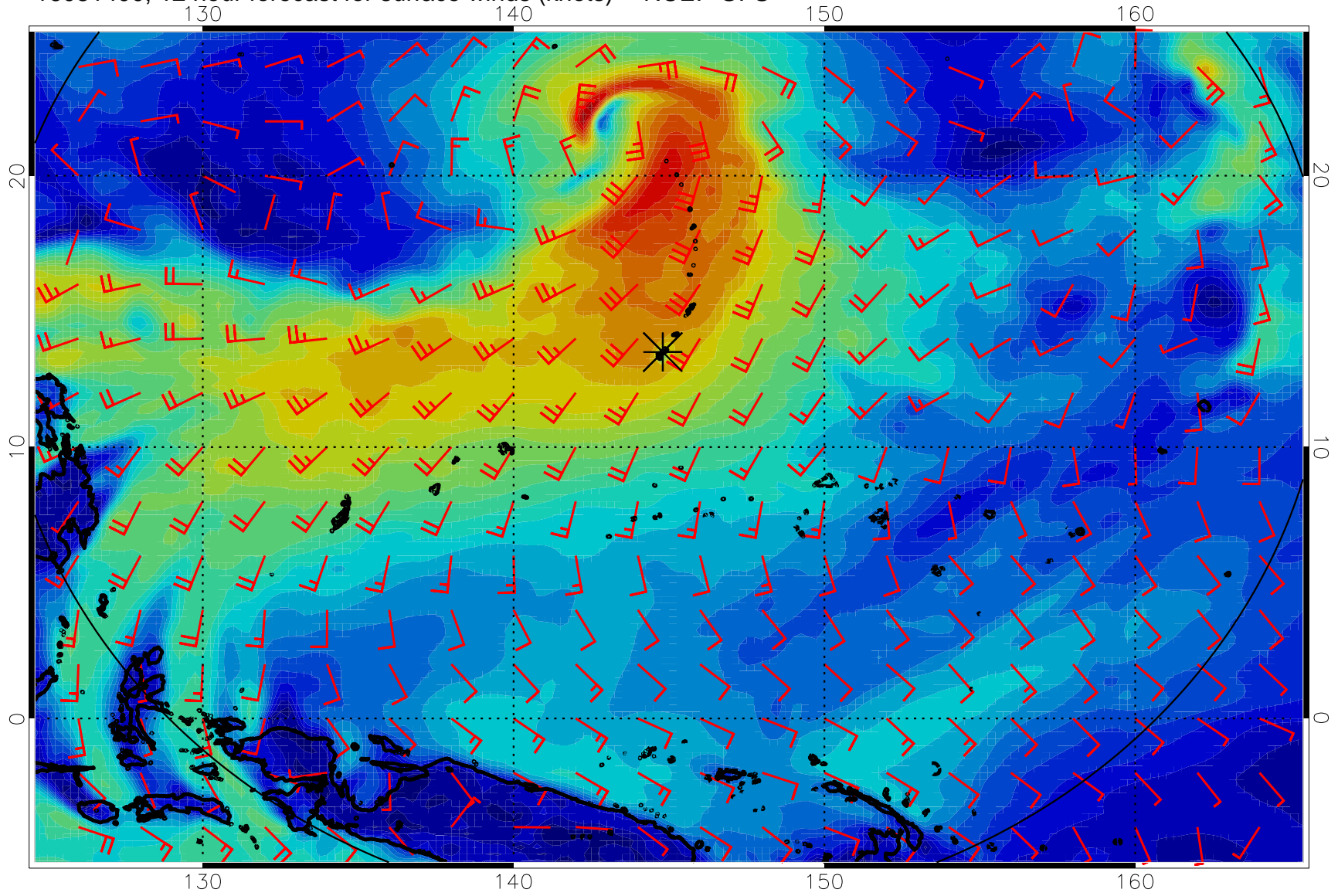
16081400, 12 hour forecast for surface winds (knots) -- NCEP GFS
