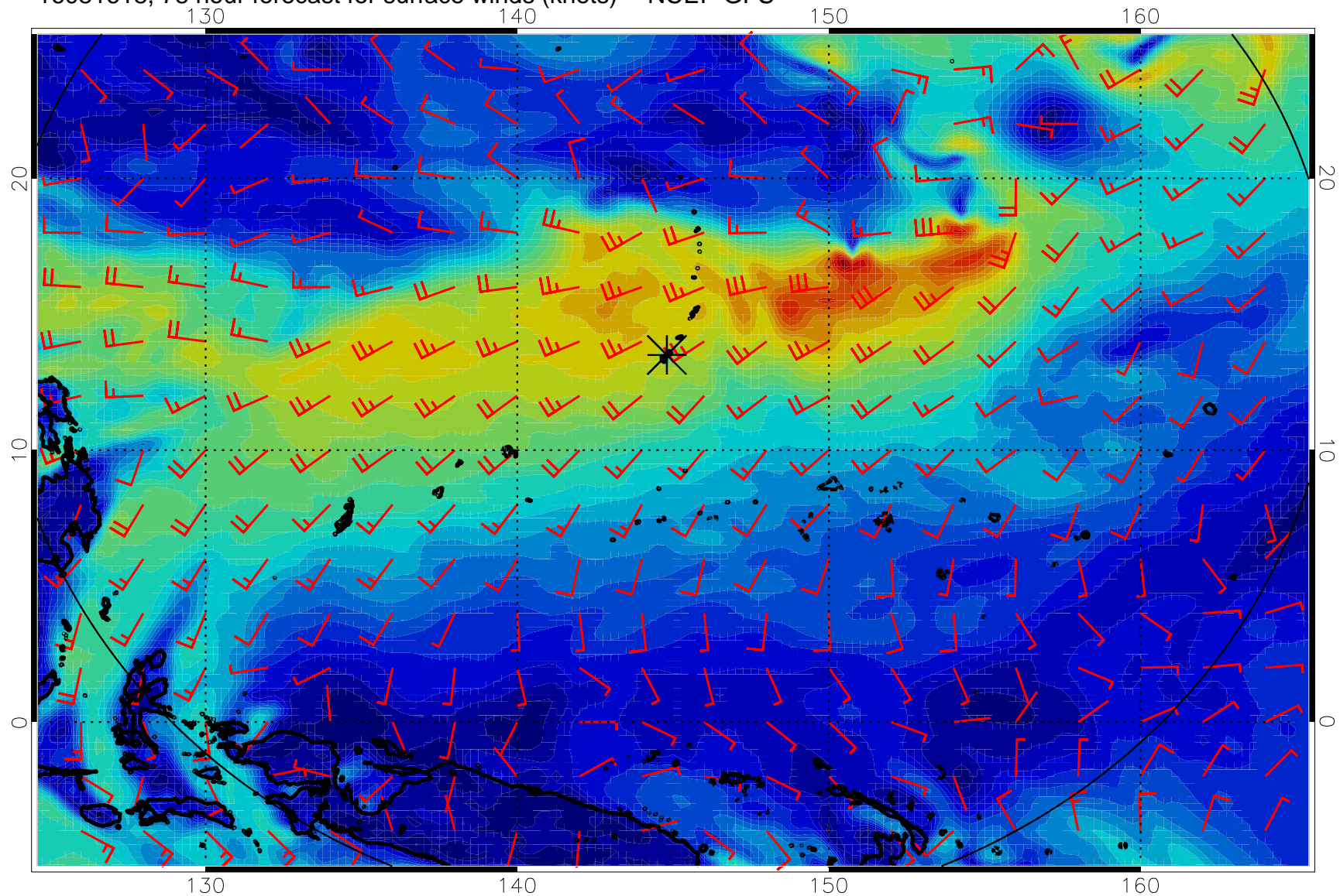
16081618, 78 hour forecast for surface winds (knots) -- NCEP GFS
