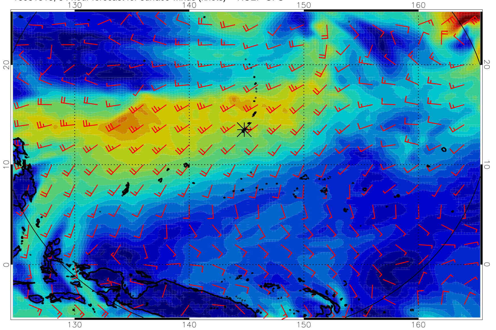
16081518, 54 hour forecast for surface winds (knots) -- NCEP GFS
