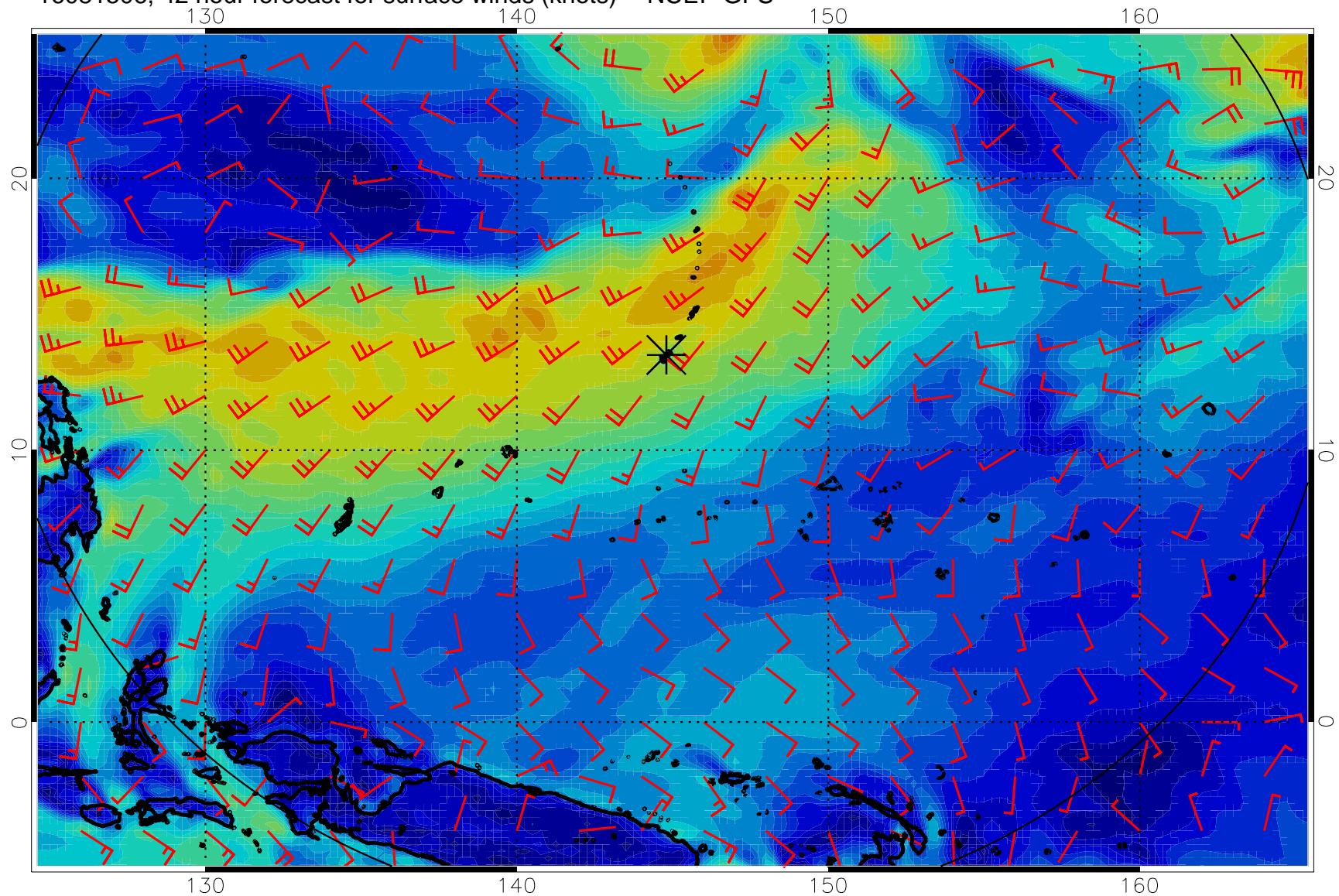
16081506, 42 hour forecast for surface winds (knots) -- NCEP GFS
