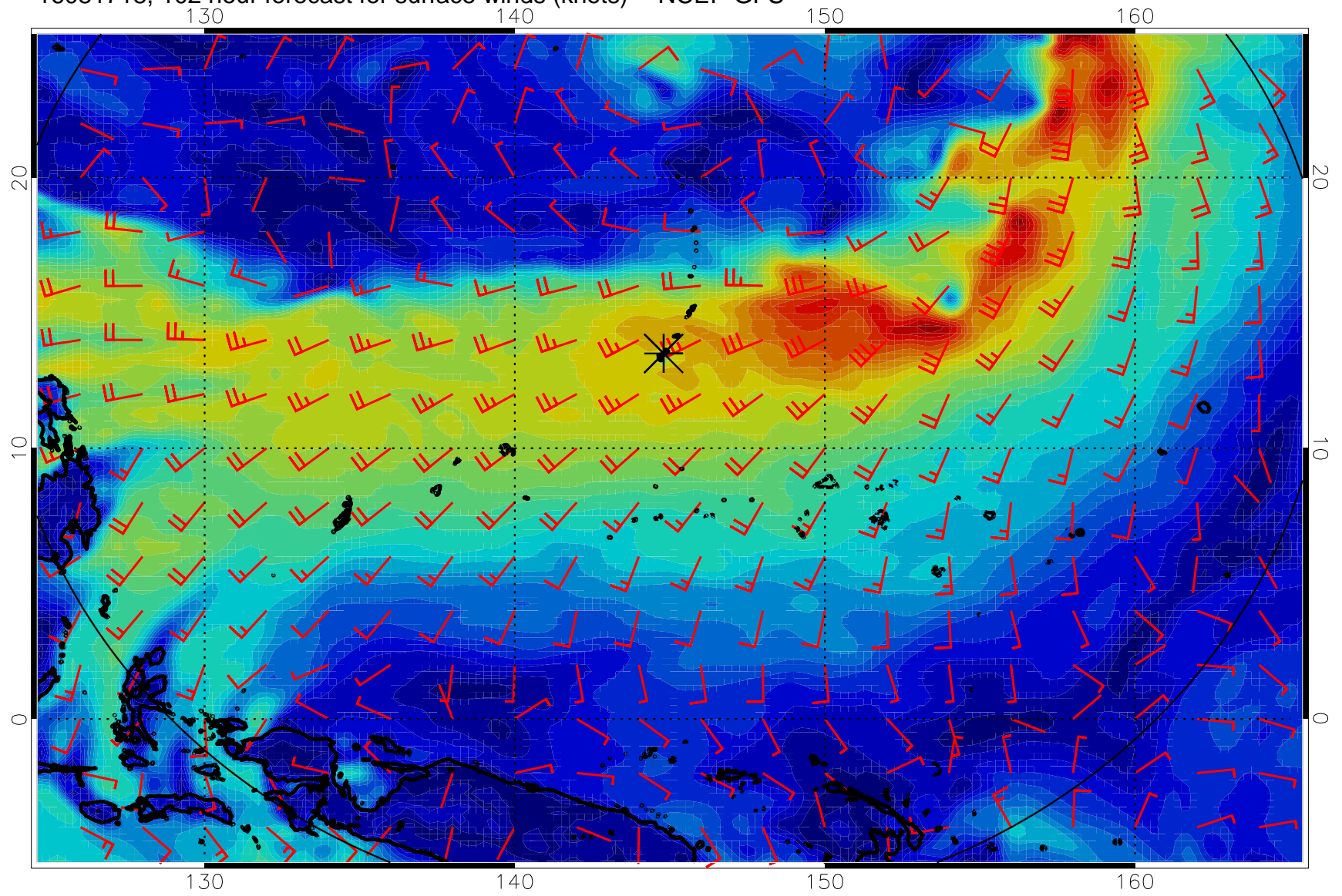
16081718, 102 hour forecast for surface winds (knots) -- NCEP GFS
