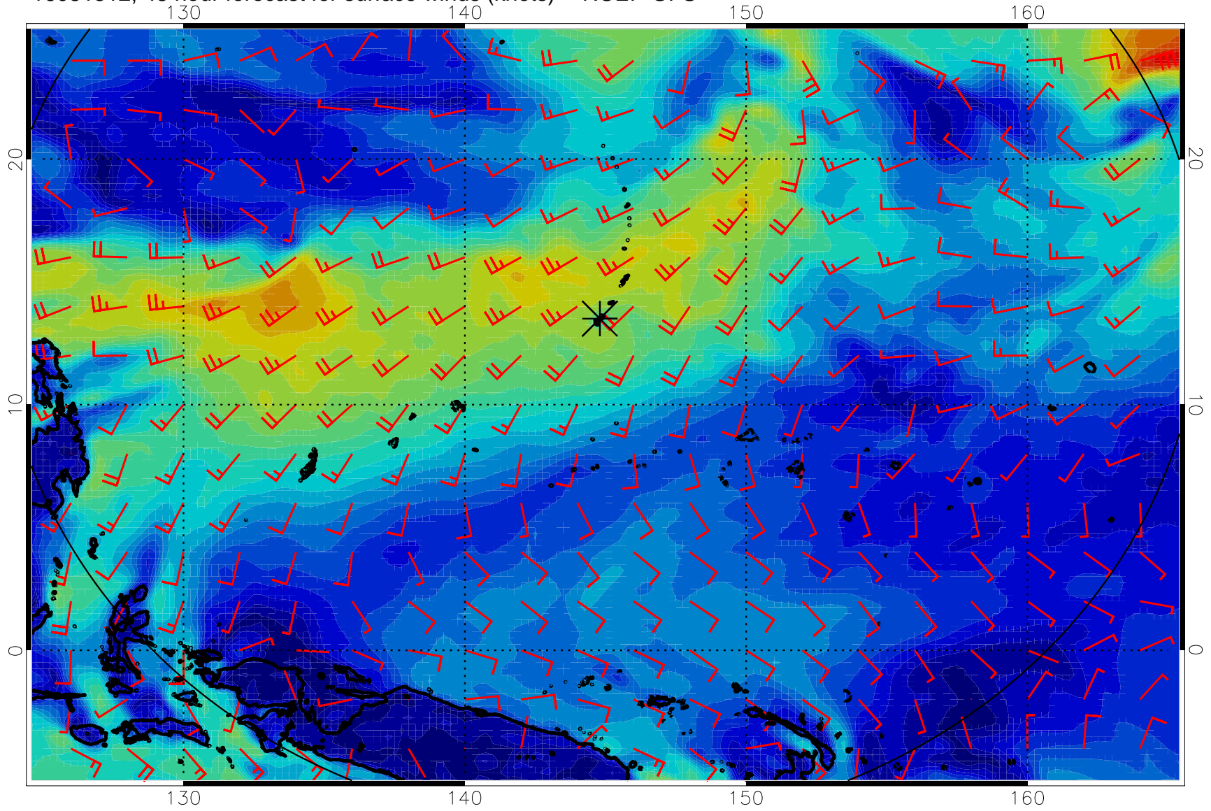
16081512, 48 hour forecast for surface winds (knots) -- NCEP GFS
