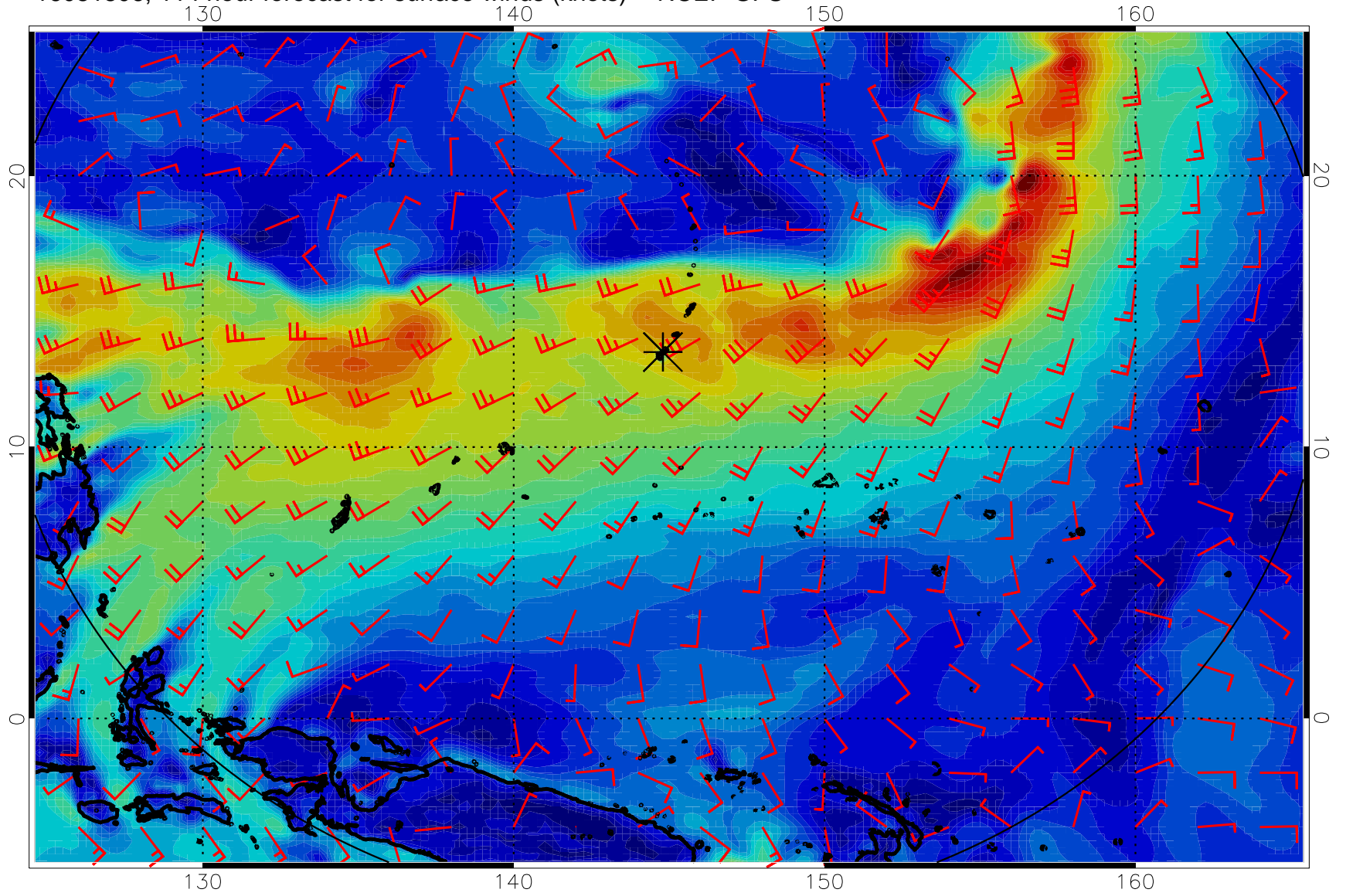
16081806, 114 hour forecast for surface winds (knots) -- NCEP GFS
