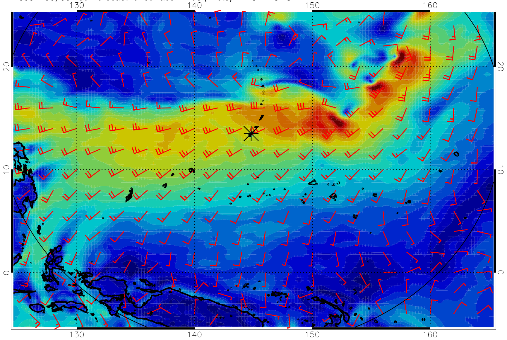
16081706, 90 hour forecast for surface winds (knots) -- NCEP GFS
