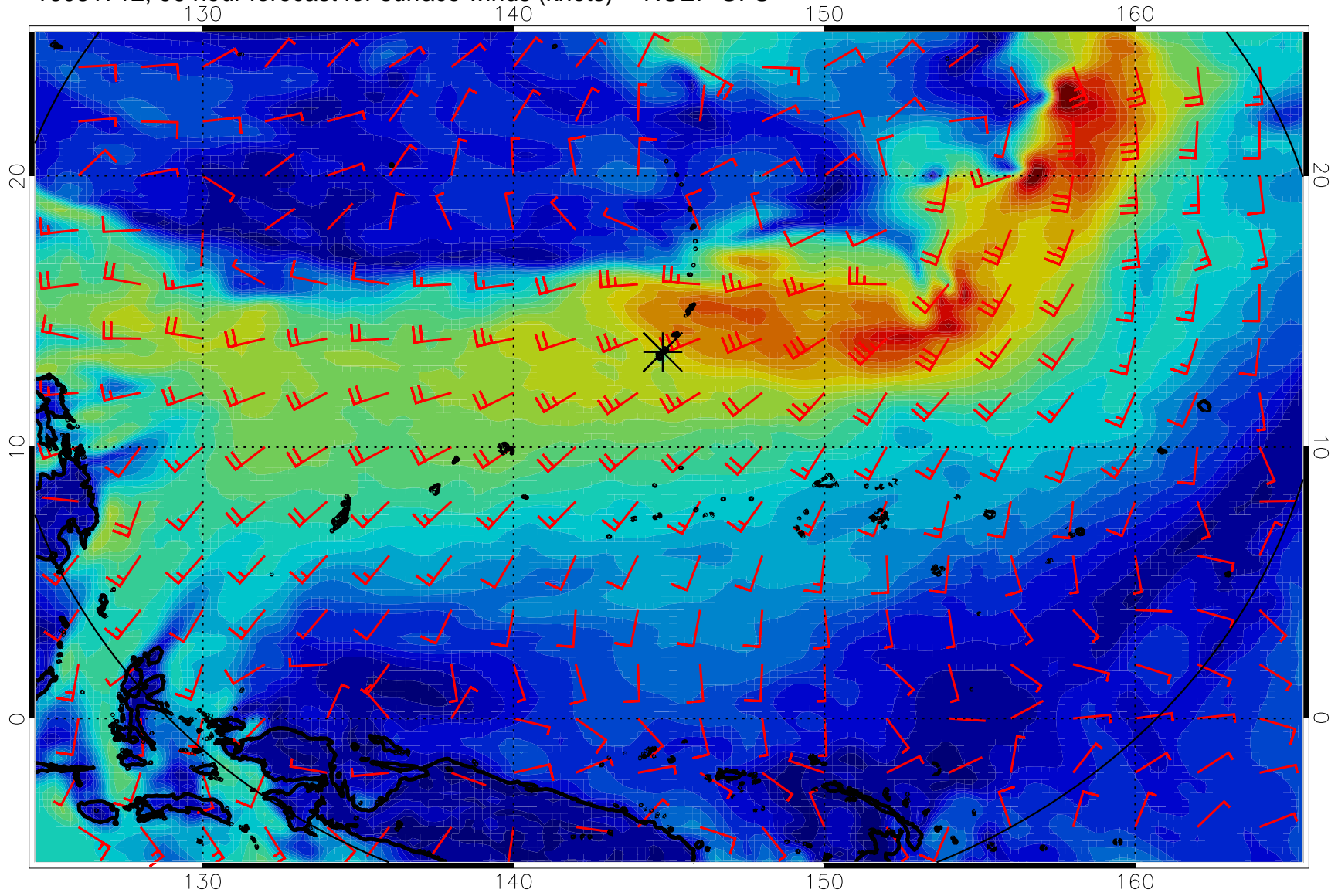
16081712, 96 hour forecast for surface winds (knots) -- NCEP GFS
