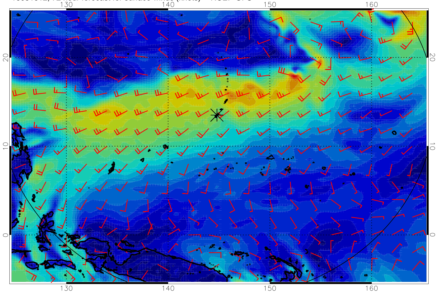
16081612, 72 hour forecast for surface winds (knots) -- NCEP GFS
