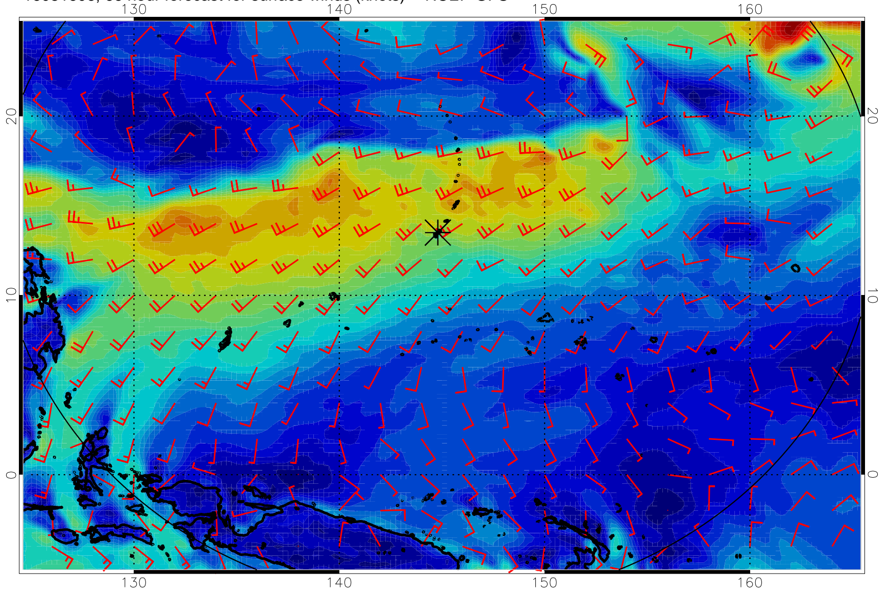
16081606, 66 hour forecast for surface winds (knots) -- NCEP GFS
