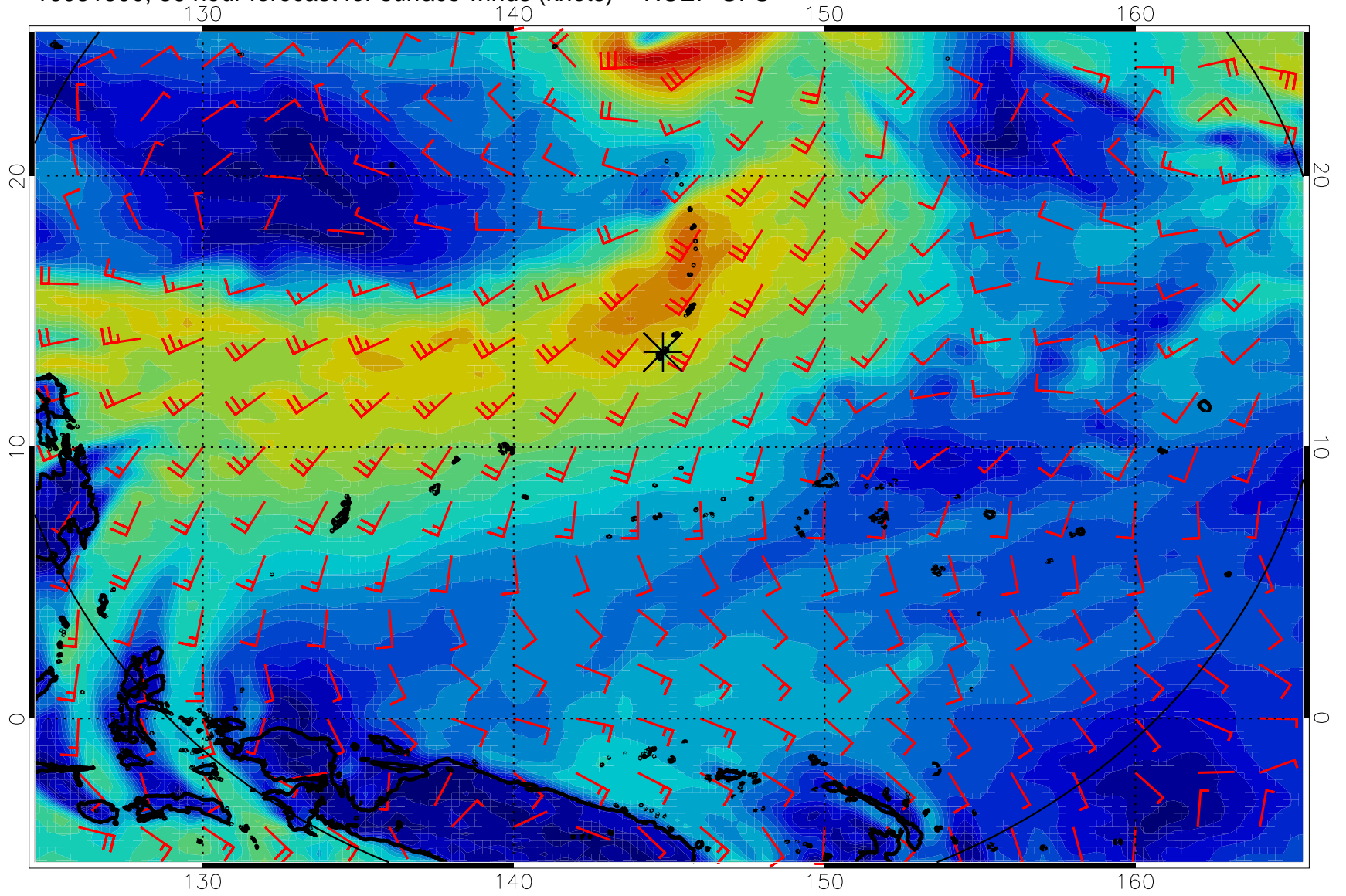
16081500, 36 hour forecast for surface winds (knots) -- NCEP GFS
