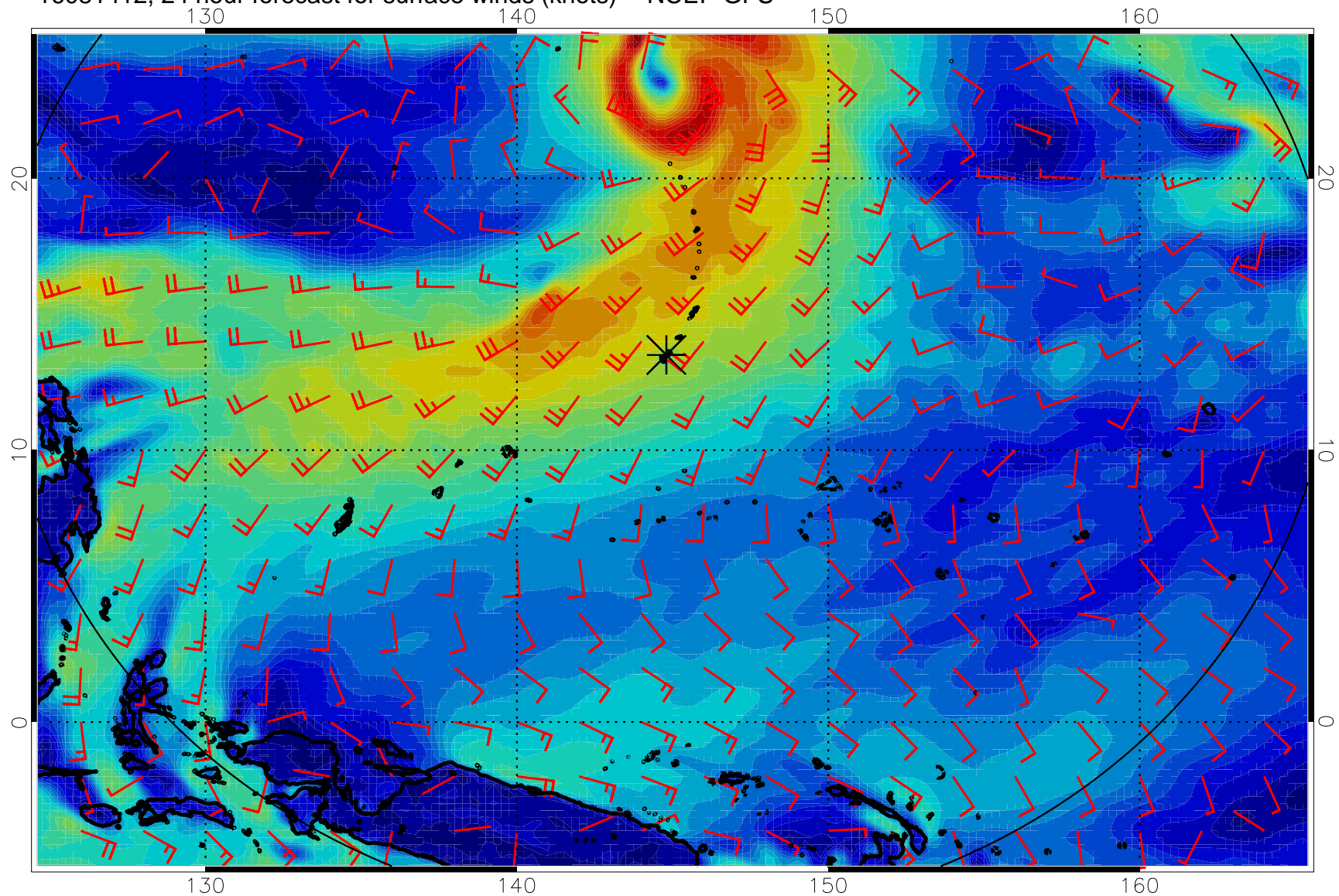
16081412, 24 hour forecast for surface winds (knots) -- NCEP GFS
