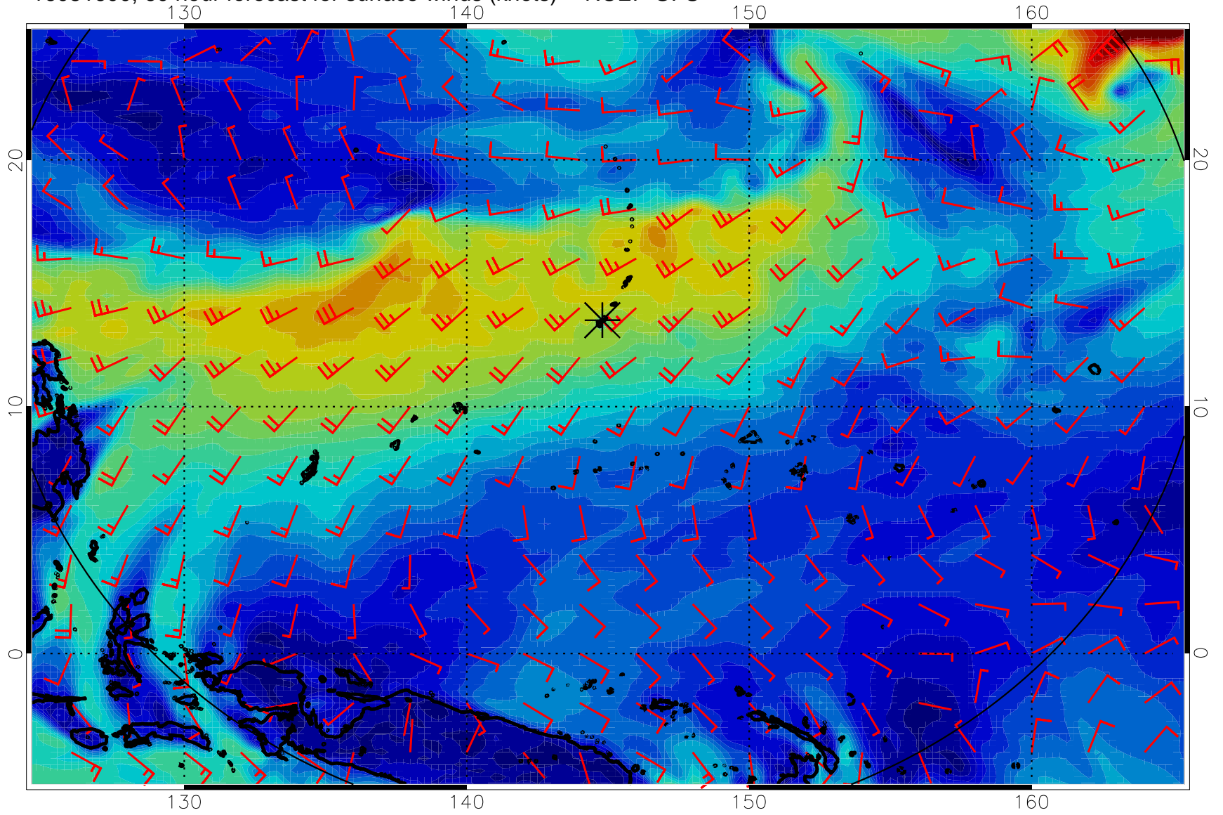
16081600, 60 hour forecast for surface winds (knots) -- NCEP GFS
