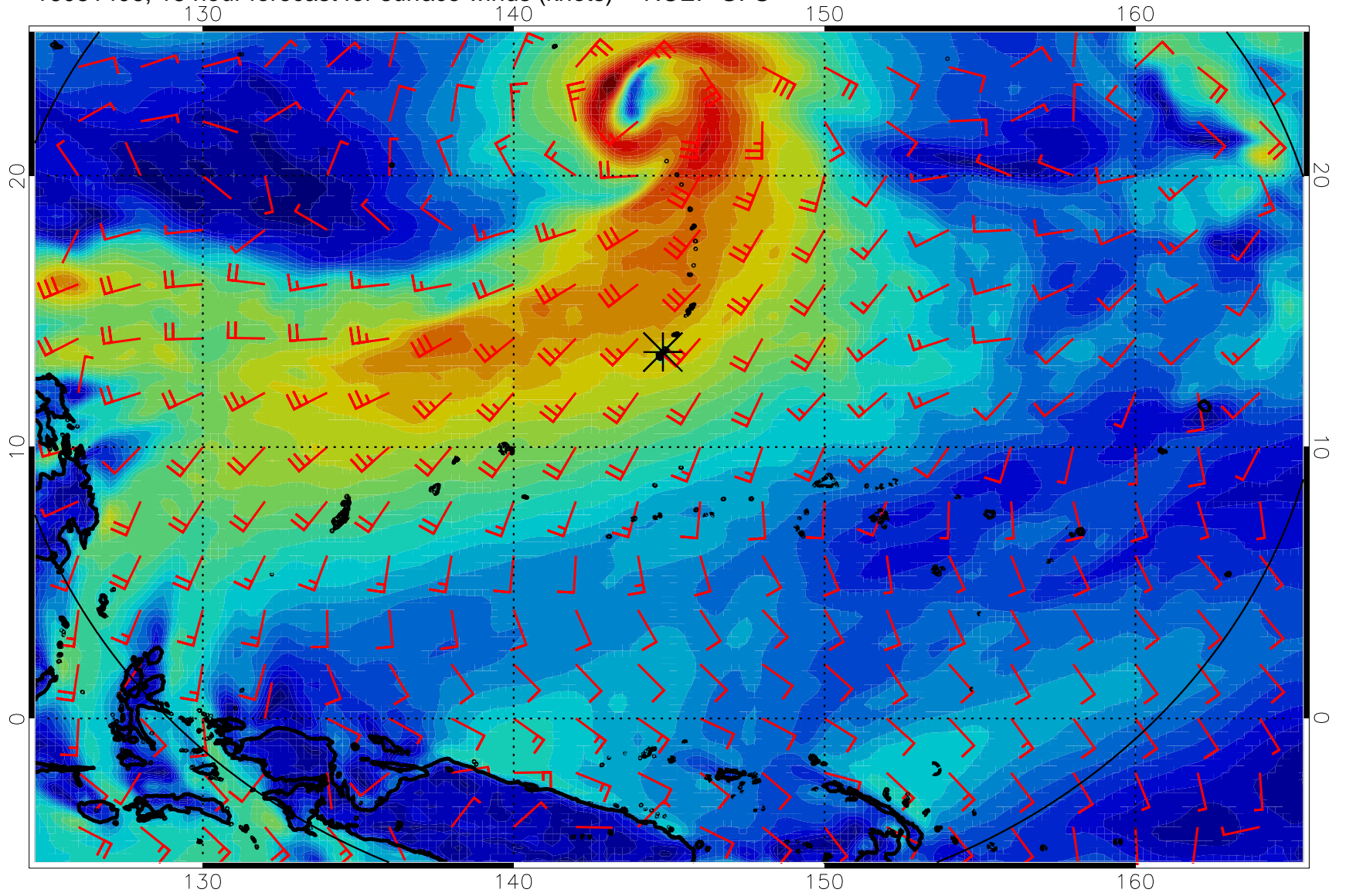
16081406, 18 hour forecast for surface winds (knots) -- NCEP GFS
