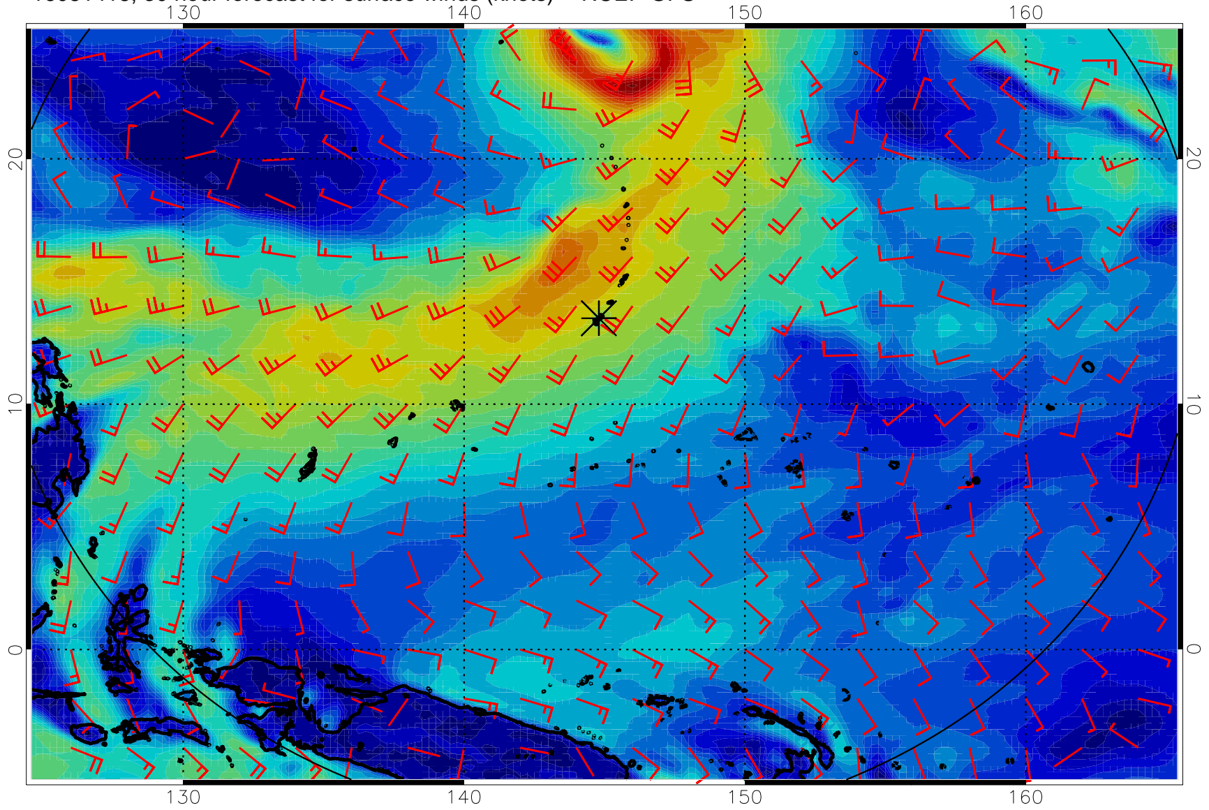
16081418, 30 hour forecast for surface winds (knots) -- NCEP GFS
