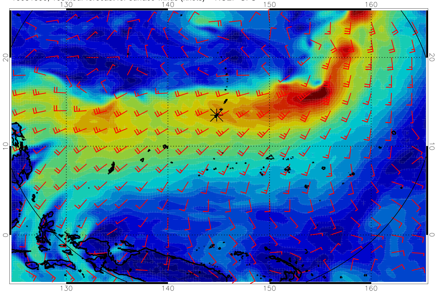
16081800, 108 hour forecast for surface winds (knots) -- NCEP GFS
