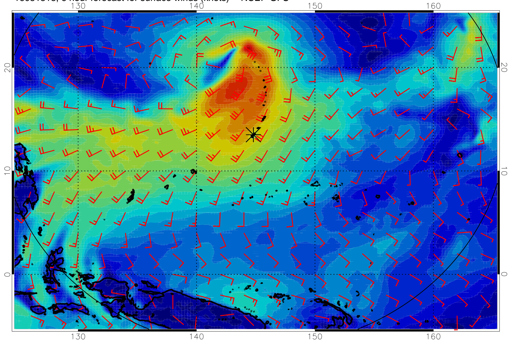
16081318, 6 hour forecast for surface winds (knots) -- NCEP GFS
