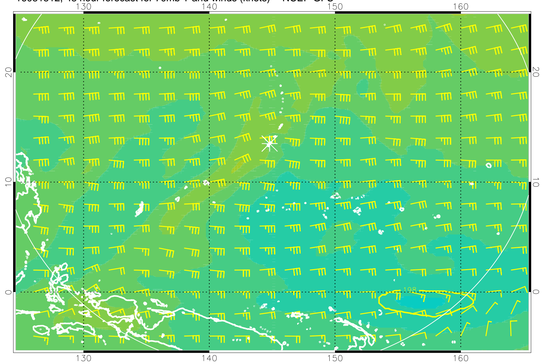
16081512, 48 hour forecast for 70mb T and winds (knots) -- NCEP GFS
