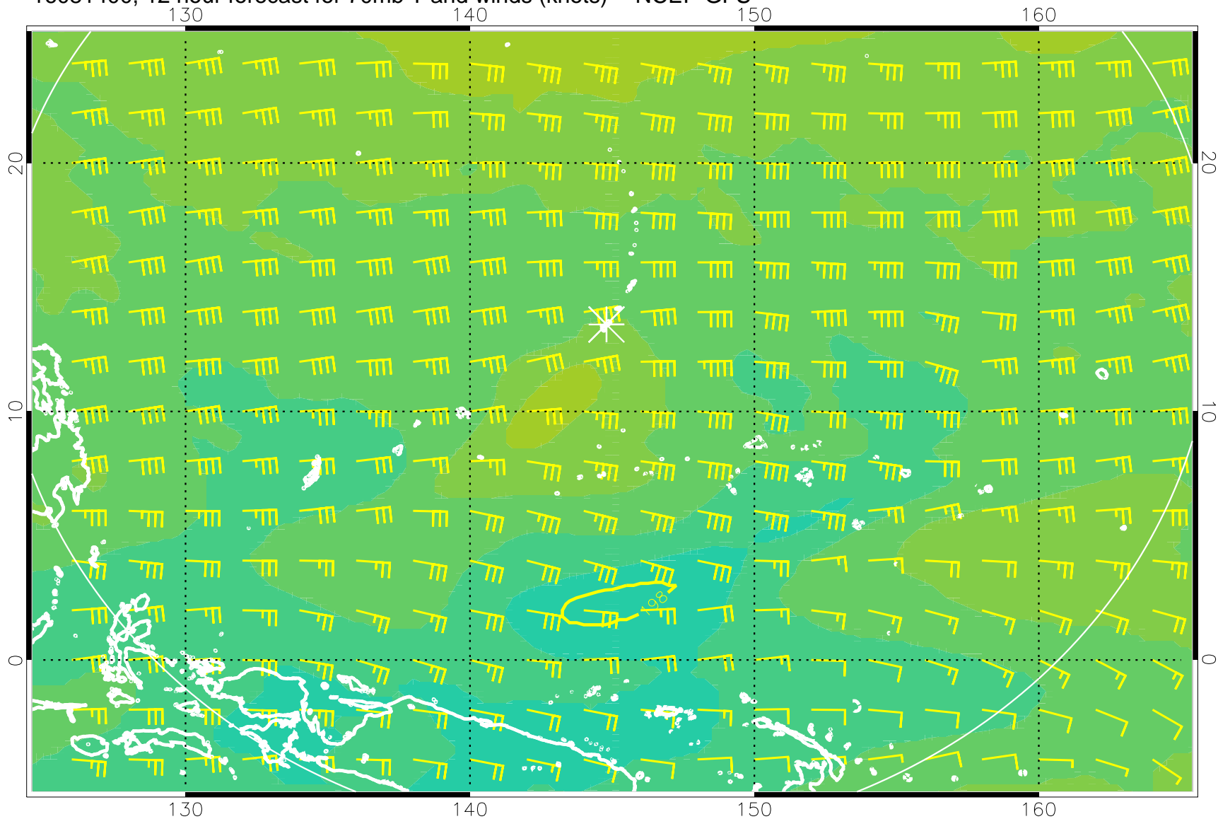
16081400, 12 hour forecast for 70mb T and winds (knots) -- NCEP GFS
