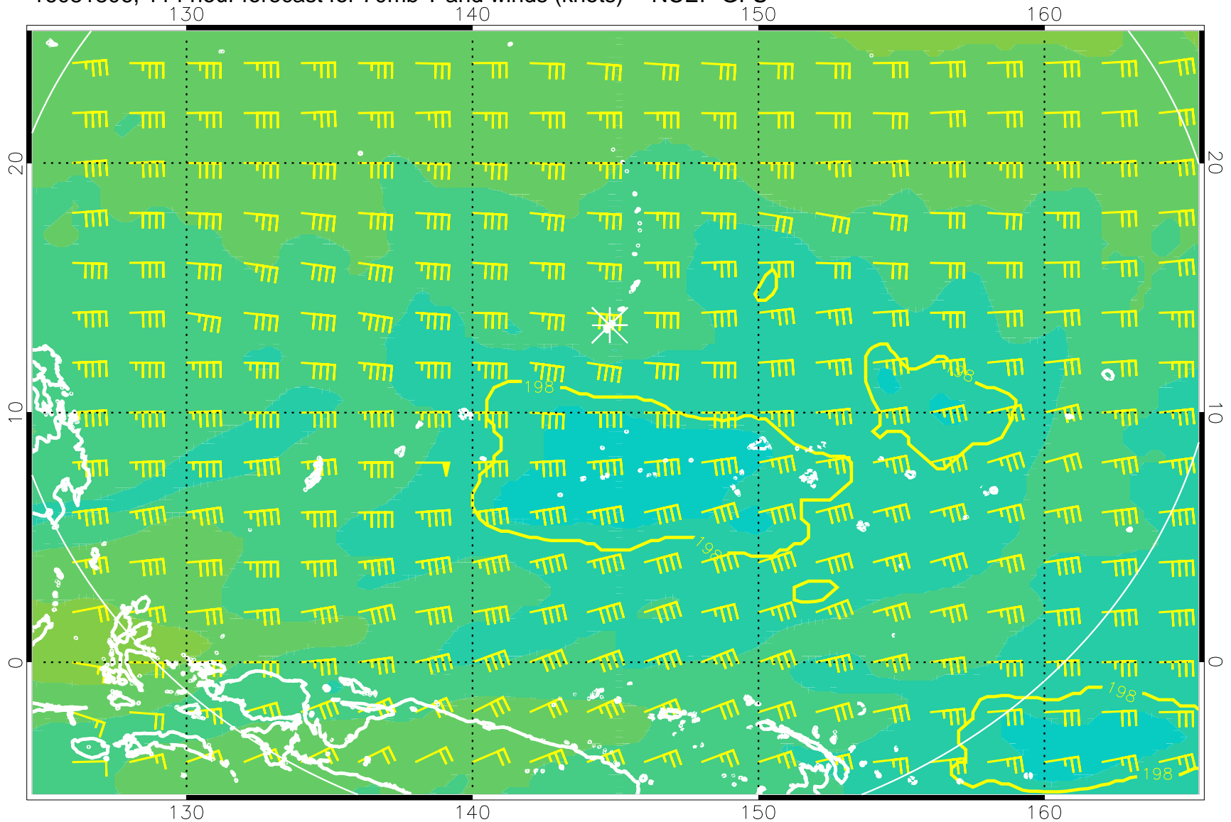
16081806, 114 hour forecast for 70mb T and winds (knots) -- NCEP GFS
