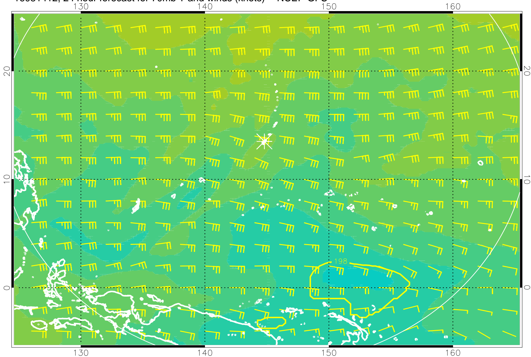
16081412, 24 hour forecast for 70mb T and winds (knots) -- NCEP GFS
