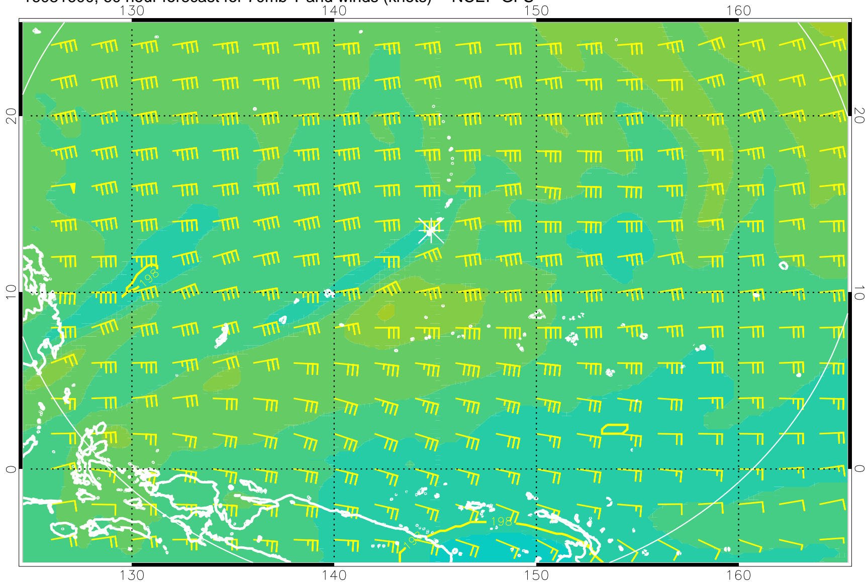
16081600, 60 hour forecast for 70mb T and winds (knots) -- NCEP GFS
