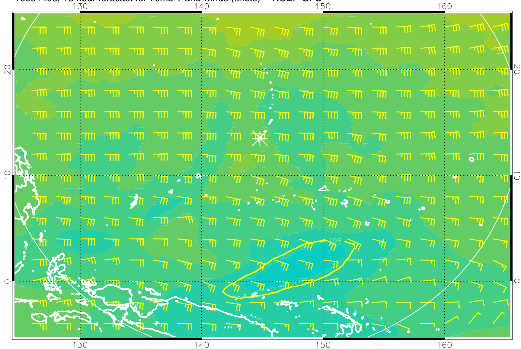
16081406, 18 hour forecast for 70mb T and winds (knots) -- NCEP GFS
