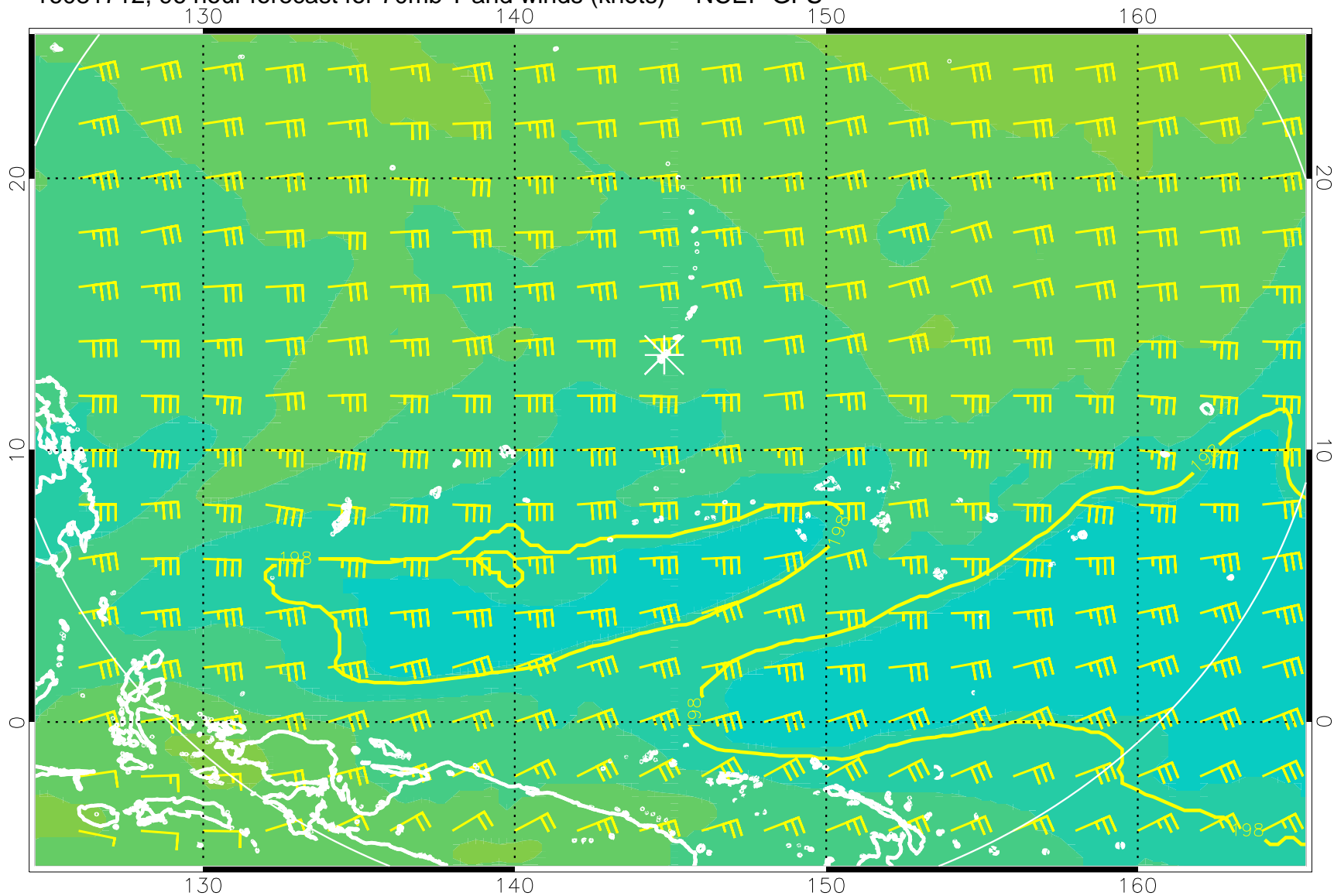
16081712, 96 hour forecast for 70mb T and winds (knots) -- NCEP GFS
