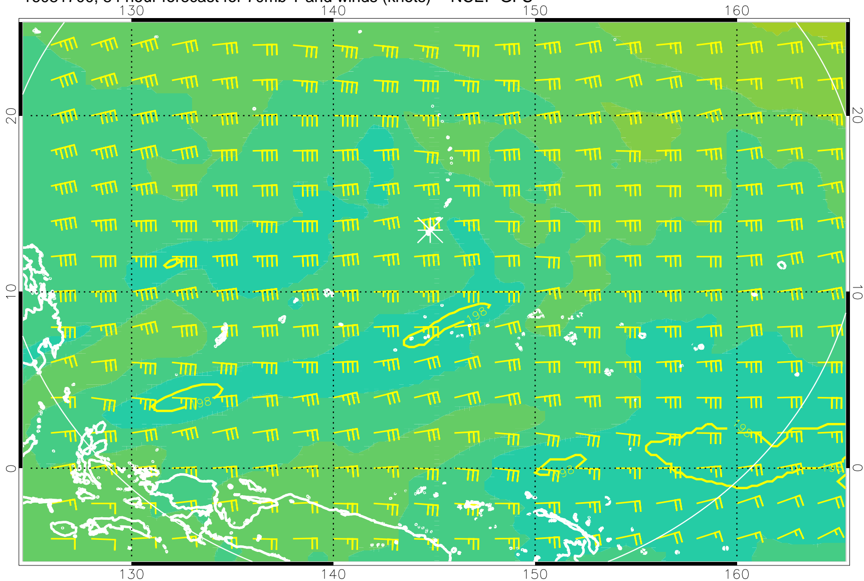
16081700, 84 hour forecast for 70mb T and winds (knots) -- NCEP GFS
