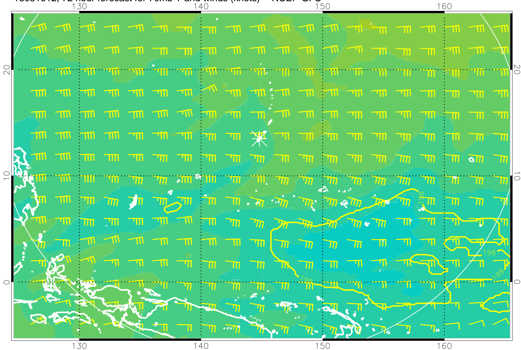
16081612, 72 hour forecast for 70mb T and winds (knots) -- NCEP GFS
