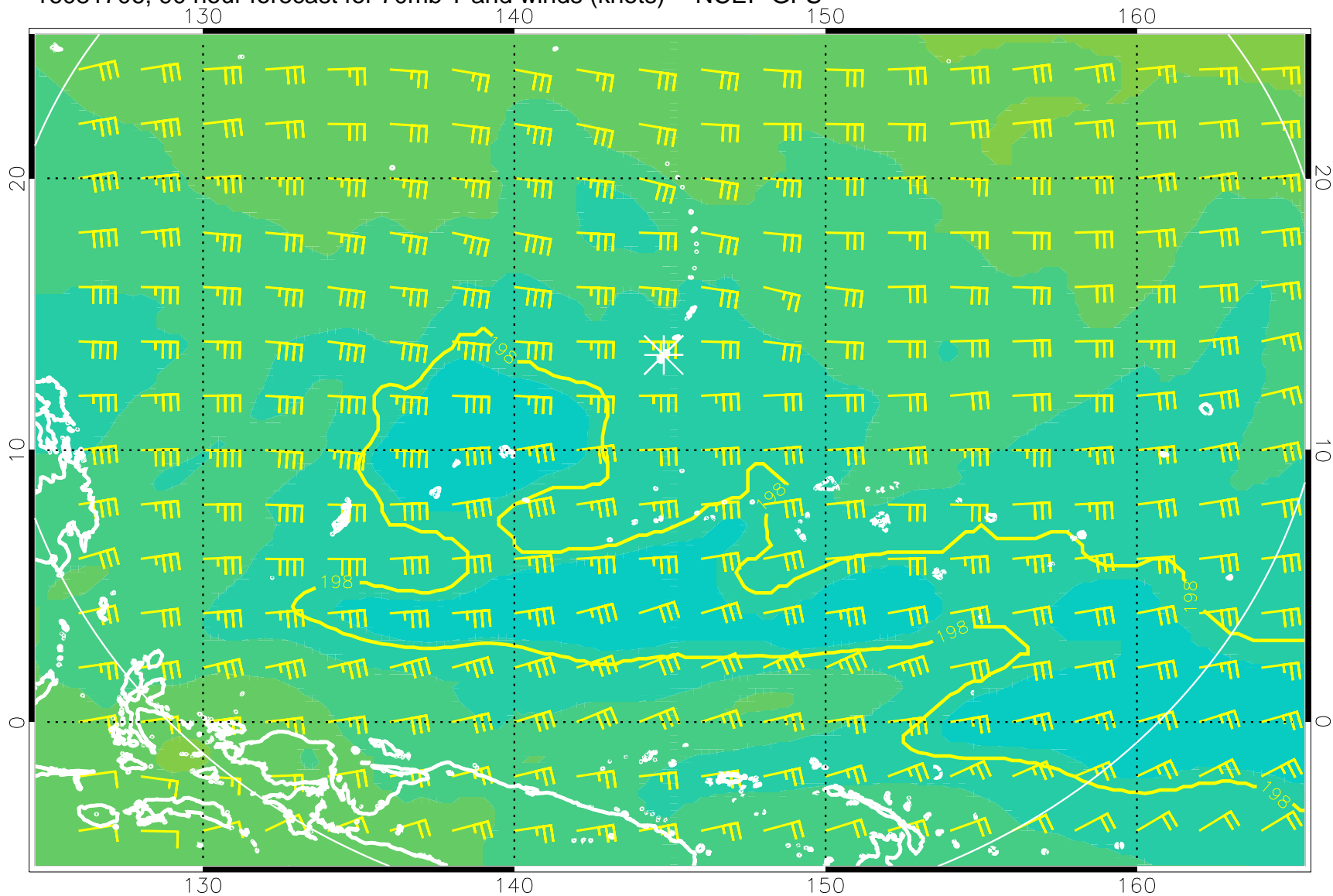
16081706, 90 hour forecast for 70mb T and winds (knots) -- NCEP GFS
