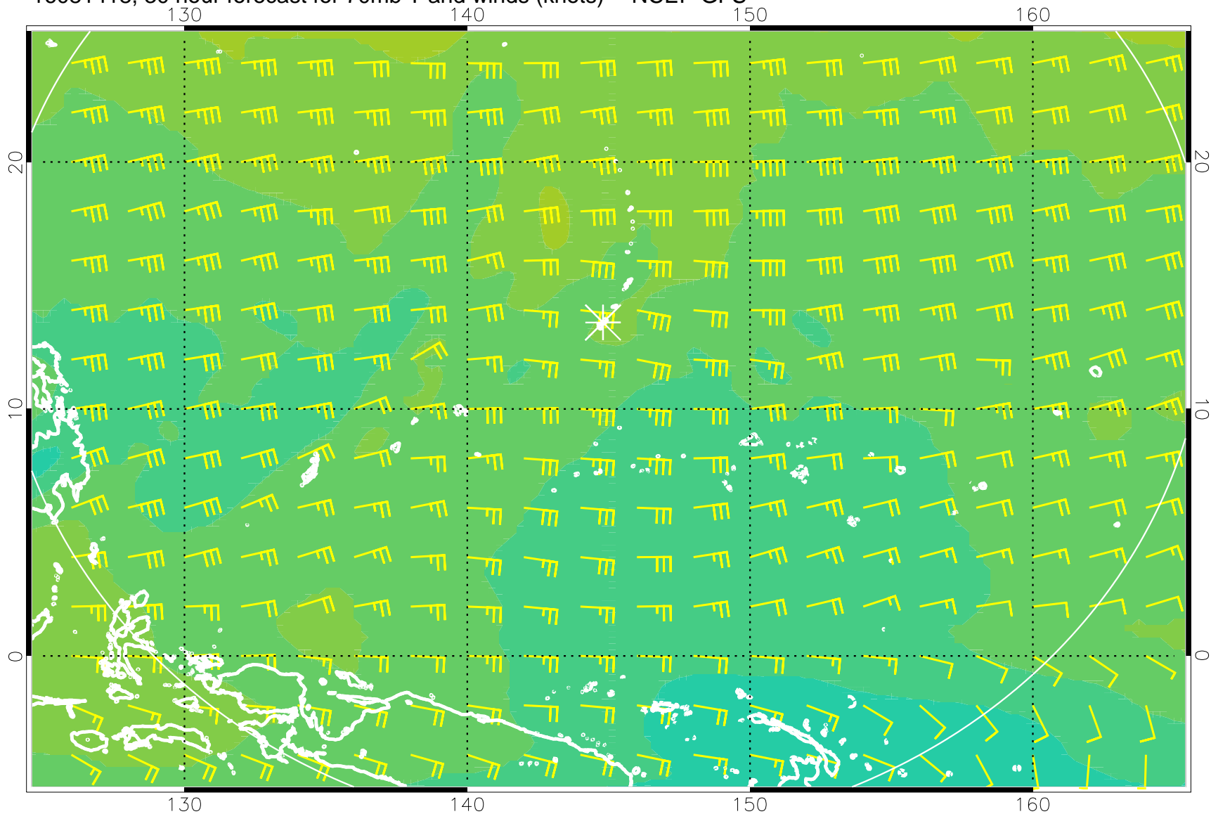
16081418, 30 hour forecast for 70mb T and winds (knots) -- NCEP GFS
