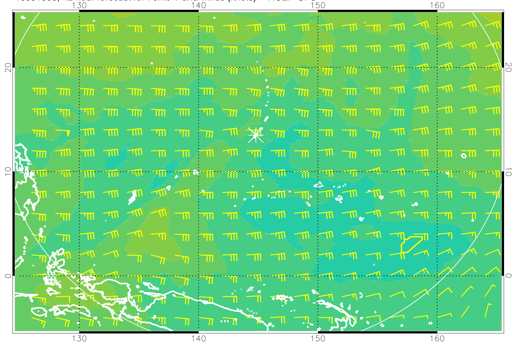
16081506, 42 hour forecast for 70mb T and winds (knots) -- NCEP GFS
