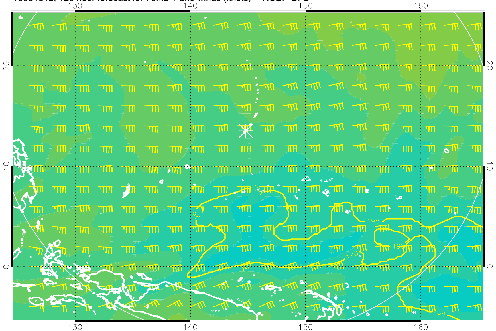
16081812, 120 hour forecast for 70mb T and winds (knots) -- NCEP GFS
