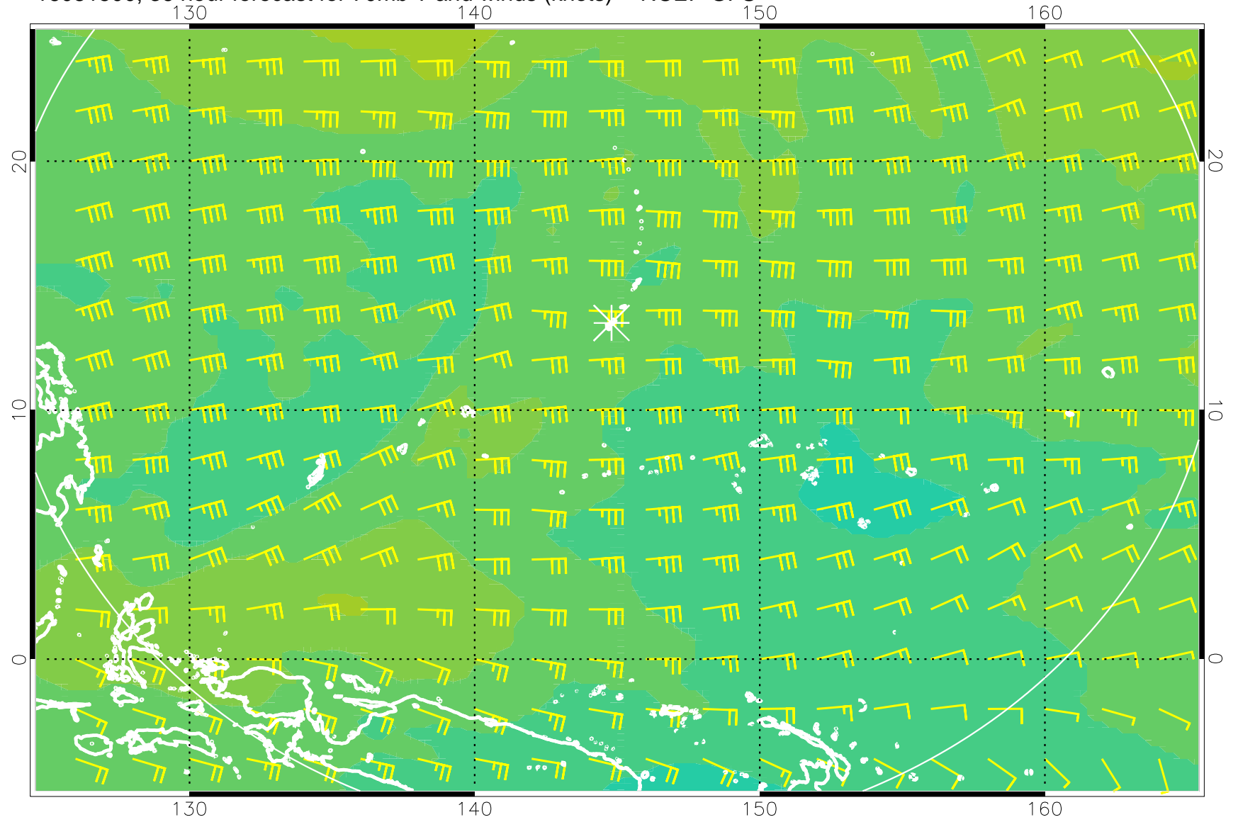
16081500, 36 hour forecast for 70mb T and winds (knots) -- NCEP GFS
