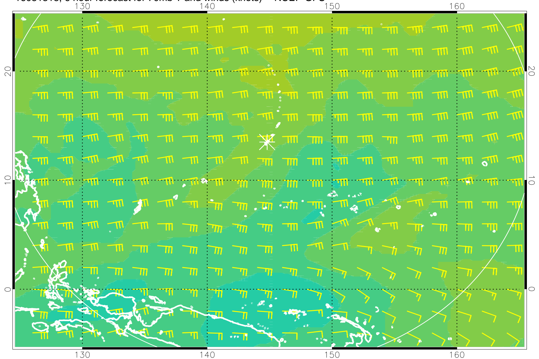
16081318, 6 hour forecast for 70mb T and winds (knots) -- NCEP GFS
