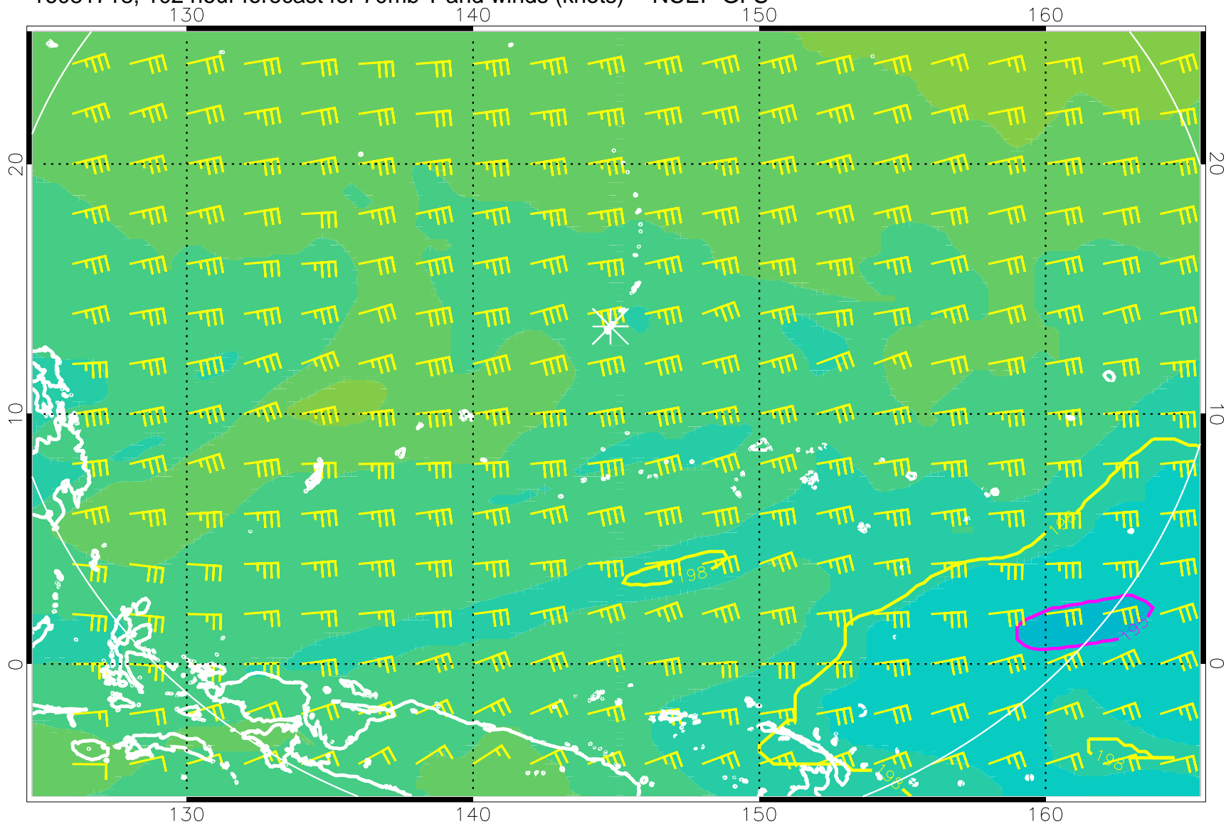
16081718, 102 hour forecast for 70mb T and winds (knots) -- NCEP GFS
