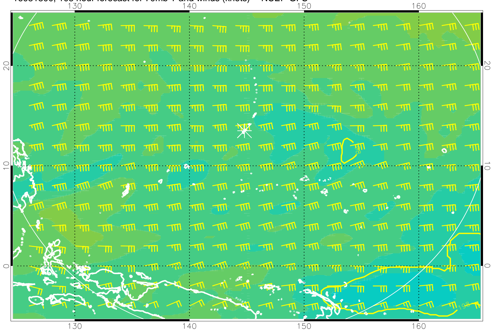
16081800, 108 hour forecast for 70mb T and winds (knots) -- NCEP GFS
