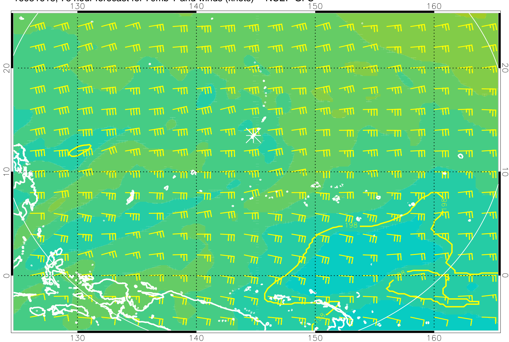
16081618, 78 hour forecast for 70mb T and winds (knots) -- NCEP GFS
