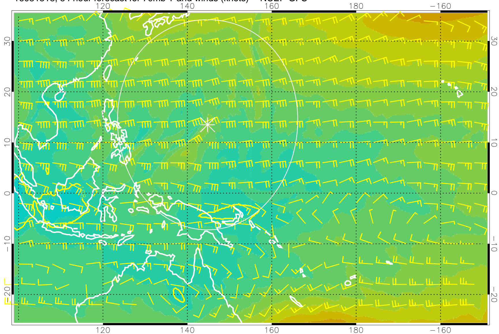
16081518, 54 hour forecast for 70mb T and winds (knots) -- NCEP GFS
