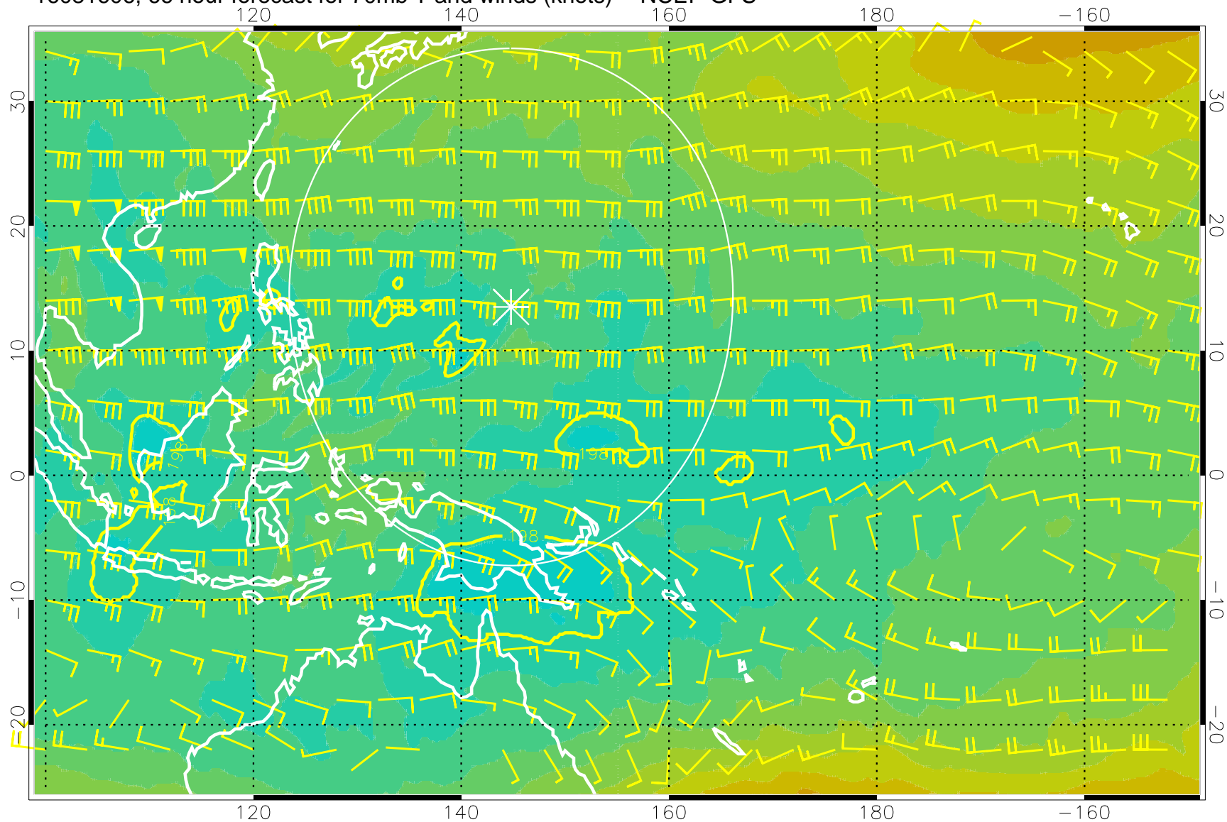
16081606, 66 hour forecast for 70mb T and winds (knots) -- NCEP GFS
