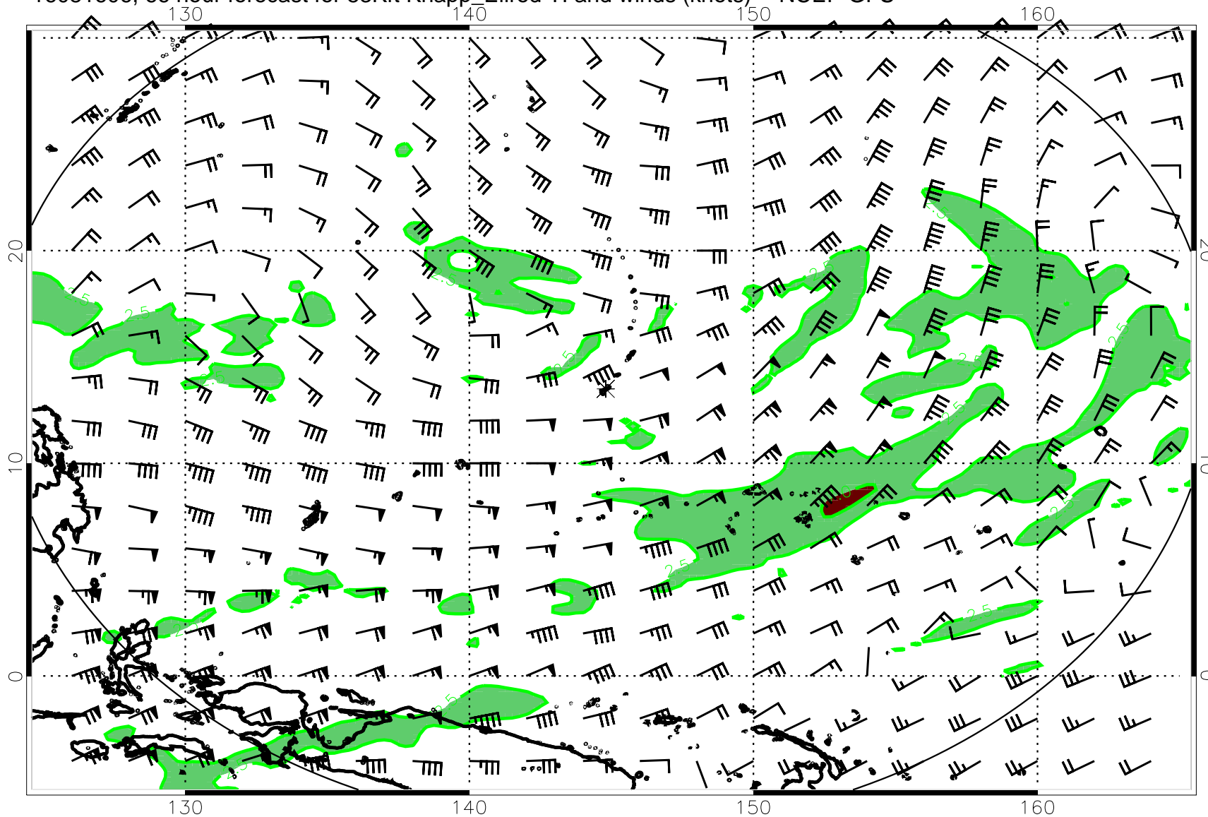
16081606, 66 hour forecast for 53Kft Knapp_Ellrod TI and winds (knots) -- NCEP GFS
