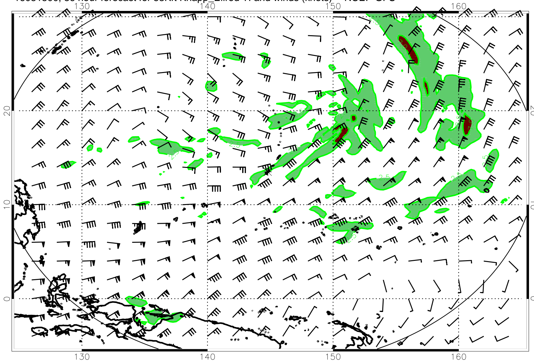
16081500, 36 hour forecast for 53Kft Knapp_Ellrod TI and winds (knots) -- NCEP GFS
