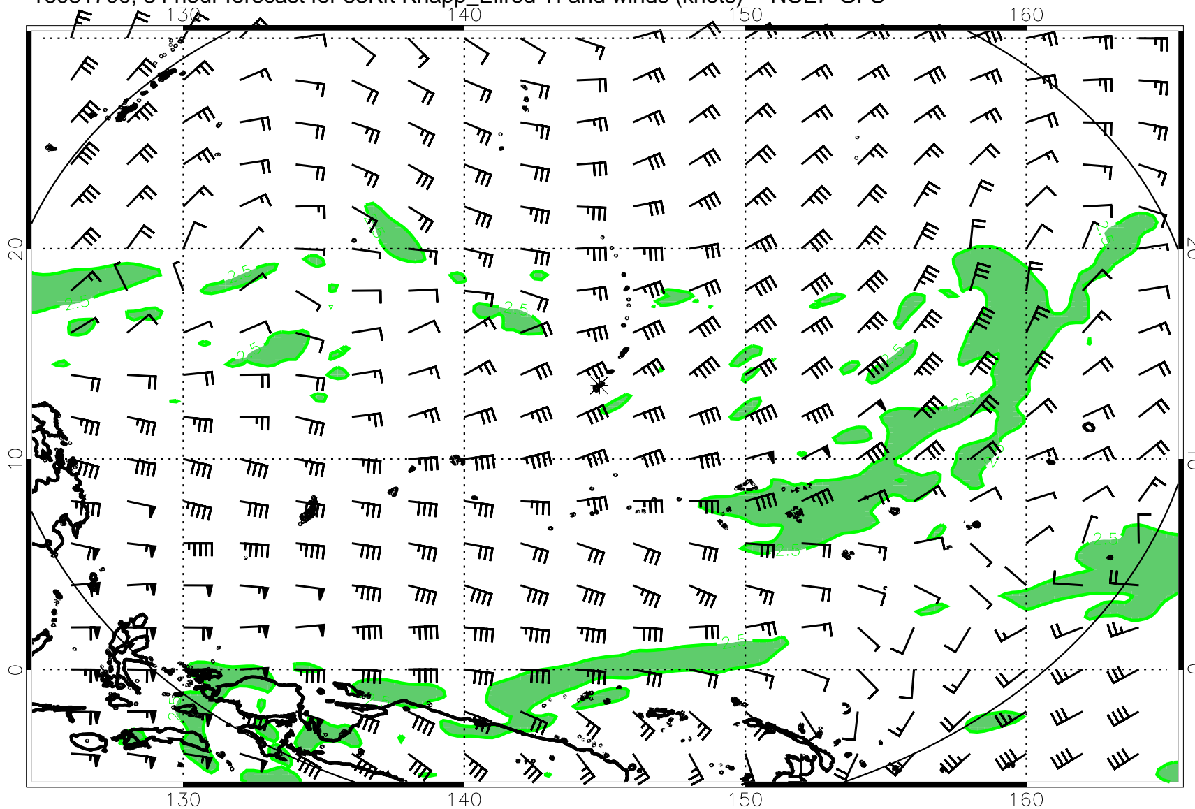
16081700, 84 hour forecast for 53Kft Knapp_Ellrod TI and winds (knots) -- NCEP GFS
