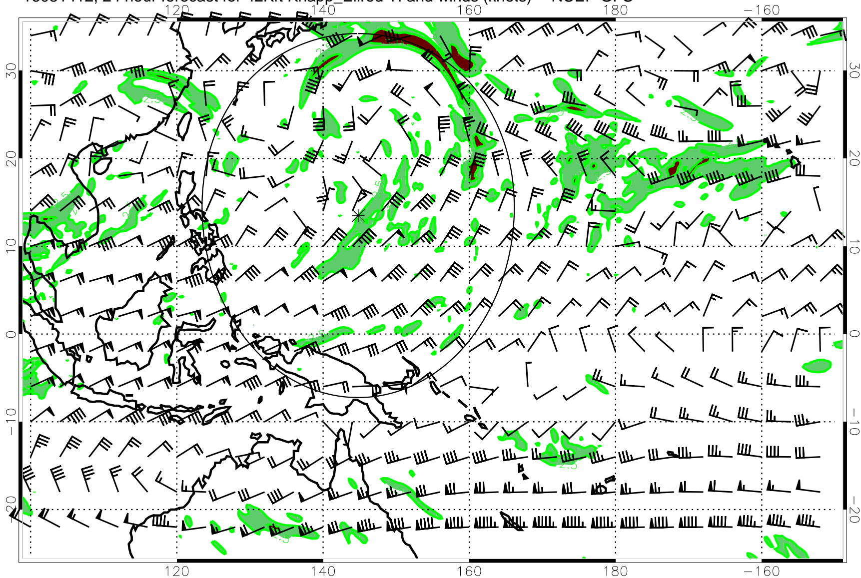
16081412, 24 hour forecast for 42Kft Knapp_Ellrod TI and winds (knots) -- NCEP GFS
