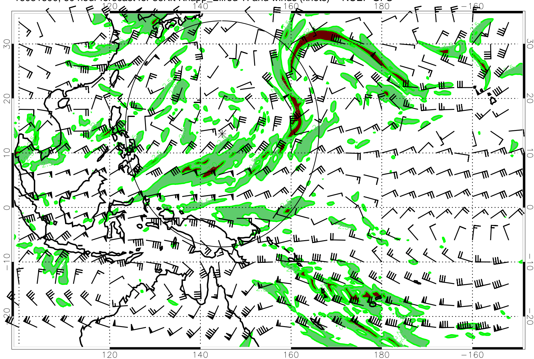
16081600, 60 hour forecast for 36Kft Knapp_Ellrod TI and winds (knots) -- NCEP GFS
