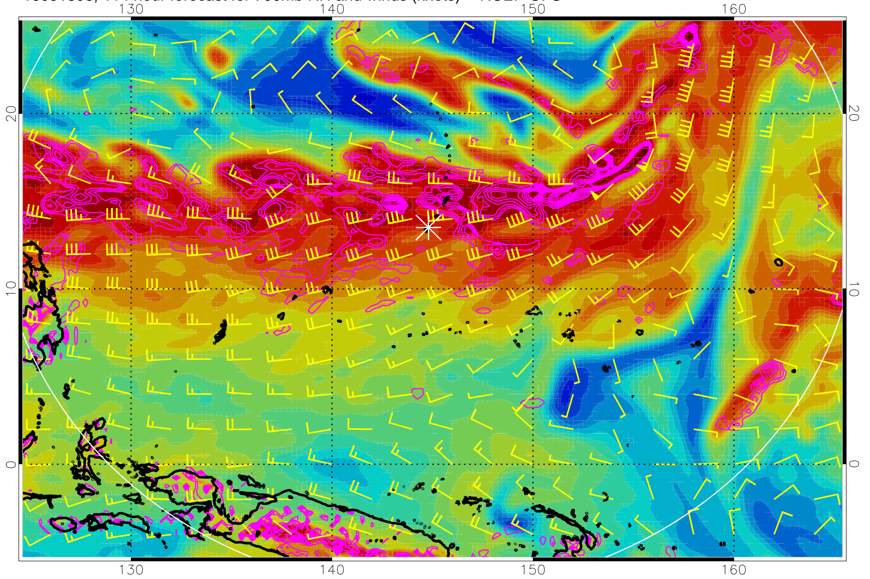
16081806, 114 hour forecast for 700mb RH and winds (knots) -- NCEP GFS
