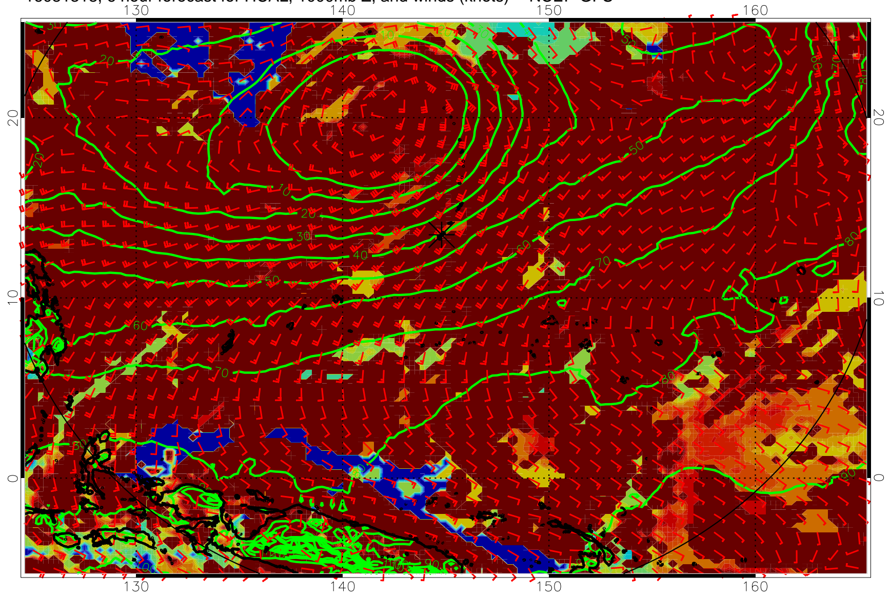
16081318, 6 hour forecast for HCAL, 1000mb Z, and winds (knots) -- NCEP GFS
