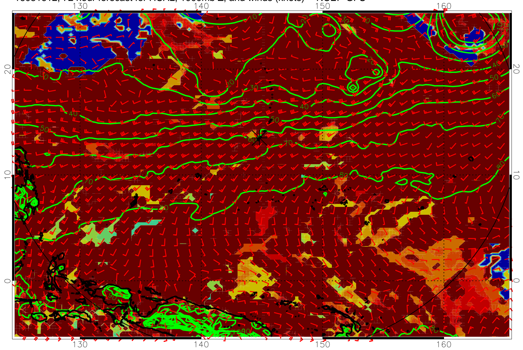
16081612, 72 hour forecast for HCAL, 1000mb Z, and winds (knots) -- NCEP GFS
