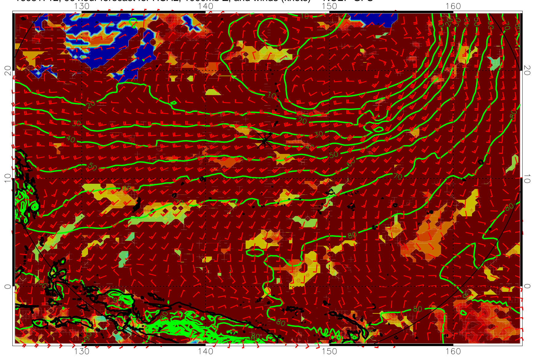
16081712, 96 hour forecast for HCAL, 1000mb Z, and winds (knots) -- NCEP GFS
