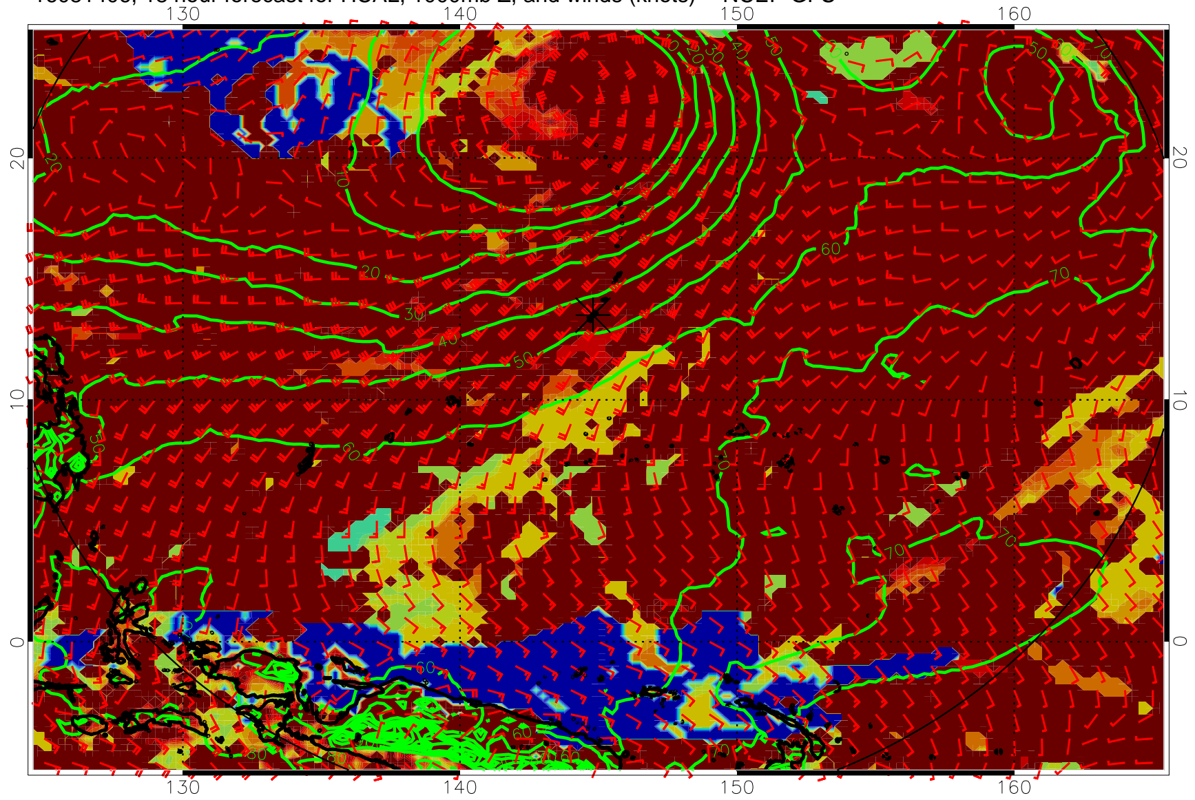
16081406, 18 hour forecast for HCAL, 1000mb Z, and winds (knots) -- NCEP GFS
