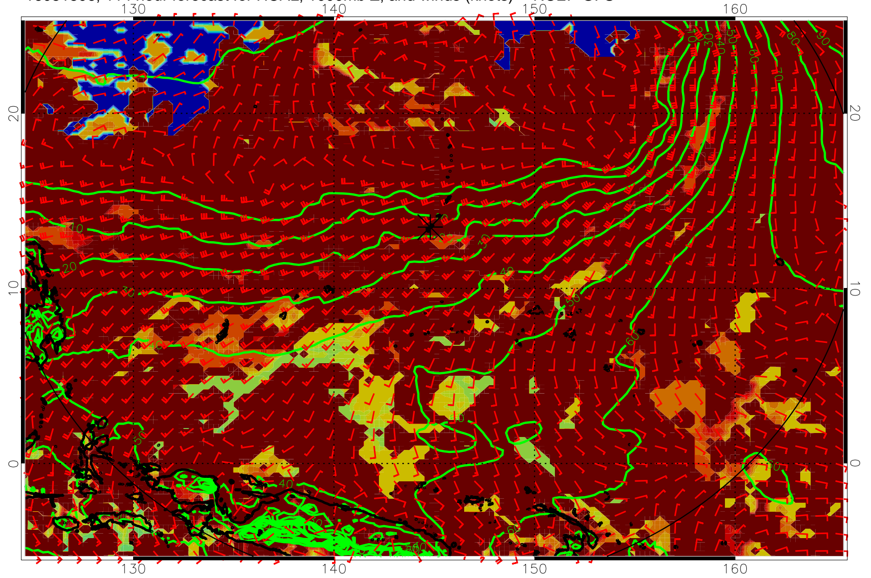
16081806, 114 hour forecast for HCAL, 1000mb Z, and winds (knots) -- NCEP GFS
