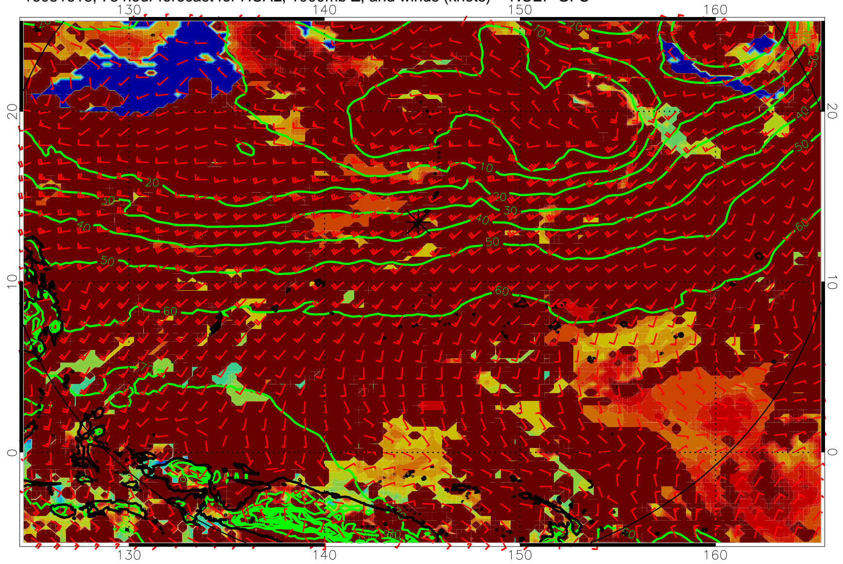
16081618, 78 hour forecast for HCAL, 1000mb Z, and winds (knots) -- NCEP GFS
