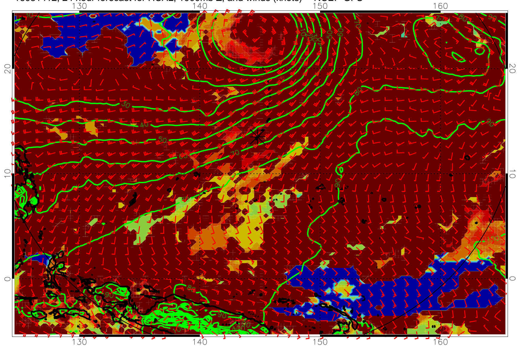
16081412, 24 hour forecast for HCAL, 1000mb Z, and winds (knots) -- NCEP GFS
