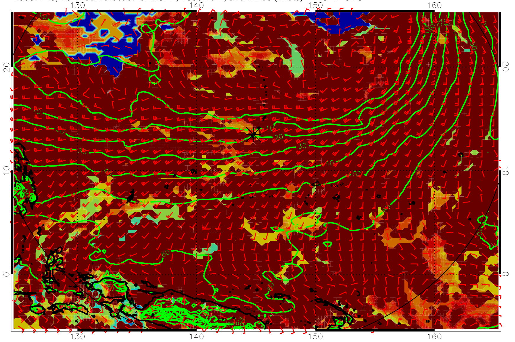
16081718, 102 hour forecast for HCAL, 1000mb Z, and winds (knots) -- NCEP GFS
