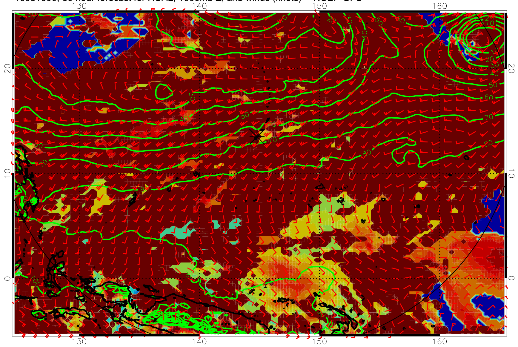
16081600, 60 hour forecast for HCAL, 1000mb Z, and winds (knots) -- NCEP GFS
