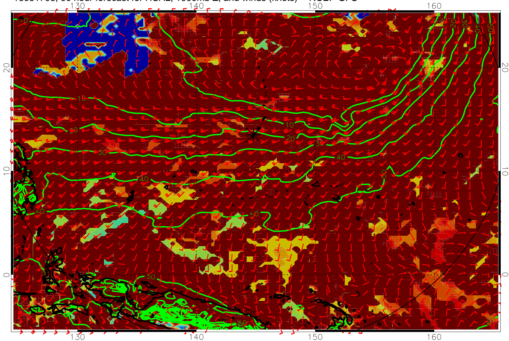
16081706, 90 hour forecast for HCAL, 1000mb Z, and winds (knots) -- NCEP GFS
