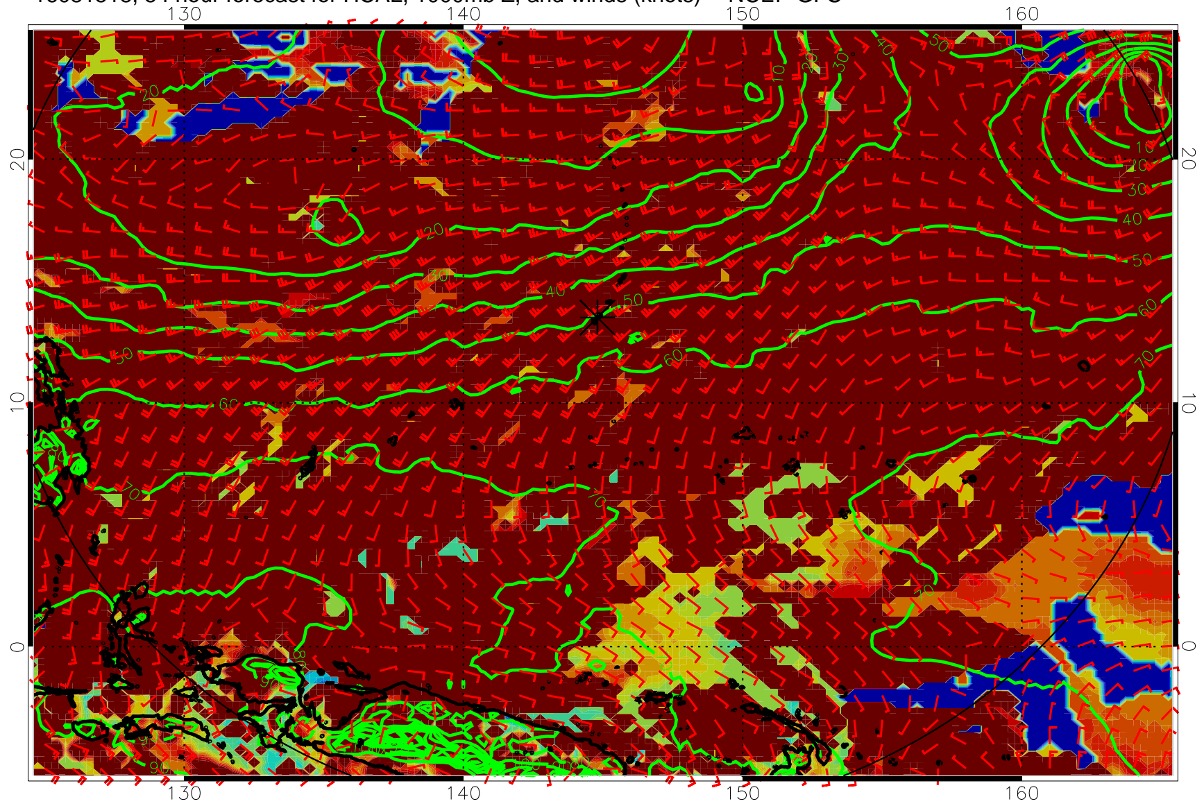
16081518, 54 hour forecast for HCAL, 1000mb Z, and winds (knots) -- NCEP GFS
