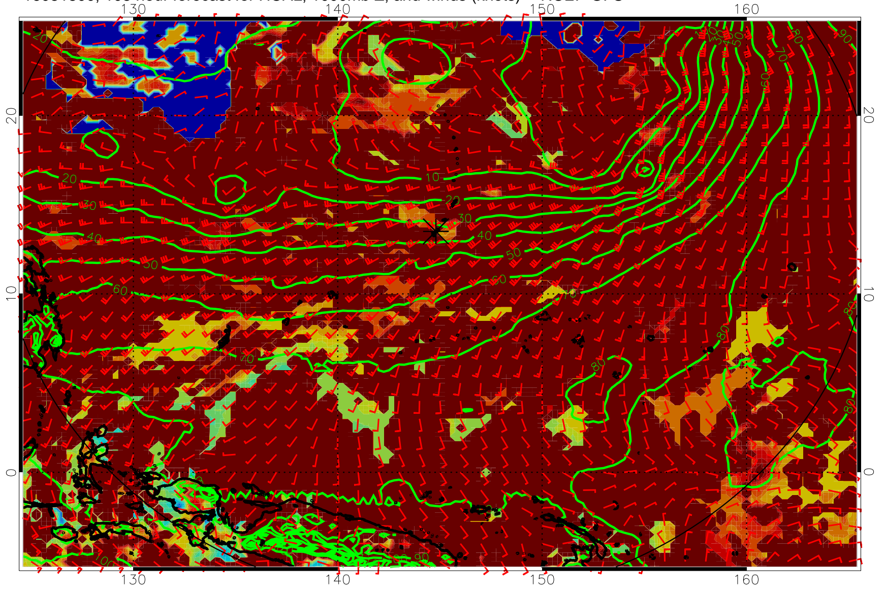
16081800, 108 hour forecast for HCAL, 1000mb Z, and winds (knots) -- NCEP GFS
