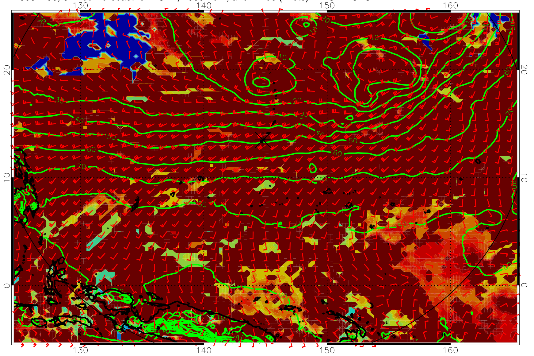
16081700, 84 hour forecast for HCAL, 1000mb Z, and winds (knots) -- NCEP GFS
