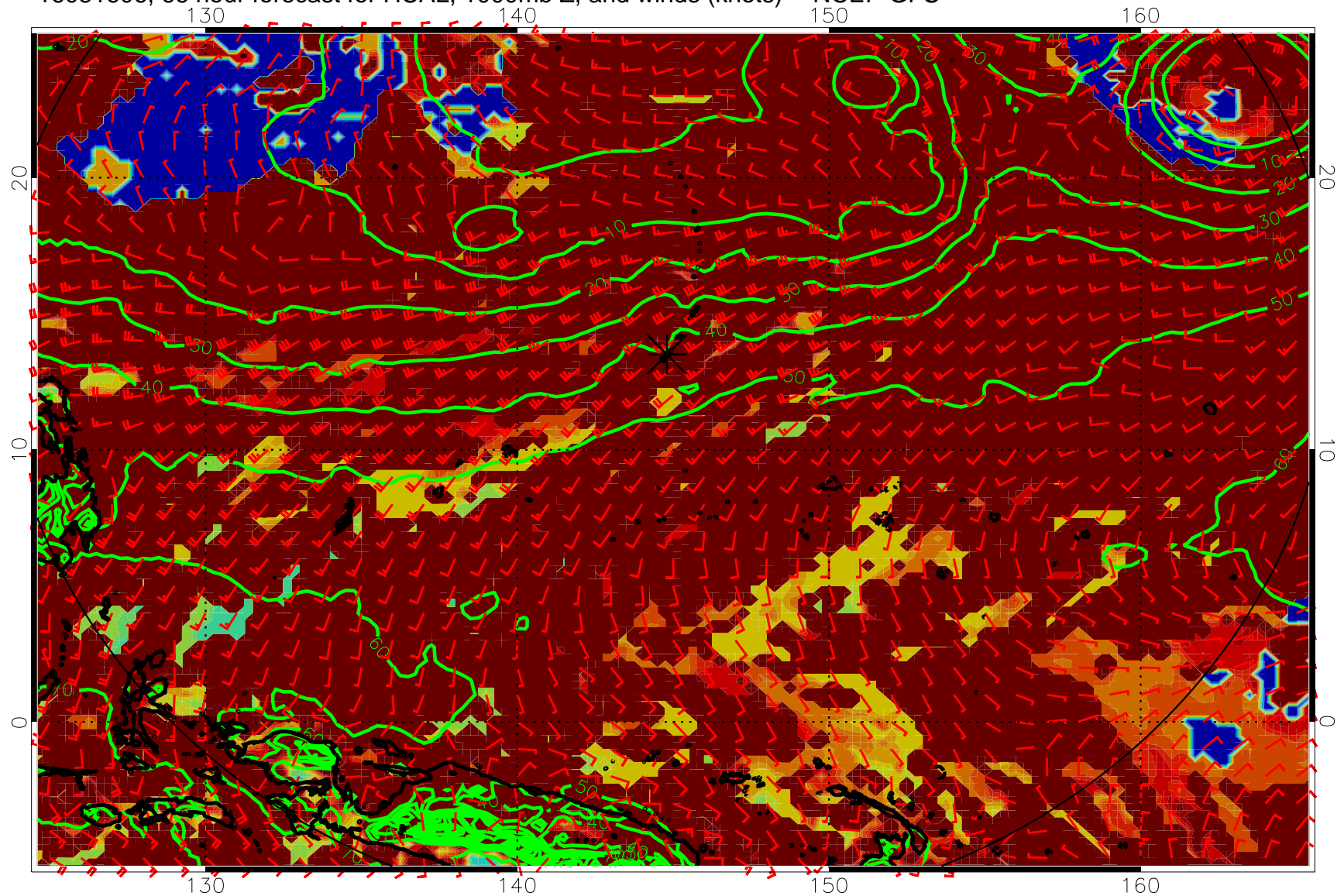
16081606, 66 hour forecast for HCAL, 1000mb Z, and winds (knots) -- NCEP GFS
