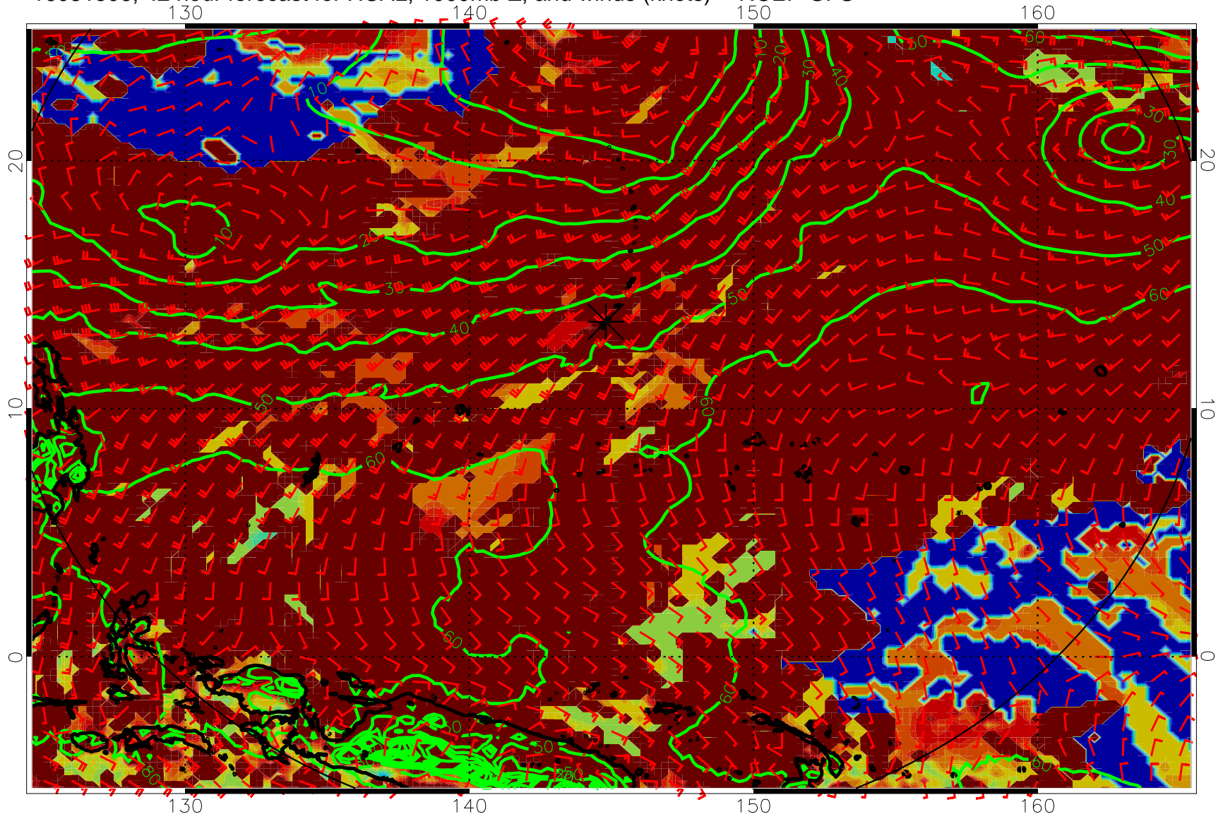
16081506, 42 hour forecast for HCAL, 1000mb Z, and winds (knots) -- NCEP GFS
