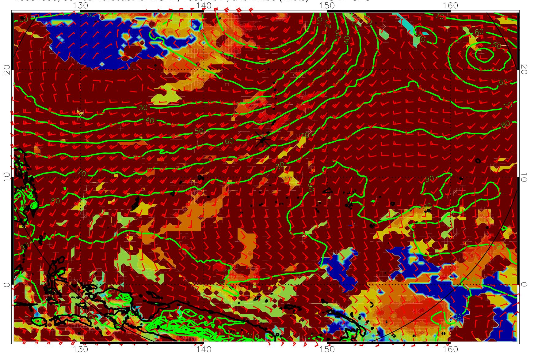
16081500, 36 hour forecast for HCAL, 1000mb Z, and winds (knots) -- NCEP GFS
