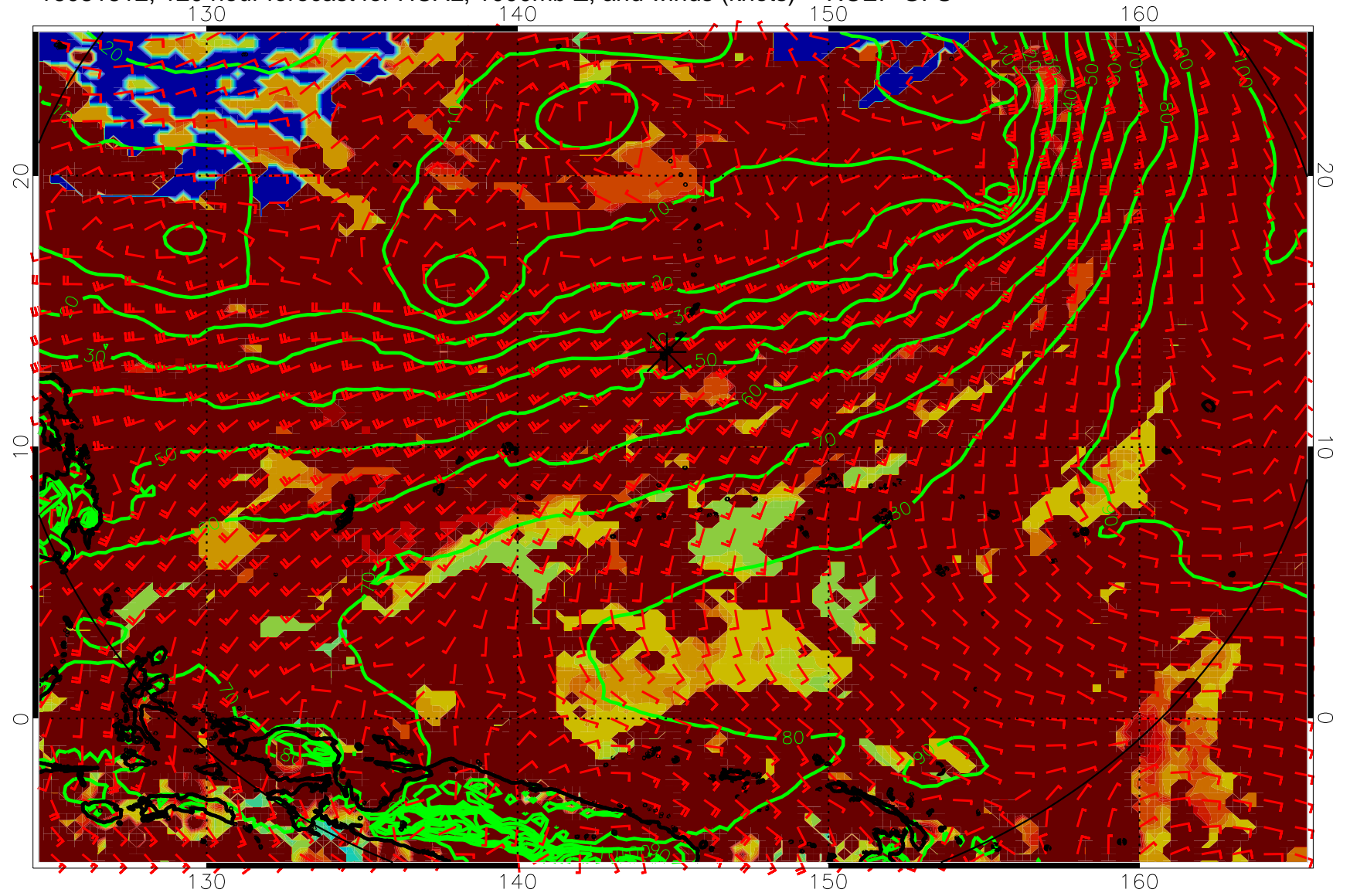
16081812, 120 hour forecast for HCAL, 1000mb Z, and winds (knots) -- NCEP GFS
