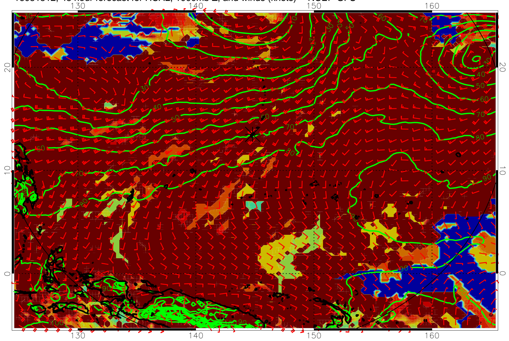
16081512, 48 hour forecast for HCAL, 1000mb Z, and winds (knots) -- NCEP GFS
