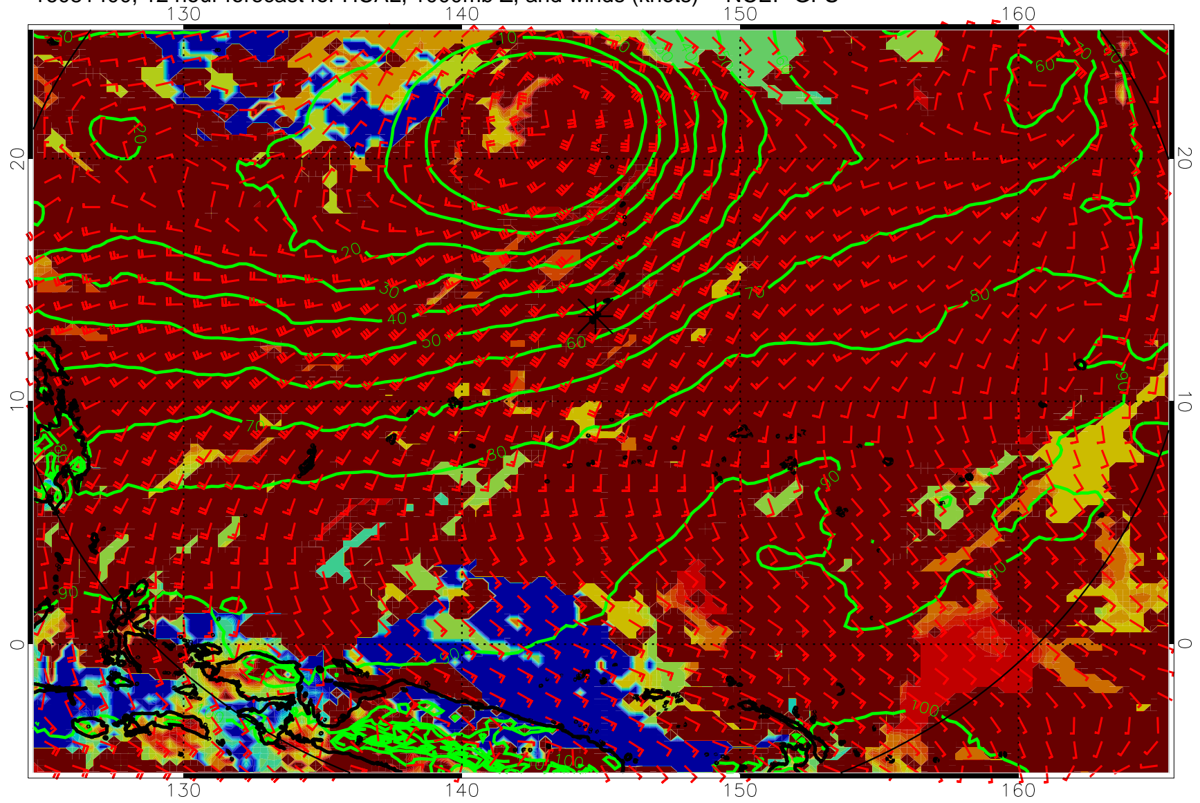
16081400, 12 hour forecast for HCAL, 1000mb Z, and winds (knots) -- NCEP GFS
