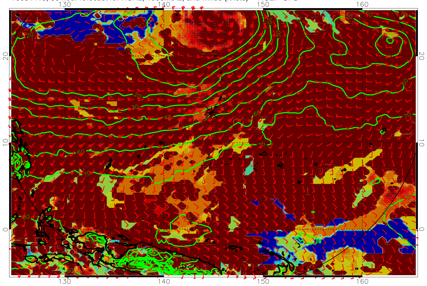
16081418, 30 hour forecast for HCAL, 1000mb Z, and winds (knots) -- NCEP GFS
