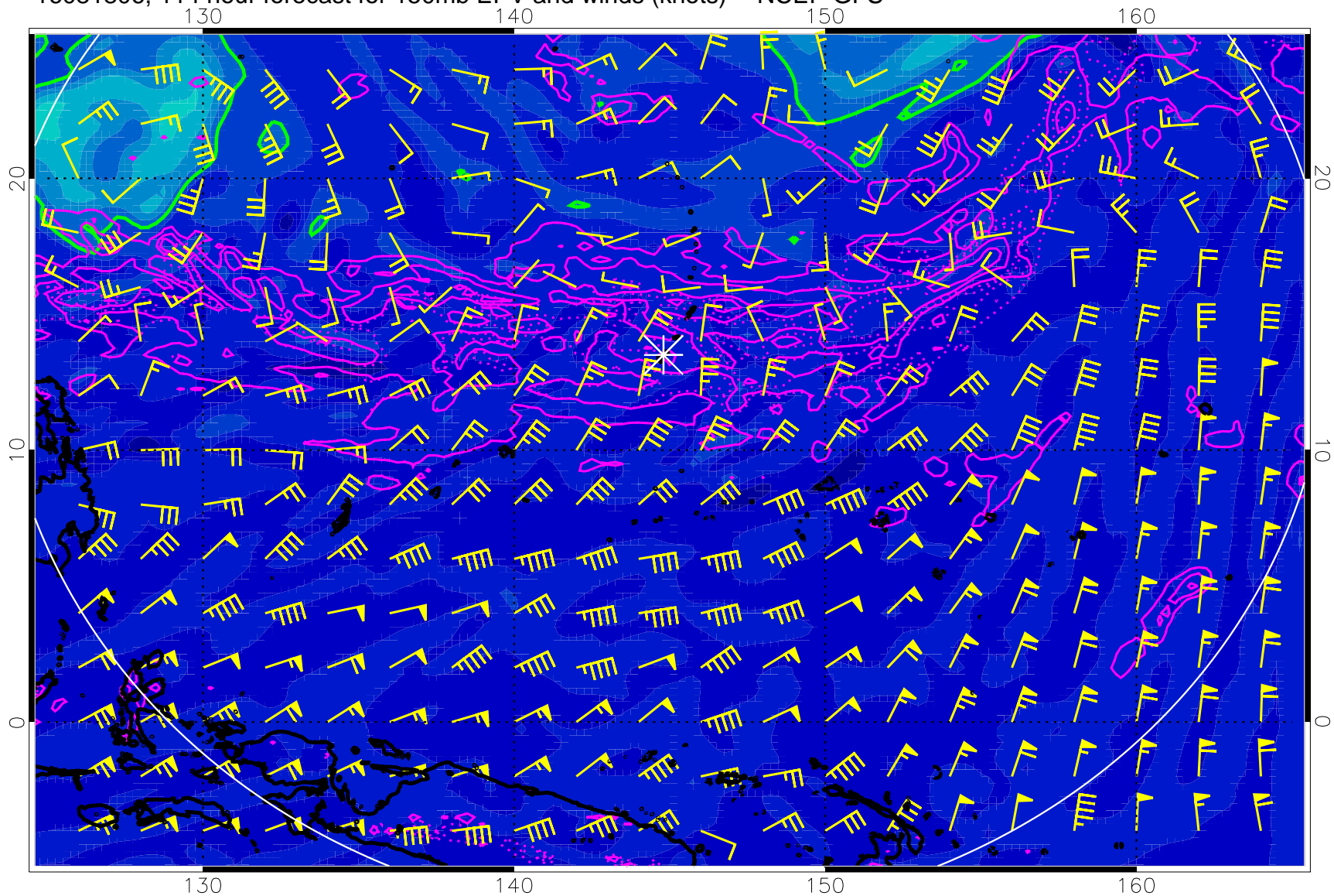
16081806, 114 hour forecast for 150mb EPV and winds (knots) -- NCEP GFS
