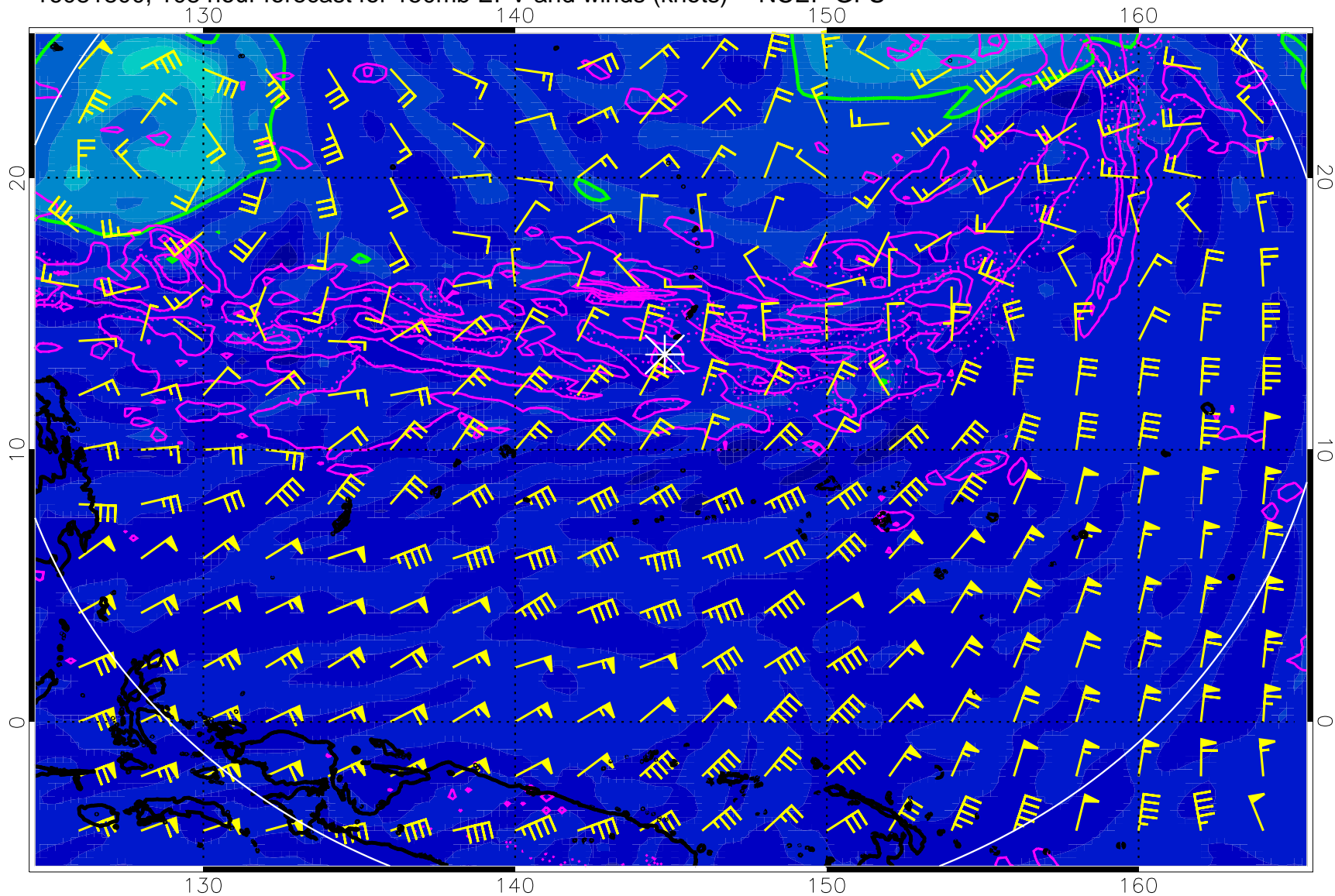
16081800, 108 hour forecast for 150mb EPV and winds (knots) -- NCEP GFS
