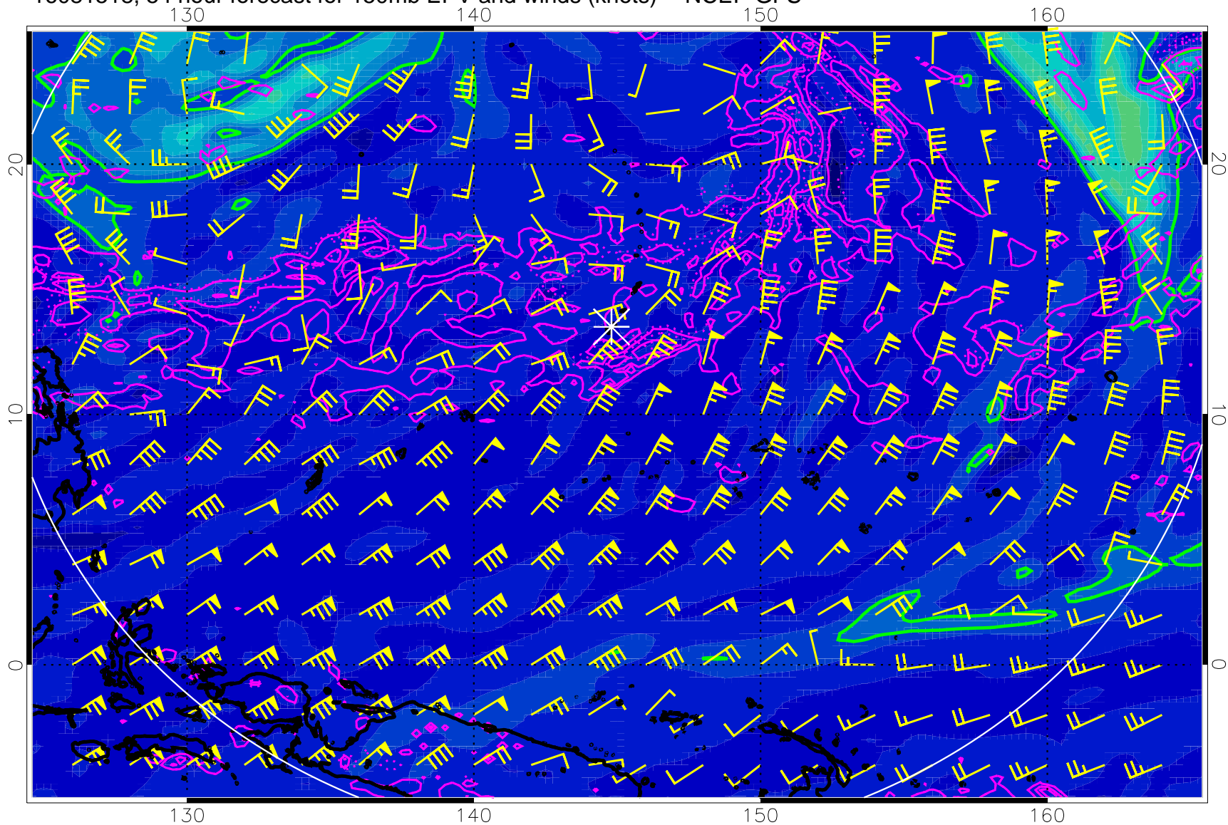
16081518, 54 hour forecast for 150mb EPV and winds (knots) -- NCEP GFS
