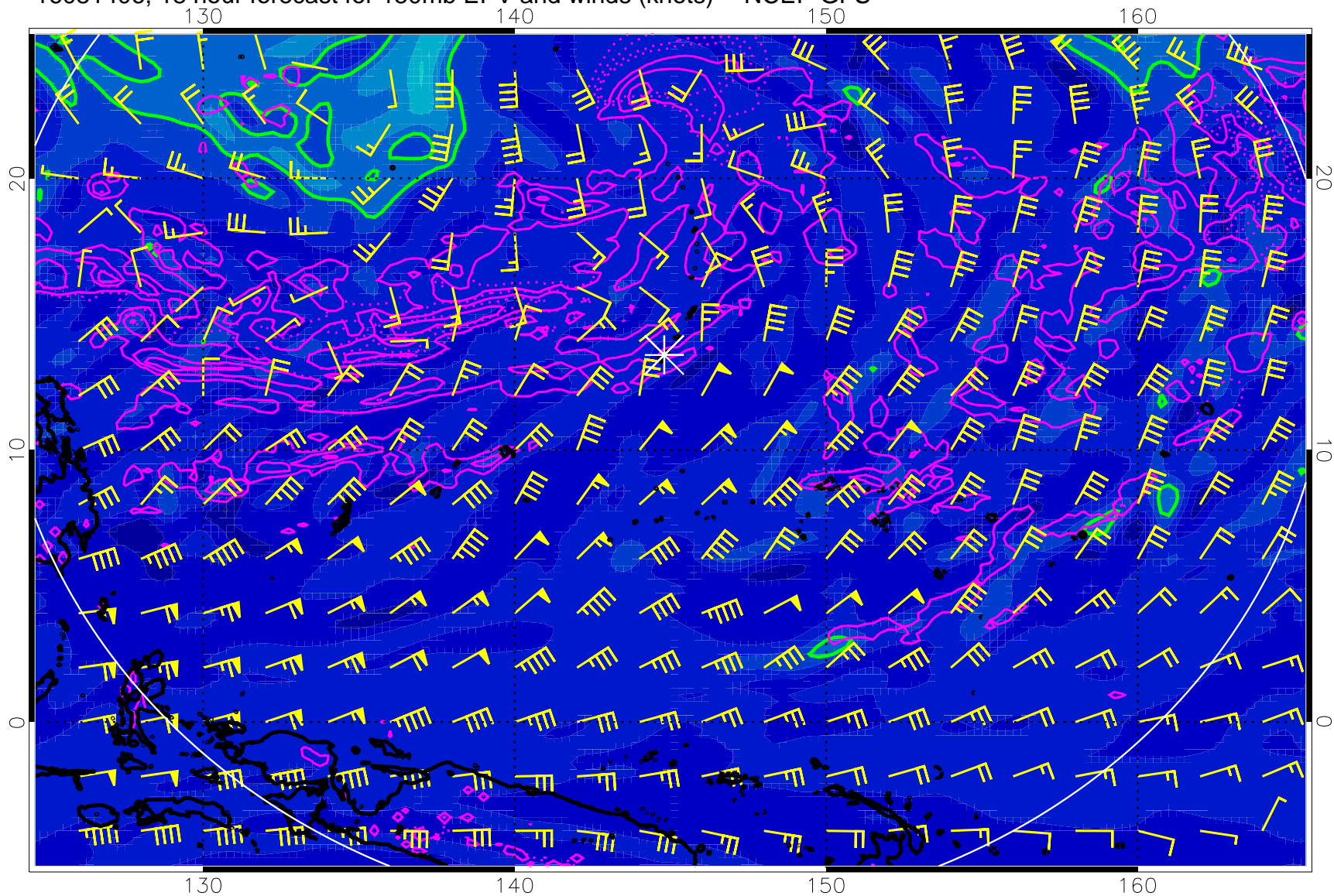
16081406, 18 hour forecast for 150mb EPV and winds (knots) -- NCEP GFS
