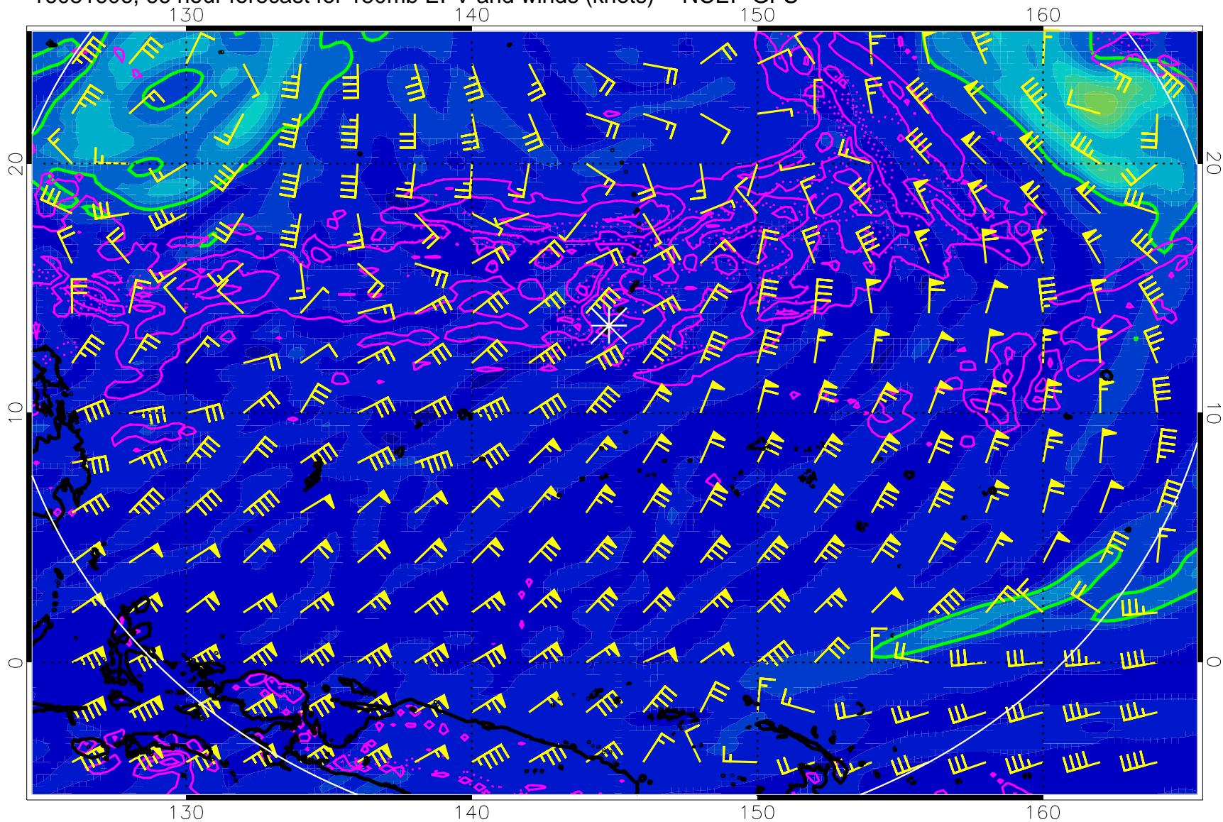
16081606, 66 hour forecast for 150mb EPV and winds (knots) -- NCEP GFS
