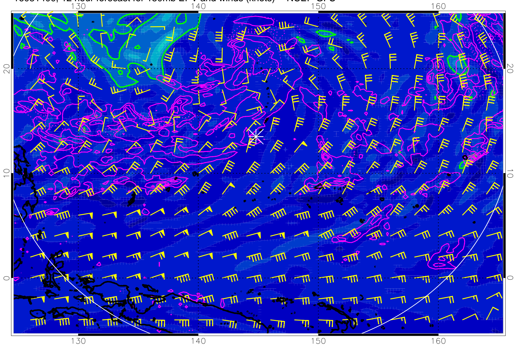
16081400, 12 hour forecast for 150mb EPV and winds (knots) -- NCEP GFS
