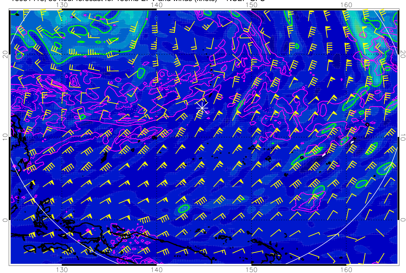
16081418, 30 hour forecast for 150mb EPV and winds (knots) -- NCEP GFS
