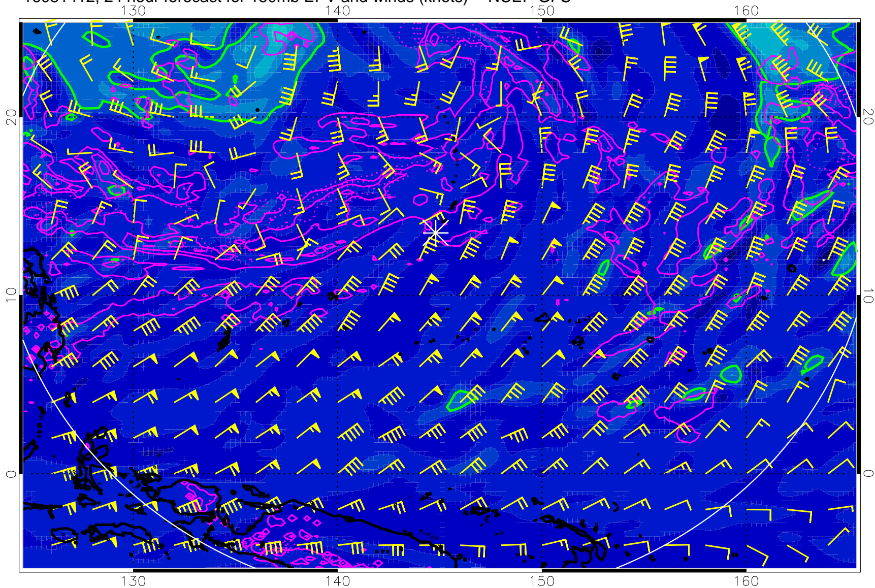
16081412, 24 hour forecast for 150mb EPV and winds (knots) -- NCEP GFS
