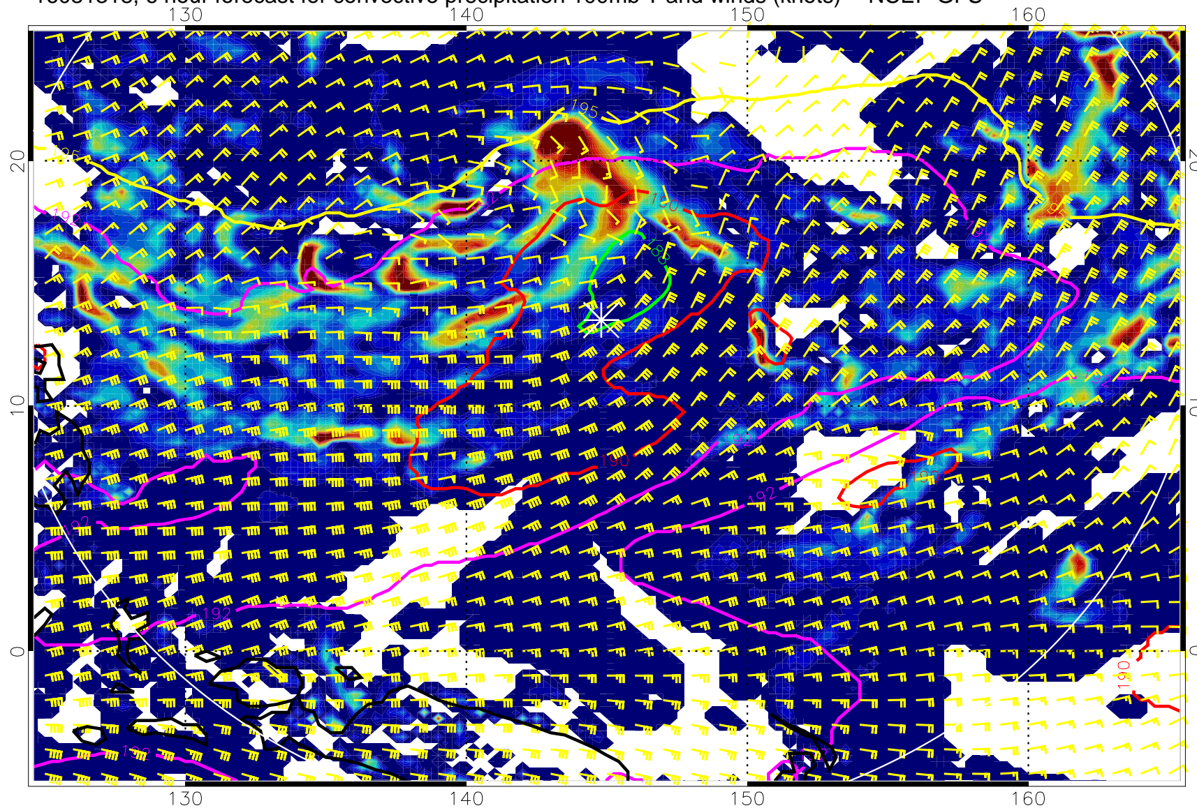
16081318, 6 hour forecast for convective precipitation 100mb T and winds (knots) -- NCEP GFS
