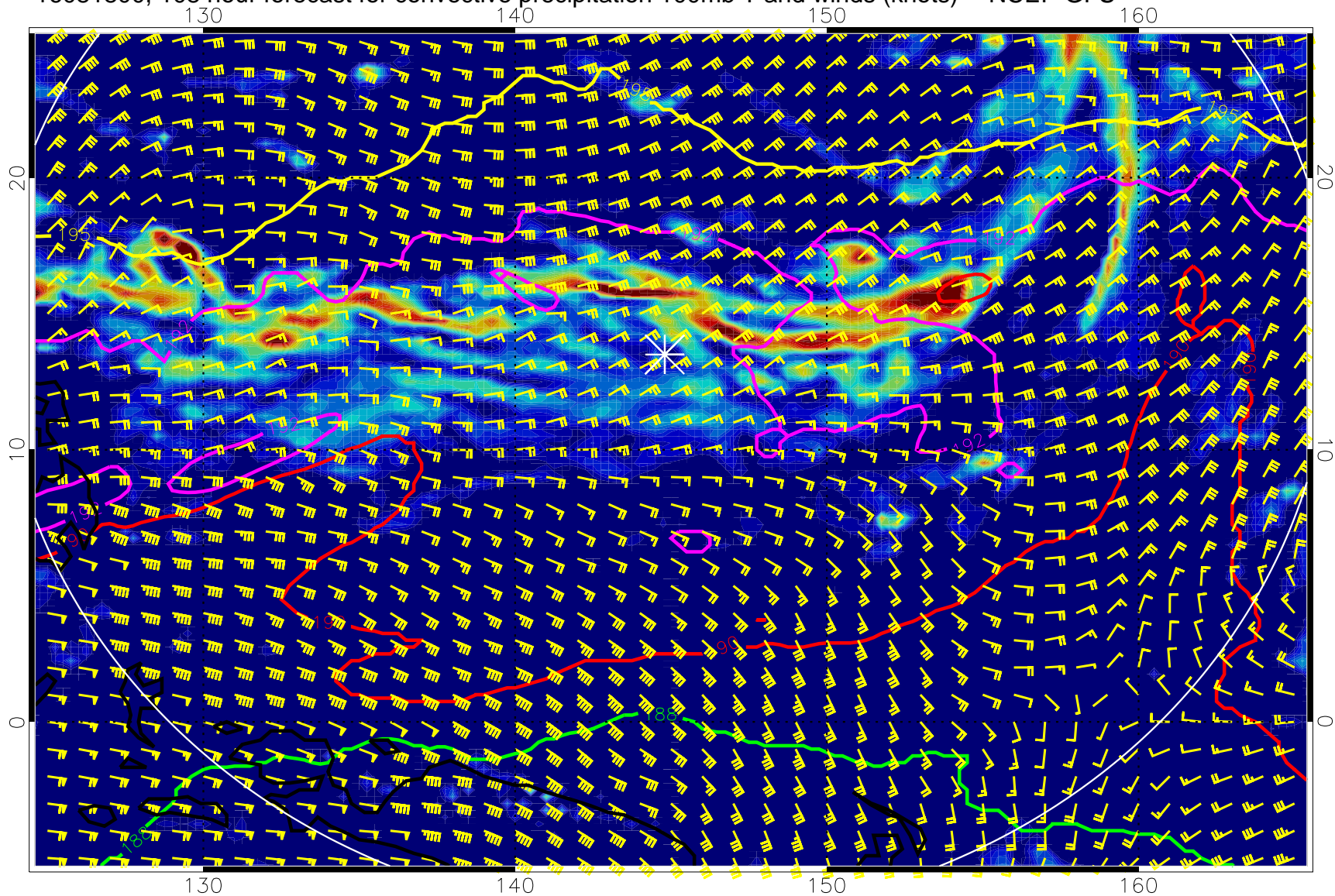
16081800, 108 hour forecast for convective precipitation 100mb T and winds (knots) -- NCEP GFS
