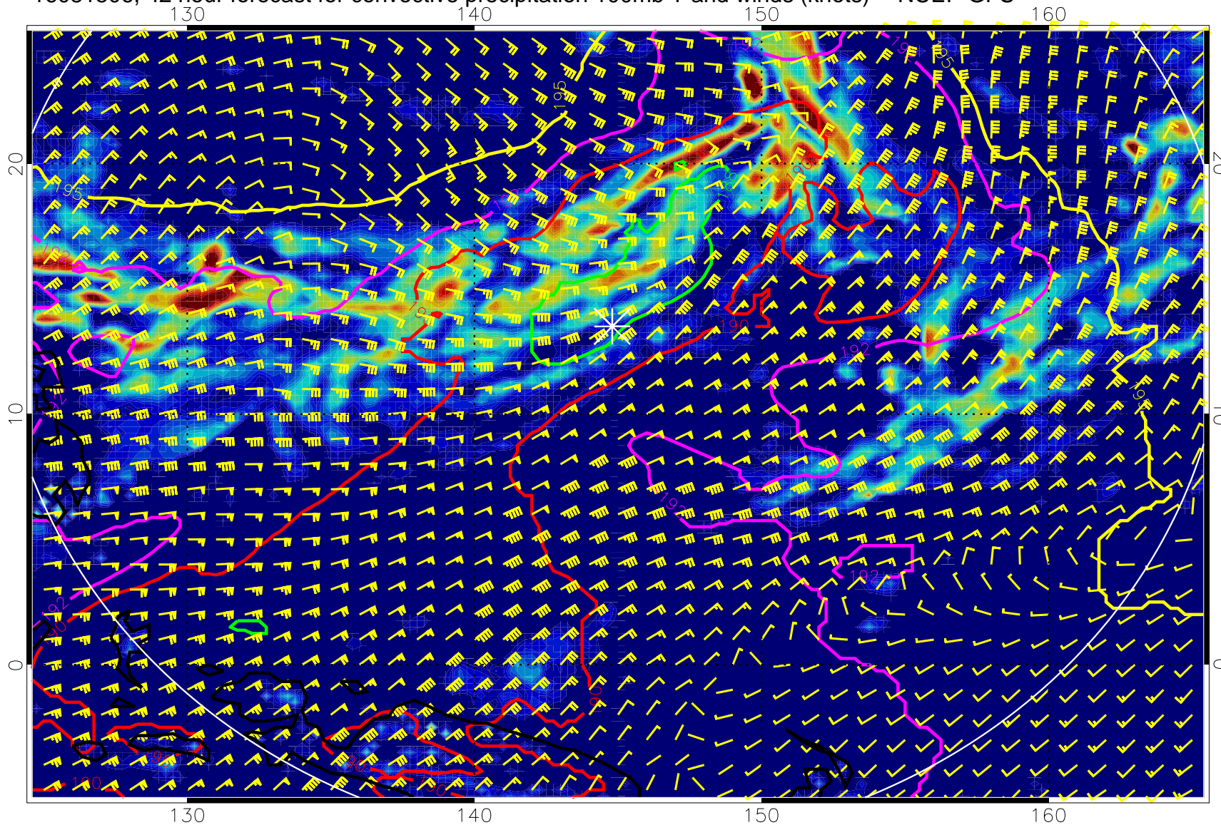
16081506, 42 hour forecast for convective precipitation 100mb T and winds (knots) -- NCEP GFS
