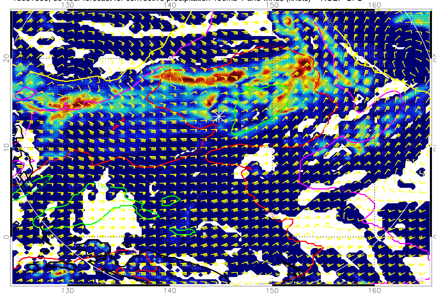
16081606, 66 hour forecast for convective precipitation 100mb T and winds (knots) -- NCEP GFS
