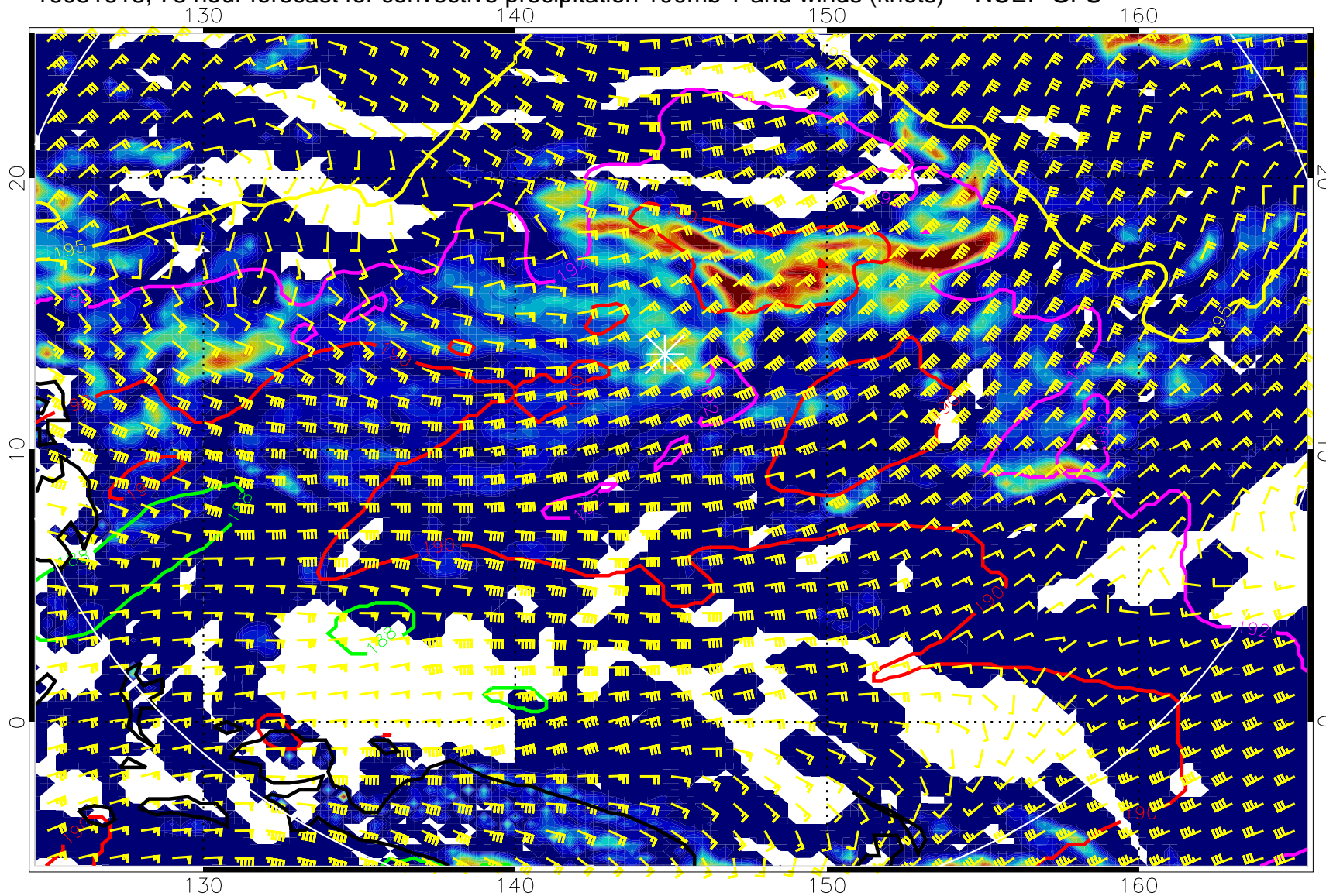
16081618, 78 hour forecast for convective precipitation 100mb T and winds (knots) -- NCEP GFS
