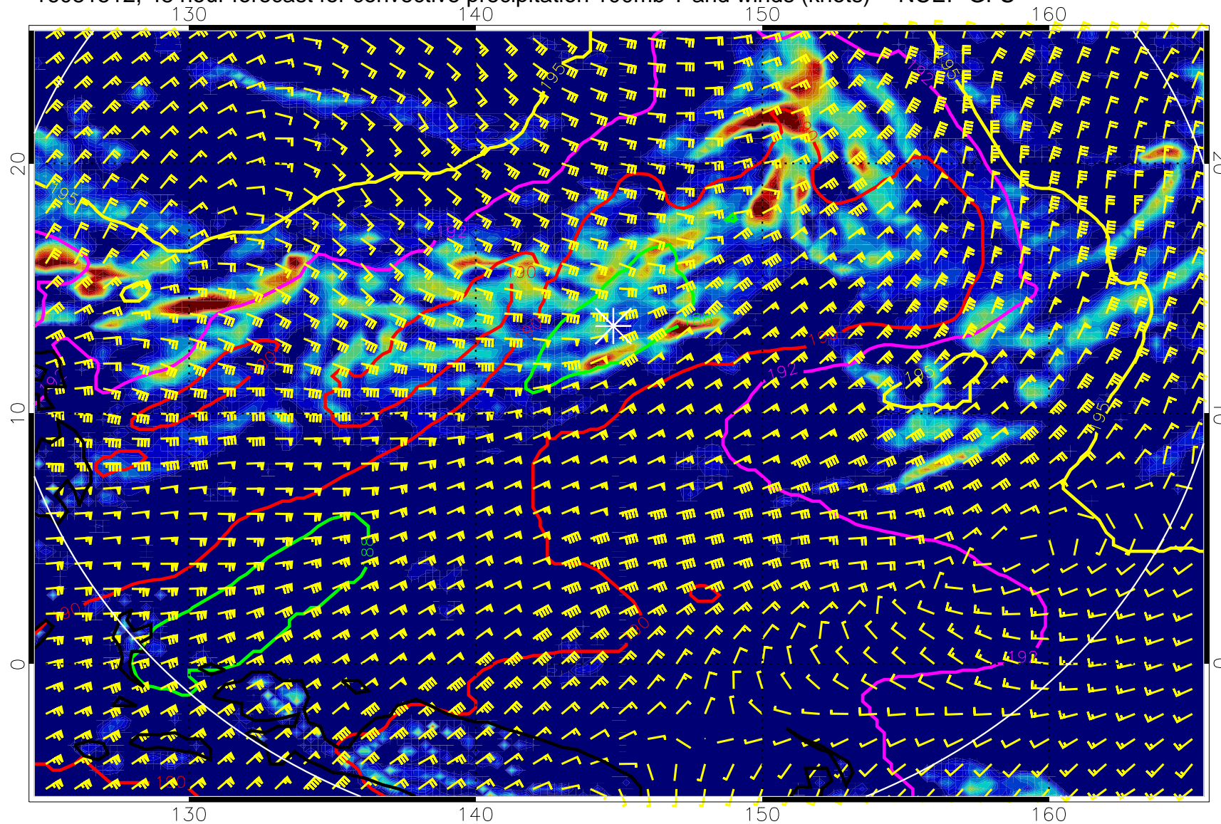
16081512, 48 hour forecast for convective precipitation 100mb T and winds (knots) -- NCEP GFS
