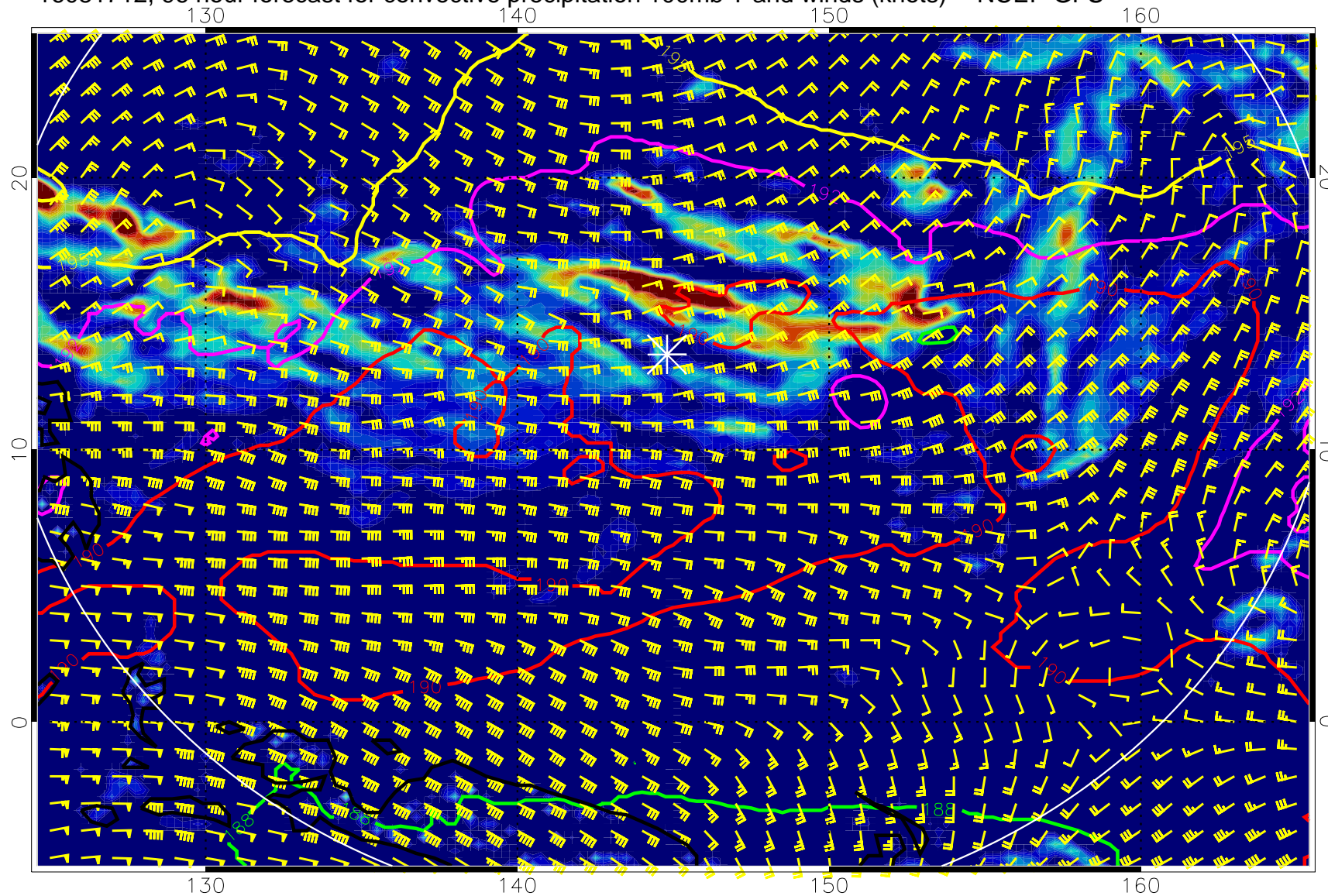
16081712, 96 hour forecast for convective precipitation 100mb T and winds (knots) -- NCEP GFS
