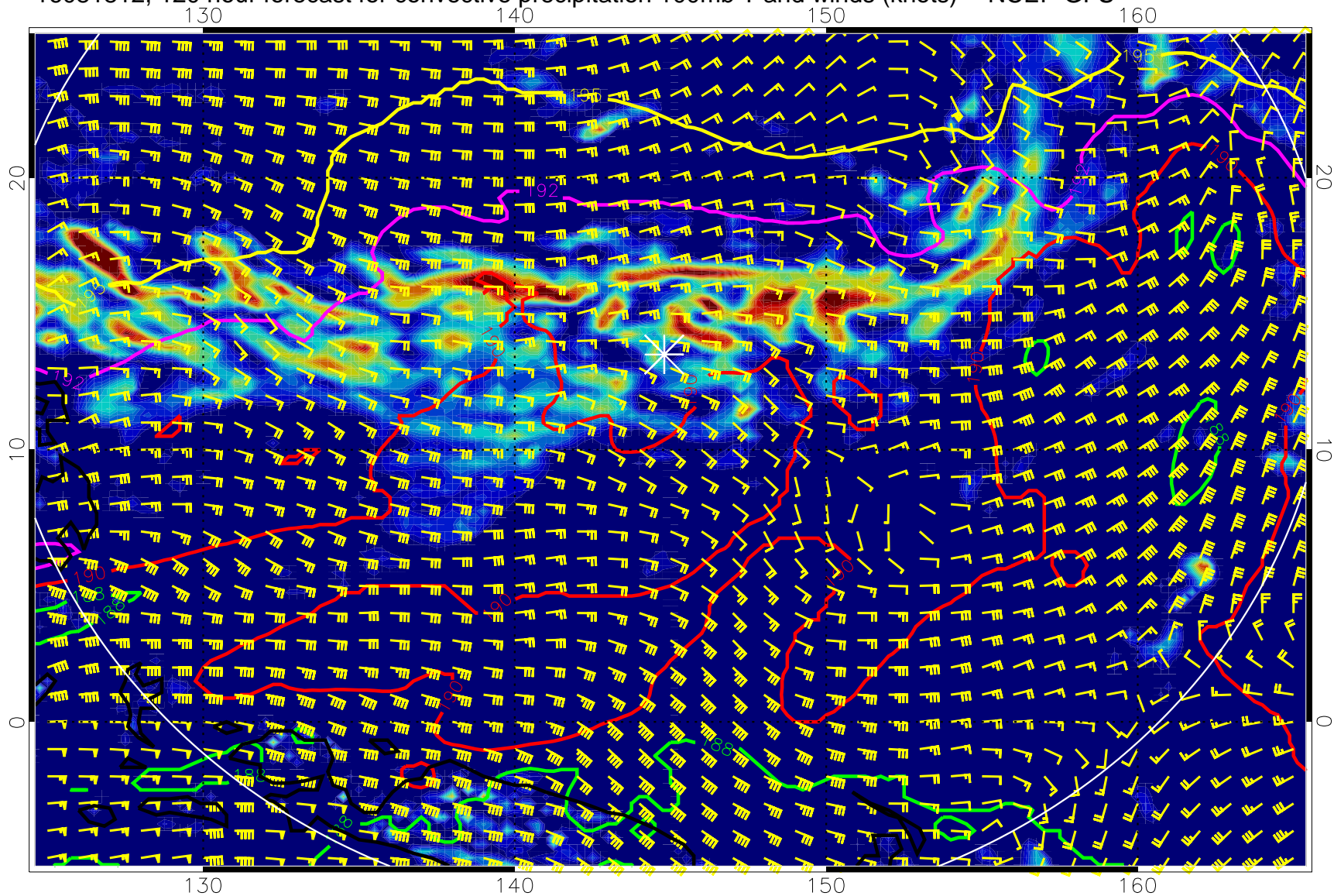
16081812, 120 hour forecast for convective precipitation 100mb T and winds (knots) -- NCEP GFS
