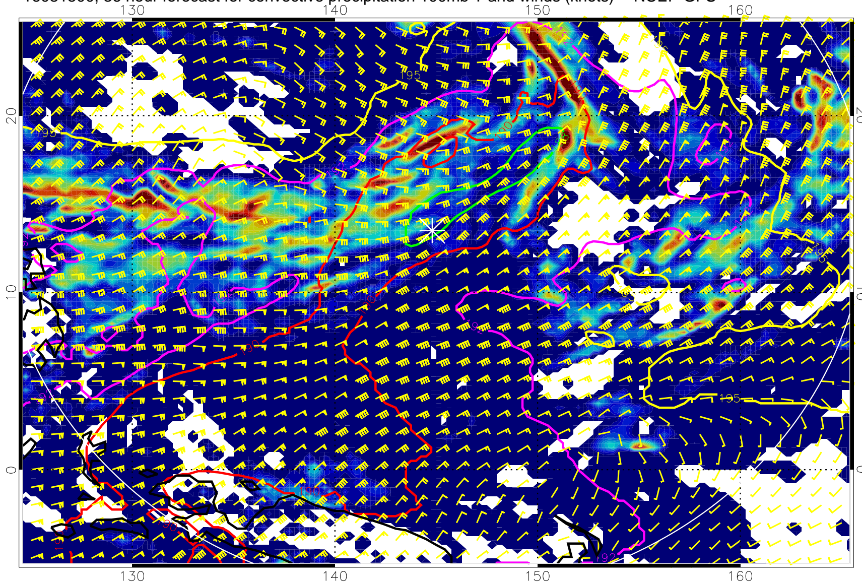
16081500, 36 hour forecast for convective precipitation 100mb T and winds (knots) -- NCEP GFS
