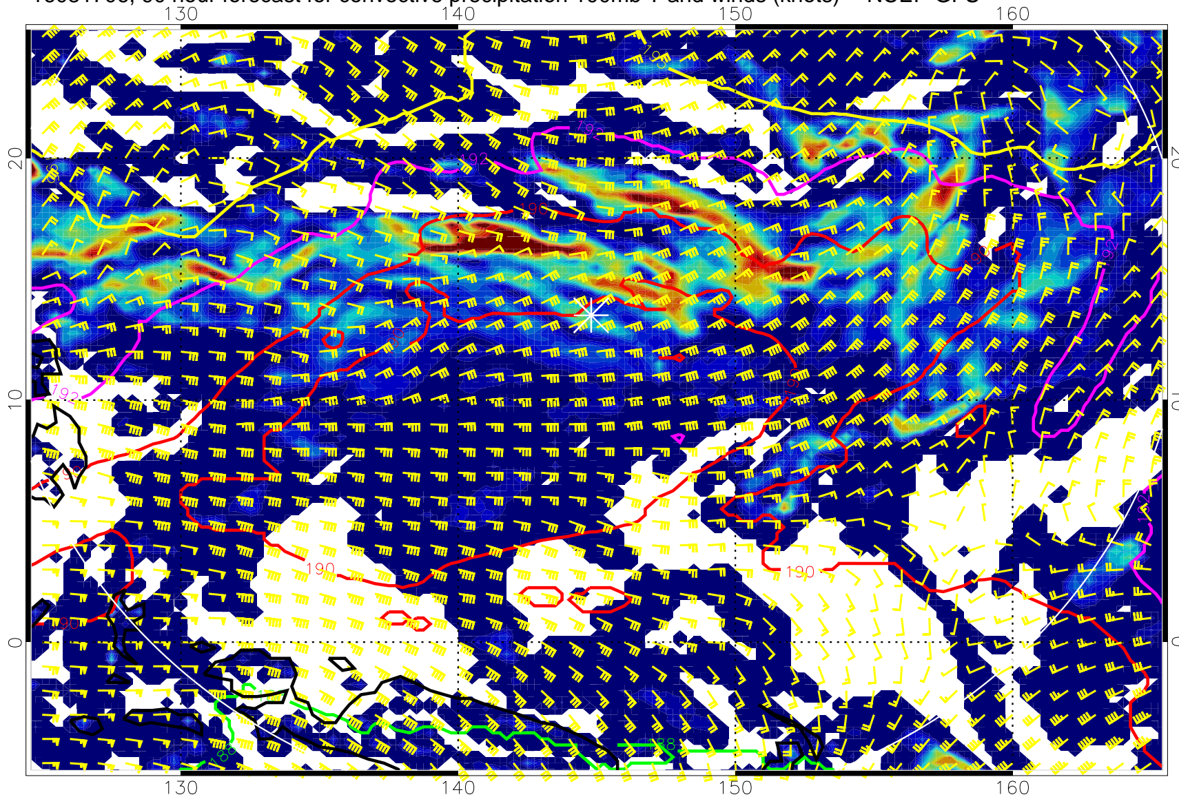
16081706, 90 hour forecast for convective precipitation 100mb T and winds (knots) -- NCEP GFS
