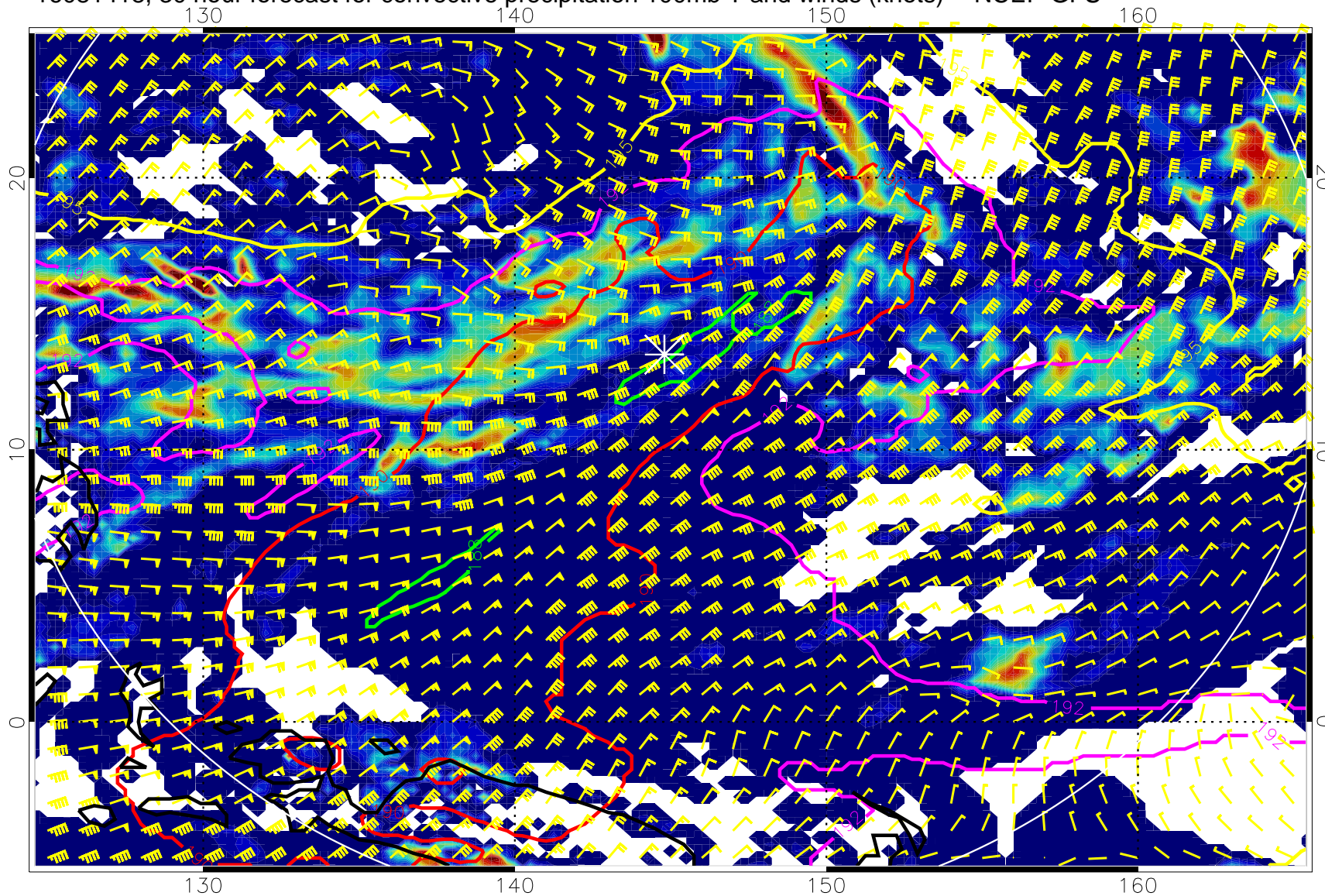
16081418, 30 hour forecast for convective precipitation 100mb T and winds (knots) -- NCEP GFS
