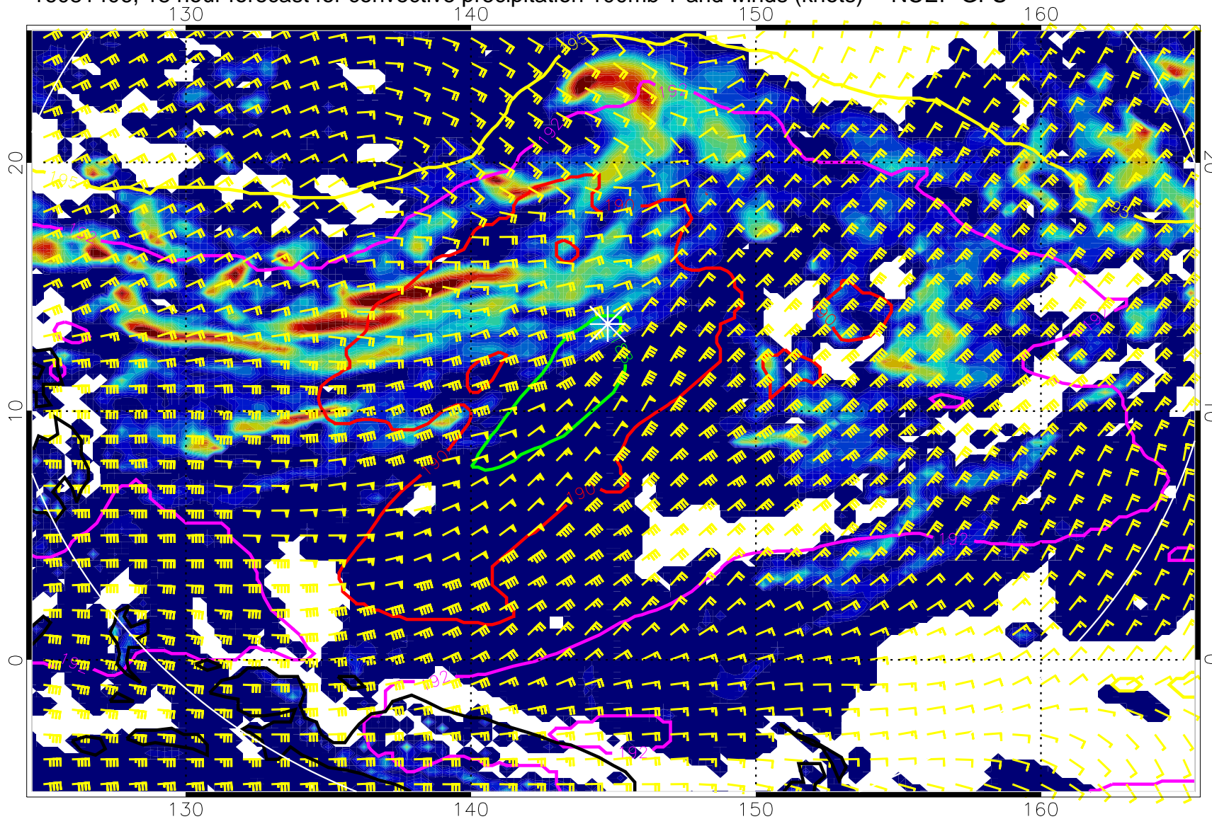
16081406, 18 hour forecast for convective precipitation 100mb T and winds (knots) -- NCEP GFS
