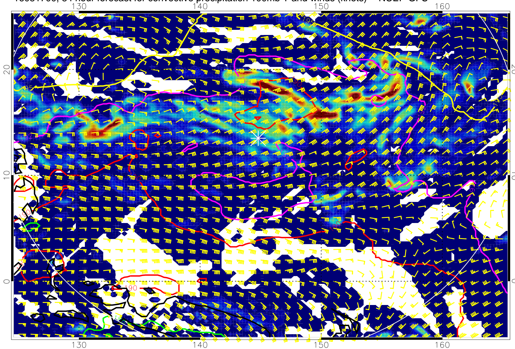
16081700, 84 hour forecast for convective precipitation 100mb T and winds (knots) -- NCEP GFS
