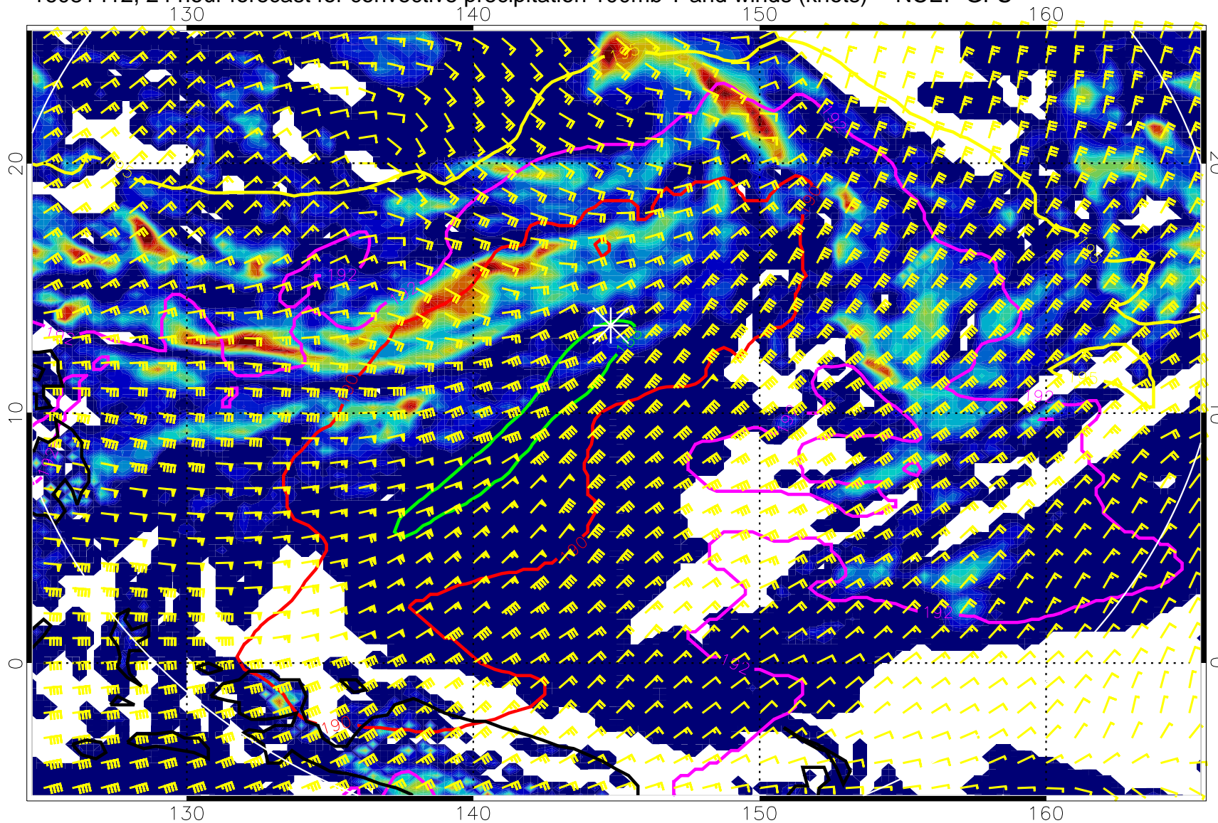
16081412, 24 hour forecast for convective precipitation 100mb T and winds (knots) -- NCEP GFS
