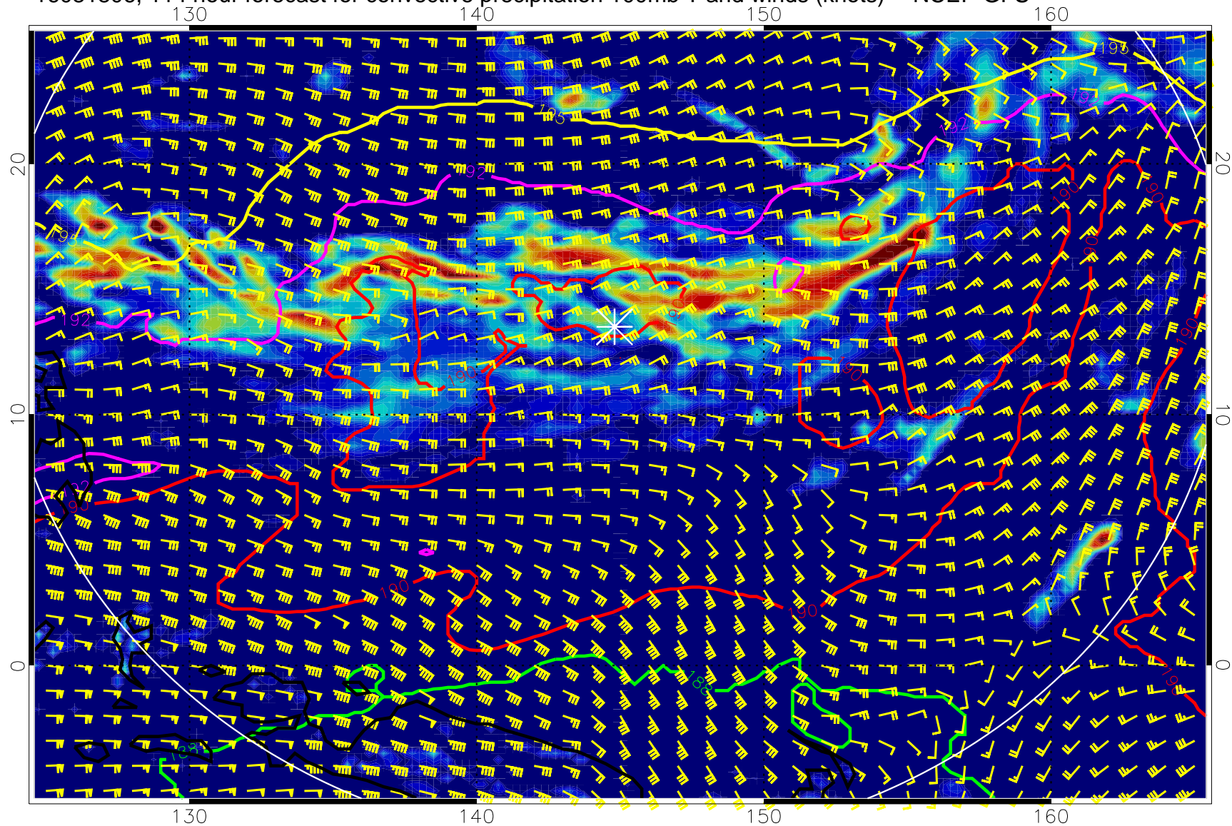
16081806, 114 hour forecast for convective precipitation 100mb T and winds (knots) -- NCEP GFS
