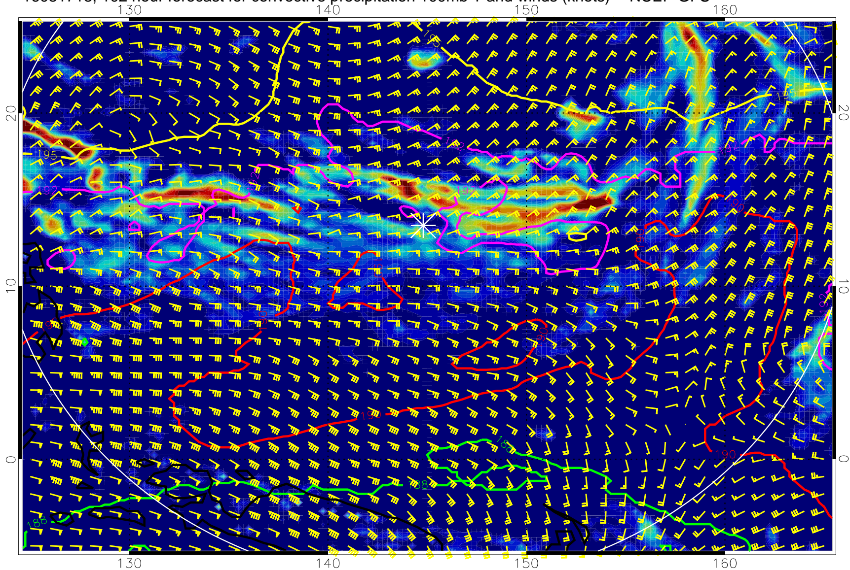
16081718, 102 hour forecast for convective precipitation 100mb T and winds (knots) -- NCEP GFS
