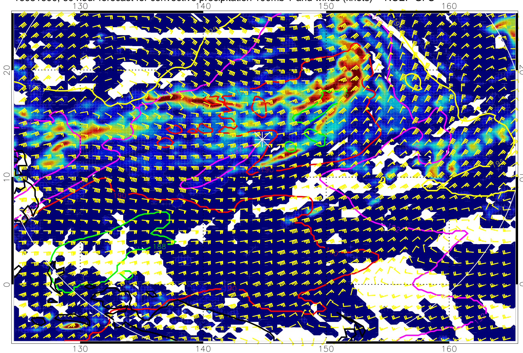
16081600, 60 hour forecast for convective precipitation 100mb T and winds (knots) -- NCEP GFS
