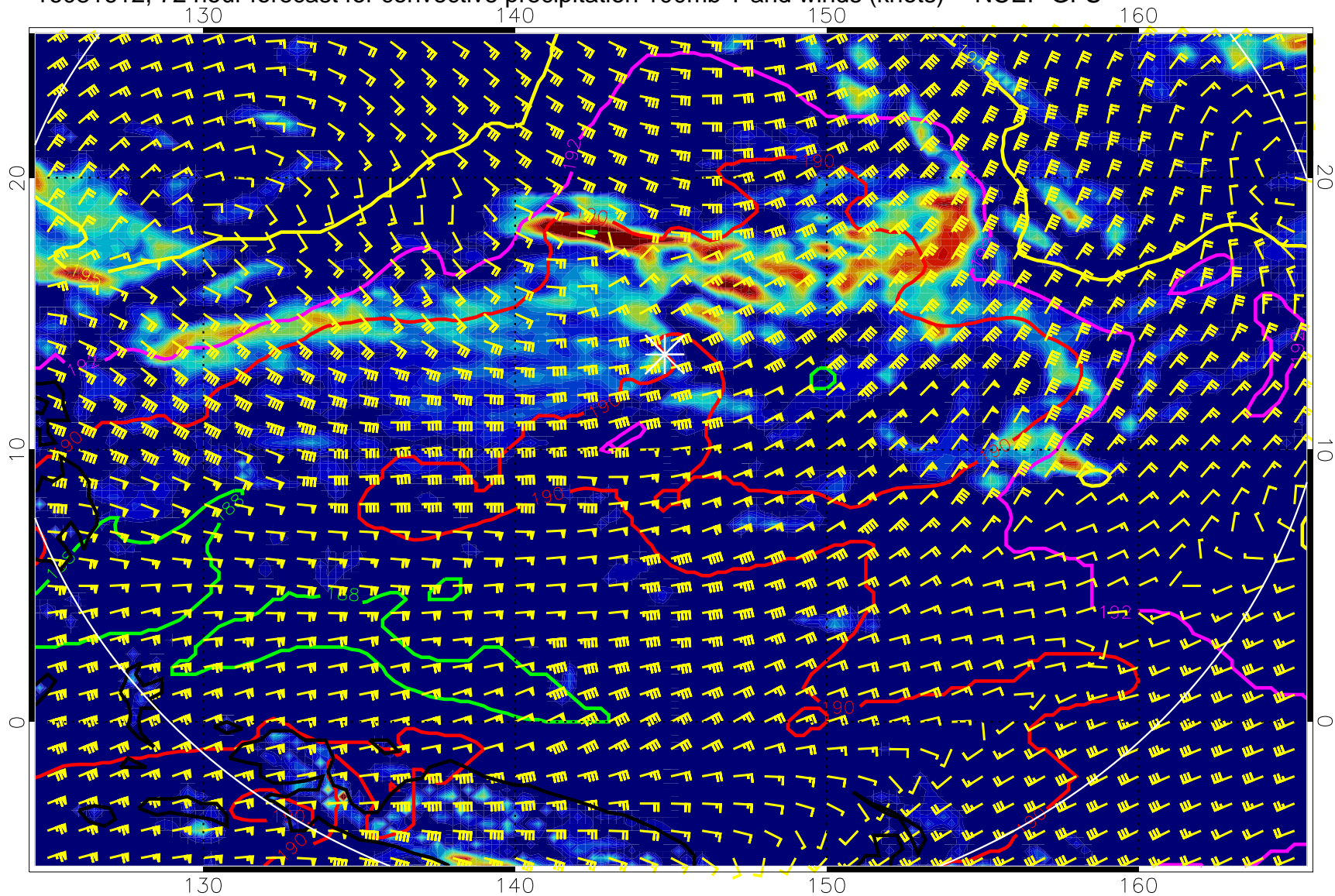
16081612, 72 hour forecast for convective precipitation 100mb T and winds (knots) -- NCEP GFS
