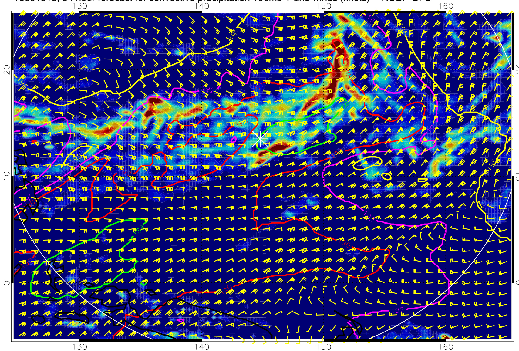
16081518, 54 hour forecast for convective precipitation 100mb T and winds (knots) -- NCEP GFS
