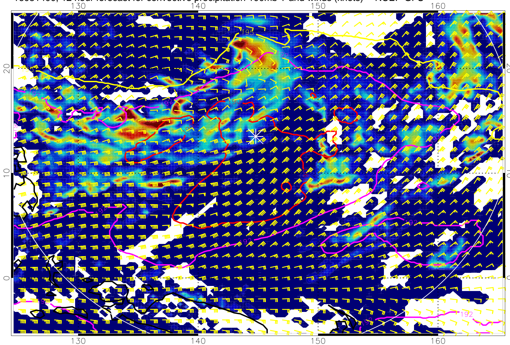
16081400, 12 hour forecast for convective precipitation 100mb T and winds (knots) -- NCEP GFS
