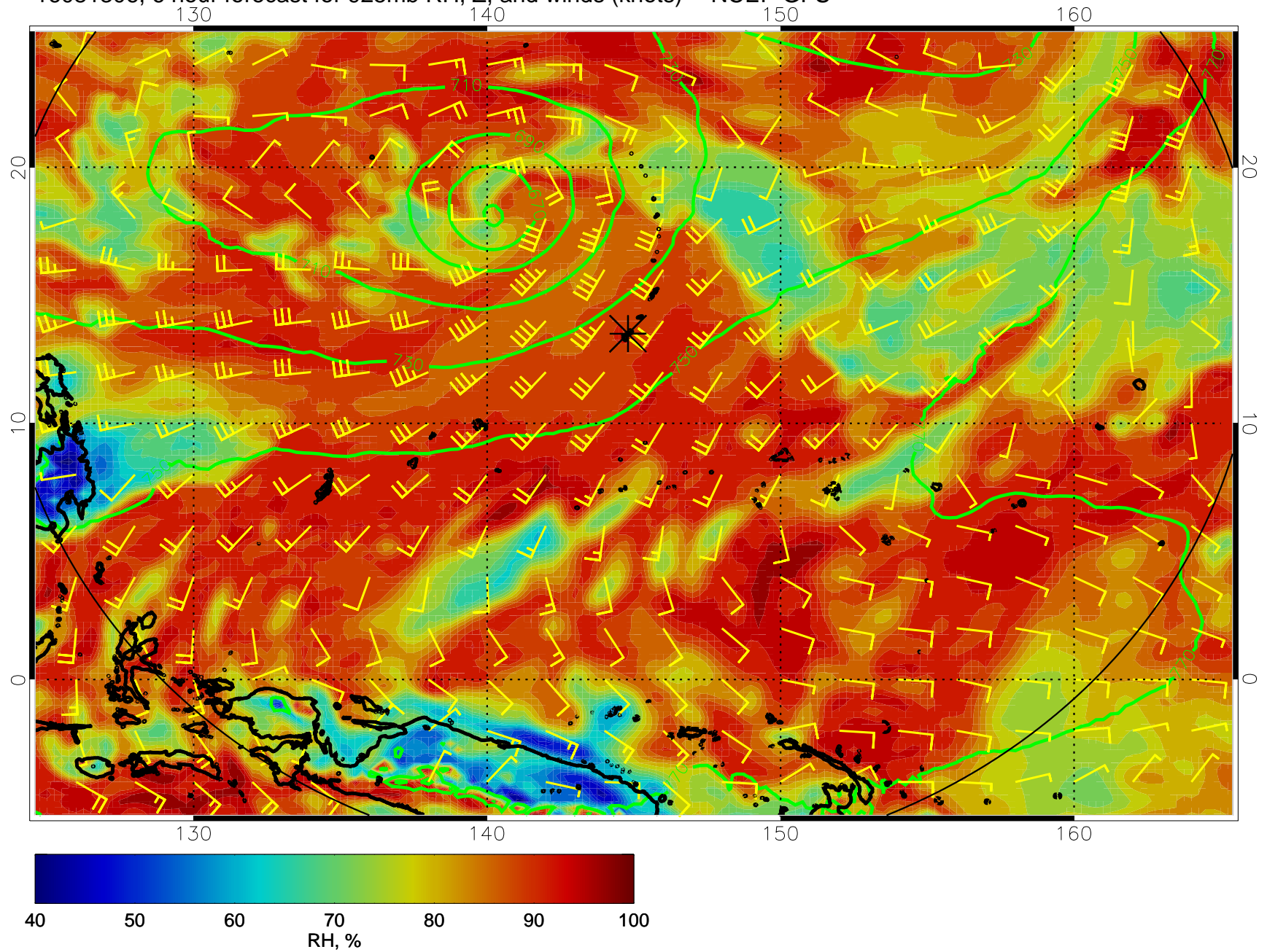
16081306, 6 hour forecast for 925mb RH, Z, and winds (knots) -- NCEP GFS
