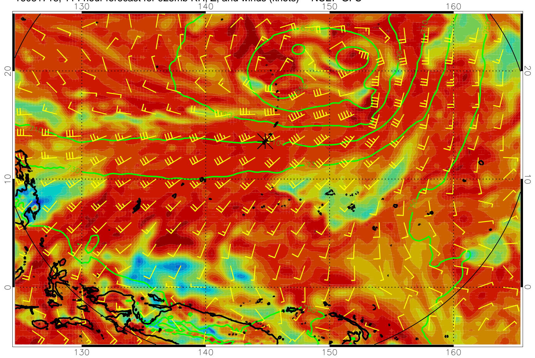
16081718, 114 hour forecast for 925mb RH, Z, and winds (knots) -- NCEP GFS
