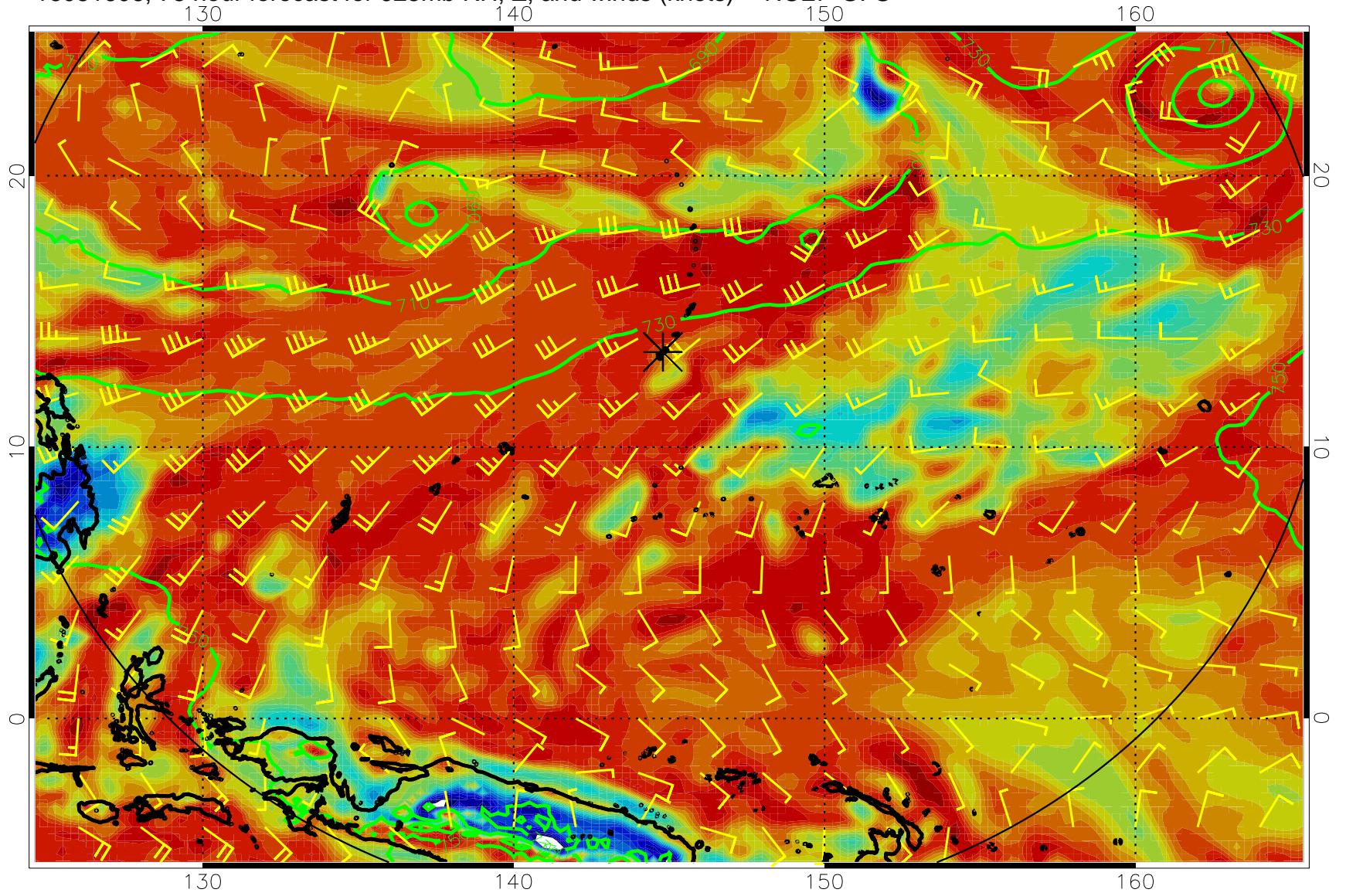
16081606, 78 hour forecast for 925mb RH, Z, and winds (knots) -- NCEP GFS
