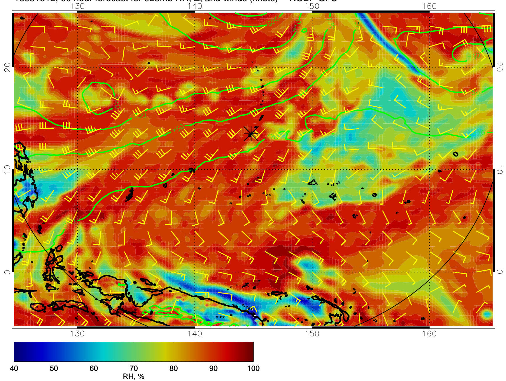
16081512, 60 hour forecast for 925mb RH, Z, and winds (knots) -- NCEP GFS
