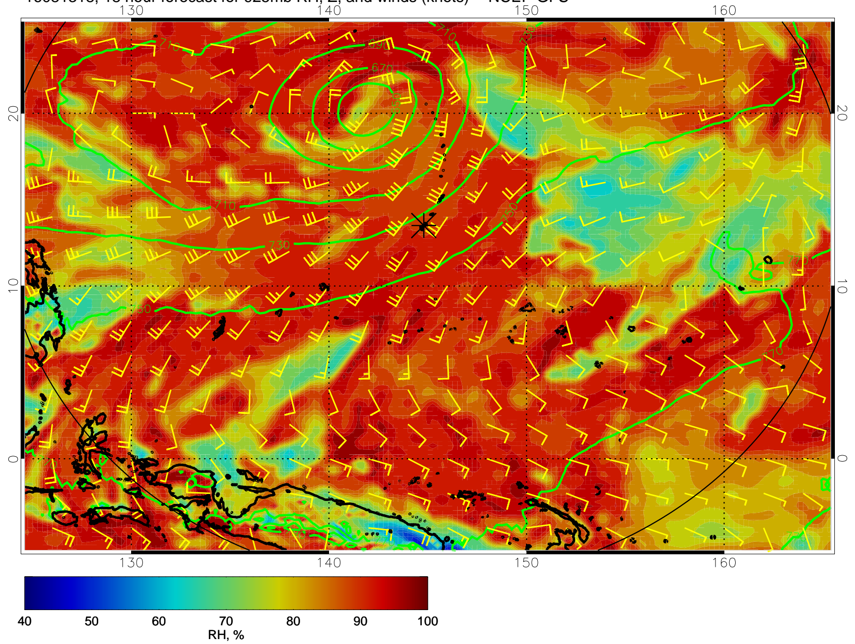
16081318, 18 hour forecast for 925mb RH, Z, and winds (knots) -- NCEP GFS
