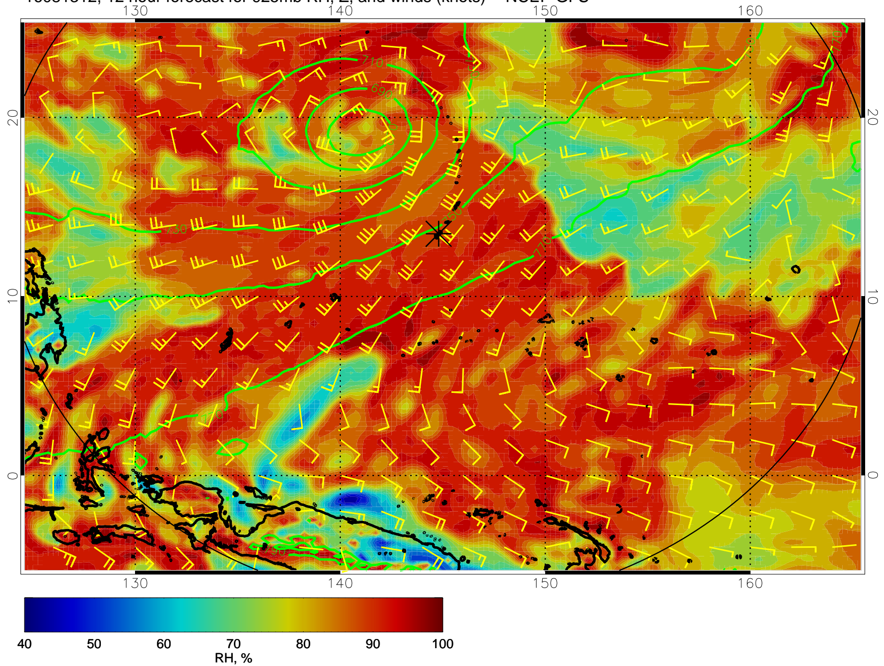
16081312, 12 hour forecast for 925mb RH, Z, and winds (knots) -- NCEP GFS
