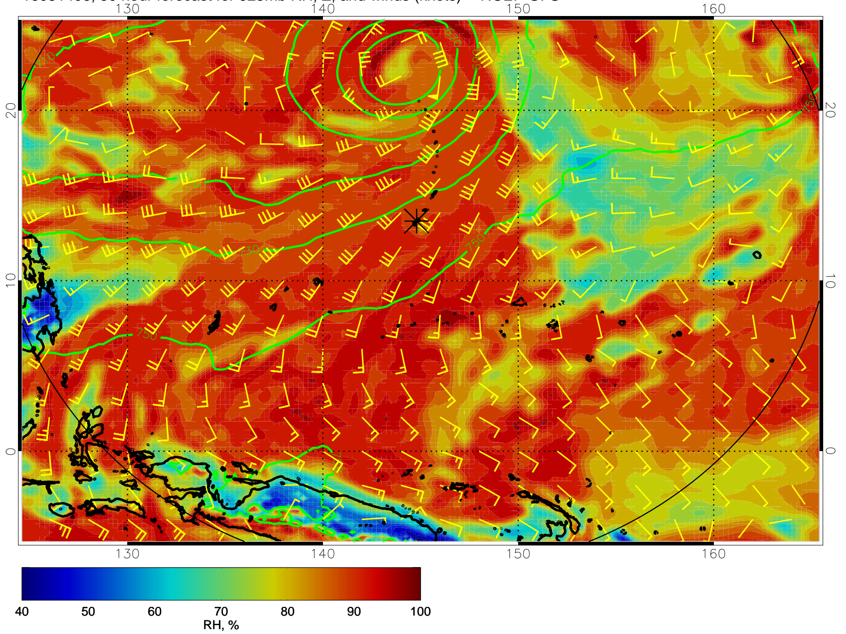
16081406, 30 hour forecast for 925mb RH, Z, and winds (knots) -- NCEP GFS
