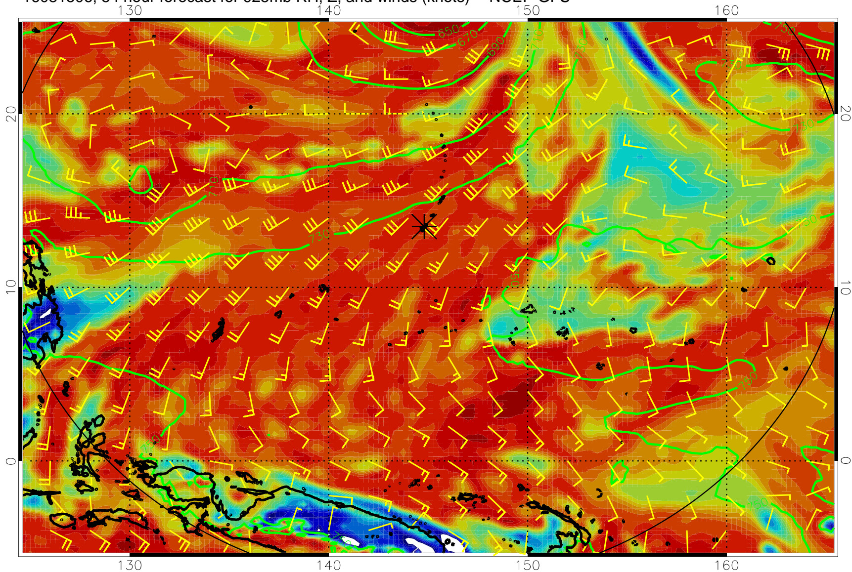
16081506, 54 hour forecast for 925mb RH, Z, and winds (knots) -- NCEP GFS
