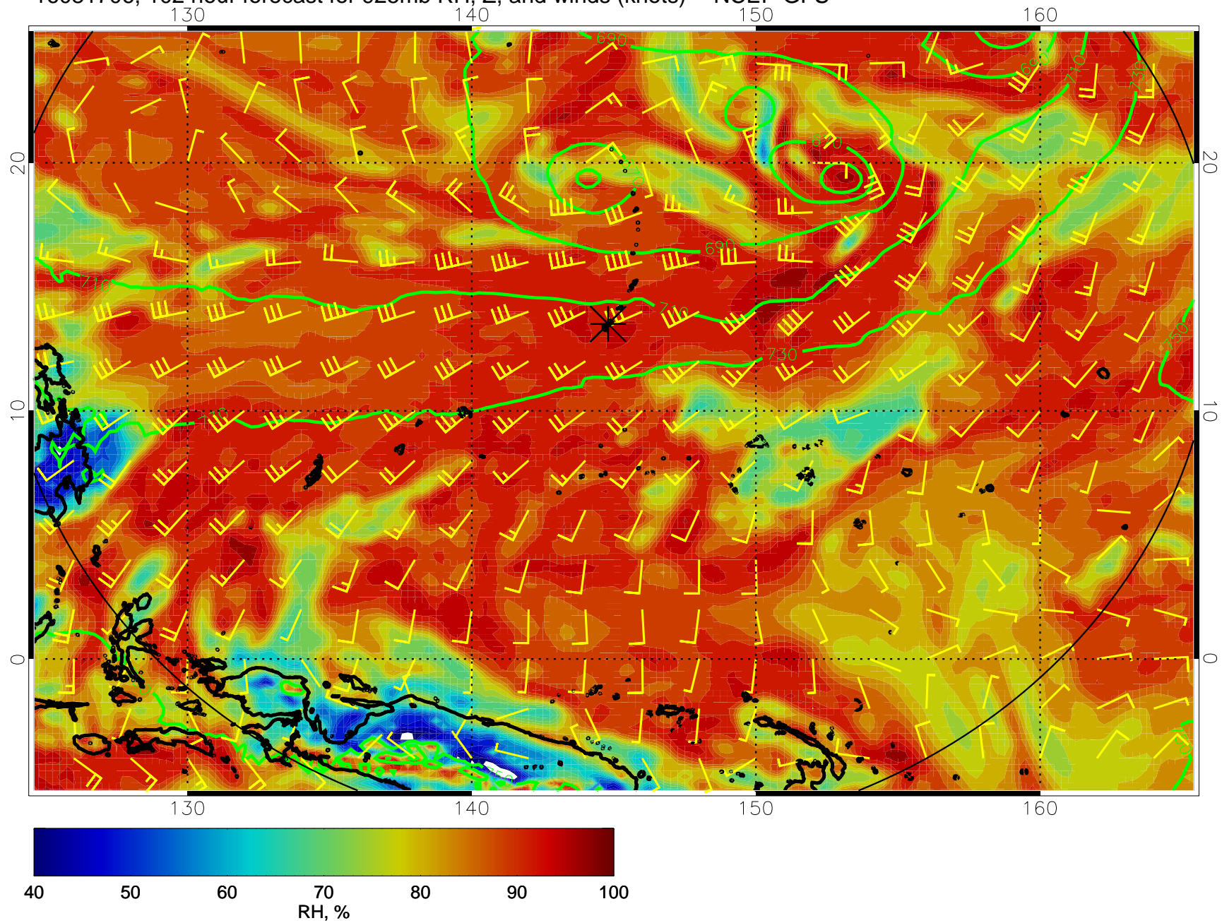
16081706, 102 hour forecast for 925mb RH, Z, and winds (knots) -- NCEP GFS
