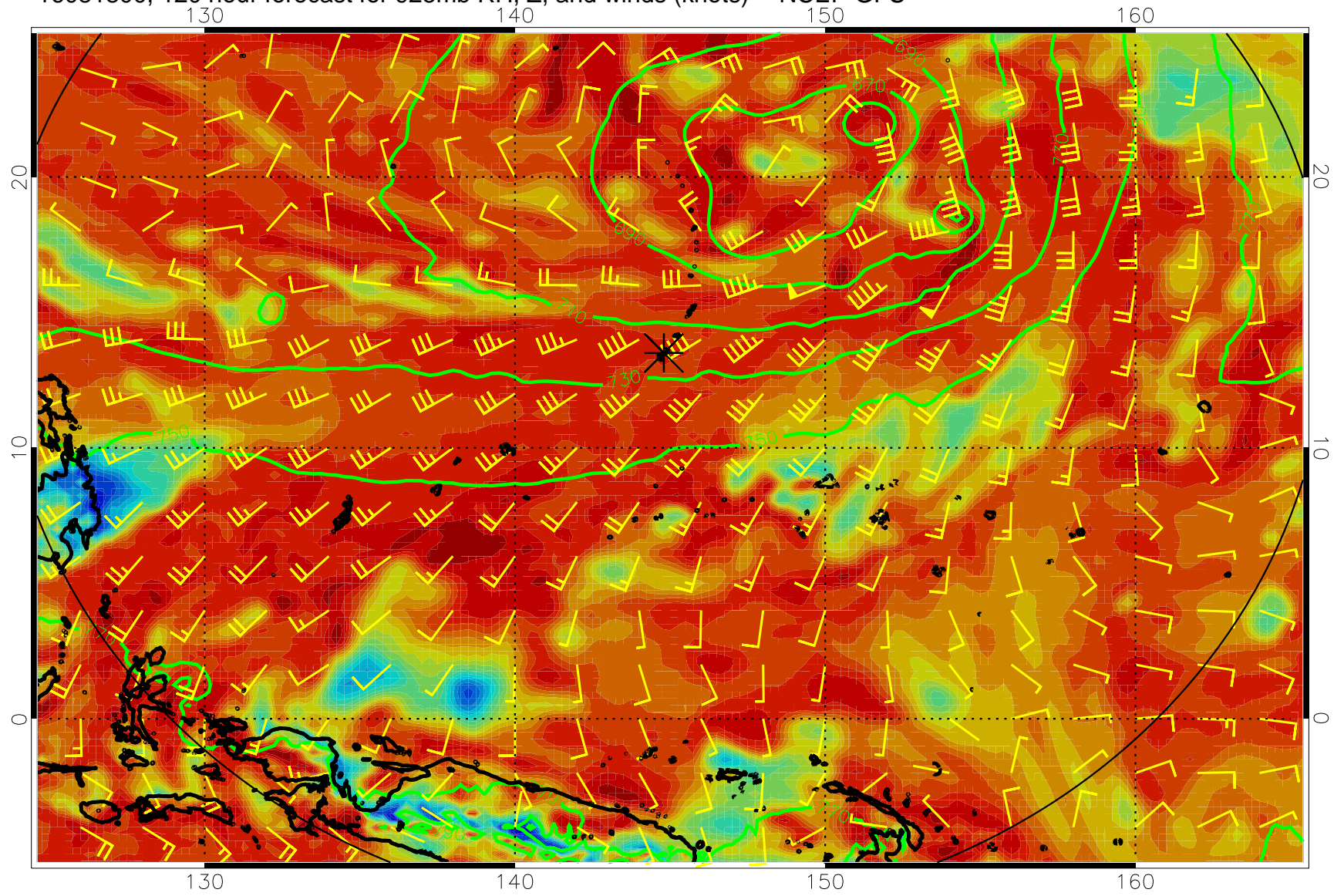
16081800, 120 hour forecast for 925mb RH, Z, and winds (knots) -- NCEP GFS
