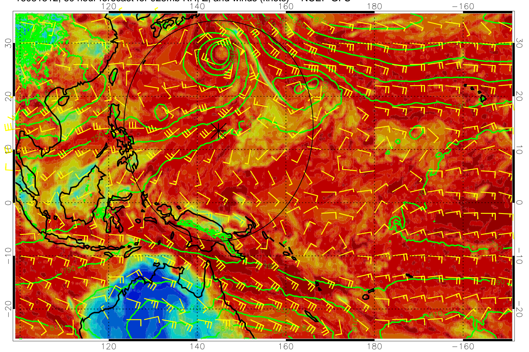
16081512, 60 hour forecast for 925mb RH, Z, and winds (knots) -- NCEP GFS
