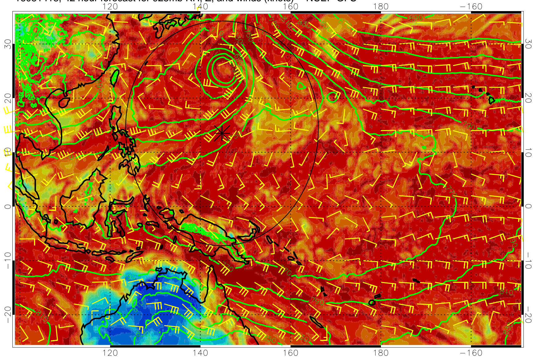
16081418, 42 hour forecast for 925mb RH, Z, and winds (knots) -- NCEP GFS
