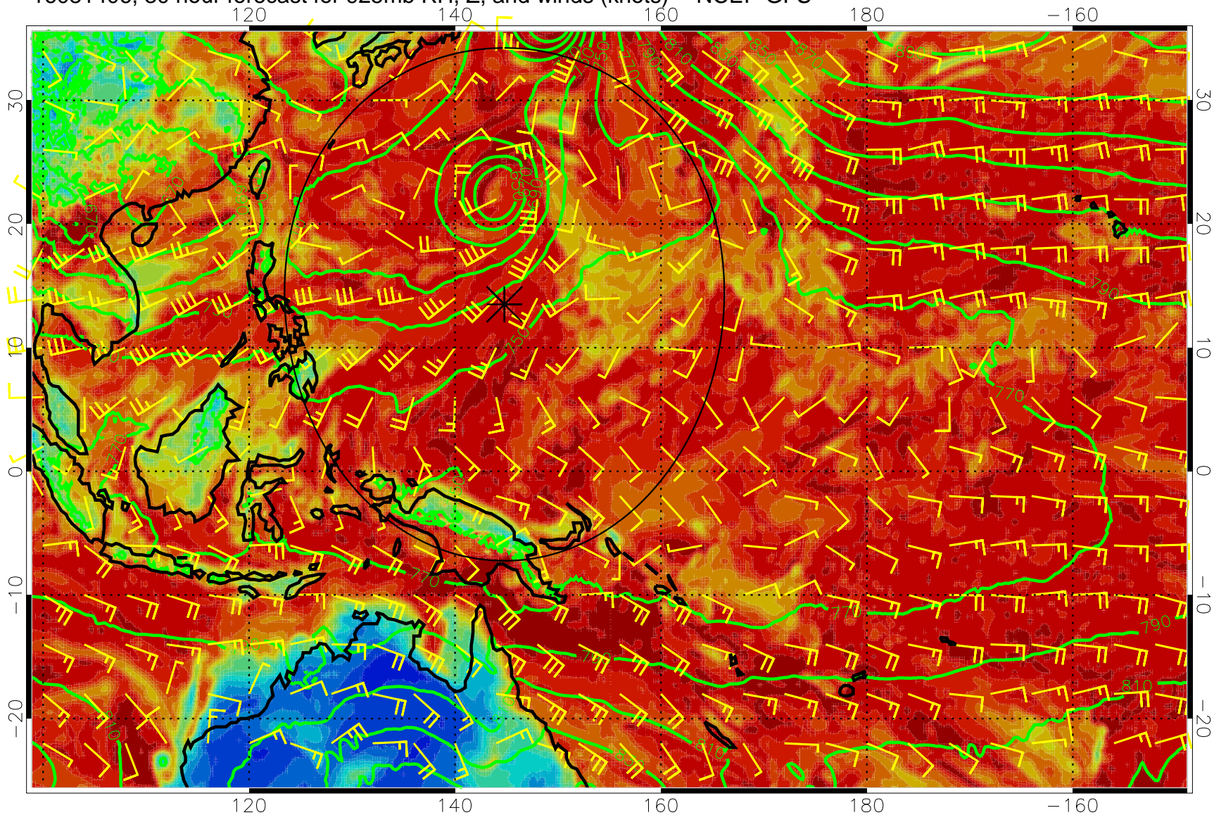
16081406, 30 hour forecast for 925mb RH, Z, and winds (knots) -- NCEP GFS
