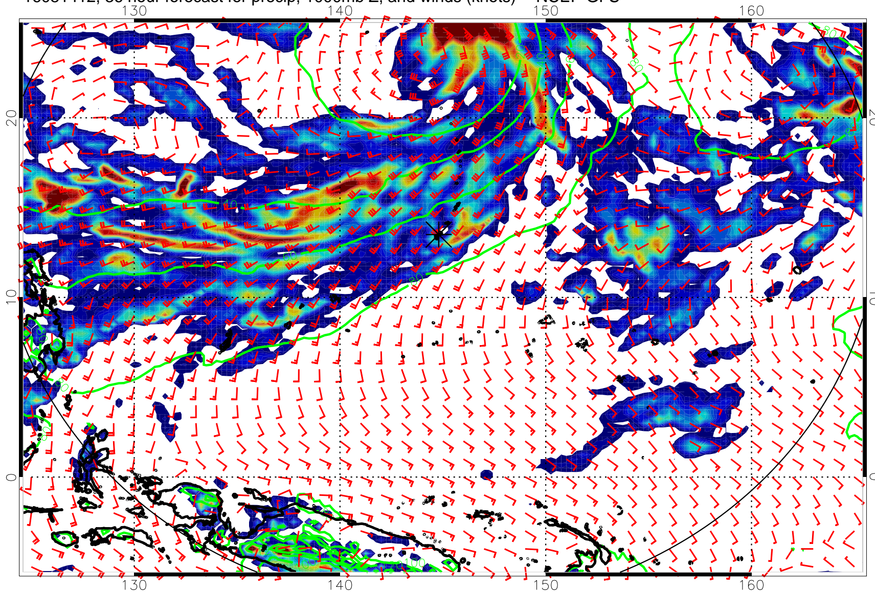
16081412, 36 hour forecast for precip, 1000mb Z, and winds (knots) -- NCEP GFS
