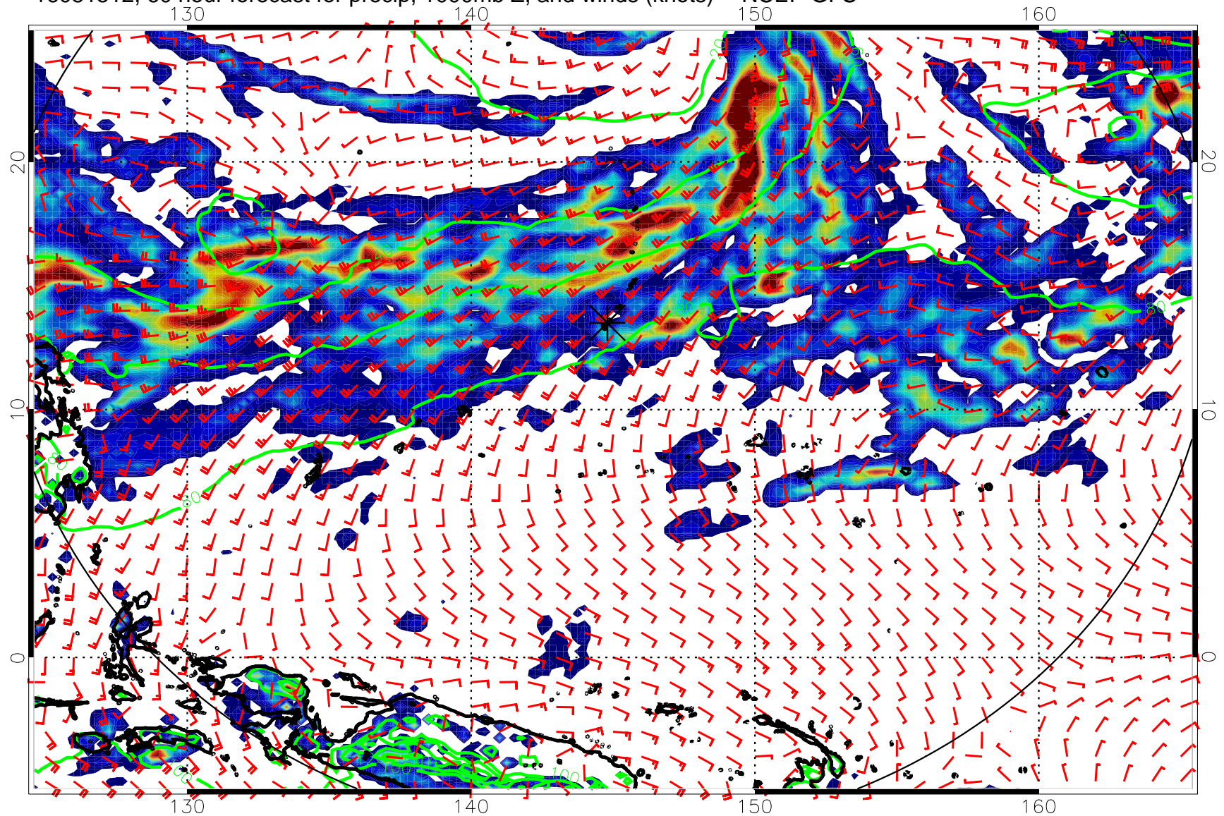
16081512, 60 hour forecast for precip, 1000mb Z, and winds (knots) -- NCEP GFS
