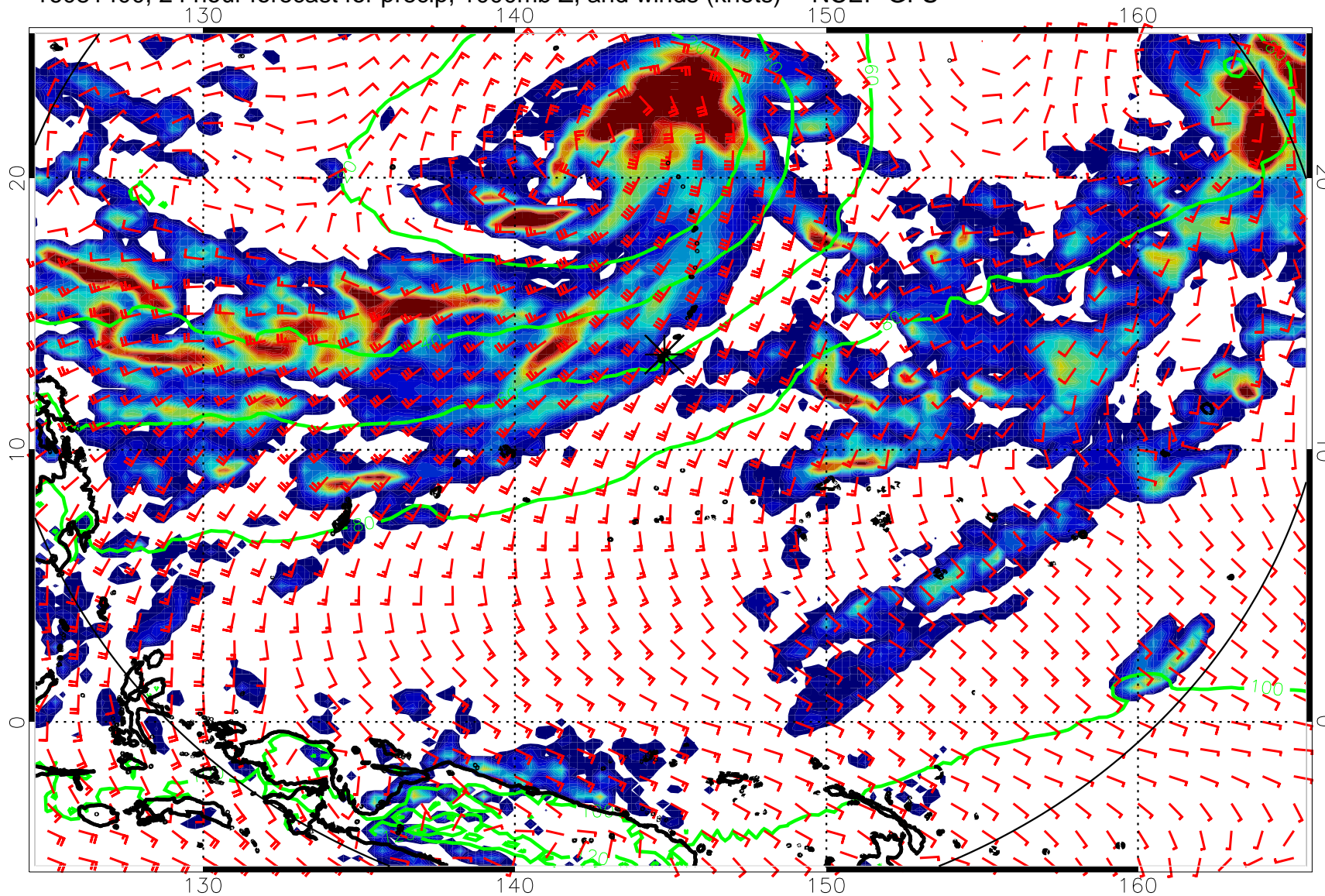
16081400, 24 hour forecast for precip, 1000mb Z, and winds (knots) -- NCEP GFS
