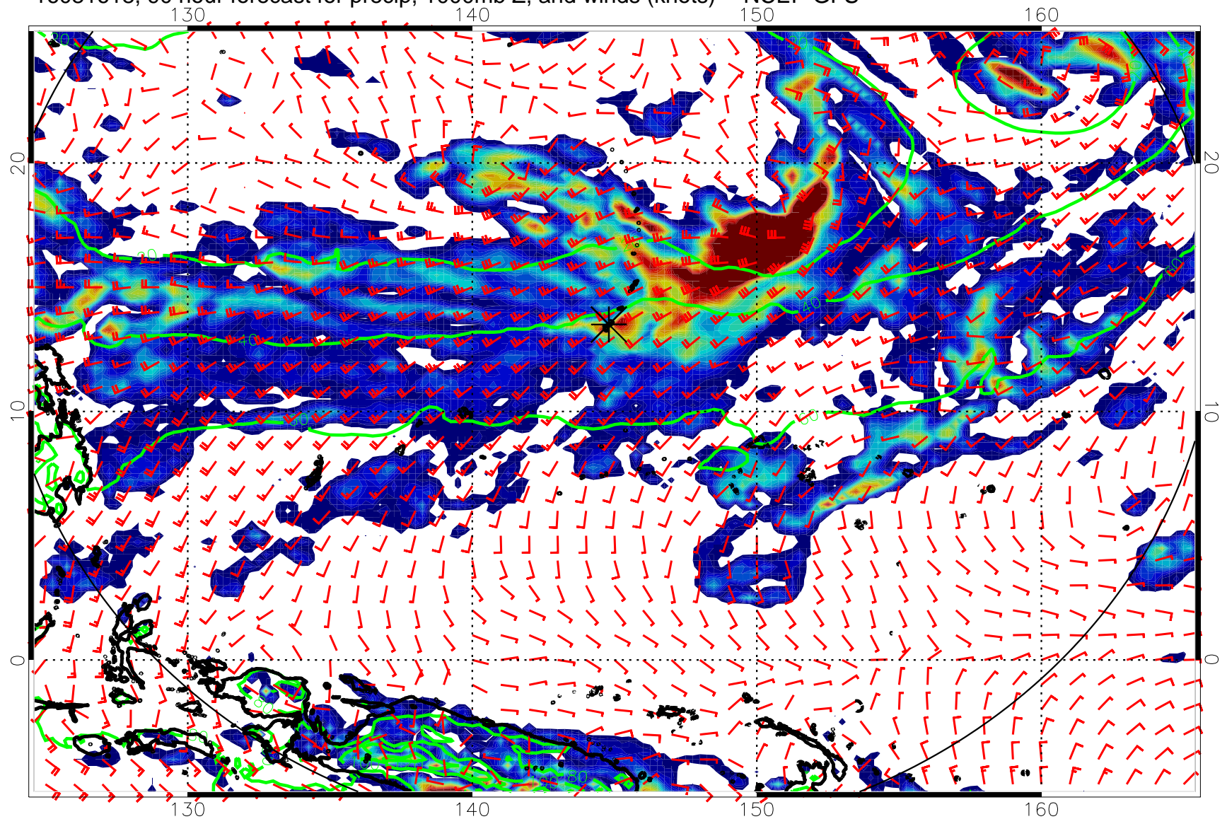
16081618, 90 hour forecast for precip, 1000mb Z, and winds (knots) -- NCEP GFS
