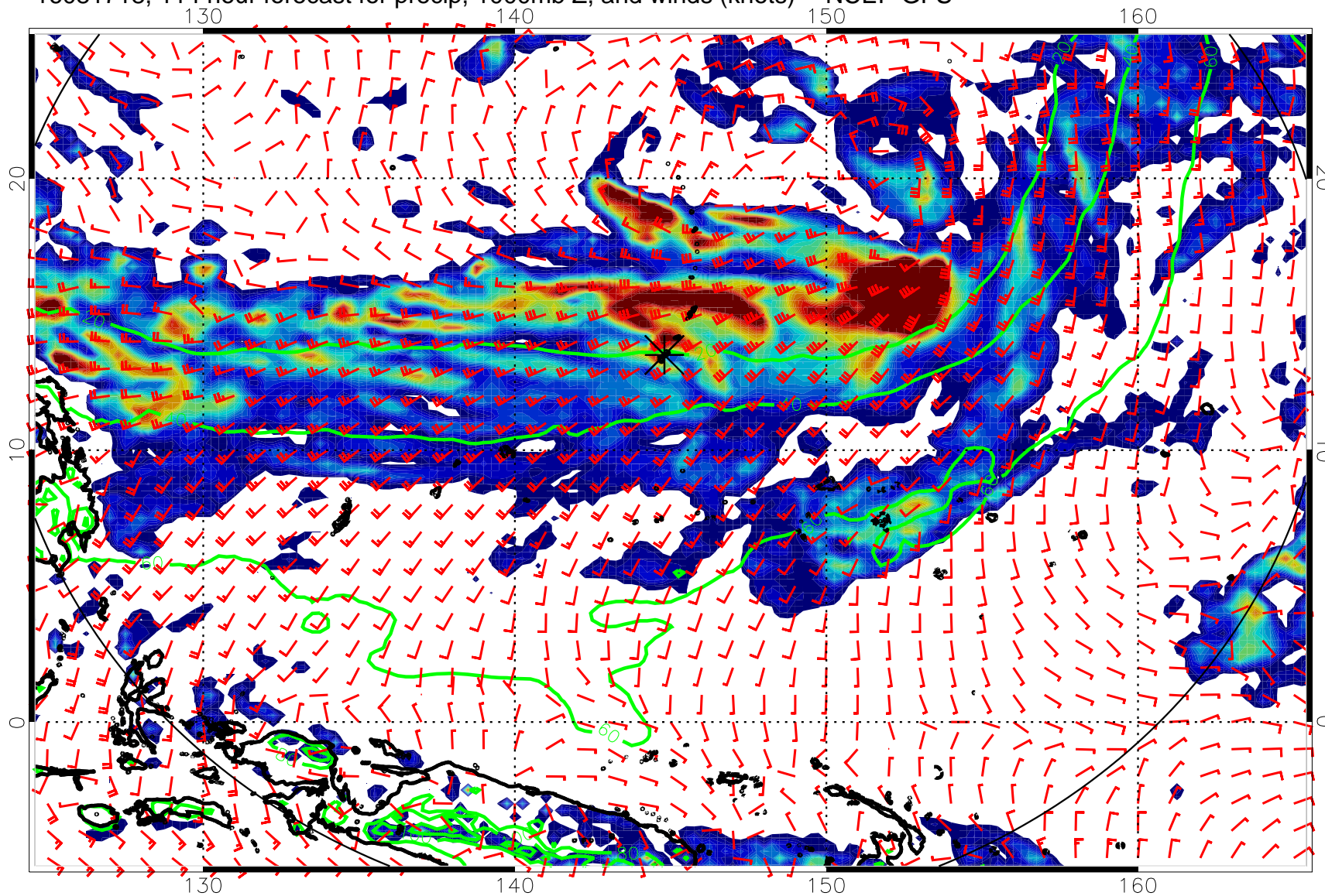
16081718, 114 hour forecast for precip, 1000mb Z, and winds (knots) -- NCEP GFS
