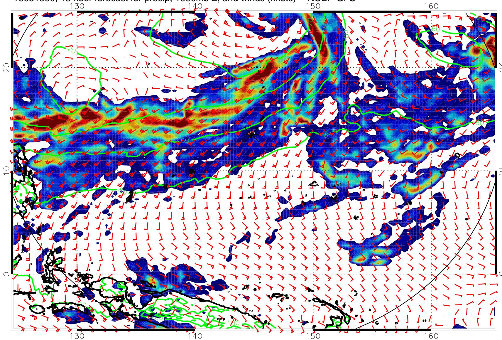
16081500, 48 hour forecast for precip, 1000mb Z, and winds (knots) -- NCEP GFS
