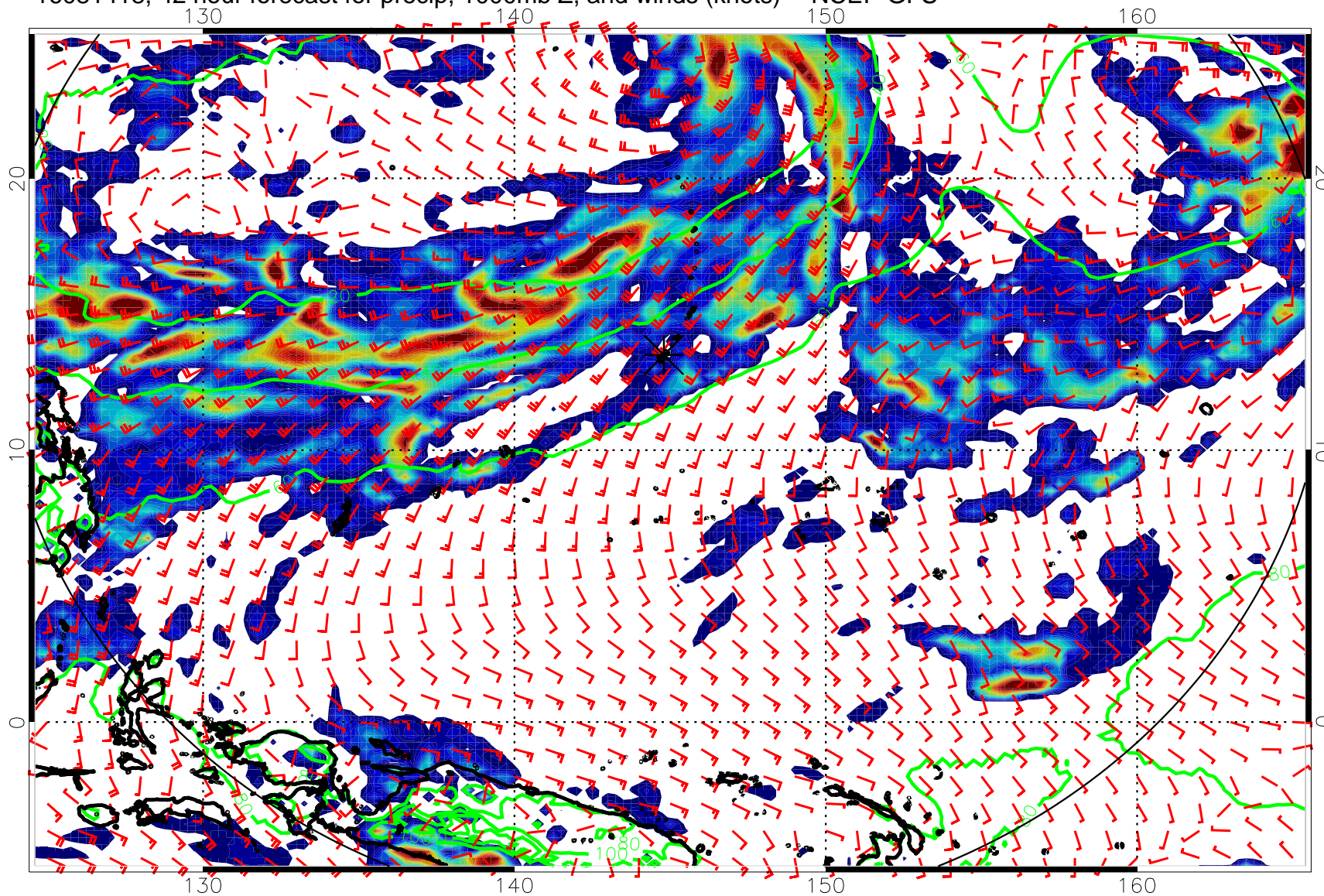
16081418, 42 hour forecast for precip, 1000mb Z, and winds (knots) -- NCEP GFS
