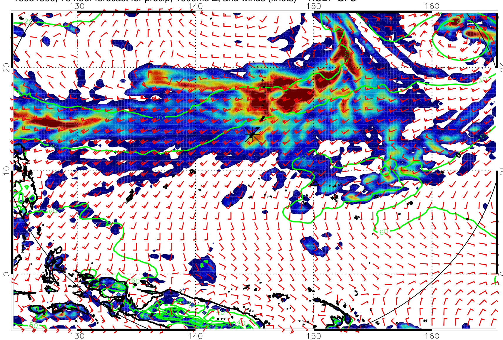
16081606, 78 hour forecast for precip, 1000mb Z, and winds (knots) -- NCEP GFS
