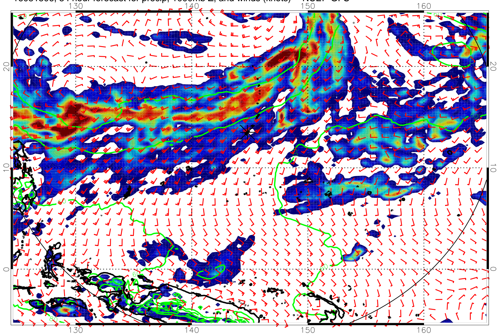
16081506, 54 hour forecast for precip, 1000mb Z, and winds (knots) -- NCEP GFS
