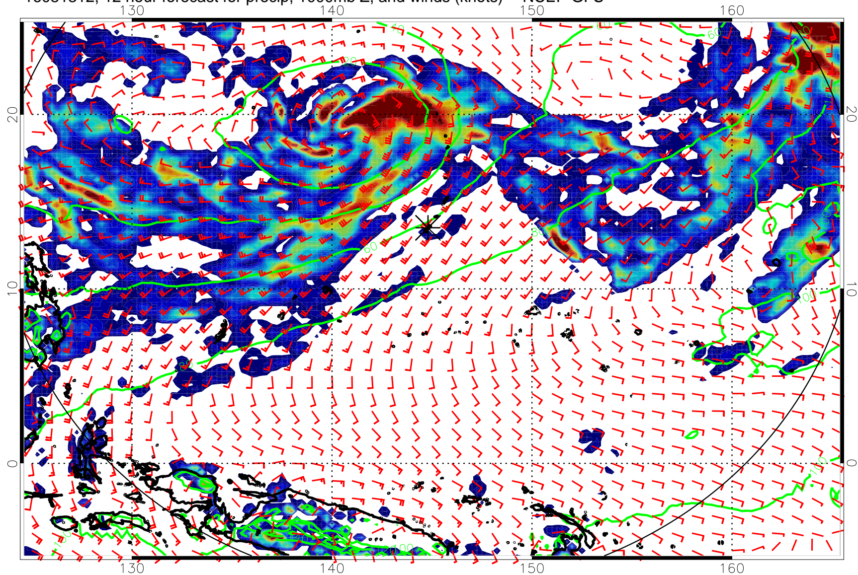
16081312, 12 hour forecast for precip, 1000mb Z, and winds (knots) -- NCEP GFS
