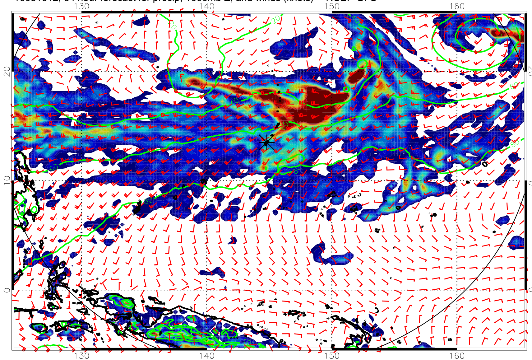
16081612, 84 hour forecast for precip, 1000mb Z, and winds (knots) -- NCEP GFS
