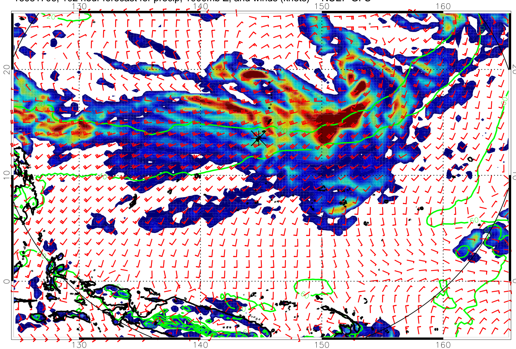
16081706, 102 hour forecast for precip, 1000mb Z, and winds (knots) -- NCEP GFS
