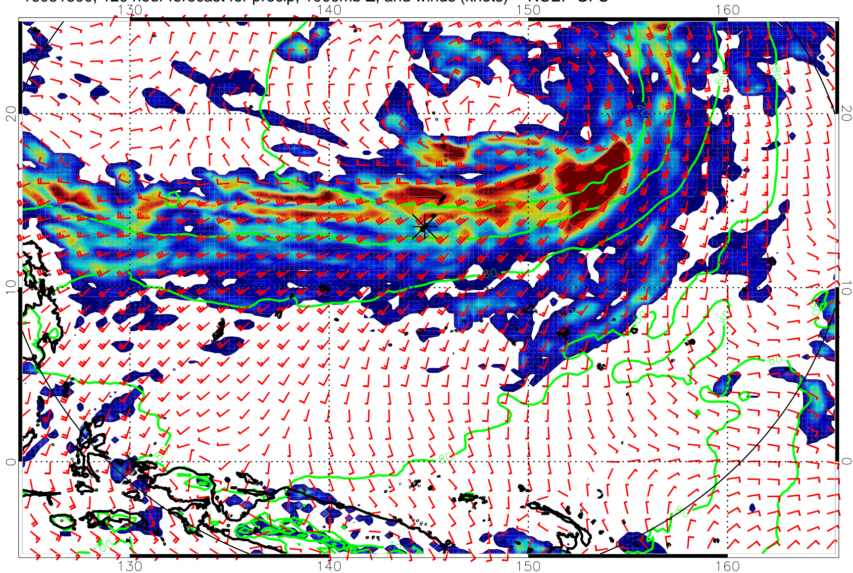
16081800, 120 hour forecast for precip, 1000mb Z, and winds (knots) -- NCEP GFS
