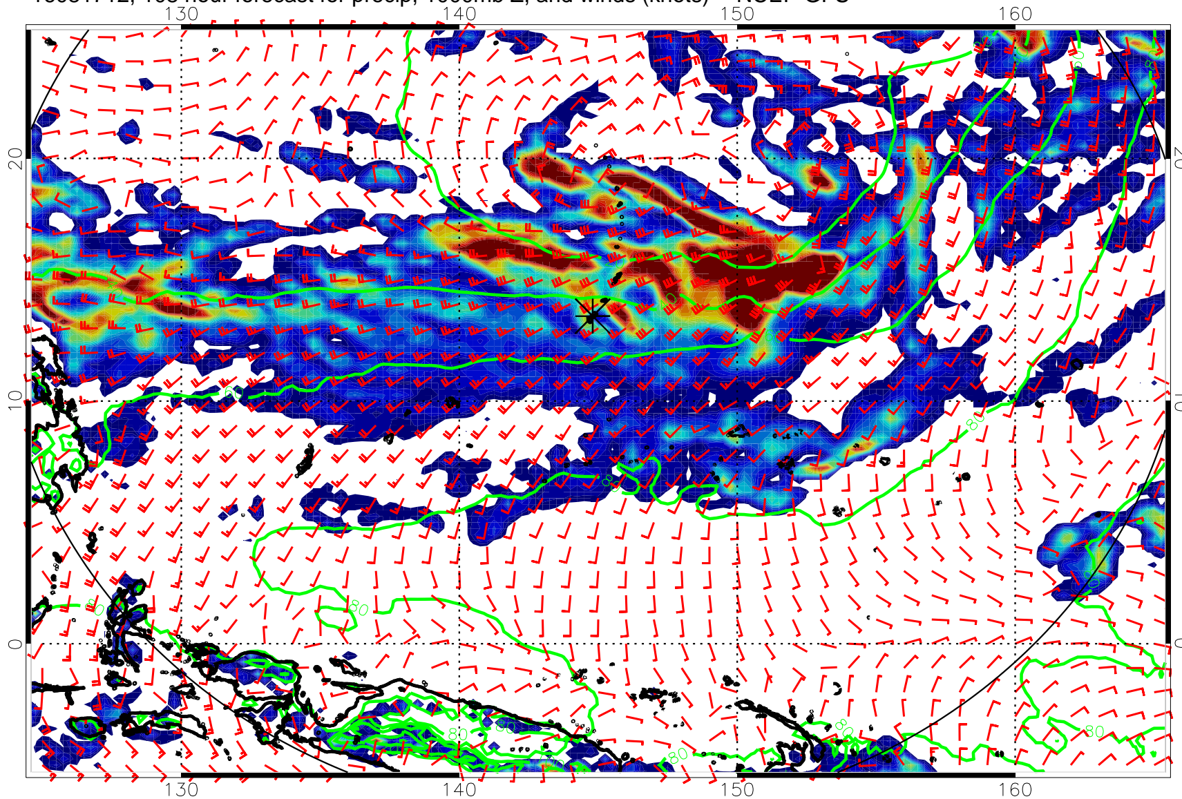
16081712, 108 hour forecast for precip, 1000mb Z, and winds (knots) -- NCEP GFS
