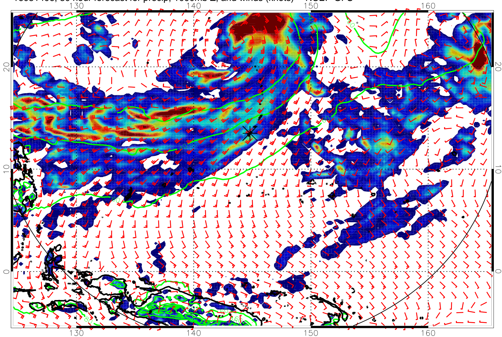
16081406, 30 hour forecast for precip, 1000mb Z, and winds (knots) -- NCEP GFS
