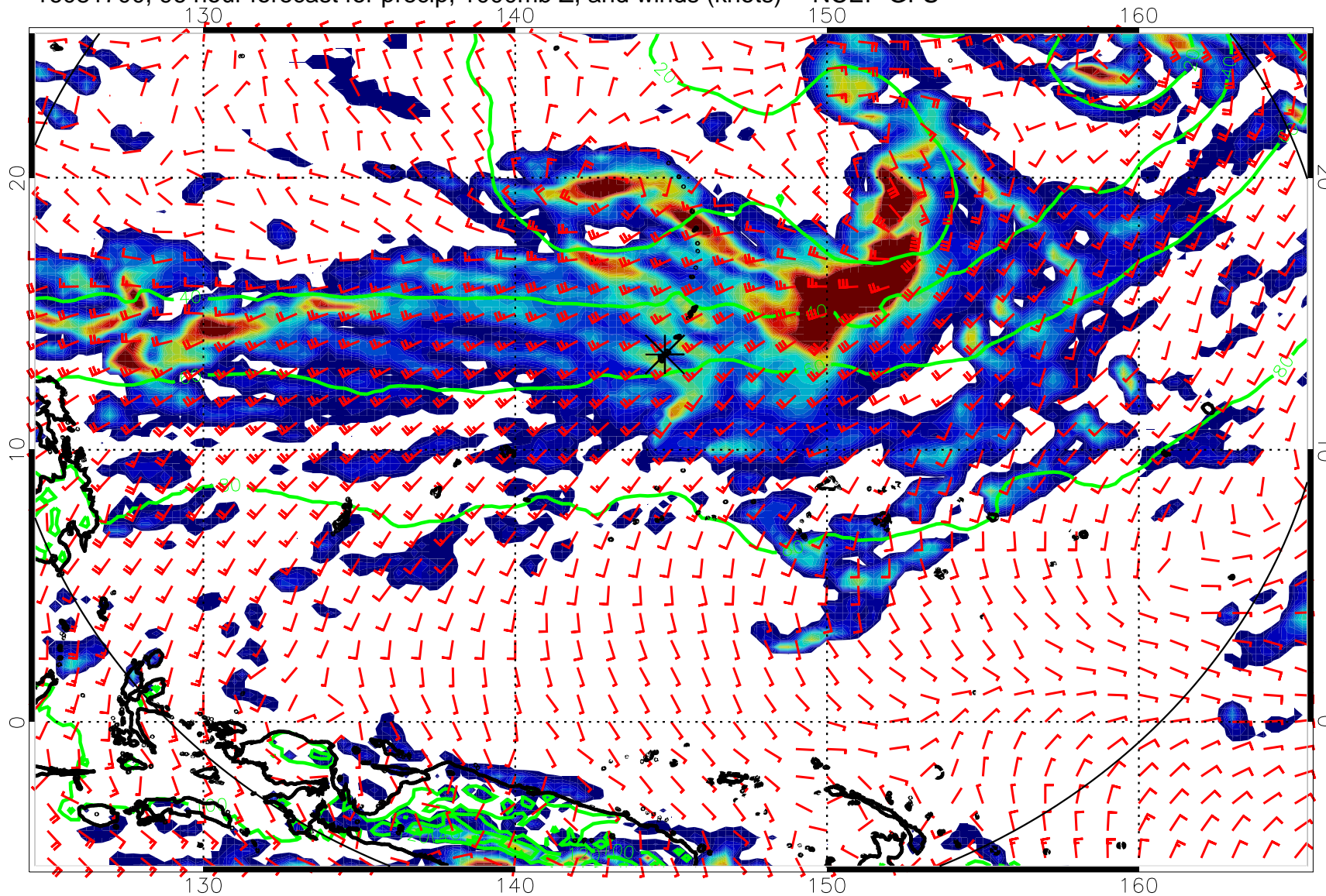
16081700, 96 hour forecast for precip, 1000mb Z, and winds (knots) -- NCEP GFS
