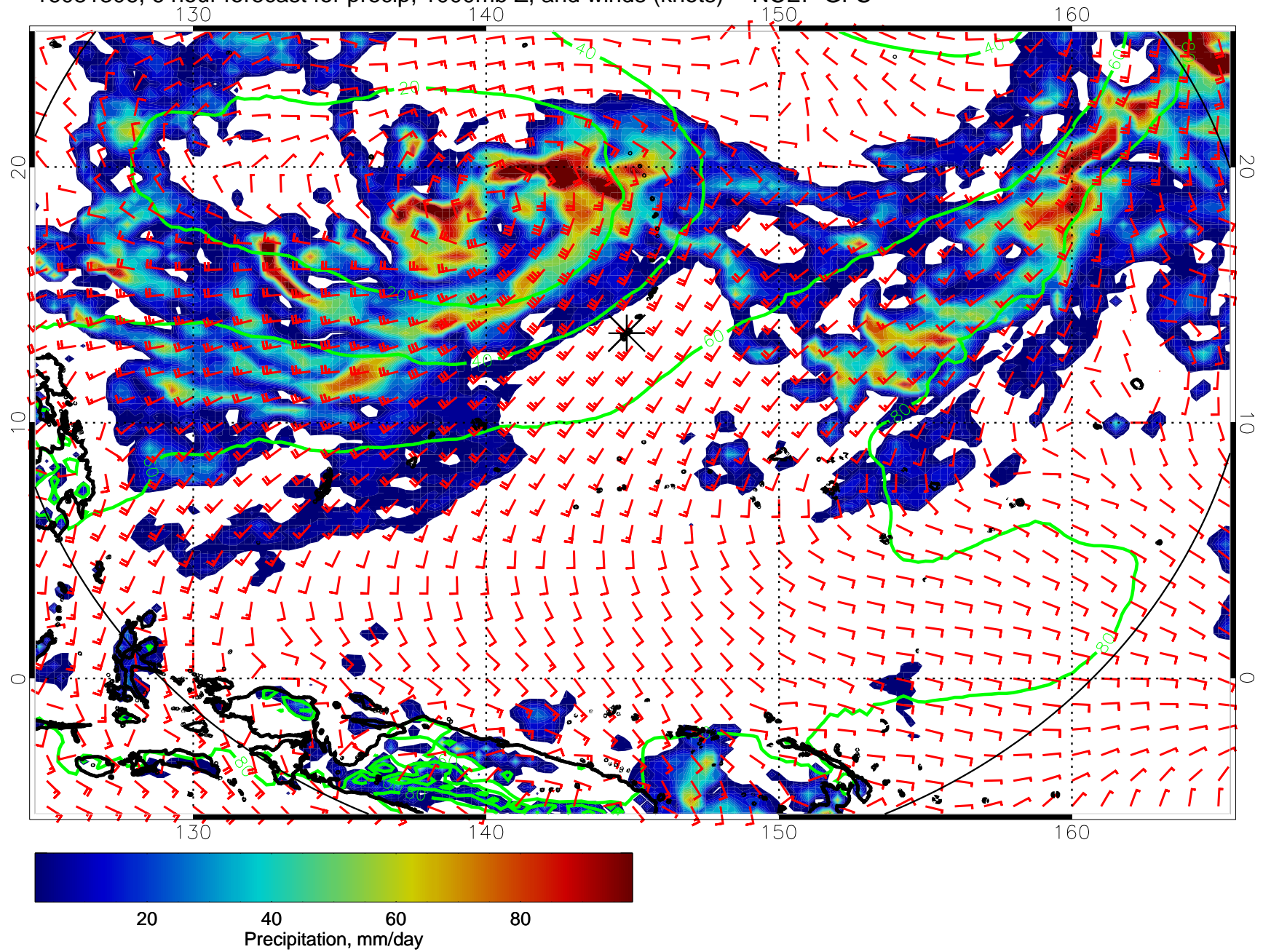
16081306, 6 hour forecast for precip, 1000mb Z, and winds (knots) -- NCEP GFS
