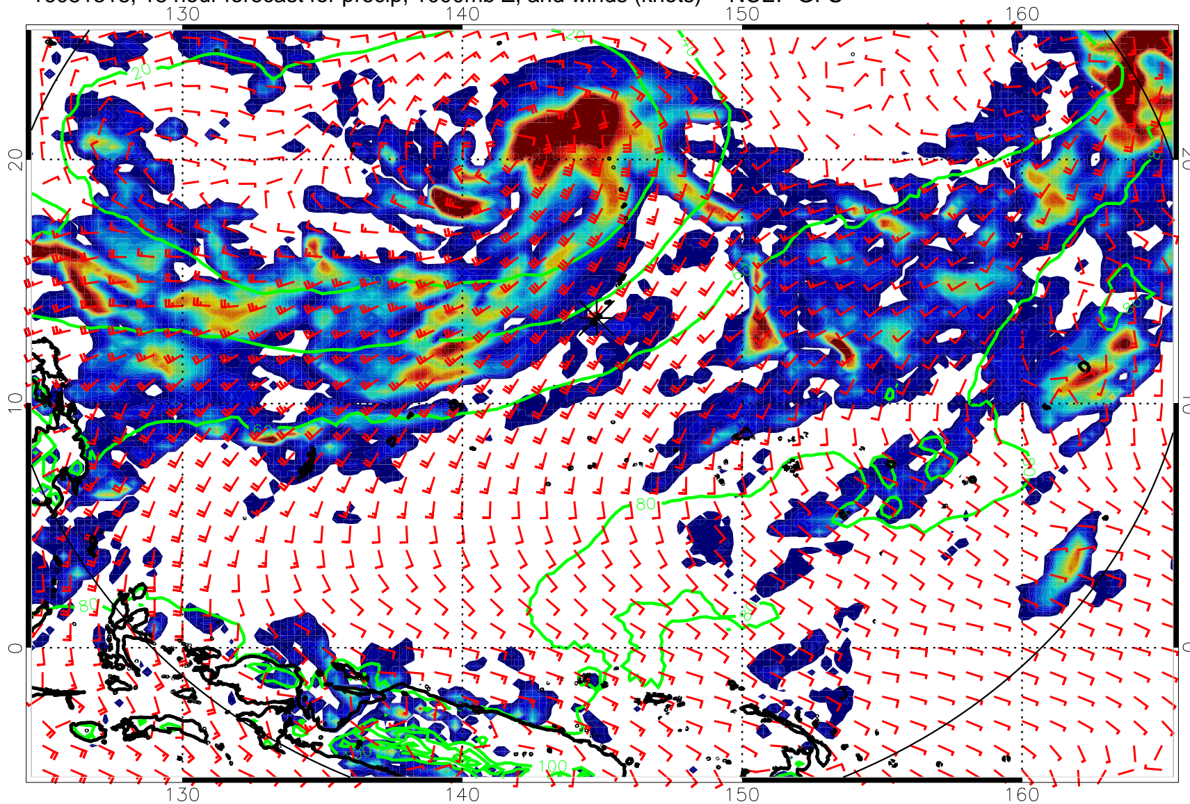
16081318, 18 hour forecast for precip, 1000mb Z, and winds (knots) -- NCEP GFS
