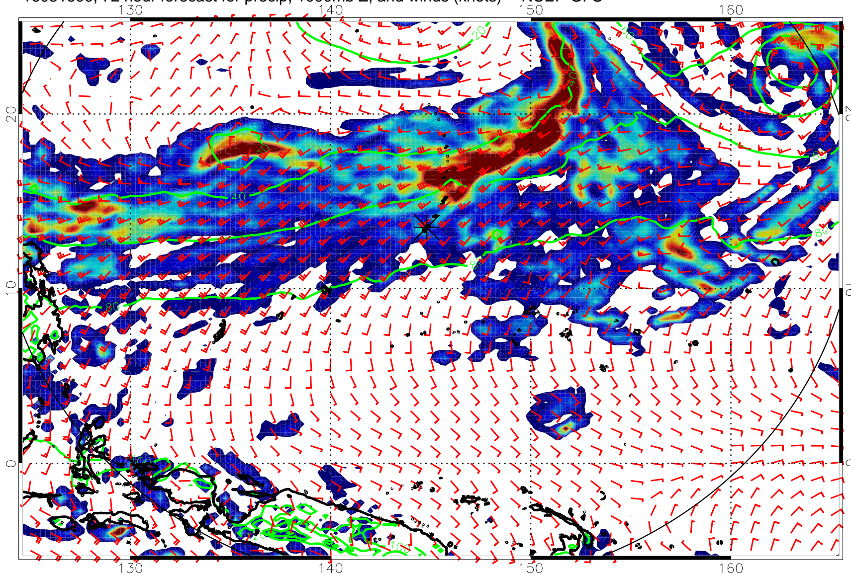
16081600, 72 hour forecast for precip, 1000mb Z, and winds (knots) -- NCEP GFS
