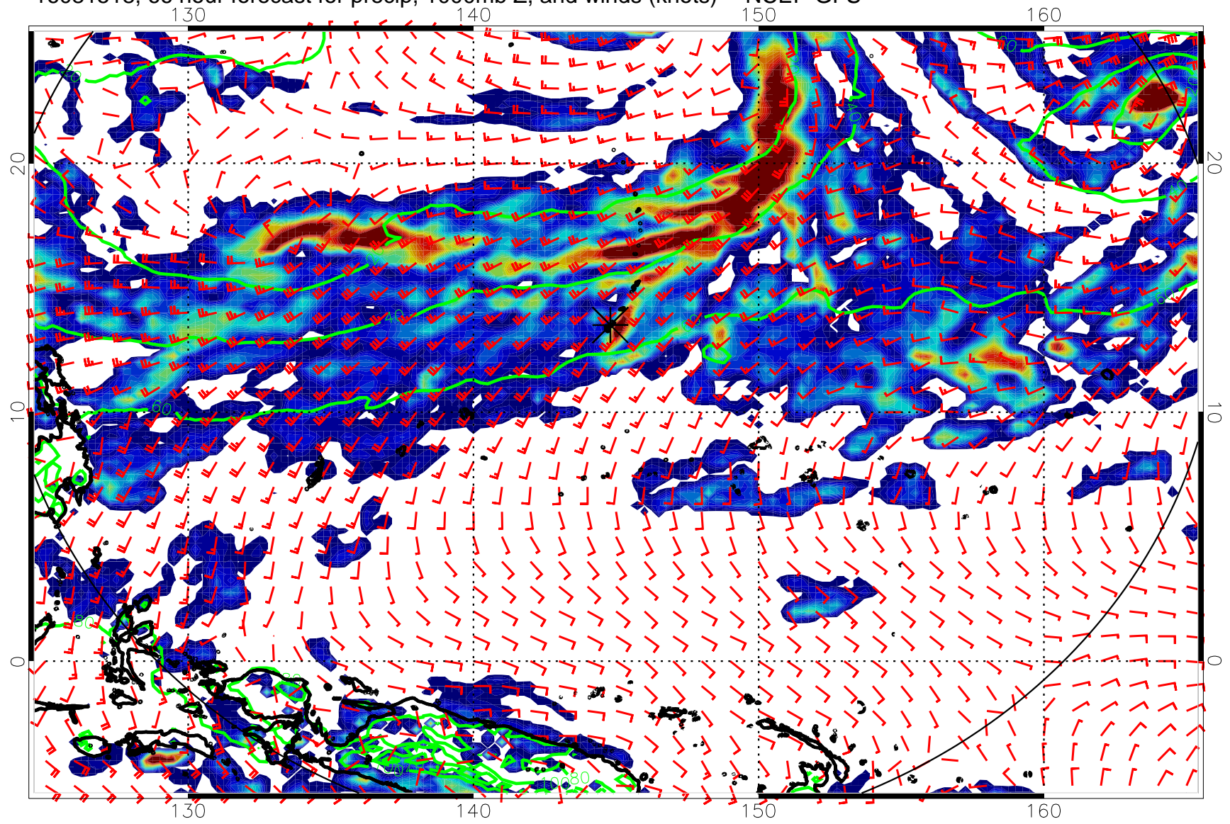
16081518, 66 hour forecast for precip, 1000mb Z, and winds (knots) -- NCEP GFS
