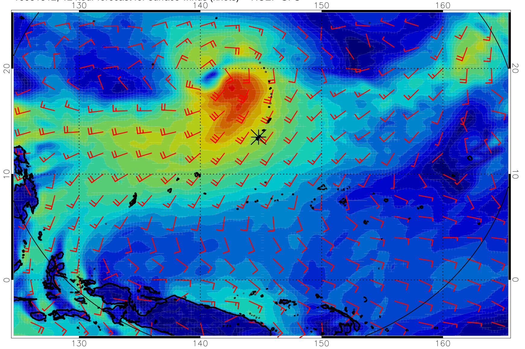
16081312, 12 hour forecast for surface winds (knots) -- NCEP GFS
