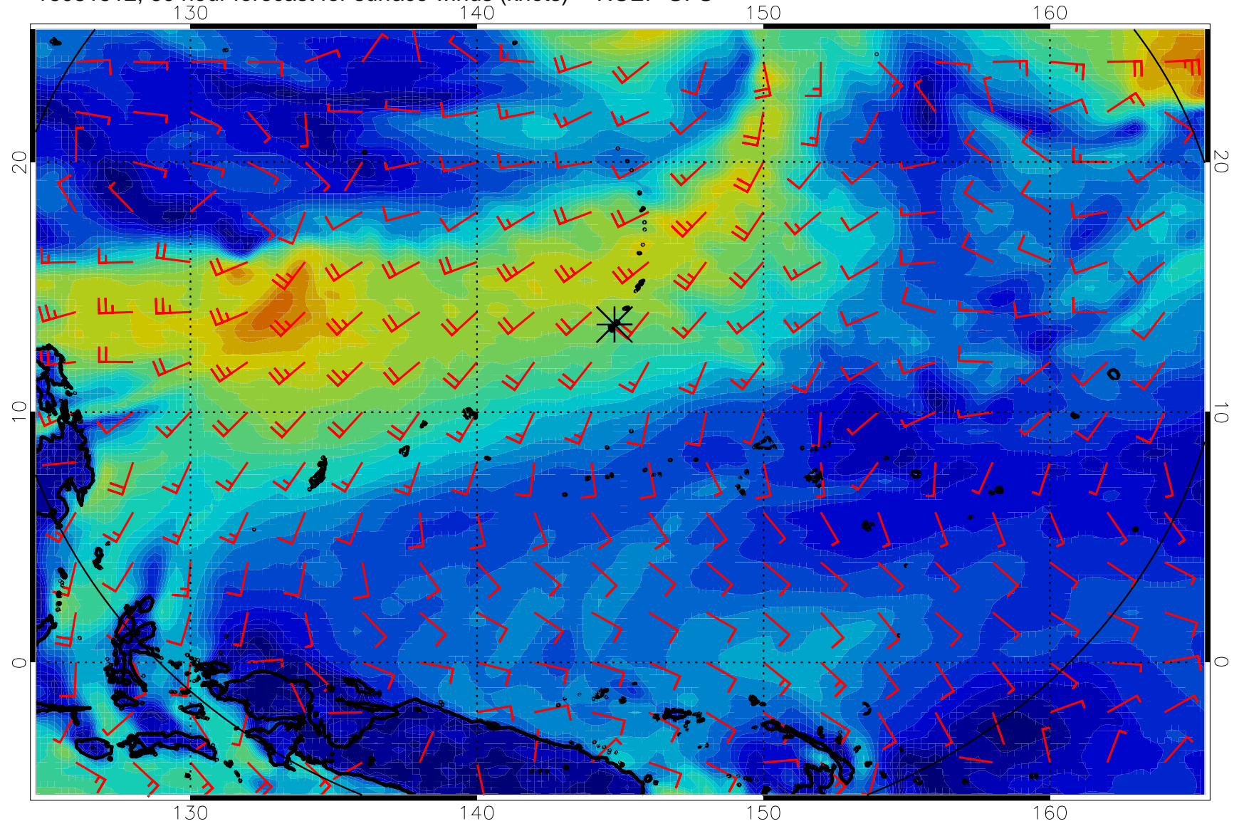
16081512, 60 hour forecast for surface winds (knots) -- NCEP GFS
