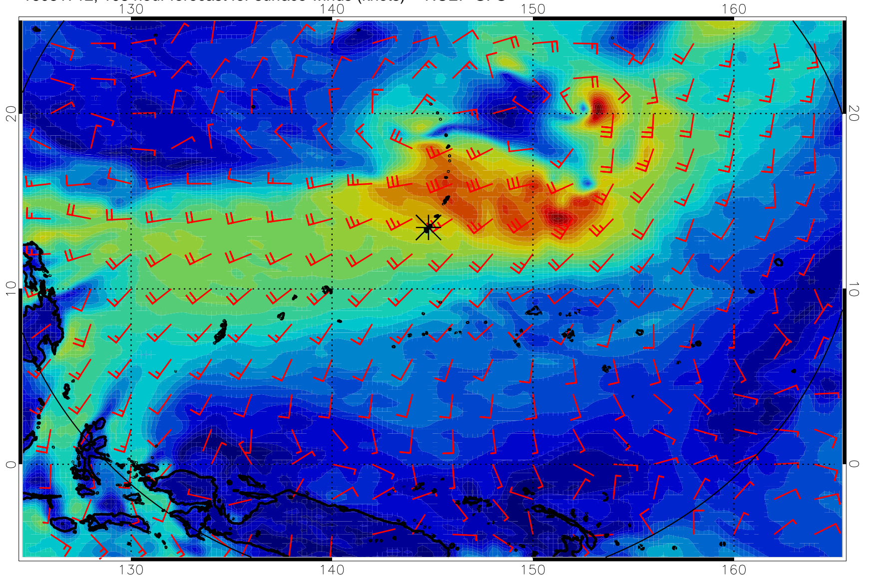
16081712, 108 hour forecast for surface winds (knots) -- NCEP GFS
