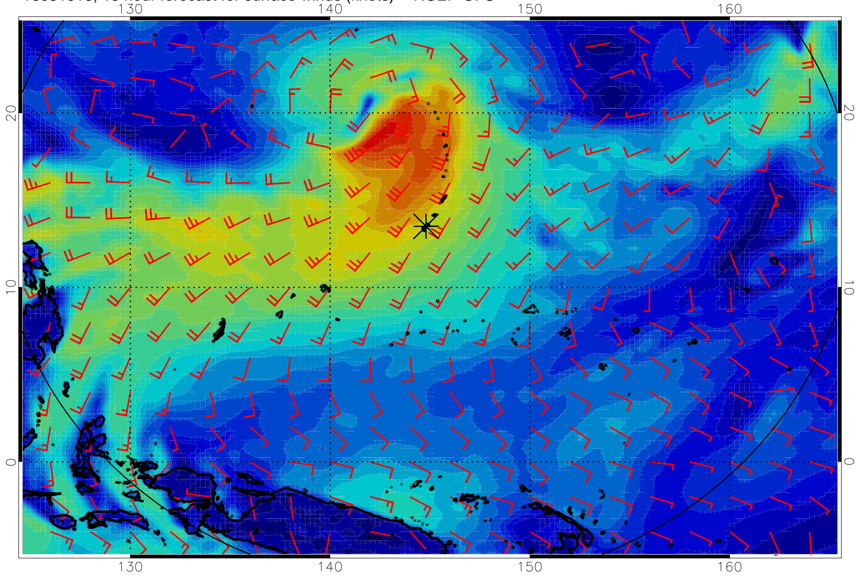
16081318, 18 hour forecast for surface winds (knots) -- NCEP GFS
