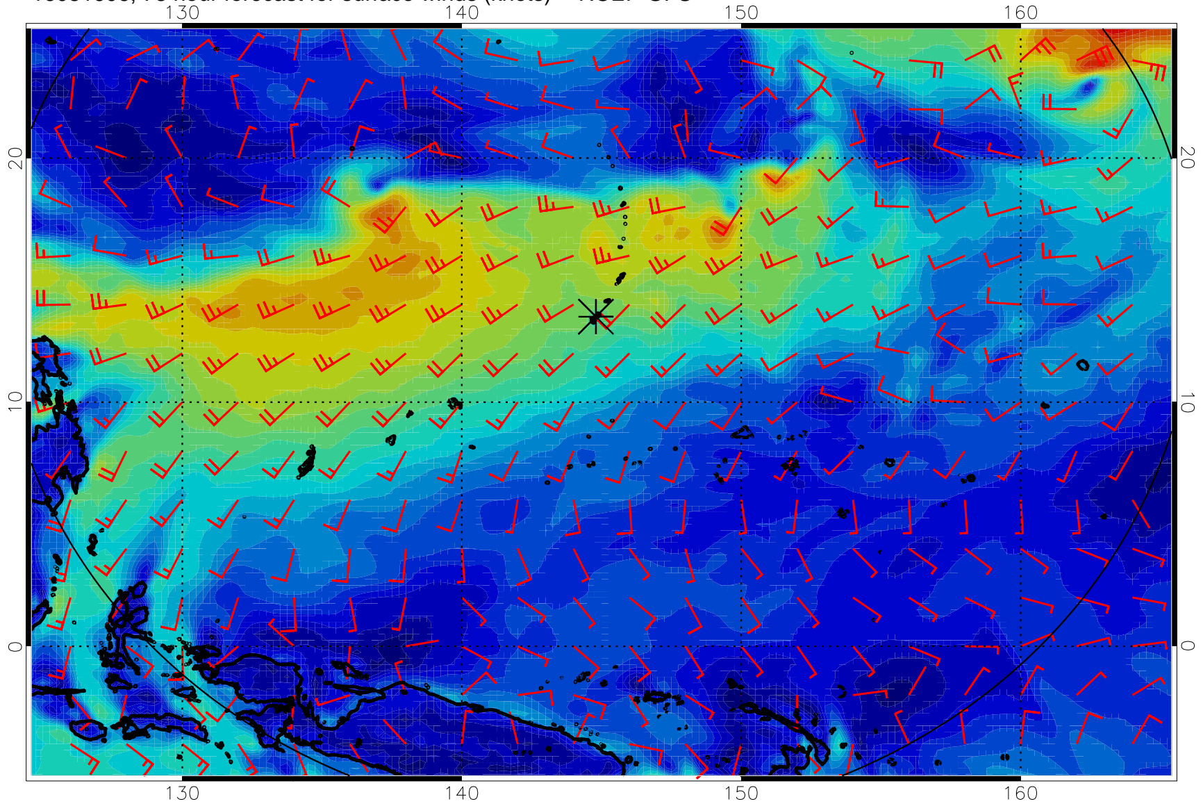
16081606, 78 hour forecast for surface winds (knots) -- NCEP GFS
