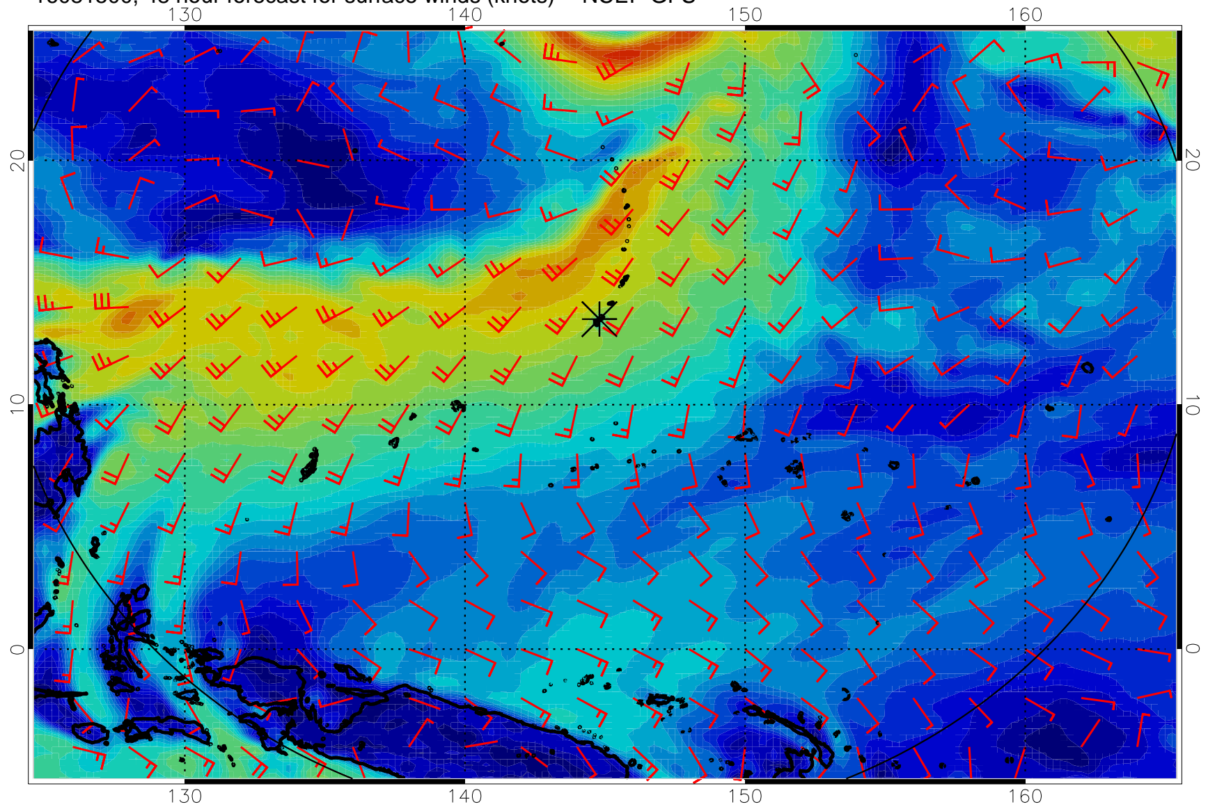
16081500, 48 hour forecast for surface winds (knots) -- NCEP GFS
