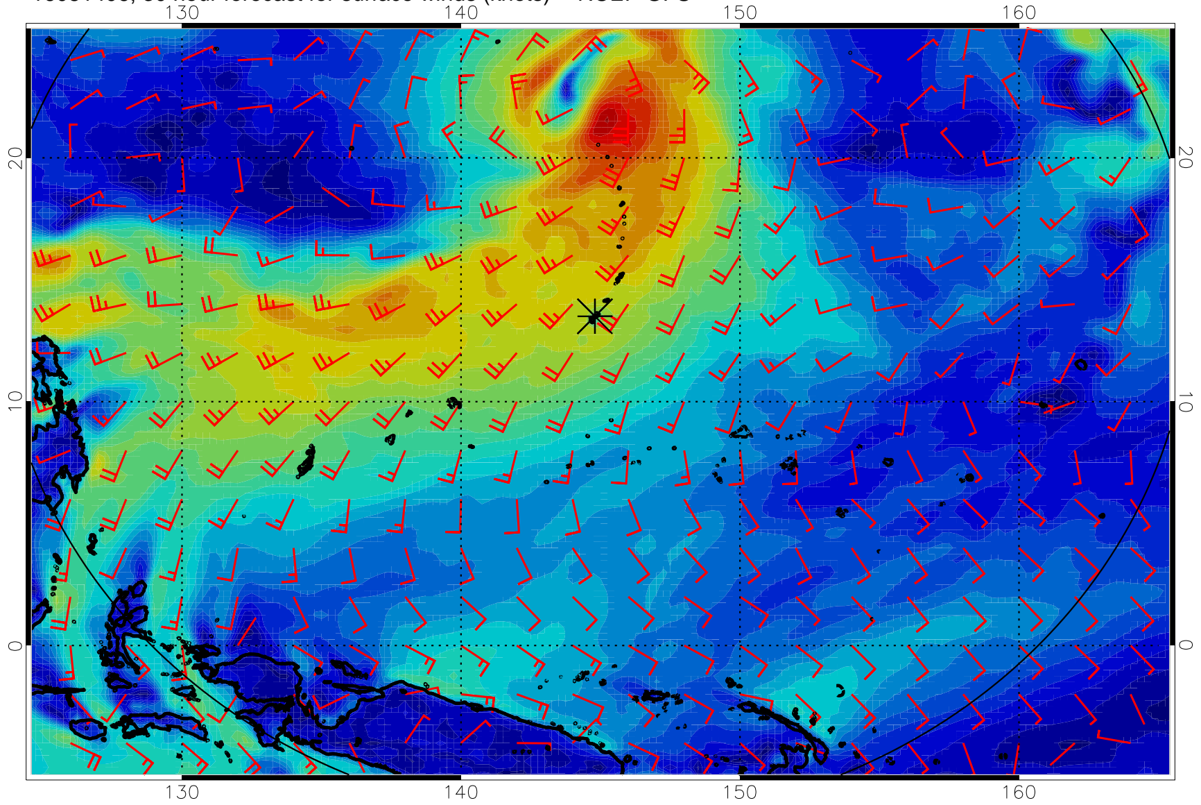
16081406, 30 hour forecast for surface winds (knots) -- NCEP GFS
