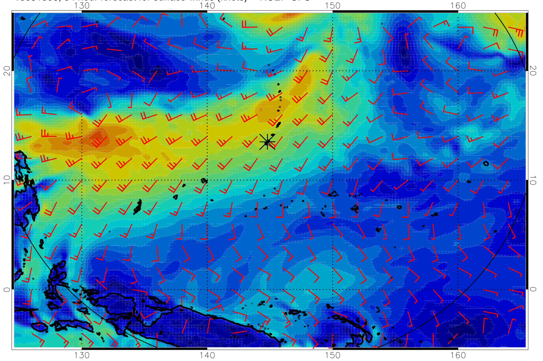
16081506, 54 hour forecast for surface winds (knots) -- NCEP GFS
