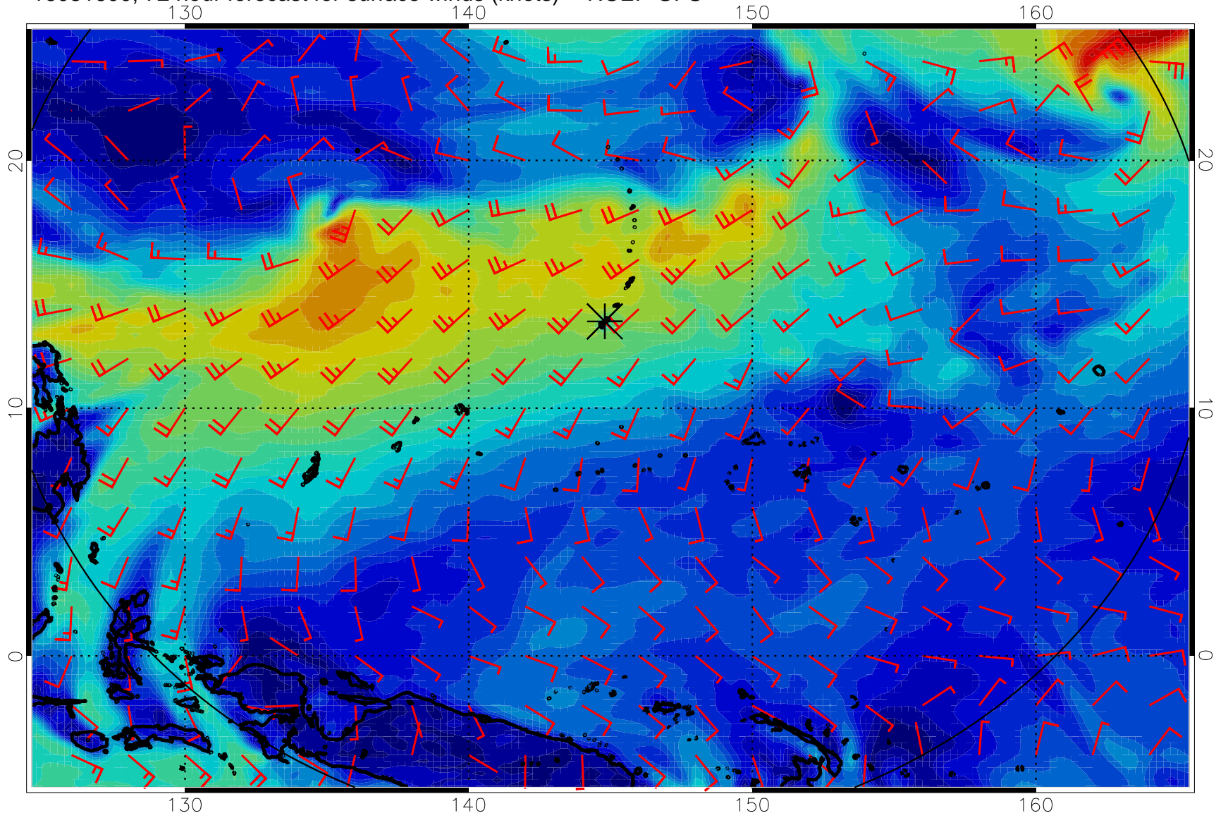
16081600, 72 hour forecast for surface winds (knots) -- NCEP GFS
