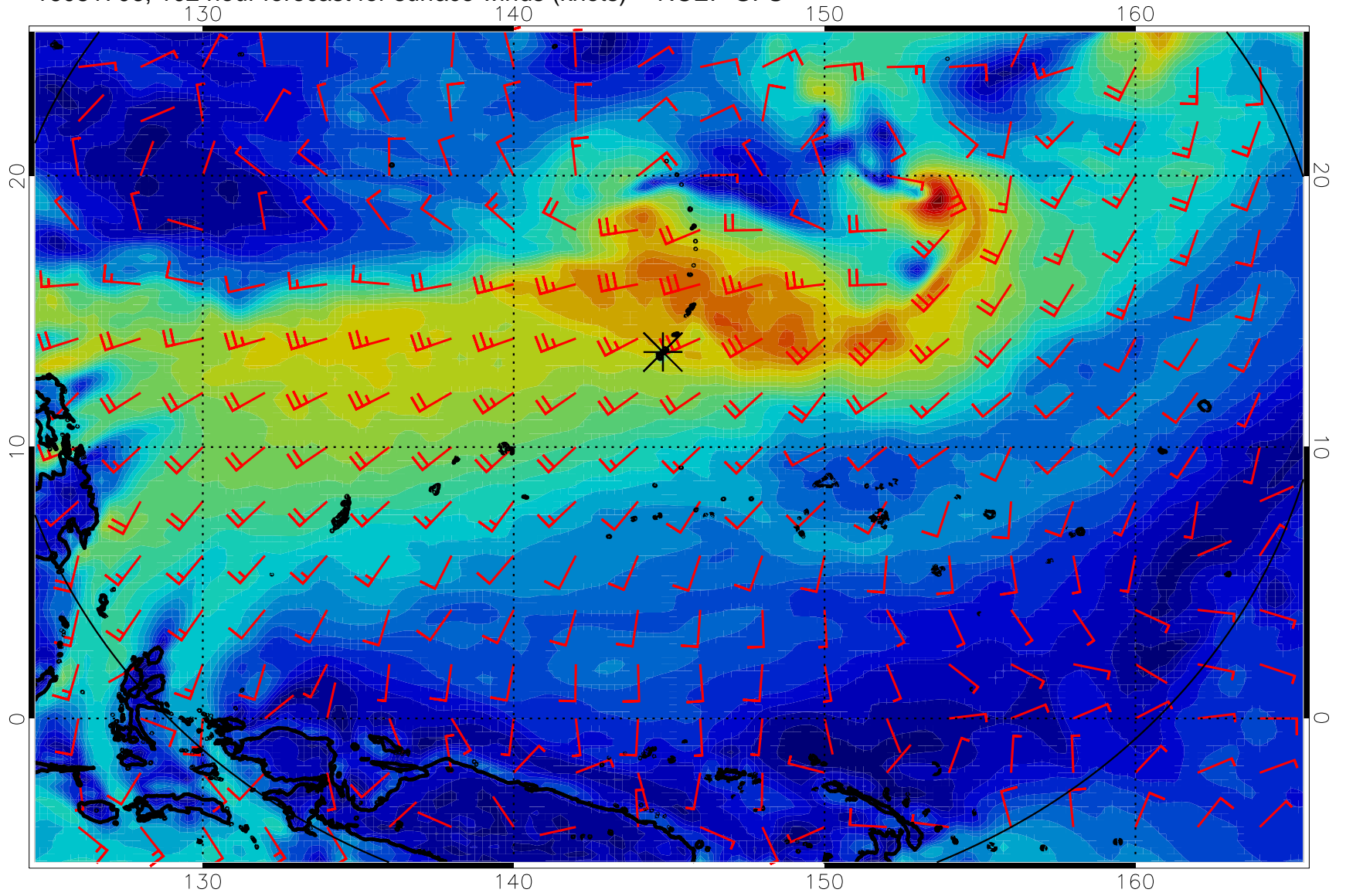
16081706, 102 hour forecast for surface winds (knots) -- NCEP GFS
