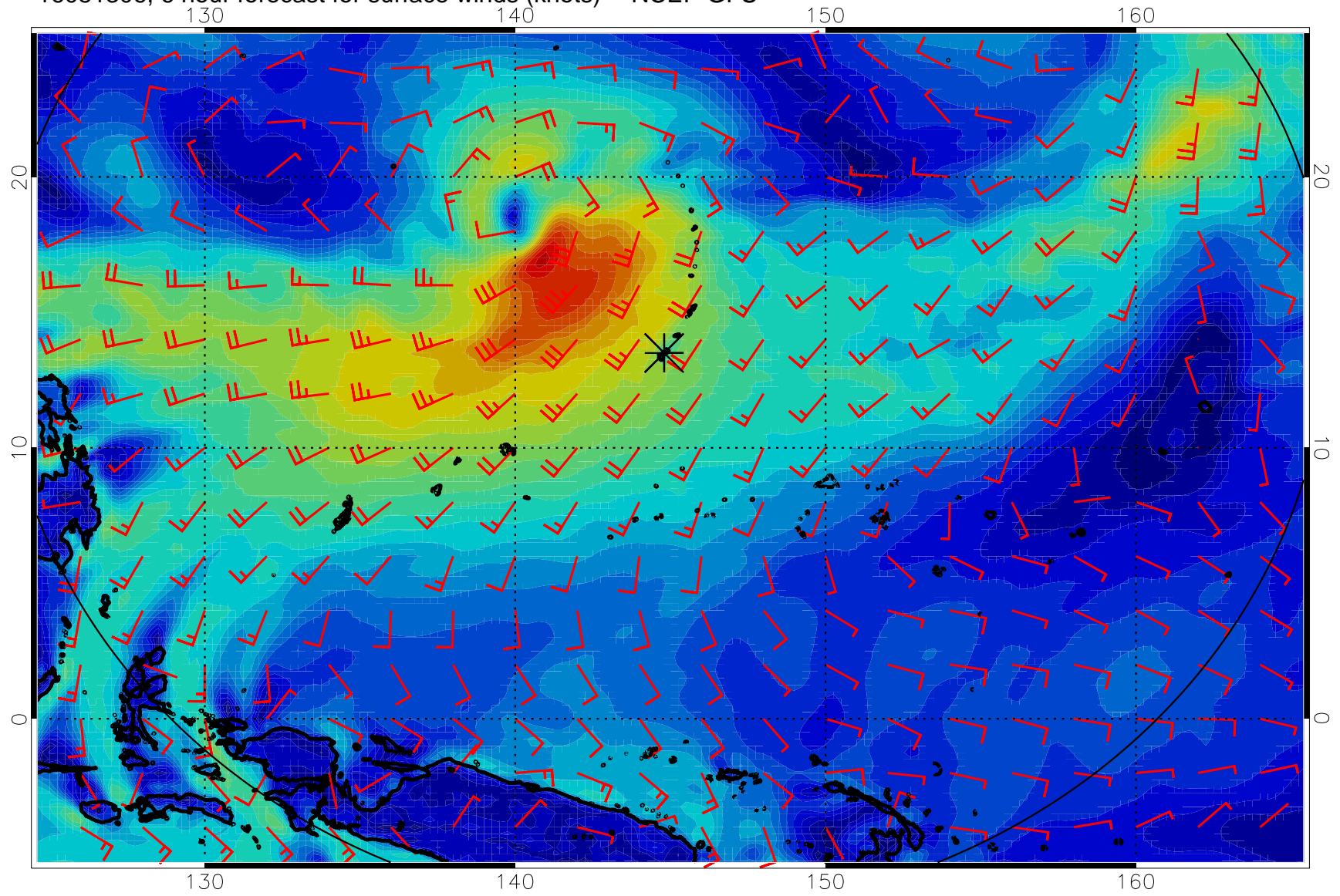
16081306, 6 hour forecast for surface winds (knots) -- NCEP GFS
