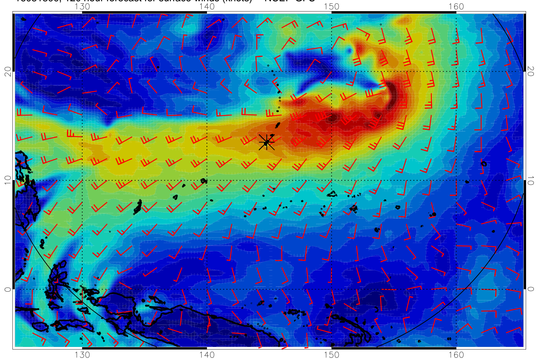
16081800, 120 hour forecast for surface winds (knots) -- NCEP GFS
