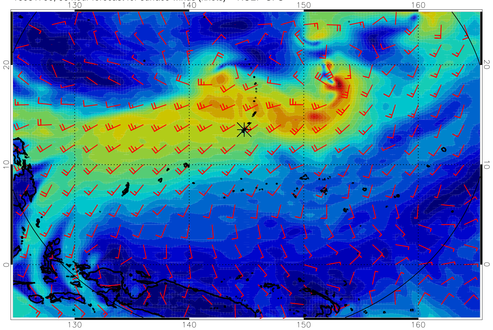
16081700, 96 hour forecast for surface winds (knots) -- NCEP GFS
