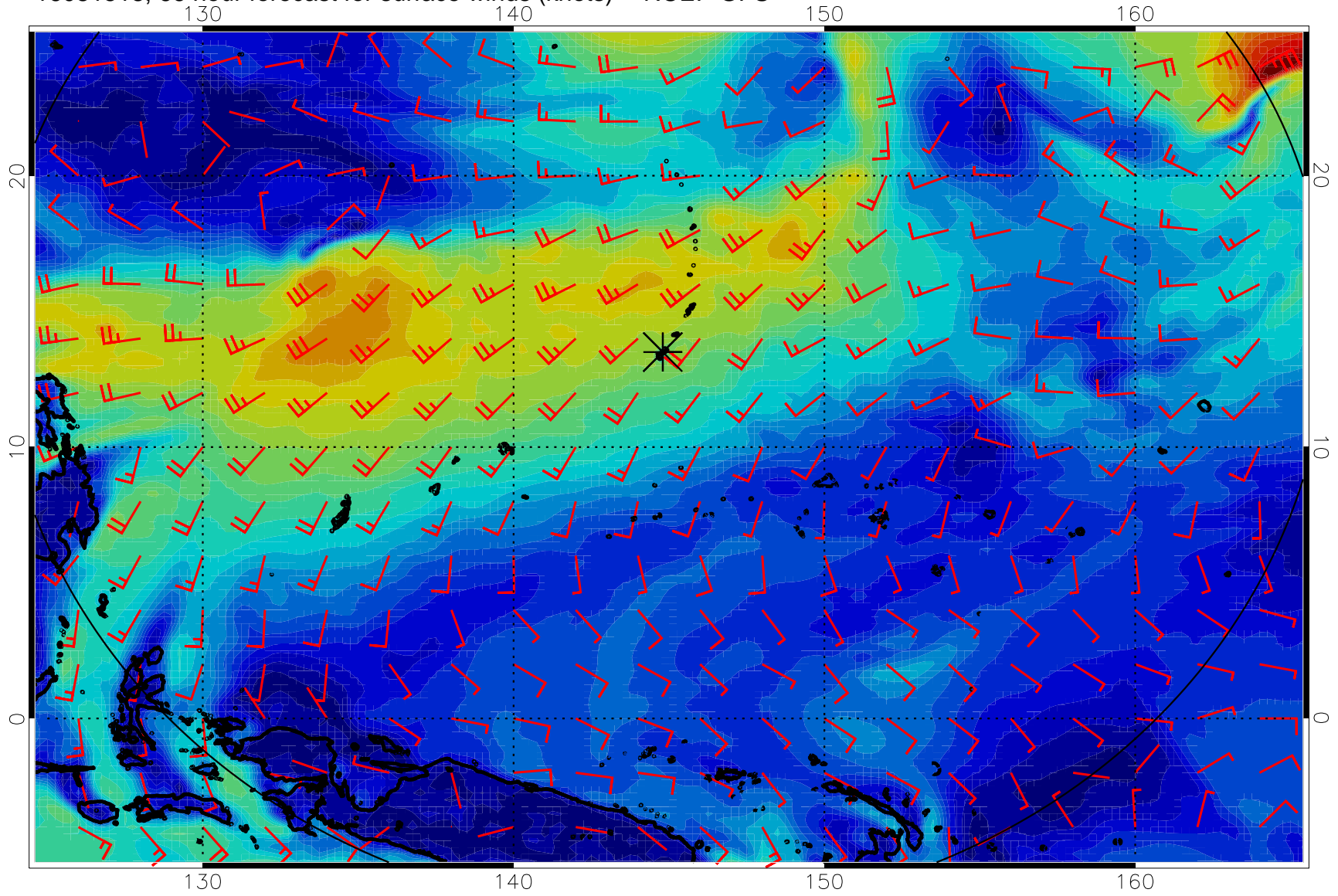
16081518, 66 hour forecast for surface winds (knots) -- NCEP GFS
