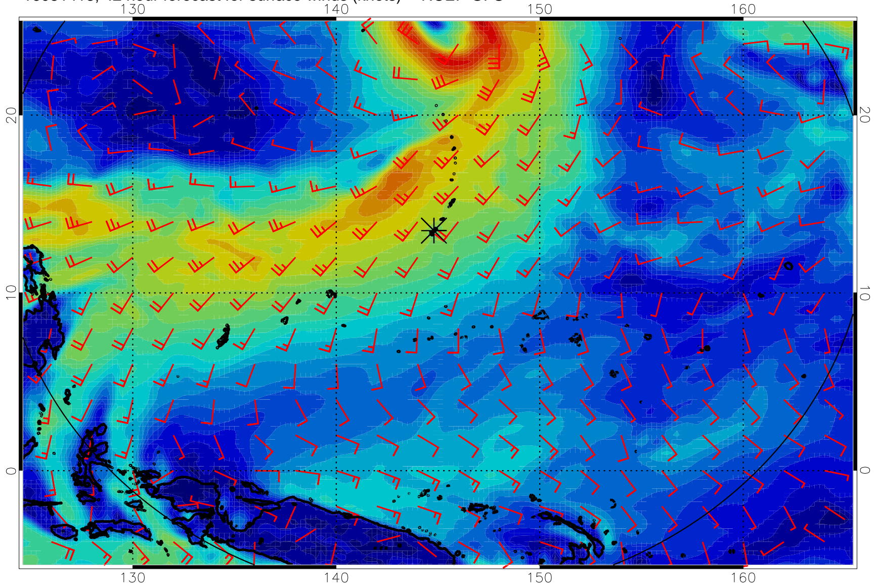
16081418, 42 hour forecast for surface winds (knots) -- NCEP GFS
