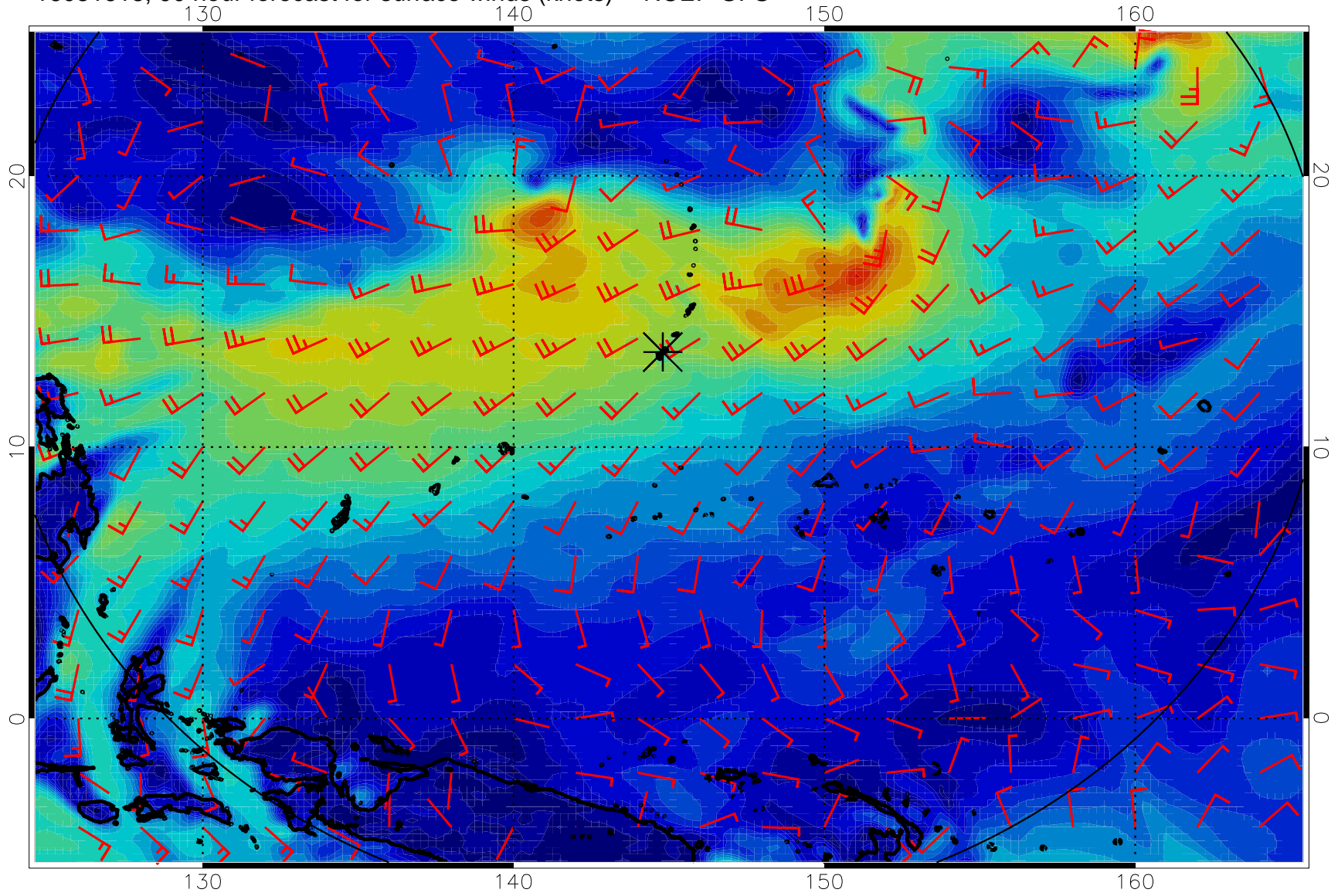
16081618, 90 hour forecast for surface winds (knots) -- NCEP GFS
