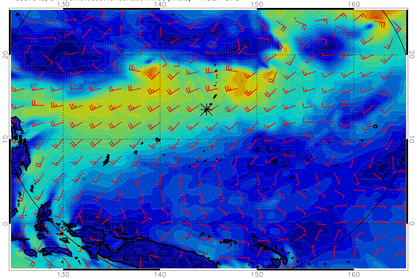
16081612, 84 hour forecast for surface winds (knots) -- NCEP GFS
