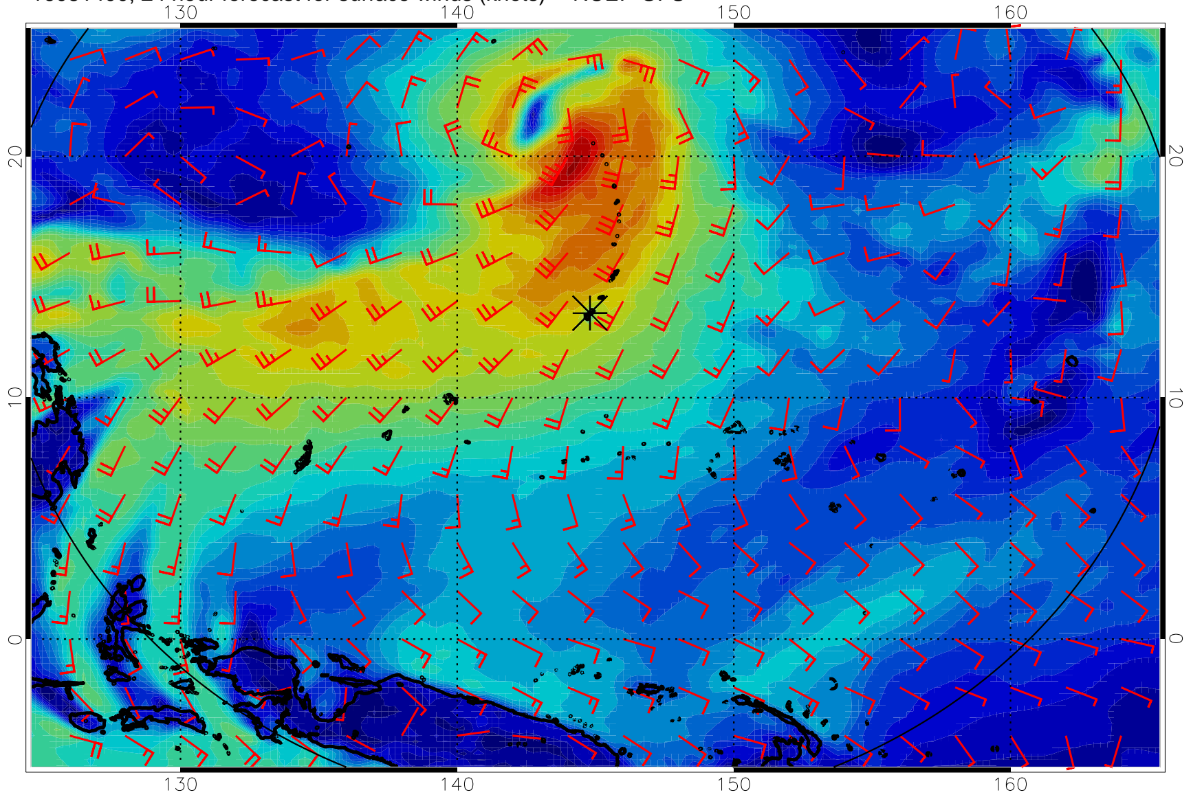
16081400, 24 hour forecast for surface winds (knots) -- NCEP GFS
