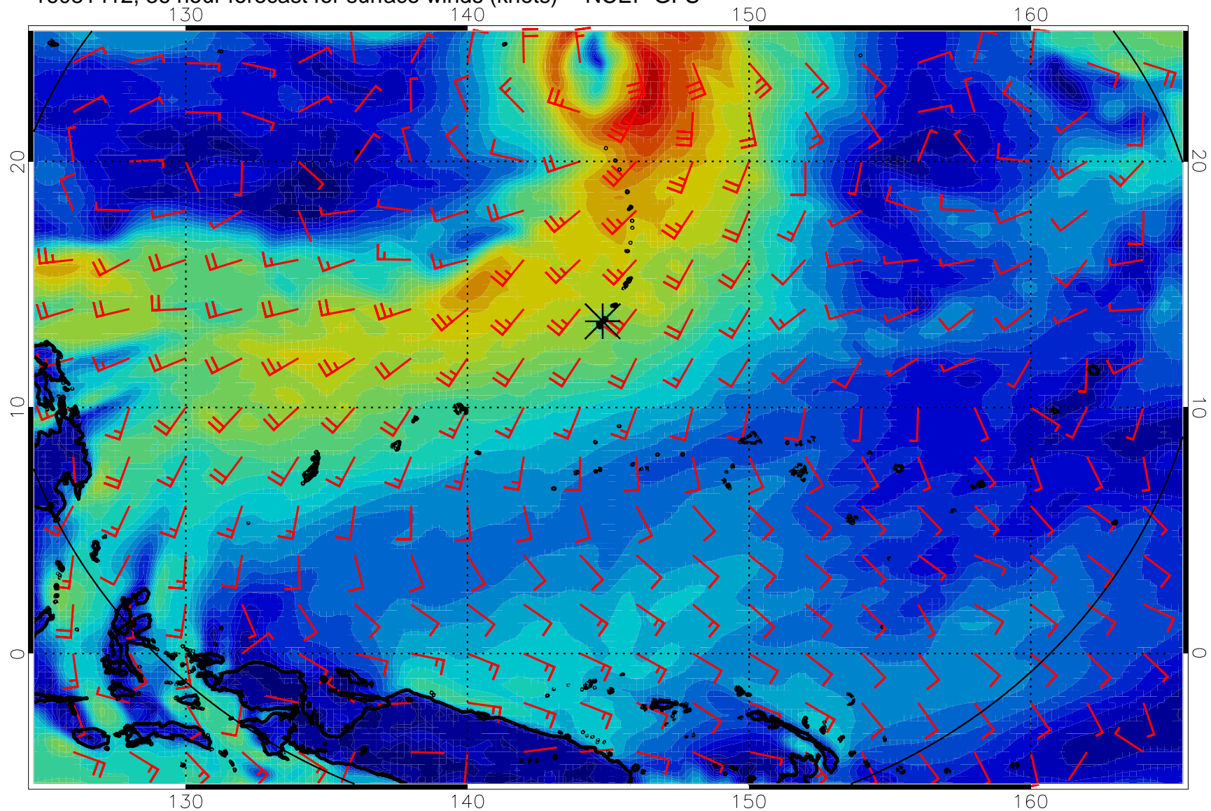
16081412, 36 hour forecast for surface winds (knots) -- NCEP GFS
