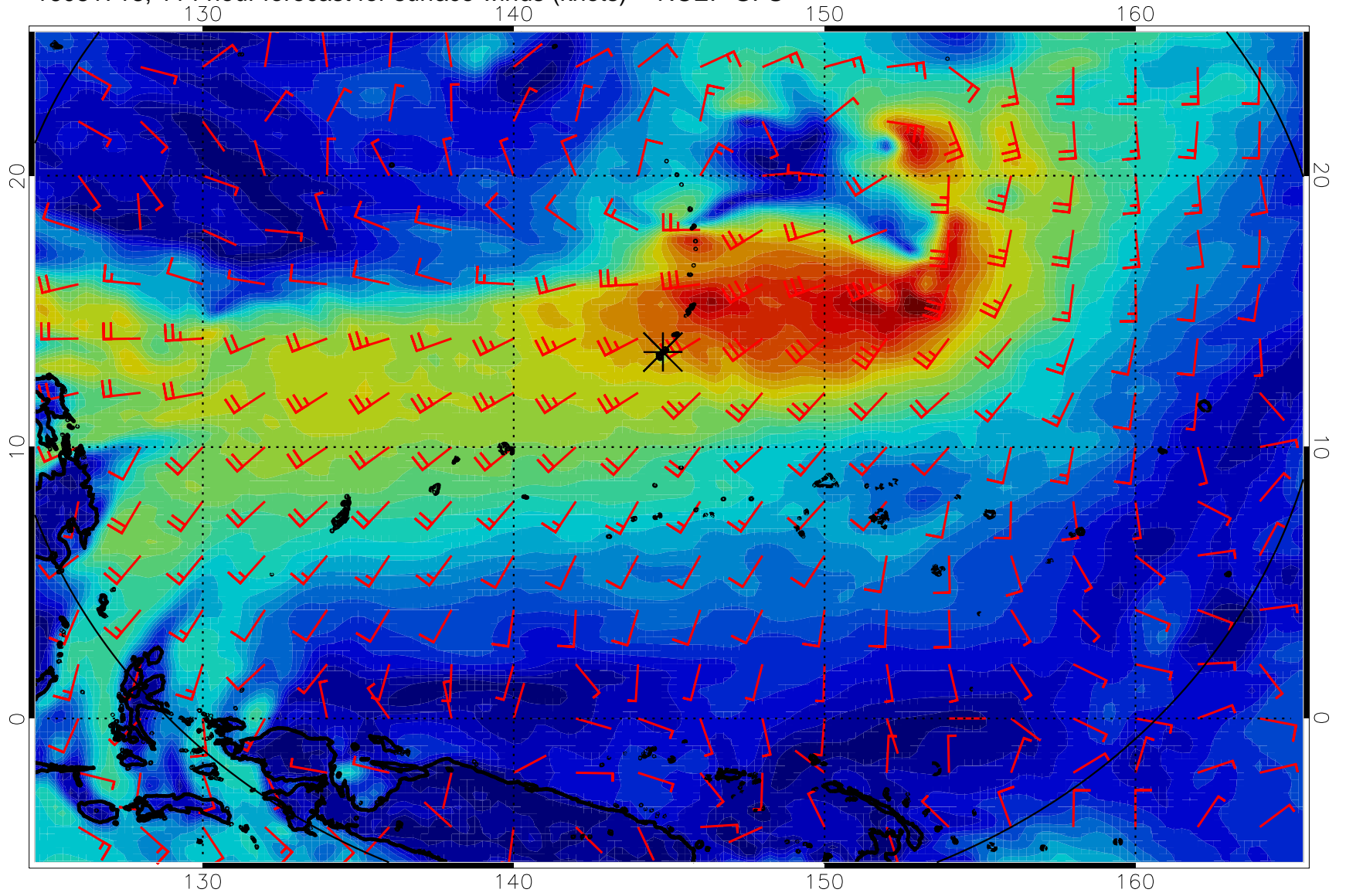
16081718, 114 hour forecast for surface winds (knots) -- NCEP GFS
