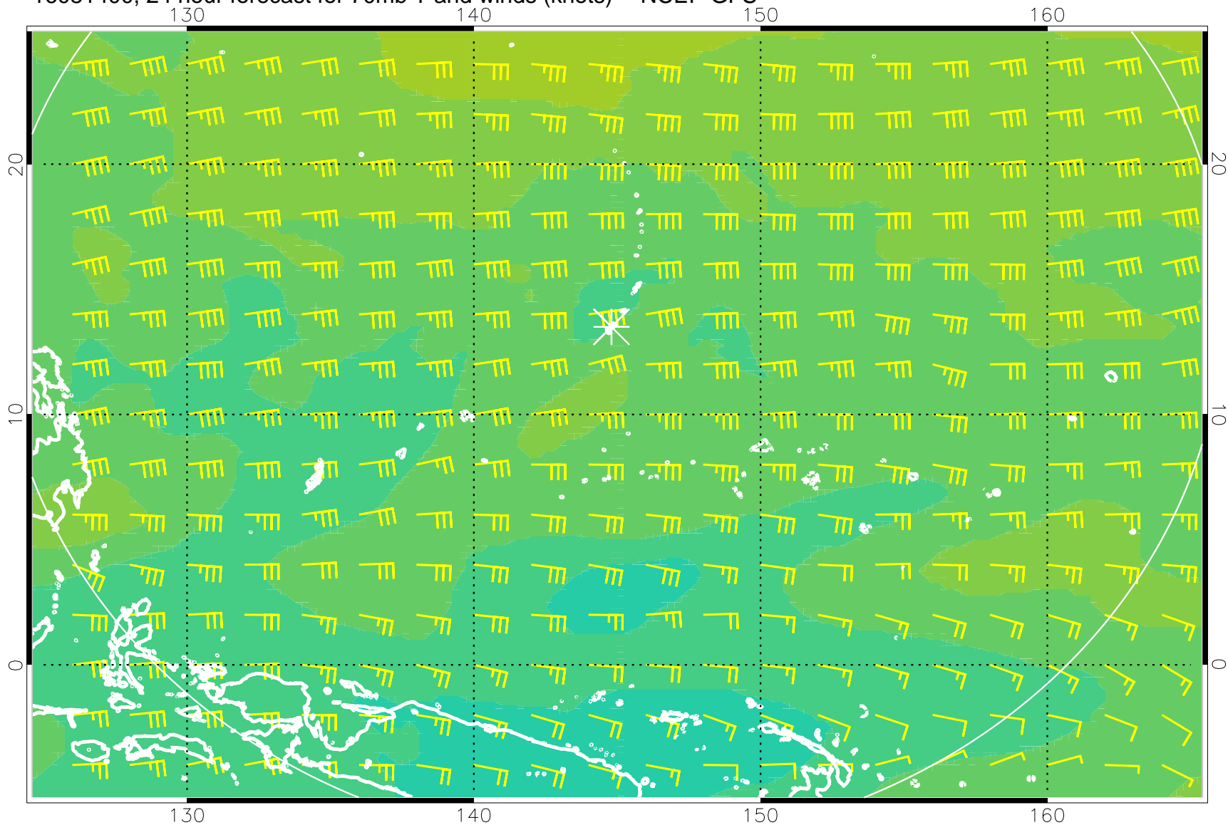
16081400, 24 hour forecast for 70mb T and winds (knots) -- NCEP GFS
