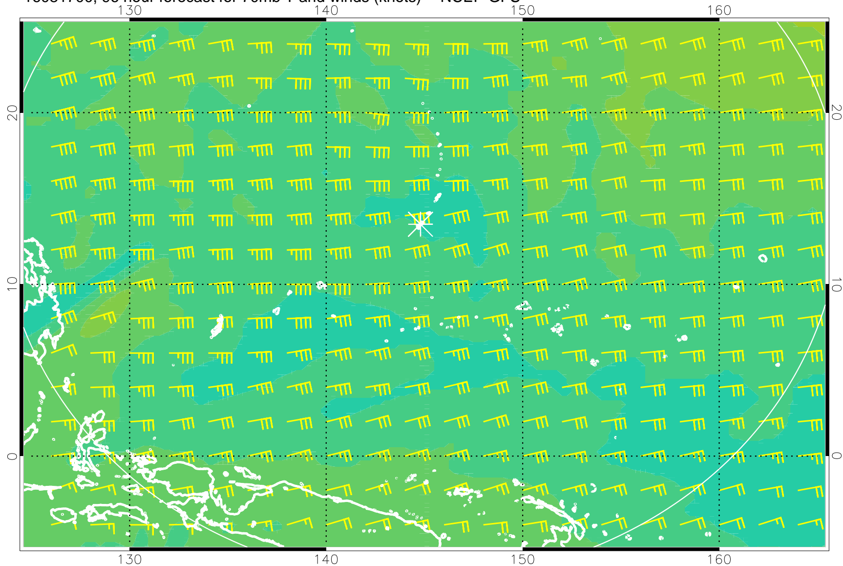
16081700, 96 hour forecast for 70mb T and winds (knots) -- NCEP GFS
