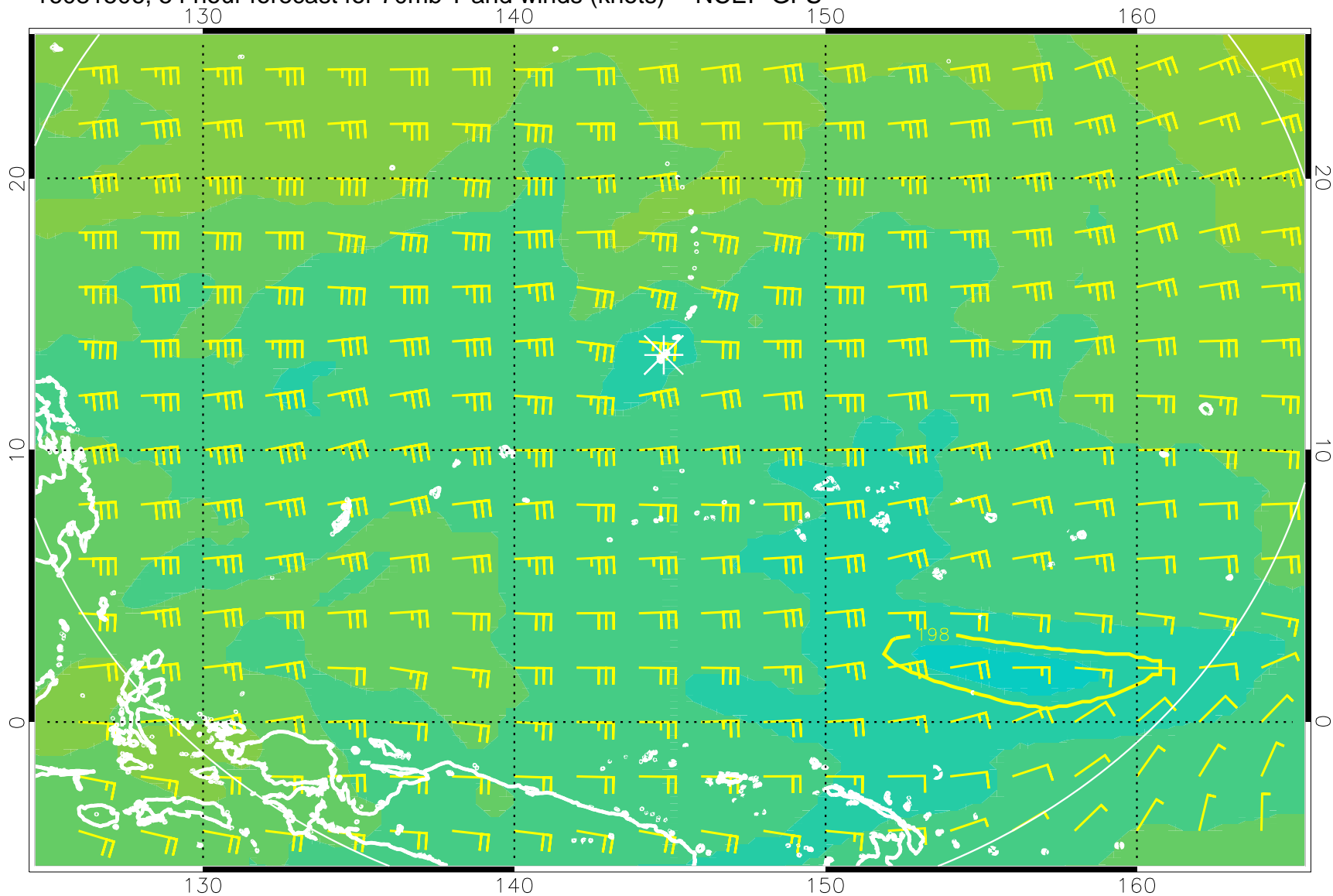
16081506, 54 hour forecast for 70mb T and winds (knots) -- NCEP GFS
