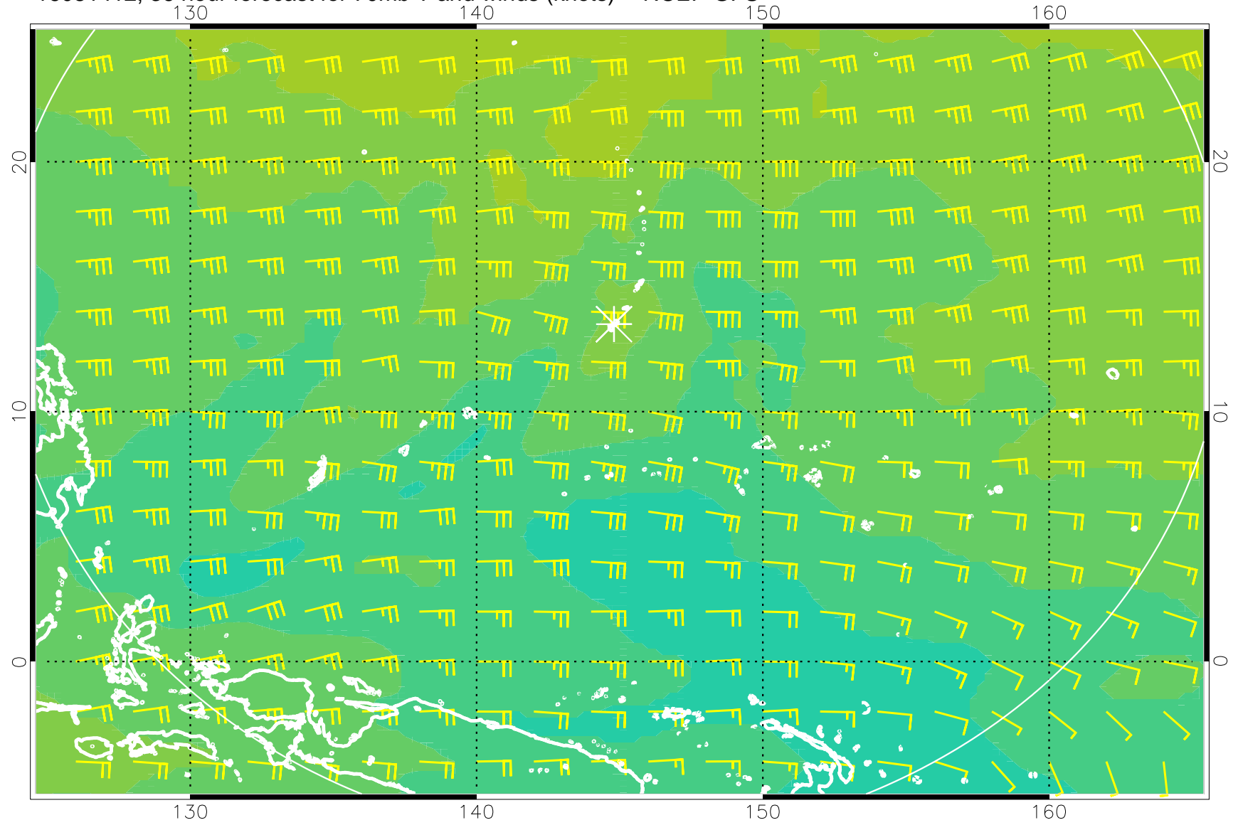
16081412, 36 hour forecast for 70mb T and winds (knots) -- NCEP GFS
