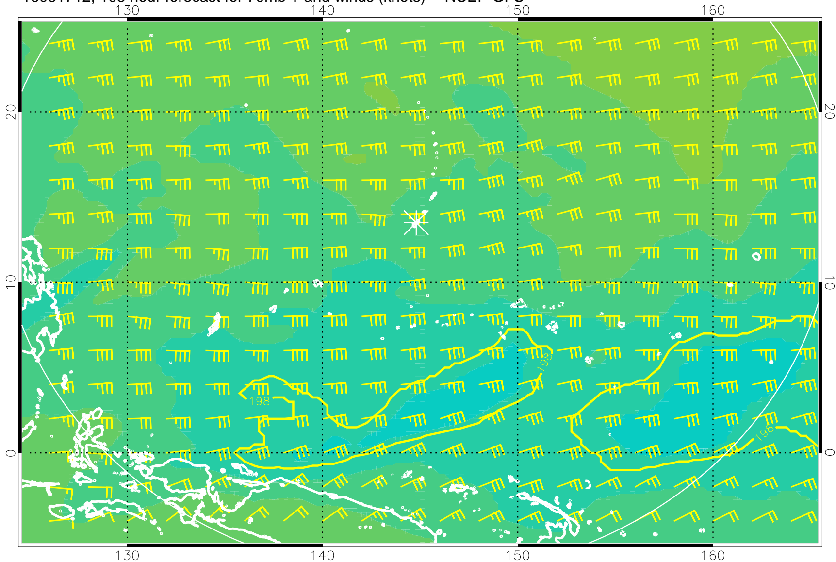
16081712, 108 hour forecast for 70mb T and winds (knots) -- NCEP GFS
