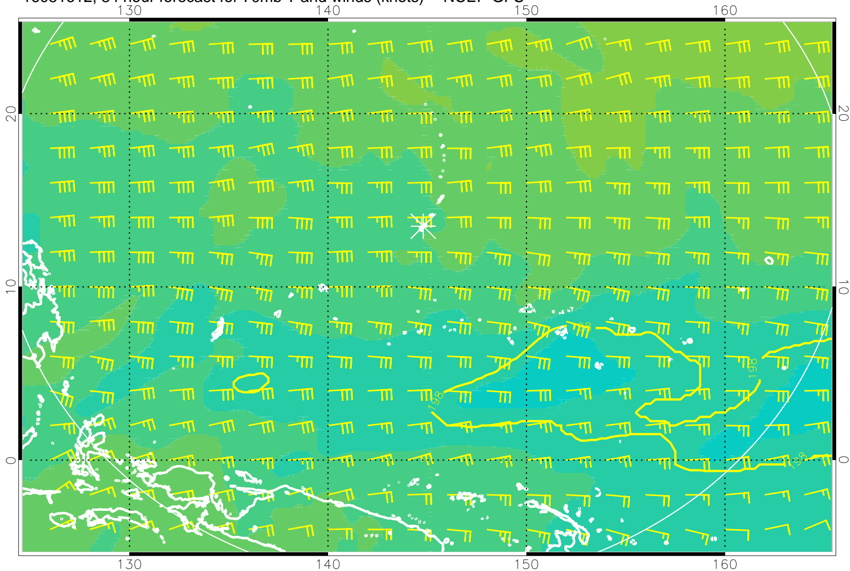
16081612, 84 hour forecast for 70mb T and winds (knots) -- NCEP GFS
