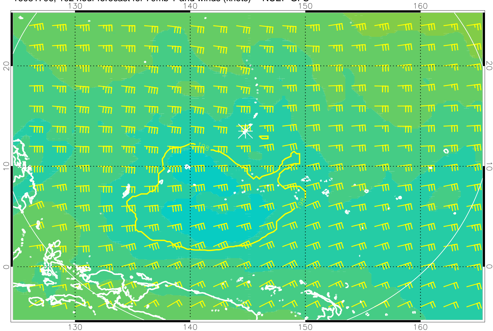
16081706, 102 hour forecast for 70mb T and winds (knots) -- NCEP GFS
