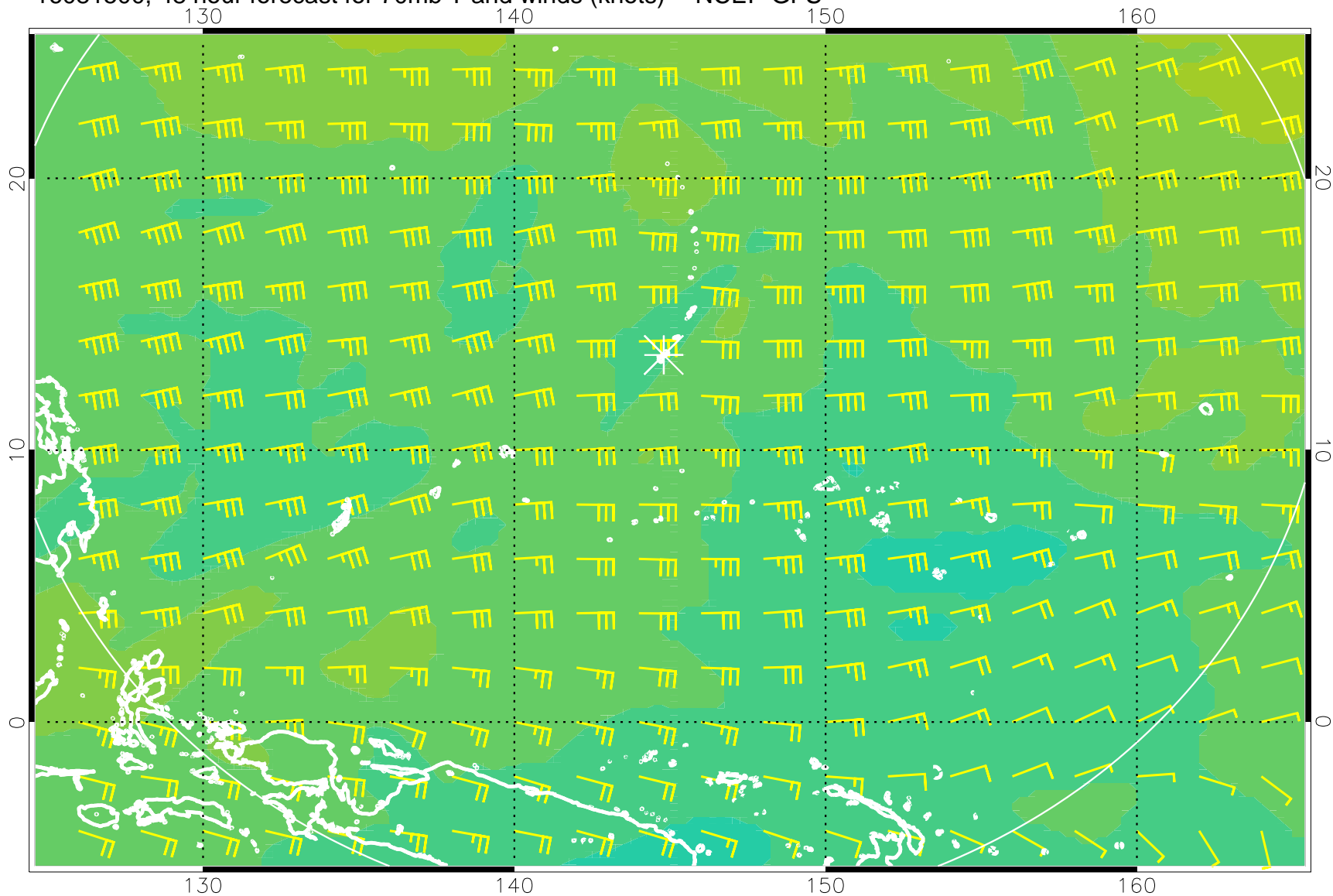
16081500, 48 hour forecast for 70mb T and winds (knots) -- NCEP GFS
