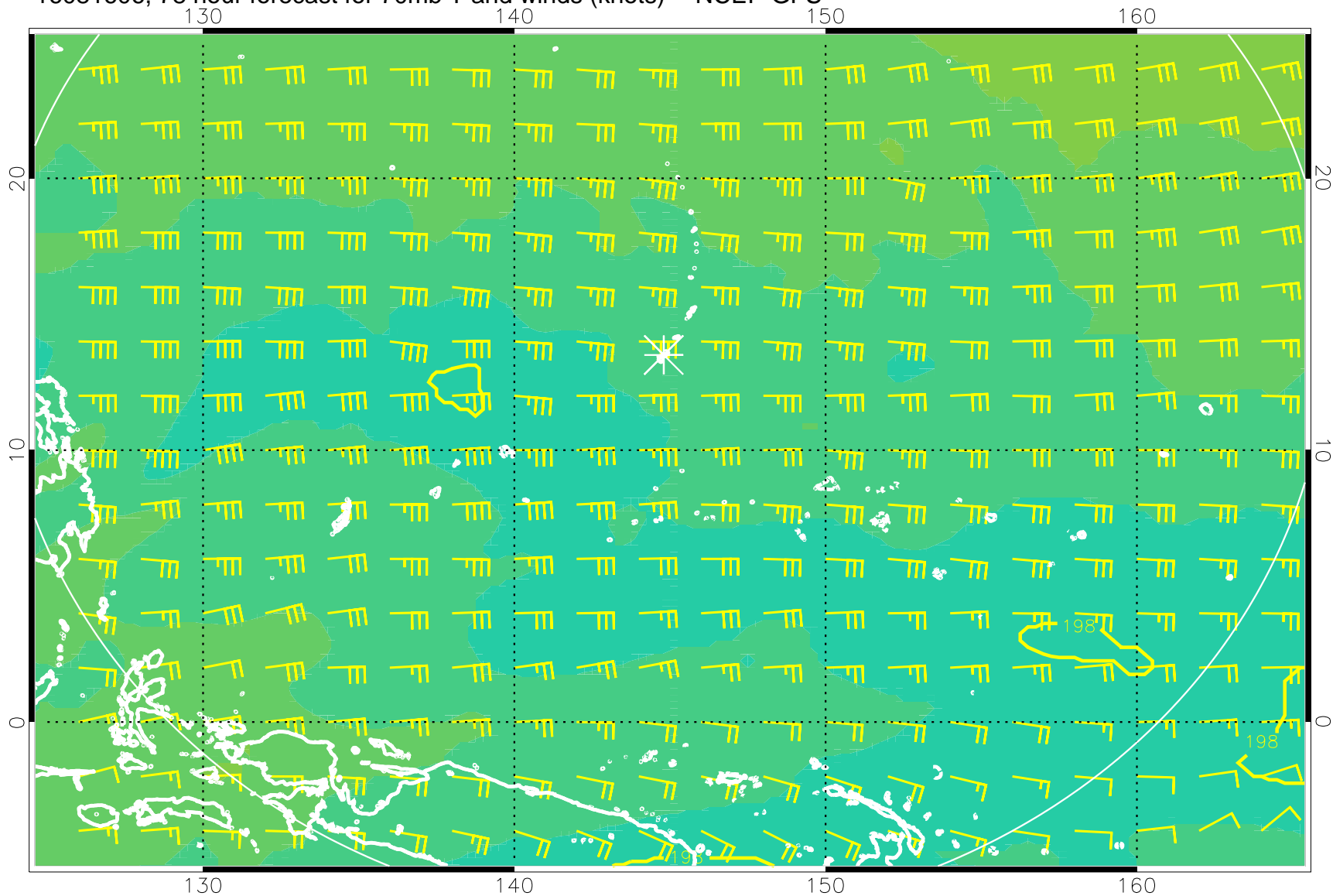
16081606, 78 hour forecast for 70mb T and winds (knots) -- NCEP GFS
