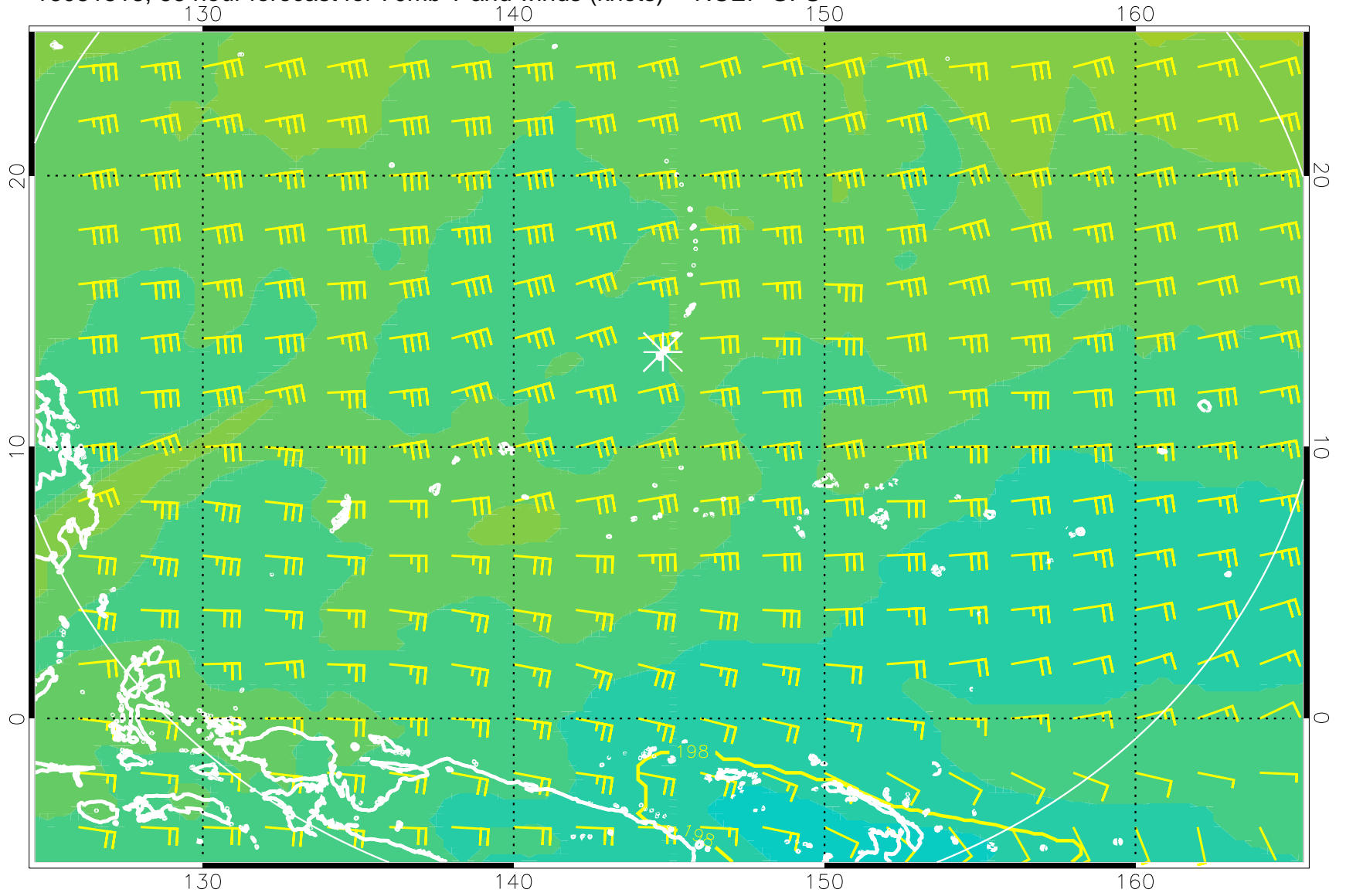
16081518, 66 hour forecast for 70mb T and winds (knots) -- NCEP GFS
