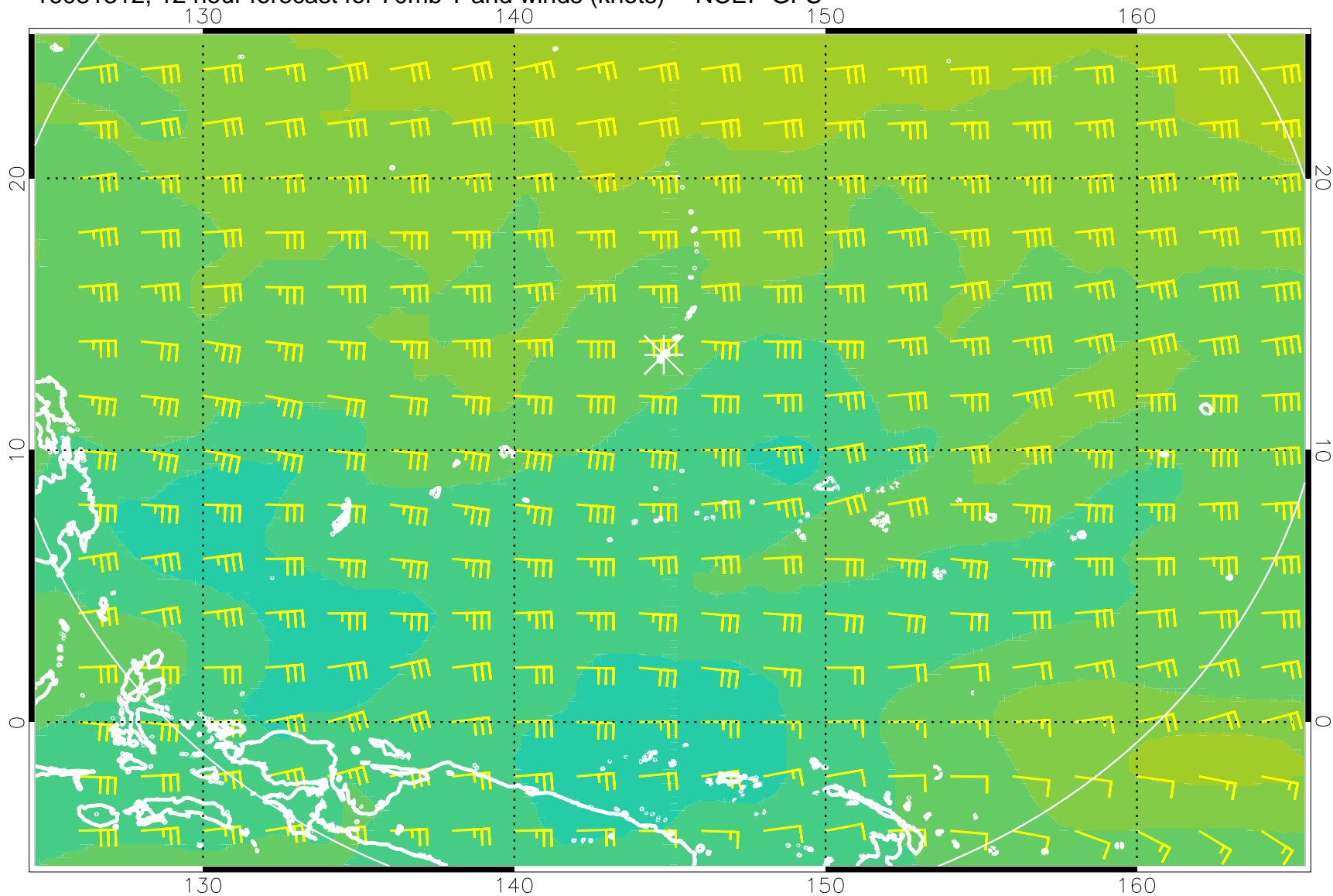
16081312, 12 hour forecast for 70mb T and winds (knots) -- NCEP GFS
