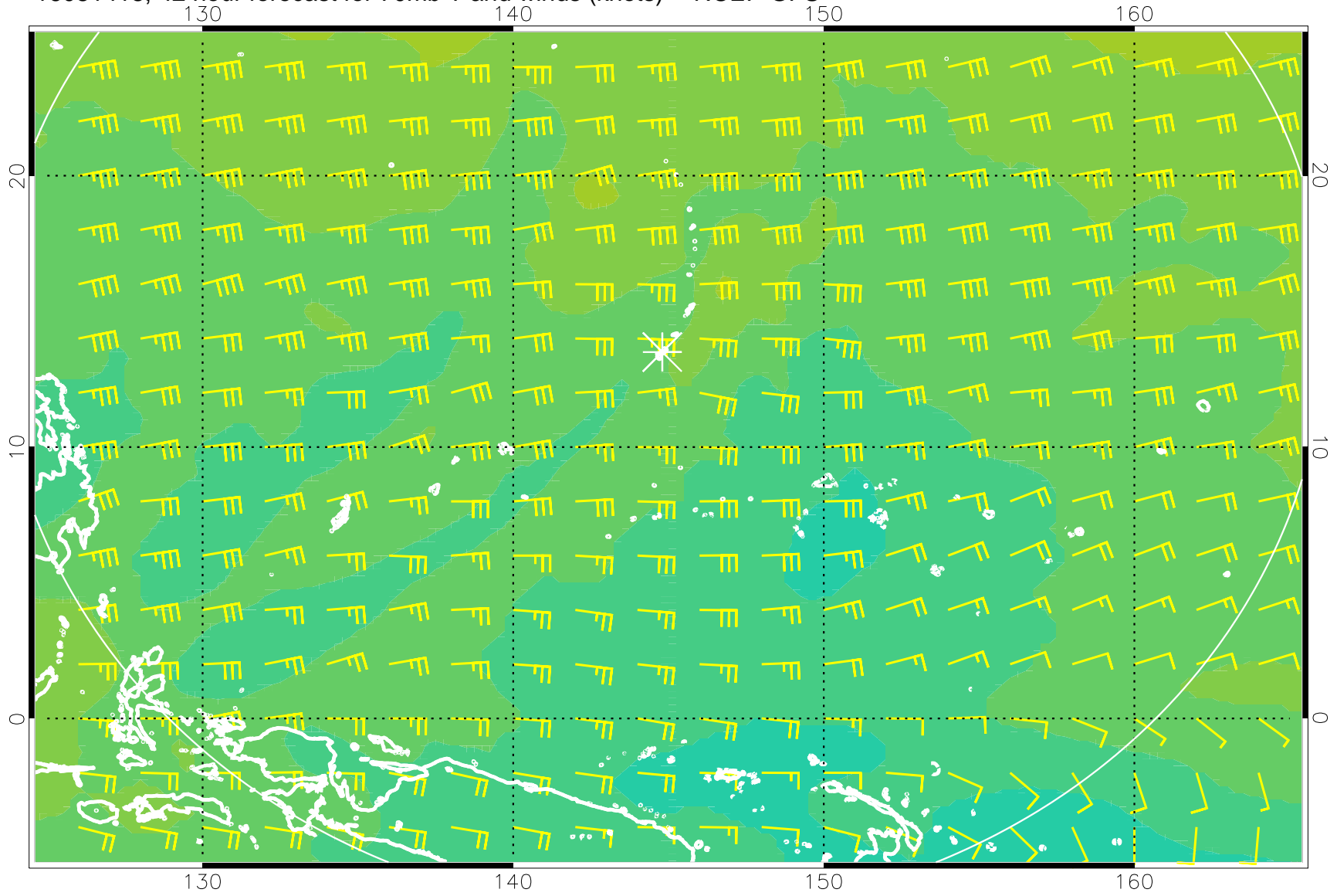
16081418, 42 hour forecast for 70mb T and winds (knots) -- NCEP GFS
