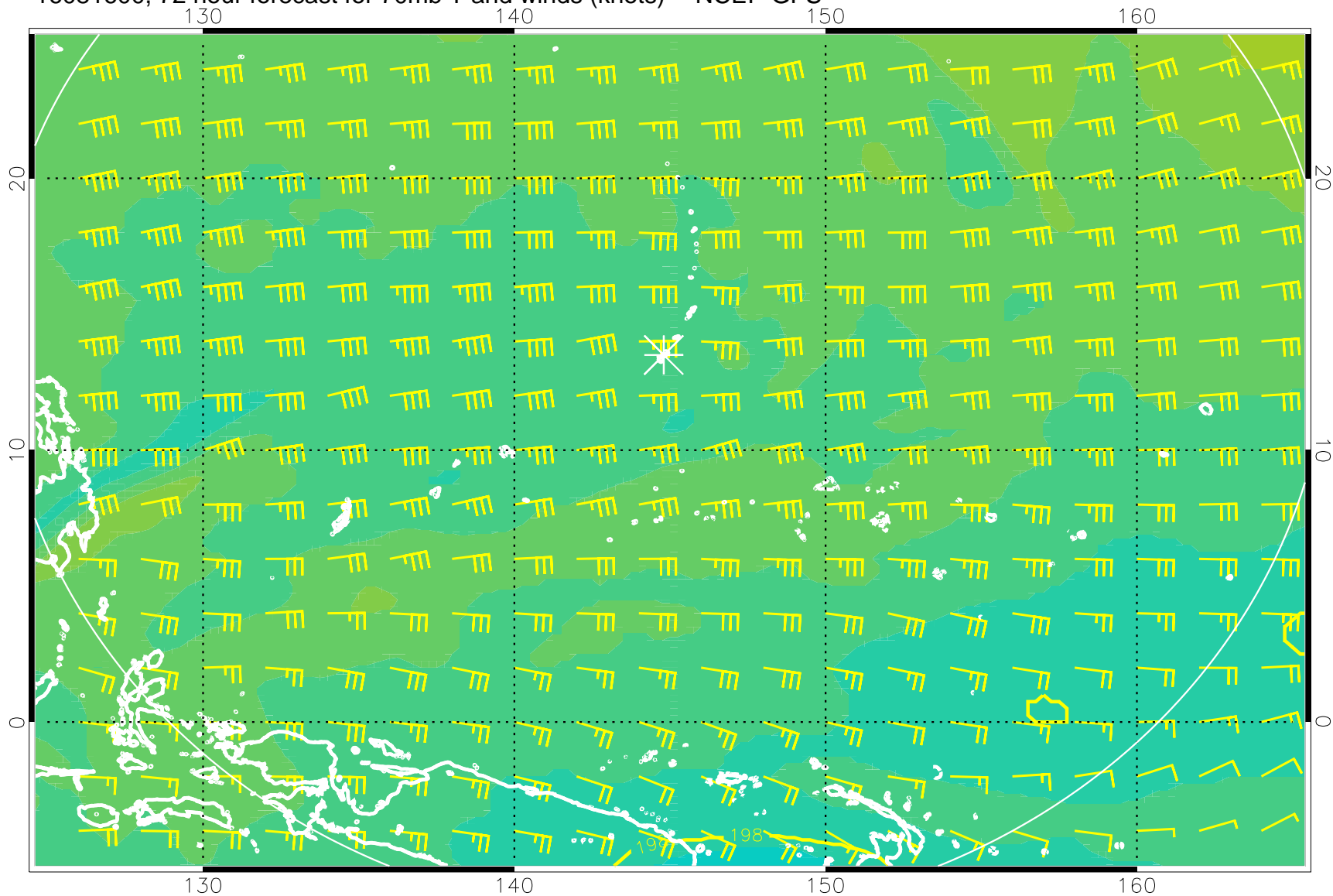
16081600, 72 hour forecast for 70mb T and winds (knots) -- NCEP GFS
