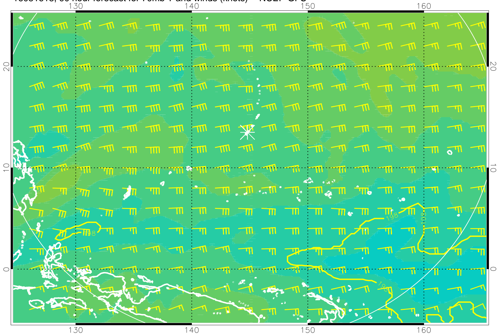
16081618, 90 hour forecast for 70mb T and winds (knots) -- NCEP GFS
