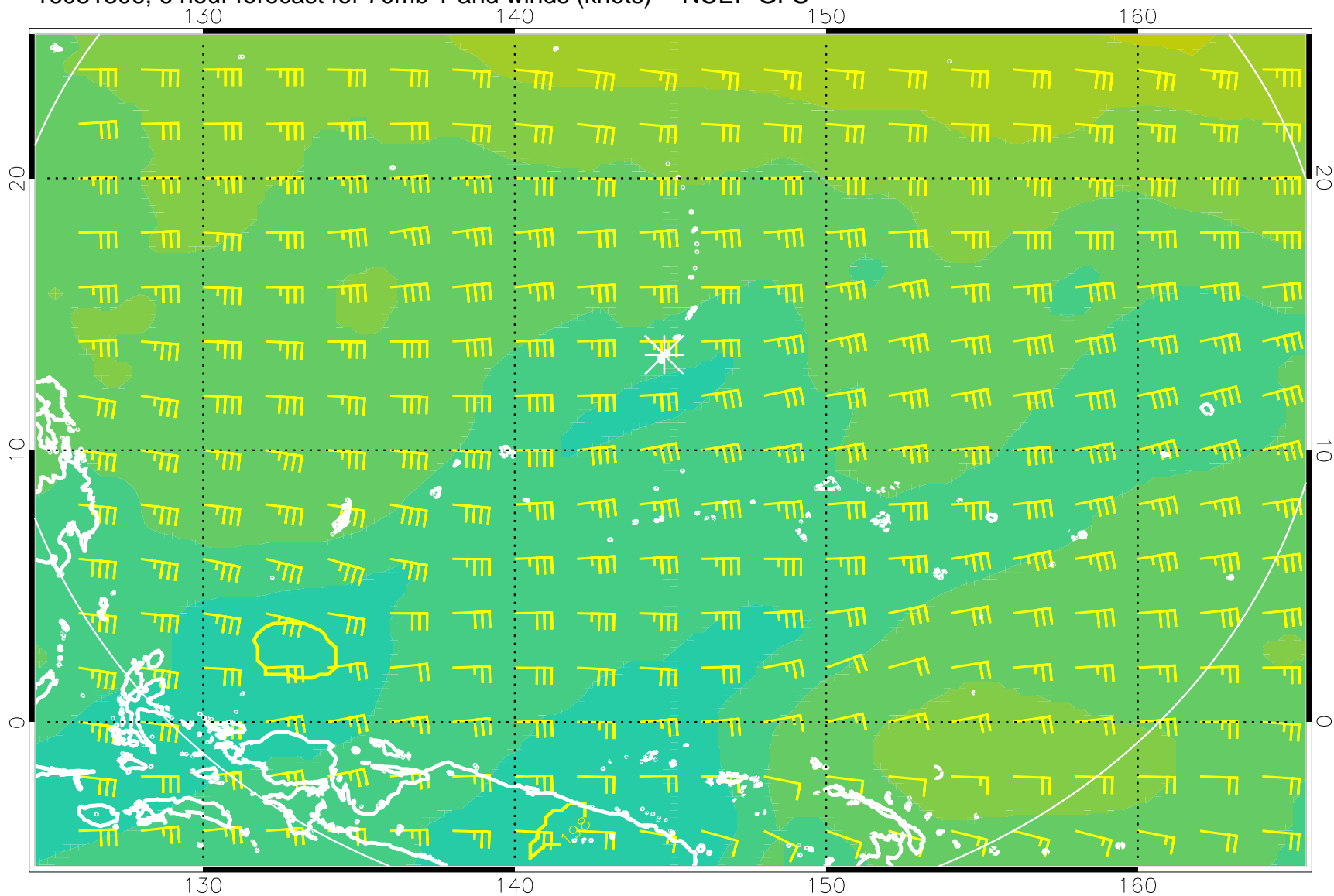
16081306, 6 hour forecast for 70mb T and winds (knots) -- NCEP GFS
