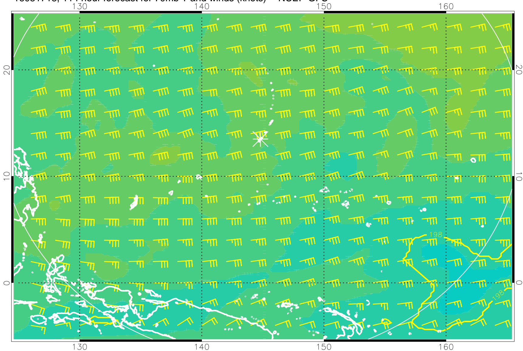
16081718, 114 hour forecast for 70mb T and winds (knots) -- NCEP GFS
