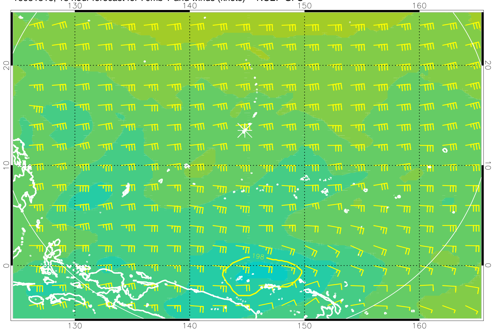
16081318, 18 hour forecast for 70mb T and winds (knots) -- NCEP GFS
