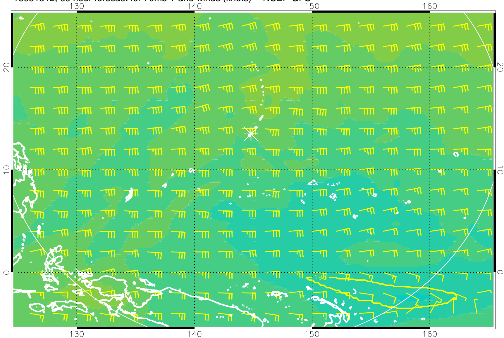
16081512, 60 hour forecast for 70mb T and winds (knots) -- NCEP GFS
