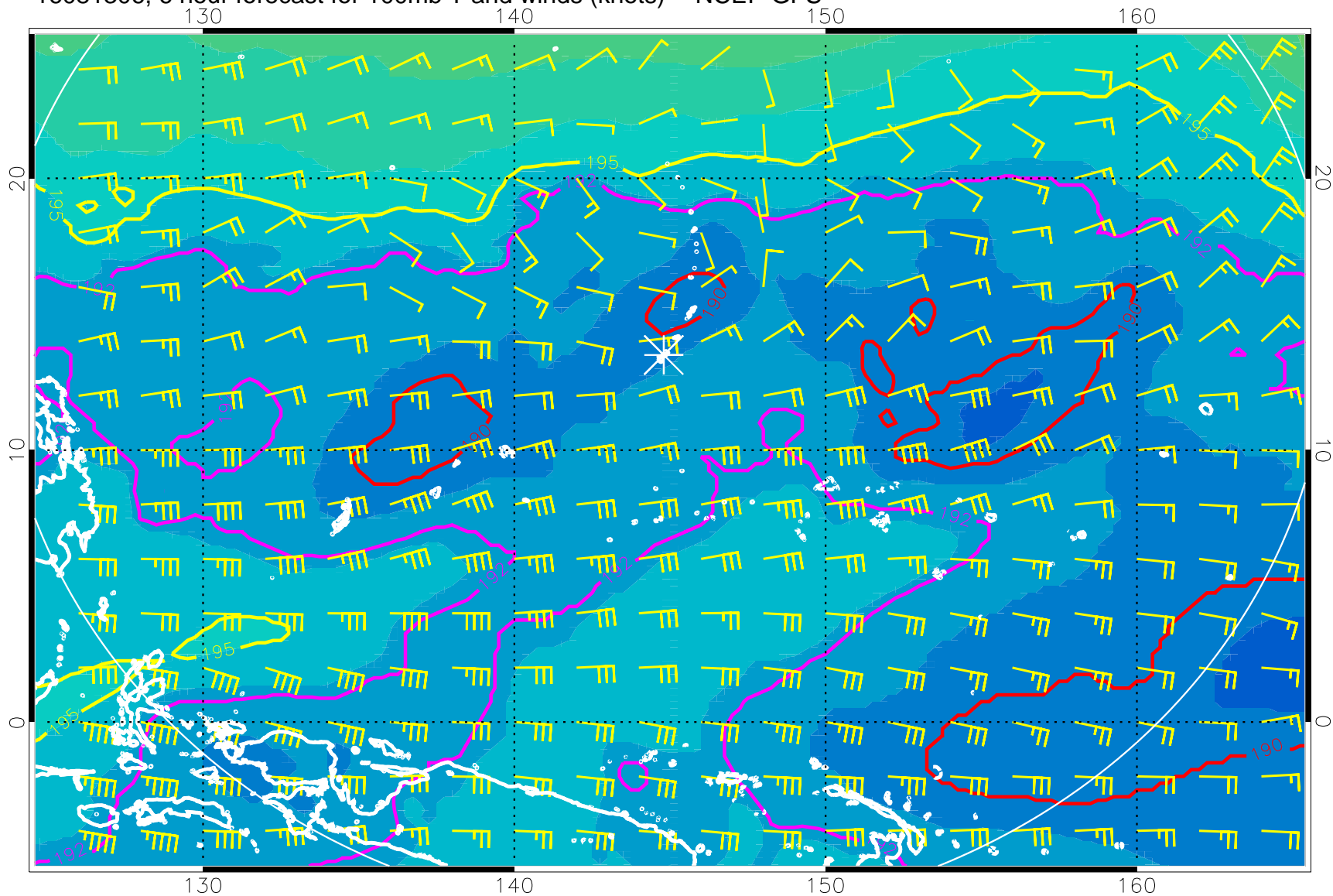
16081306, 6 hour forecast for 100mb T and winds (knots) -- NCEP GFS
