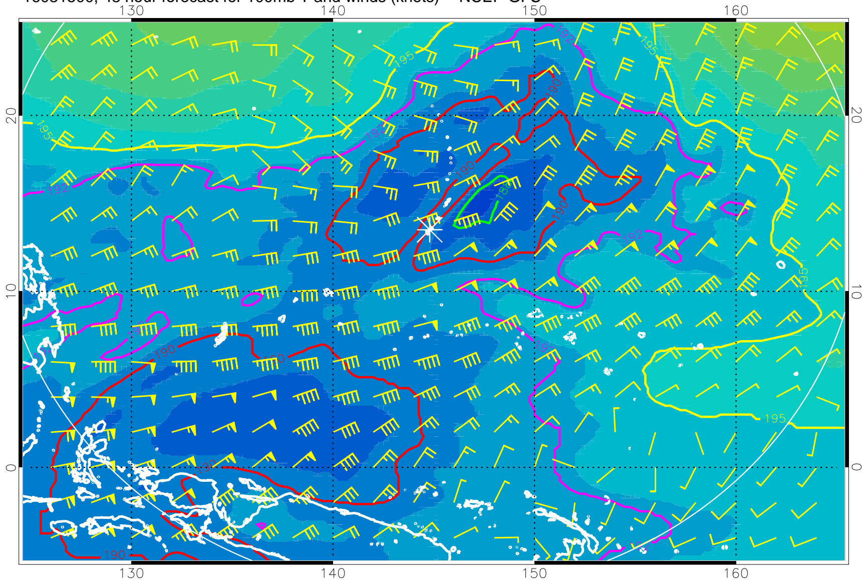
16081500, 48 hour forecast for 100mb T and winds (knots) -- NCEP GFS
