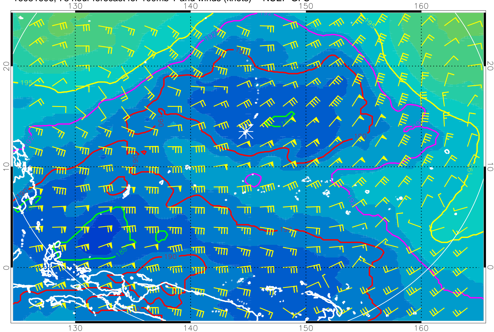
16081606, 78 hour forecast for 100mb T and winds (knots) -- NCEP GFS
