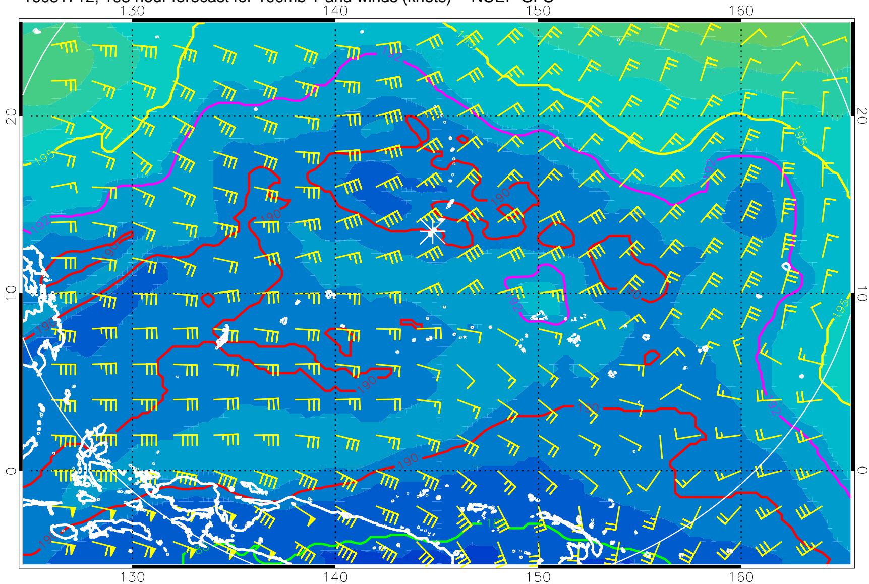
16081712, 108 hour forecast for 100mb T and winds (knots) -- NCEP GFS
