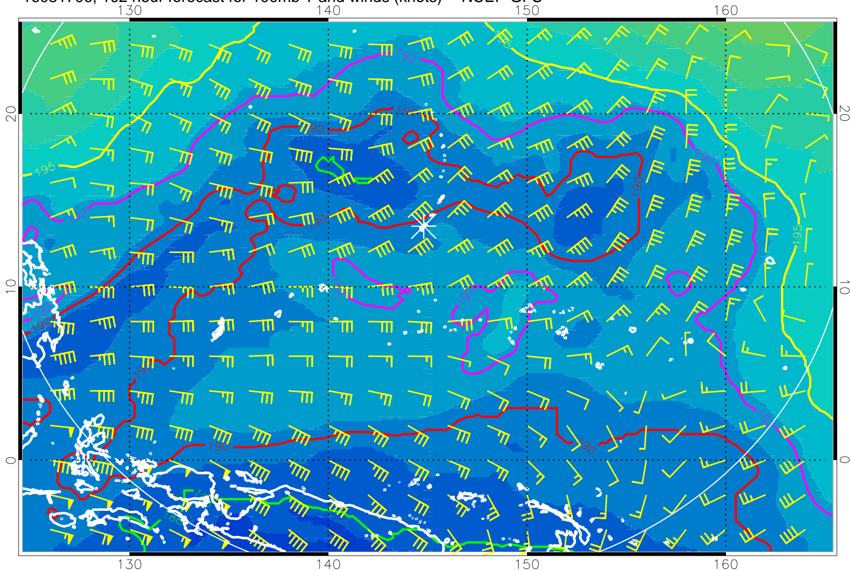
16081706, 102 hour forecast for 100mb T and winds (knots) -- NCEP GFS
