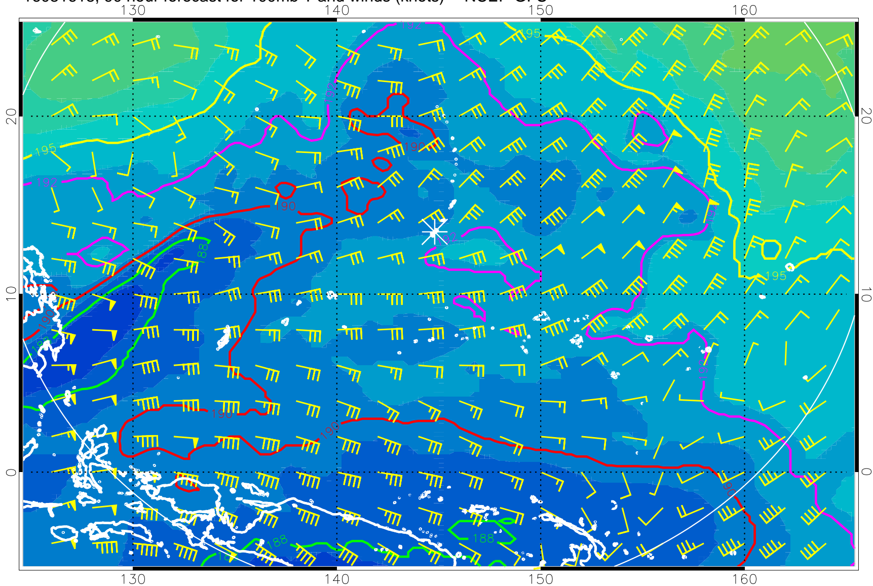
16081618, 90 hour forecast for 100mb T and winds (knots) -- NCEP GFS
