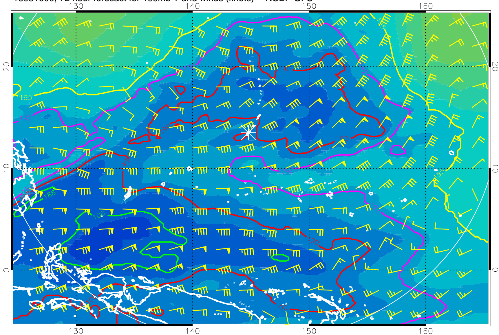
16081600, 72 hour forecast for 100mb T and winds (knots) -- NCEP GFS
