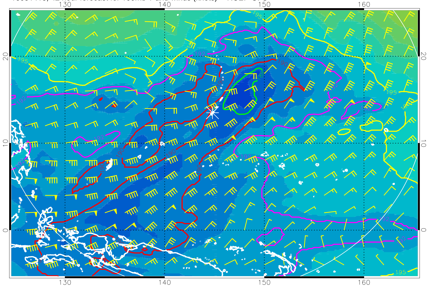
16081418, 42 hour forecast for 100mb T and winds (knots) -- NCEP GFS
