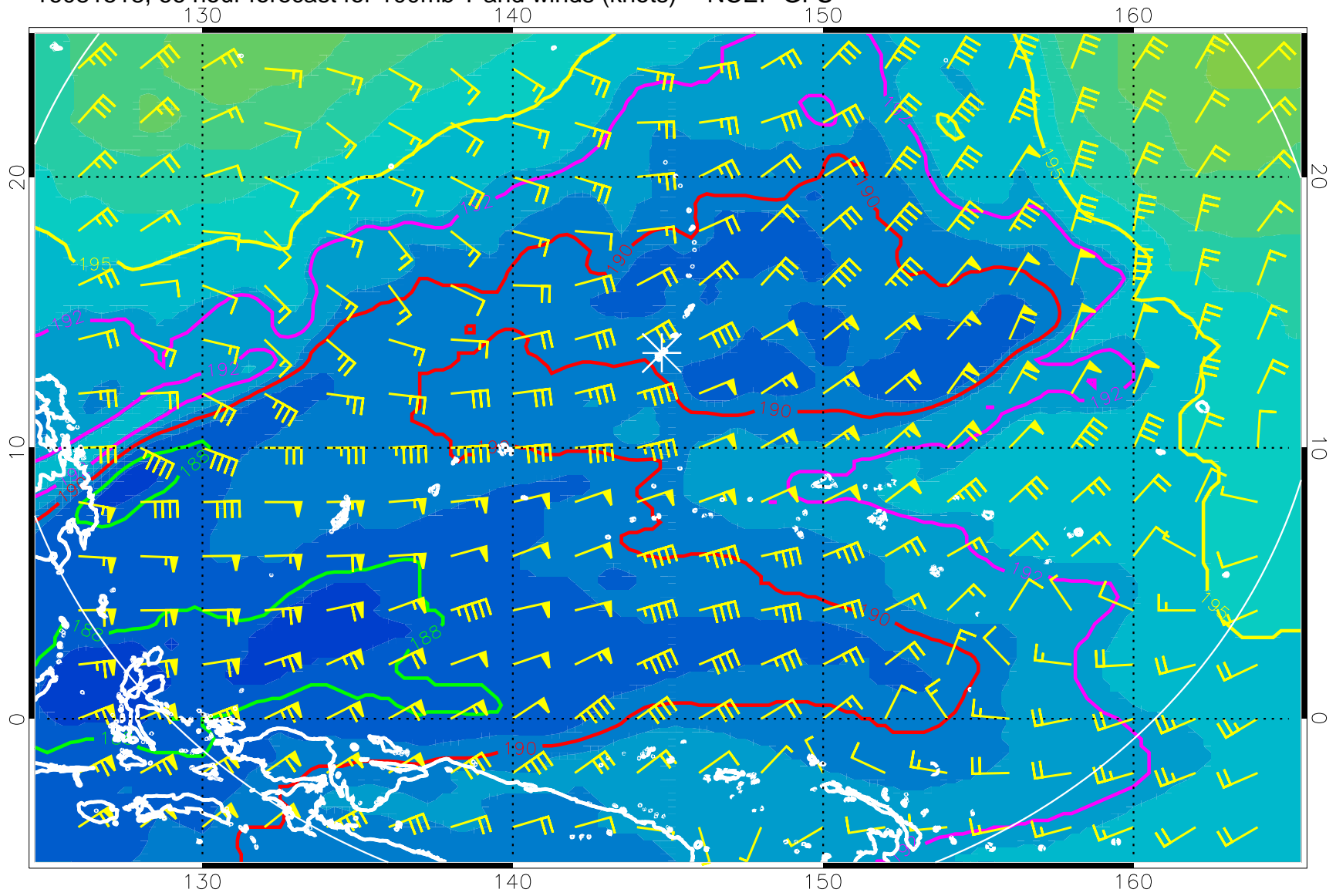
16081518, 66 hour forecast for 100mb T and winds (knots) -- NCEP GFS
