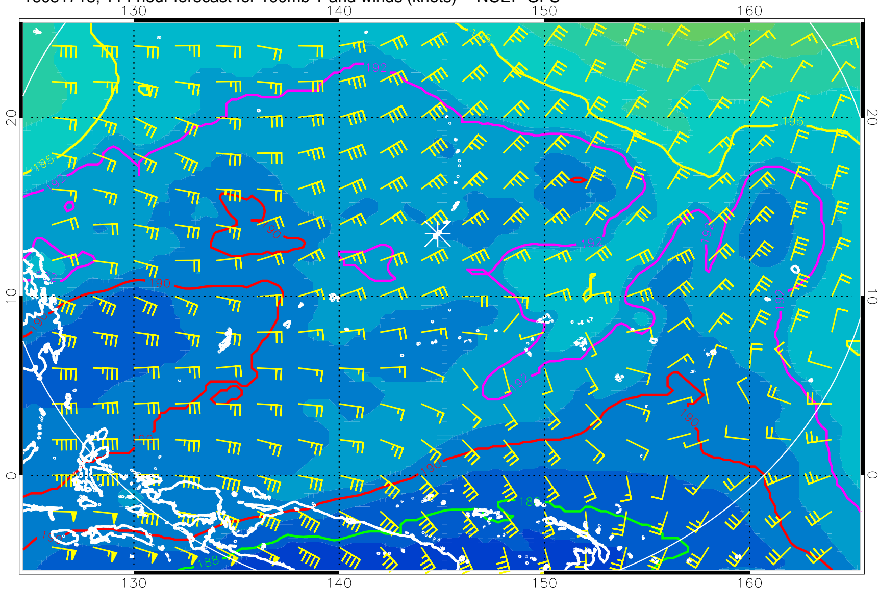
16081718, 114 hour forecast for 100mb T and winds (knots) -- NCEP GFS
