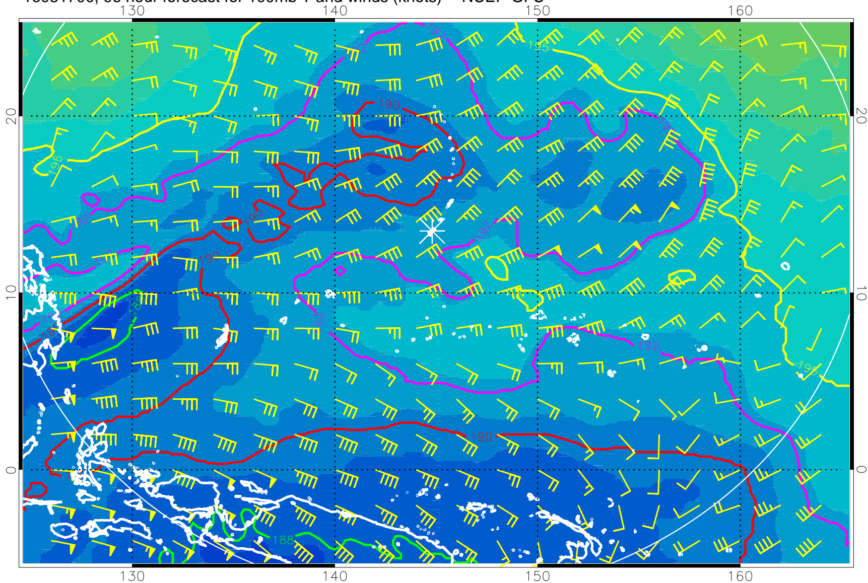
16081700, 96 hour forecast for 100mb T and winds (knots) -- NCEP GFS
