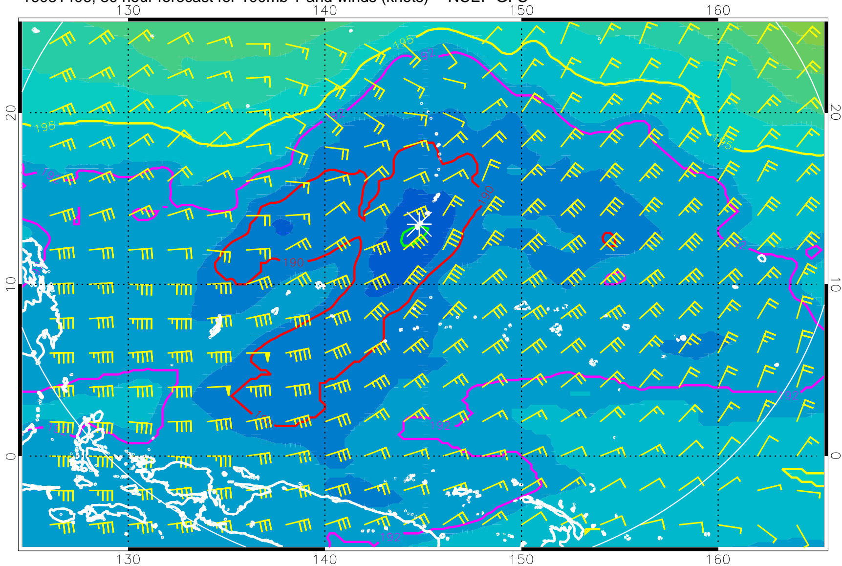
16081406, 30 hour forecast for 100mb T and winds (knots) -- NCEP GFS
