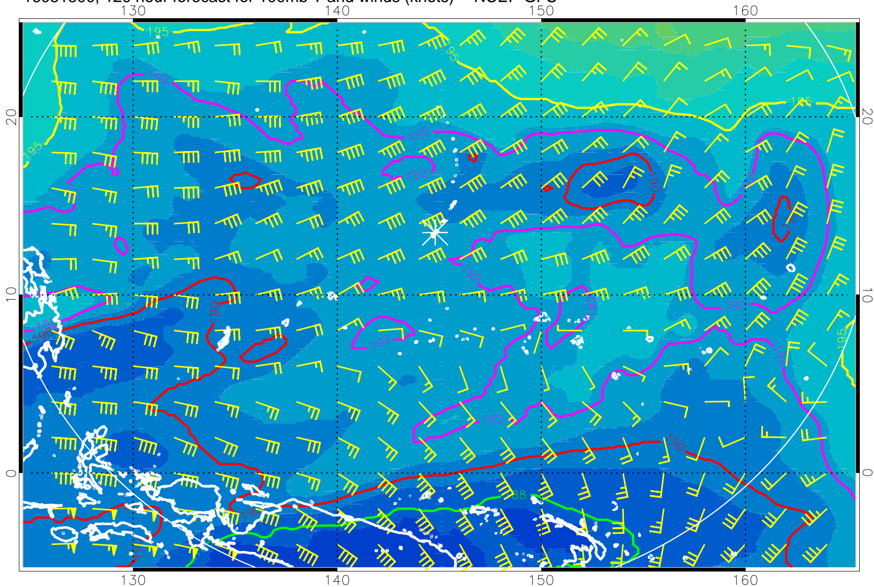
16081800, 120 hour forecast for 100mb T and winds (knots) -- NCEP GFS
