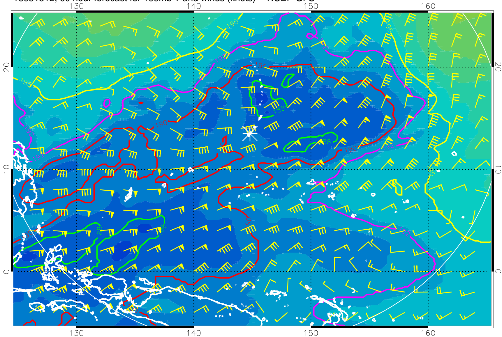
16081512, 60 hour forecast for 100mb T and winds (knots) -- NCEP GFS
