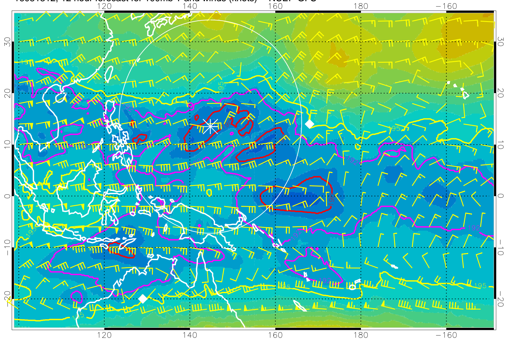
16081312, 12 hour forecast for 100mb T and winds (knots) -- NCEP GFS
