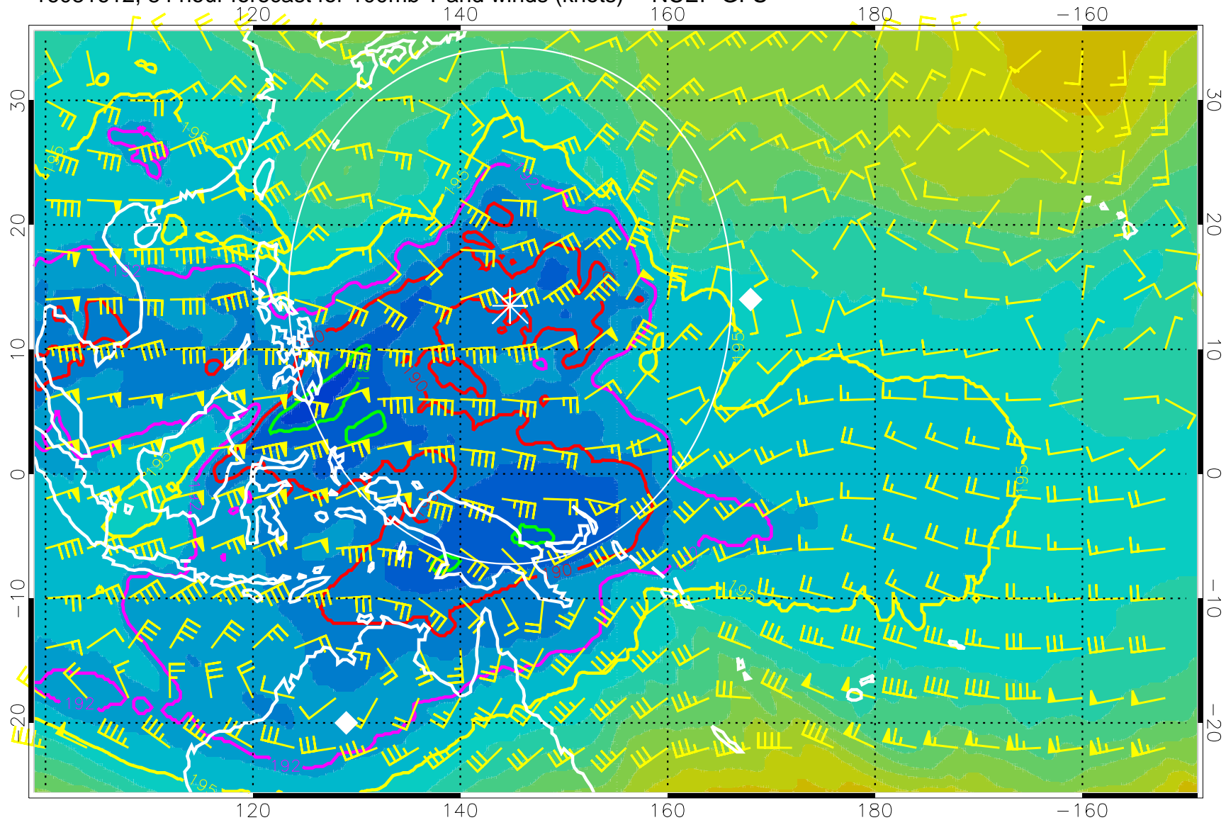
16081612, 84 hour forecast for 100mb T and winds (knots) -- NCEP GFS
