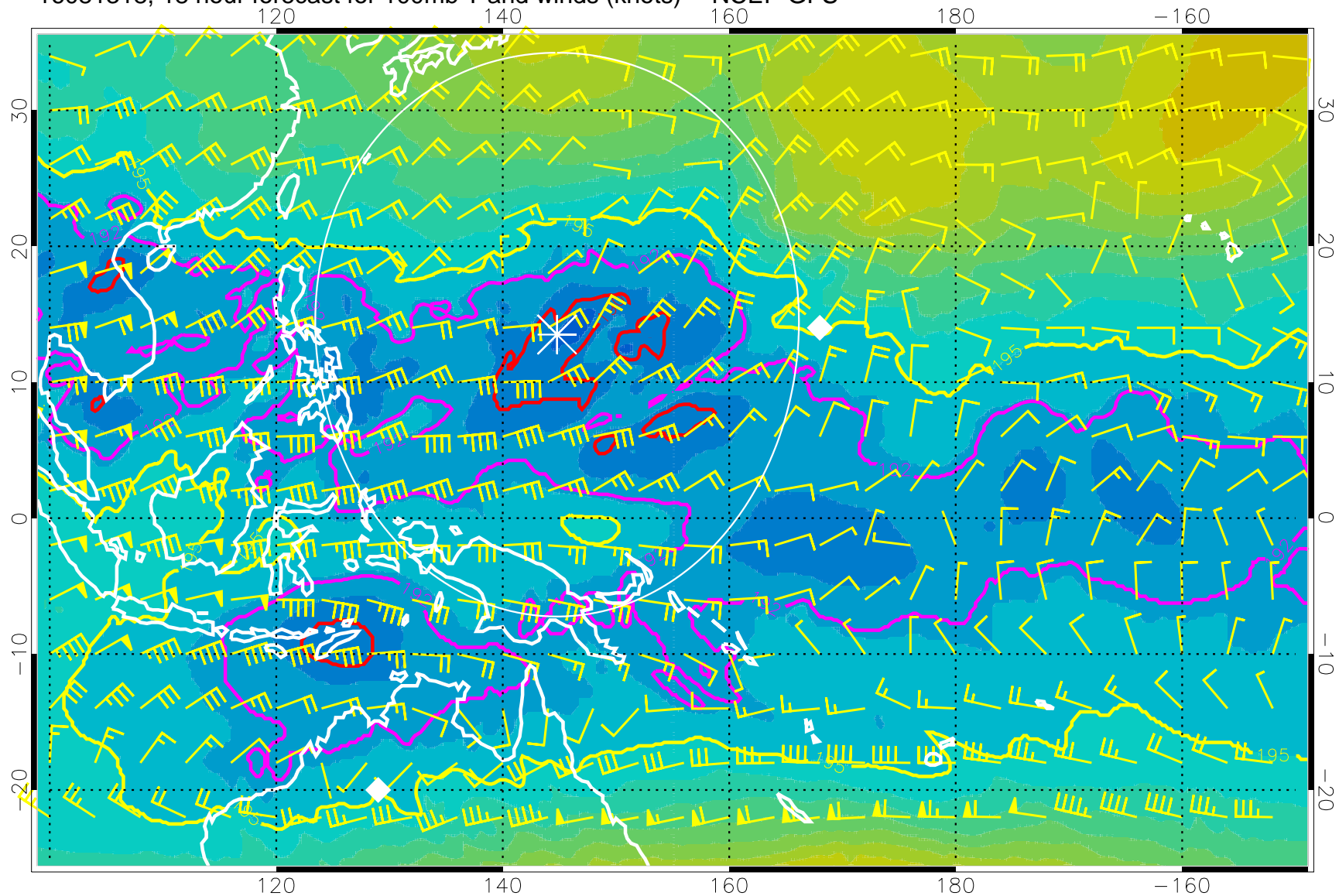
16081318, 18 hour forecast for 100mb T and winds (knots) -- NCEP GFS
