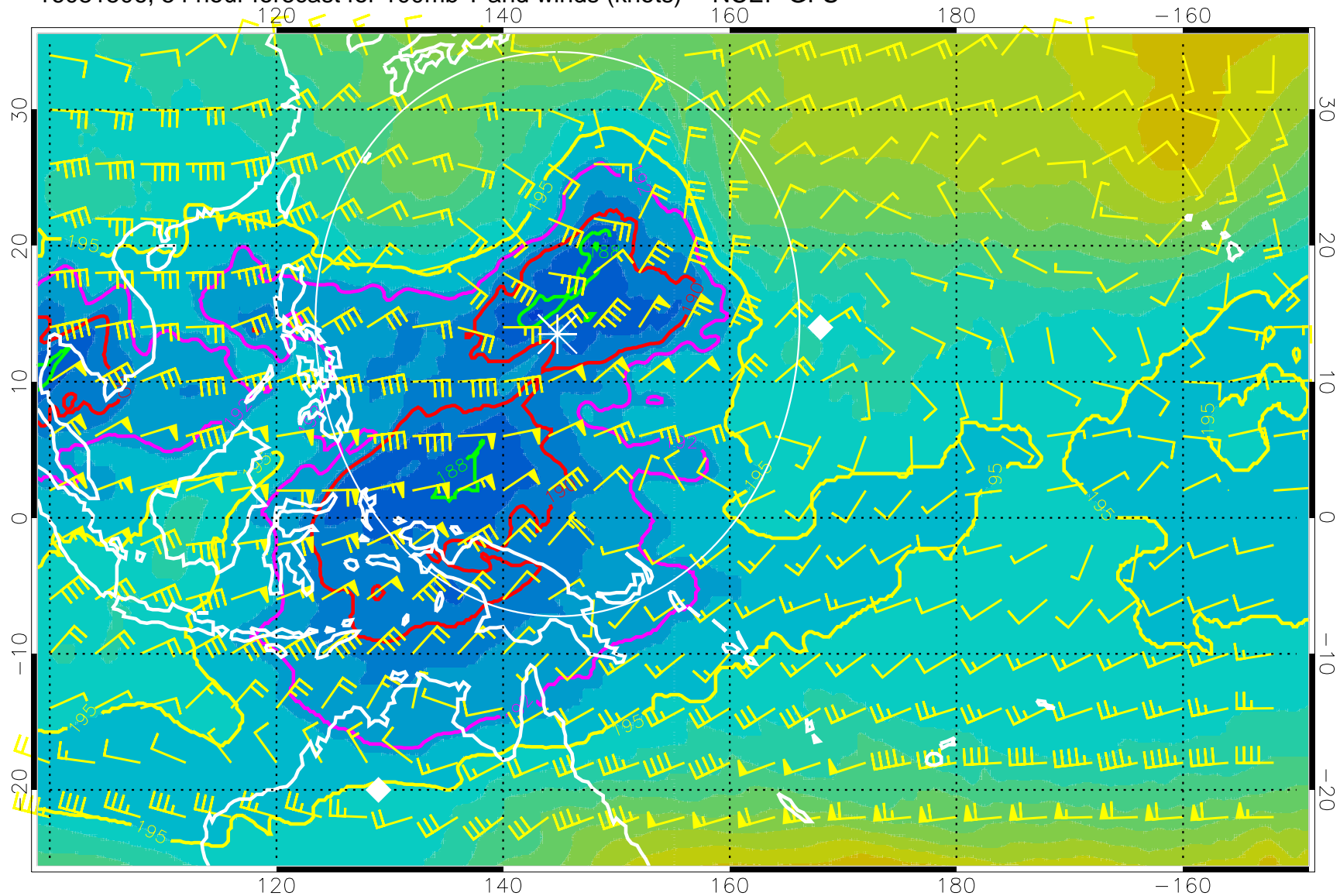
16081506, 54 hour forecast for 100mb T and winds (knots) -- NCEP GFS
