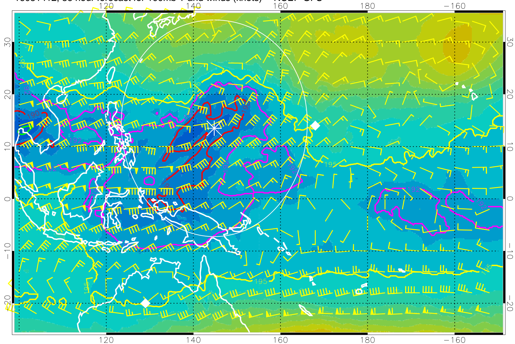
16081412, 36 hour forecast for 100mb T and winds (knots) -- NCEP GFS
