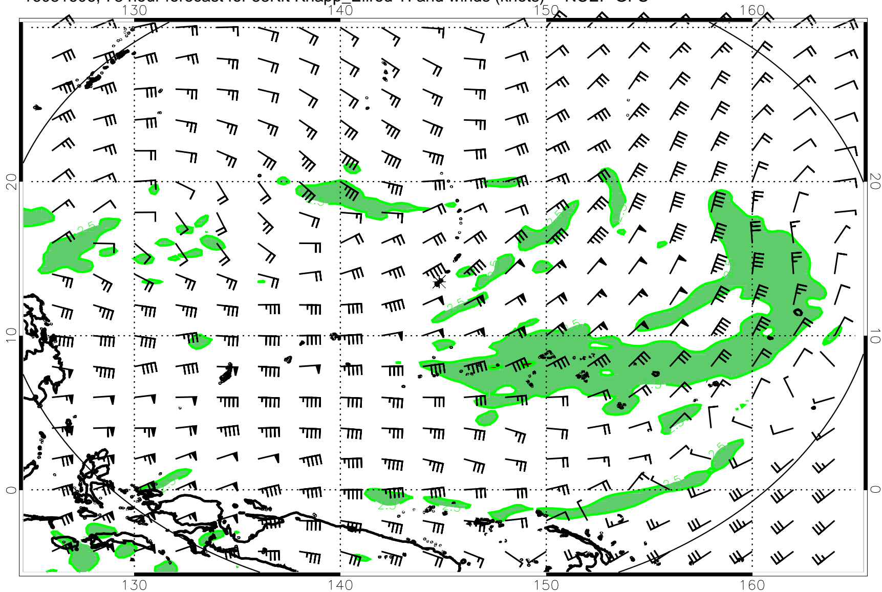
16081606, 78 hour forecast for 53Kft Knapp_Ellrod TI and winds (knots) -- NCEP GFS
