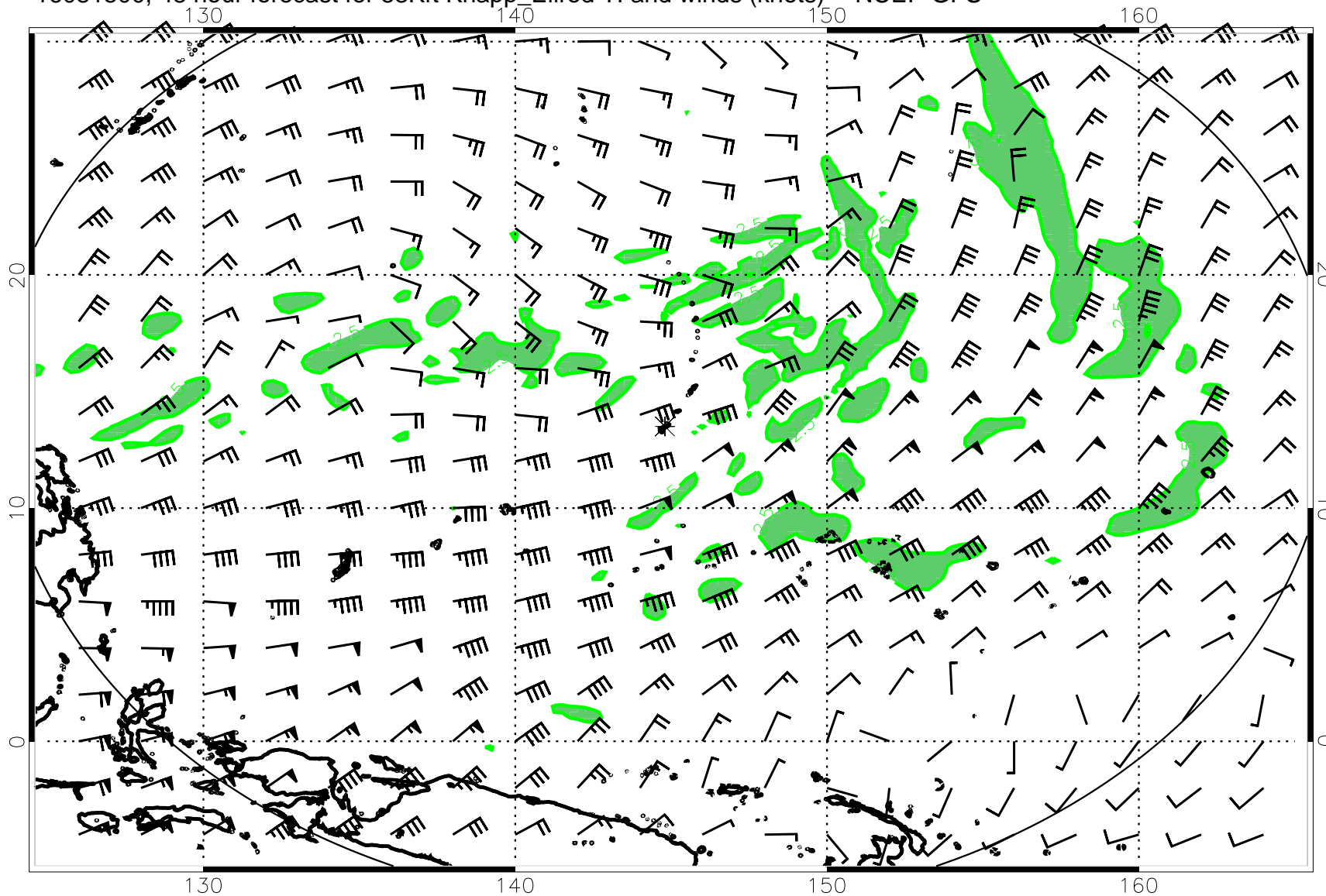
16081500, 48 hour forecast for 53Kft Knapp_Ellrod TI and winds (knots) -- NCEP GFS
