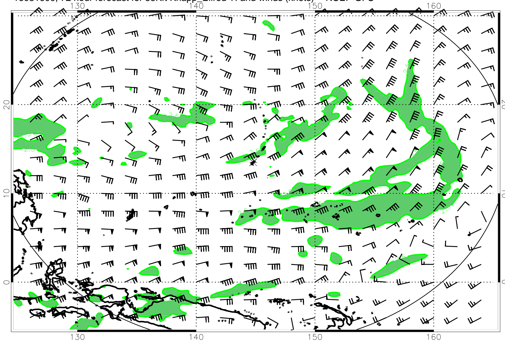
16081600, 72 hour forecast for 53Kft Knapp_Ellrod TI and winds (knots) -- NCEP GFS
