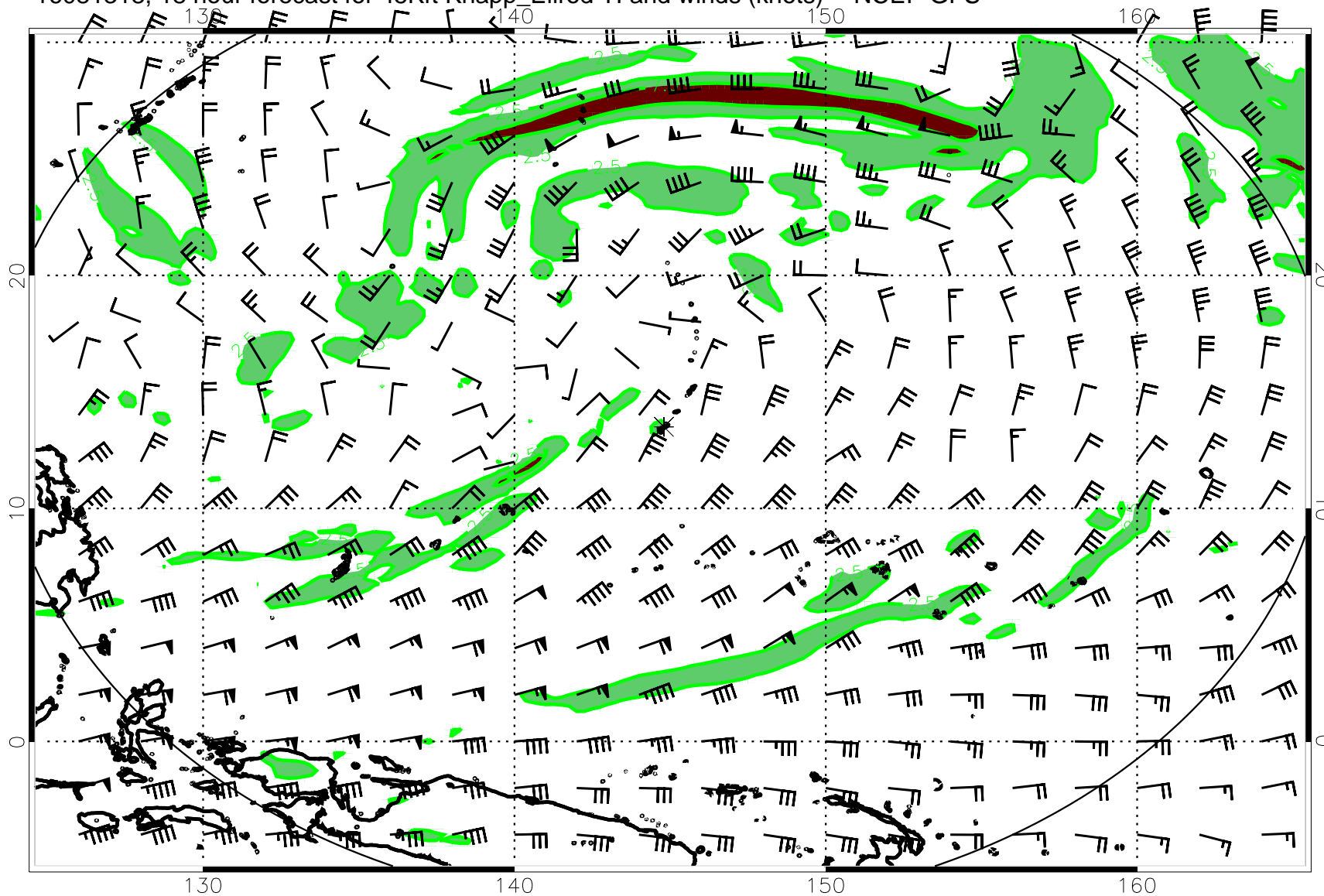
16081318, 18 hour forecast for 45Kft Knapp_Ellrod TI and winds (knots) -- NCEP GFS
