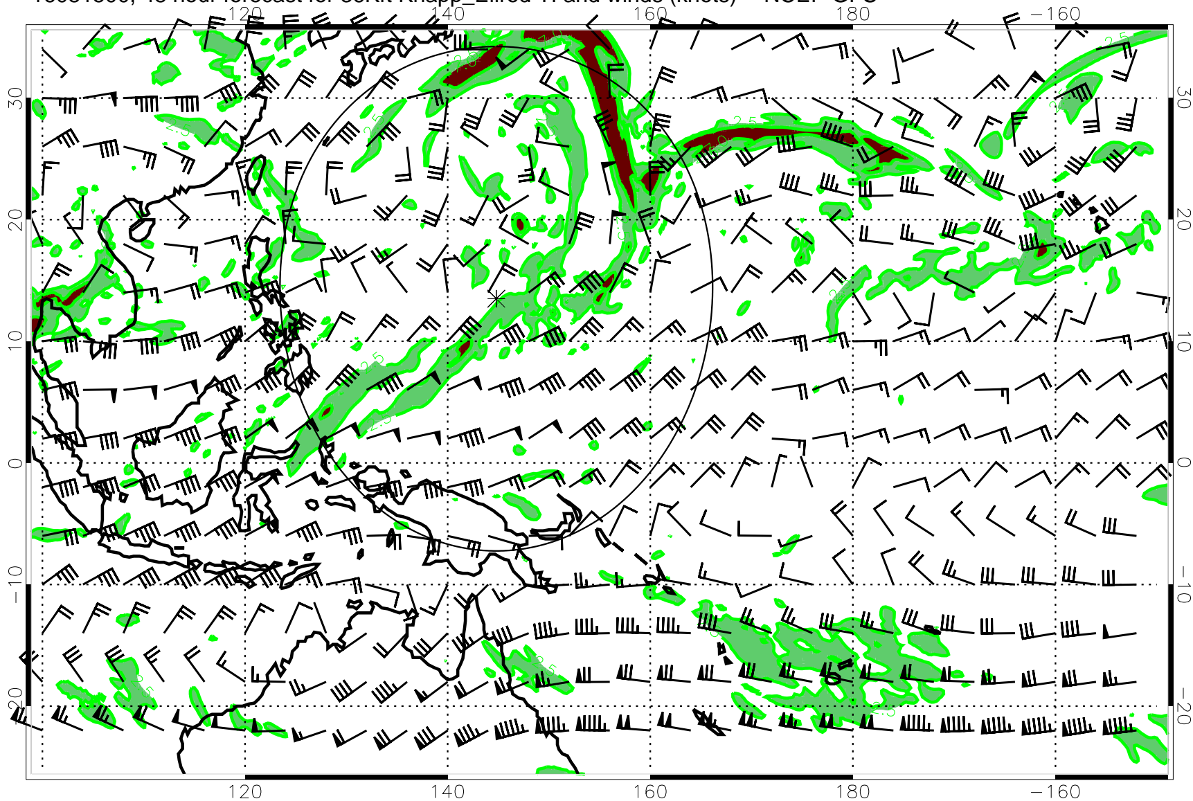
16081500, 48 hour forecast for 36Kft Knapp_Ellrod TI and winds (knots) -- NCEP GFS
