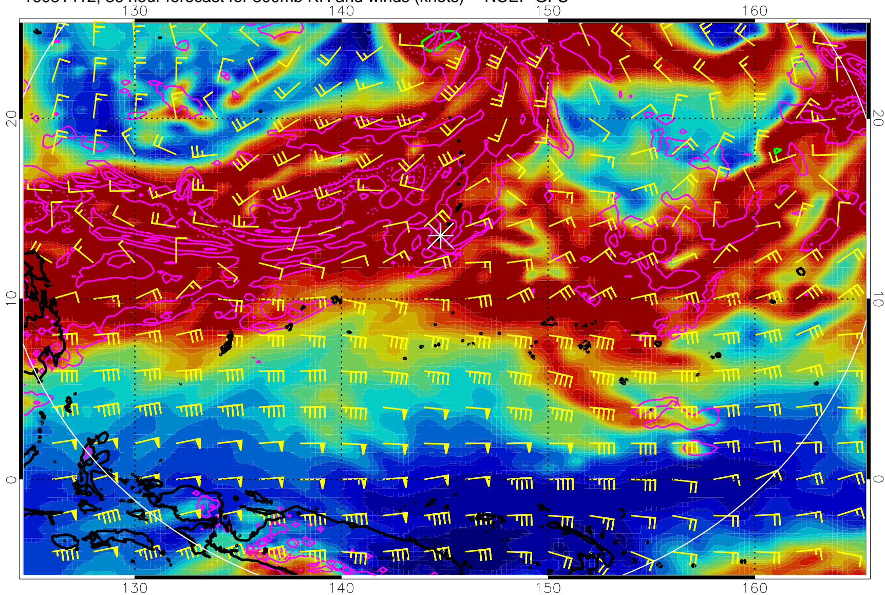
16081412, 36 hour forecast for 300mb RH and winds (knots) -- NCEP GFS
