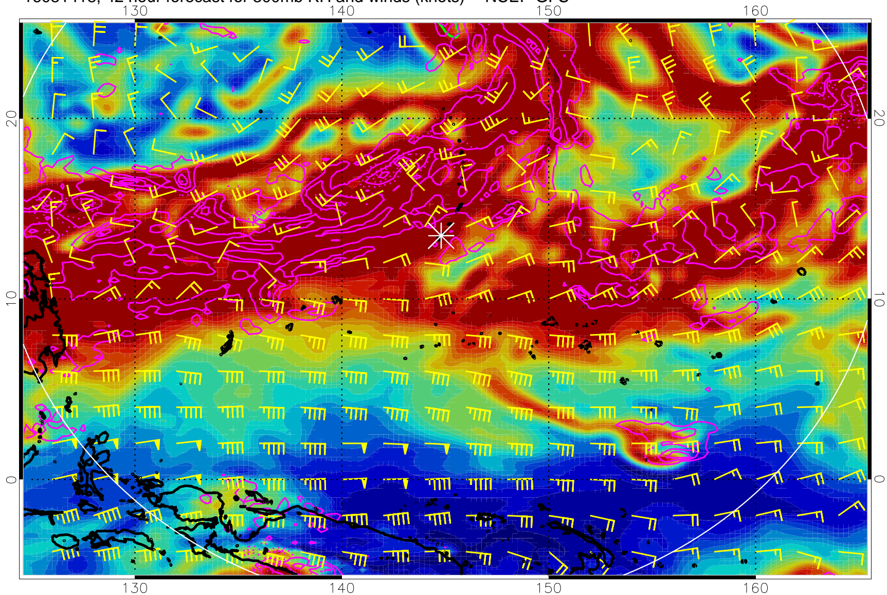
16081418, 42 hour forecast for 300mb RH and winds (knots) -- NCEP GFS
