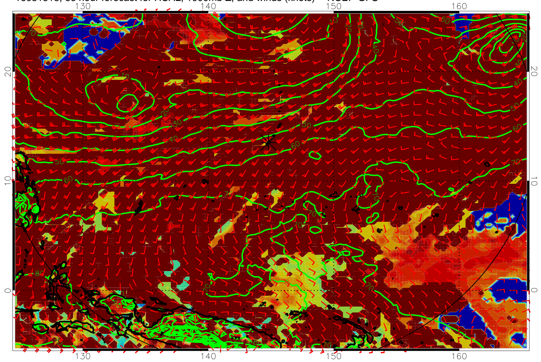
16081518, 66 hour forecast for HCAL, 1000mb Z, and winds (knots) -- NCEP GFS
