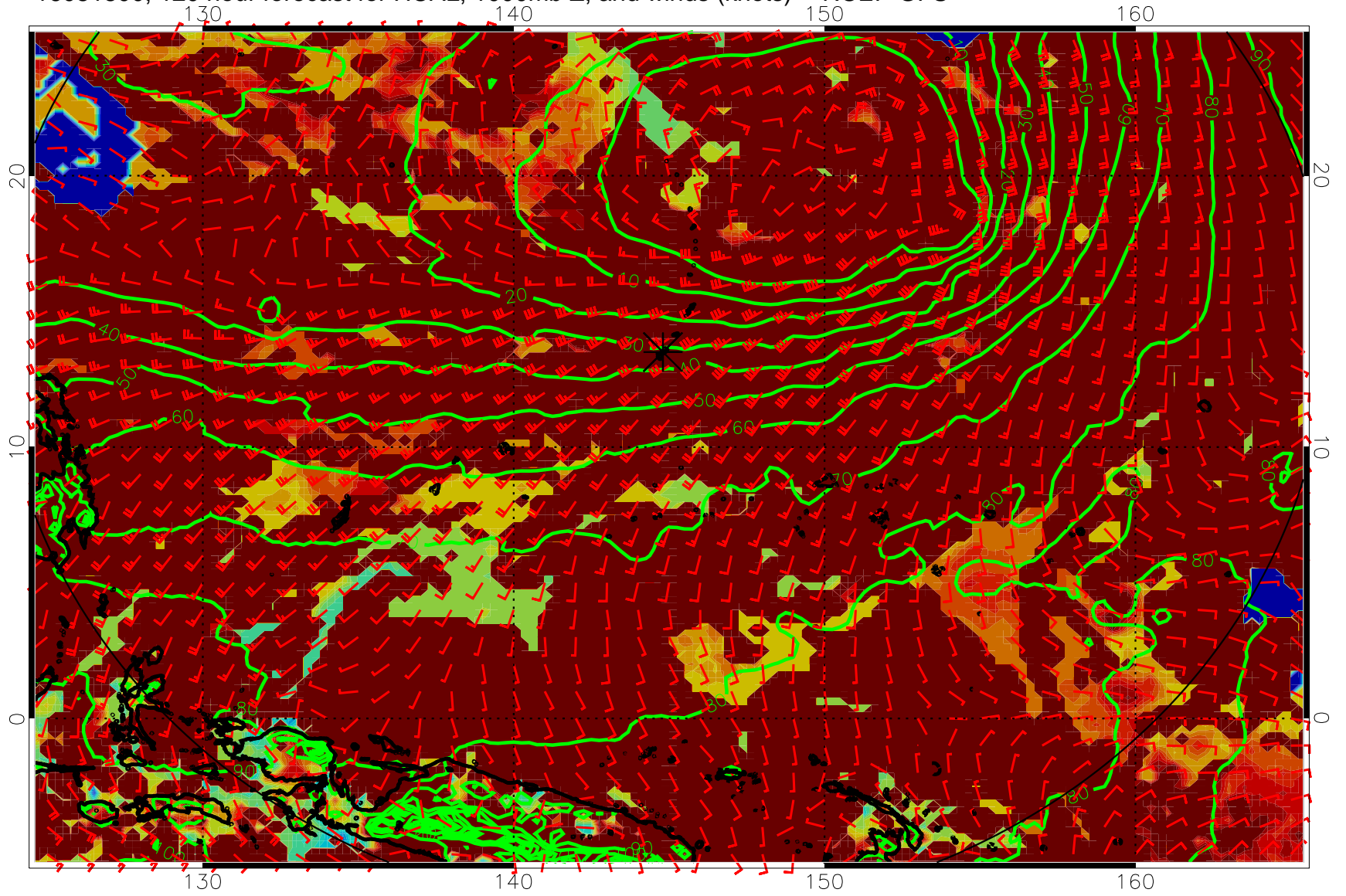
16081800, 120 hour forecast for HCAL, 1000mb Z, and winds (knots) -- NCEP GFS
