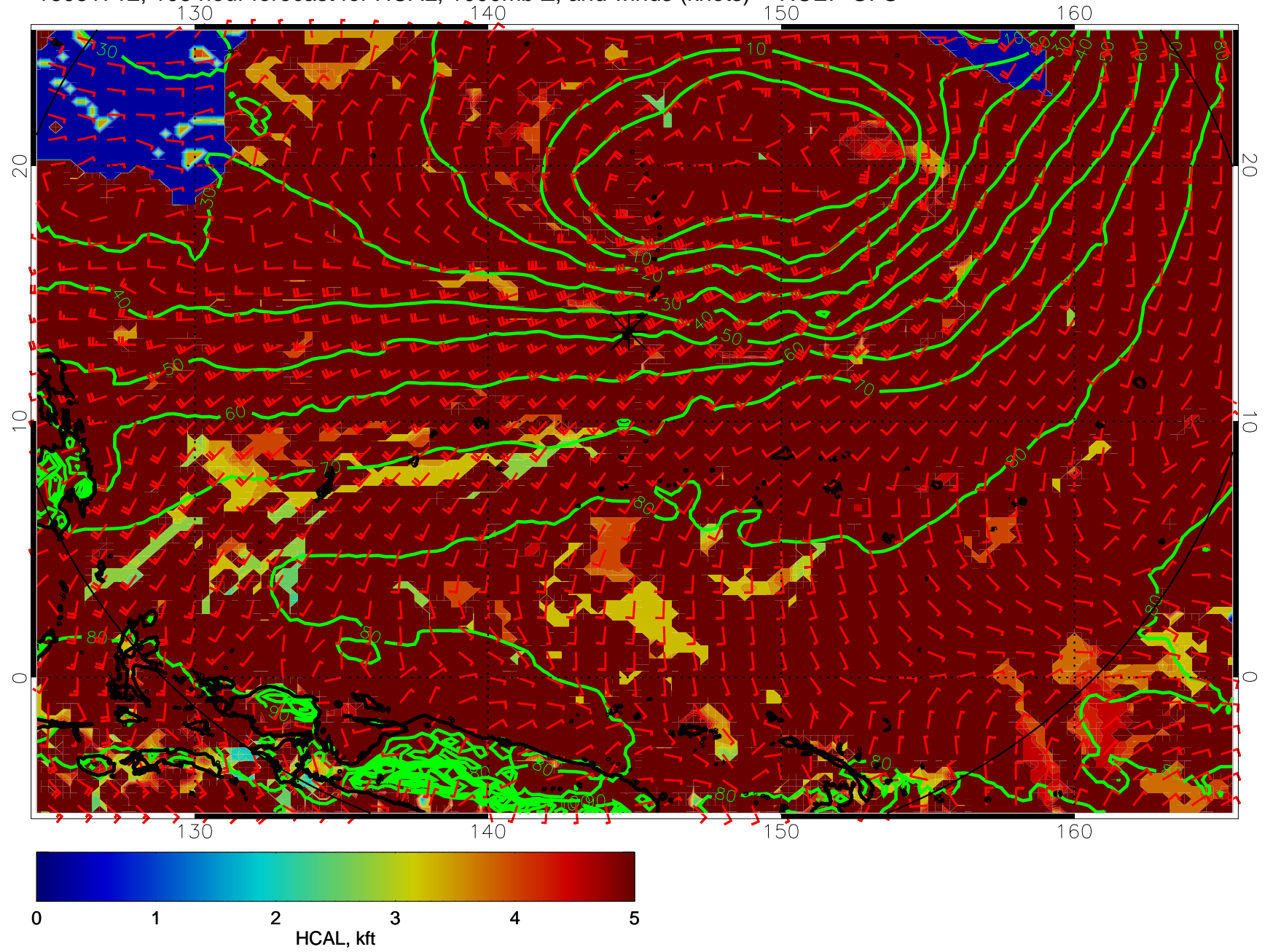
16081712, 108 hour forecast for HCAL, 1000mb Z, and winds (knots) -- NCEP GFS
