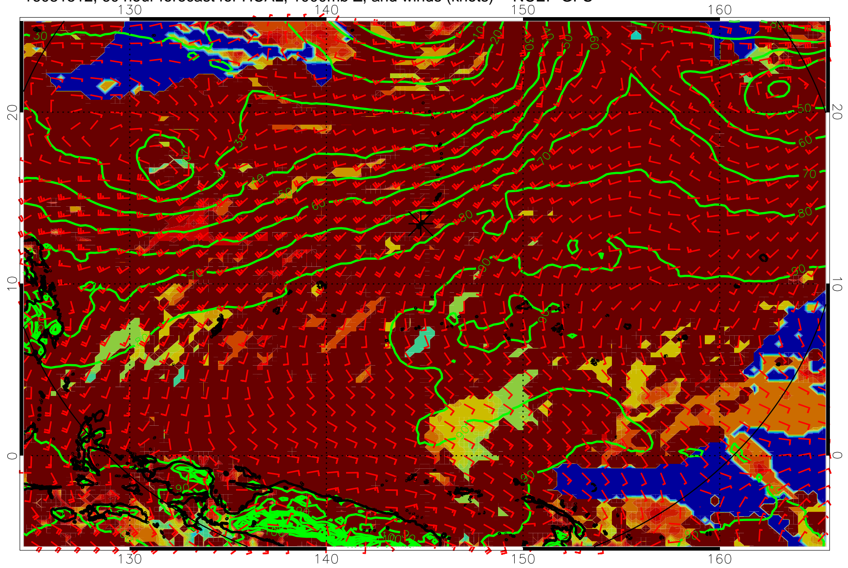
16081512, 60 hour forecast for HCAL, 1000mb Z, and winds (knots) -- NCEP GFS
