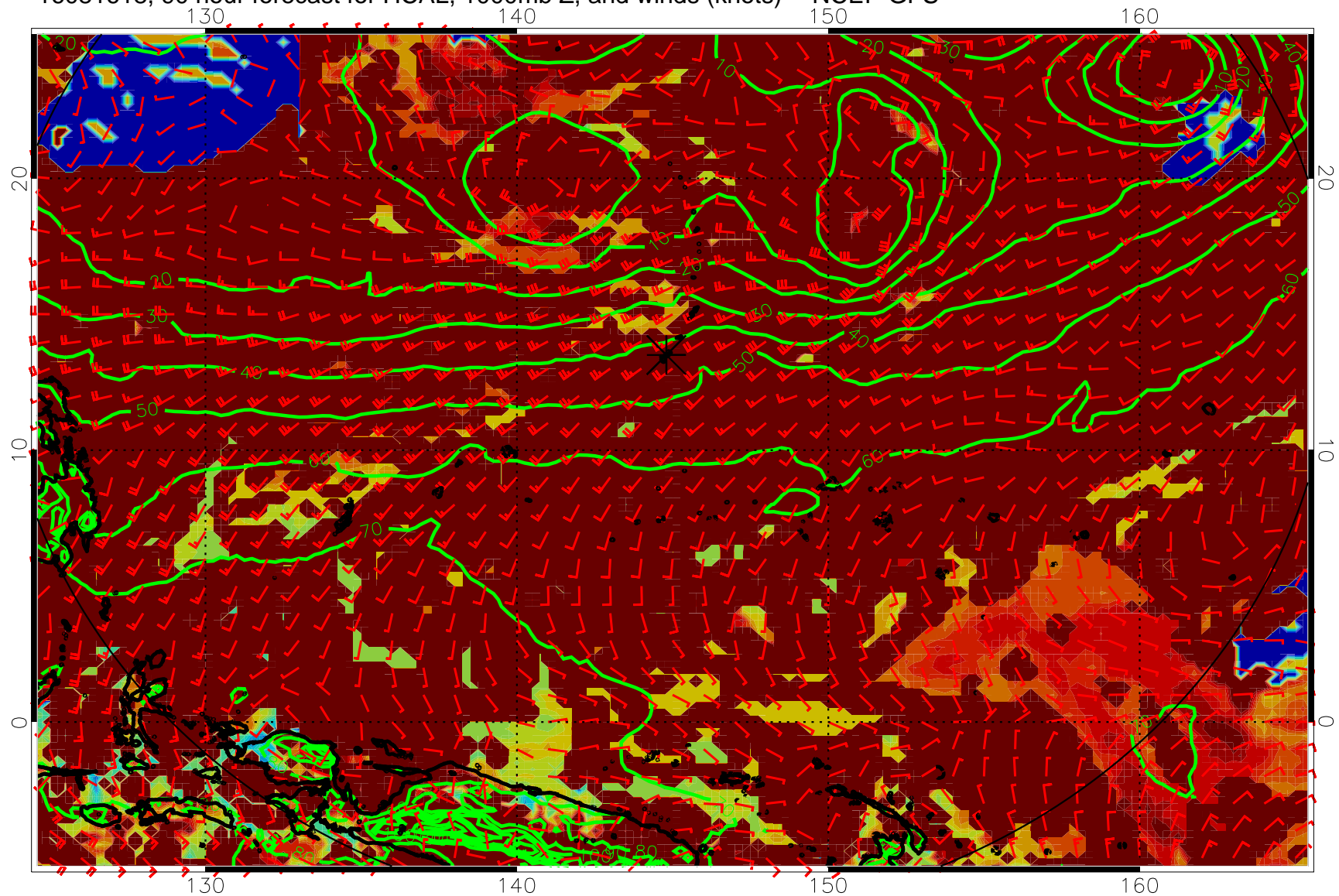
16081618, 90 hour forecast for HCAL, 1000mb Z, and winds (knots) -- NCEP GFS
