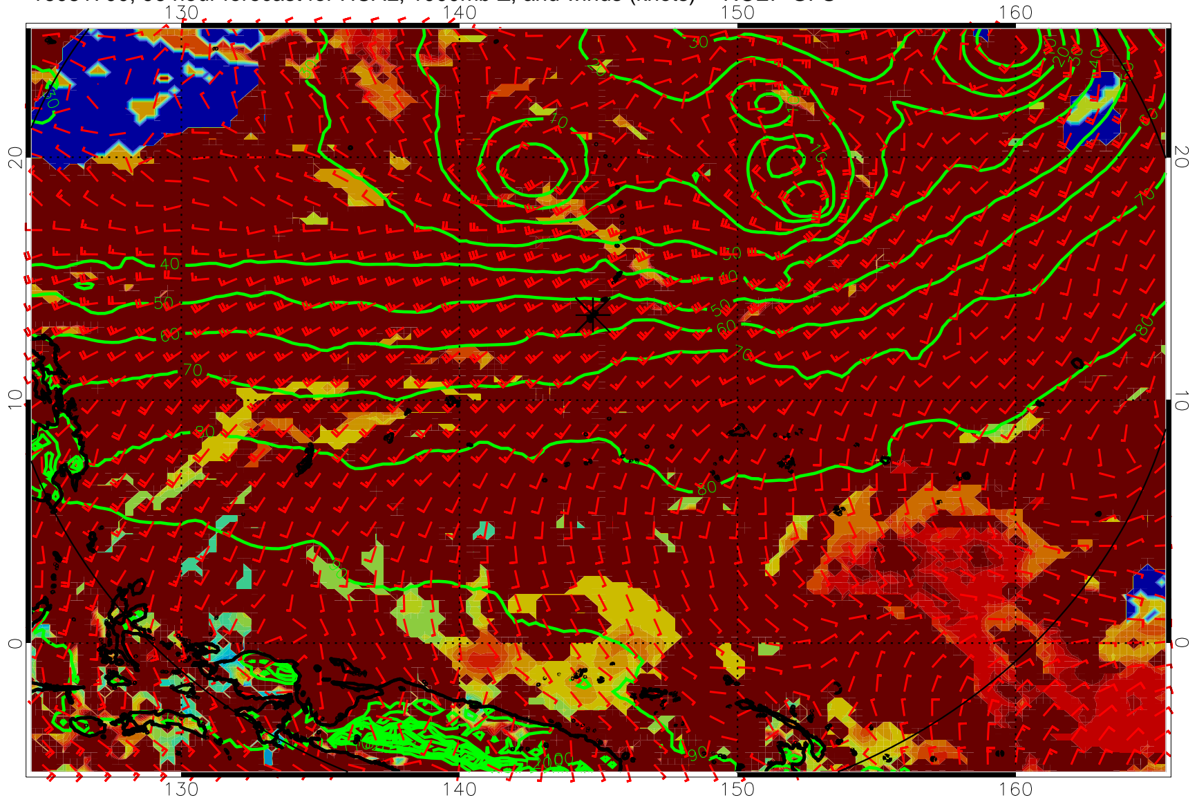
16081700, 96 hour forecast for HCAL, 1000mb Z, and winds (knots) -- NCEP GFS
