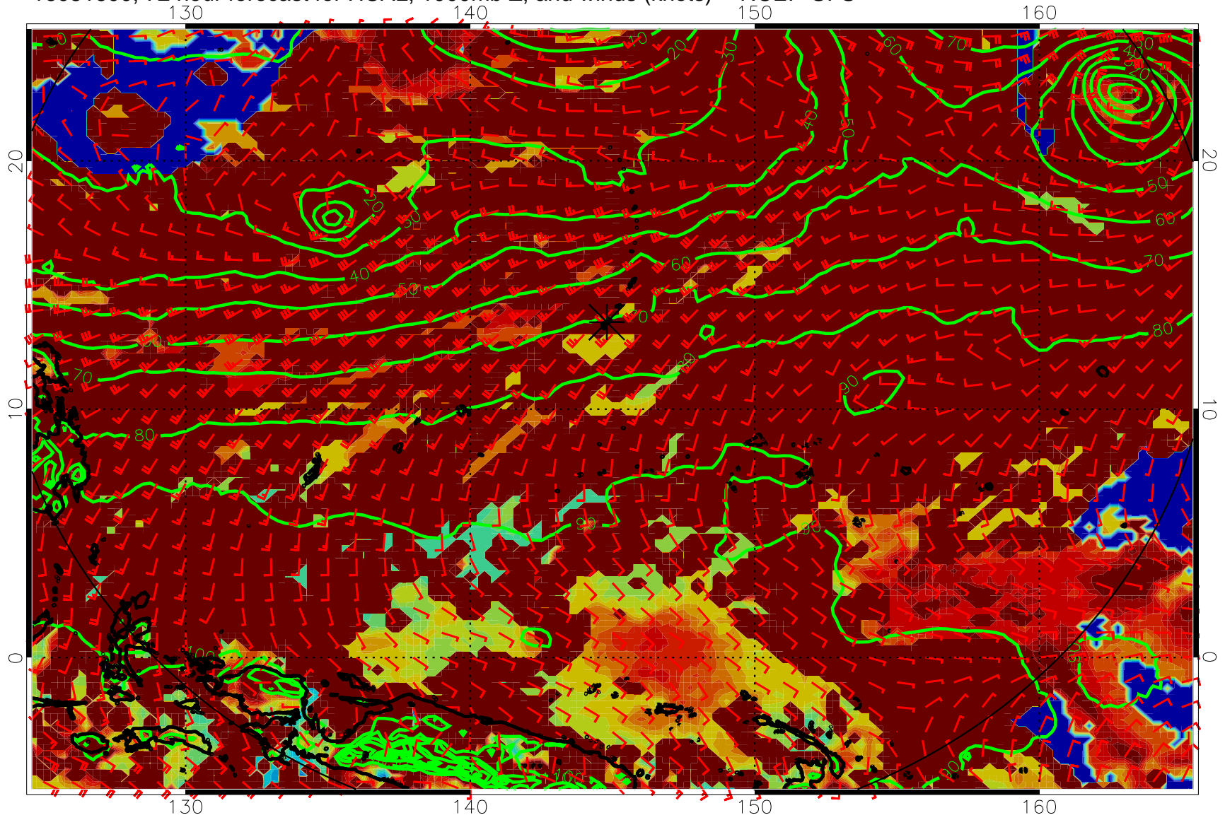
16081600, 72 hour forecast for HCAL, 1000mb Z, and winds (knots) -- NCEP GFS
