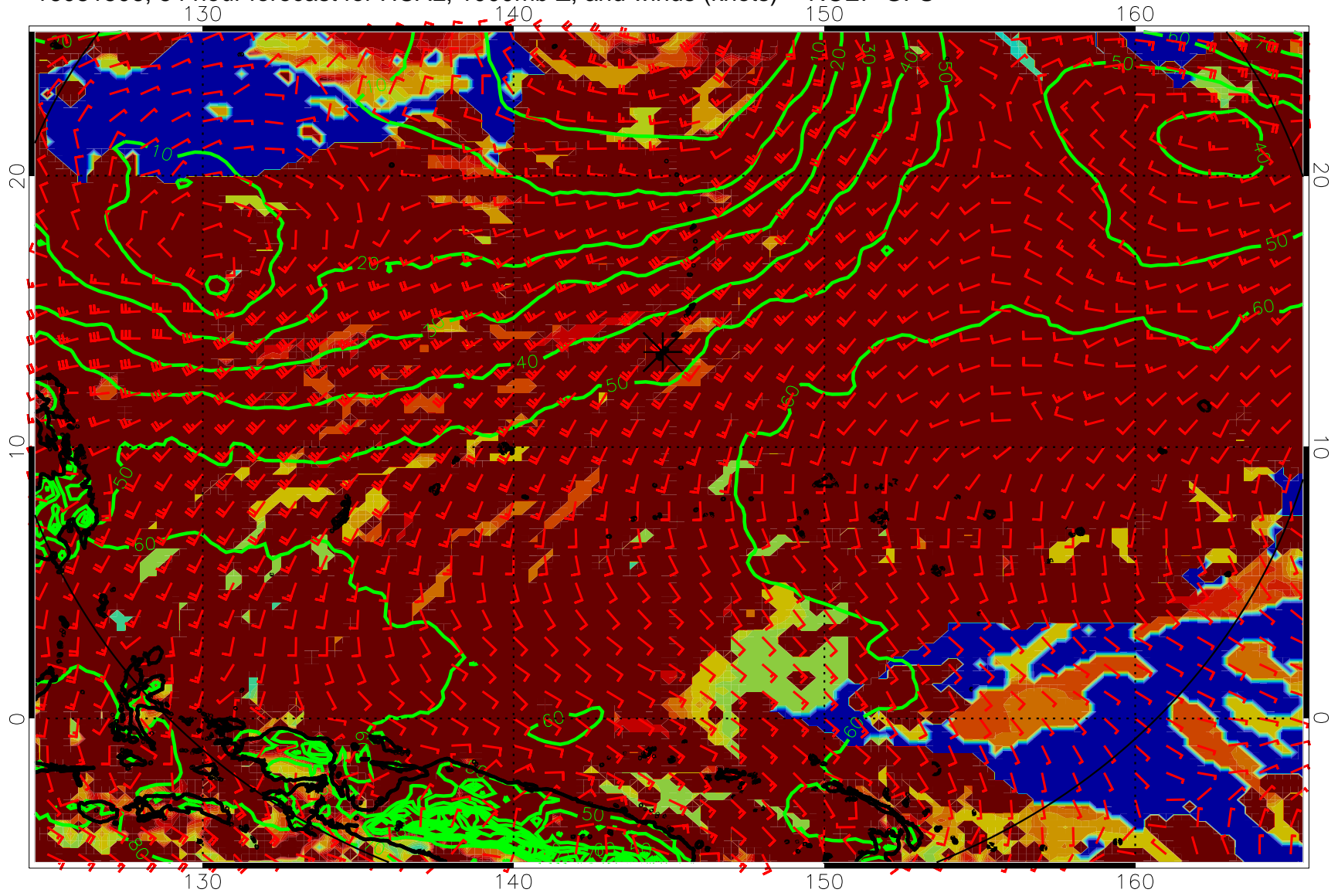
16081506, 54 hour forecast for HCAL, 1000mb Z, and winds (knots) -- NCEP GFS
