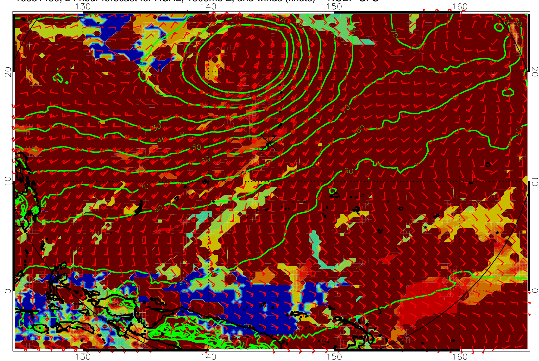
16081400, 24 hour forecast for HCAL, 1000mb Z, and winds (knots) -- NCEP GFS
