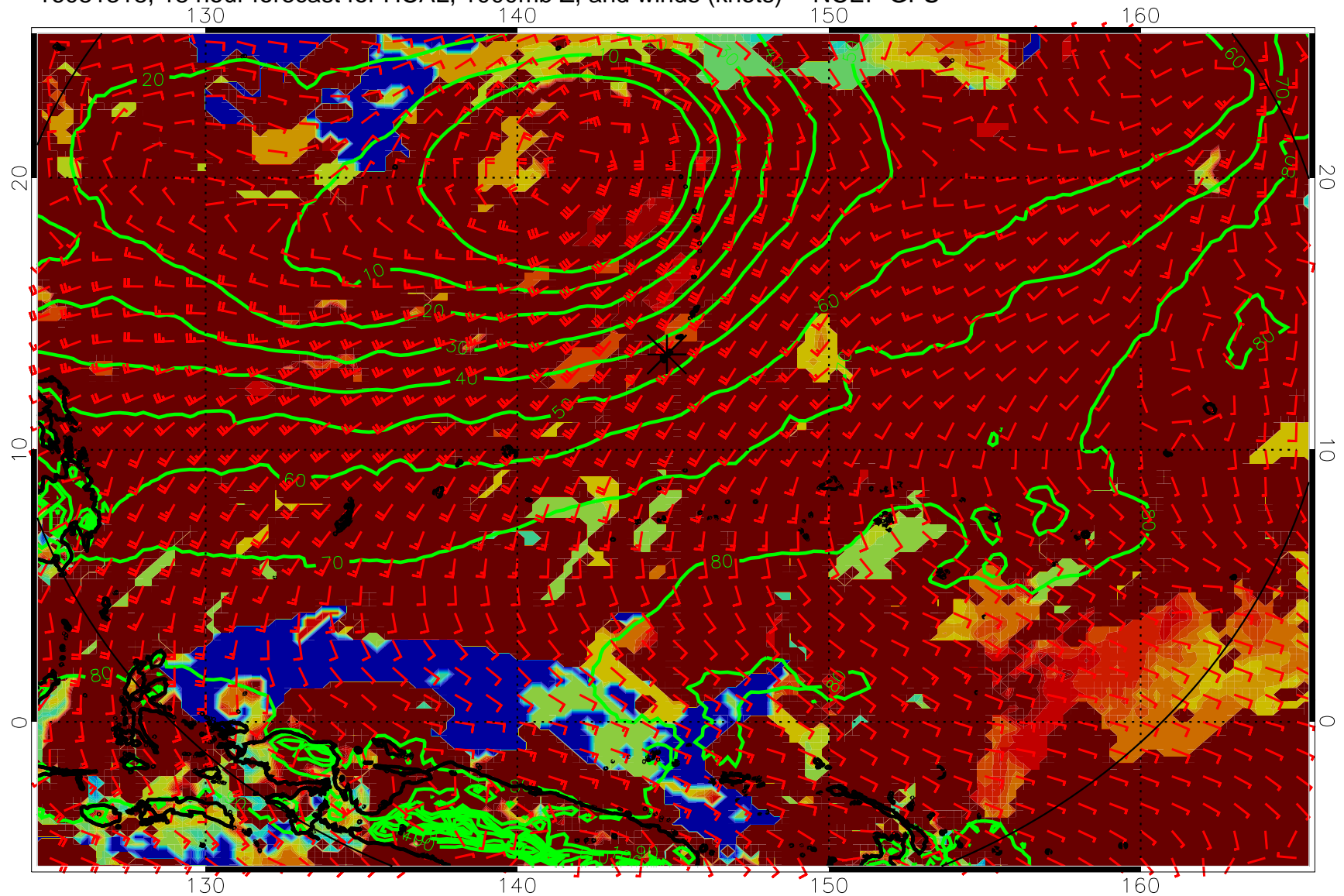
16081318, 18 hour forecast for HCAL, 1000mb Z, and winds (knots) -- NCEP GFS
