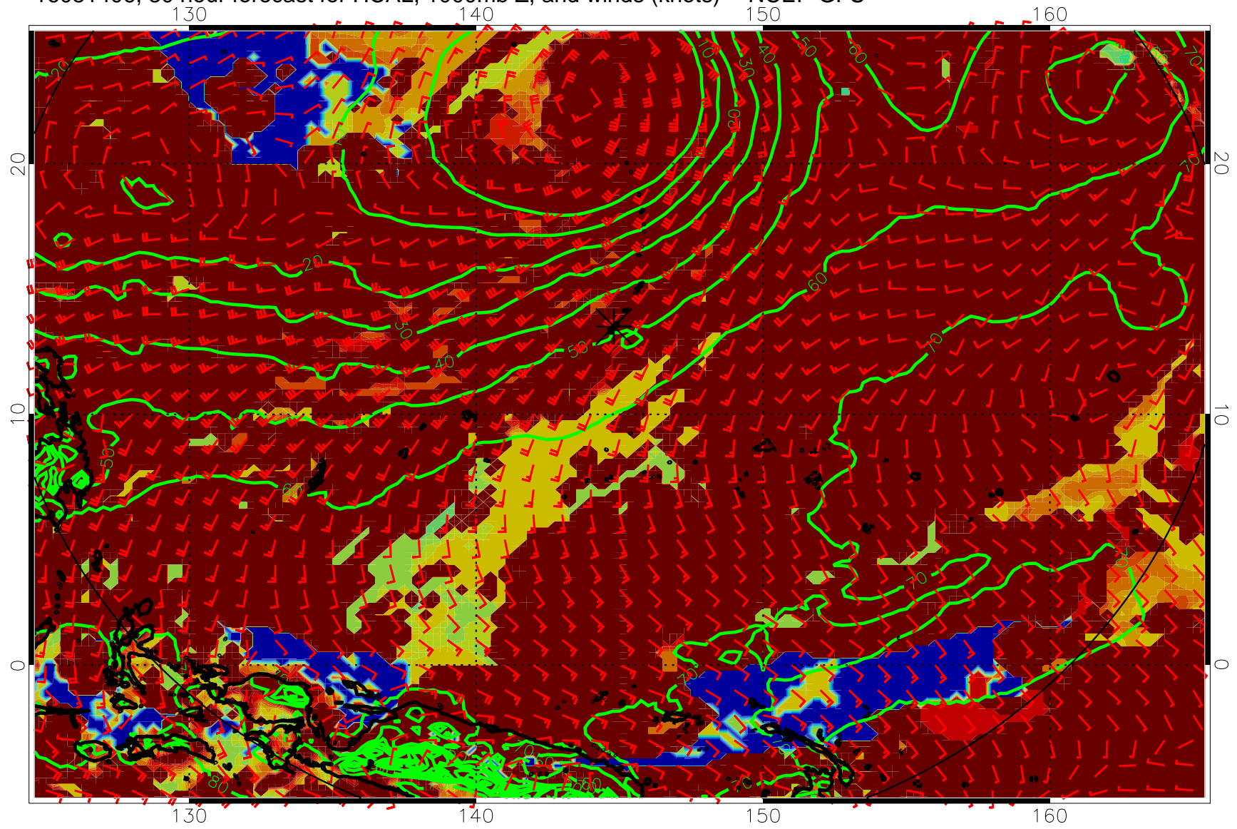
16081406, 30 hour forecast for HCAL, 1000mb Z, and winds (knots) -- NCEP GFS
