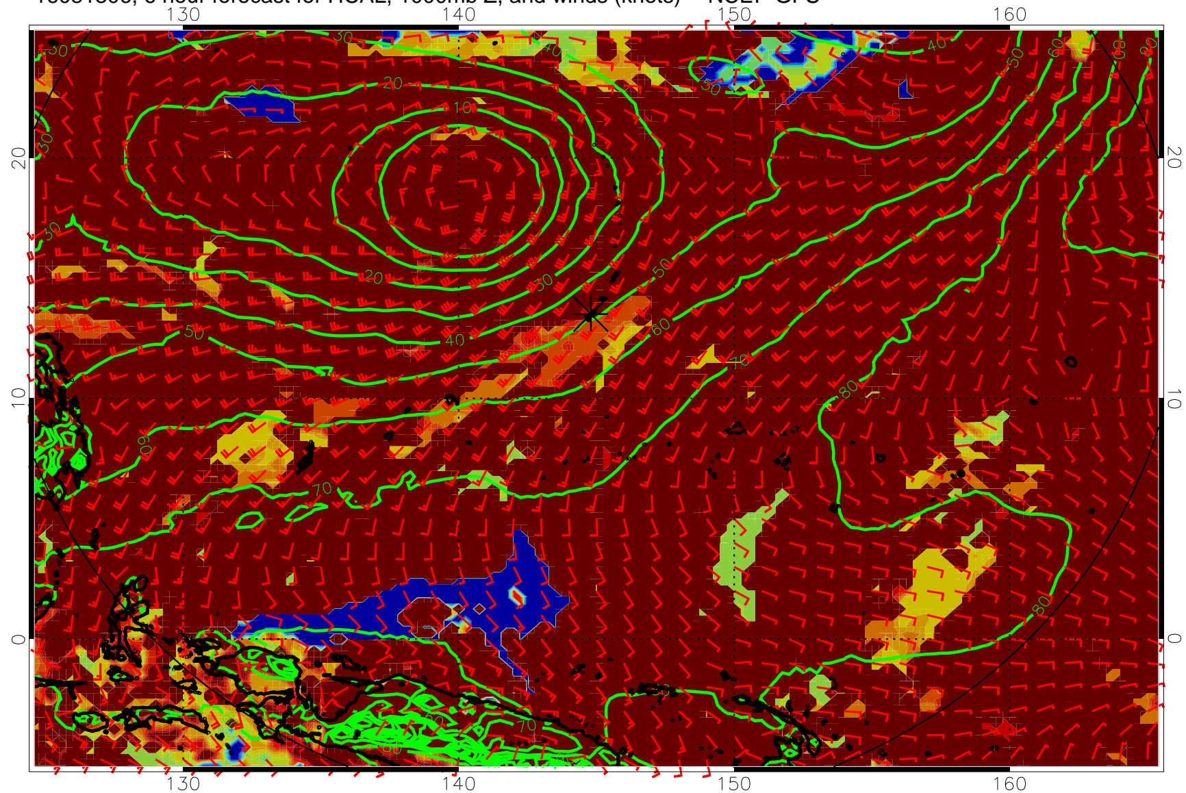
16081306, 6 hour forecast for HCAL, 1000mb Z, and winds (knots) -- NCEP GFS
