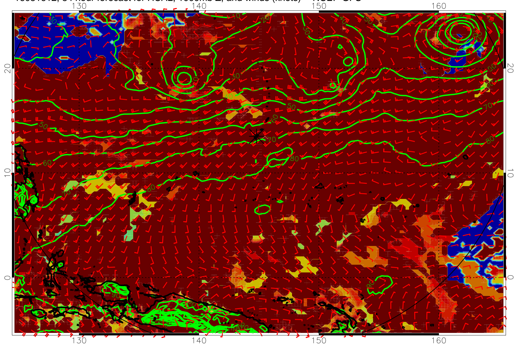
16081612, 84 hour forecast for HCAL, 1000mb Z, and winds (knots) -- NCEP GFS
