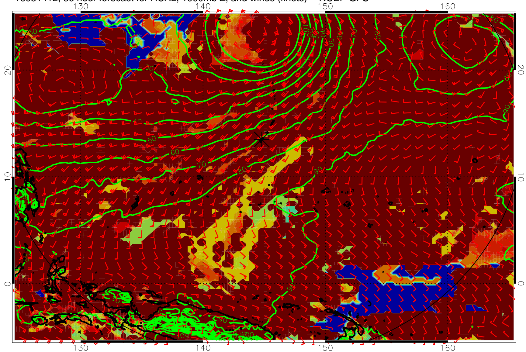
16081412, 36 hour forecast for HCAL, 1000mb Z, and winds (knots) -- NCEP GFS
