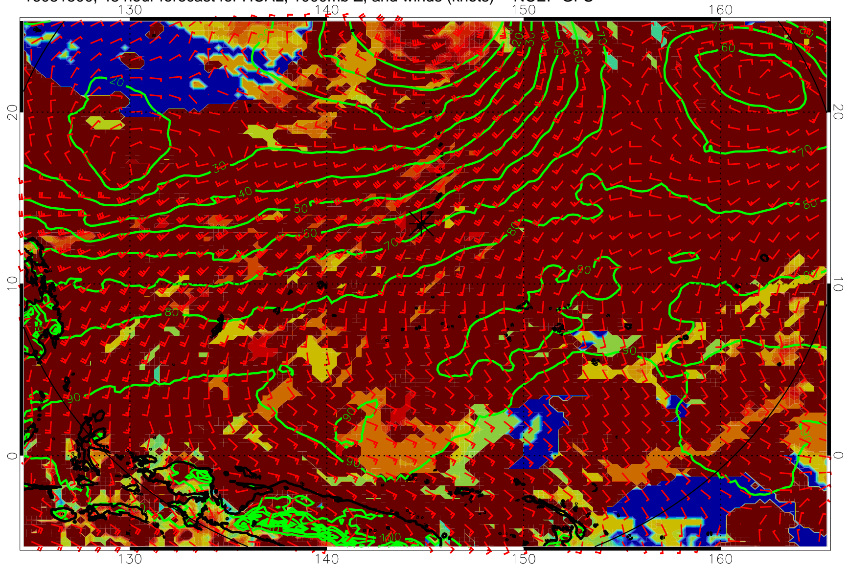
16081500, 48 hour forecast for HCAL, 1000mb Z, and winds (knots) -- NCEP GFS
