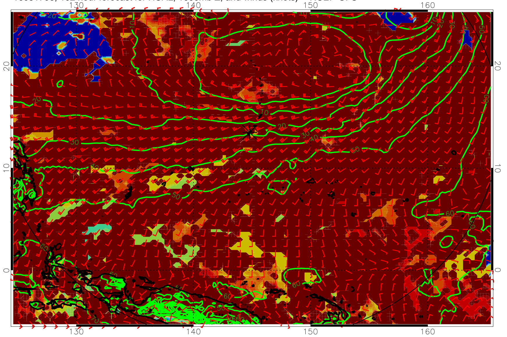
16081706, 102 hour forecast for HCAL, 1000mb Z, and winds (knots) -- NCEP GFS
