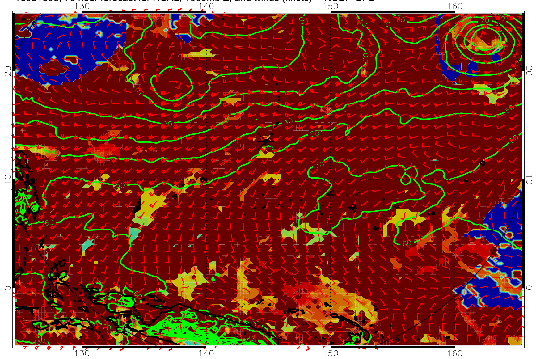
16081606, 78 hour forecast for HCAL, 1000mb Z, and winds (knots) -- NCEP GFS
