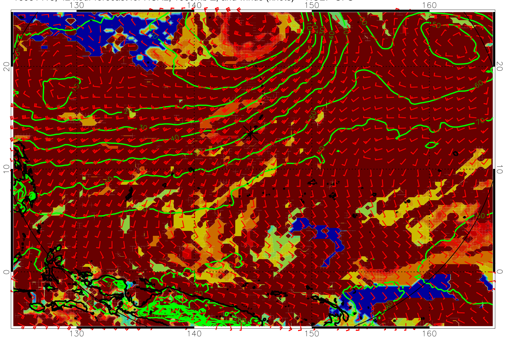
16081418, 42 hour forecast for HCAL, 1000mb Z, and winds (knots) -- NCEP GFS
