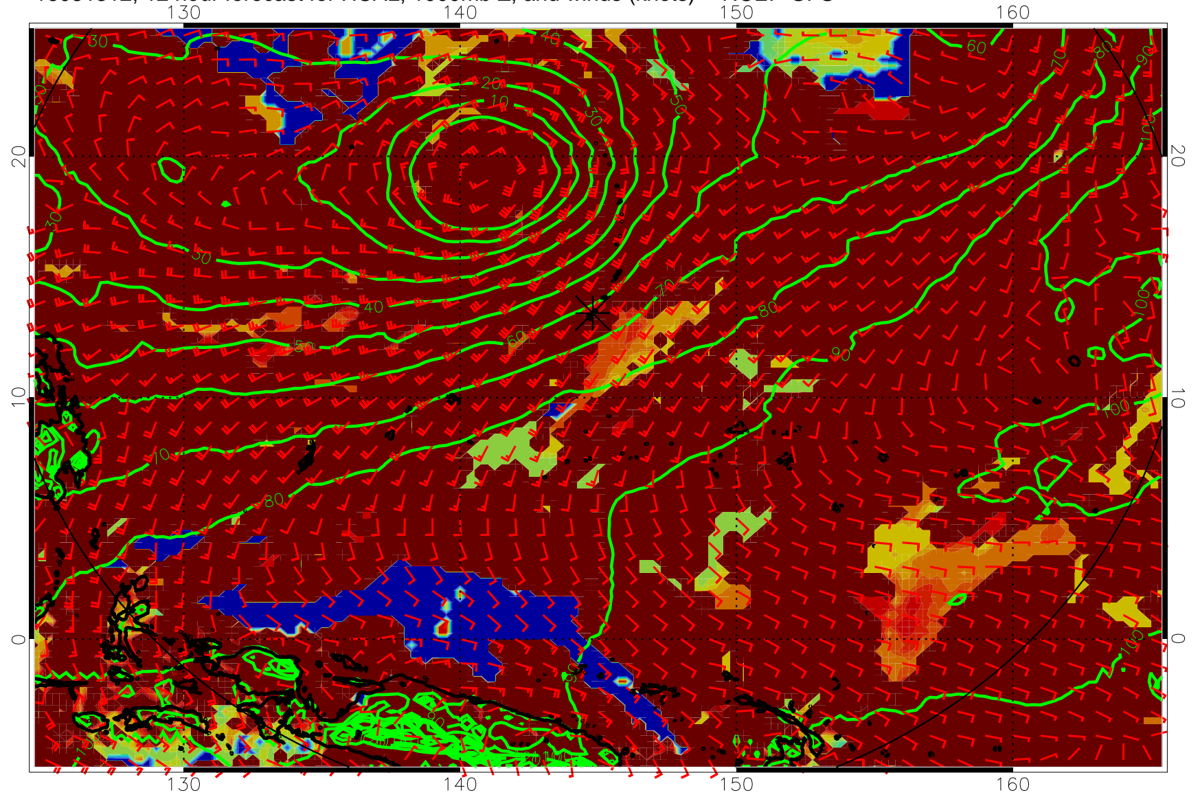
16081312, 12 hour forecast for HCAL, 1000mb Z, and winds (knots) -- NCEP GFS
