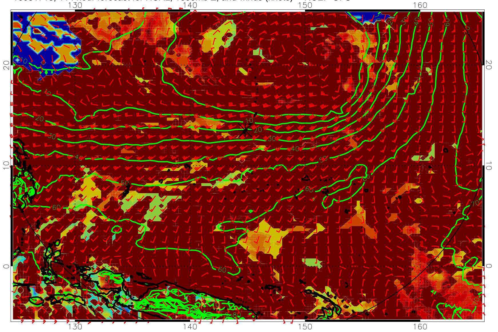
16081718, 114 hour forecast for HCAL, 1000mb Z, and winds (knots) -- NCEP GFS
