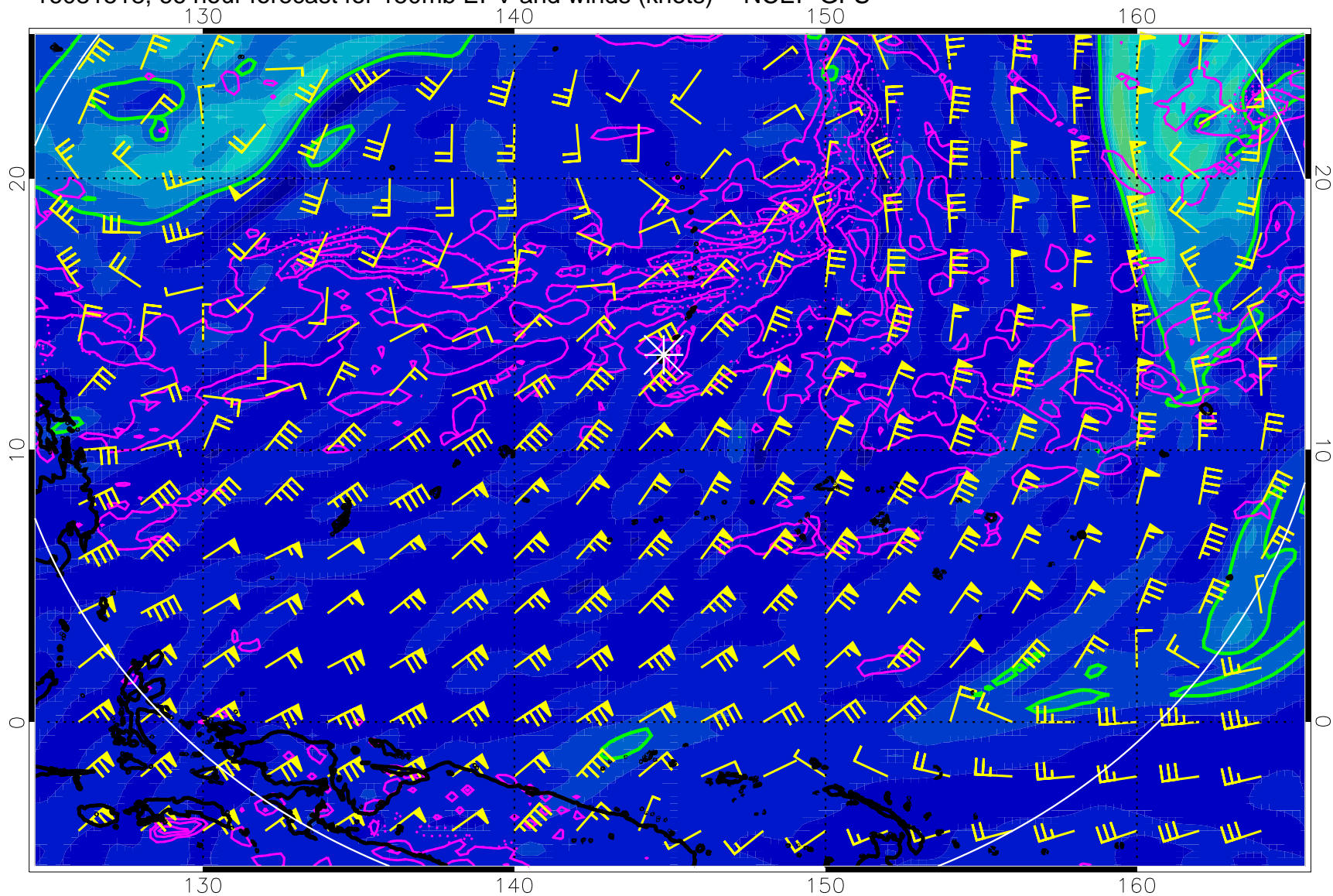
16081518, 66 hour forecast for 150mb EPV and winds (knots) -- NCEP GFS
