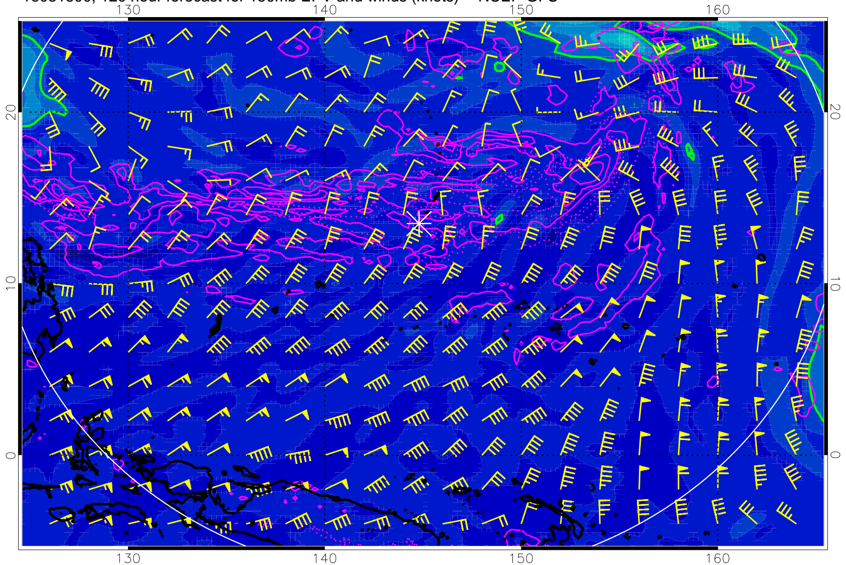
16081800, 120 hour forecast for 150mb EPV and winds (knots) -- NCEP GFS
