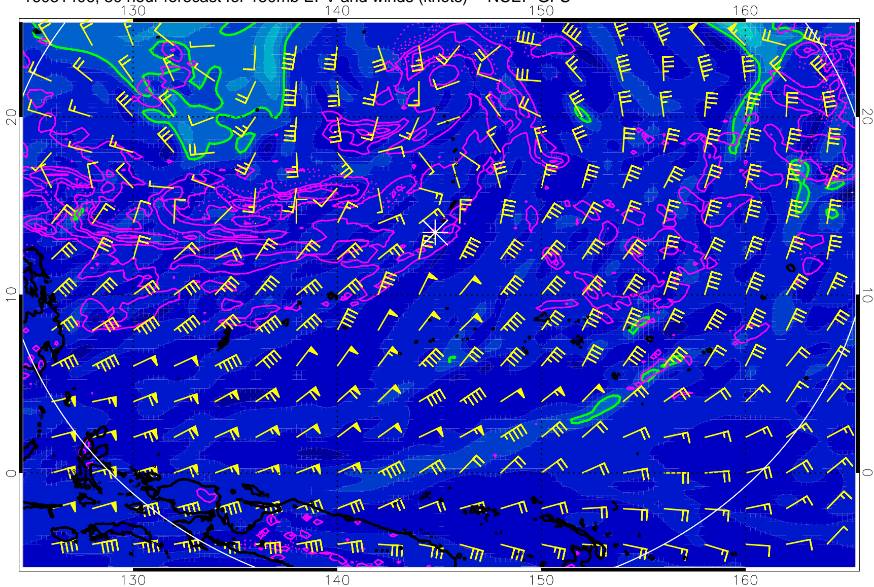
16081406, 30 hour forecast for 150mb EPV and winds (knots) -- NCEP GFS
