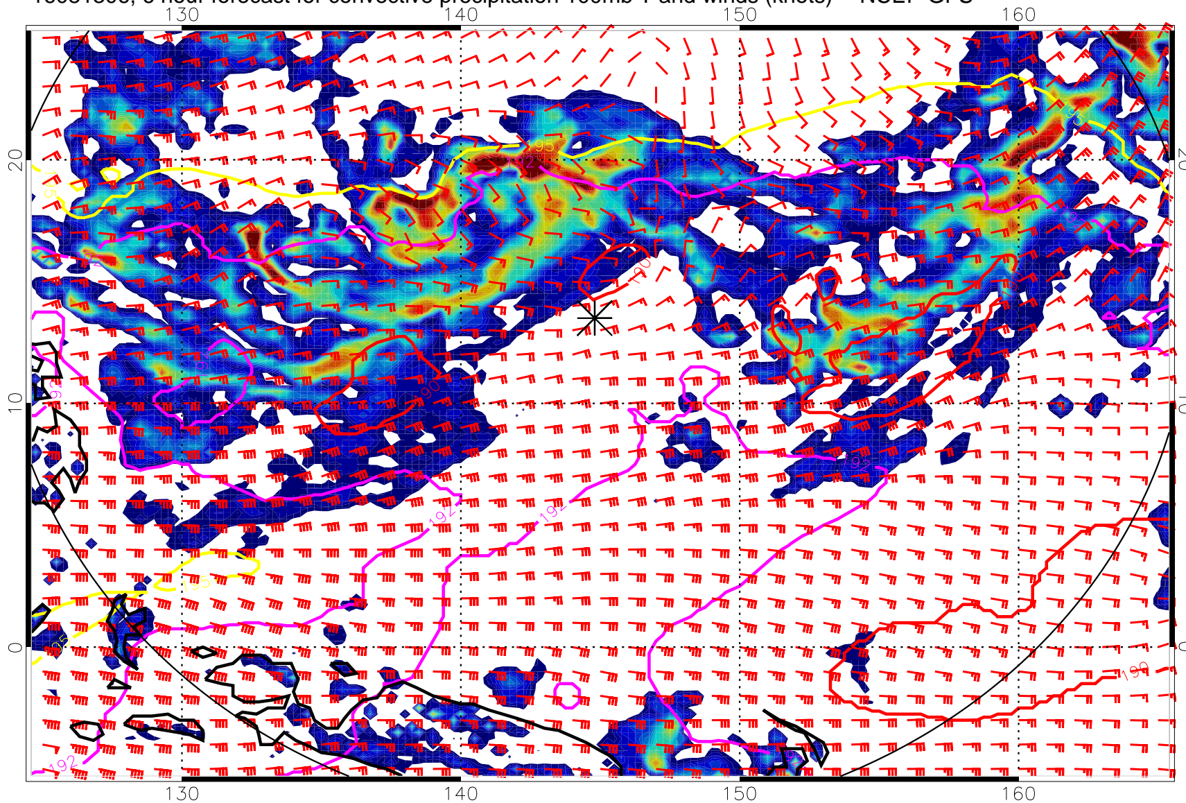
16081306, 6 hour forecast for convective precipitation 100mb T and winds (knots) -- NCEP GFS
