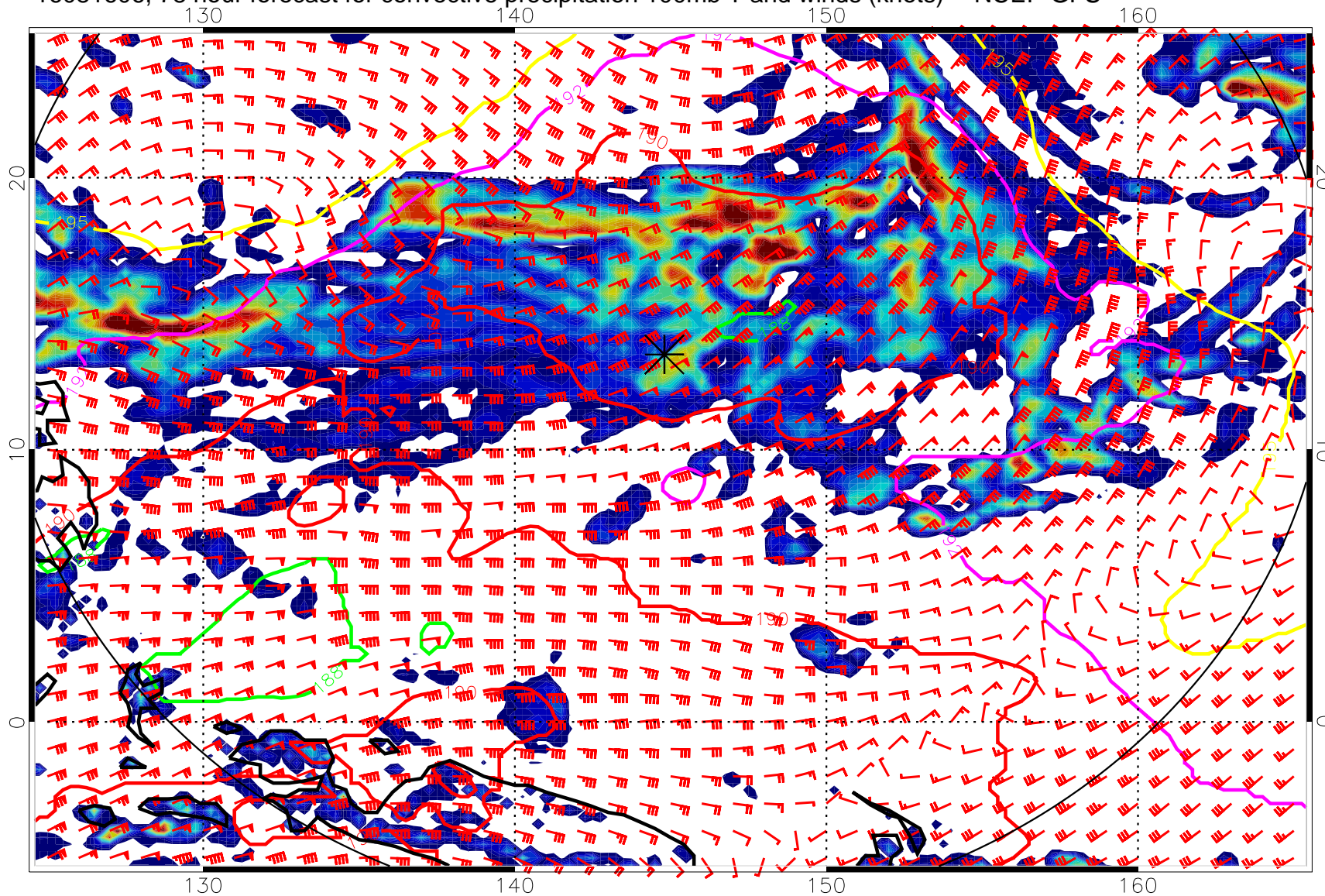
16081606, 78 hour forecast for convective precipitation 100mb T and winds (knots) -- NCEP GFS
