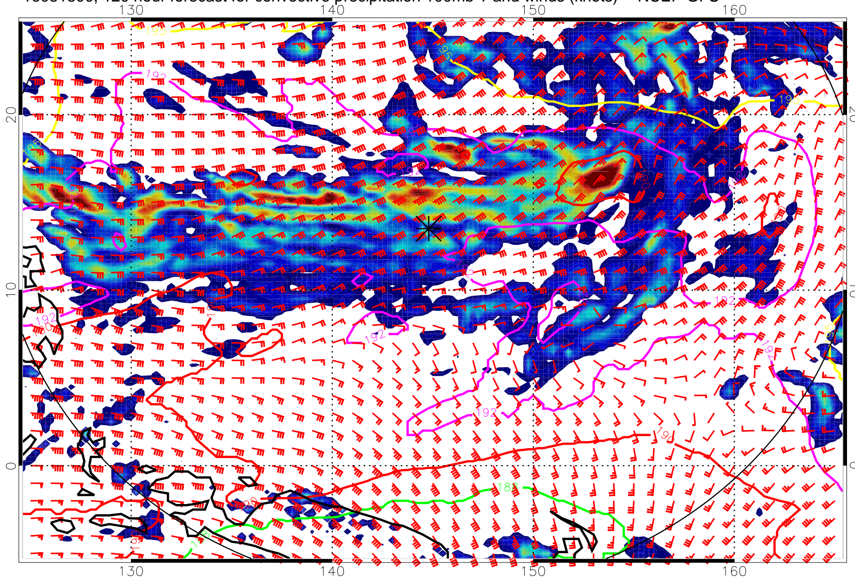
16081800, 120 hour forecast for convective precipitation 100mb T and winds (knots) -- NCEP GFS
