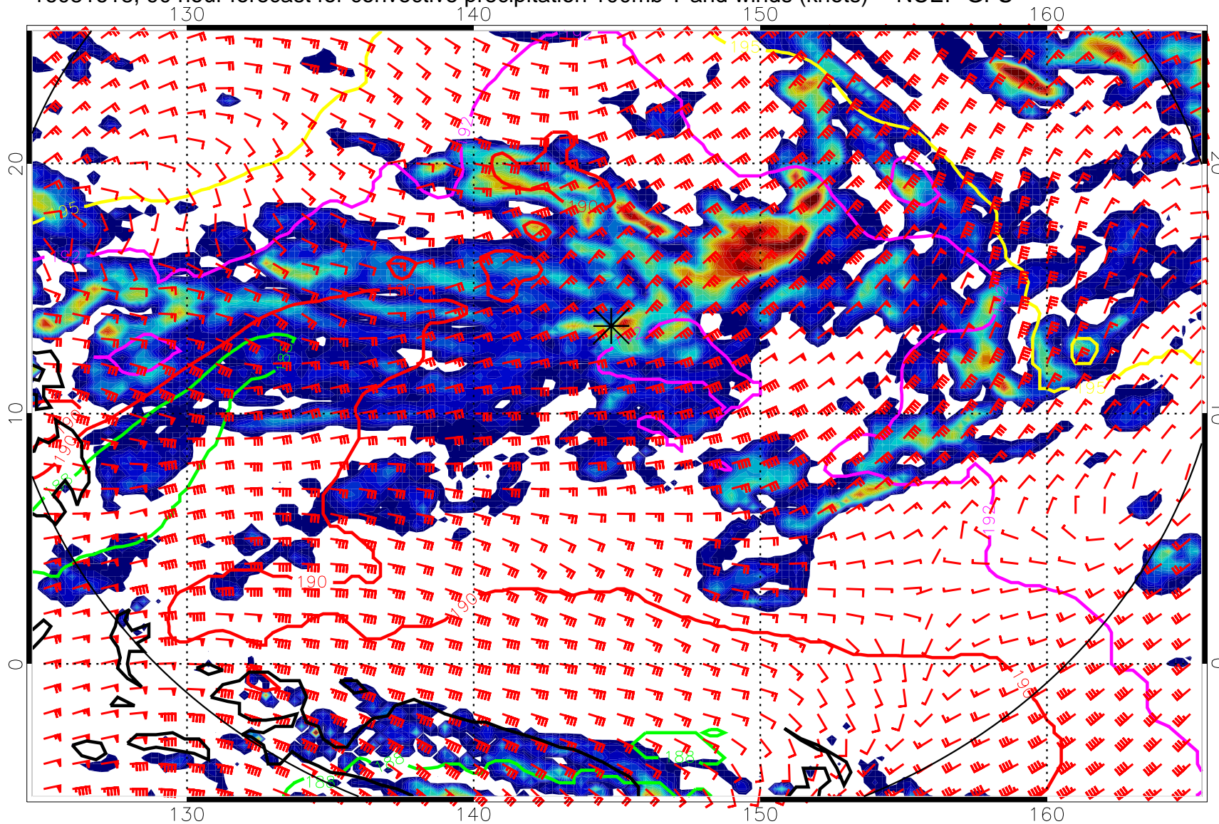
16081618, 90 hour forecast for convective precipitation 100mb T and winds (knots) -- NCEP GFS
