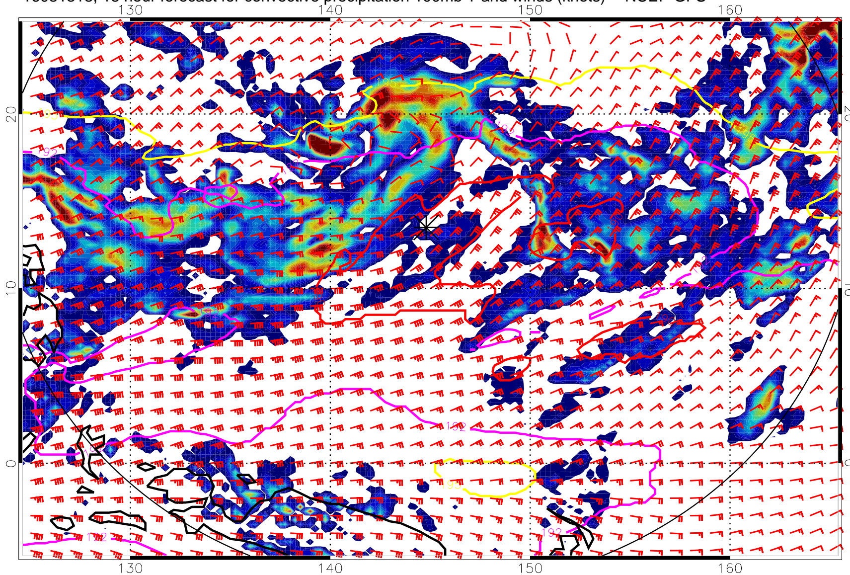
16081318, 18 hour forecast for convective precipitation 100mb T and winds (knots) -- NCEP GFS
