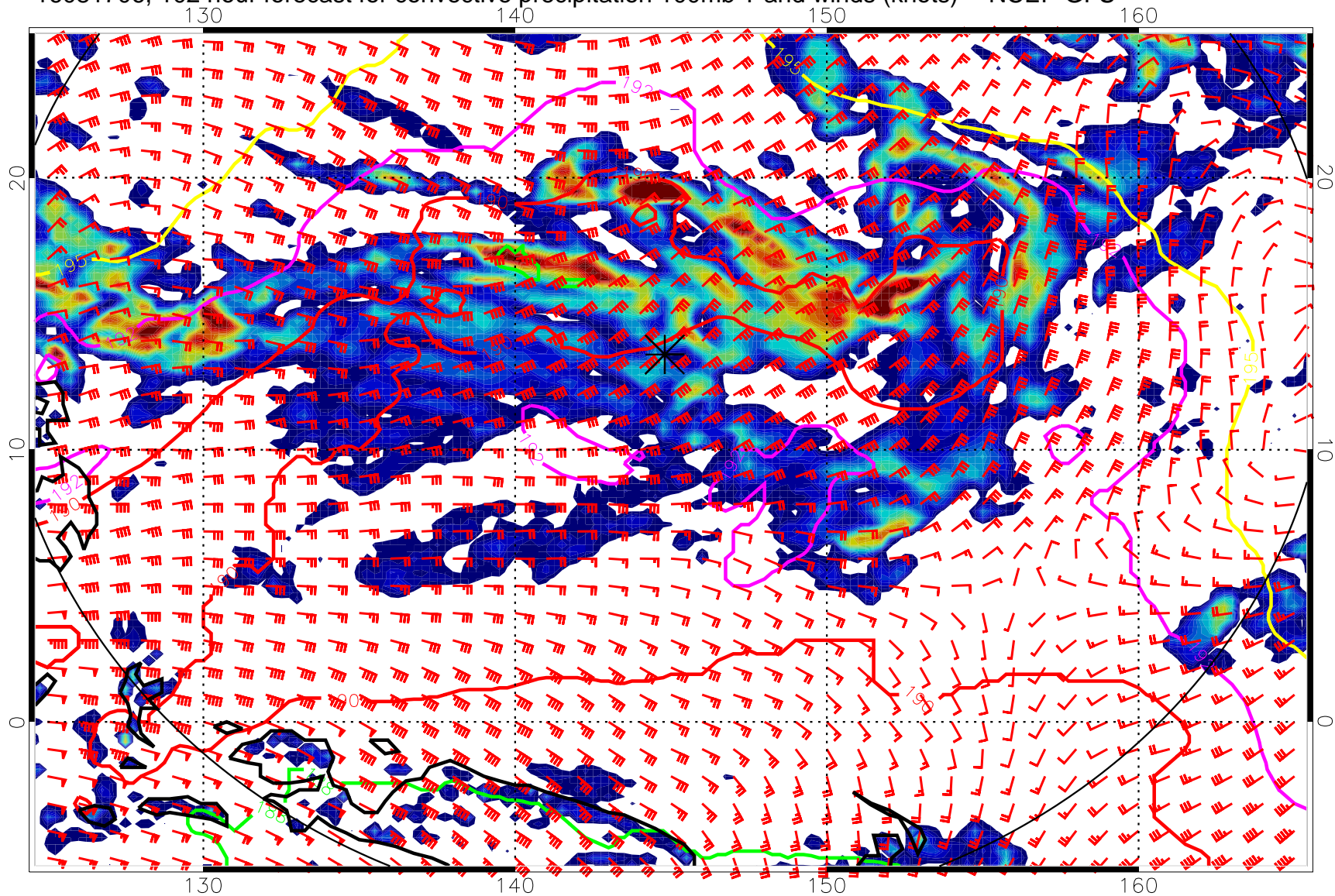
16081706, 102 hour forecast for convective precipitation 100mb T and winds (knots) -- NCEP GFS
