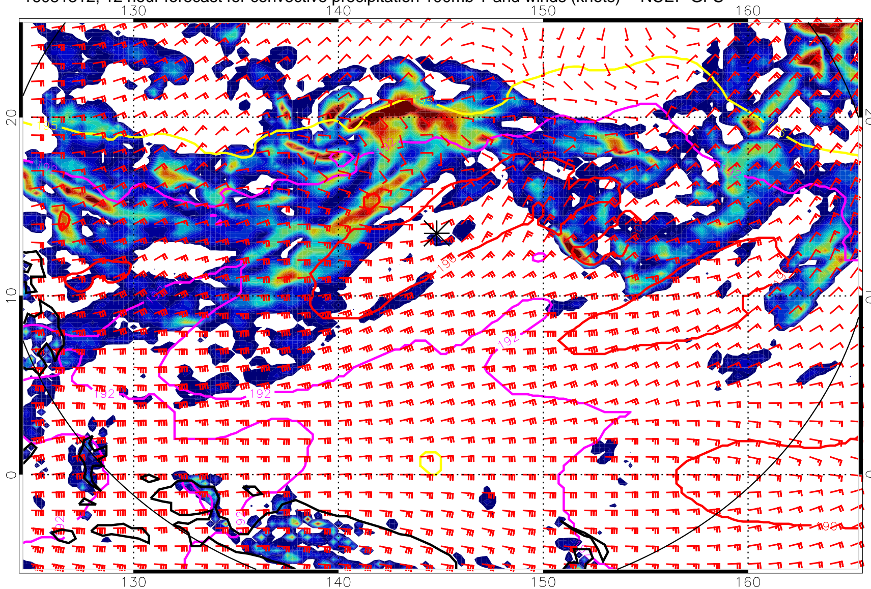
16081312, 12 hour forecast for convective precipitation 100mb T and winds (knots) -- NCEP GFS
