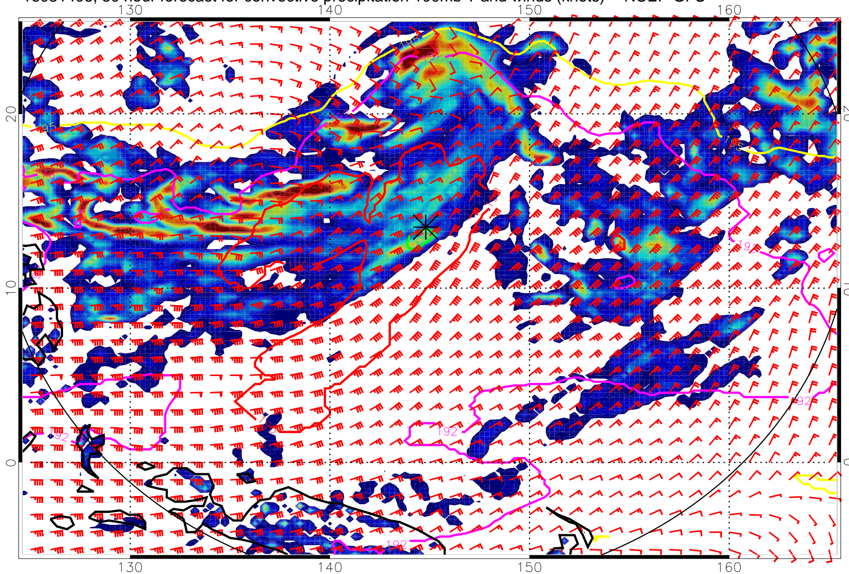
16081406, 30 hour forecast for convective precipitation 100mb T and winds (knots) -- NCEP GFS
