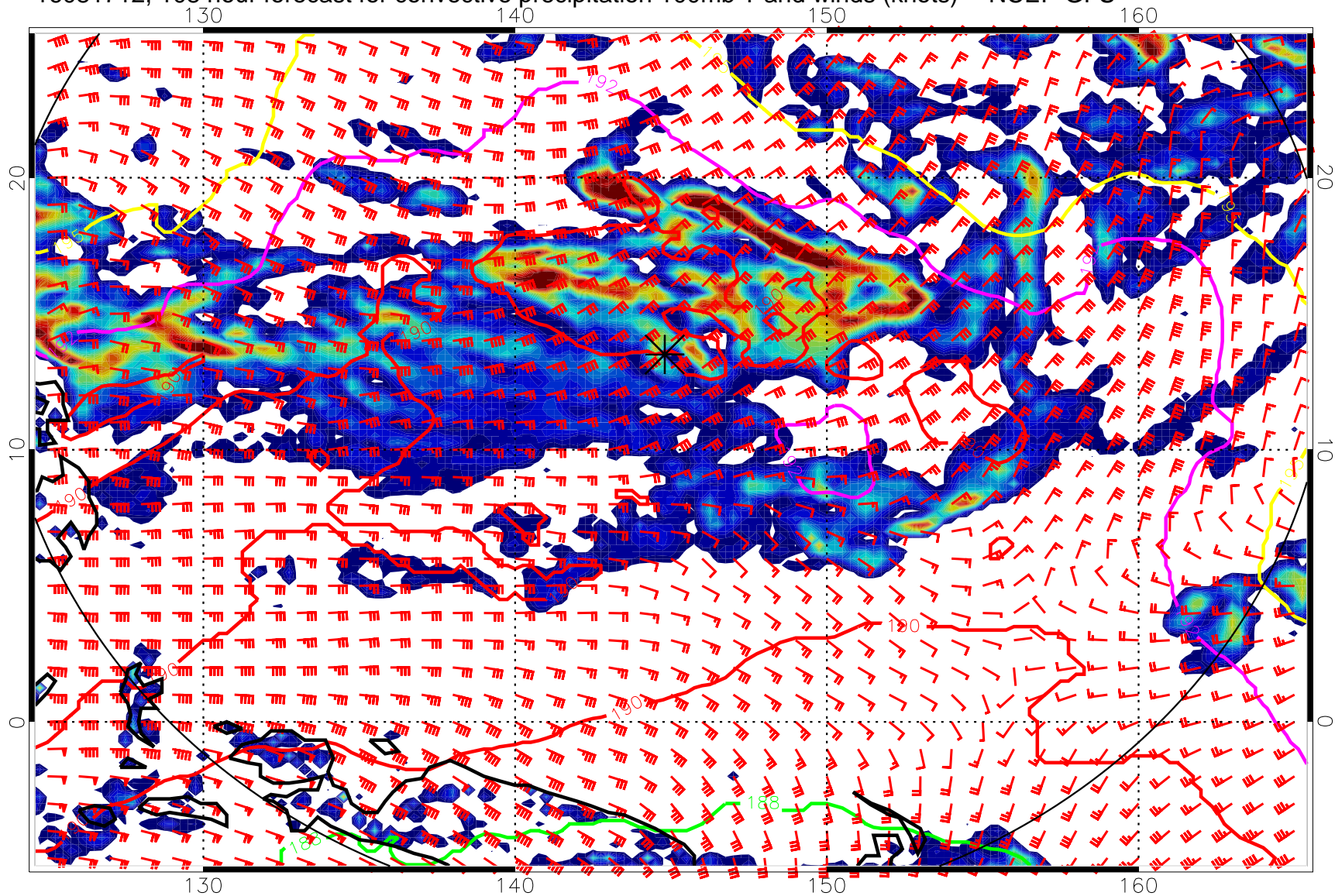
16081712, 108 hour forecast for convective precipitation 100mb T and winds (knots) -- NCEP GFS
