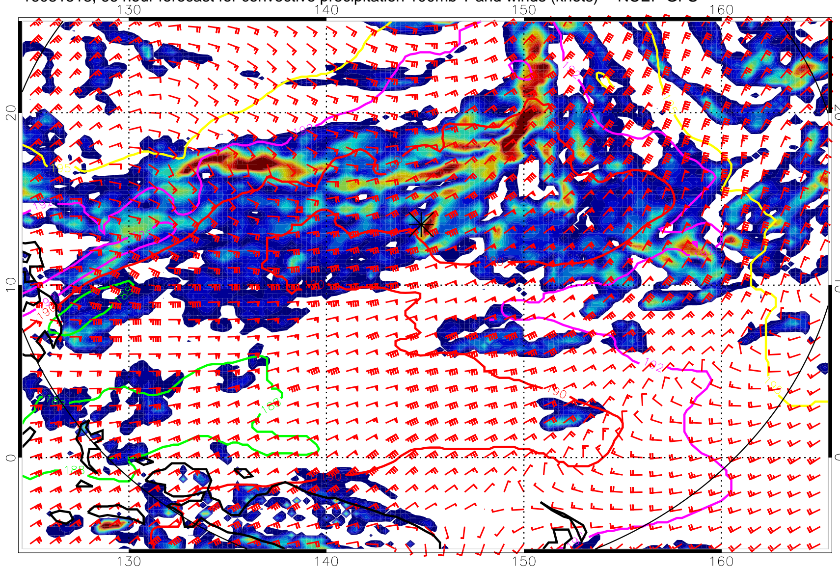
16081518, 66 hour forecast for convective precipitation 100mb T and winds (knots) -- NCEP GFS
