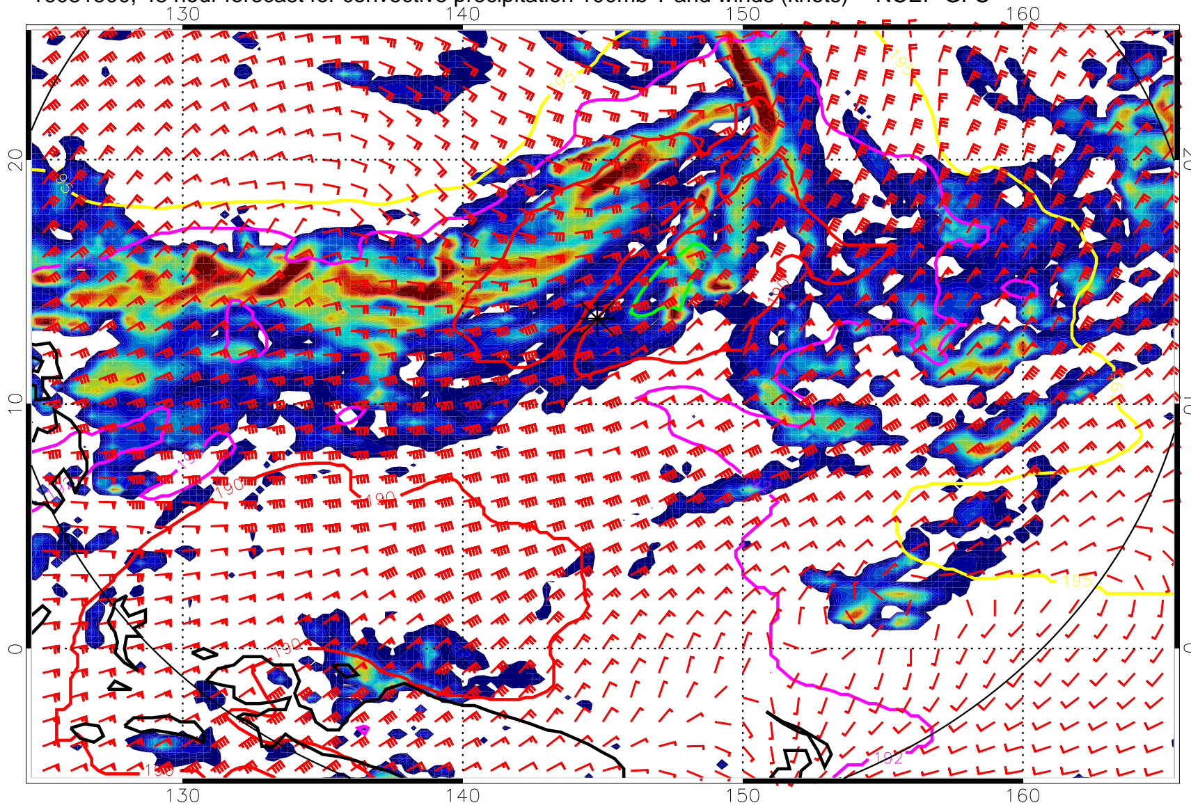
16081500, 48 hour forecast for convective precipitation 100mb T and winds (knots) -- NCEP GFS
