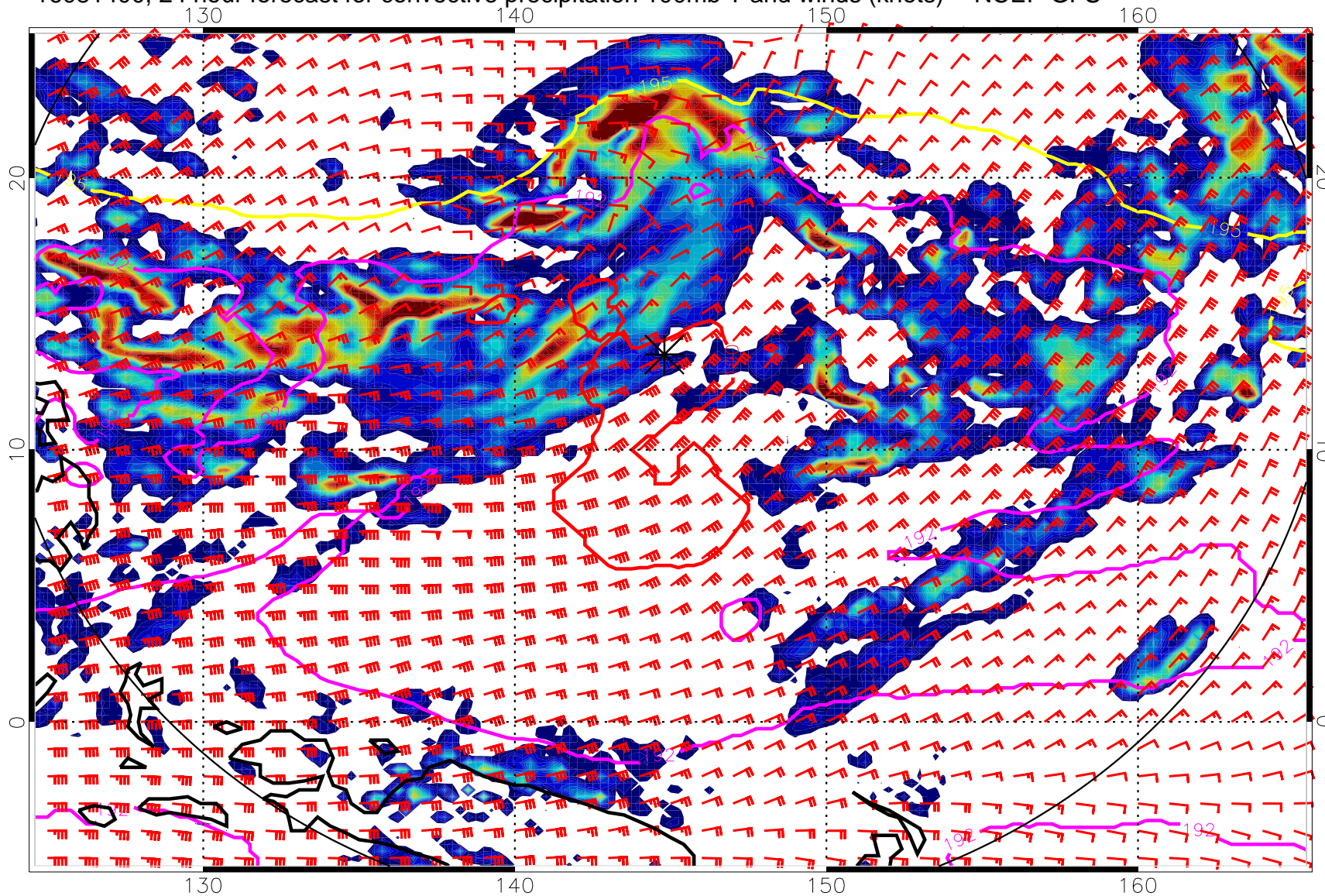
16081400, 24 hour forecast for convective precipitation 100mb T and winds (knots) -- NCEP GFS
