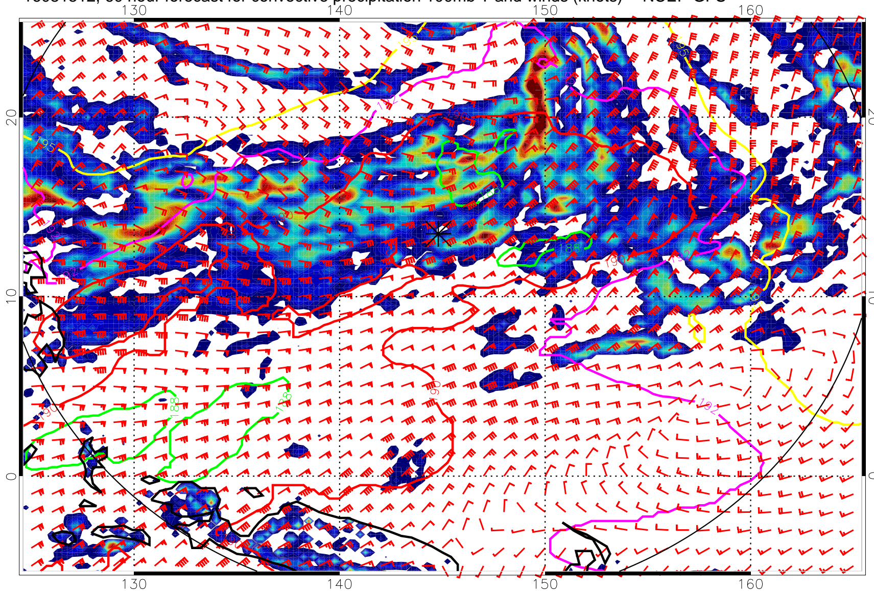
16081512, 60 hour forecast for convective precipitation 100mb T and winds (knots) -- NCEP GFS
