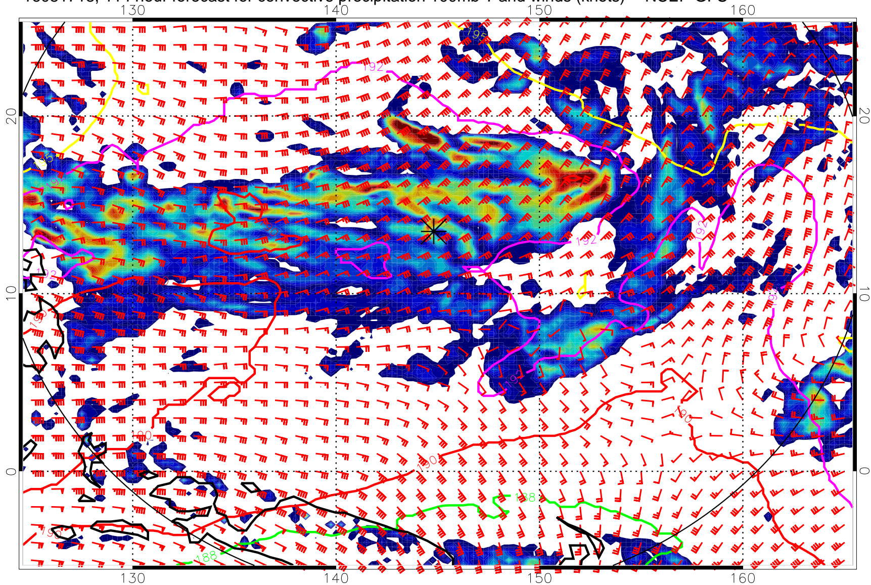
16081718, 114 hour forecast for convective precipitation 100mb T and winds (knots) -- NCEP GFS
