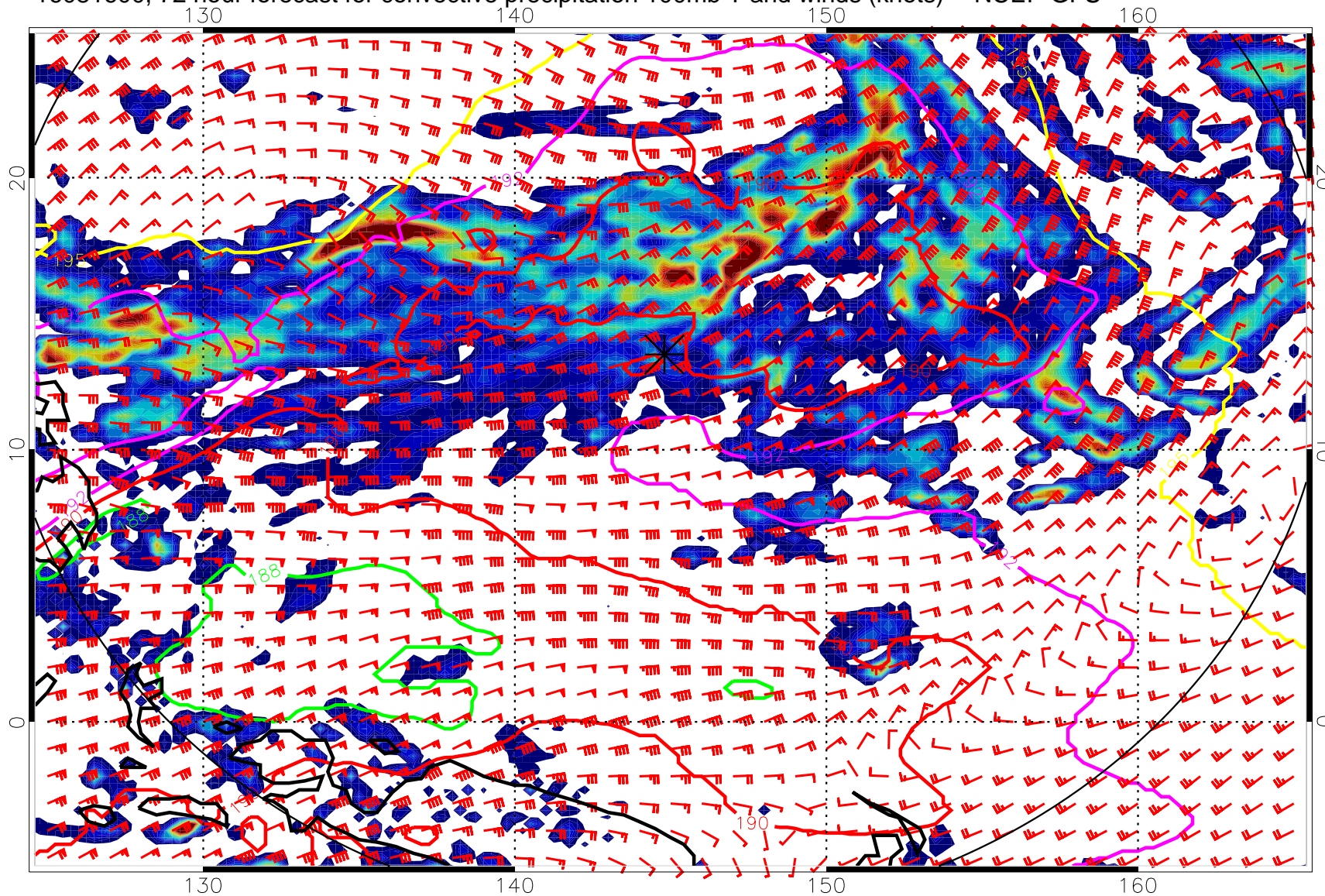
16081600, 72 hour forecast for convective precipitation 100mb T and winds (knots) -- NCEP GFS
