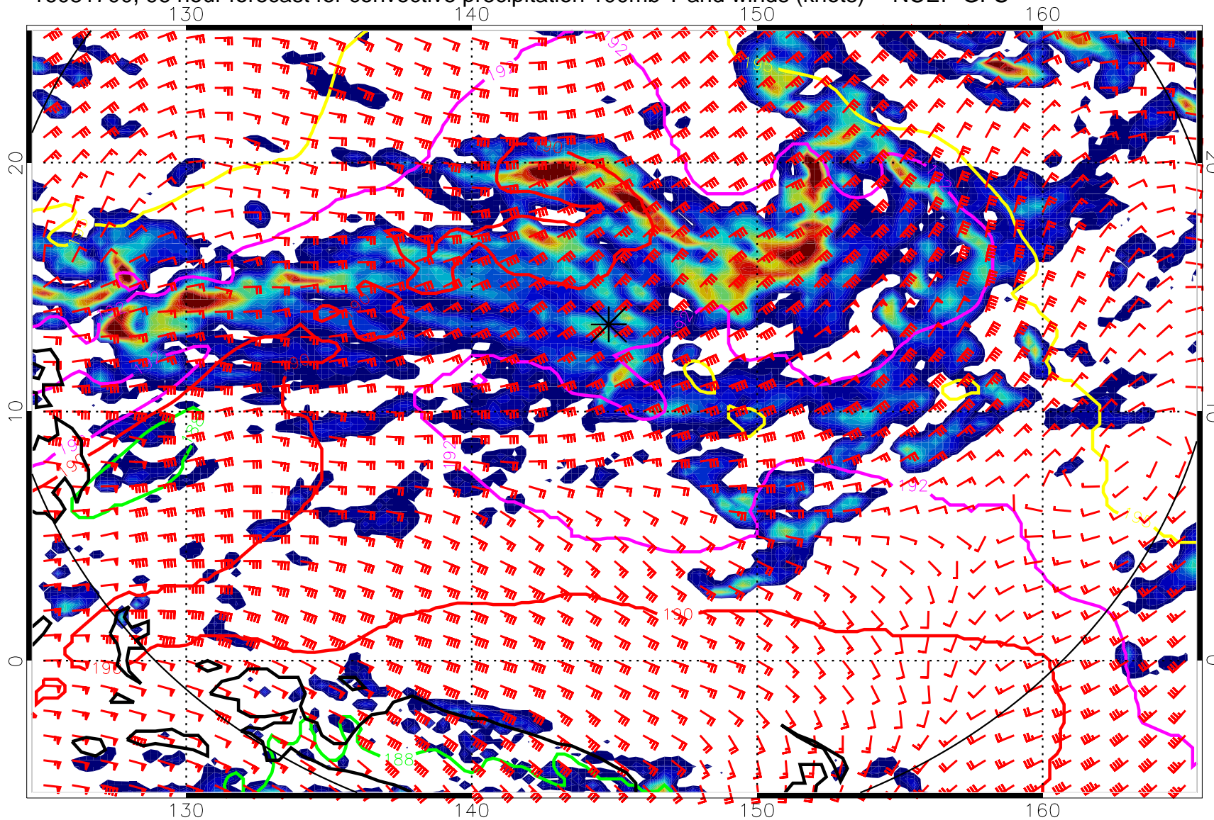
16081700, 96 hour forecast for convective precipitation 100mb T and winds (knots) -- NCEP GFS
