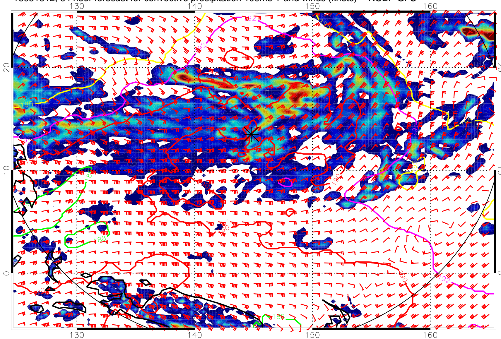
16081612, 84 hour forecast for convective precipitation 100mb T and winds (knots) -- NCEP GFS
