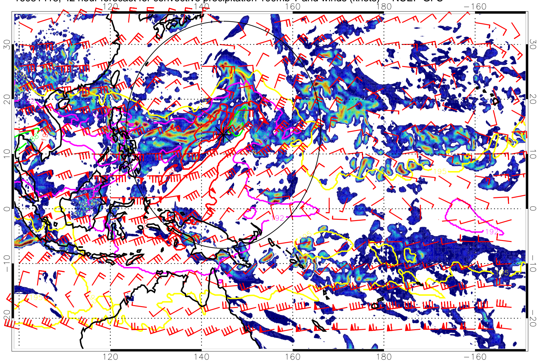
16081418, 42 hour forecast for convective precipitation 100mb T and winds (knots) -- NCEP GFS
