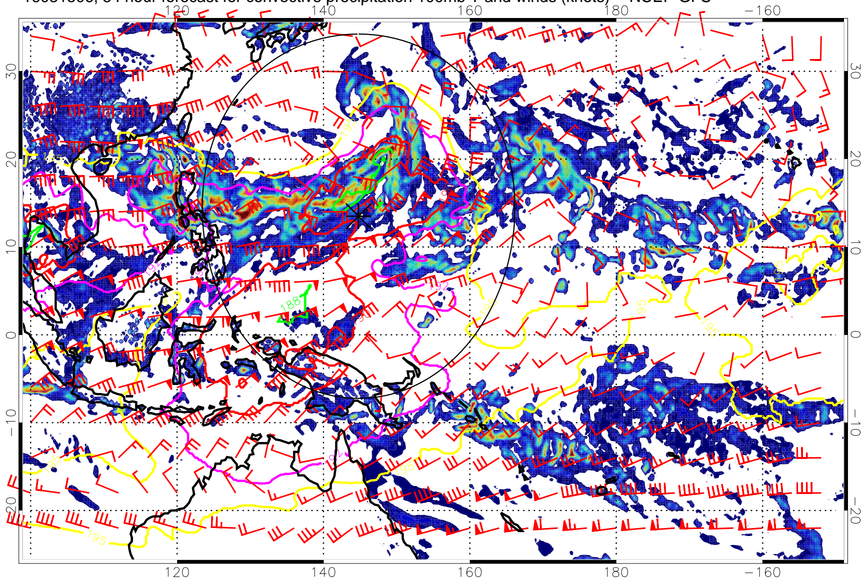
16081506, 54 hour forecast for convective precipitation 100mb T and winds (knots) -- NCEP GFS
