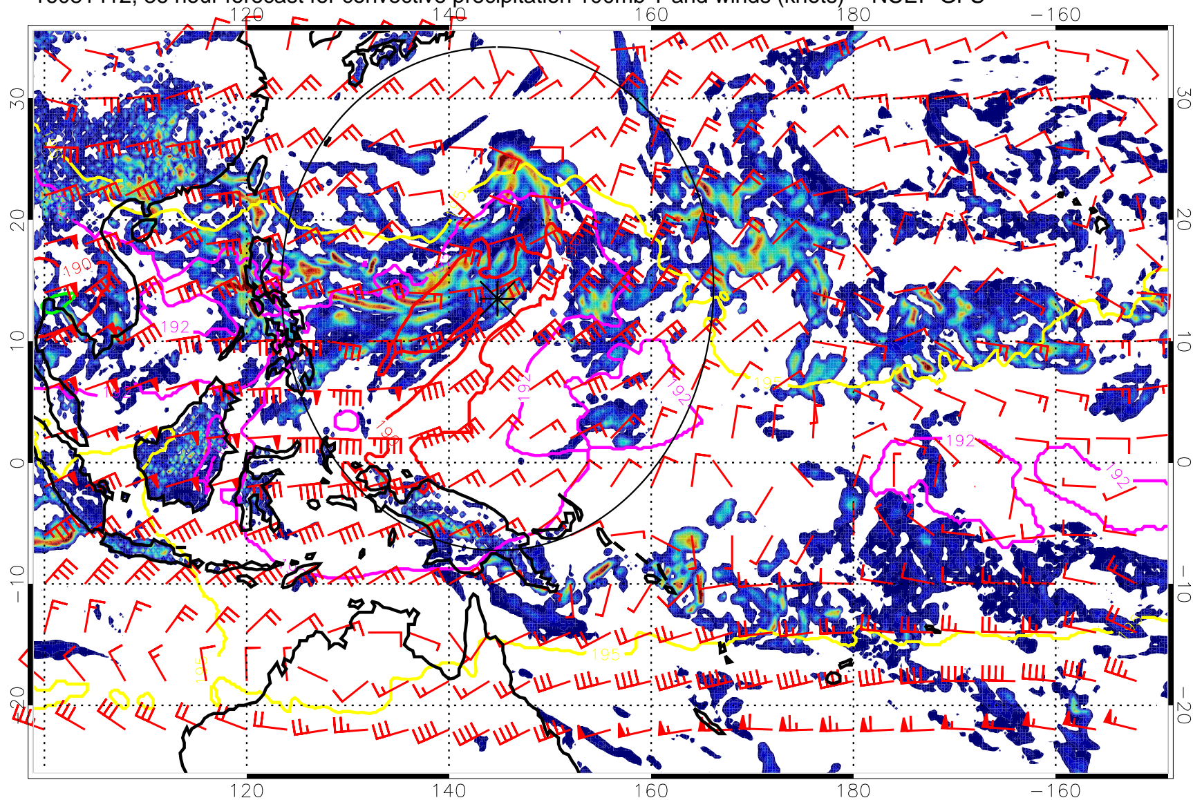
16081412, 36 hour forecast for convective precipitation 100mb T and winds (knots) -- NCEP GFS
