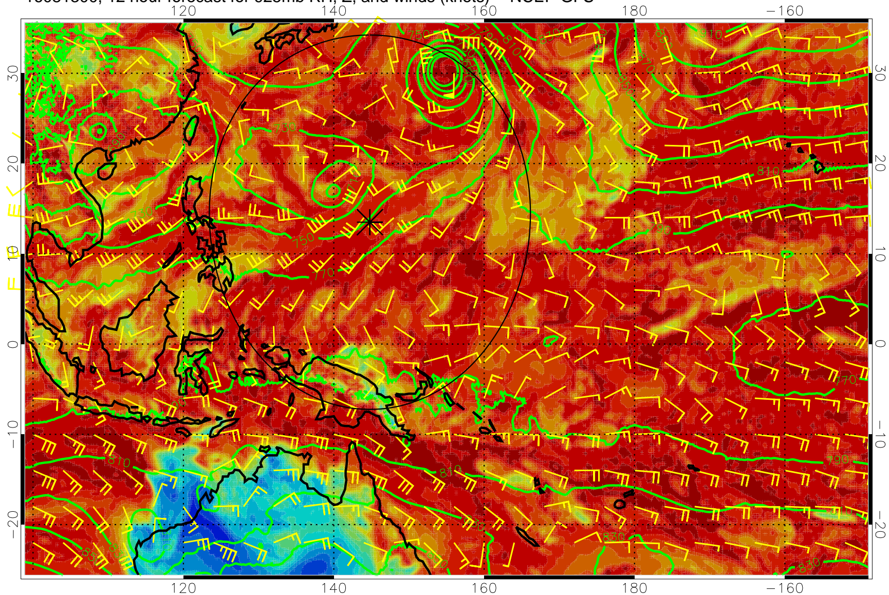
16081300, 12 hour forecast for 925mb RH, Z, and winds (knots) -- NCEP GFS
