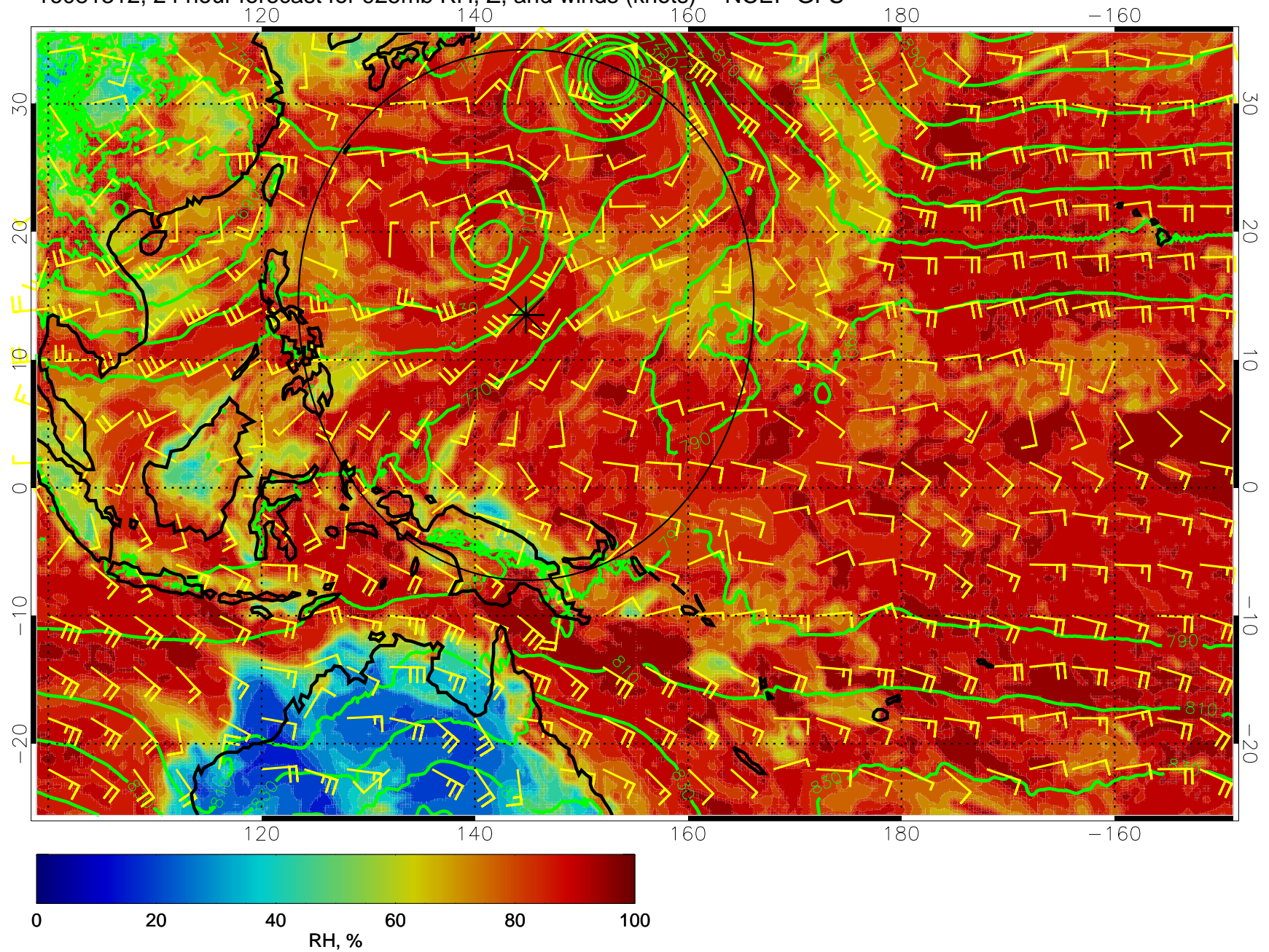
16081312, 24 hour forecast for 925mb RH, Z, and winds (knots) -- NCEP GFS
