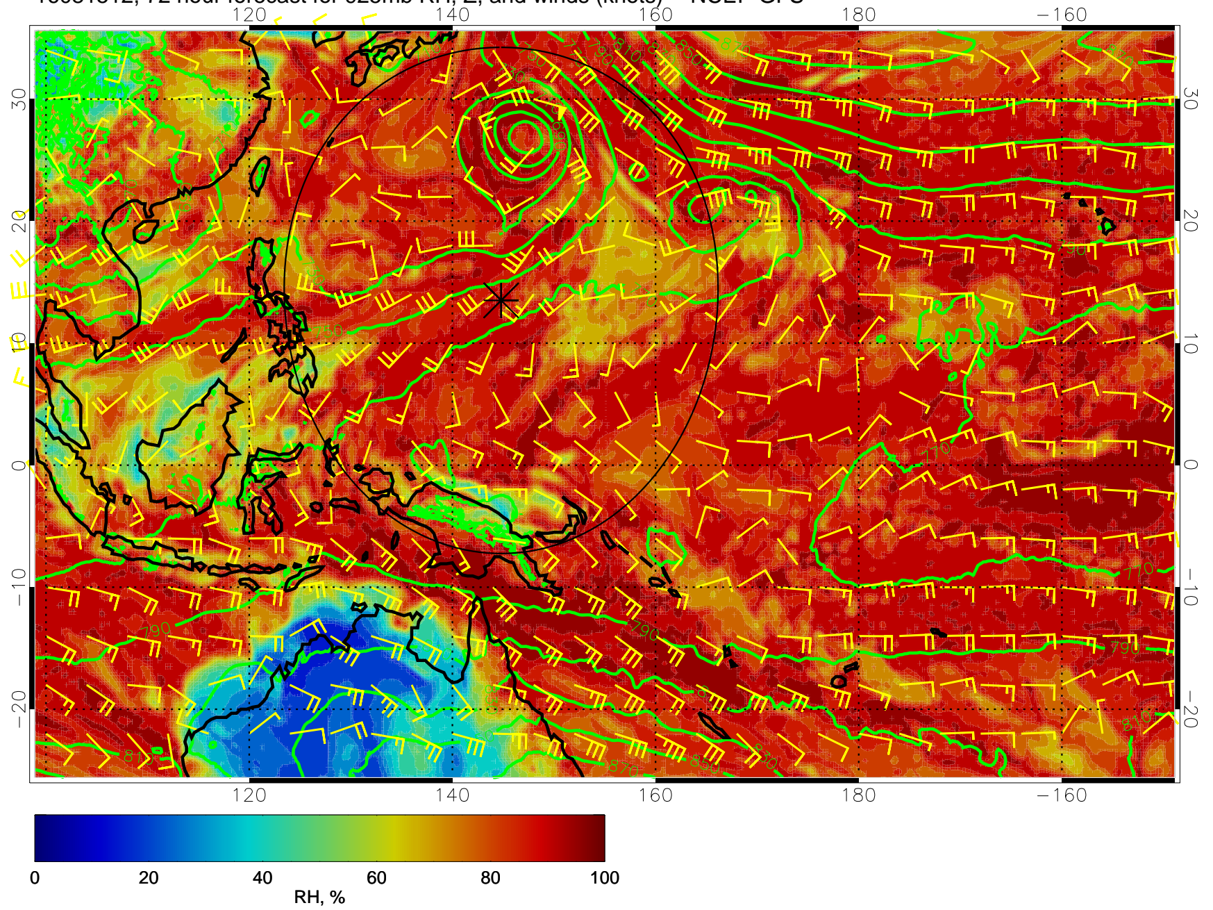
16081512, 72 hour forecast for 925mb RH, Z, and winds (knots) -- NCEP GFS
