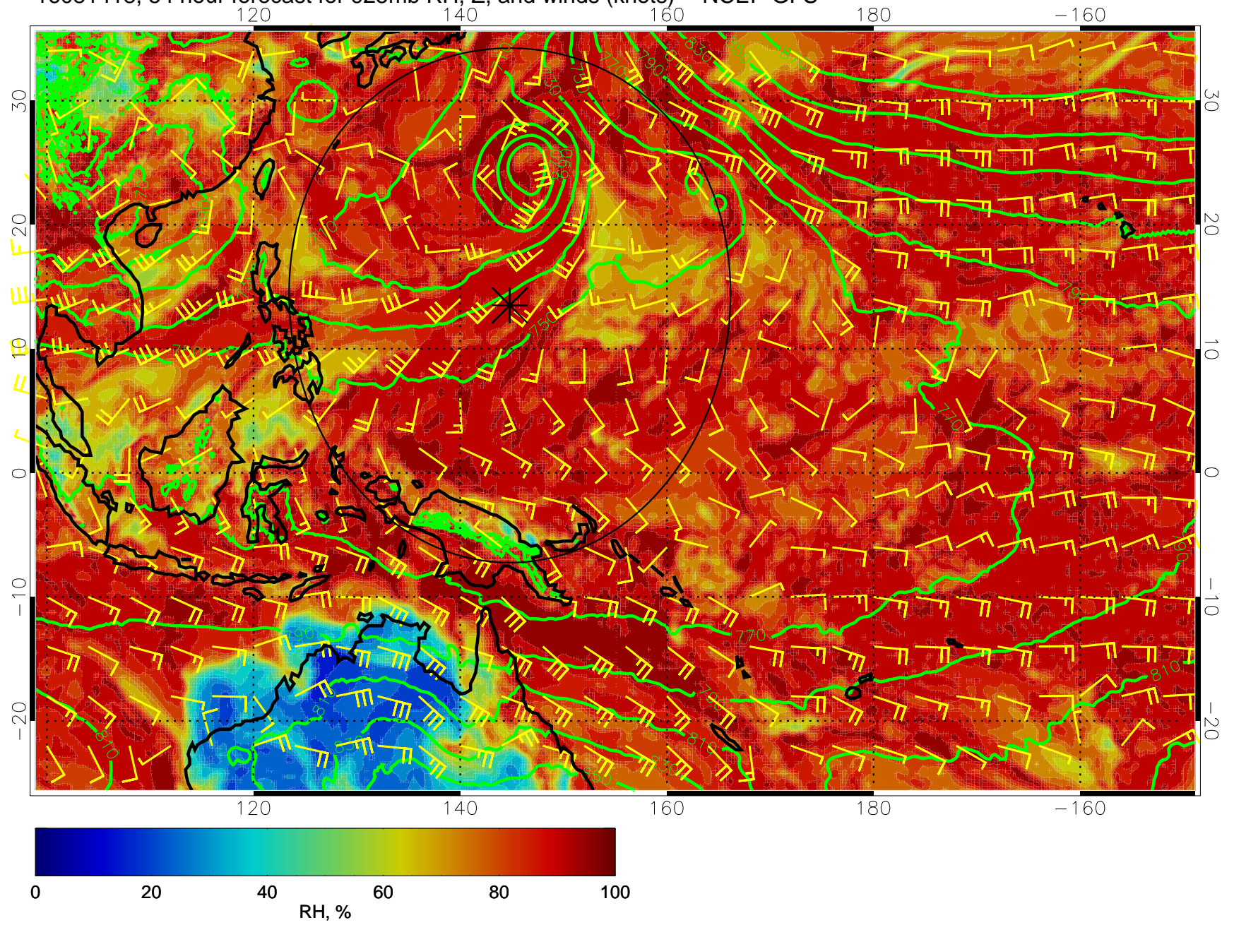
16081418, 54 hour forecast for 925mb RH, Z, and winds (knots) -- NCEP GFS
