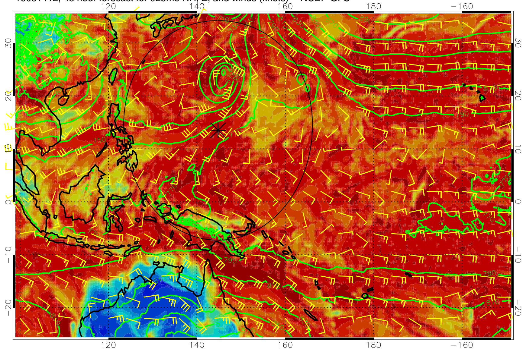
16081412, 48 hour forecast for 925mb RH, Z, and winds (knots) -- NCEP GFS
