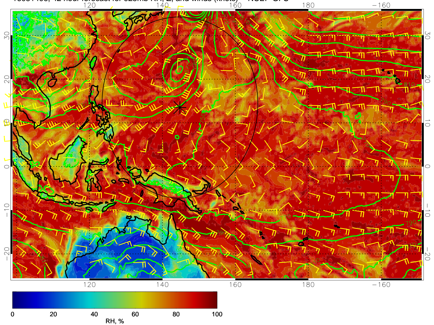
16081406, 42 hour forecast for 925mb RH, Z, and winds (knots) -- NCEP GFS
