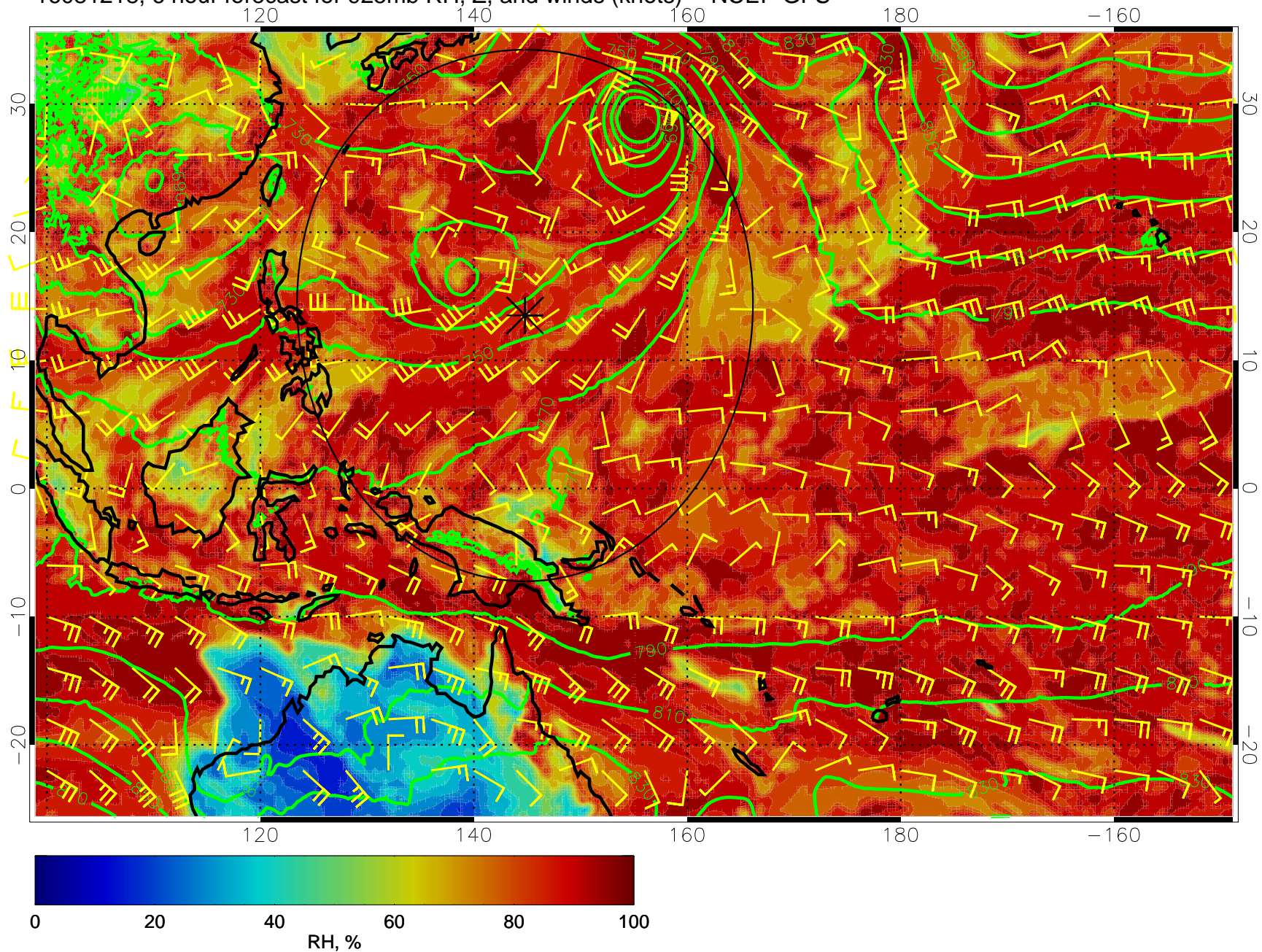
16081218, 6 hour forecast for 925mb RH, Z, and winds (knots) -- NCEP GFS
