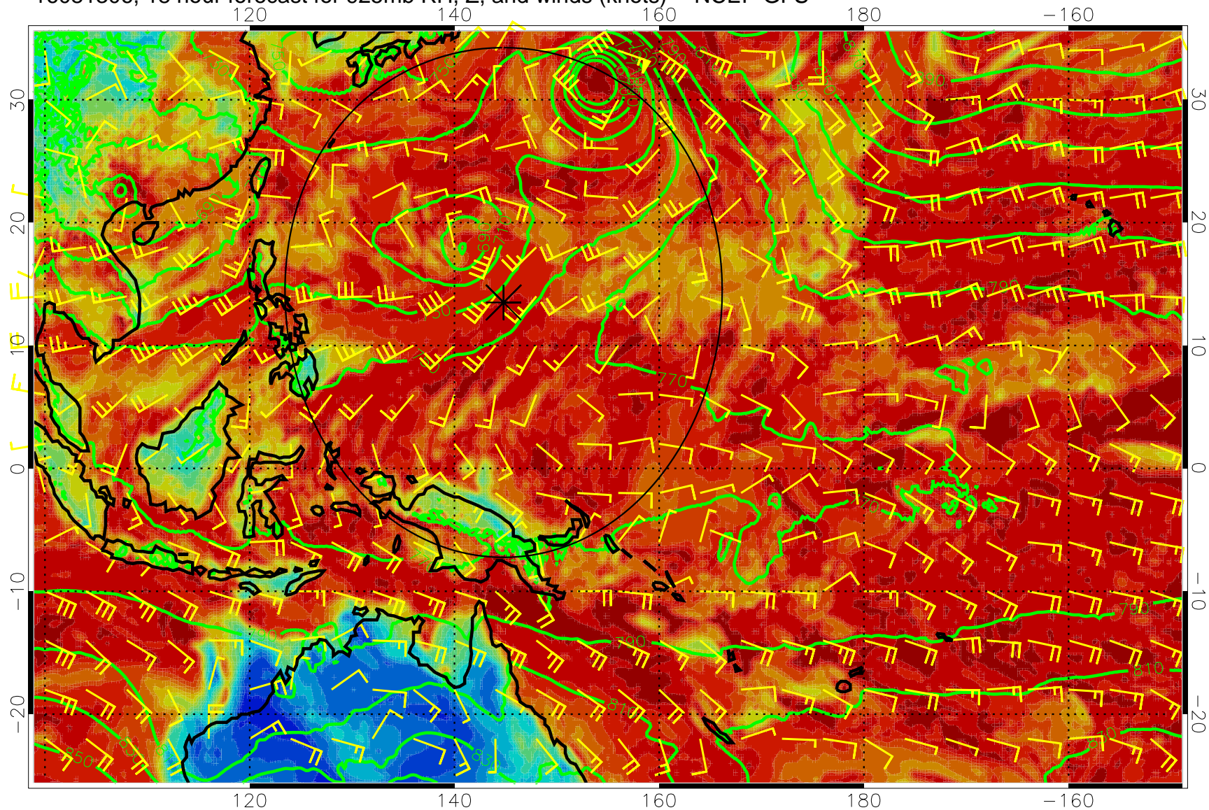
16081306, 18 hour forecast for 925mb RH, Z, and winds (knots) -- NCEP GFS
