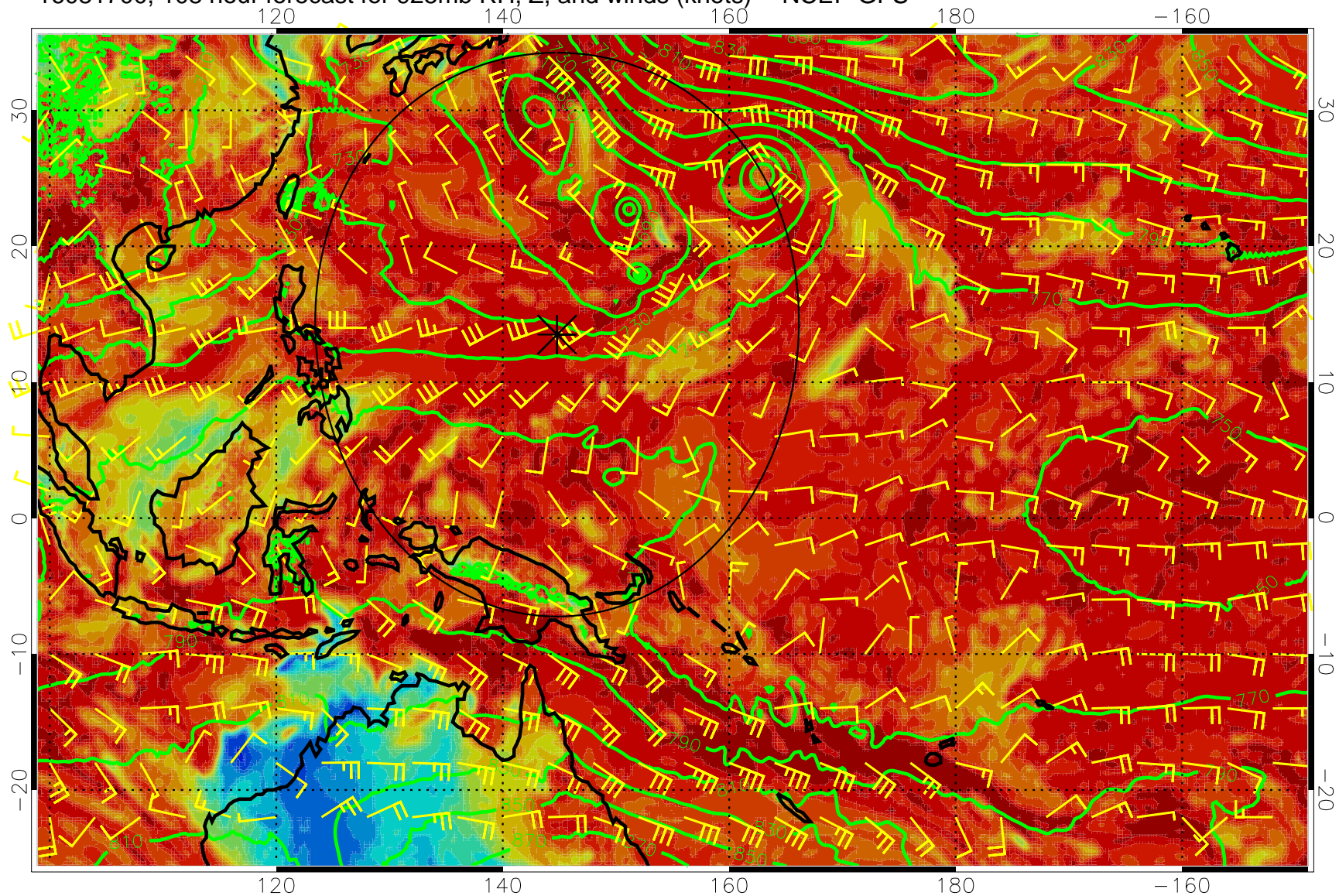
16081700, 108 hour forecast for 925mb RH, Z, and winds (knots) -- NCEP GFS
