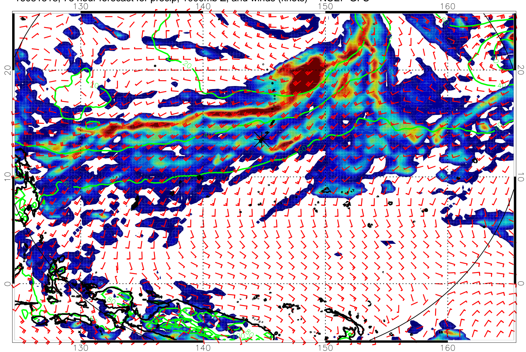
16081518, 78 hour forecast for precip, 1000mb Z, and winds (knots) -- NCEP GFS
