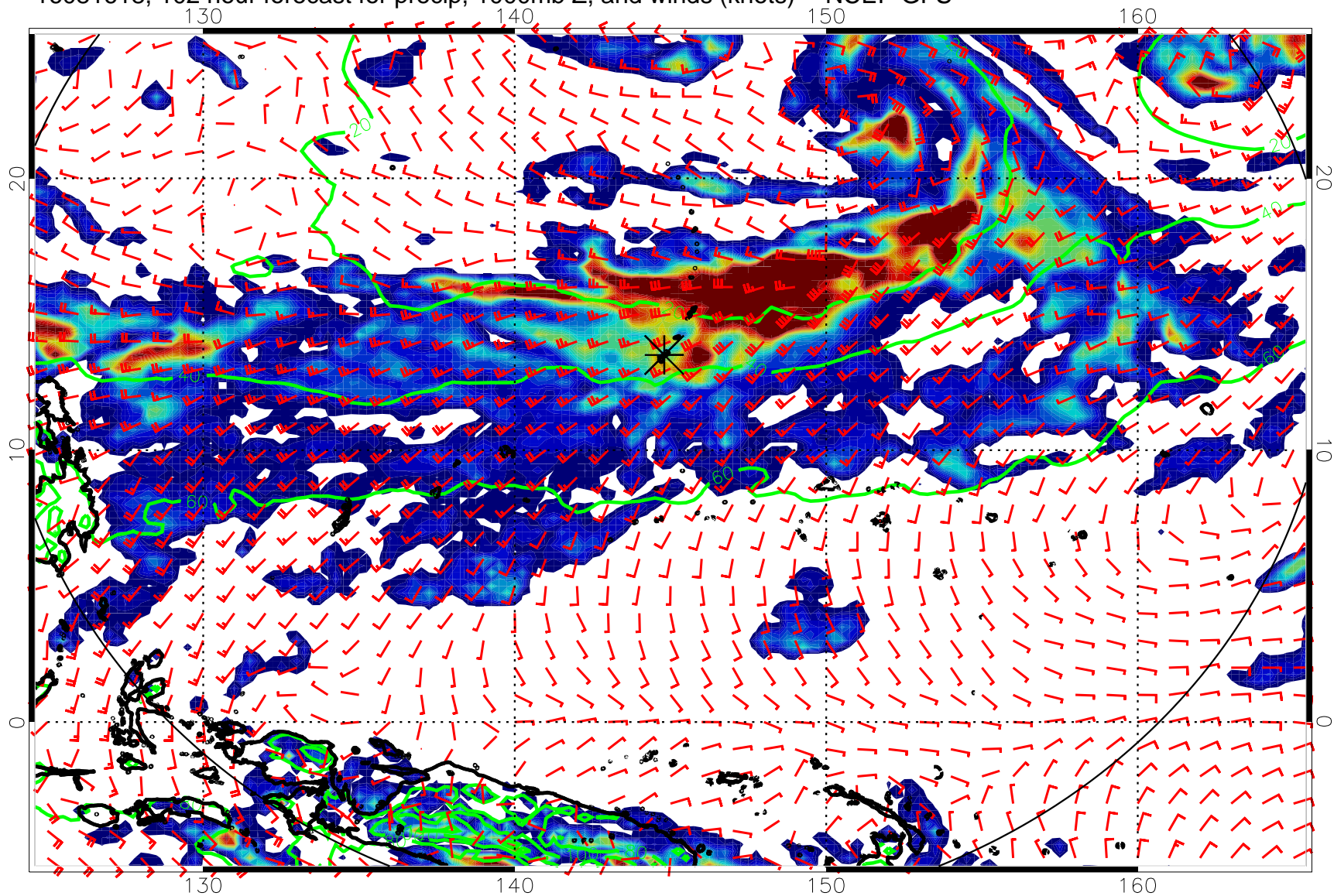
16081618, 102 hour forecast for precip, 1000mb Z, and winds (knots) -- NCEP GFS
