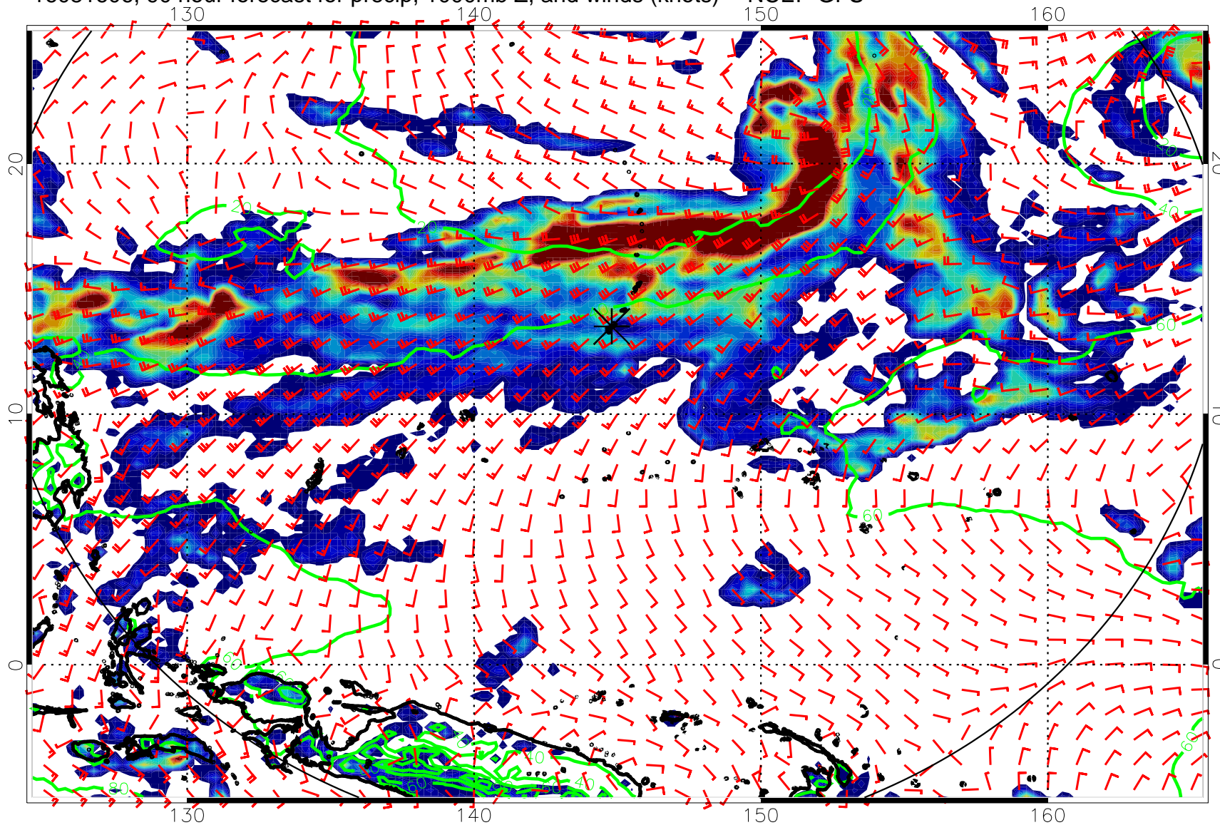
16081606, 90 hour forecast for precip, 1000mb Z, and winds (knots) -- NCEP GFS
