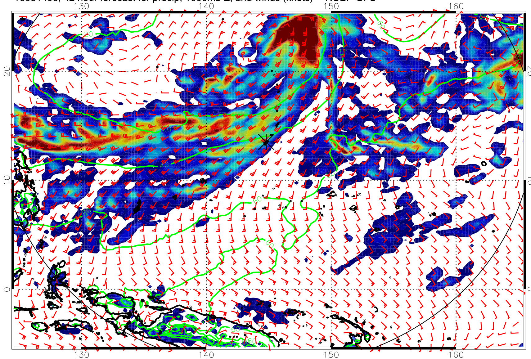
16081406, 42 hour forecast for precip, 1000mb Z, and winds (knots) -- NCEP GFS
