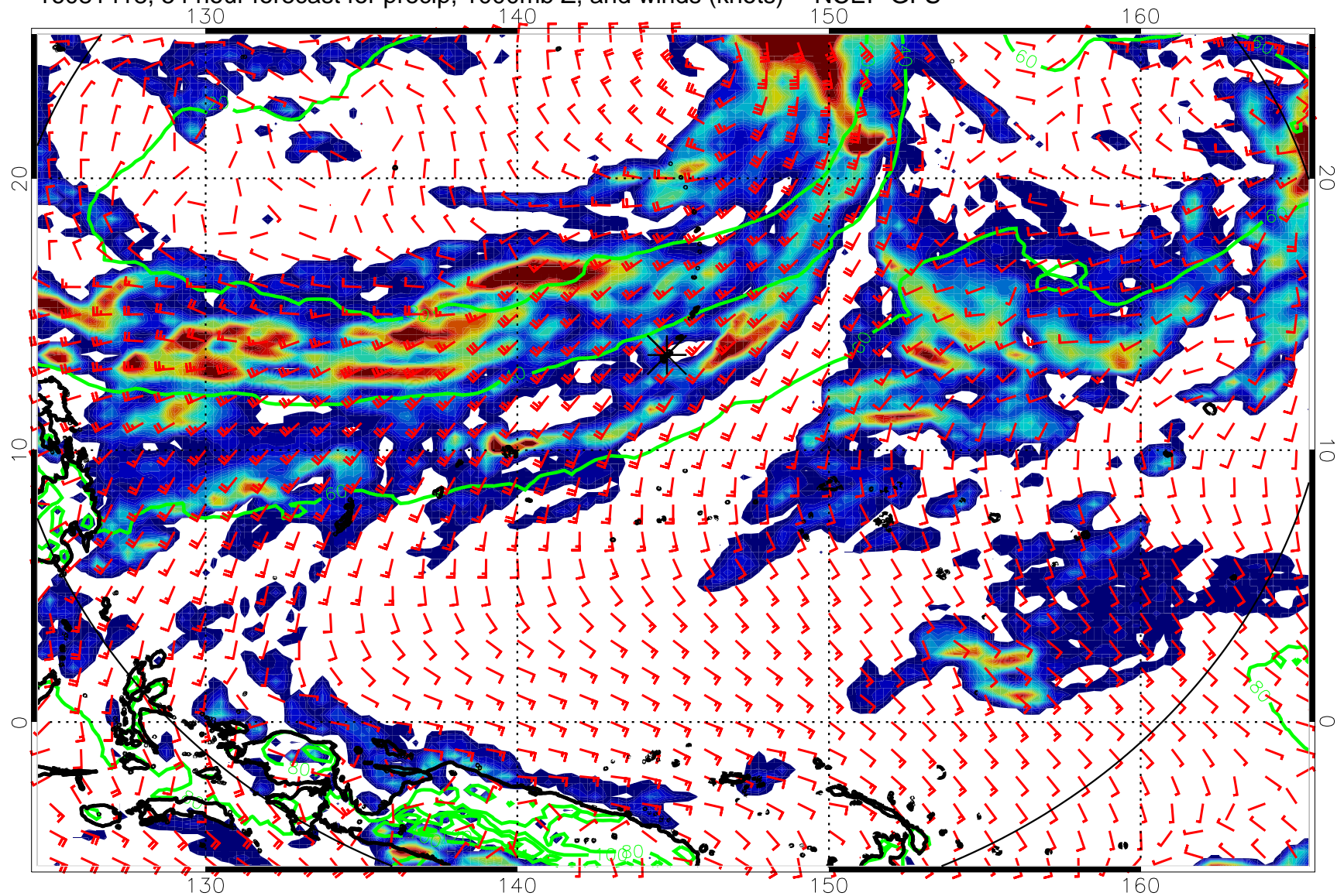
16081418, 54 hour forecast for precip, 1000mb Z, and winds (knots) -- NCEP GFS
