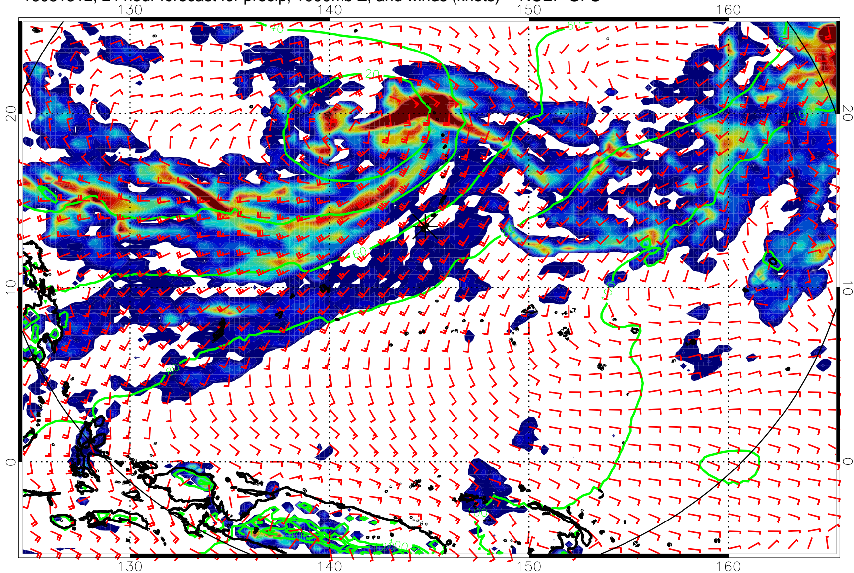
16081312, 24 hour forecast for precip, 1000mb Z, and winds (knots) -- NCEP GFS
