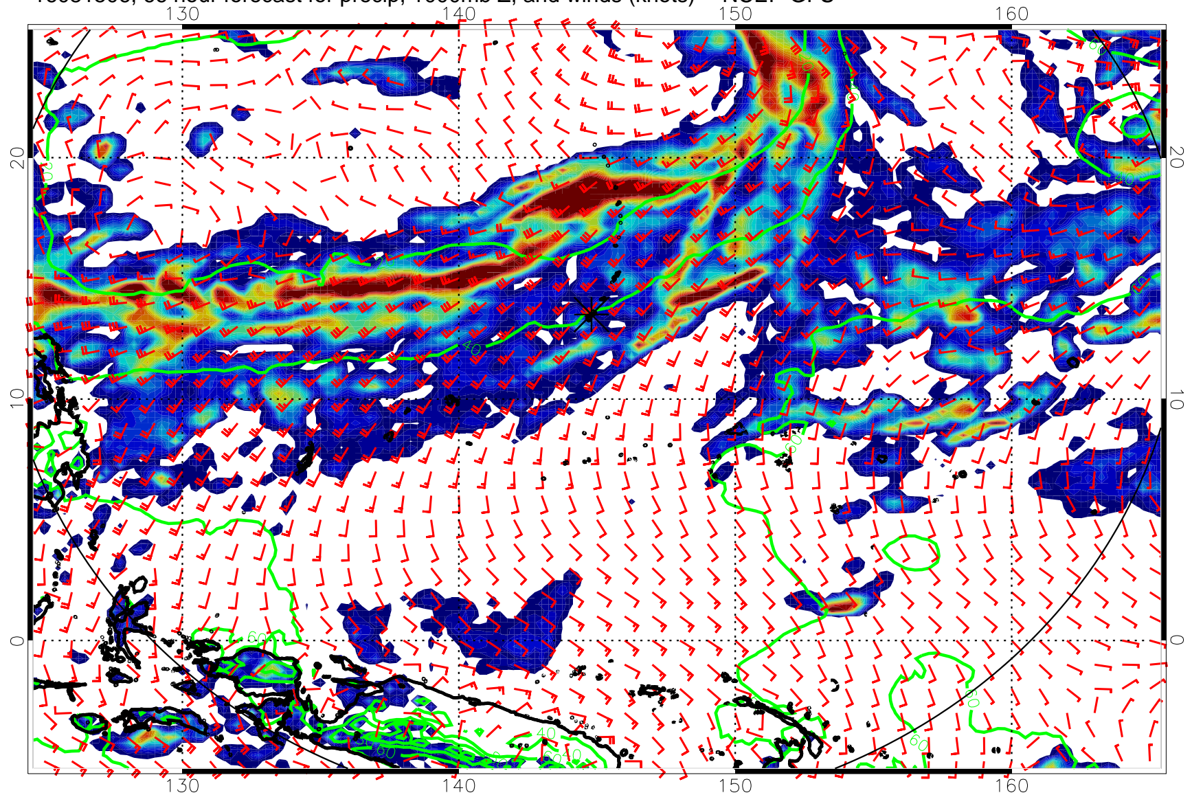
16081506, 66 hour forecast for precip, 1000mb Z, and winds (knots) -- NCEP GFS
