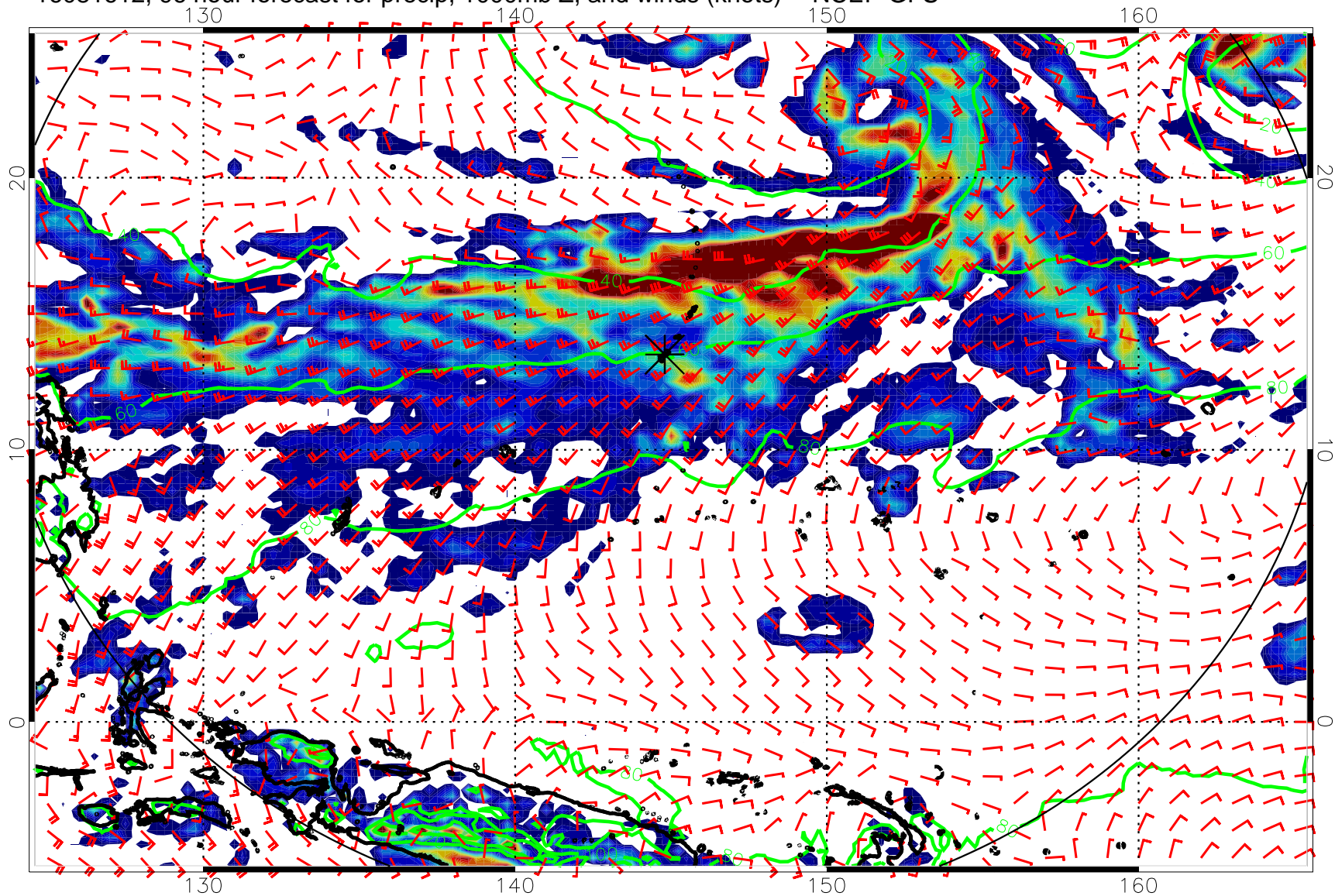
16081612, 96 hour forecast for precip, 1000mb Z, and winds (knots) -- NCEP GFS
