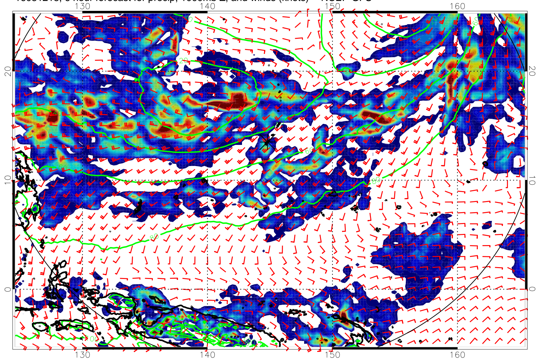
16081218, 6 hour forecast for precip, 1000mb Z, and winds (knots) -- NCEP GFS
