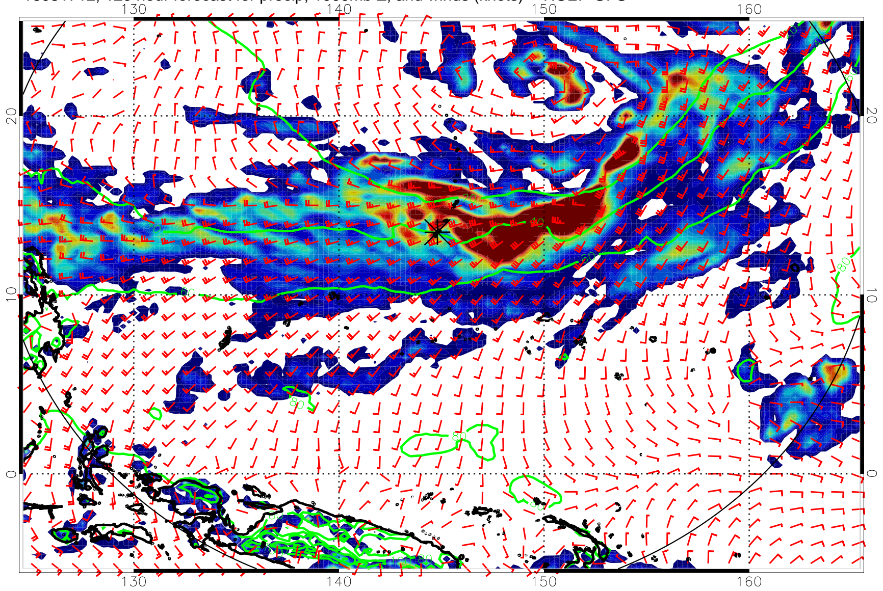
16081712, 120 hour forecast for precip, 1000mb Z, and winds (knots) -- NCEP GFS
