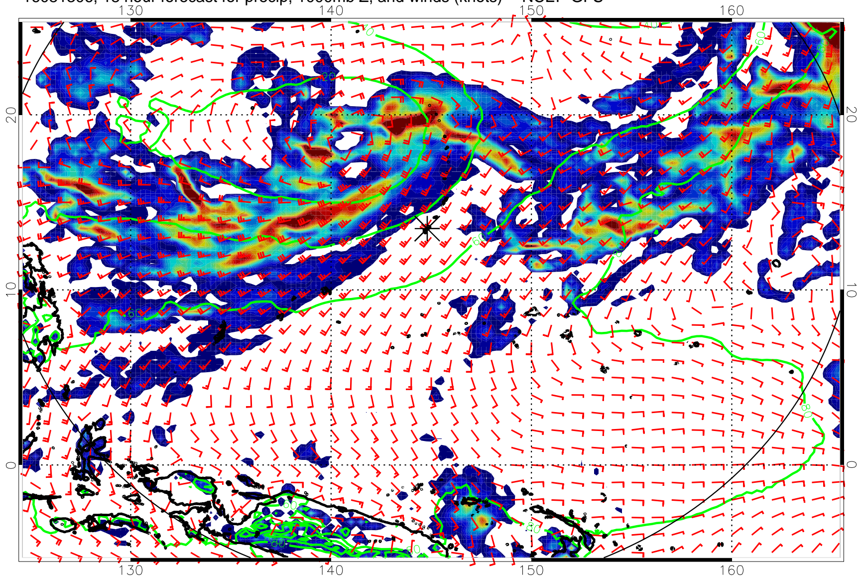
16081306, 18 hour forecast for precip, 1000mb Z, and winds (knots) -- NCEP GFS
