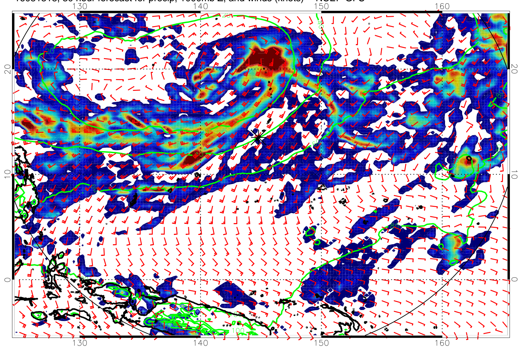
16081318, 30 hour forecast for precip, 1000mb Z, and winds (knots) -- NCEP GFS
