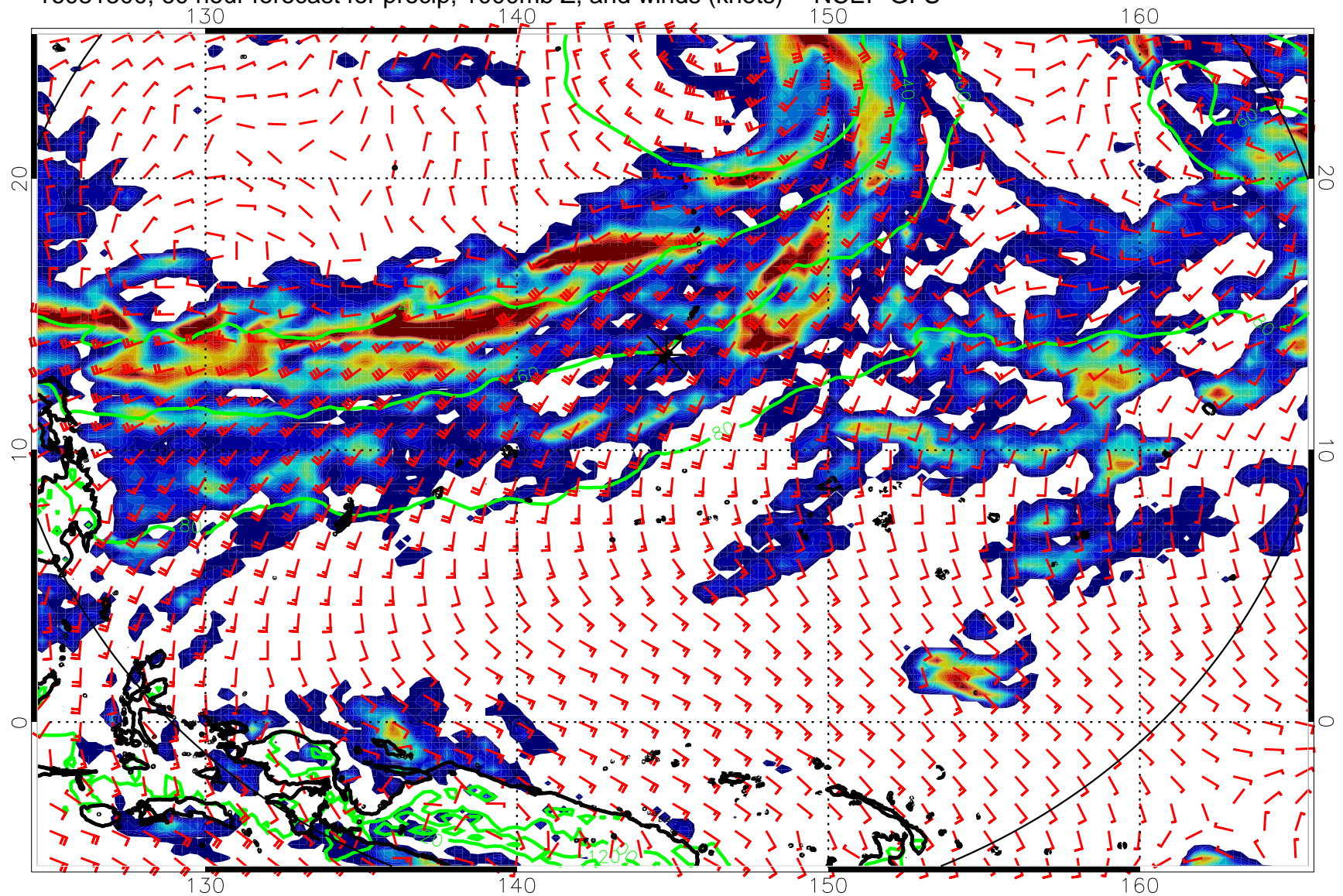
16081500, 60 hour forecast for precip, 1000mb Z, and winds (knots) -- NCEP GFS
