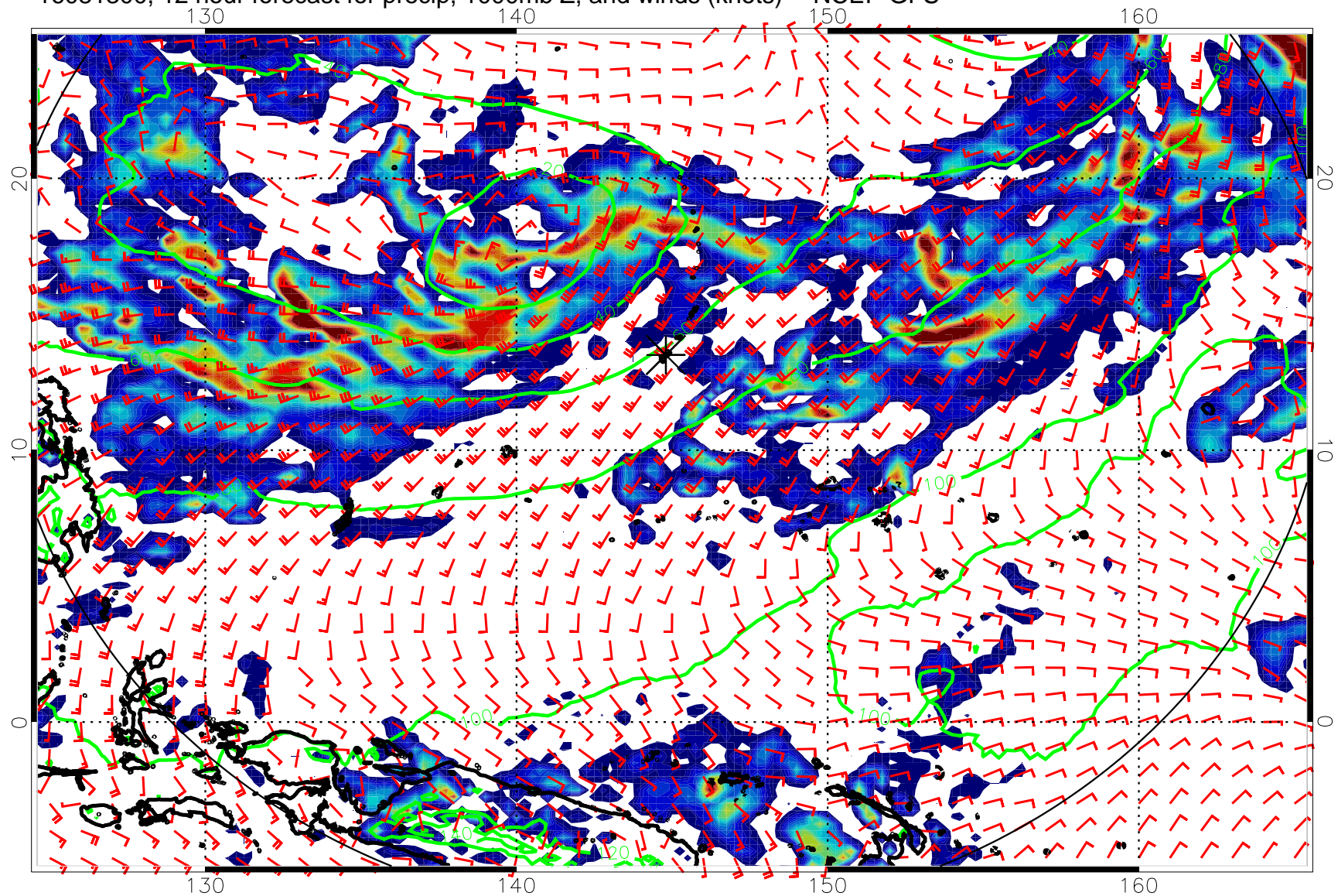
16081300, 12 hour forecast for precip, 1000mb Z, and winds (knots) -- NCEP GFS
