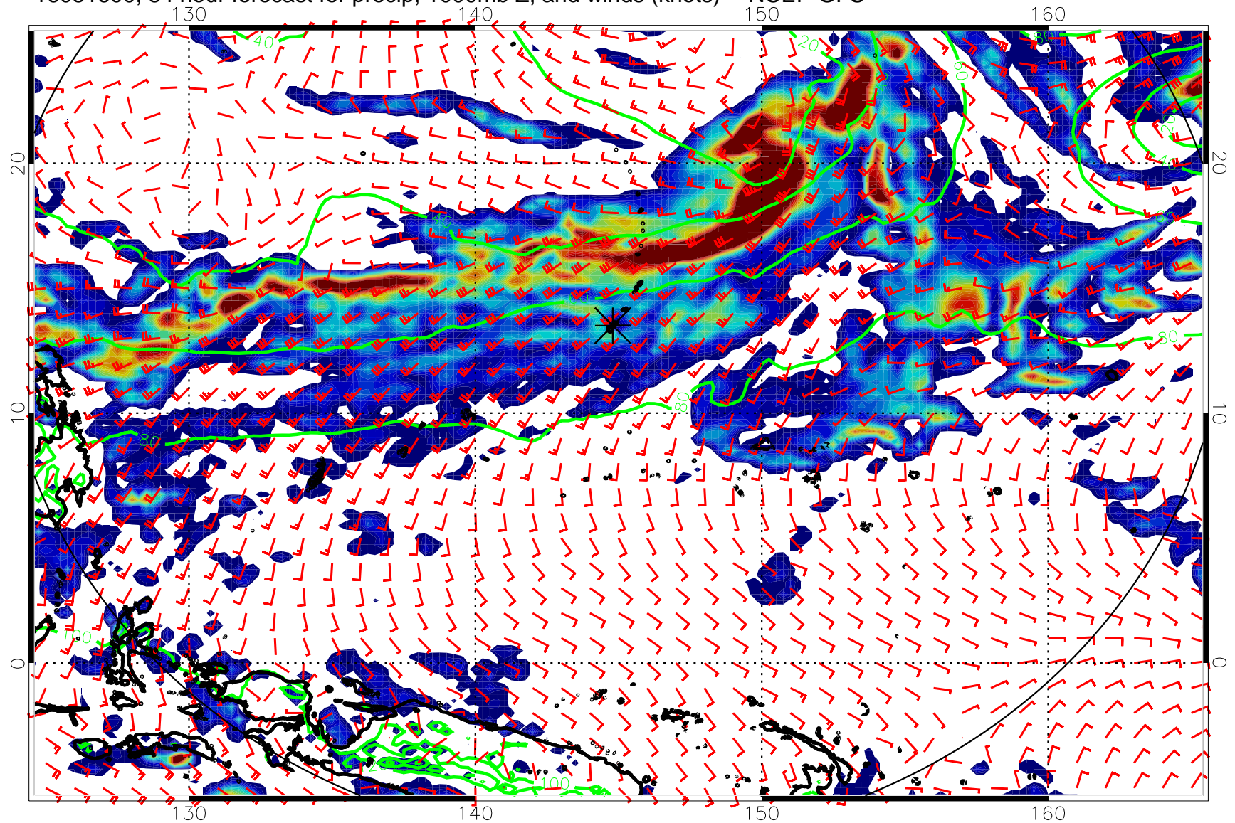
16081600, 84 hour forecast for precip, 1000mb Z, and winds (knots) -- NCEP GFS
