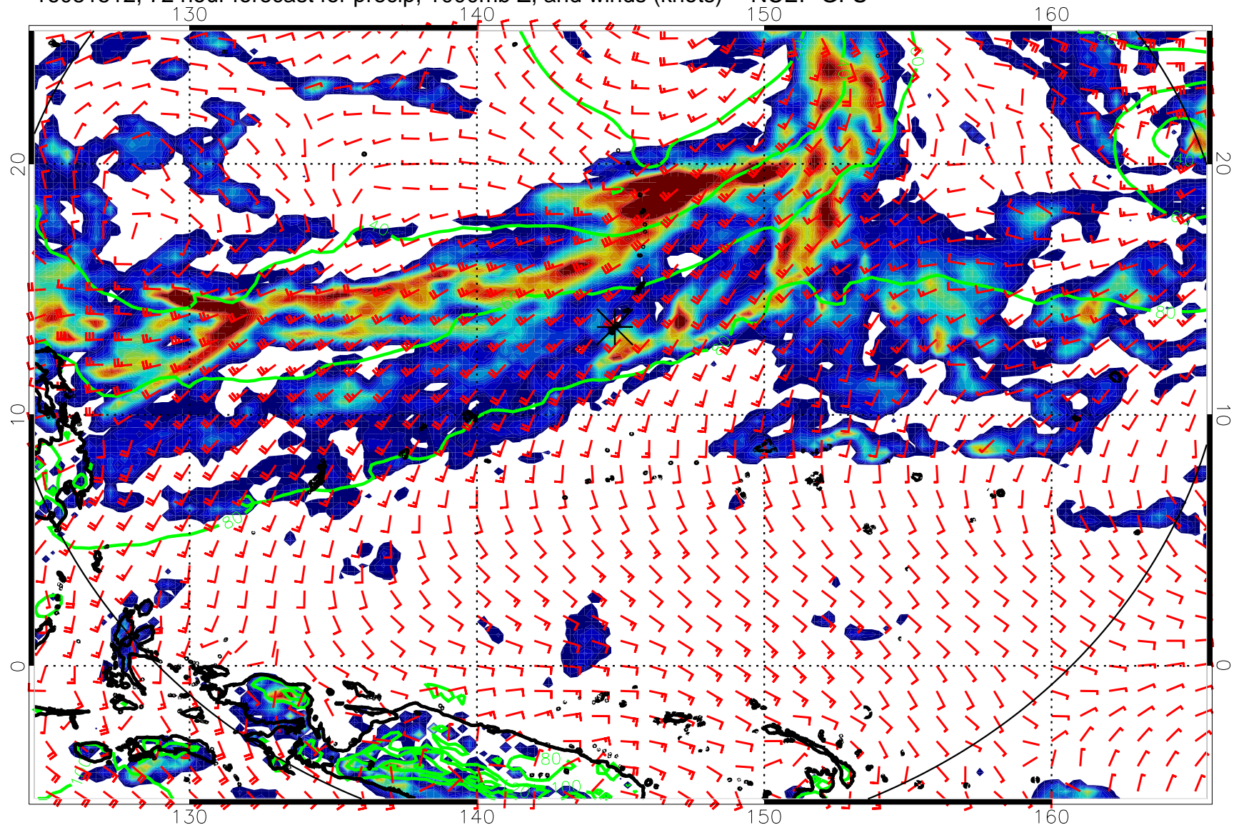
16081512, 72 hour forecast for precip, 1000mb Z, and winds (knots) -- NCEP GFS
