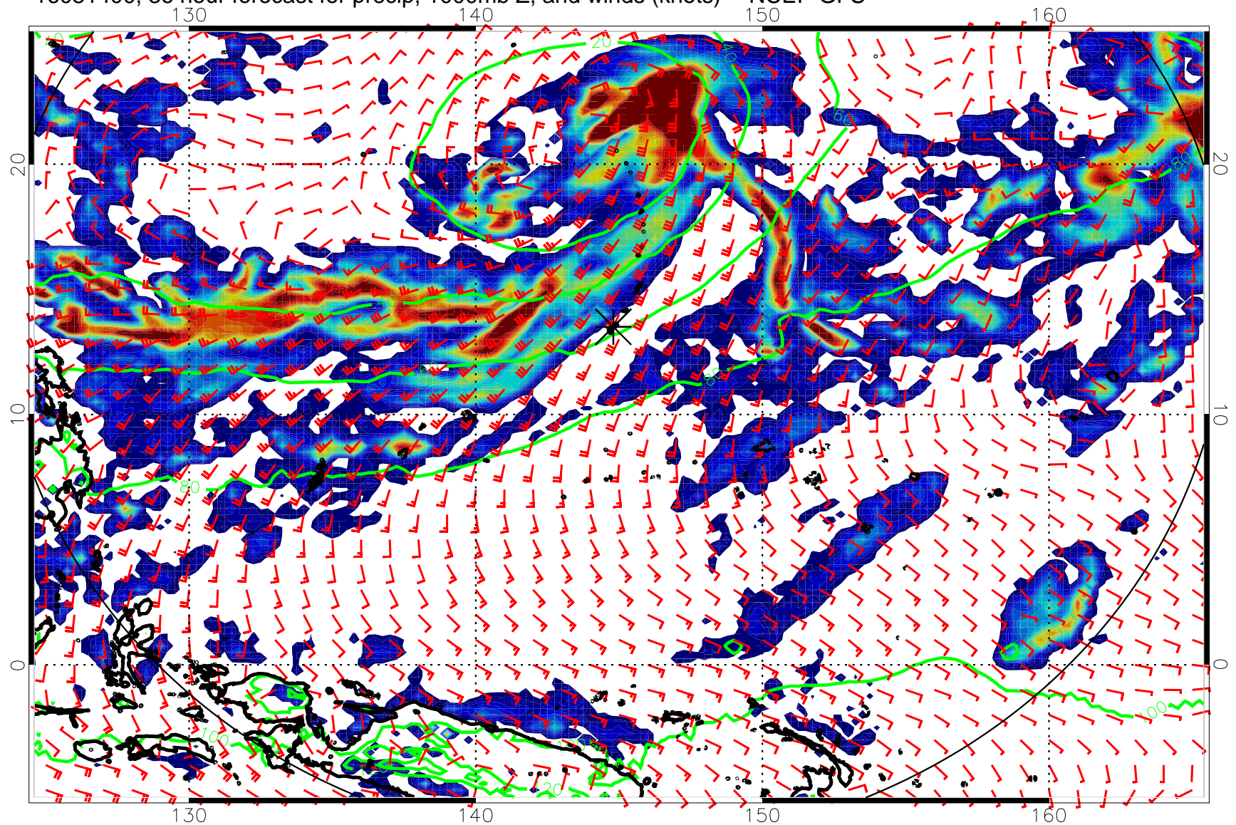
16081400, 36 hour forecast for precip, 1000mb Z, and winds (knots) -- NCEP GFS
