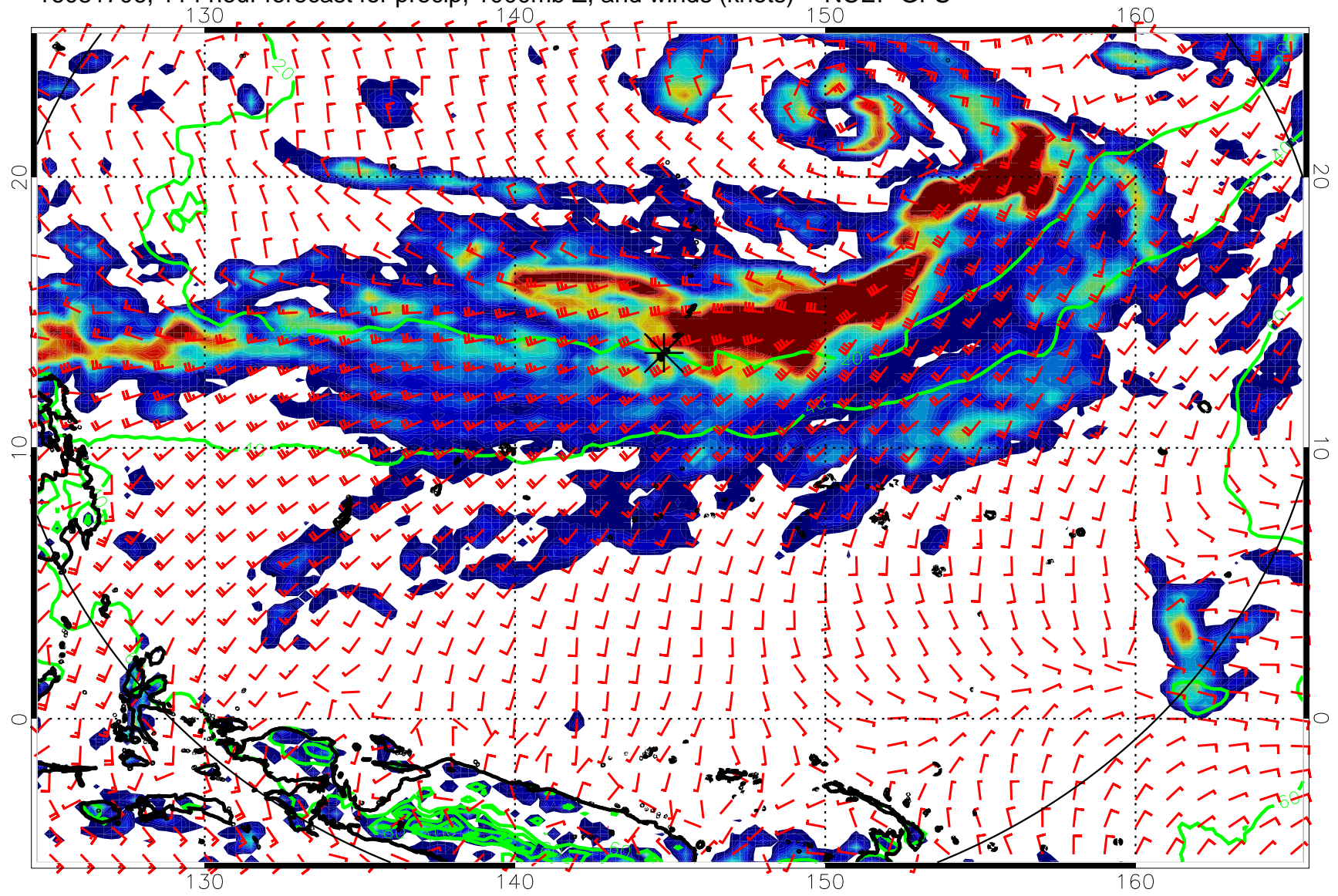
16081706, 114 hour forecast for precip, 1000mb Z, and winds (knots) -- NCEP GFS
