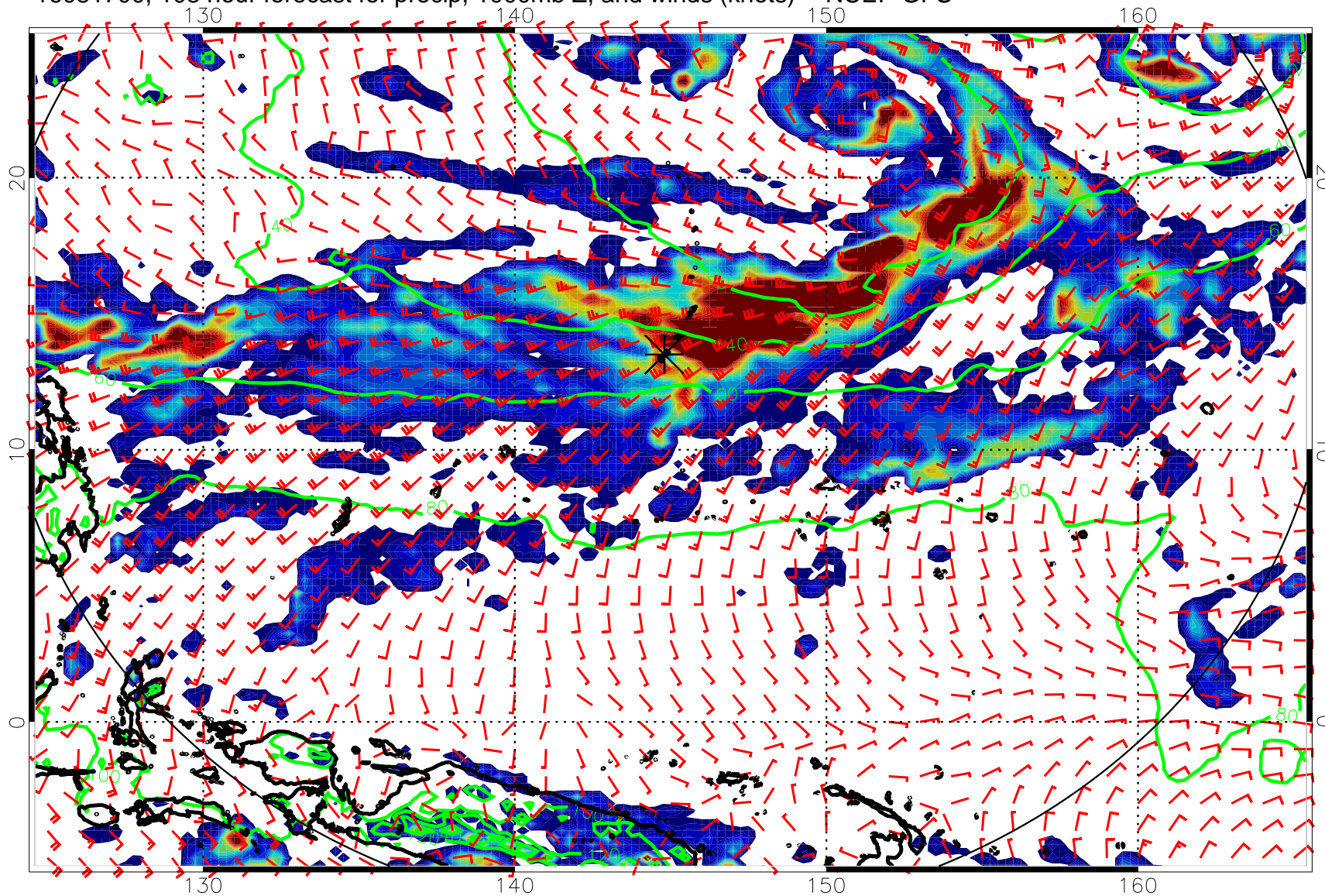
16081700, 108 hour forecast for precip, 1000mb Z, and winds (knots) -- NCEP GFS
