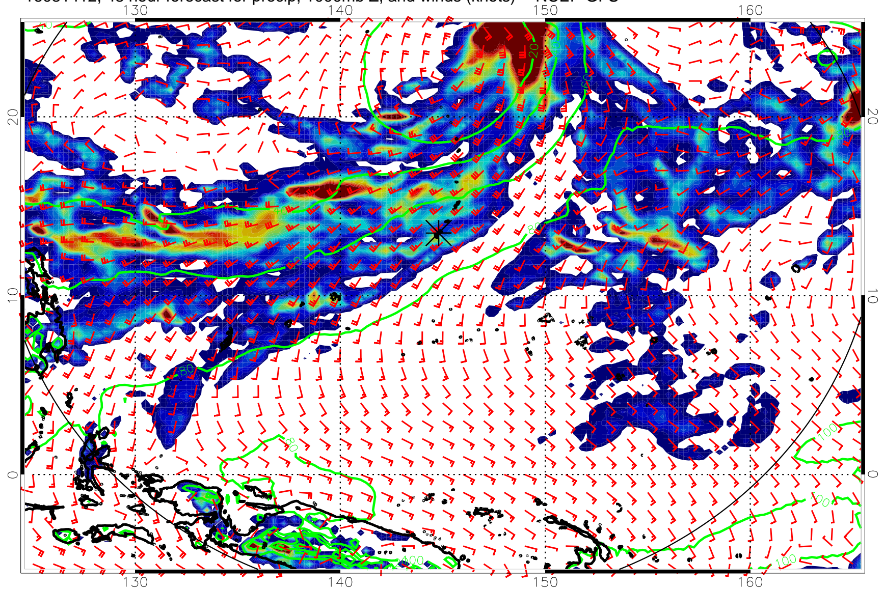
16081412, 48 hour forecast for precip, 1000mb Z, and winds (knots) -- NCEP GFS
