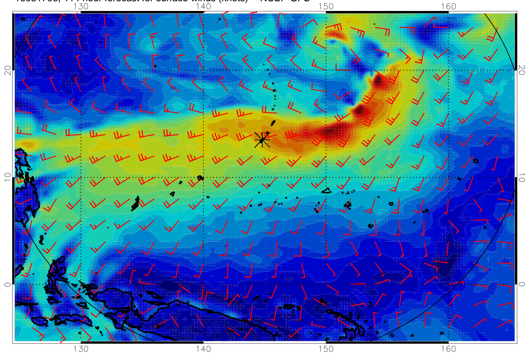
16081706, 114 hour forecast for surface winds (knots) -- NCEP GFS
