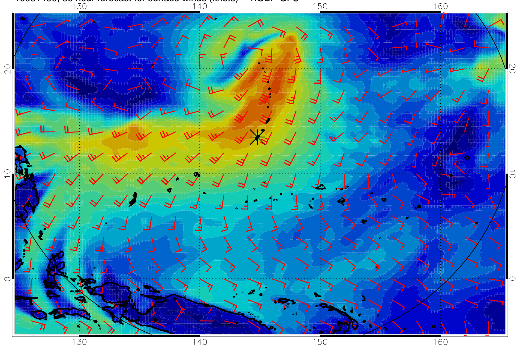
16081400, 36 hour forecast for surface winds (knots) -- NCEP GFS
