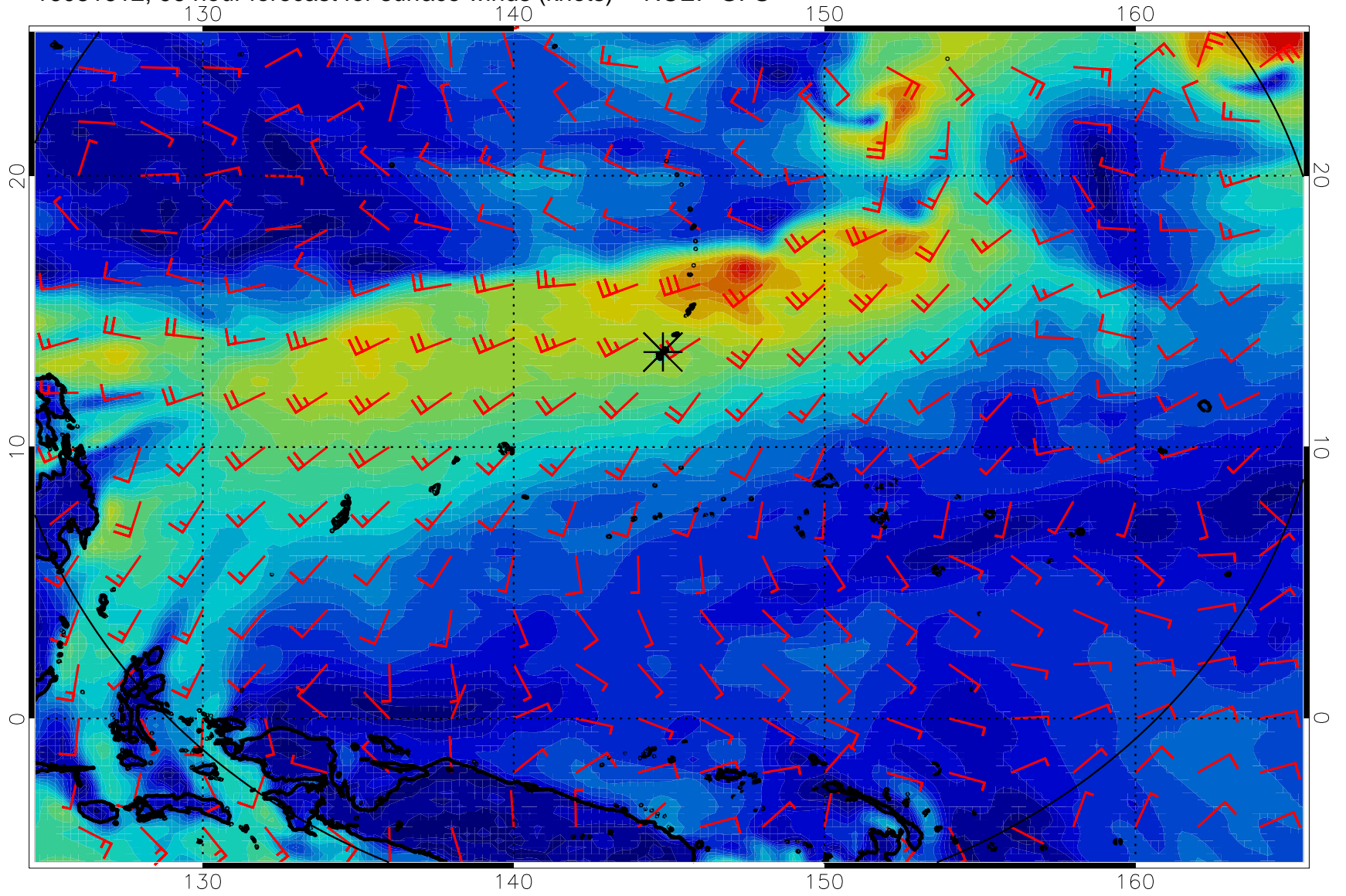
16081612, 96 hour forecast for surface winds (knots) -- NCEP GFS
