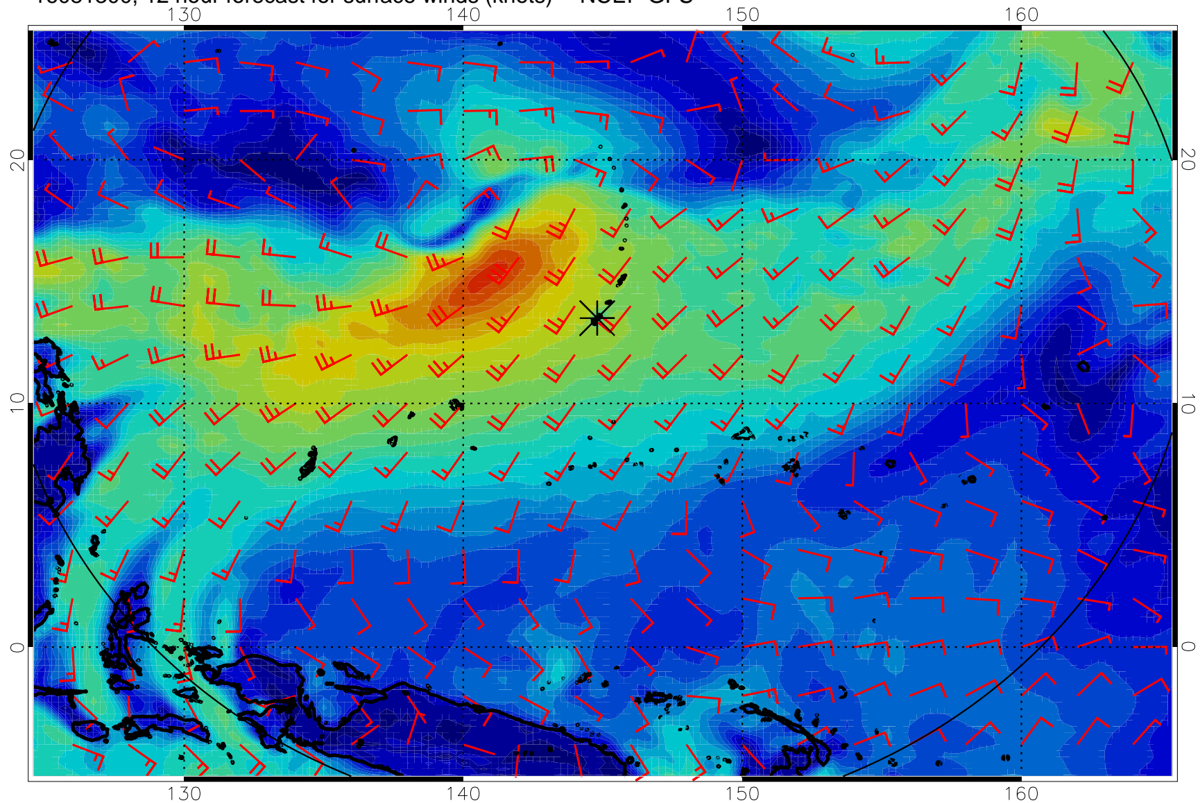
16081300, 12 hour forecast for surface winds (knots) -- NCEP GFS
