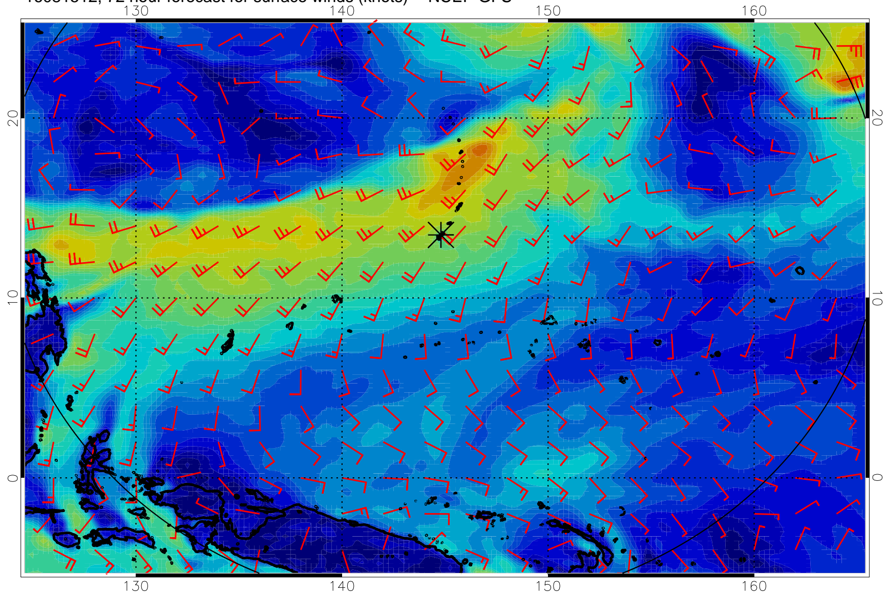
16081512, 72 hour forecast for surface winds (knots) -- NCEP GFS
