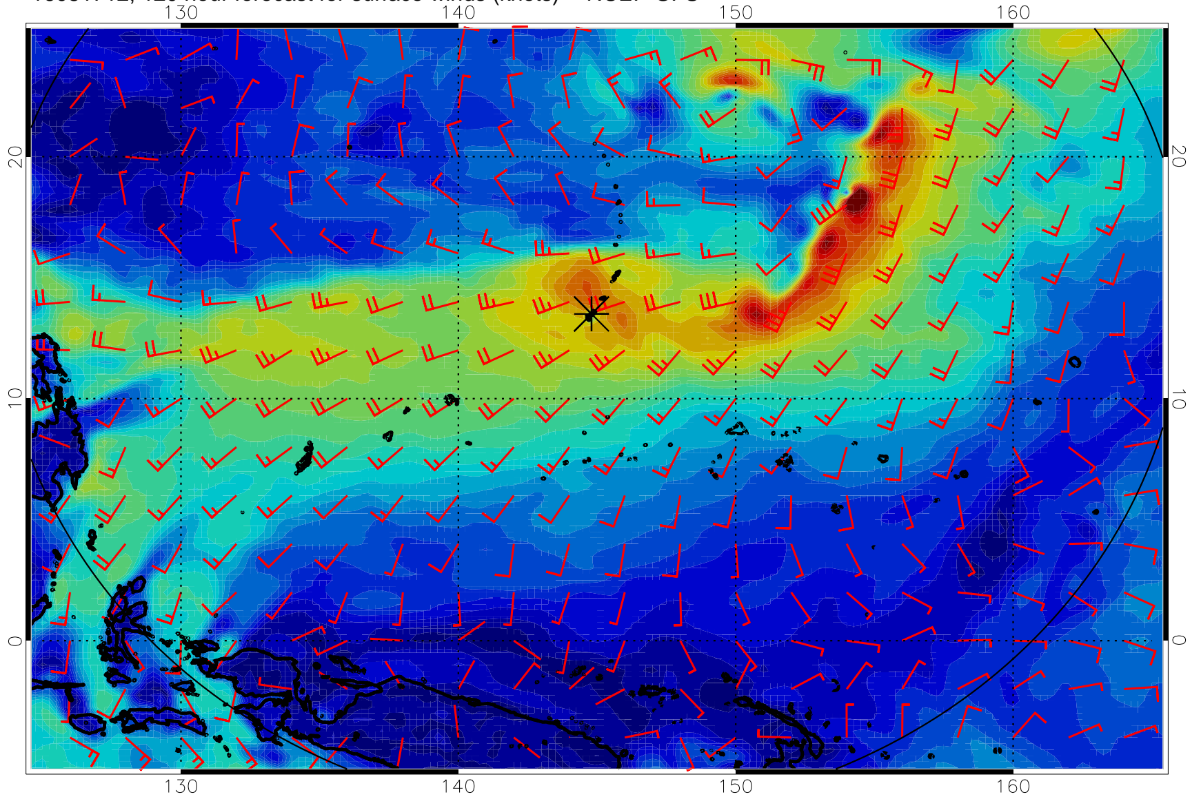
16081712, 120 hour forecast for surface winds (knots) -- NCEP GFS
