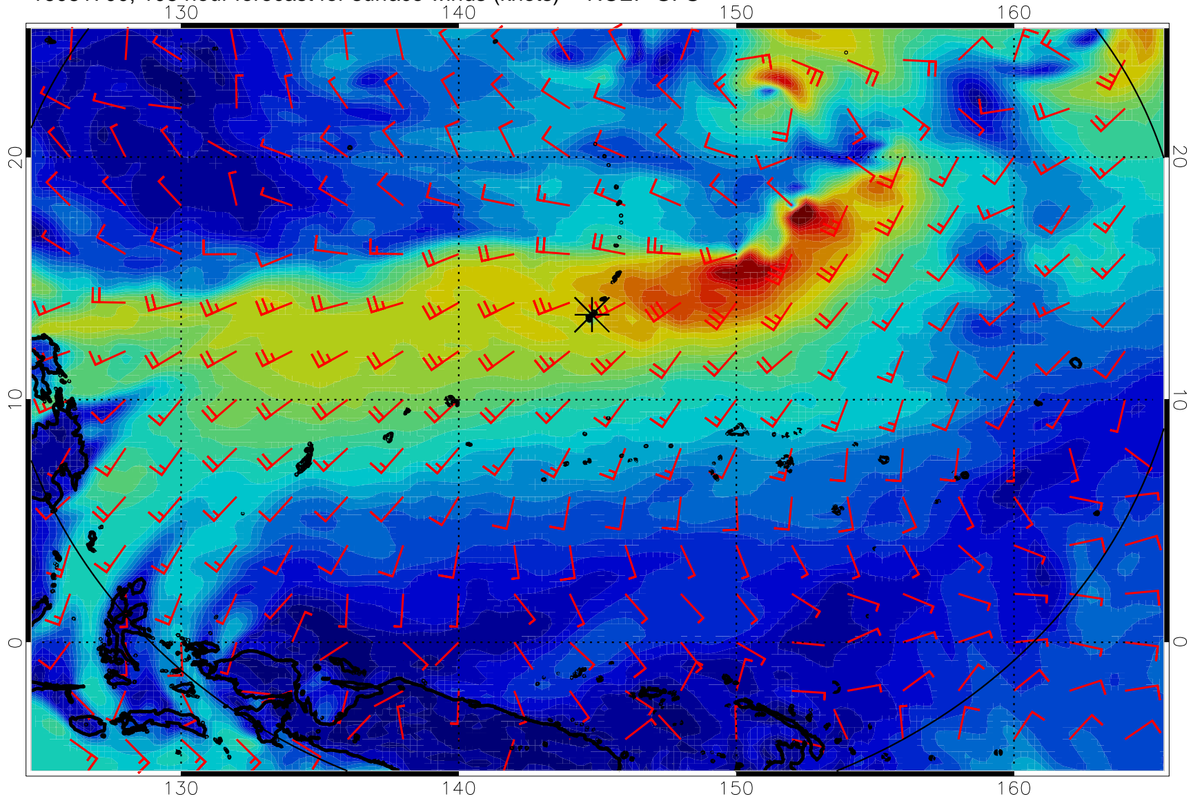
16081700, 108 hour forecast for surface winds (knots) -- NCEP GFS
