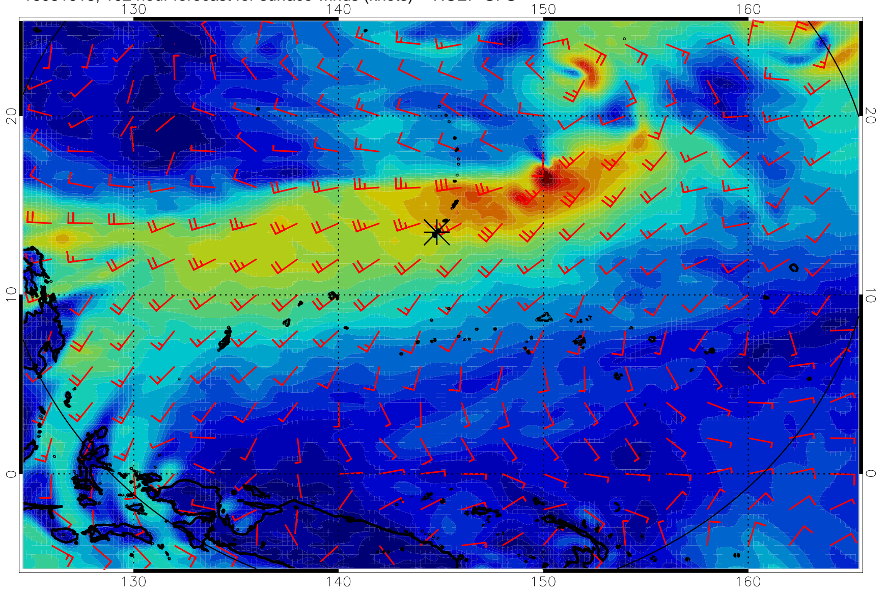
16081618, 102 hour forecast for surface winds (knots) -- NCEP GFS
