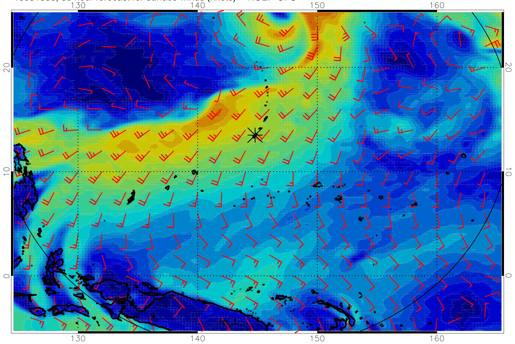
16081500, 60 hour forecast for surface winds (knots) -- NCEP GFS
