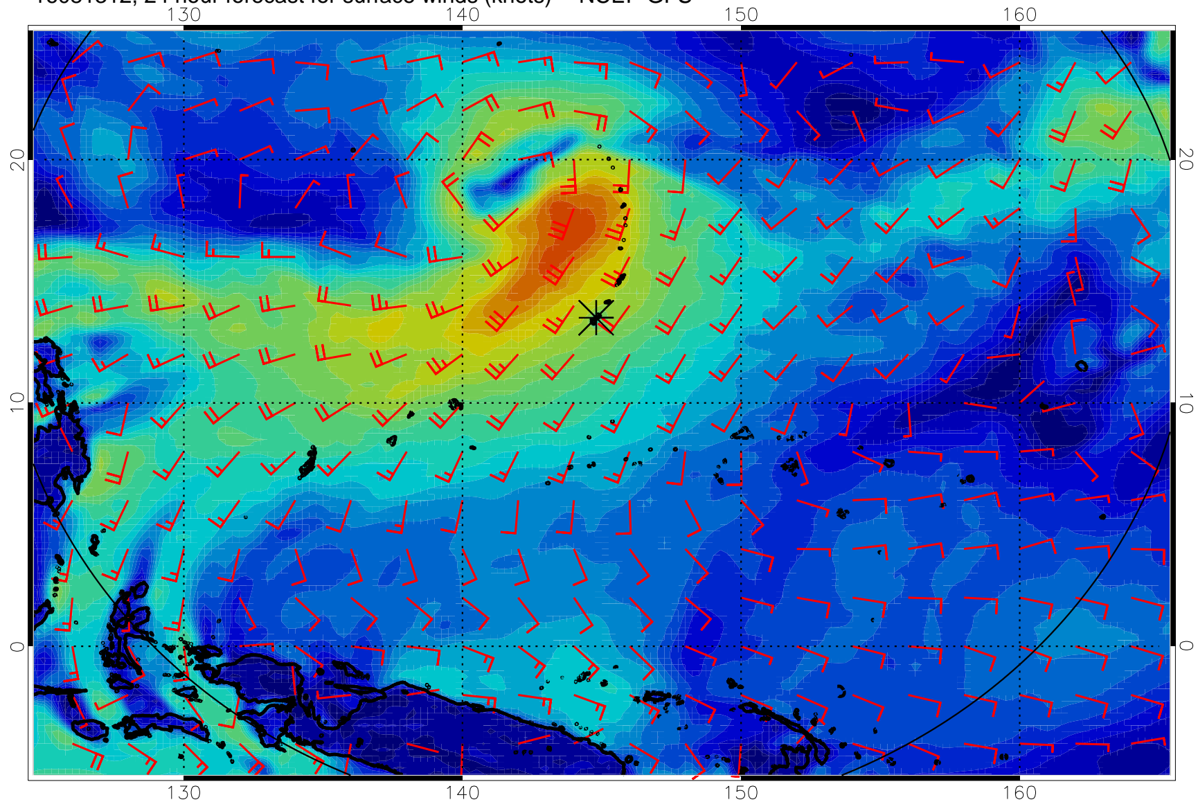
16081312, 24 hour forecast for surface winds (knots) -- NCEP GFS
