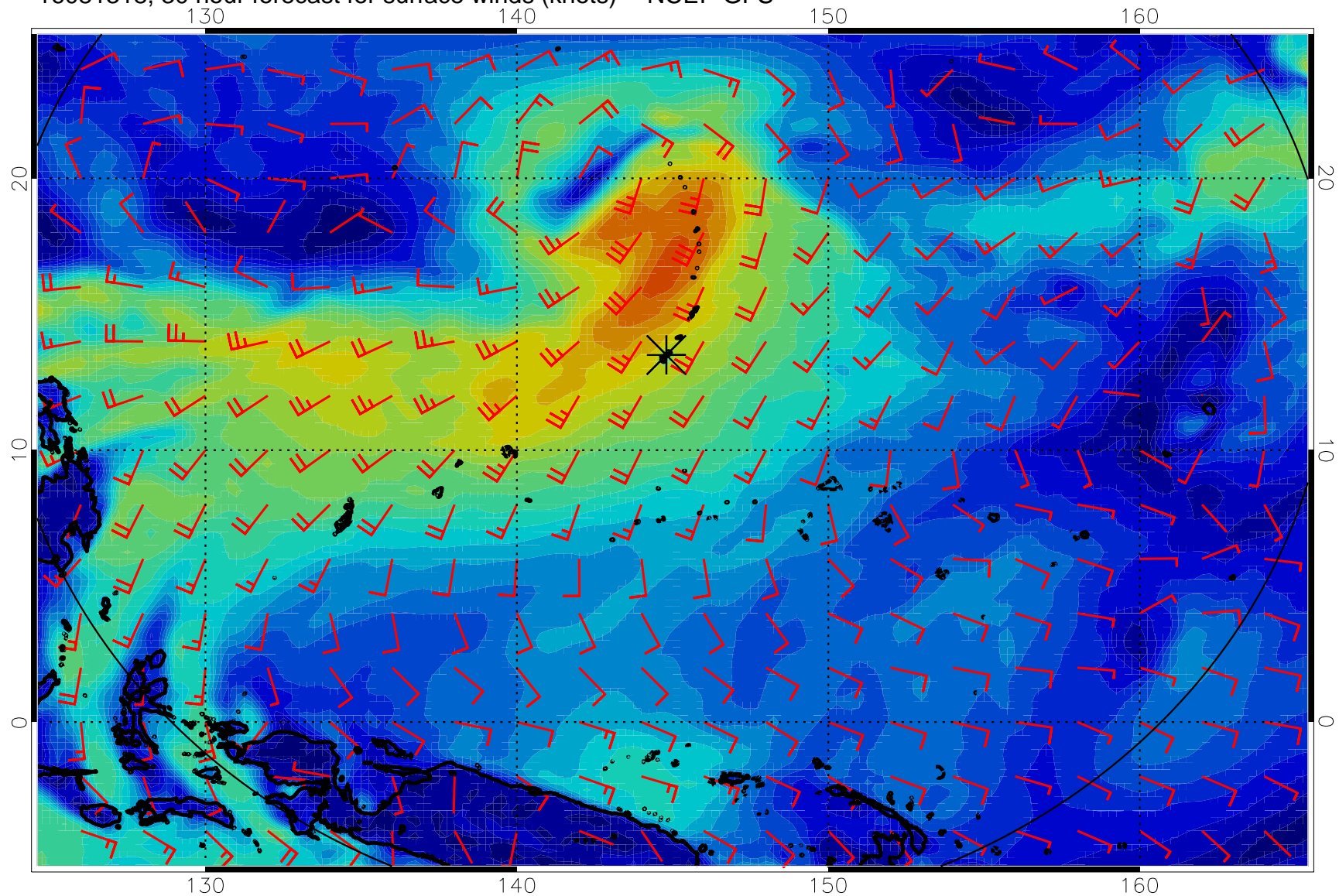
16081318, 30 hour forecast for surface winds (knots) -- NCEP GFS
