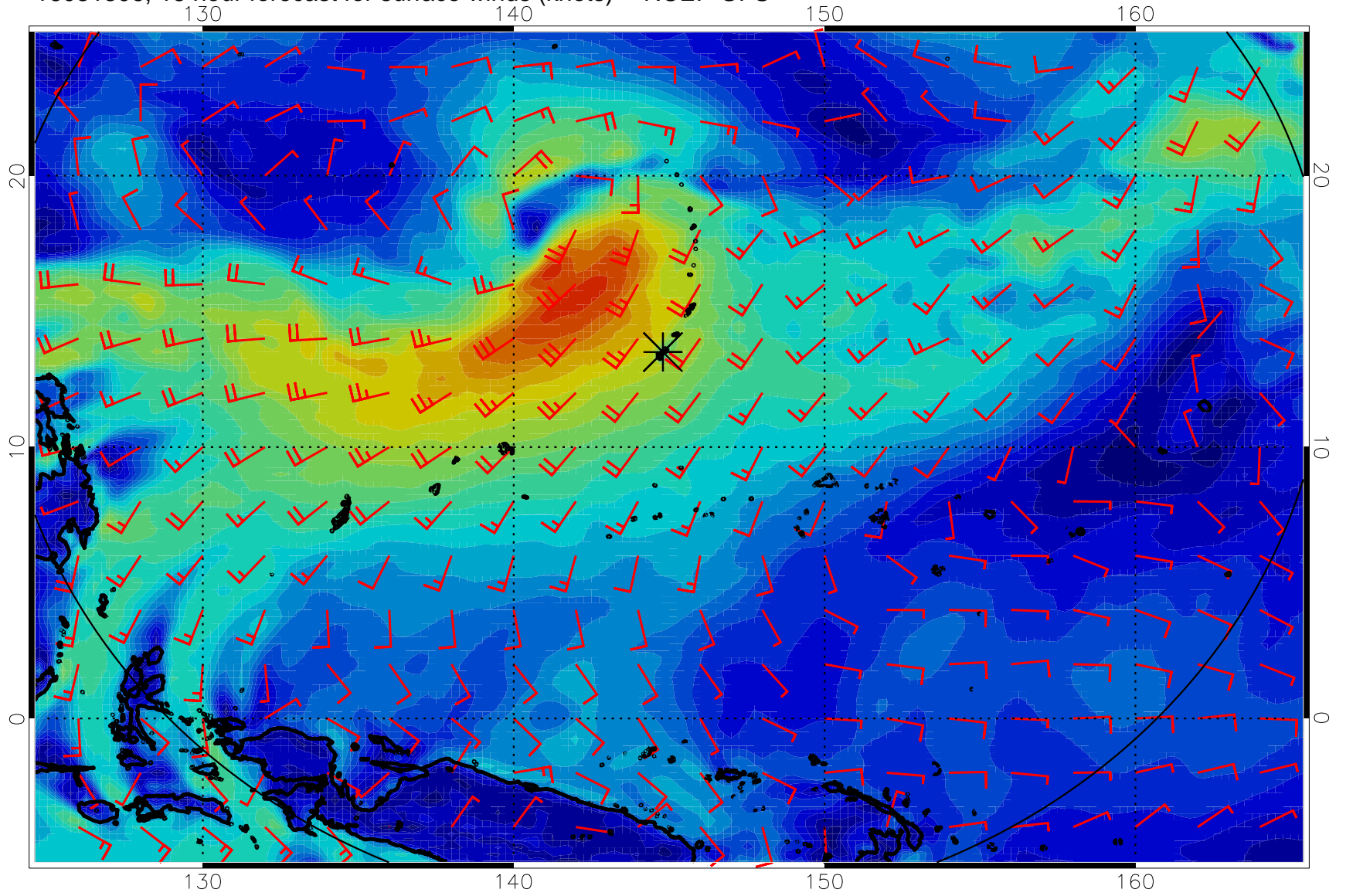
16081306, 18 hour forecast for surface winds (knots) -- NCEP GFS
