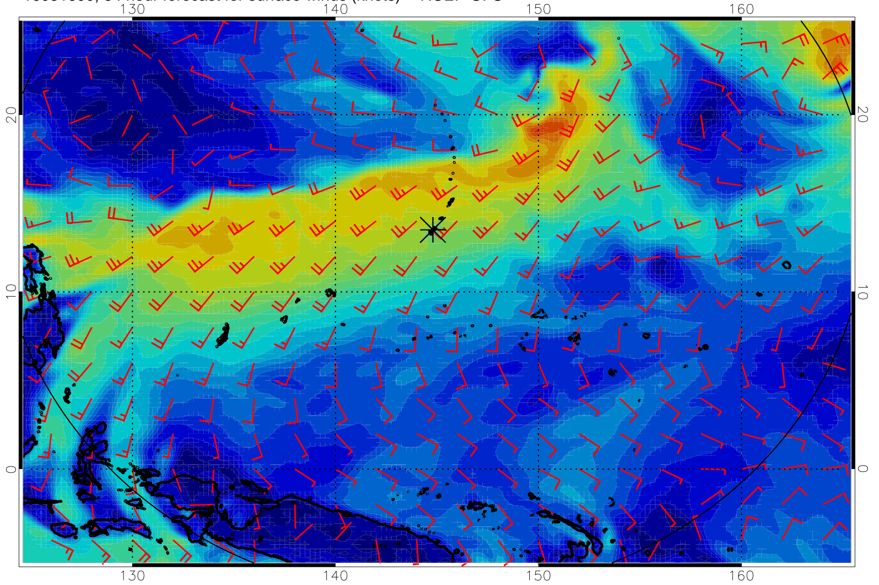
16081600, 84 hour forecast for surface winds (knots) -- NCEP GFS
