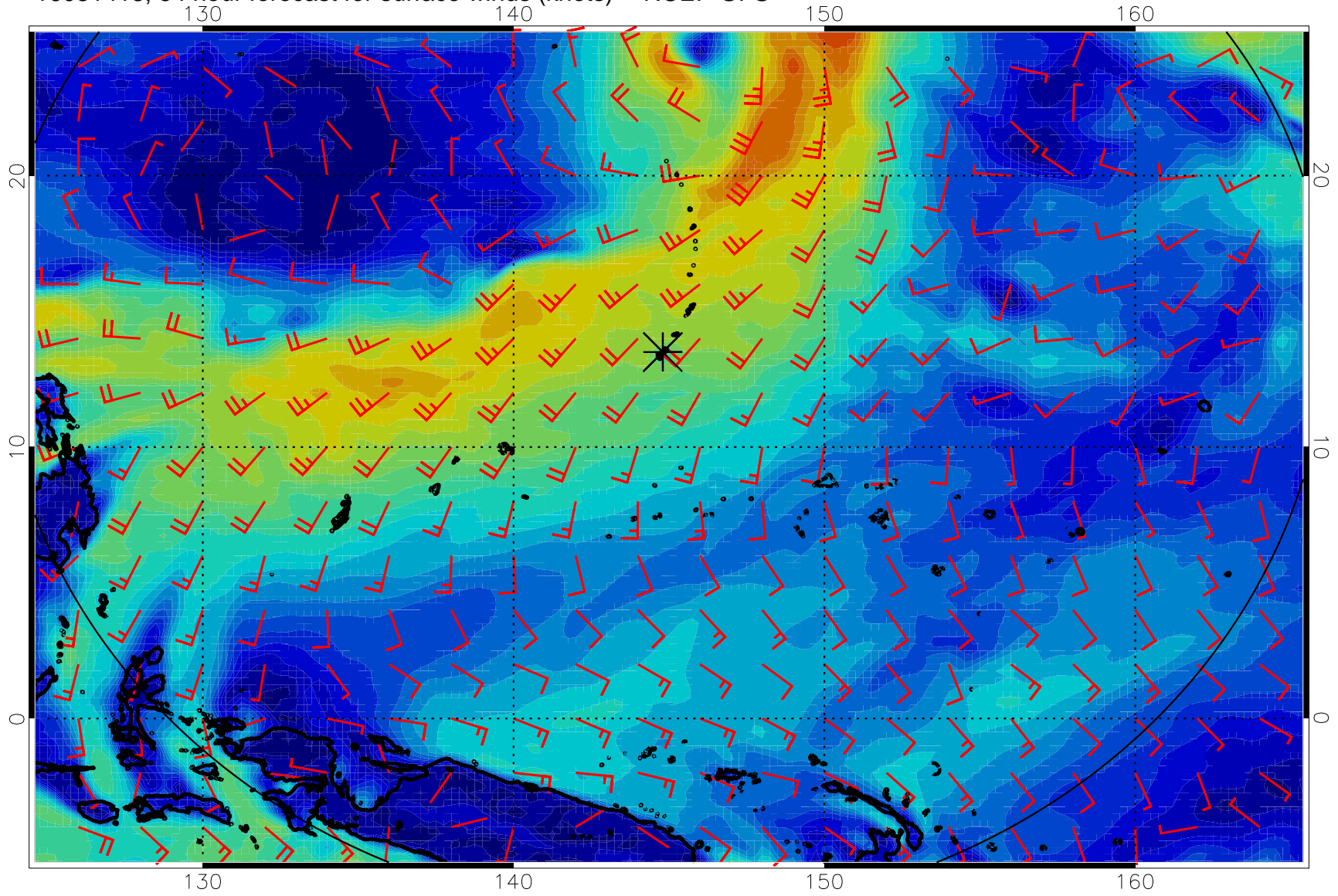
16081418, 54 hour forecast for surface winds (knots) -- NCEP GFS
