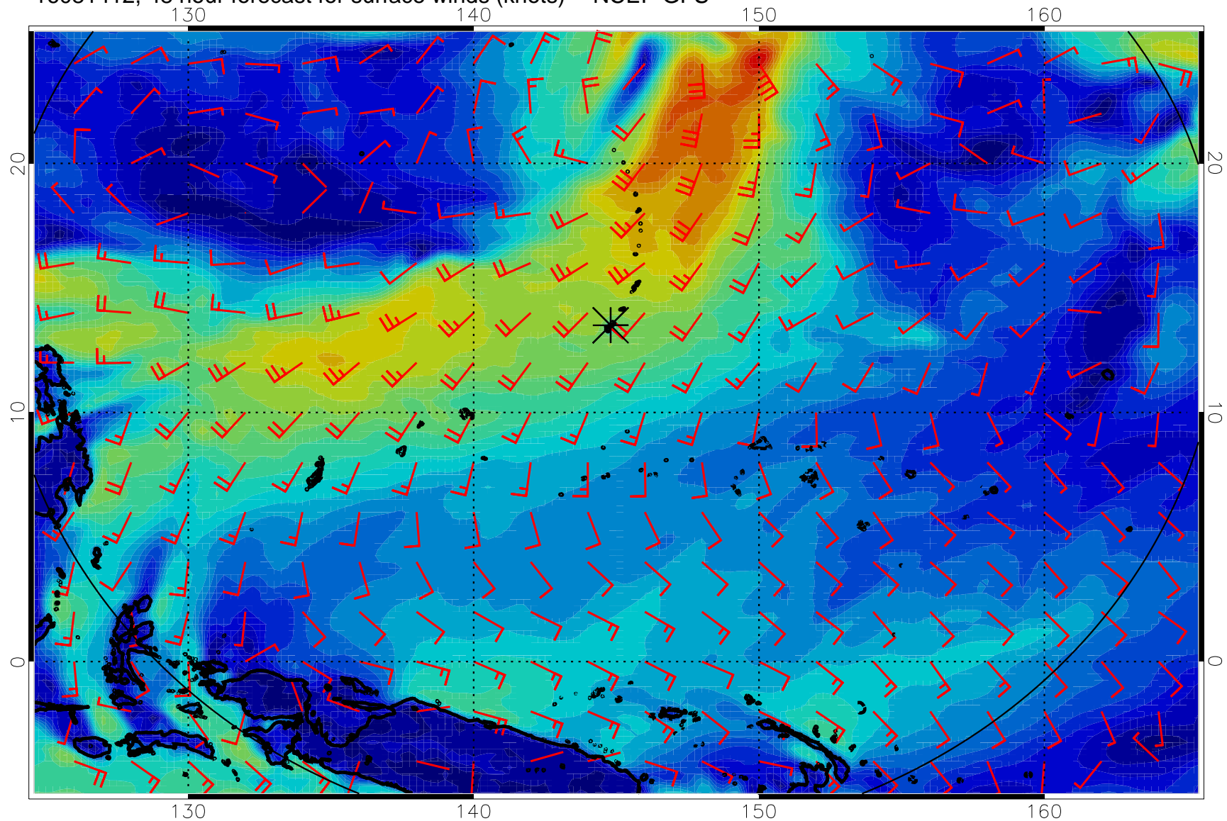
16081412, 48 hour forecast for surface winds (knots) -- NCEP GFS
