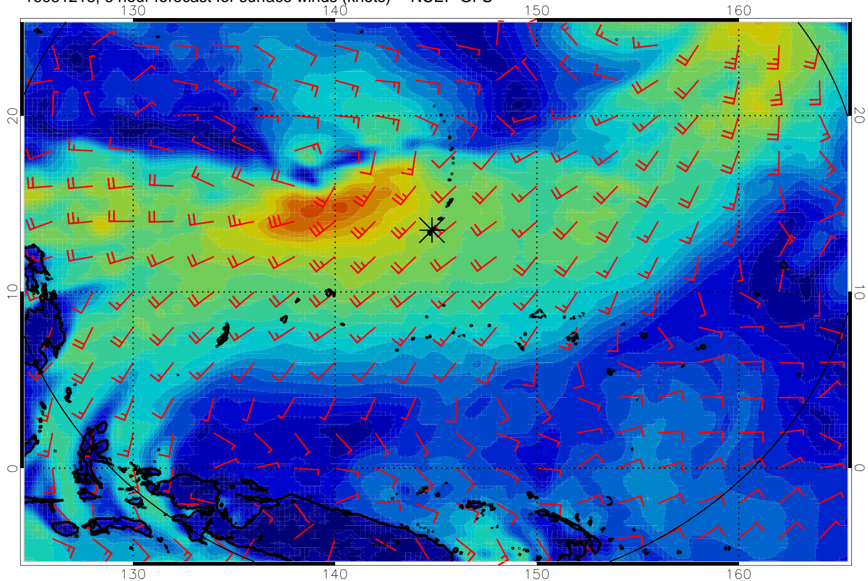
16081218, 6 hour forecast for surface winds (knots) -- NCEP GFS
