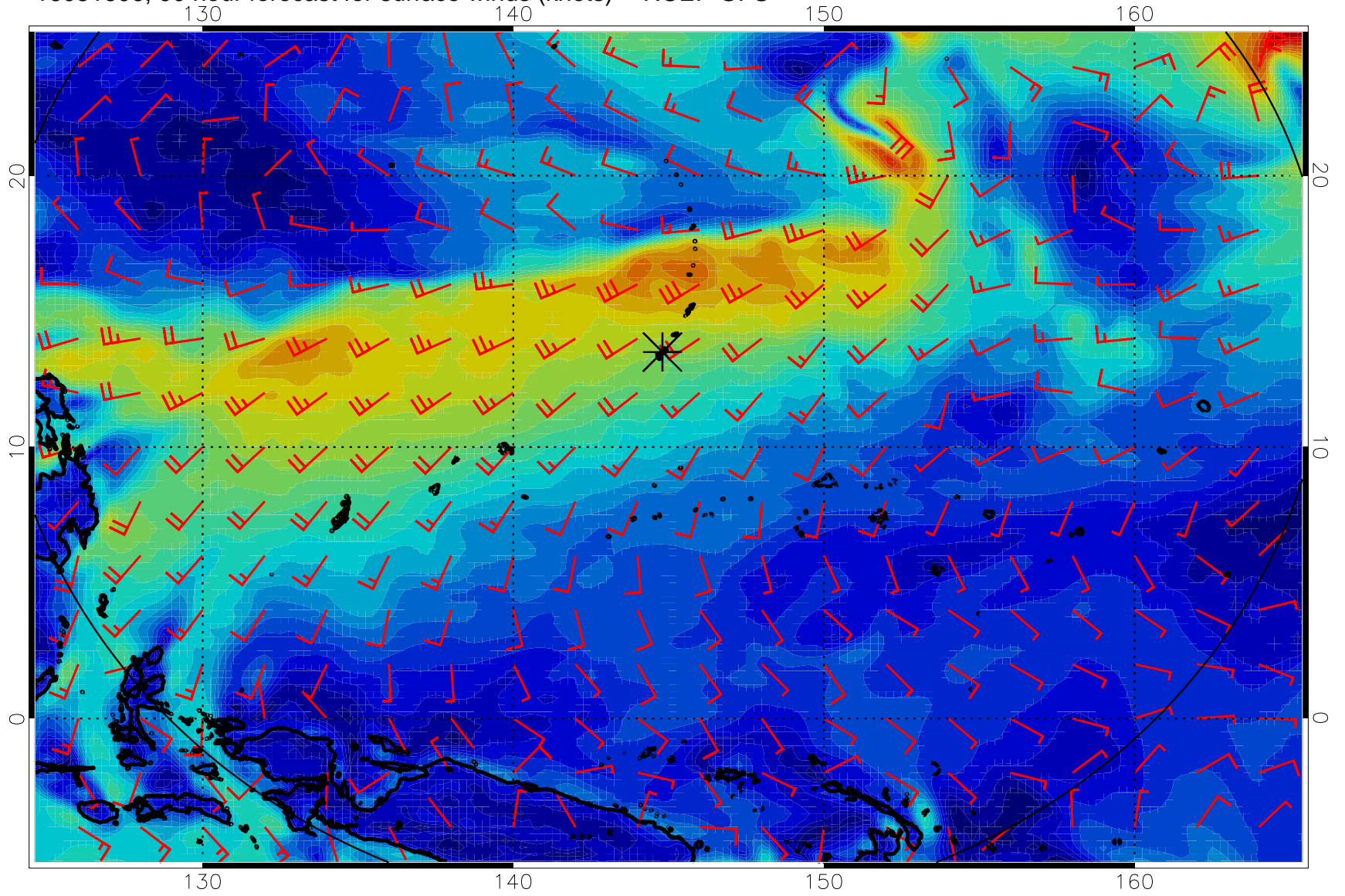
16081606, 90 hour forecast for surface winds (knots) -- NCEP GFS
