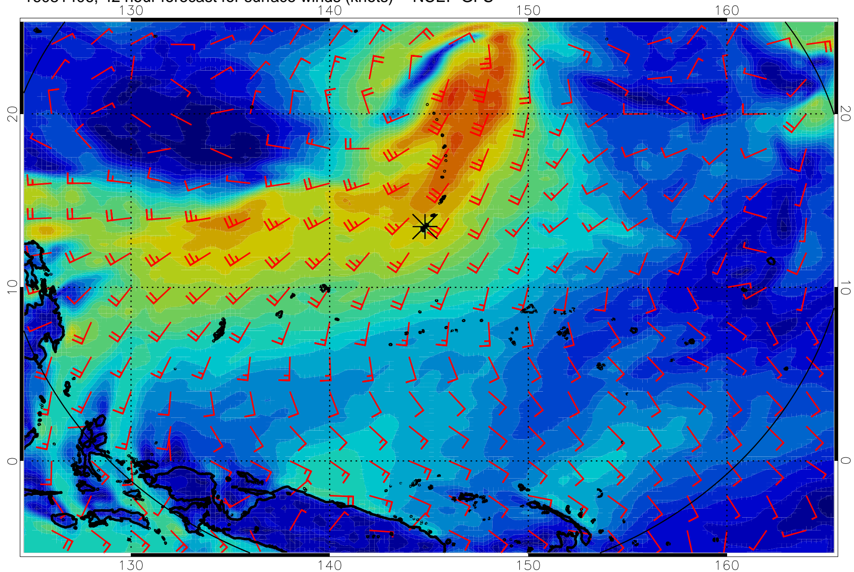
16081406, 42 hour forecast for surface winds (knots) -- NCEP GFS
