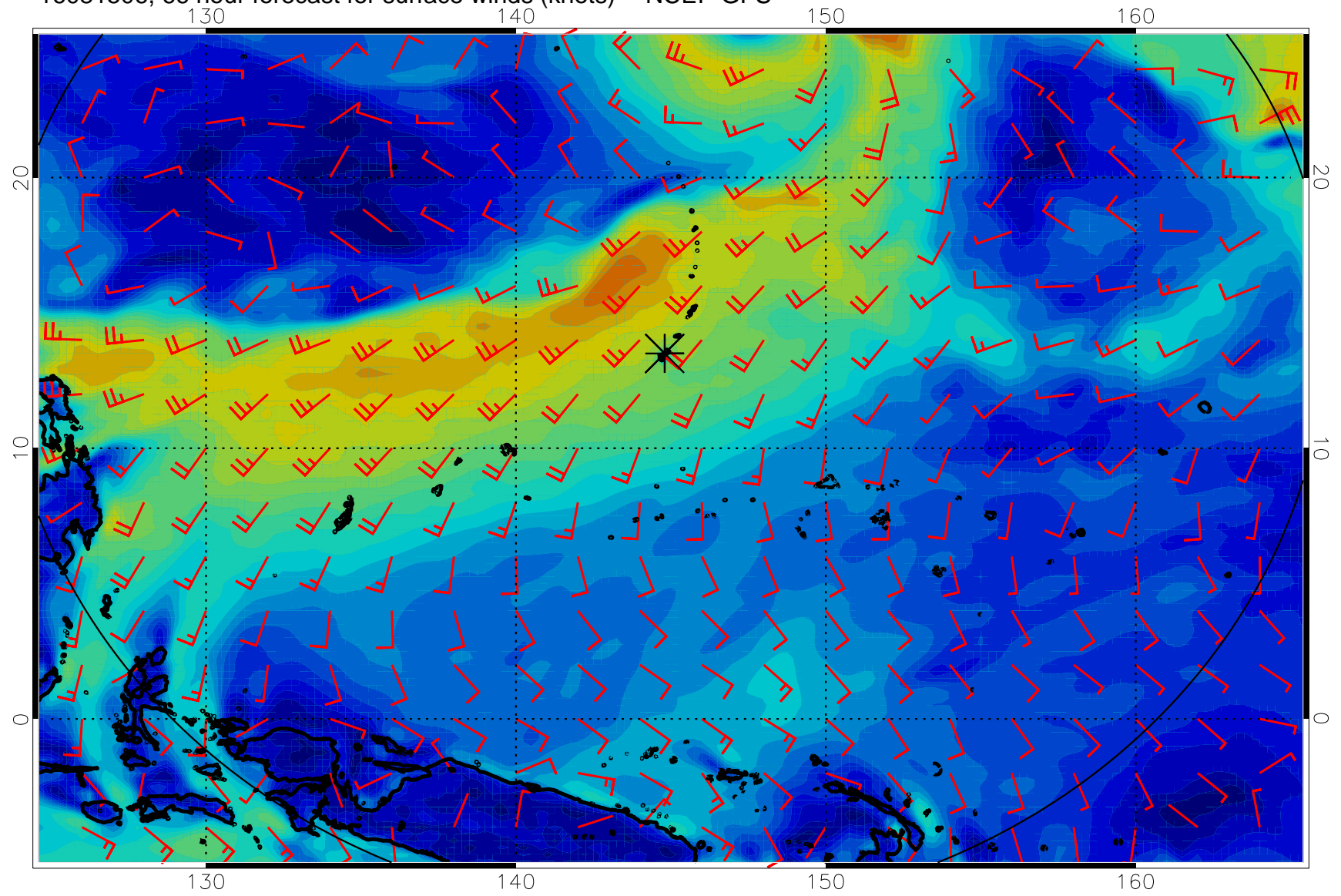
16081506, 66 hour forecast for surface winds (knots) -- NCEP GFS
