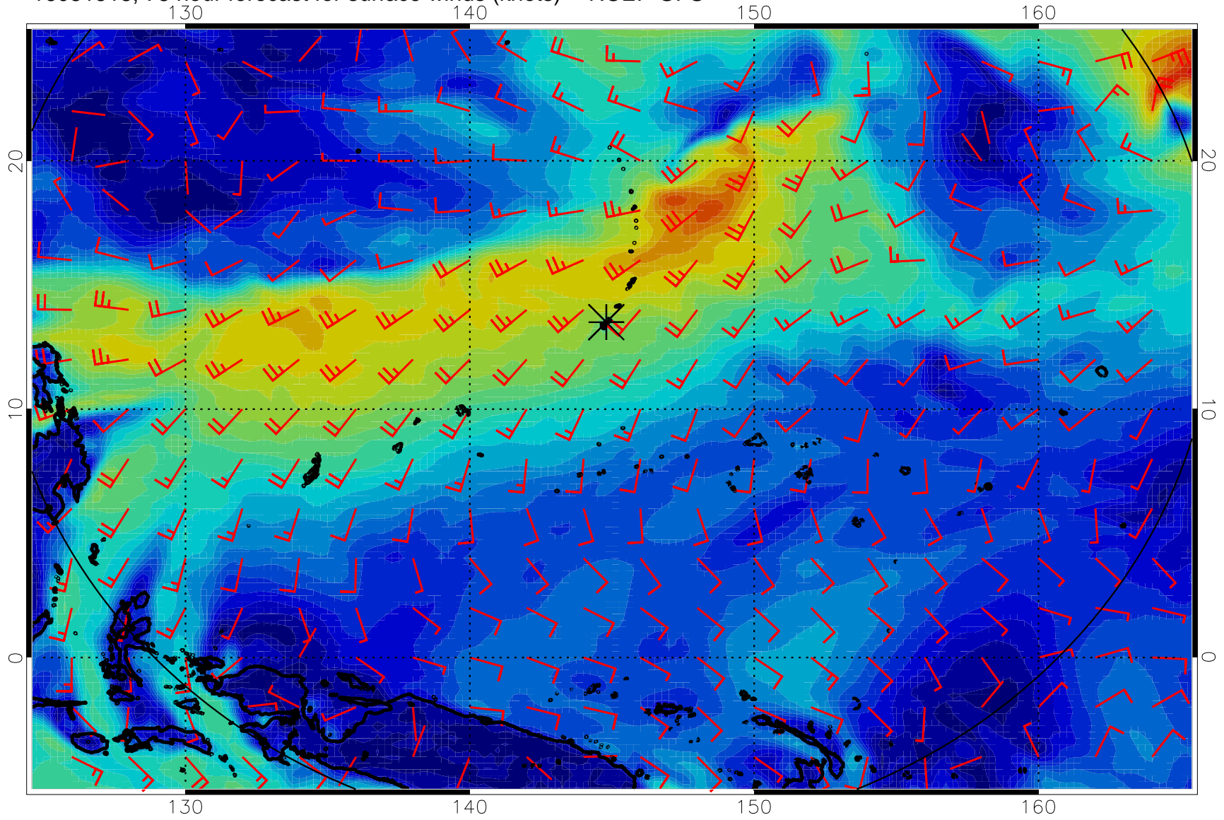
16081518, 78 hour forecast for surface winds (knots) -- NCEP GFS
