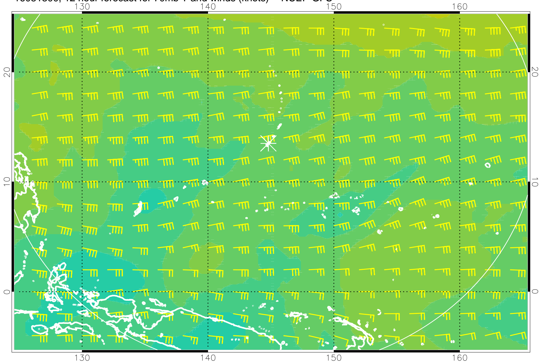
16081300, 12 hour forecast for 70mb T and winds (knots) -- NCEP GFS
