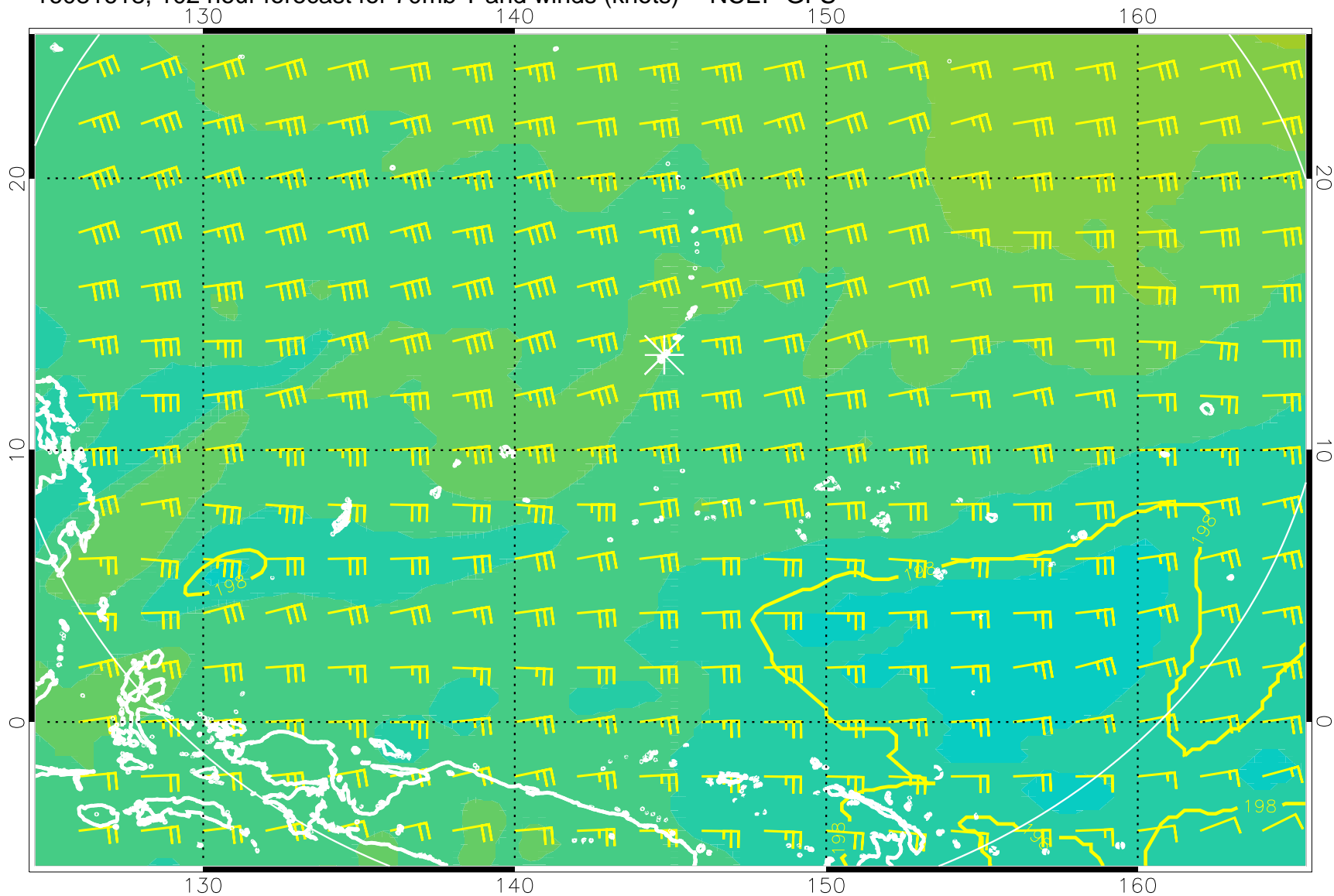
16081618, 102 hour forecast for 70mb T and winds (knots) -- NCEP GFS
