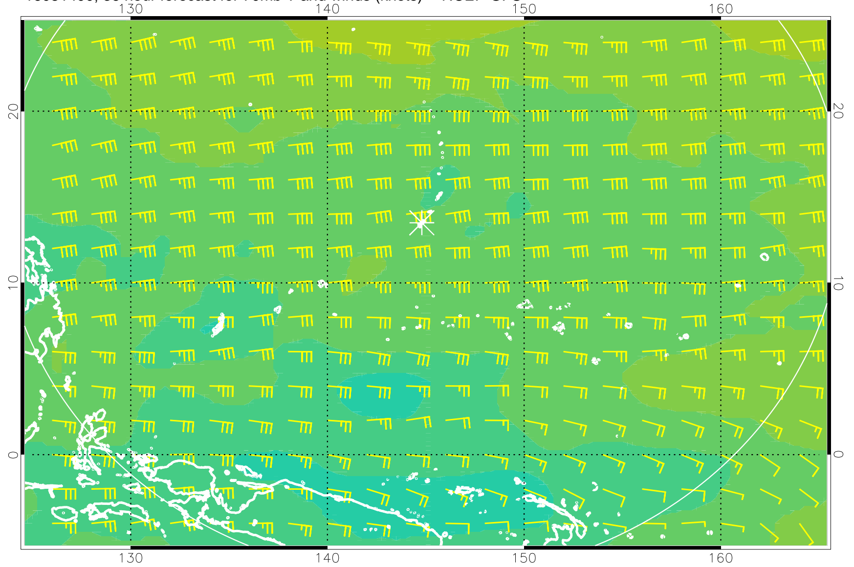
16081400, 36 hour forecast for 70mb T and winds (knots) -- NCEP GFS
