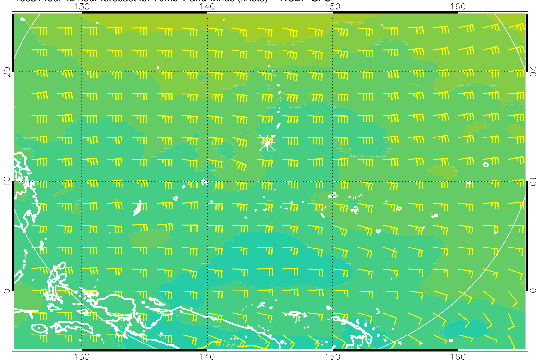
16081406, 42 hour forecast for 70mb T and winds (knots) -- NCEP GFS
