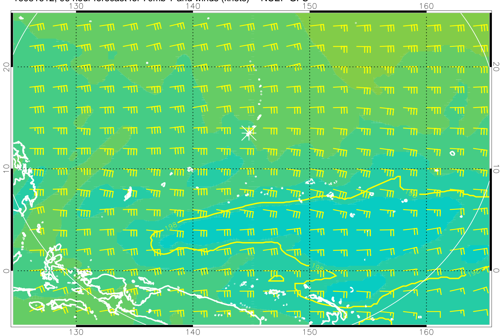
16081612, 96 hour forecast for 70mb T and winds (knots) -- NCEP GFS
