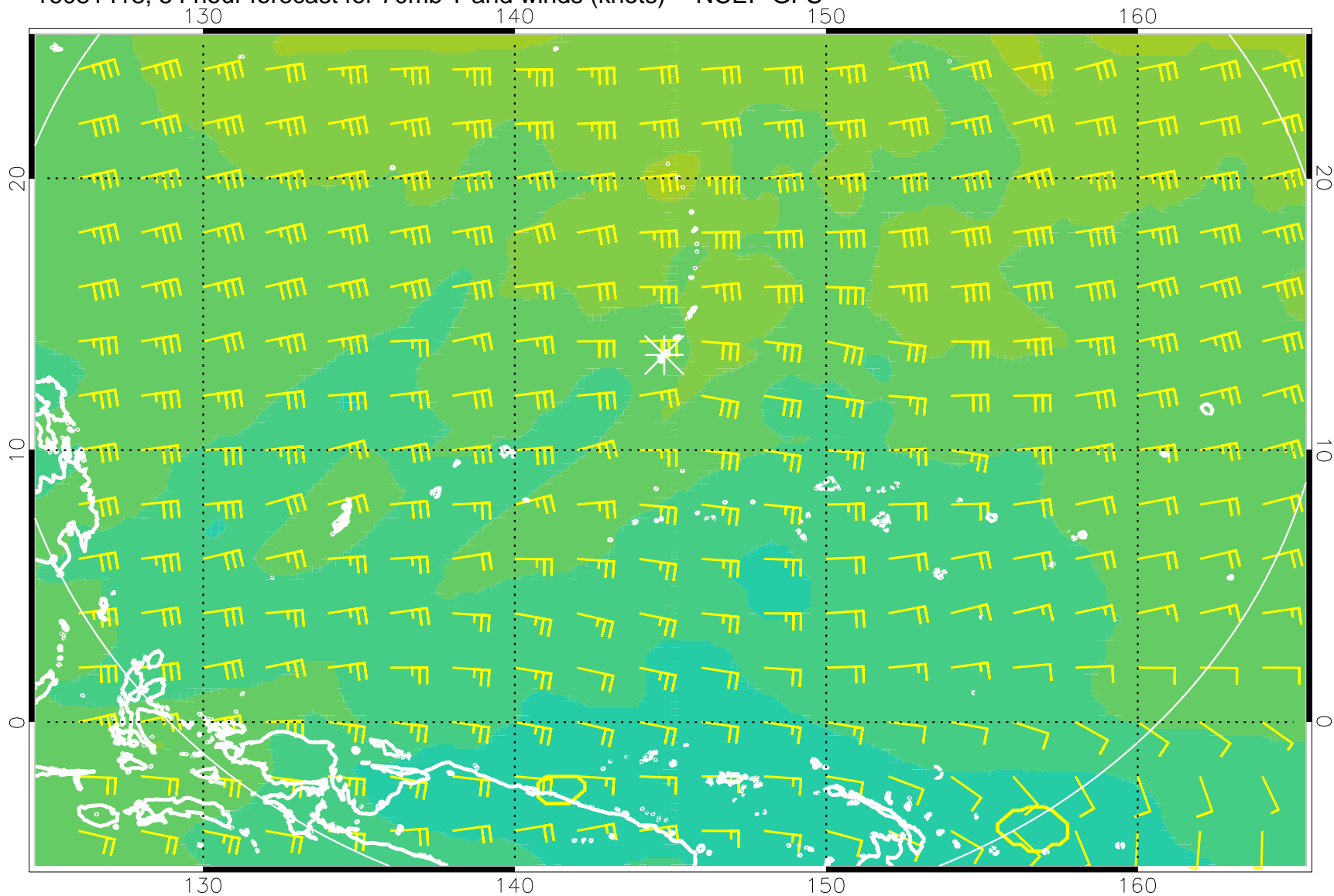
16081418, 54 hour forecast for 70mb T and winds (knots) -- NCEP GFS
