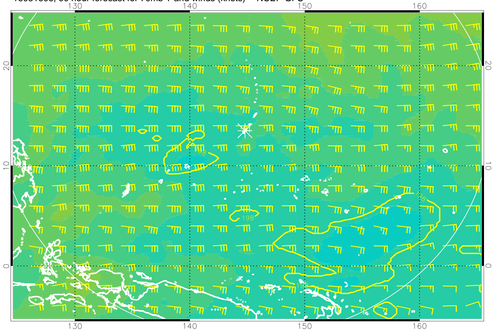
16081606, 90 hour forecast for 70mb T and winds (knots) -- NCEP GFS
