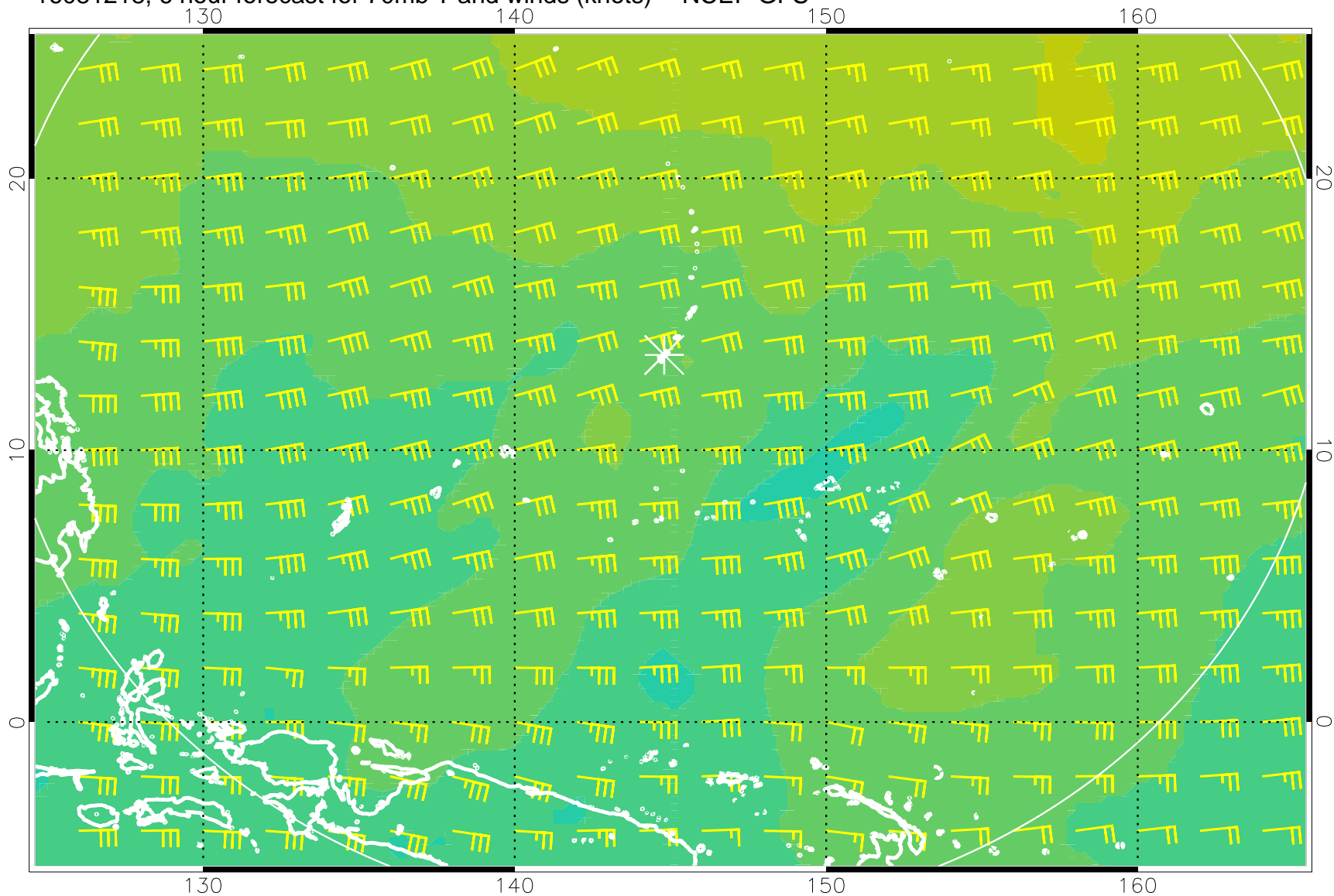
16081218, 6 hour forecast for 70mb T and winds (knots) -- NCEP GFS
