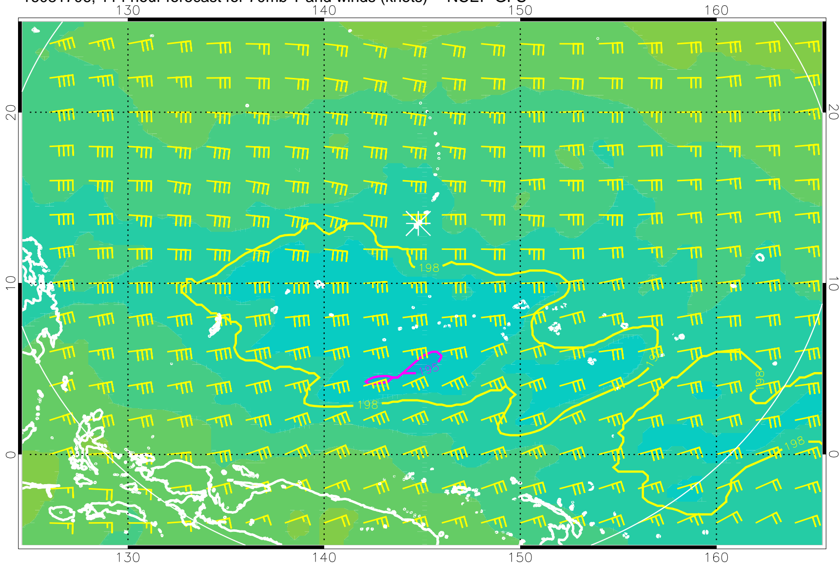
16081706, 114 hour forecast for 70mb T and winds (knots) -- NCEP GFS
