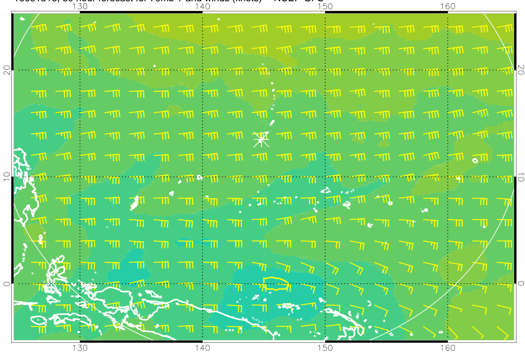
16081318, 30 hour forecast for 70mb T and winds (knots) -- NCEP GFS
