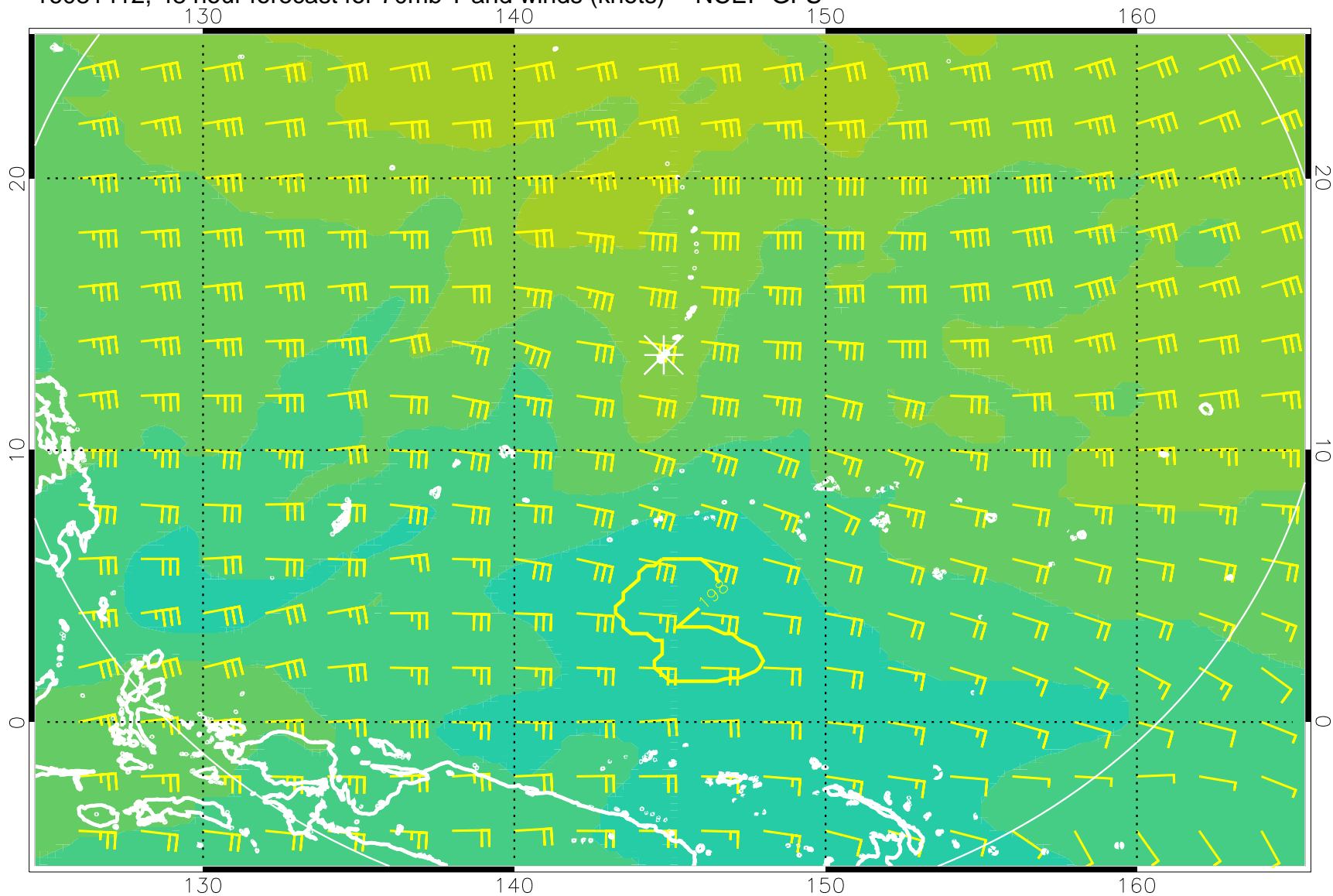
16081412, 48 hour forecast for 70mb T and winds (knots) -- NCEP GFS
