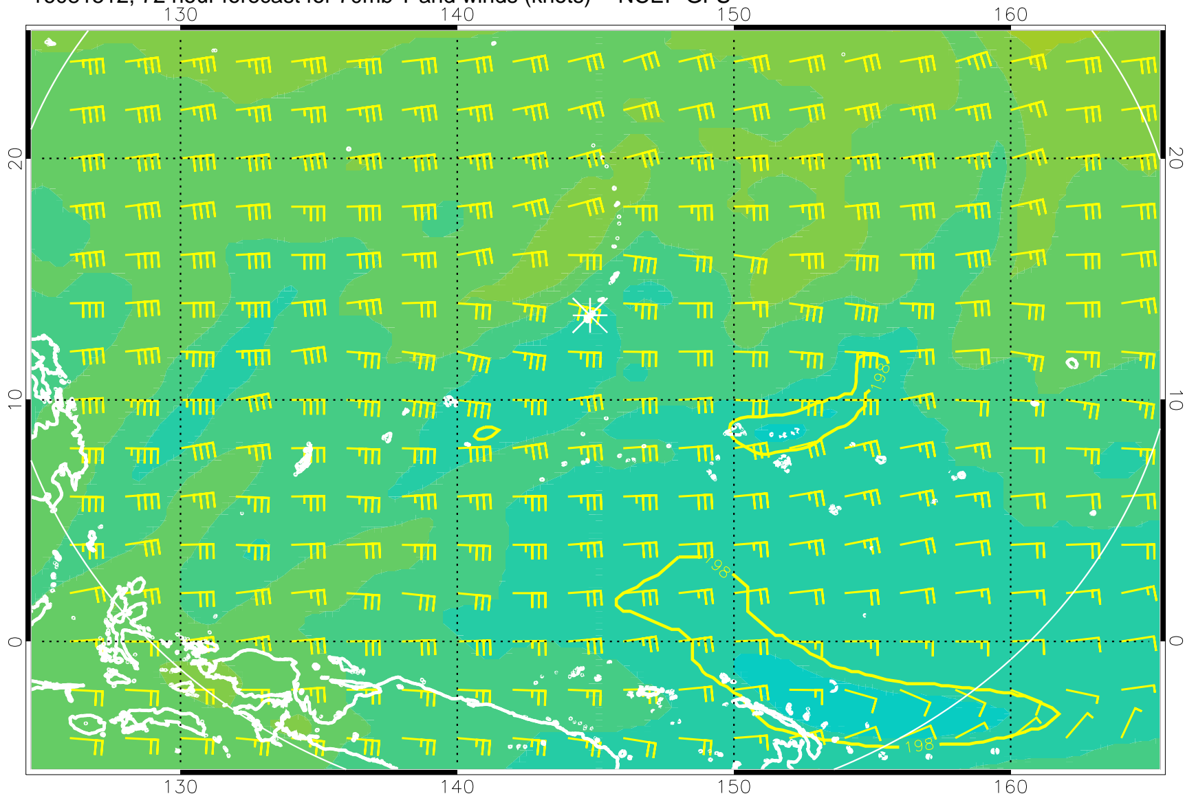
16081512, 72 hour forecast for 70mb T and winds (knots) -- NCEP GFS
