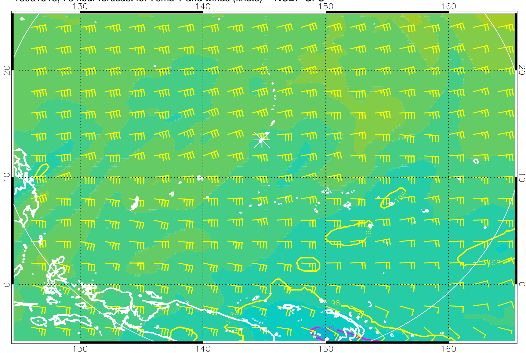
16081518, 78 hour forecast for 70mb T and winds (knots) -- NCEP GFS
