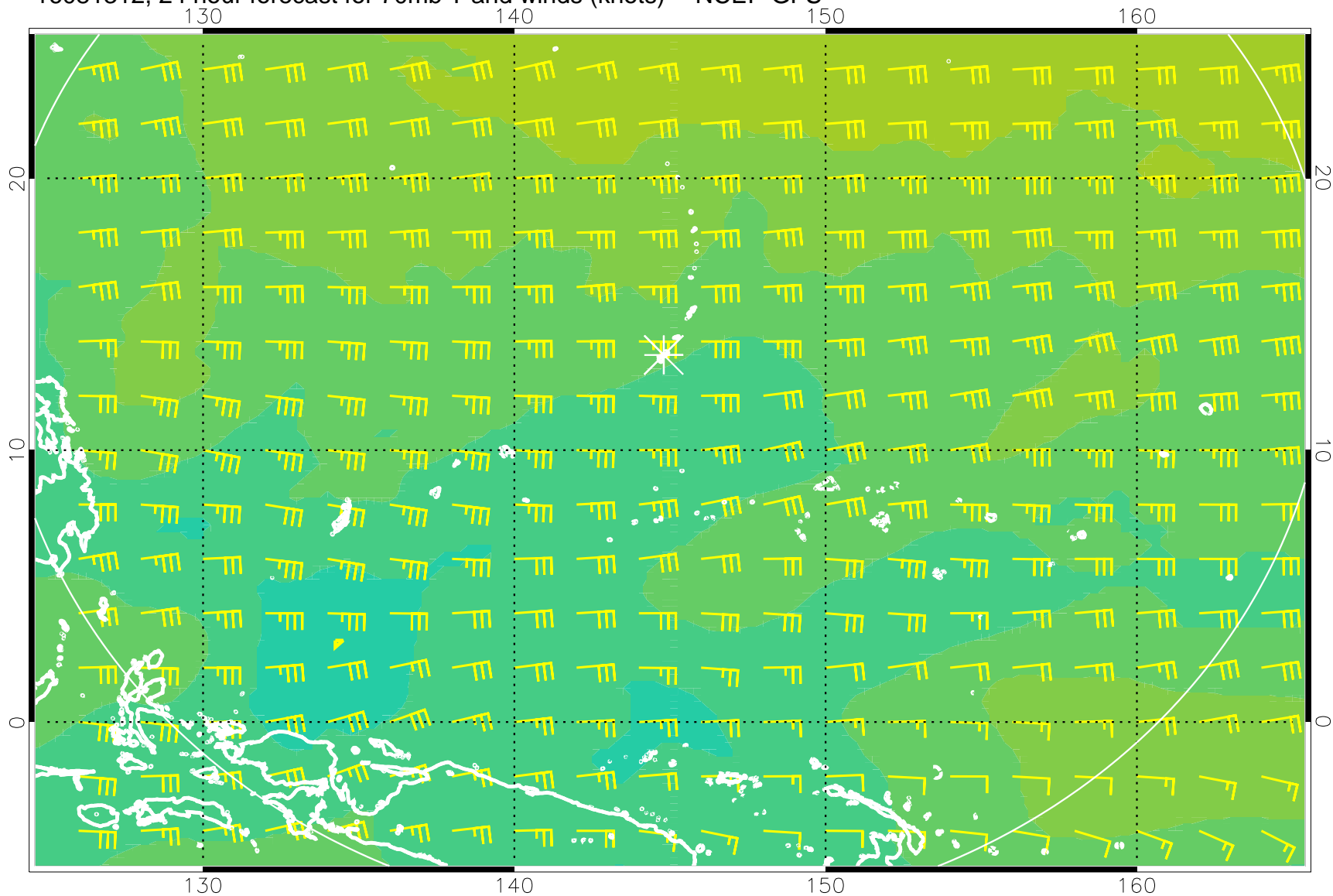
16081312, 24 hour forecast for 70mb T and winds (knots) -- NCEP GFS
