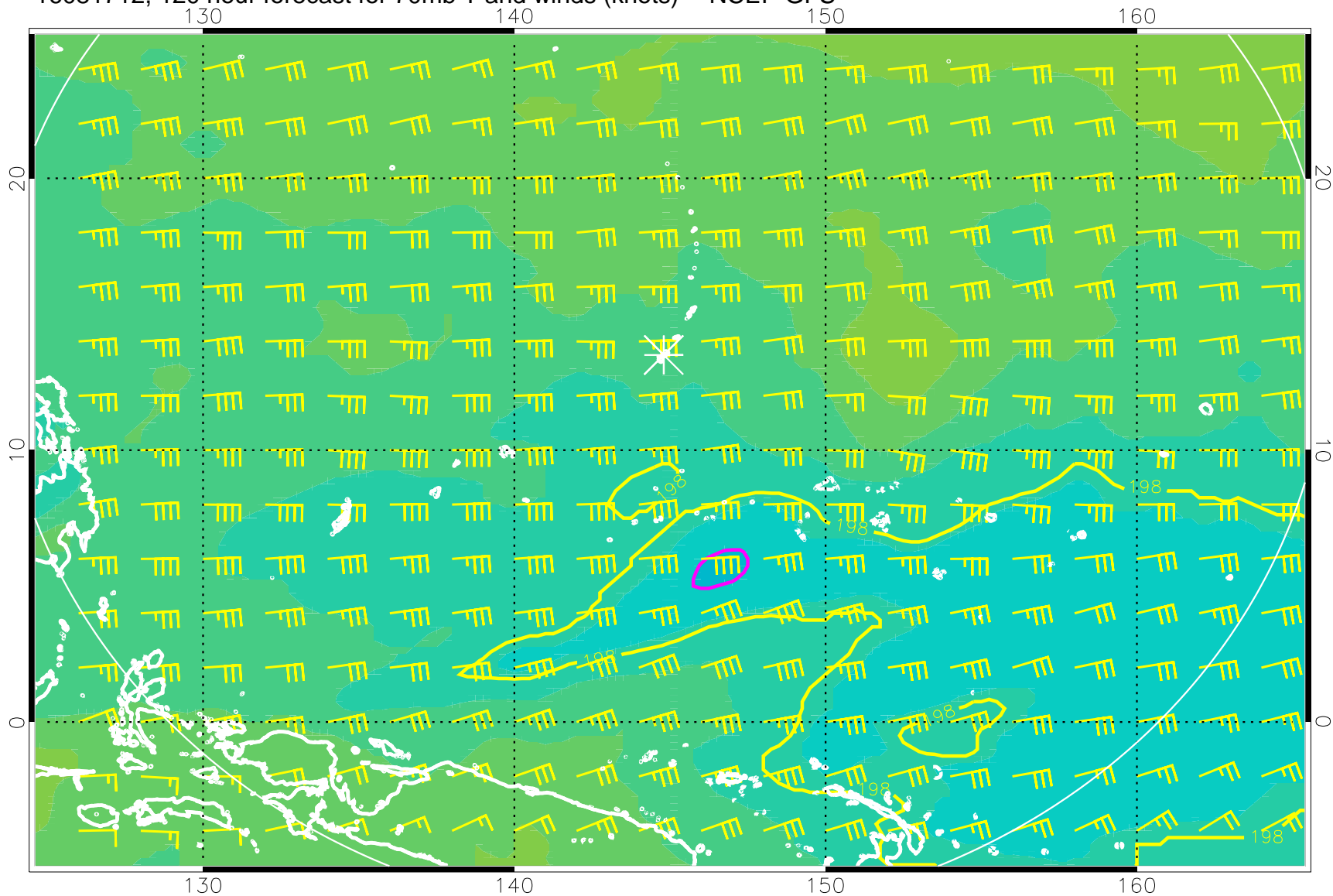
16081712, 120 hour forecast for 70mb T and winds (knots) -- NCEP GFS
