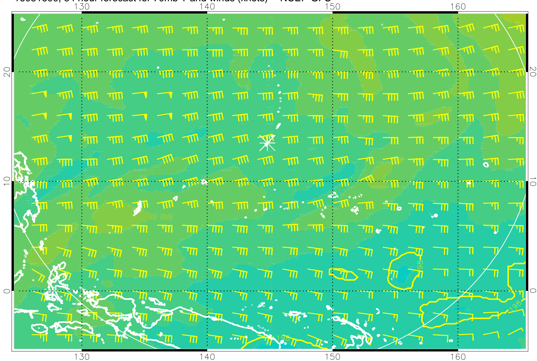
16081600, 84 hour forecast for 70mb T and winds (knots) -- NCEP GFS
