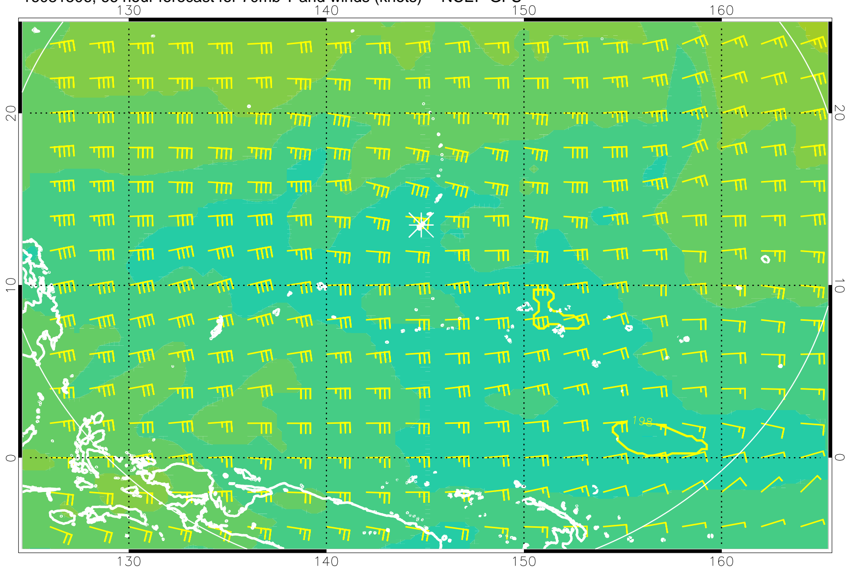
16081506, 66 hour forecast for 70mb T and winds (knots) -- NCEP GFS
