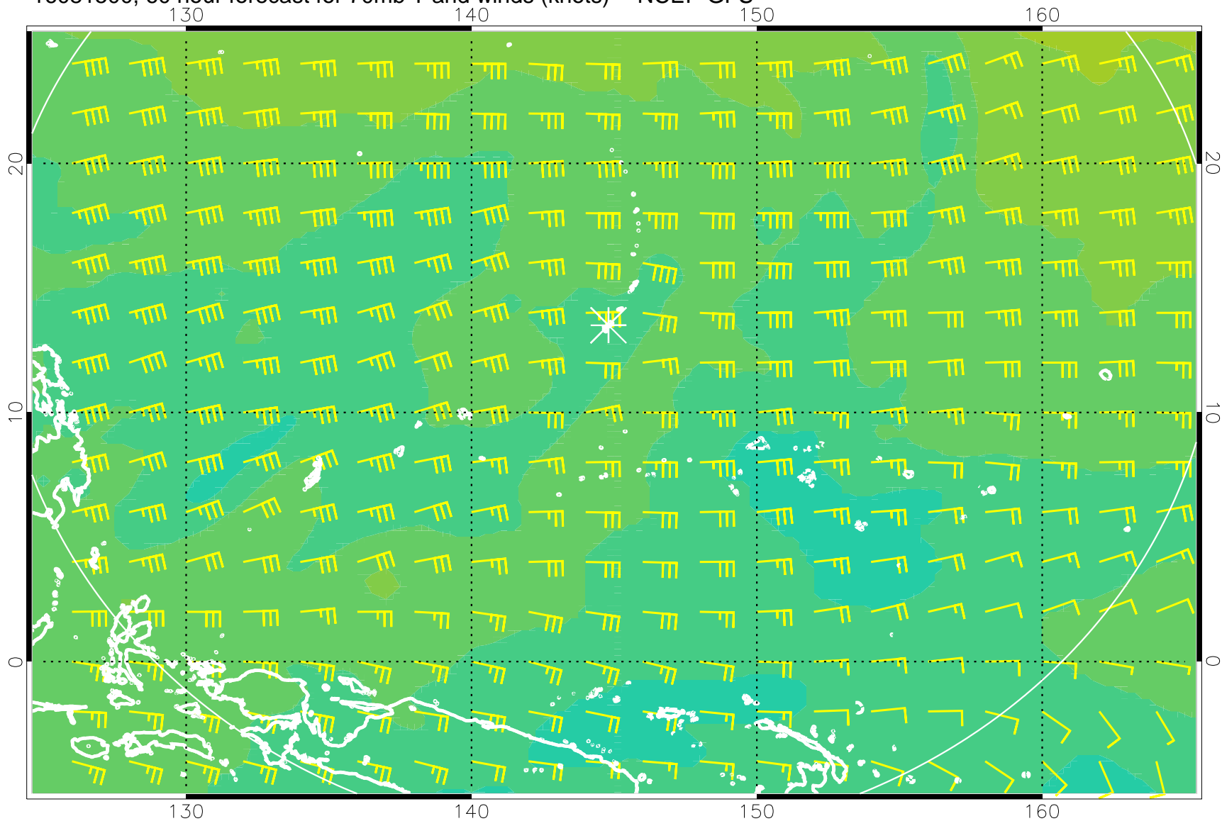
16081500, 60 hour forecast for 70mb T and winds (knots) -- NCEP GFS
