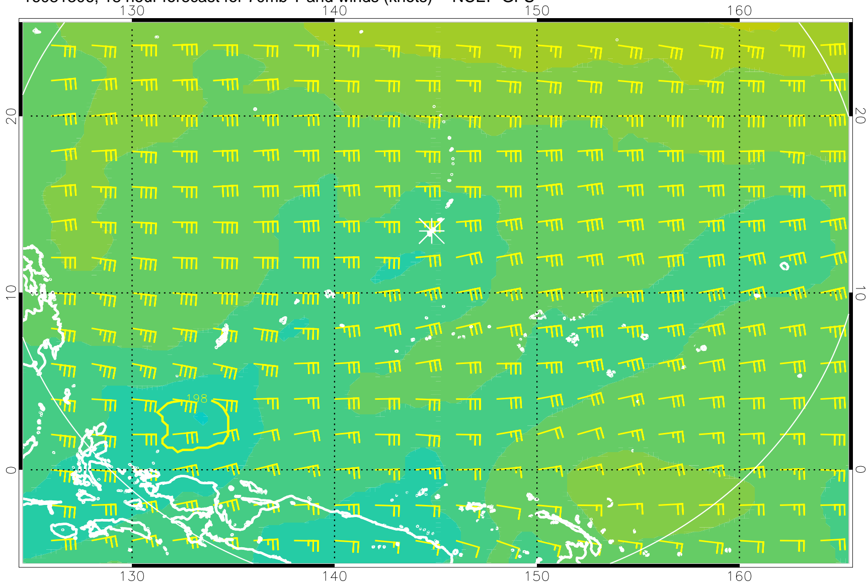
16081306, 18 hour forecast for 70mb T and winds (knots) -- NCEP GFS
