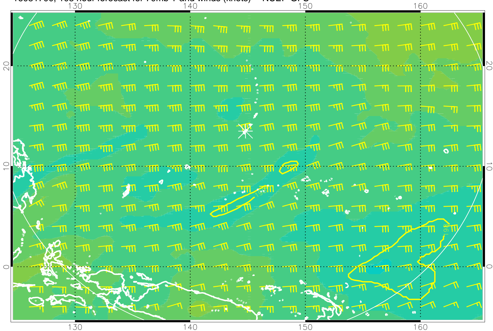
16081700, 108 hour forecast for 70mb T and winds (knots) -- NCEP GFS
