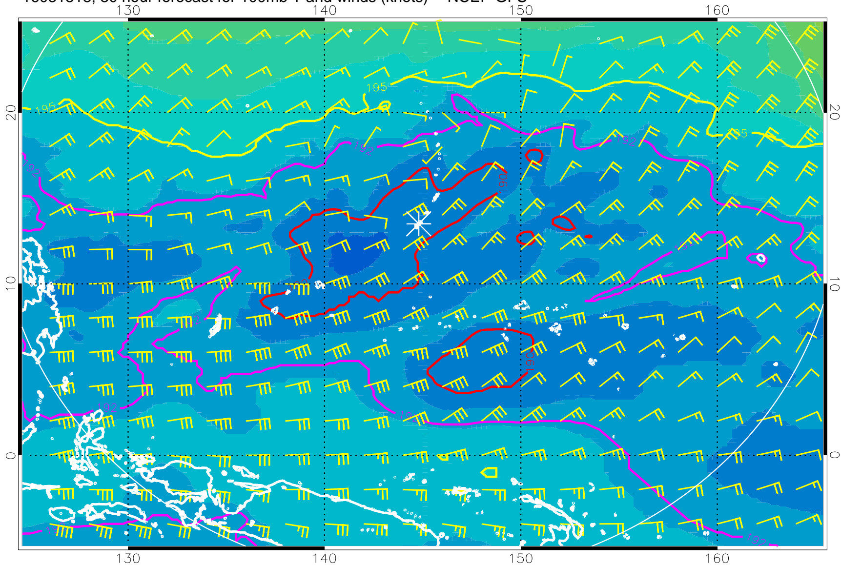
16081318, 30 hour forecast for 100mb T and winds (knots) -- NCEP GFS
