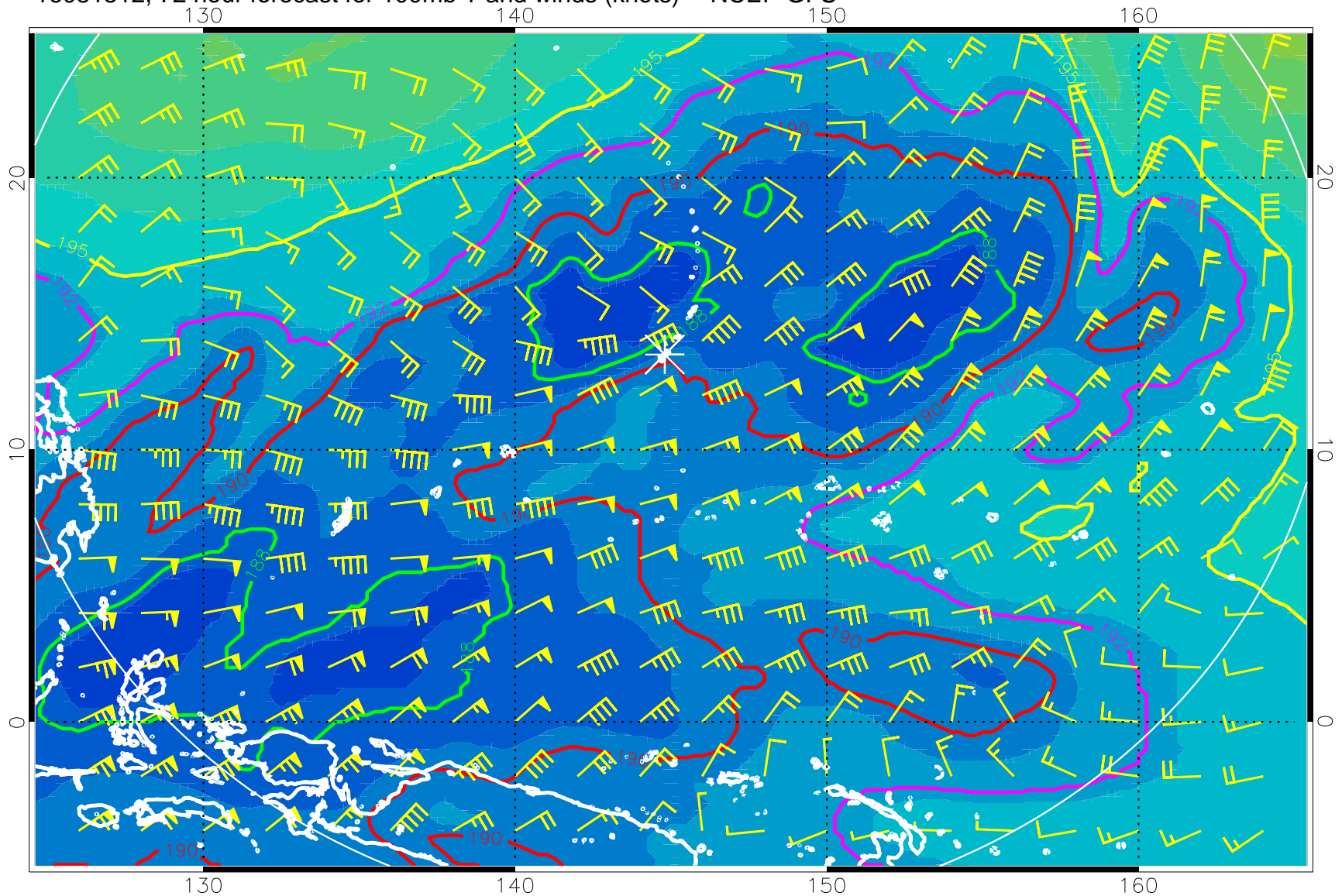
16081512, 72 hour forecast for 100mb T and winds (knots) -- NCEP GFS
