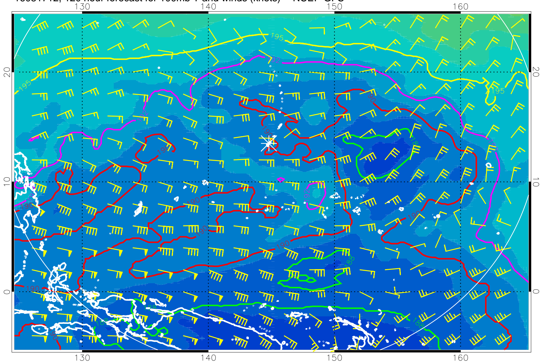
16081712, 120 hour forecast for 100mb T and winds (knots) -- NCEP GFS
