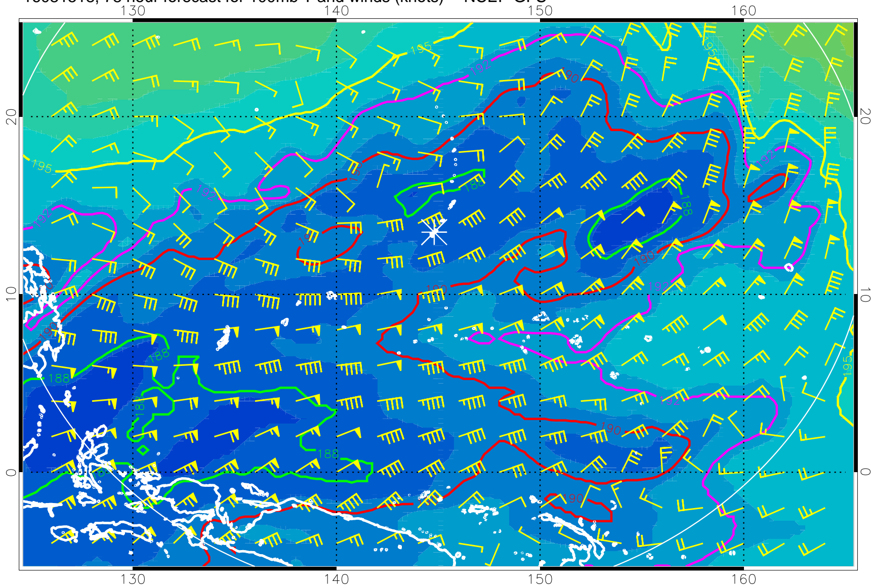
16081518, 78 hour forecast for 100mb T and winds (knots) -- NCEP GFS
