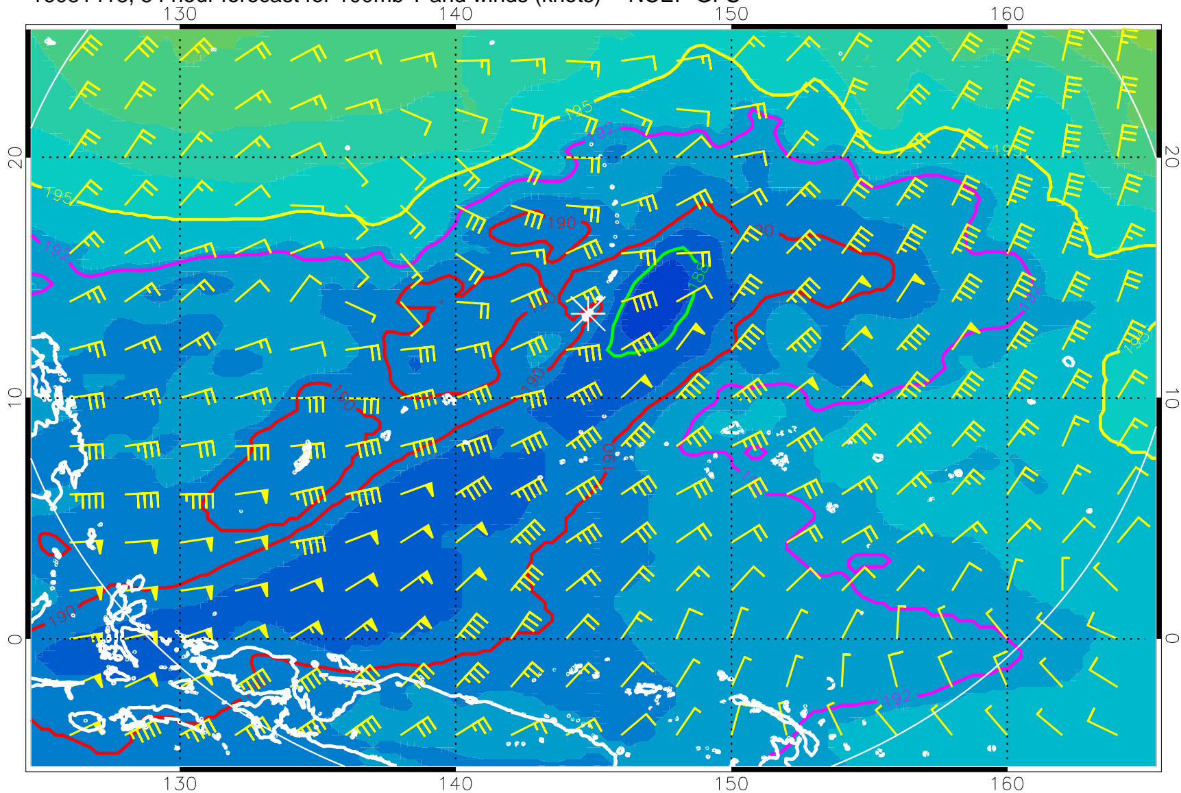
16081418, 54 hour forecast for 100mb T and winds (knots) -- NCEP GFS
