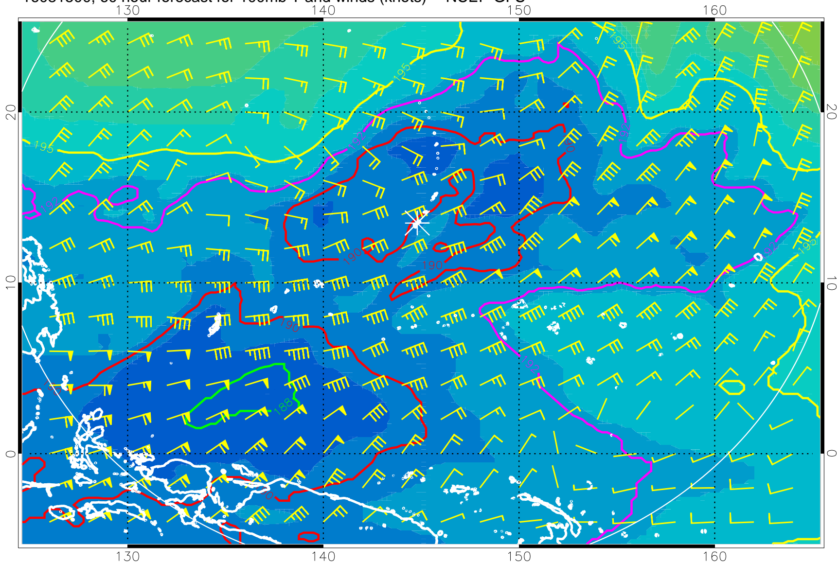
16081500, 60 hour forecast for 100mb T and winds (knots) -- NCEP GFS
