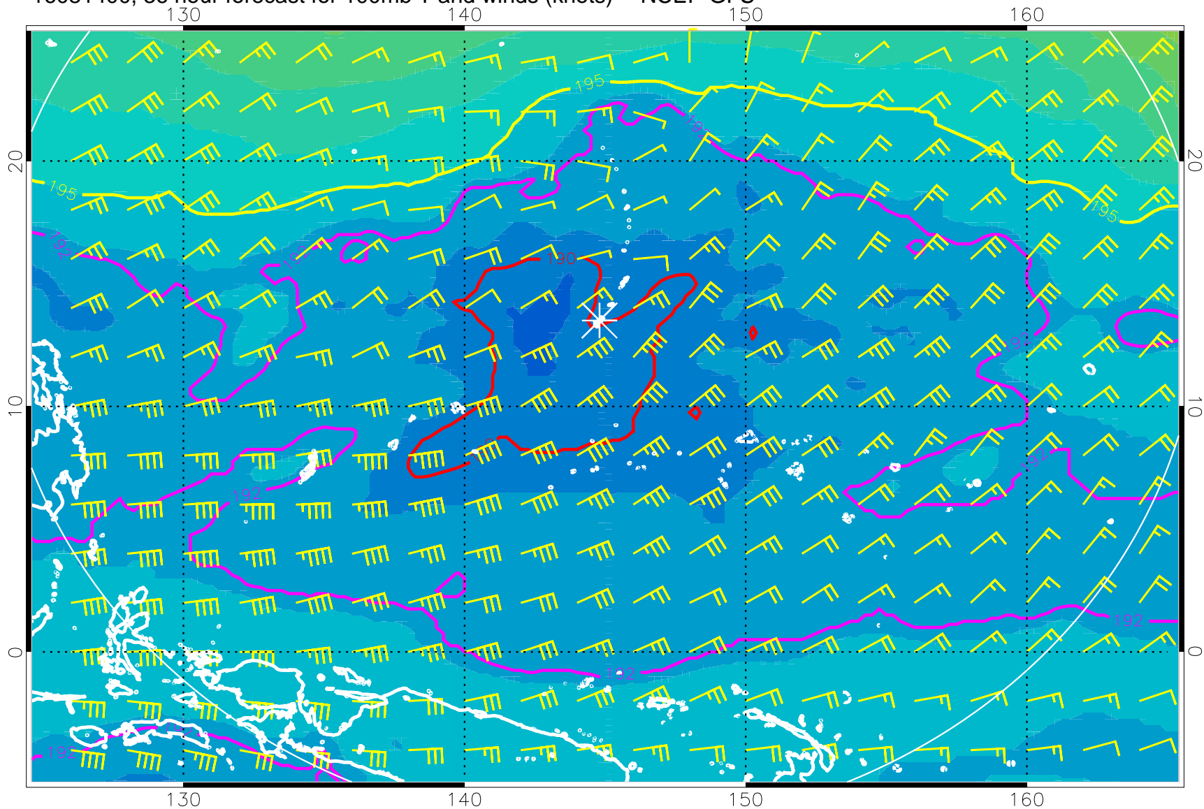
16081400, 36 hour forecast for 100mb T and winds (knots) -- NCEP GFS
