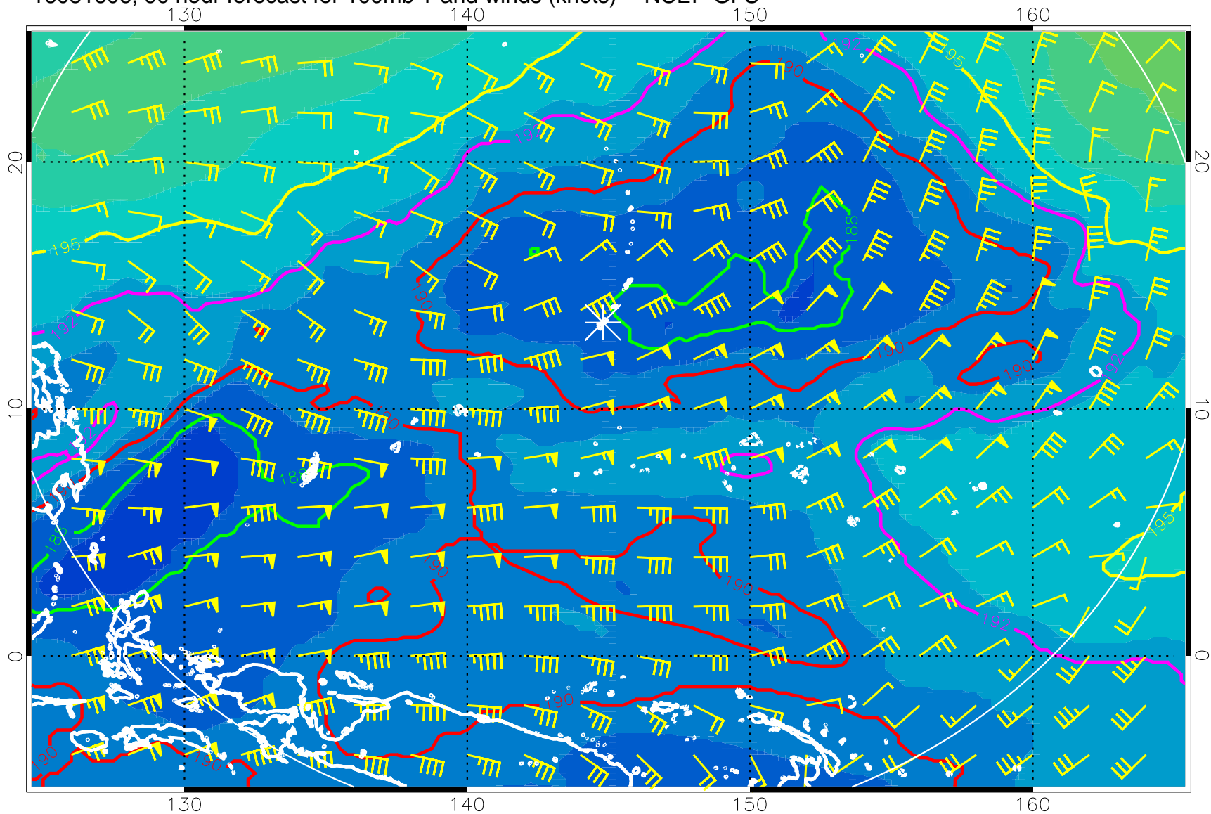
16081606, 90 hour forecast for 100mb T and winds (knots) -- NCEP GFS
