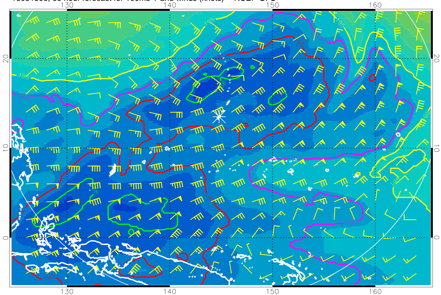
16081506, 66 hour forecast for 100mb T and winds (knots) -- NCEP GFS
