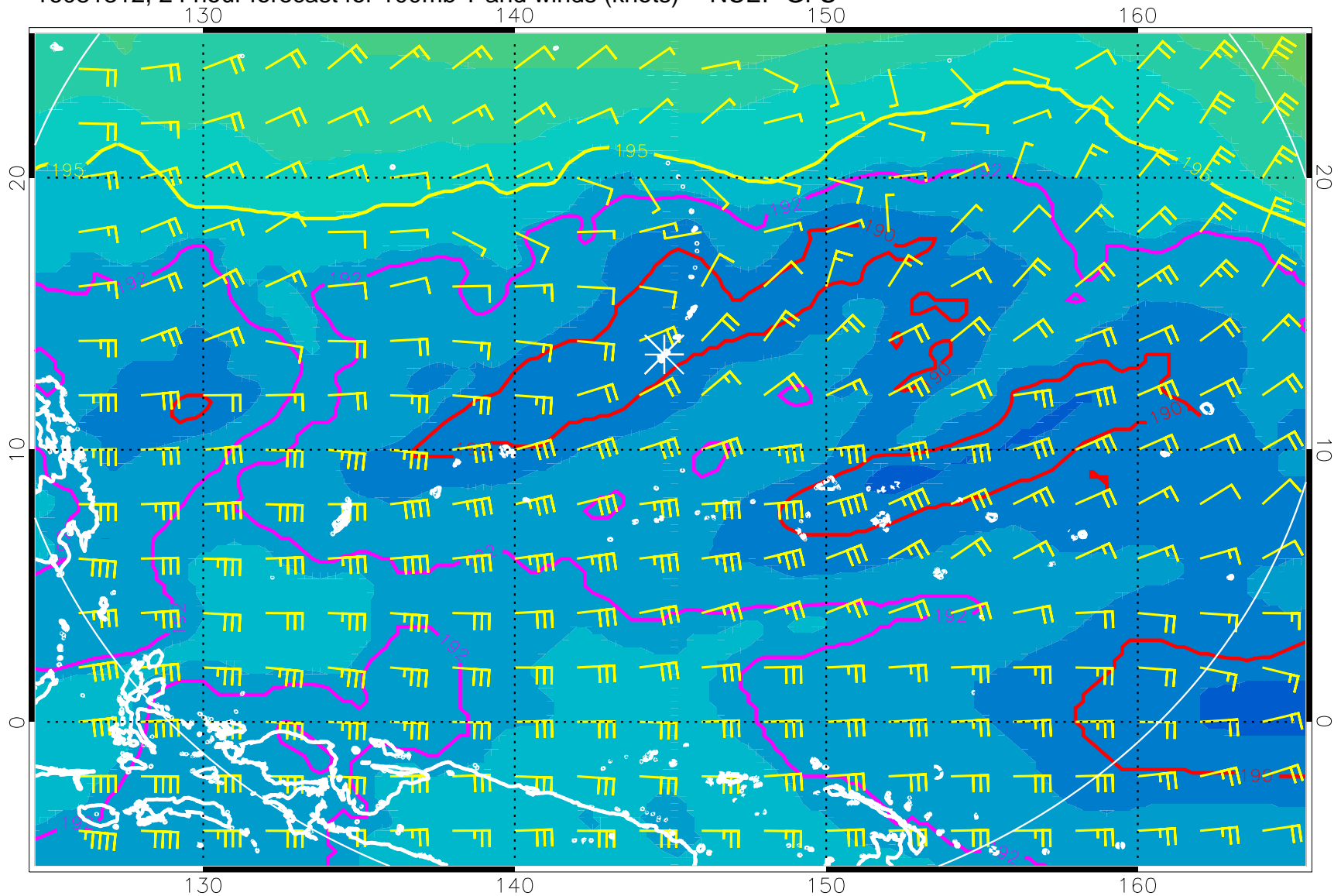
16081312, 24 hour forecast for 100mb T and winds (knots) -- NCEP GFS
