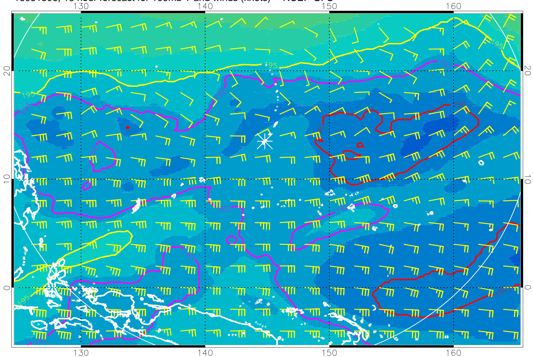
16081306, 18 hour forecast for 100mb T and winds (knots) -- NCEP GFS
