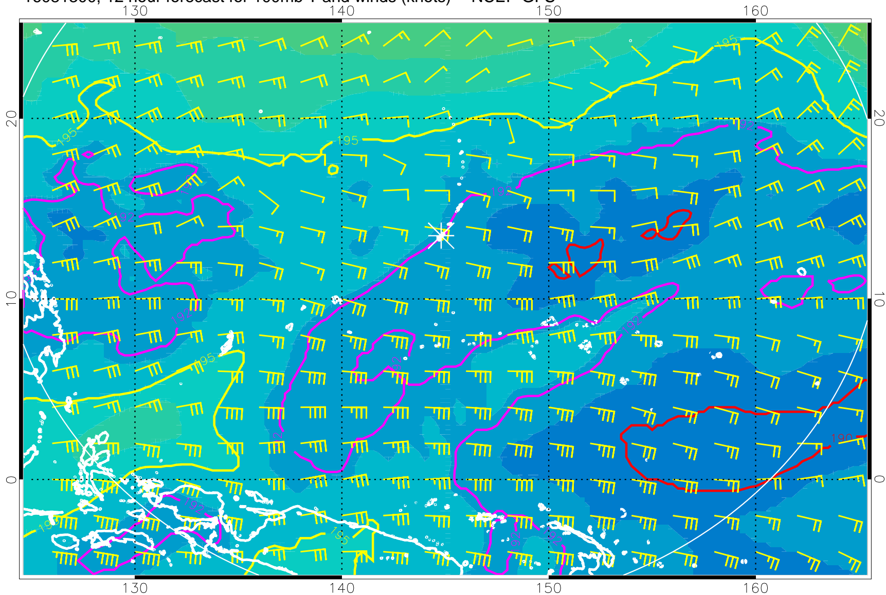
16081300, 12 hour forecast for 100mb T and winds (knots) -- NCEP GFS
