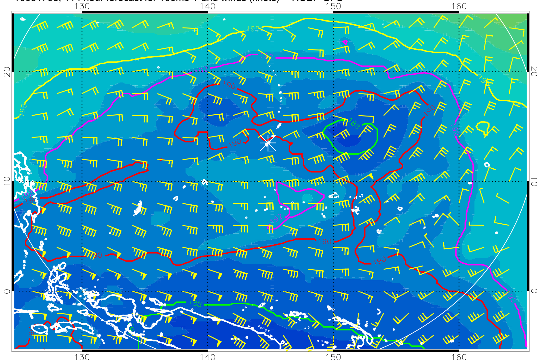
16081706, 114 hour forecast for 100mb T and winds (knots) -- NCEP GFS
